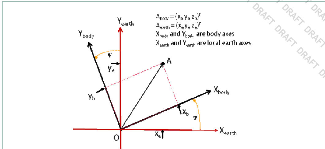
Fig 47. The X-Y plane illustrates rotation from earth into body frame about the Z axis
