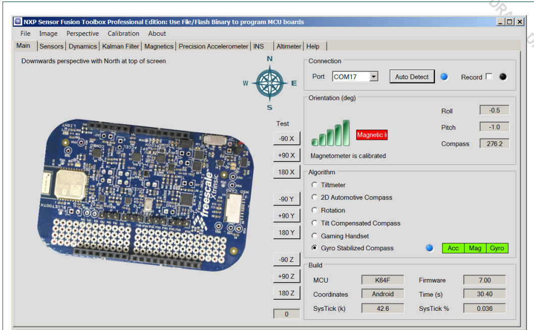
Fig 28. Step function test features in the Sensor Fusion Toolbox for Windows
