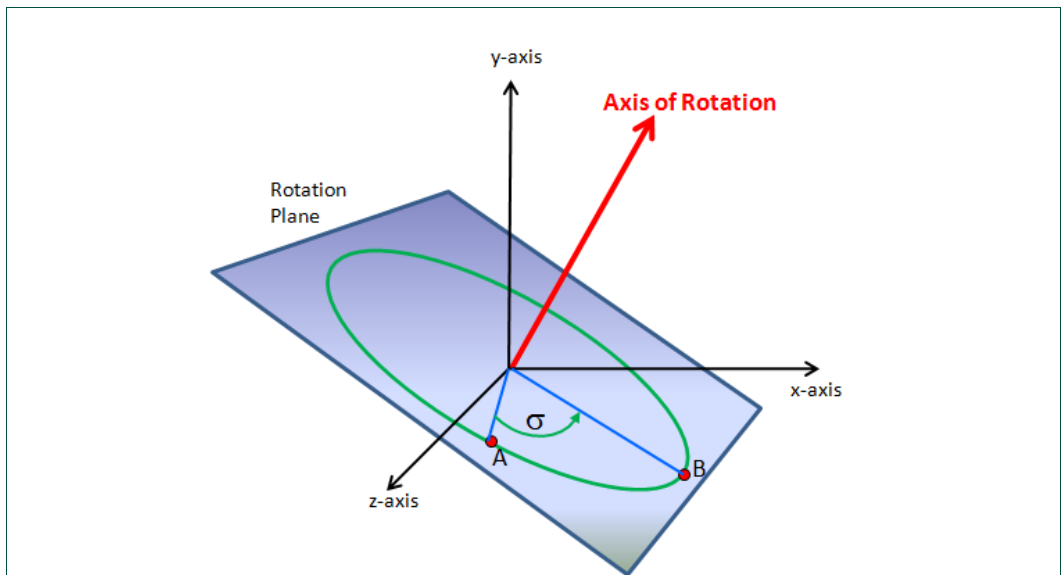
Fig 53. Looking at Just the Rotation Plane and Axis of Rotation
