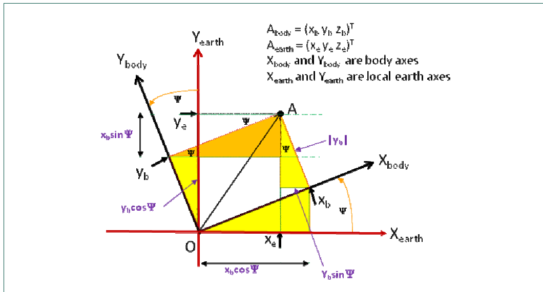
Fig 48. Physical justification for terms in the rotation matrix
