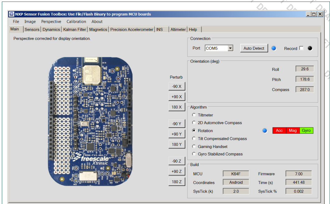
Fig 43. Starting gyroscope orientation test
