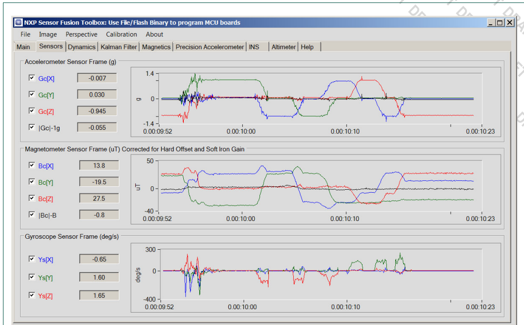
Fig 40. The Sensors tab in the Sensor Fusion Toolbox for Windows
