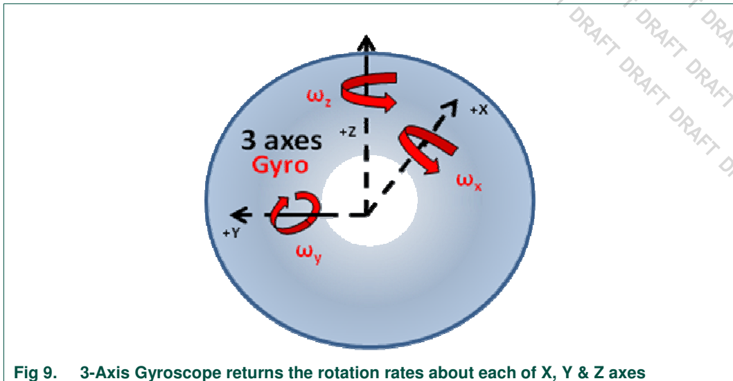
Fig 9. 3-Axis Gyroscope returns the rotation rates about each of X, Y & Z axes
