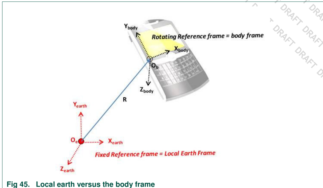
Fig 45. Local earth versus the body frame
