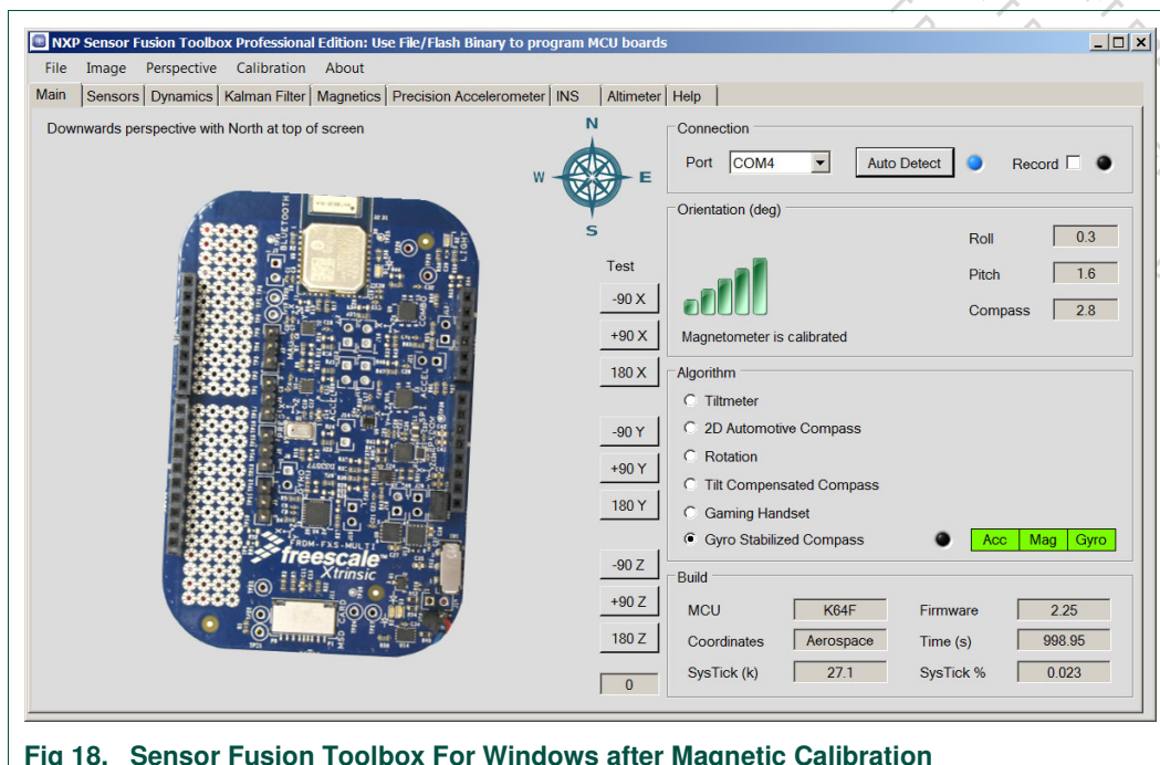
Fig 18. Sensor Fusion Toolbox For Windows after Magnetic Calibration
