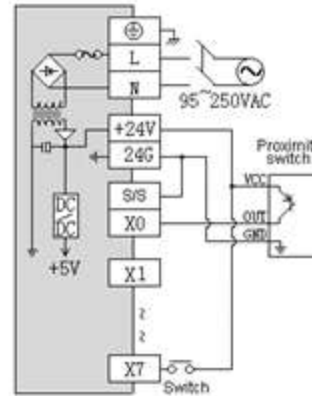
PNP Internal power
