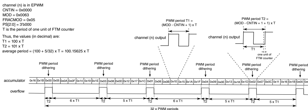
Figure 45-118. Example of Average Period when the PWM Period Dithering is used with the Up Counting
