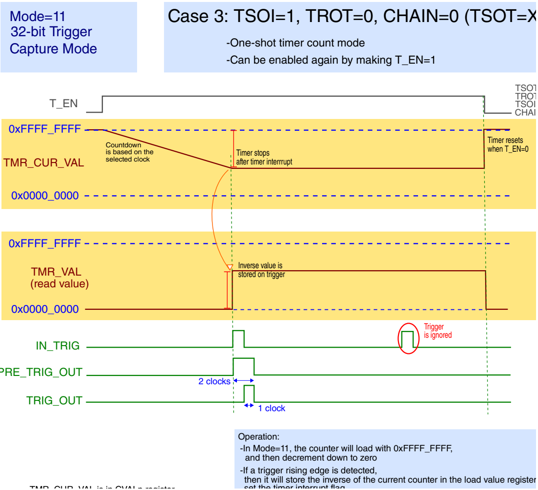
Figure 46-18. Case 3: TSOT = X, TROT = 0, TSOI = 1, CHAIN = 0
