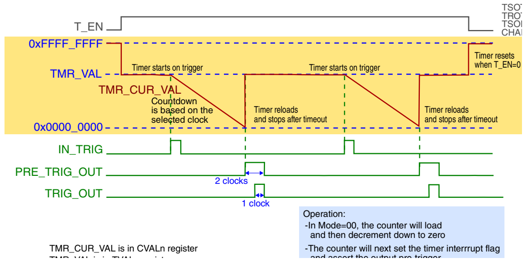
Figure 46-10. Case 6: TSOT = 1, TROT = 0, TSOI = 1, CHAIN = 0
