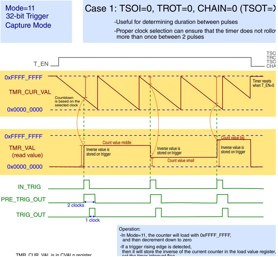
Figure 46-16. Case 1: TSOT = X, TROT = 0, TSOI = 0, CHAIN = 0
