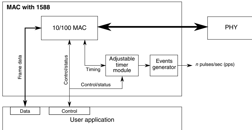
Figure 55-9. IEEE 1588 functions overview
