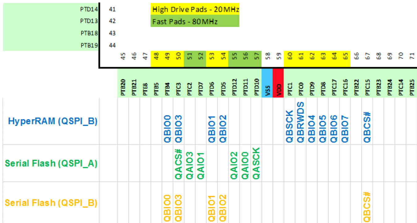
Figure 37-1. External memory options
