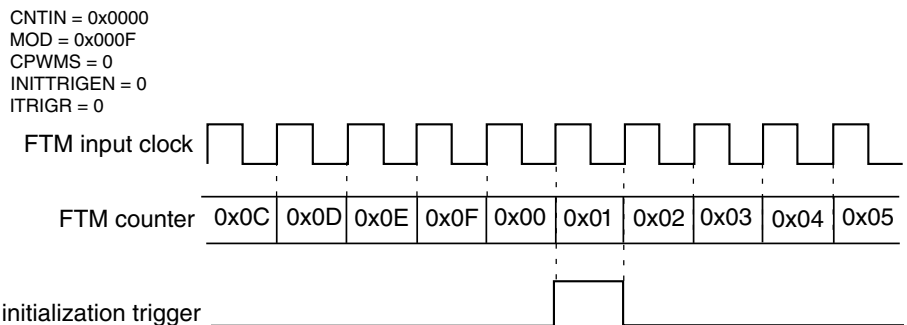
Figure 45-88. Example of the generation of the initialization trigger in the case 1. 2. When there is a write to CNT register.
