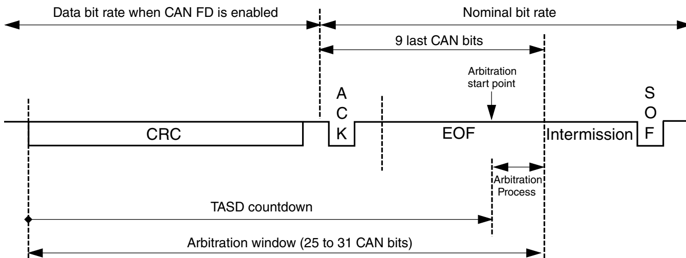
Figure 53-12. Optimal Tx Arbitration start point
