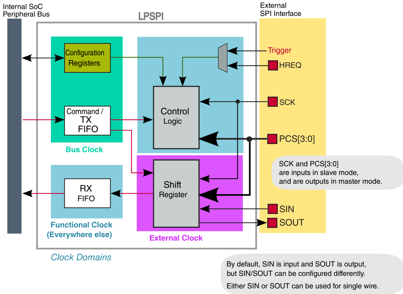
Figure 49-4. Block Diagram
