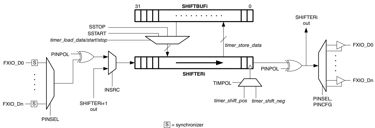
Figure 52-2. Shifter Microarchitecture
