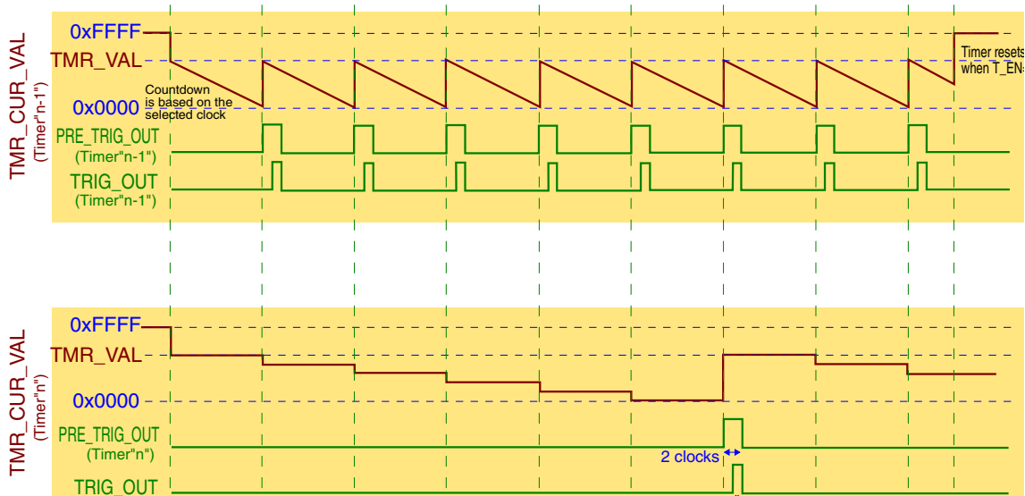
Figure 46-19. Chaining Effects
