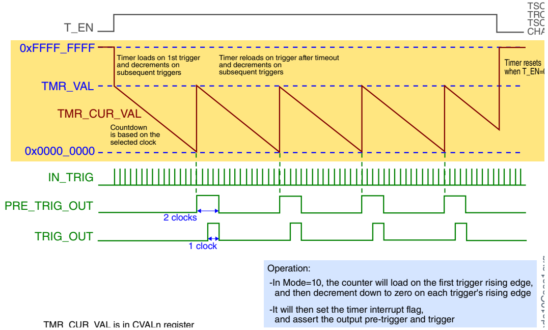
Figure 46-14. Case 1: TSOT = X, TROT = X, TSOI = 0, CHAIN = 0
