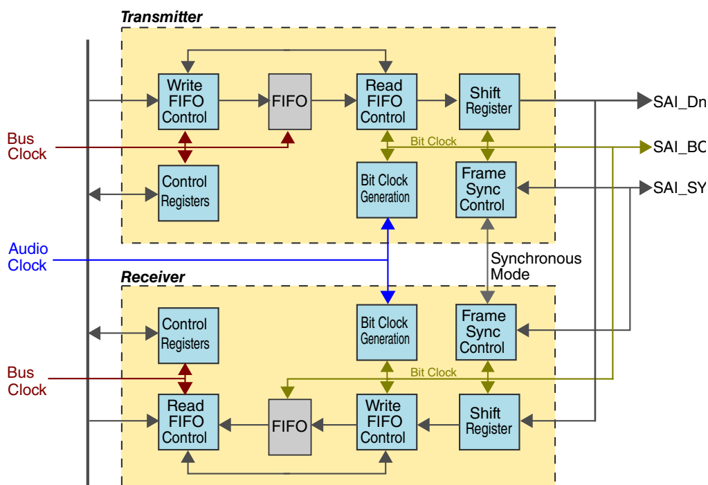
Figure 54-1. S32K148 SAI Block Diagram
