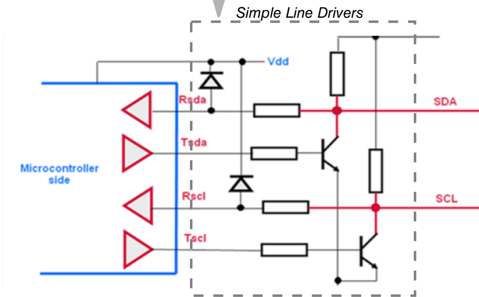
Figure 50-6. 4-Wire scheme
