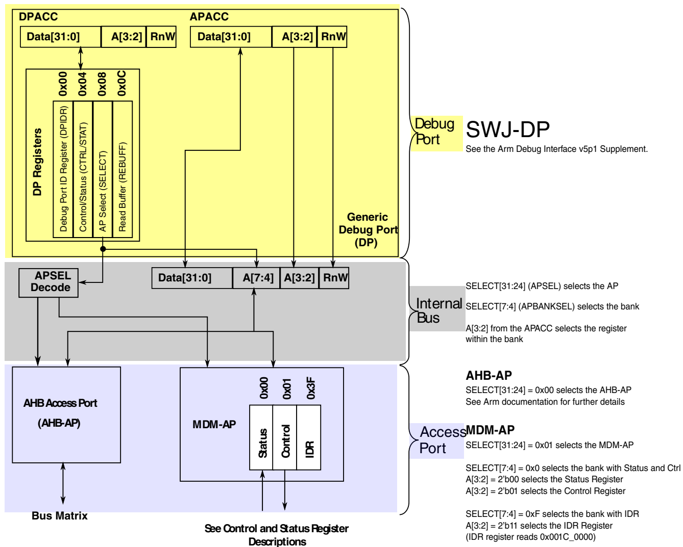
Figure 56-5. MDM AP addressing
