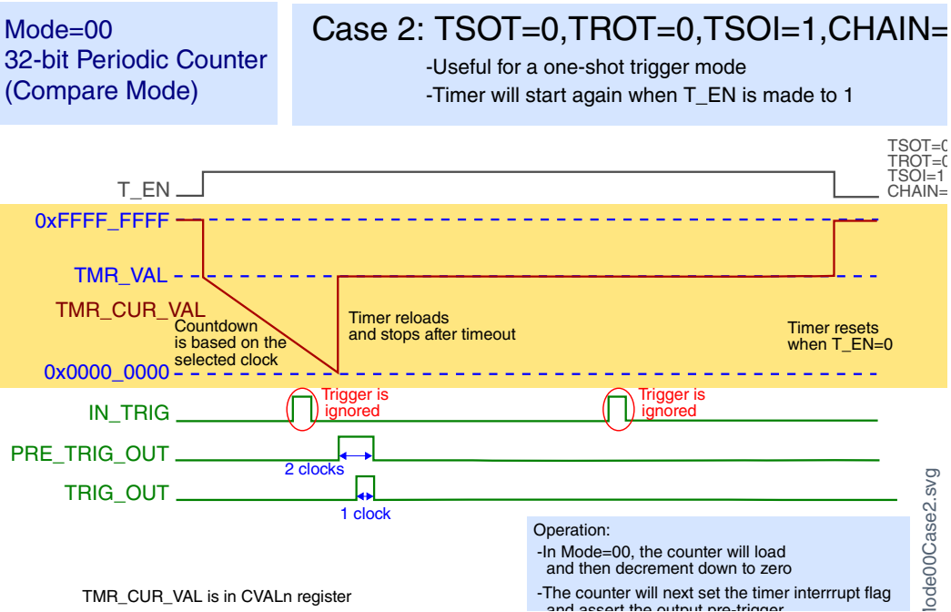
Figure 46-6. Case 2: TSOT = 0, TROT = 0, TSOI = 1, CHAIN = 0
