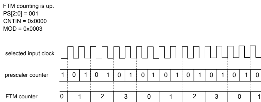
Figure 45-7. Example of the prescaler counter
