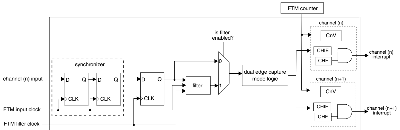
Figure 45-95. Diagram for Dual Edge Capture Mode when FLTPS[3:0] ≠ 0
