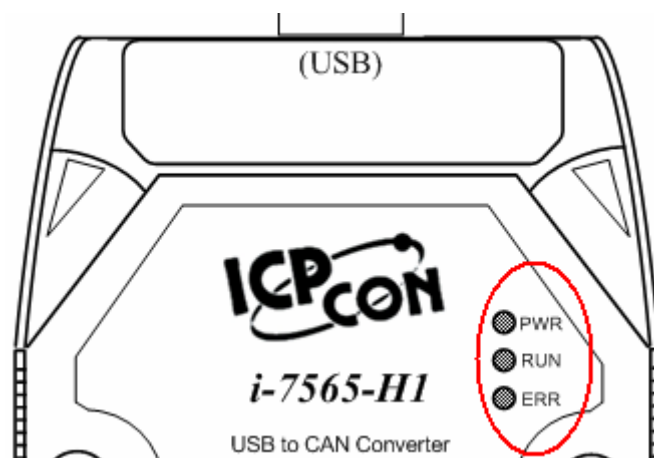
Figure 4-1: LED position of I-7565-H1/H2
