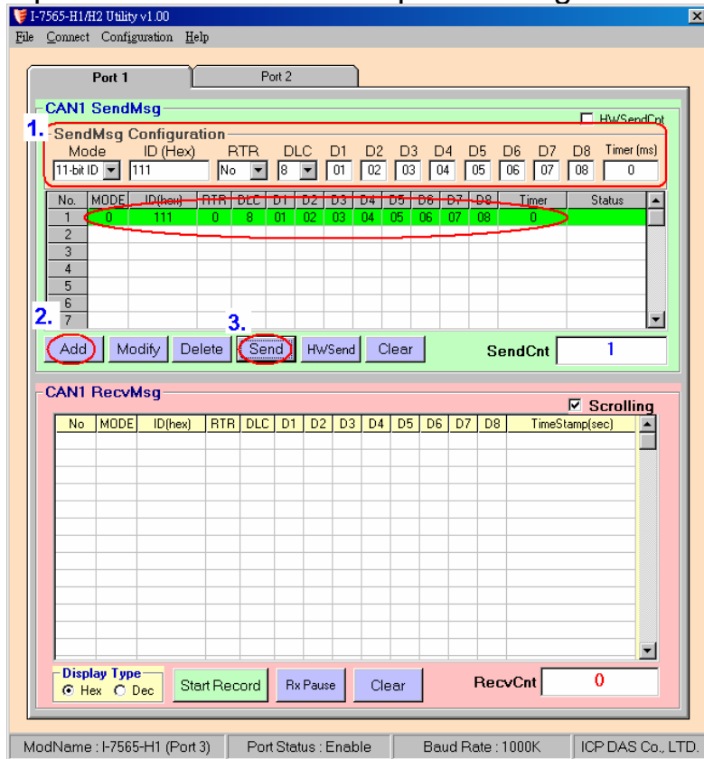
Figure 3-4: Utility of I-7565-H1 A
