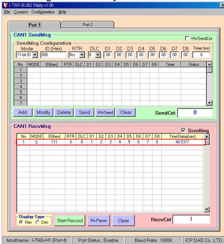
Figure 3-5: Utility of I-7565-H1 B
