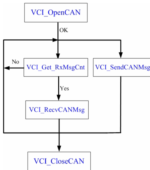
Figure 5-1: Flow Chart of API Library
