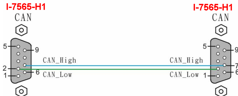
Figure 2-2: CAN bus Connection
