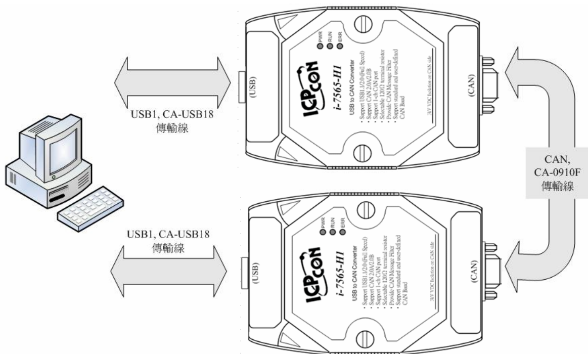
Figure 1-1: Architecture of Example
