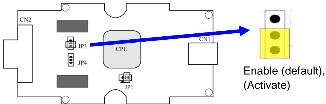
Figure 2-1: JP3 Jumper Position
