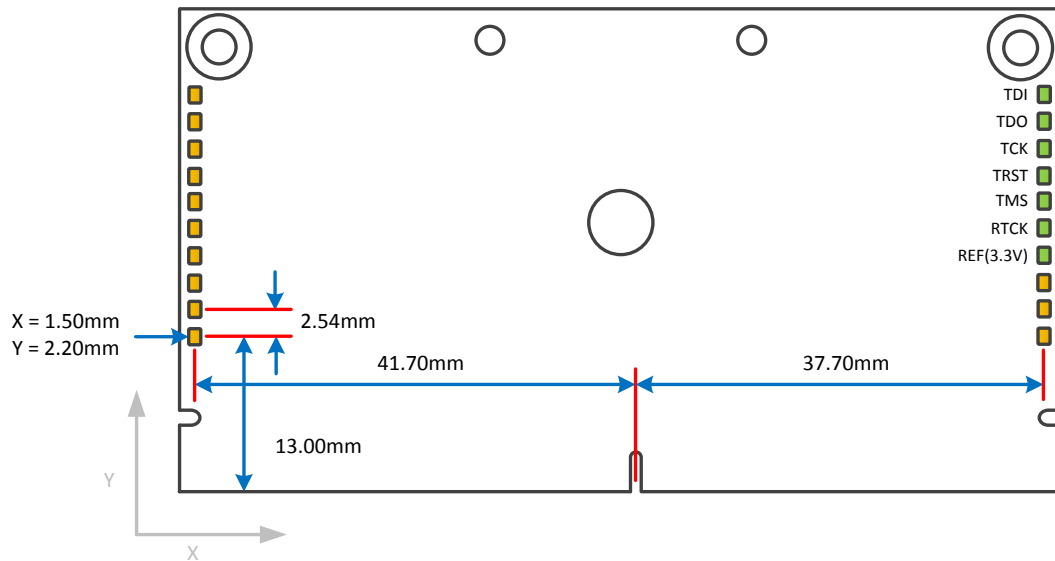
Figure 14 JTAG test point location on bottom side of module
