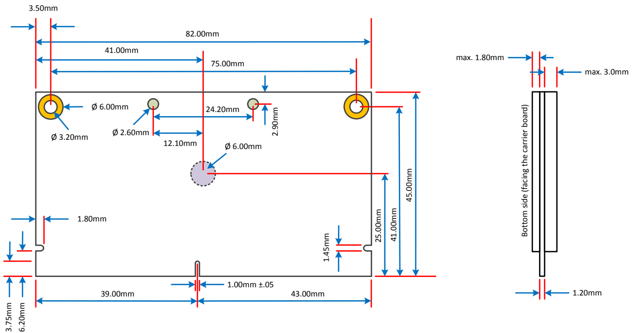
Figure 16 Mechanical dimensions of the Apalis module (top view) Tolerance for all measures: +/- 0.1mm
