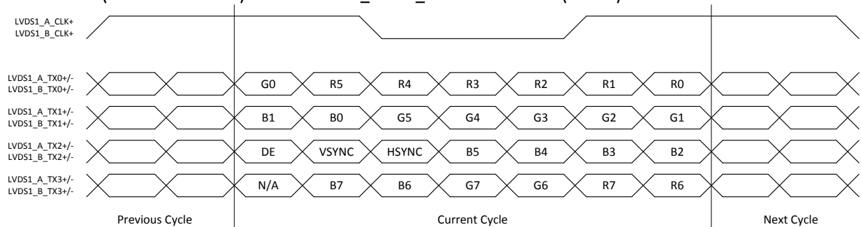
Figure 7: Common 24 bit VESA Colour Mapping (bit_mapping_ch = 0, data_width_ch = 1)
