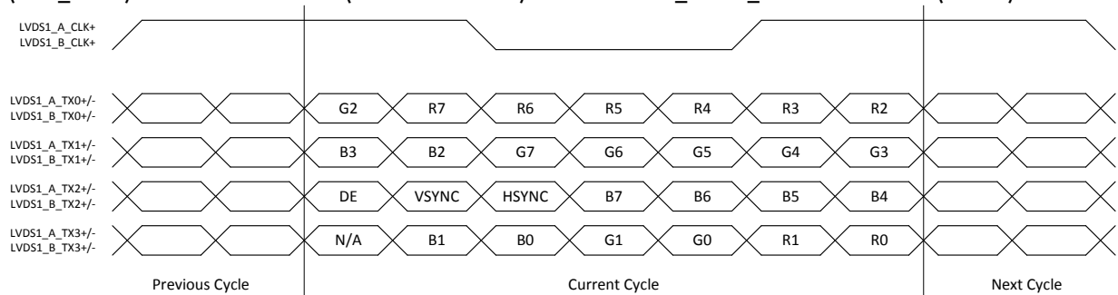
Figure 6: 24 bit / 18 bit Compatible Colour Mapping (bit_mapping_ch = 1, data_width_ch = 1)
