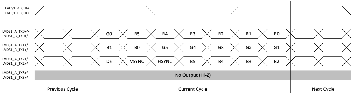
Figure 8: 18 bit Mode (bit_mapping_ch = 0, data_width_ch = 0)
