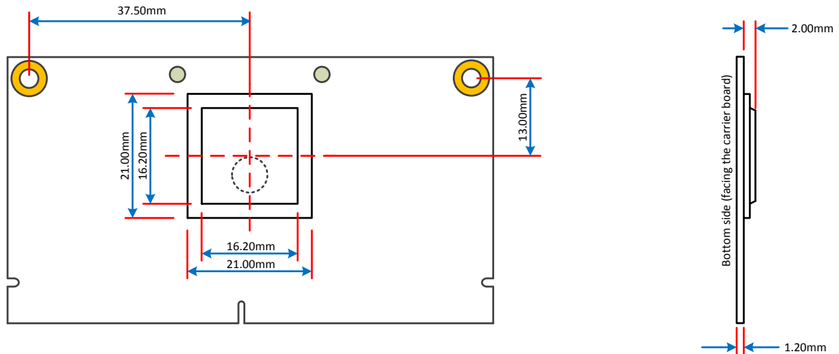
Figure 18 Mechanical position of Freescale i.MX 6 industrial temperature version (top view) Tolerance for all measures: +/- 0.1mm
