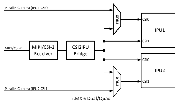
Figure 13: Camera Interface input connectivity
