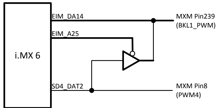
Figure 11: Backlight PWM output circuit
