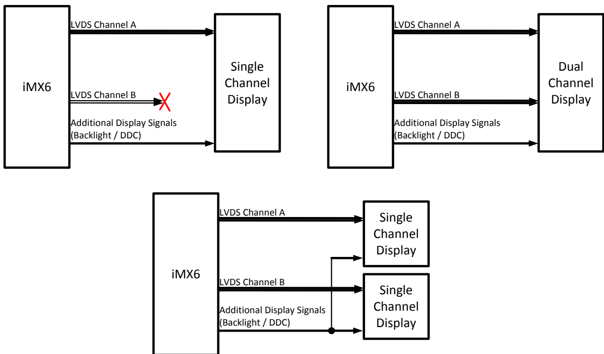
Figure 9: Available LVDS Display configurations
