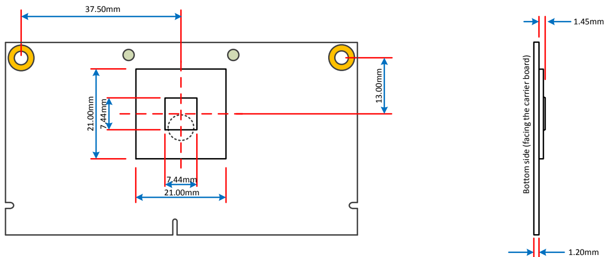
Figure 17 Mechanical position of Freescale i.MX 6 commercial temperature version (top view) Tolerance for all measures: +/- 0.1mm
