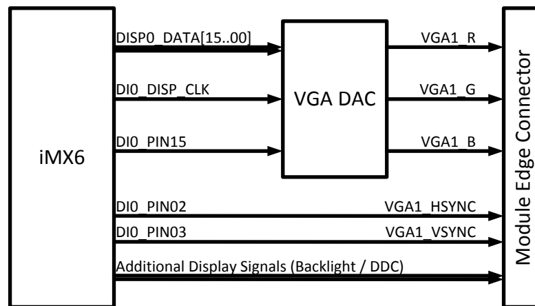
Figure 10: VGA Block Diagram
