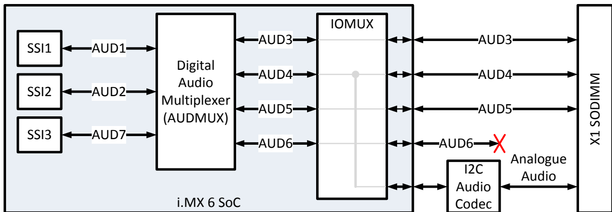
Figure 12 Audio Multiplexing
