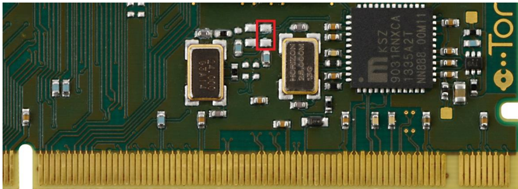
Figure 15 Location of recovery mode pads
