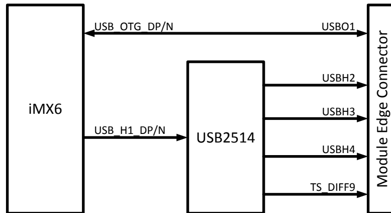
Figure 5: USB Block Diagram
