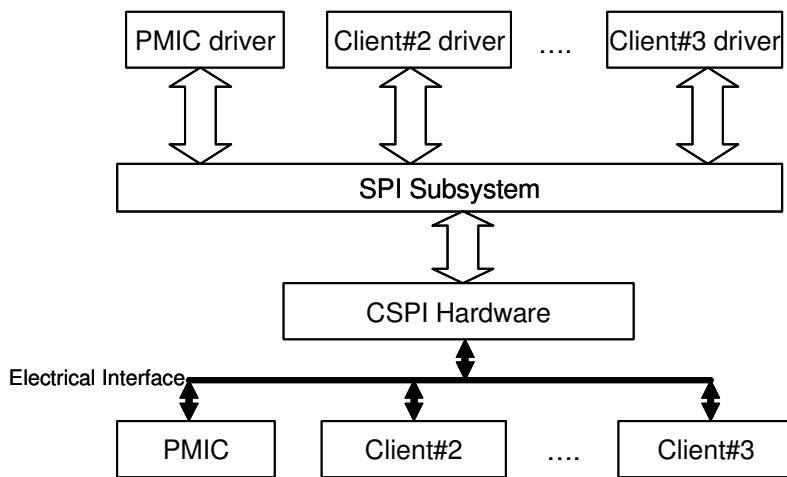
Figure 27-1. SPI Subsystem
