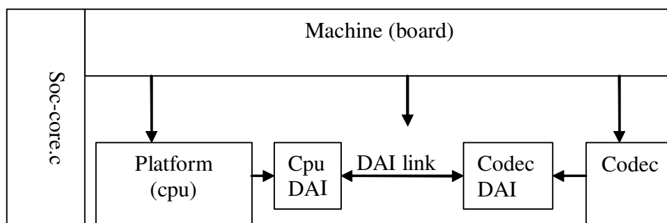
Figure 21-1. ALSA SoC Software Architecture
