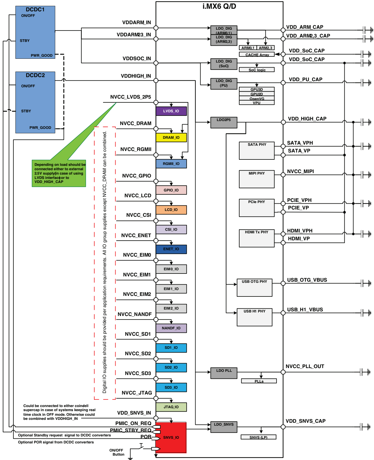
Figure 10-12. Supplying i.MX 6Dual/6Quad power using integrated PMU
