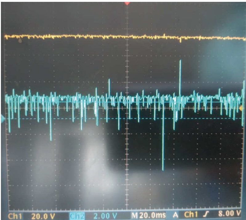
50W输出电压和TL431 REF波形
