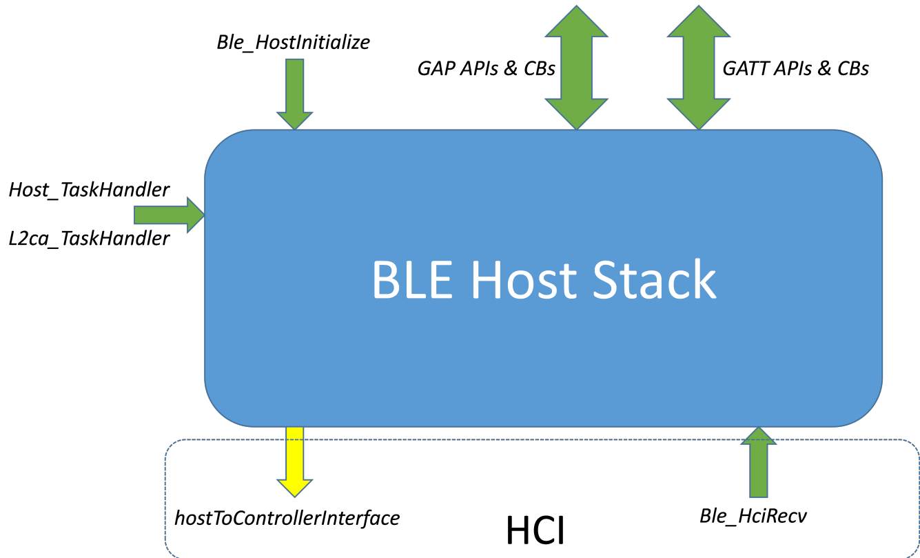
Figure 1. BLE Host Stack overview
