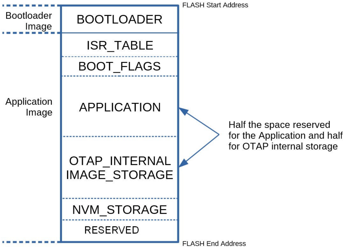
Figure 22. Device Memory Layout – Internal Image Storage
