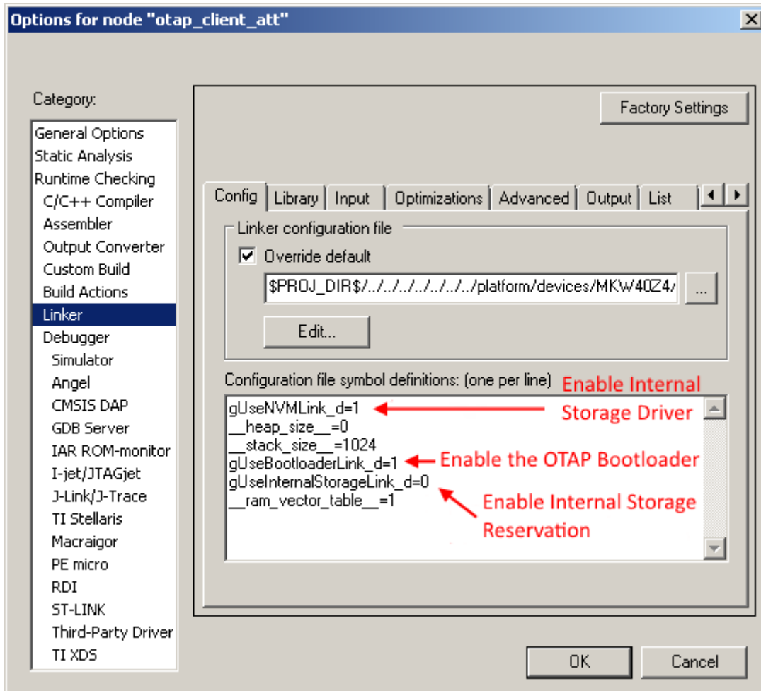
Figure 17. Linker Config IAR EW IDE - OTAP Client External Storage and Bootloader Configuration
