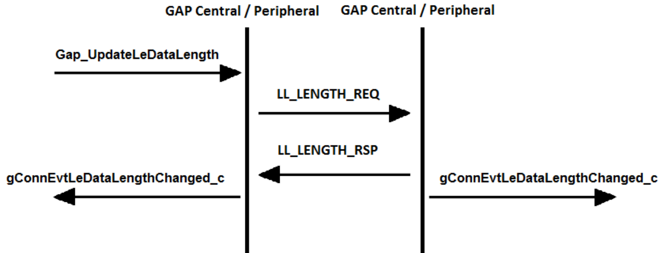
Figure 5. Data Length Update Procedure
