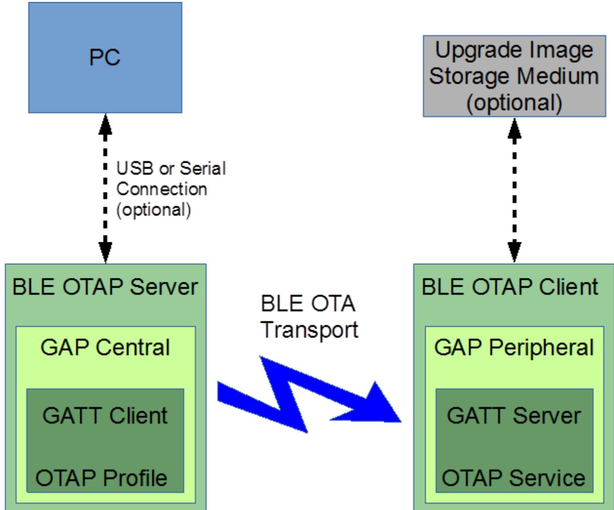
Figure 12. Typical BLE OTAP Image Upgrade Scenario
