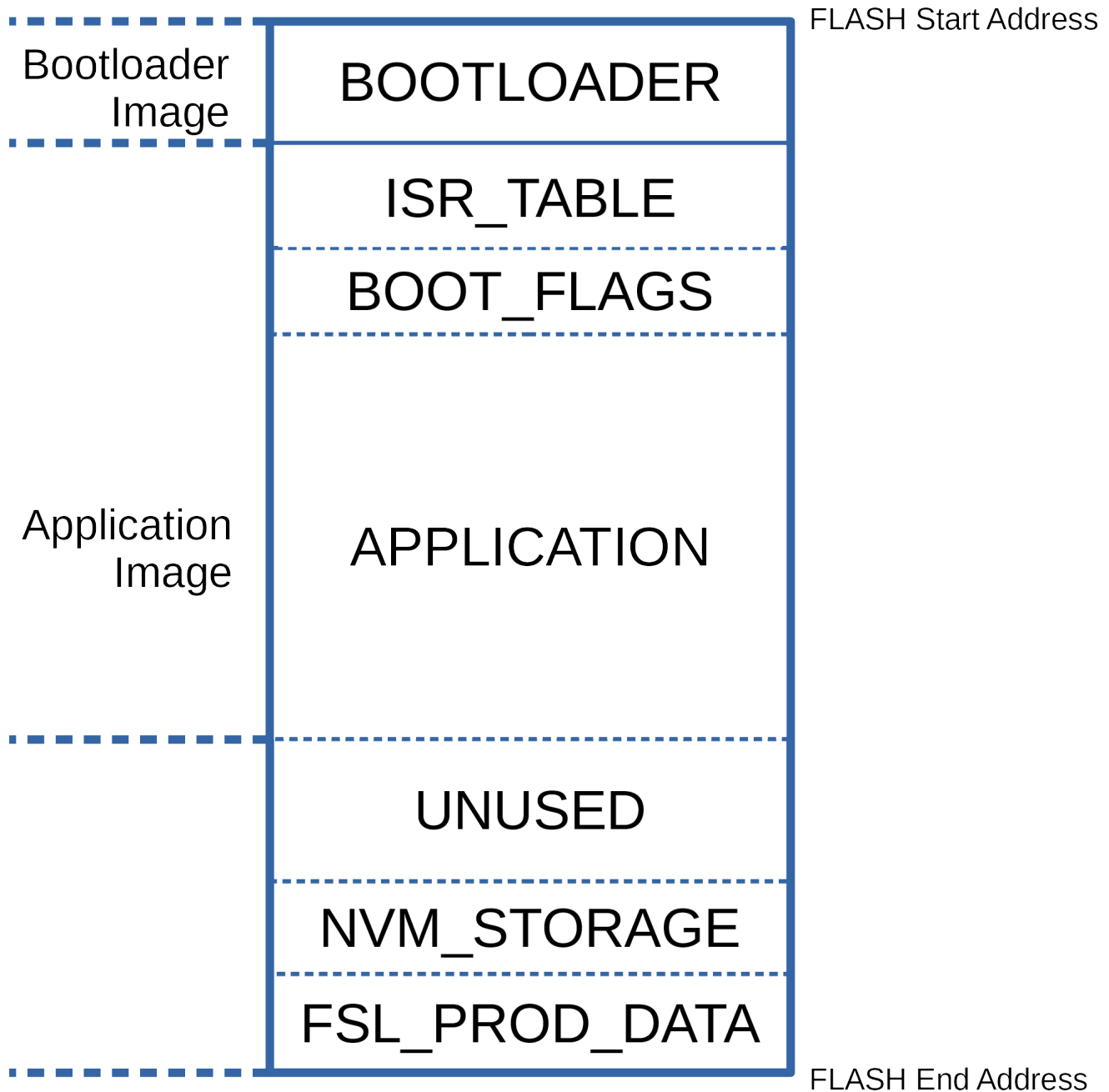
Figure 21. Device Memory Layout – External Image Storage
