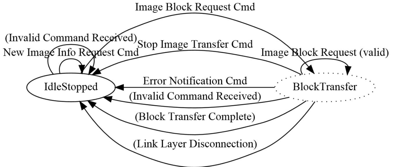
Figure 16. OTAP Server Example State Diagram
