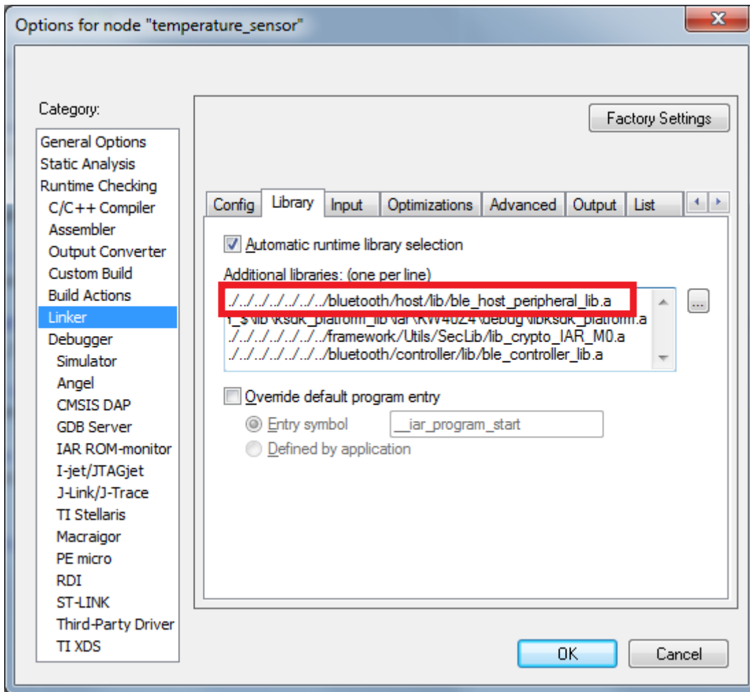
Figure 9. Linker configuration for Temperature Sensor
