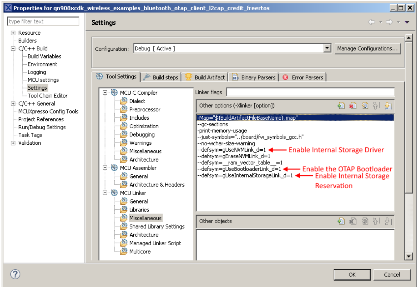
Figure 18. OTAP linker settings - MCUX
