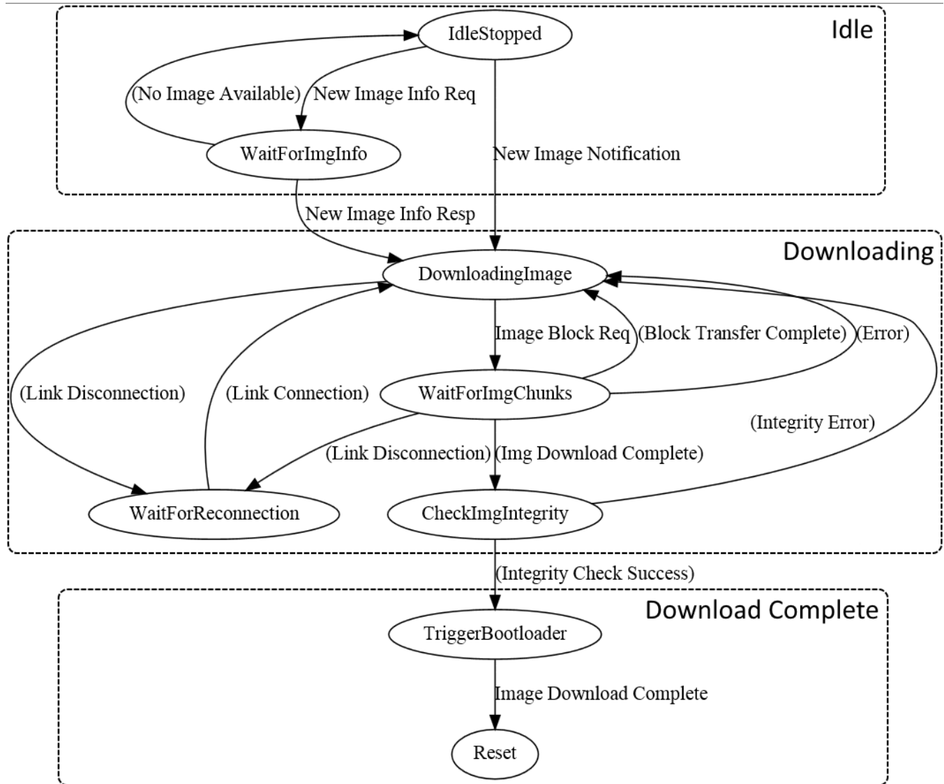
Figure 20. OTAP Client Example State Diagram
