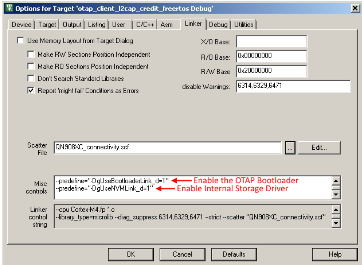
Figure 19. OTAP linker settings - Keil MDK
