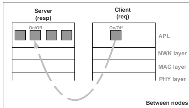
Figure 2-11. On and Off Lighting Application Stack Behavior
