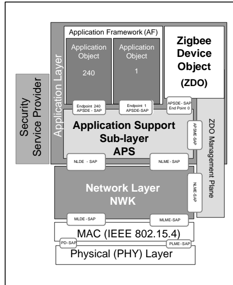
Figure 2-1. ZigBee Layers
