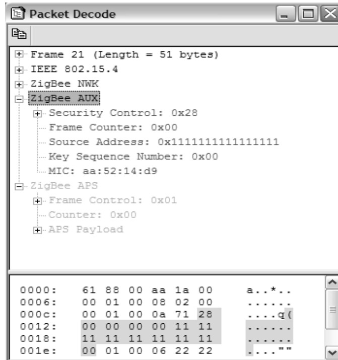
Figure 12-1. Secure ZigBee Packet Example
