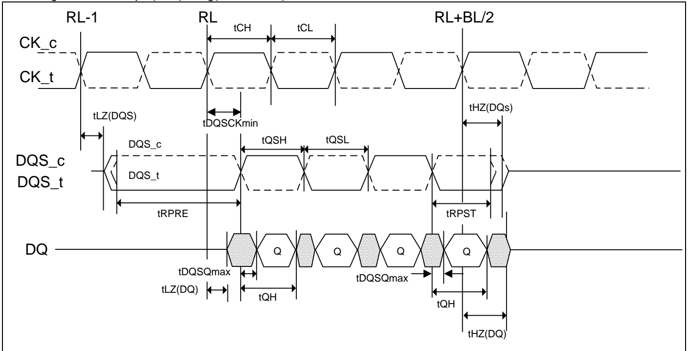
6.4.3.2 Figure of Data output(read)timing( t_{DQSKmin} )
