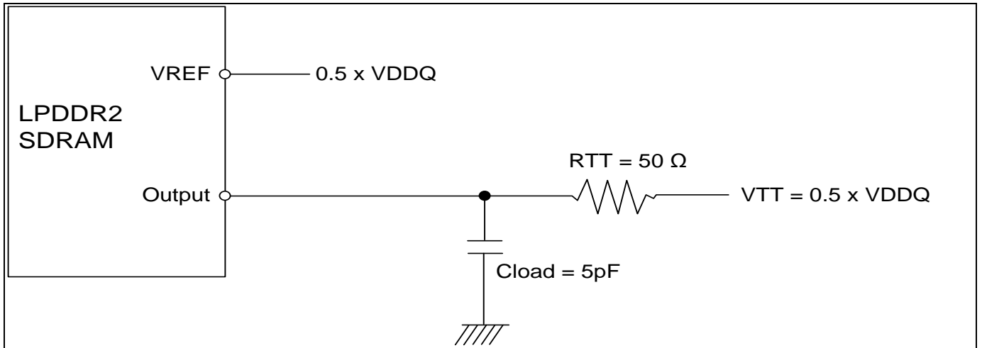
Figure of HSUL_12 Driver Output Reference Load for Timing and Slew Rate
