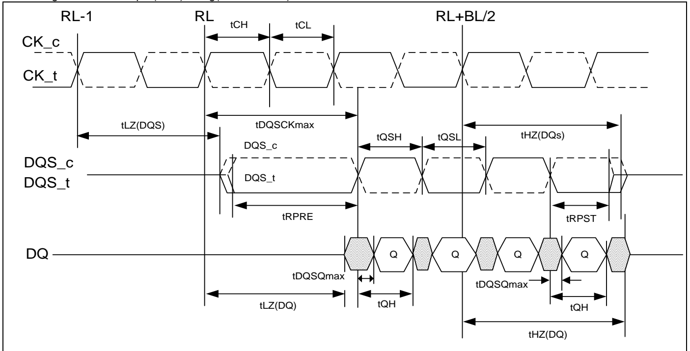
6.4.3.1 Figure of Data output(read)timing(tDQCKmax)
