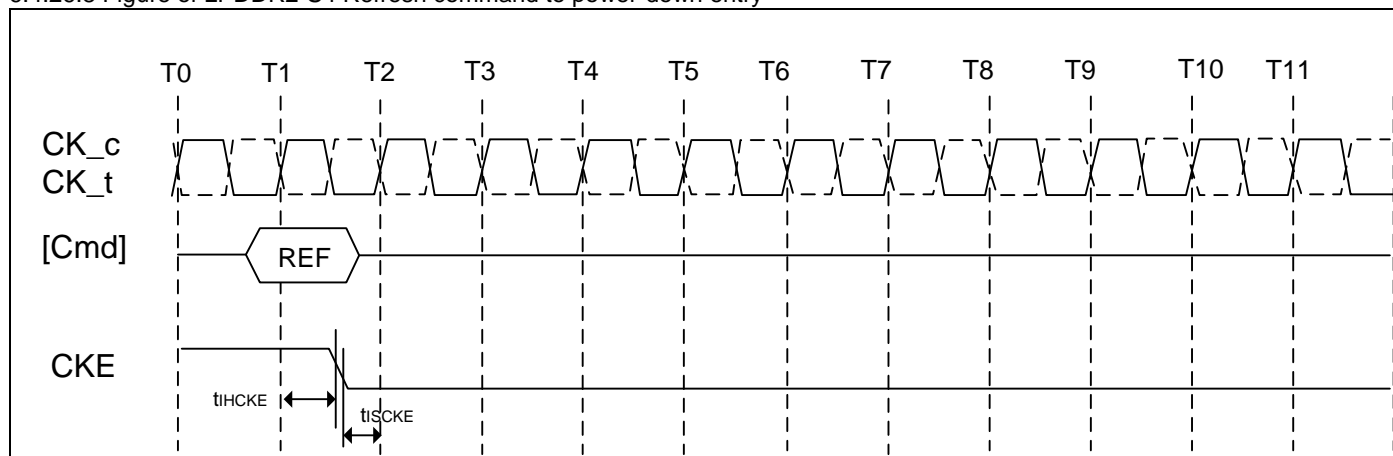
6.4.26.8 Figure of LPDDR2-S4 Refresh command to power-down entry
