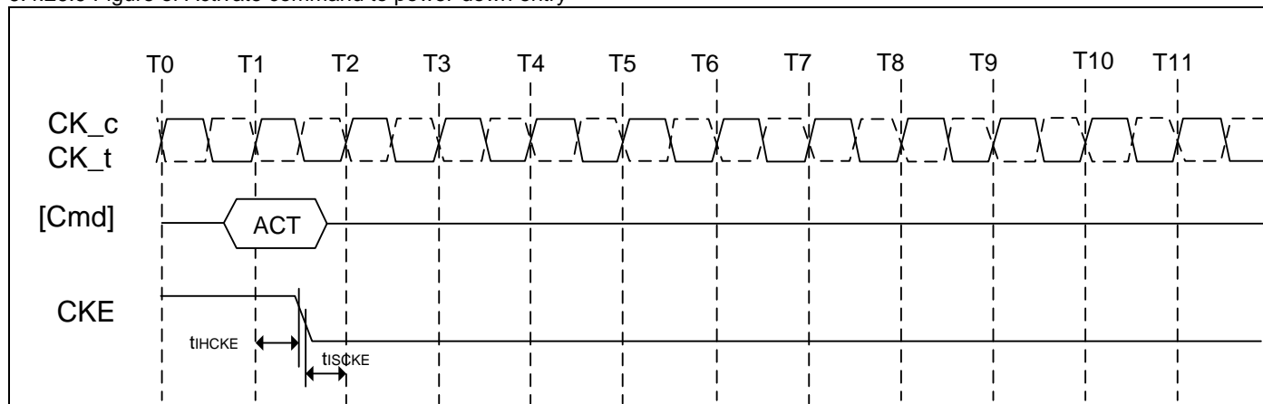
6.4.26.9 Figure of Activate command to power-down entry
