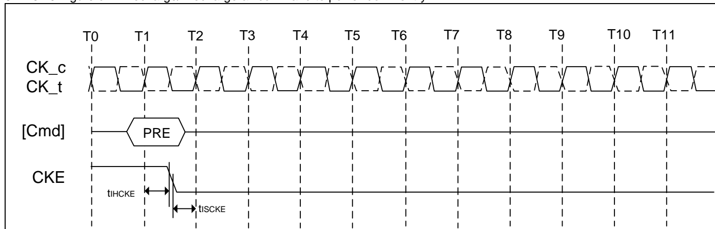
6.4.26.10 Figure of Precharge/Precharge-all command to power-down entry
