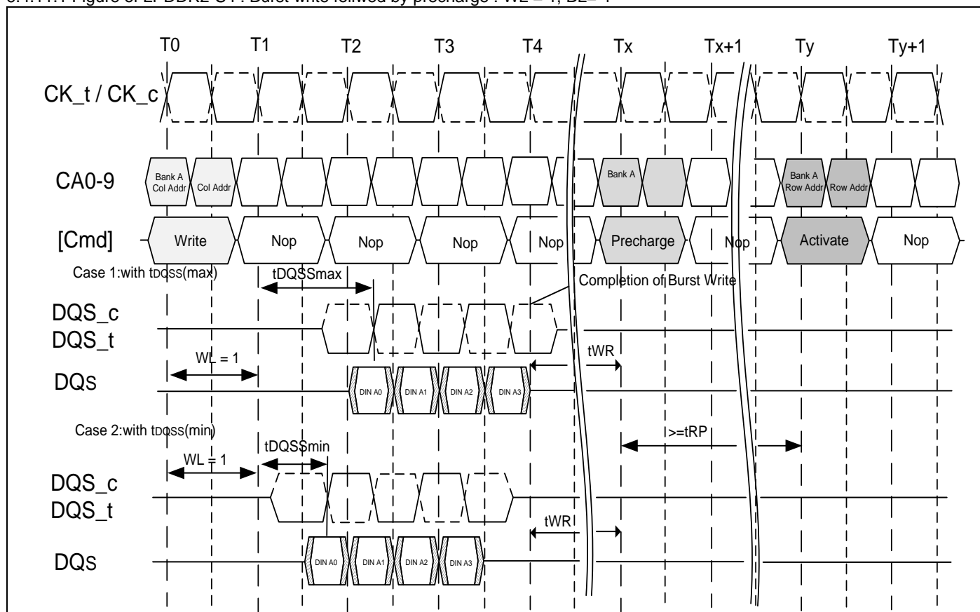
6.4.11.1 Figure of LPDDR2-S4 : Burst write follwed by precharge : WL = 1, BL= 4
