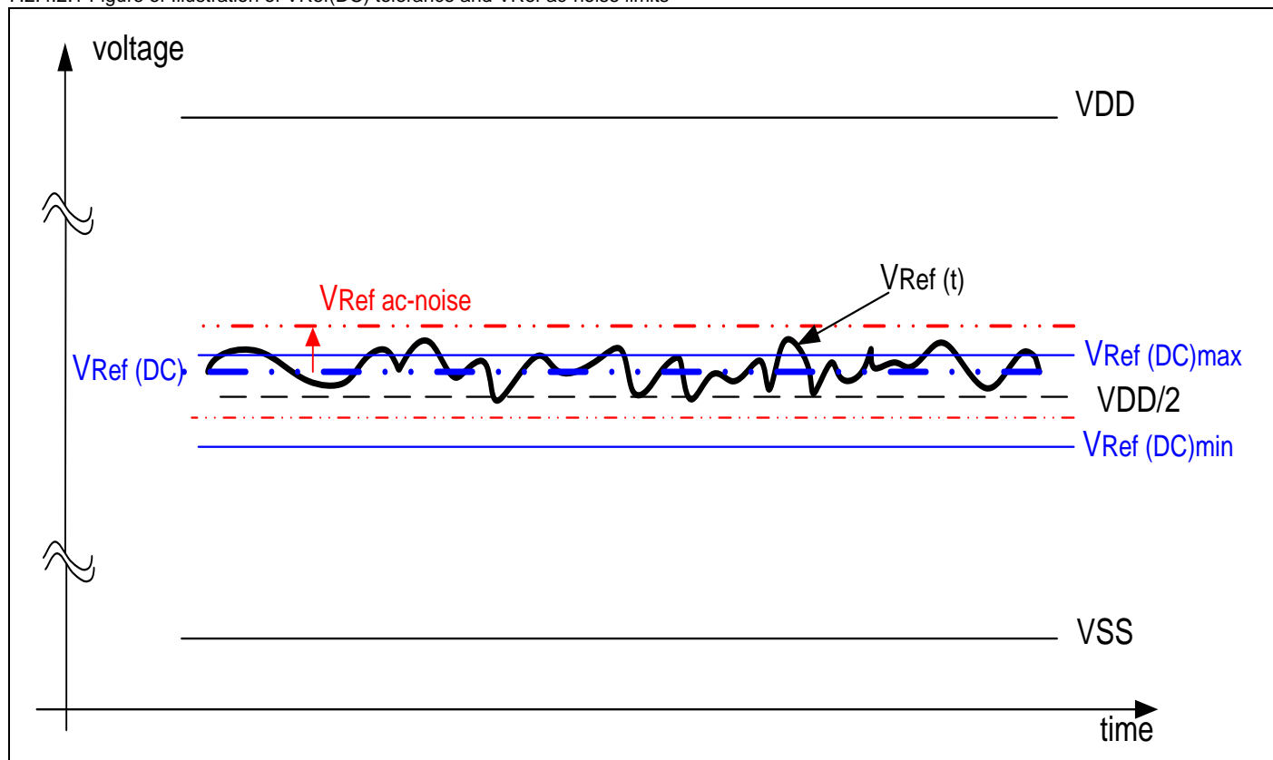
7.2.4.2.1 Figure of Illustration of VRef(DC) tolerance and VRef ac-noise limits
