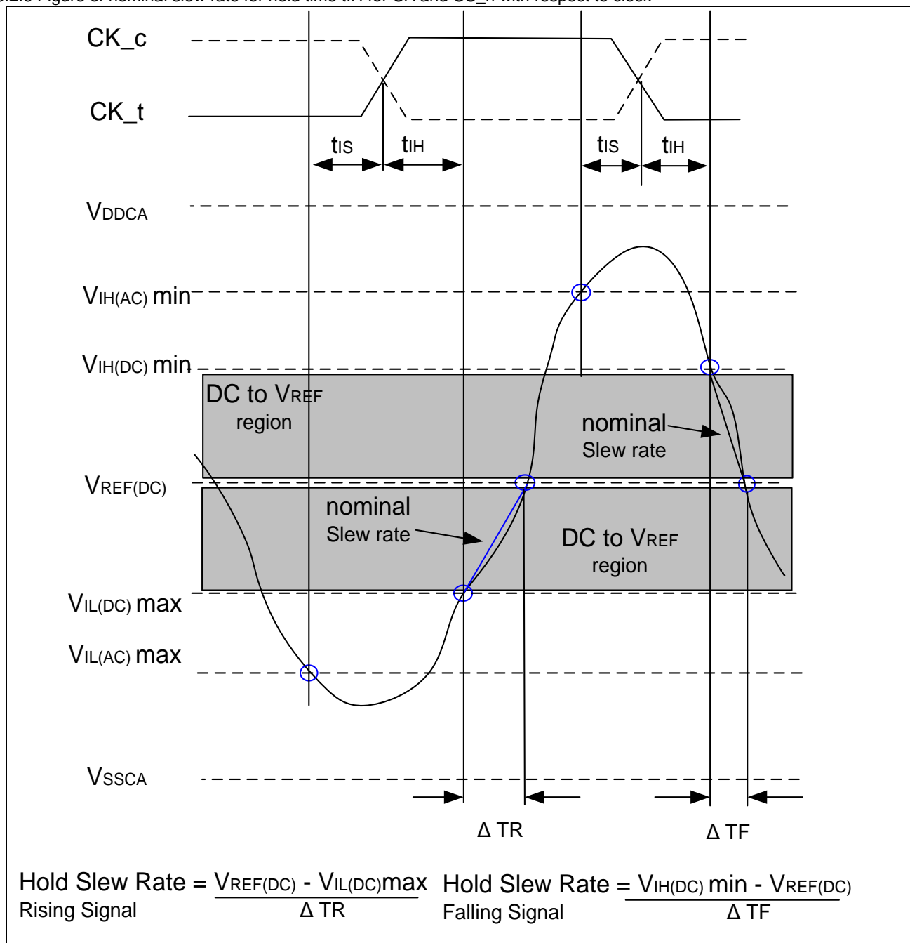
7.6.2.6 Figure of nominal slew rate for hold time t IH for CA and CS n with respect to clock
