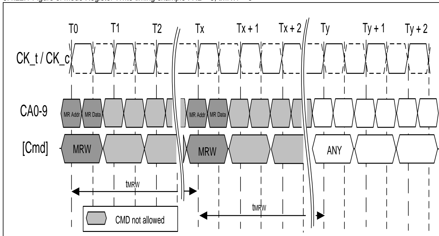
6.4.22.1 Figure of Mode Register Write timing example : RL = 3, tMRW = 5
