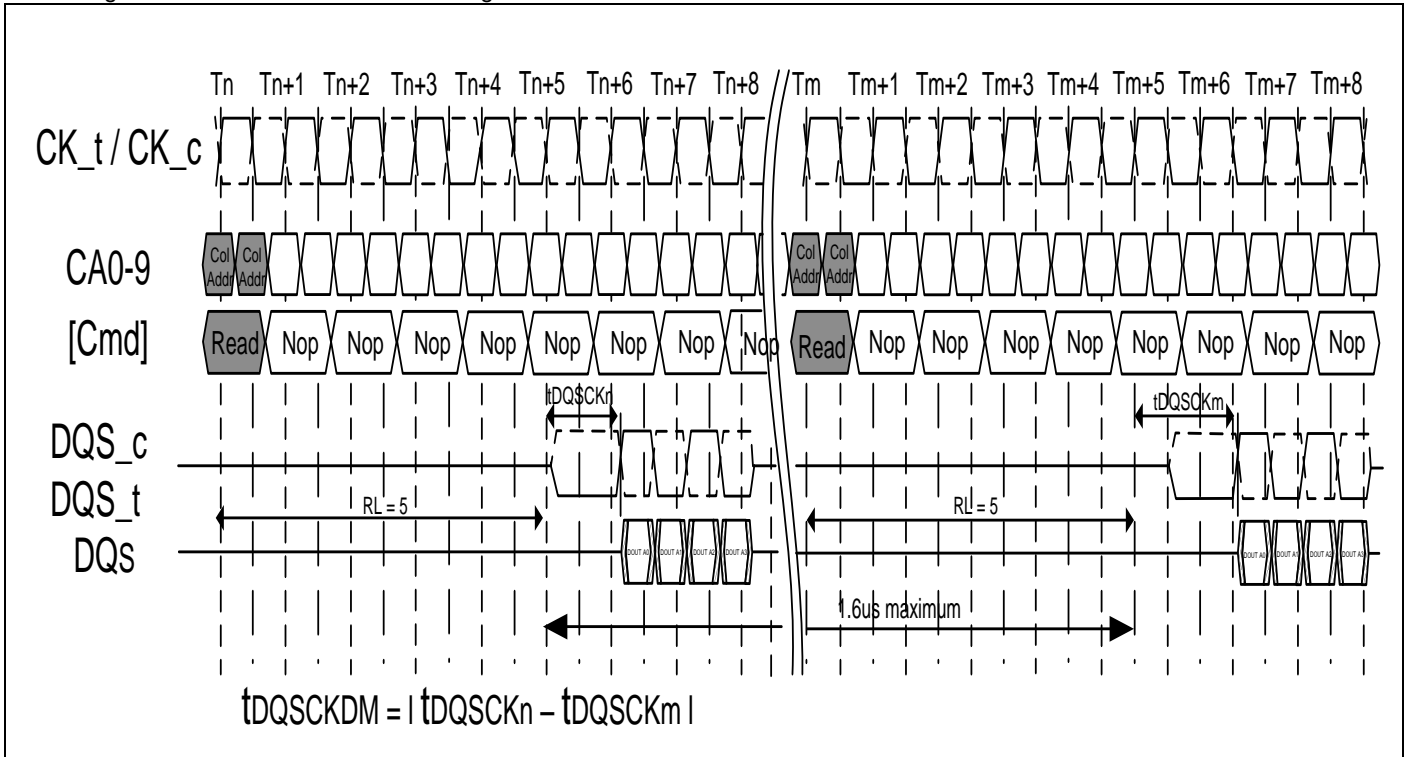
6.4.3.6 Figure of LPDDR2: tDQSKDM timing
