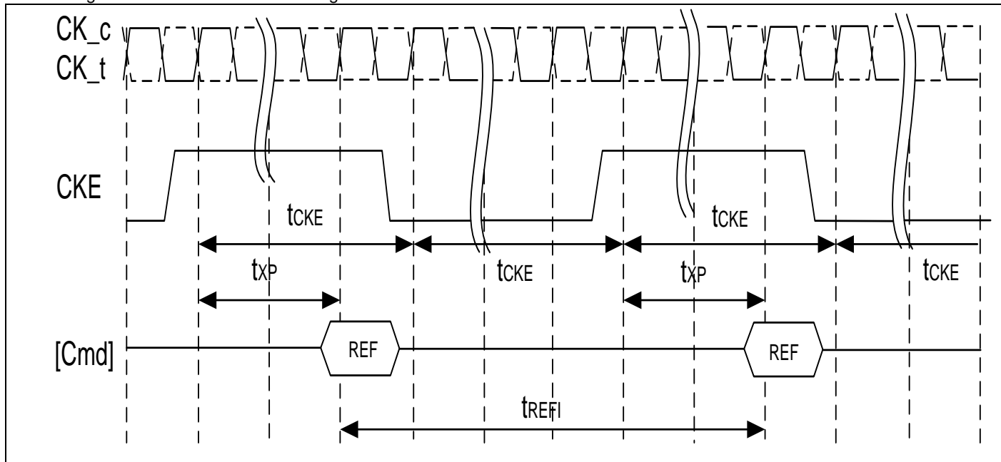
6.4.26.3 Figure of Refresh to Refresh timing with CKE intensive environment for LPDDR2 SDRAM
