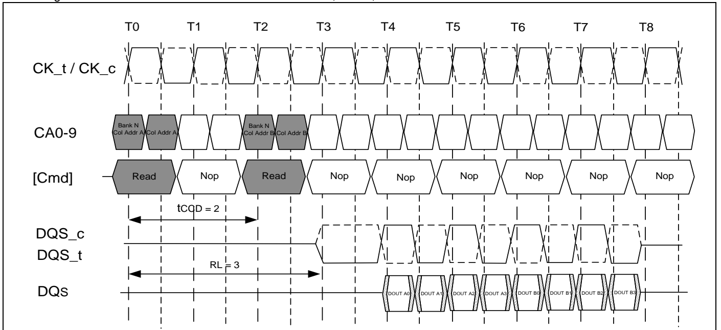
6.4.3.9 Figure of LPDDR2-S4 : Seamless burst read : RL = 3, BL = 4, tCCD=2
