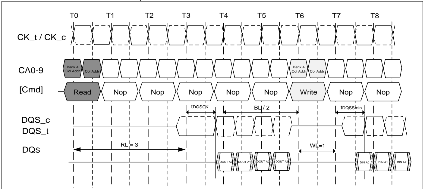
6.4.3.8 LPDDR2-S4 : Burst read followed by burst write: RL = 3, WL = 1, BL = 4
