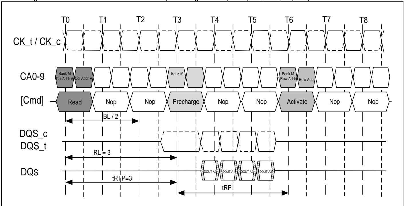
6.4.10.2 Figure of LPDDR2-S4 : Burst read followed by Precharge : RL= 3, BL=4, RU(tRTP(min)/tCK)=3
