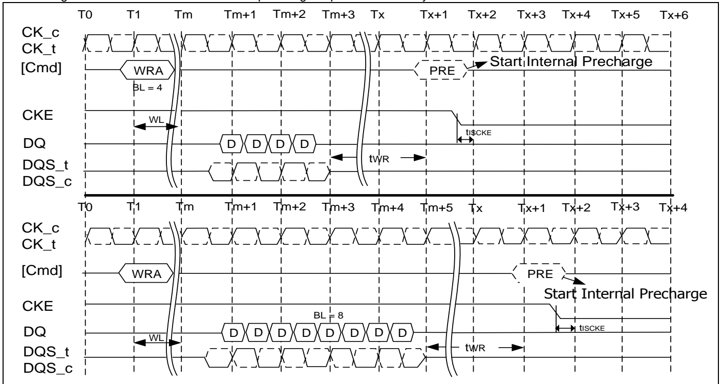
6.4.26.7 Figure of LPDDR2-S4: Write with autorecharge to power-down entry
