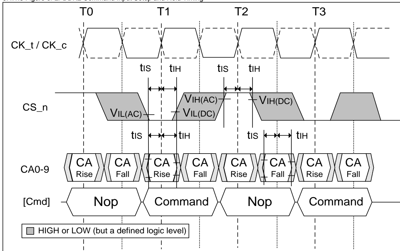
6.4.1.3 Figure of LPDDR2 Command Input Setup and Hold Timing
