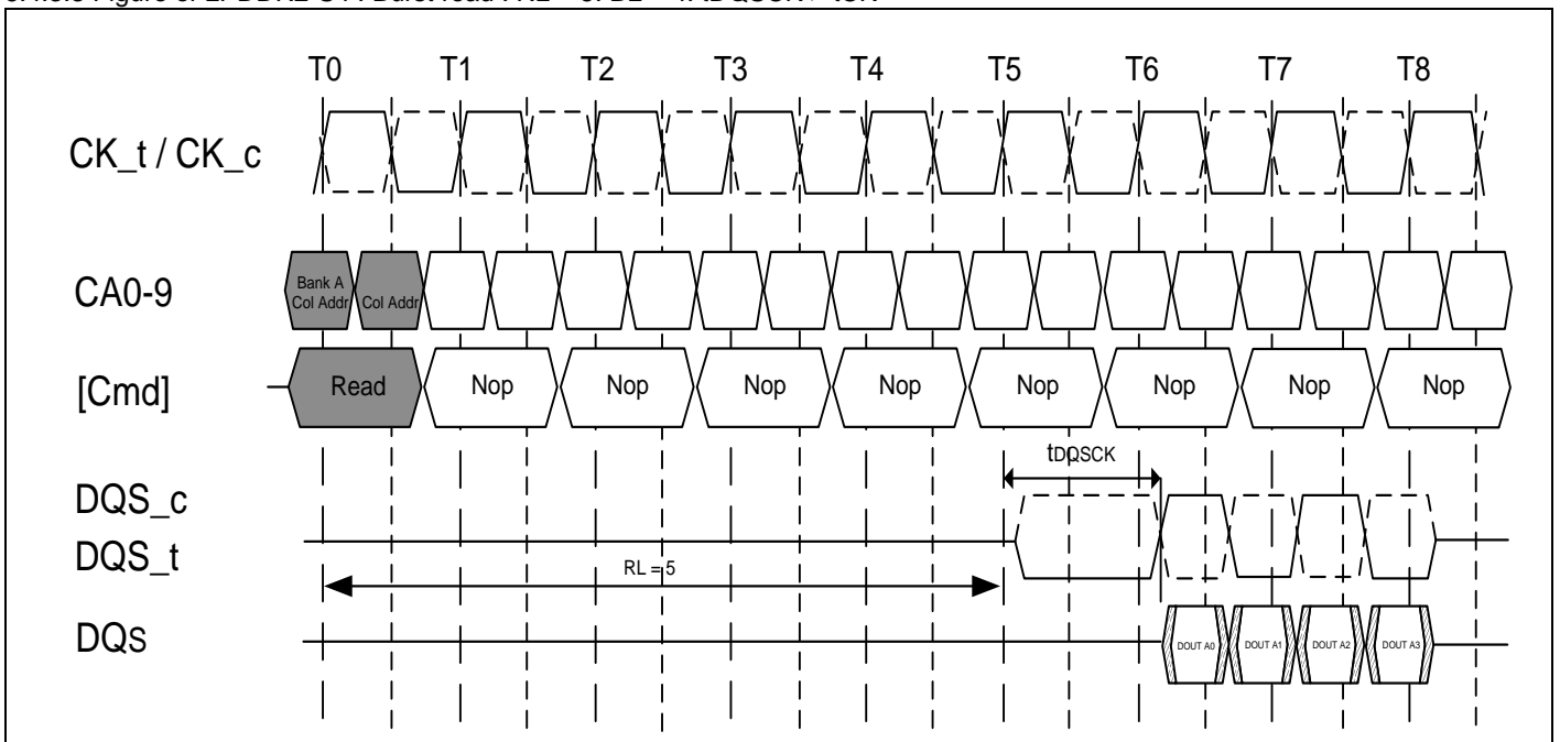
6.4.3.3 Figure of LPDDR2-S4 : Burst read : RL = 5 . BL = 4 . t_{DQSK} > t_{CK}
