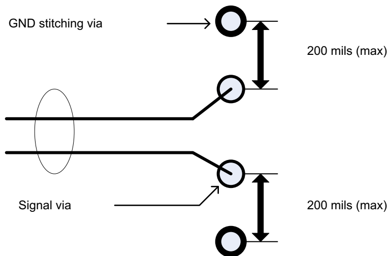
Figure 11. Stitching Vias
