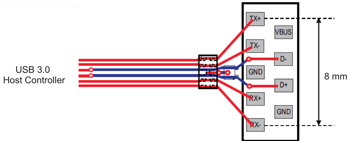
Figure 22. Flow-Through Routing
