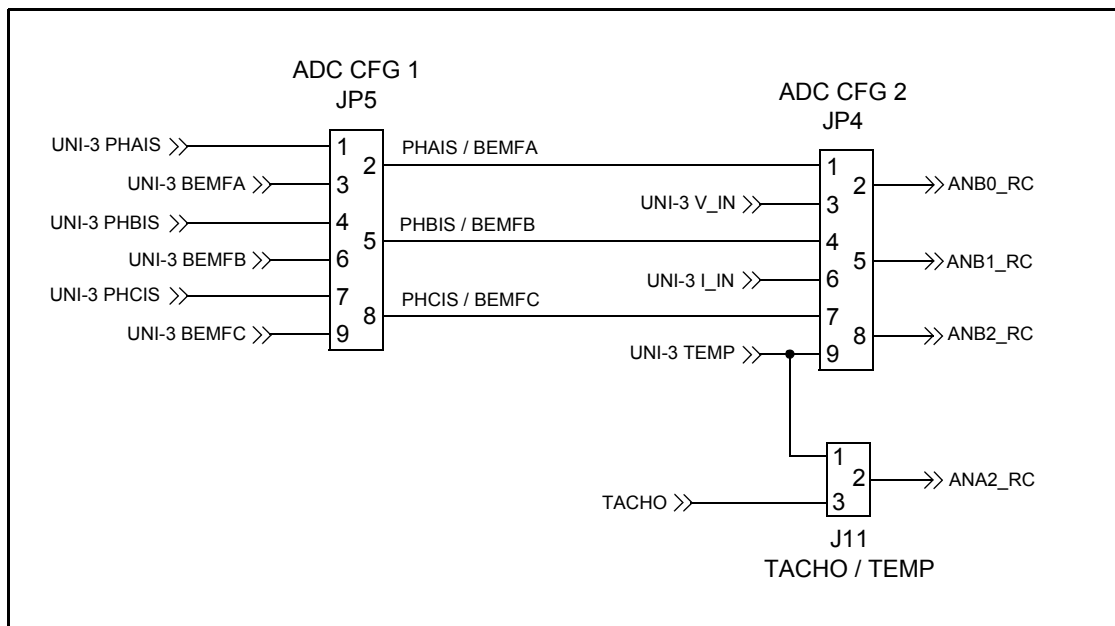
Figure 2-8. ADC input selection
