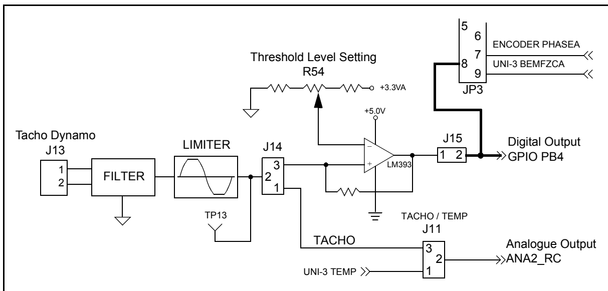
Figure 2-10. Tacho-Generator Interface
