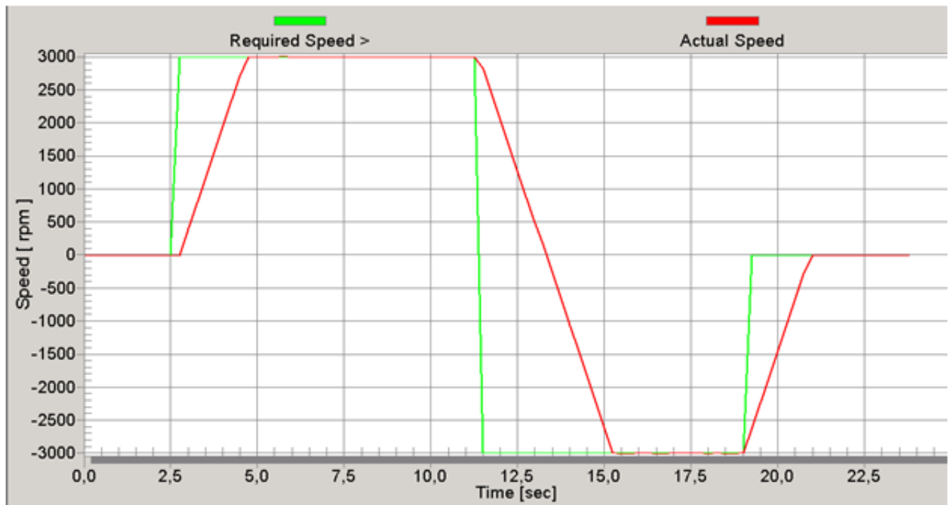
Figure 6-2. Speed profile
