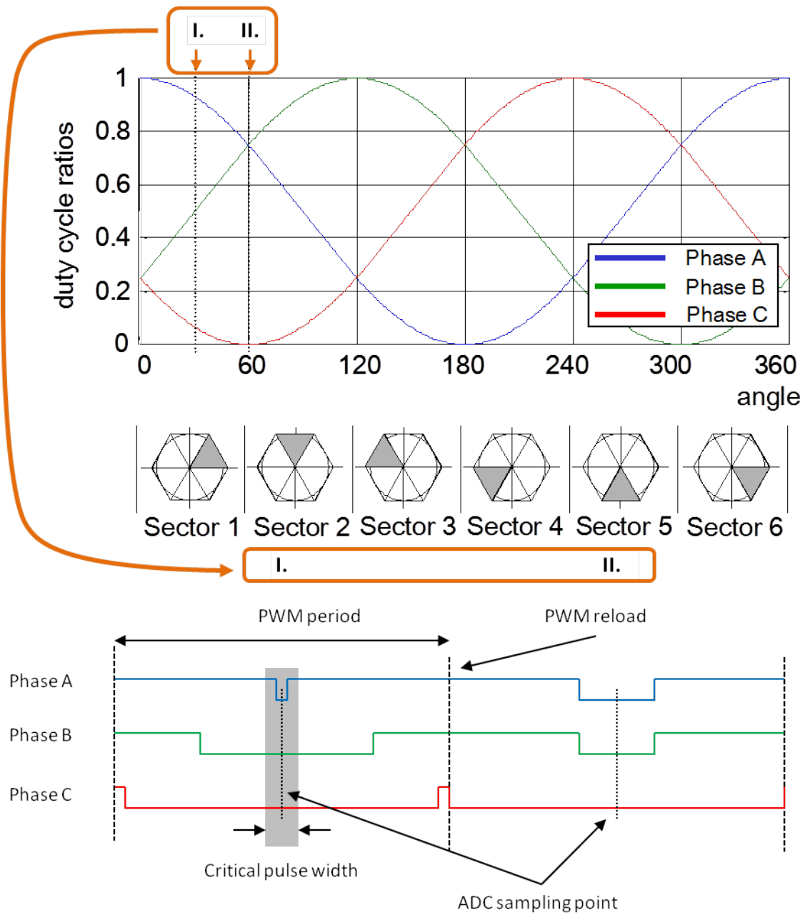
Figure 4-2. Current sensing
