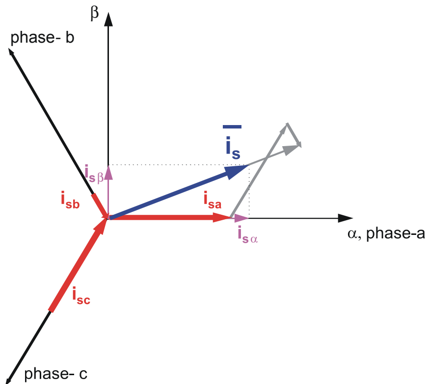
Figure 3-2. Clarke Transformation
