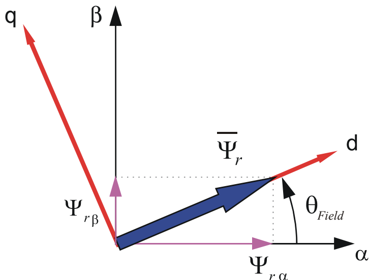
Figure 3-3. Park Transformation
