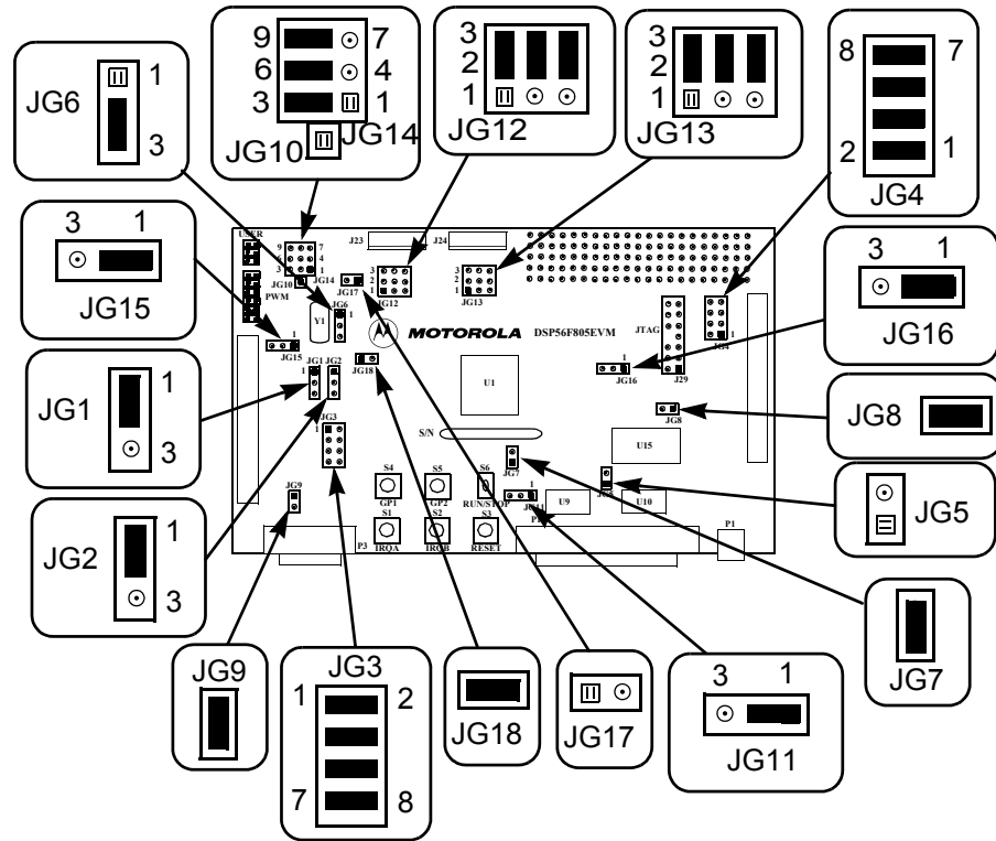
Figure 7-2. DSP56F805EVM Jumper Reference
