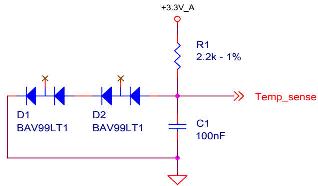
Figure 6-19. Temperature Sensing
