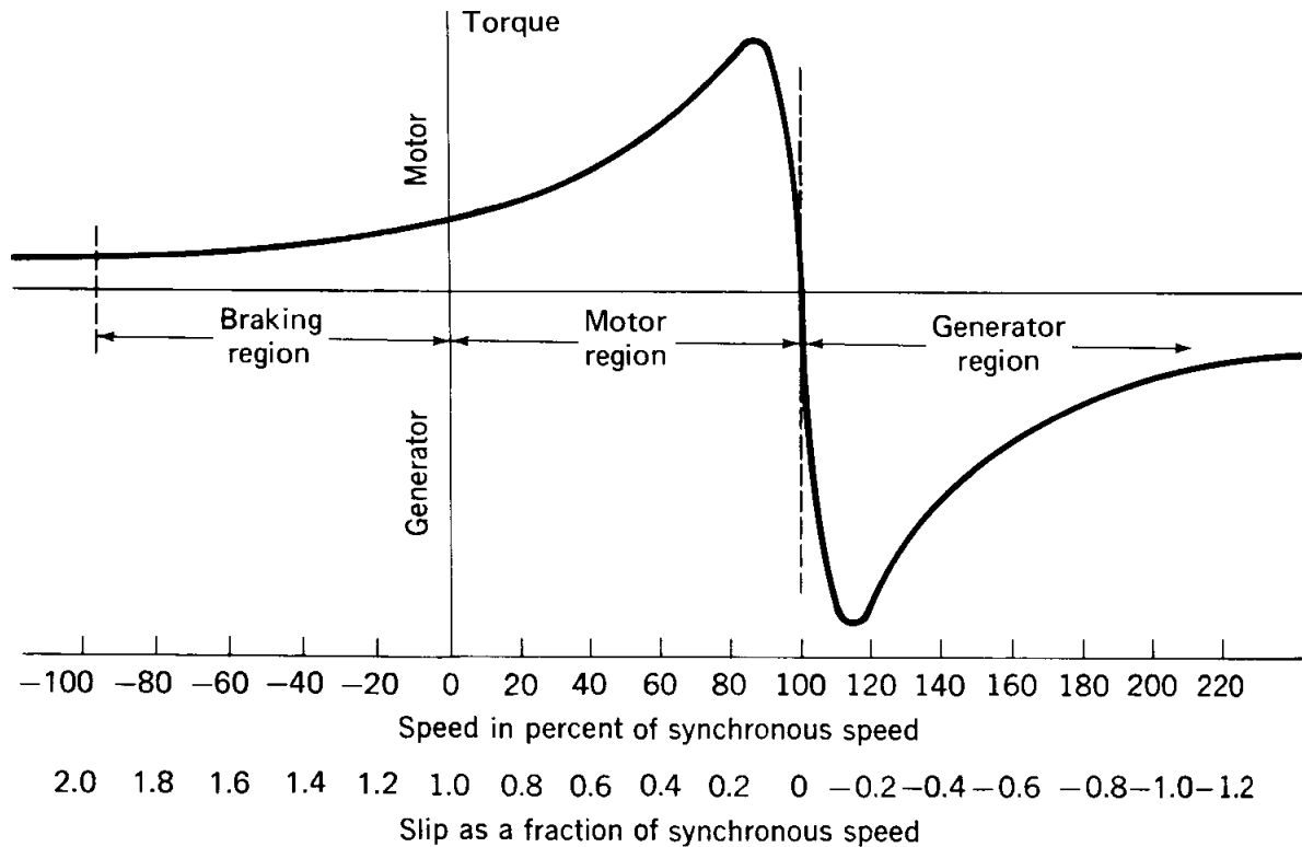
Figure 2-2. AC Induction Motor Speed-torque Characteristic
