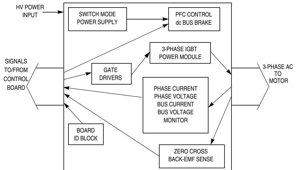
Figure 5-3. 3-Phase AC High Voltage Power Stage
