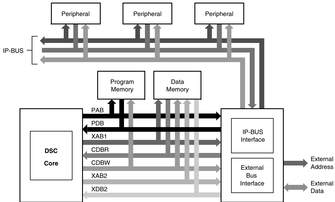
Figure 2-3. DSC Chip Architecture with External Bus
