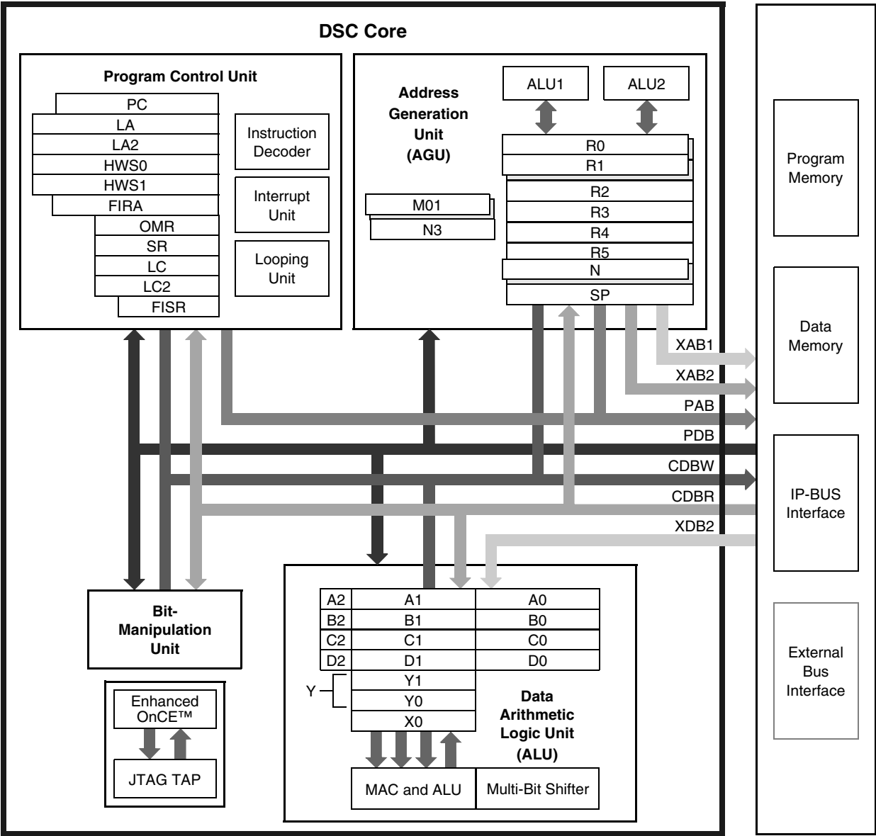
Figure 2-4. Core Block Diagram
