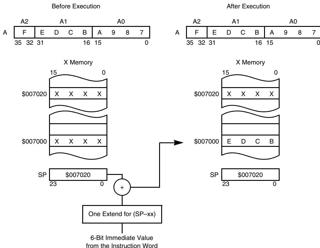
Indexed by 6-Bit Displacement Example: MOVE.W A1, X: (SP-32)
