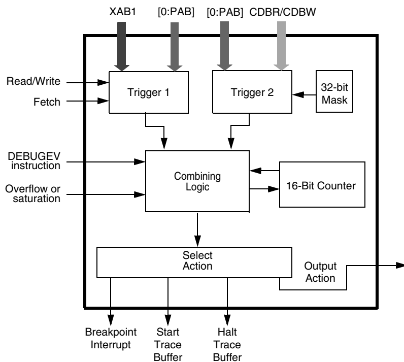
Figure 11-9. Breakpoint Unit Block Diagram
