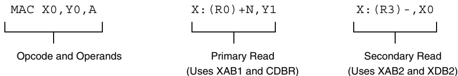
Figure 3-3. Dual Parallel Read
