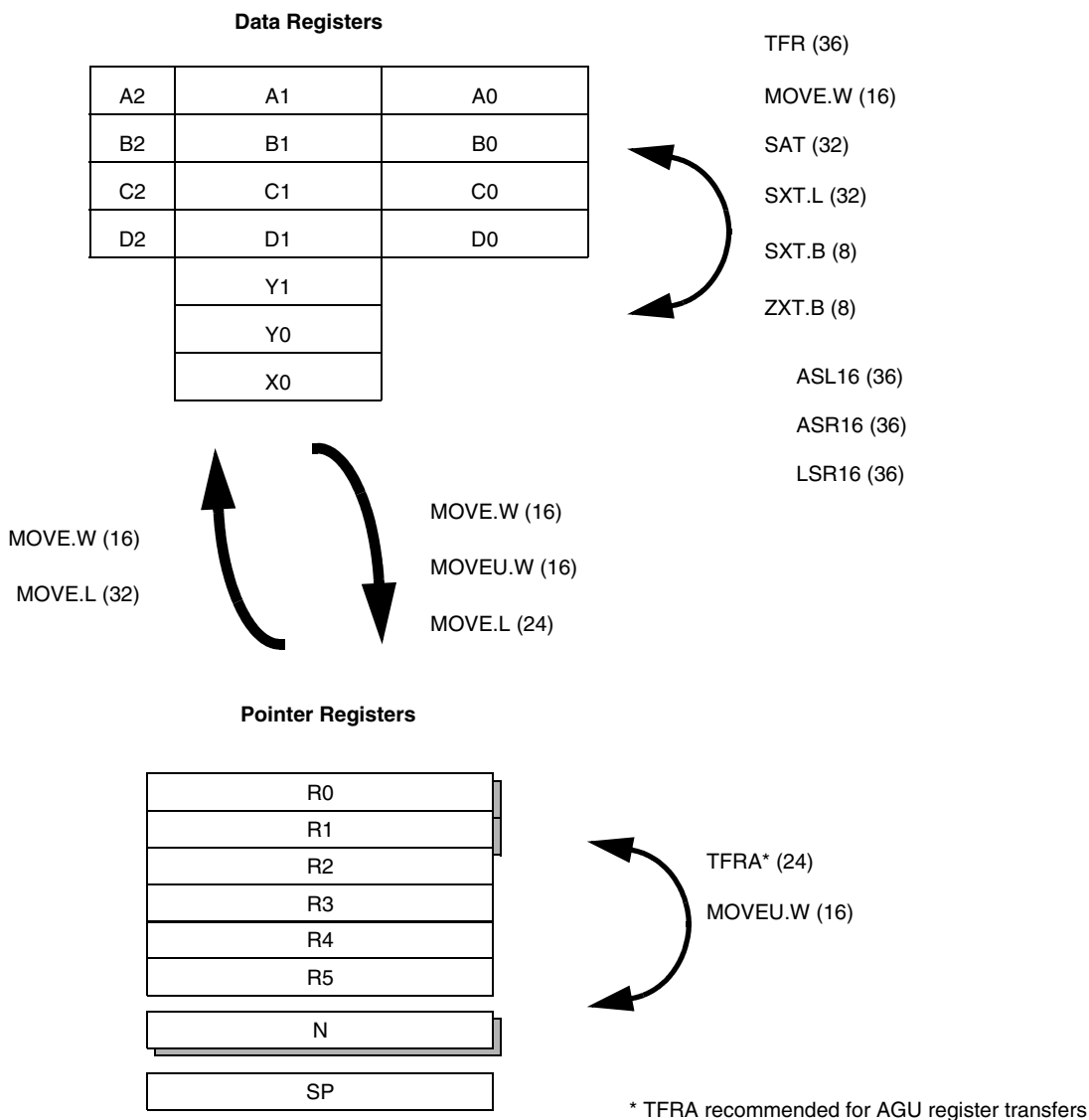
Figure 4-1. Moving Data in the Register Files
