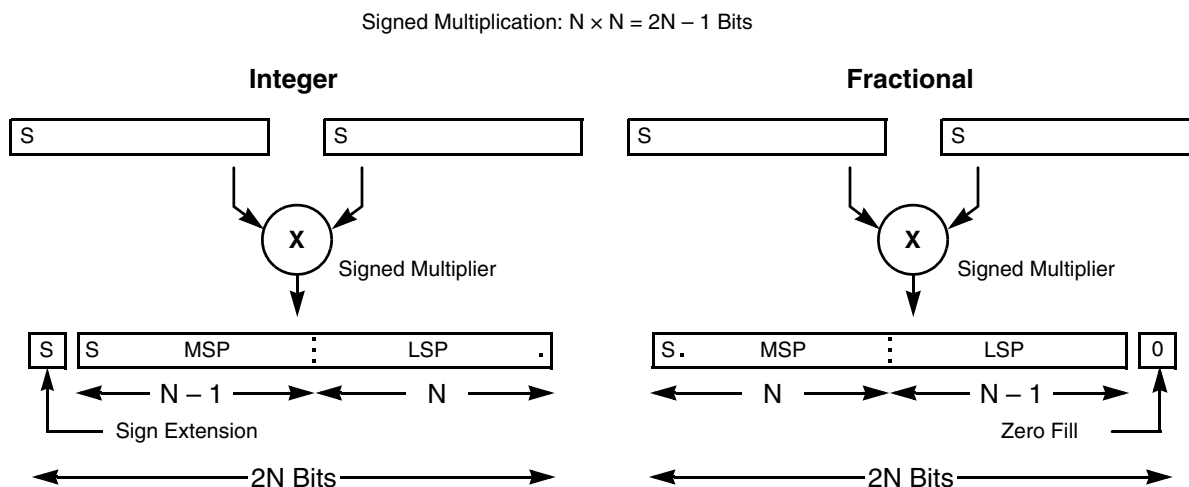
Figure 5-13. Comparison of Integer and Fractional Multiplication
