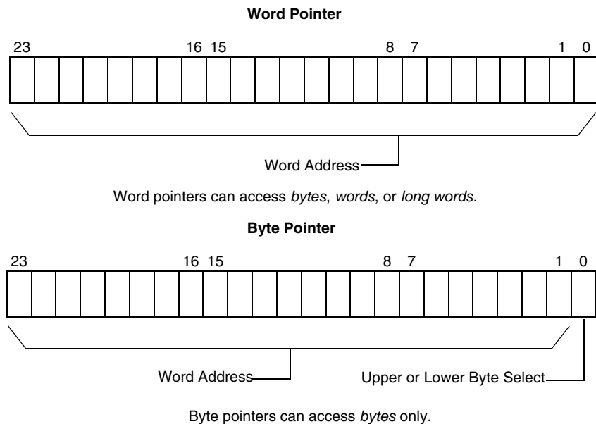
Figure 3-8. Structure of Byte and Word Addresses
