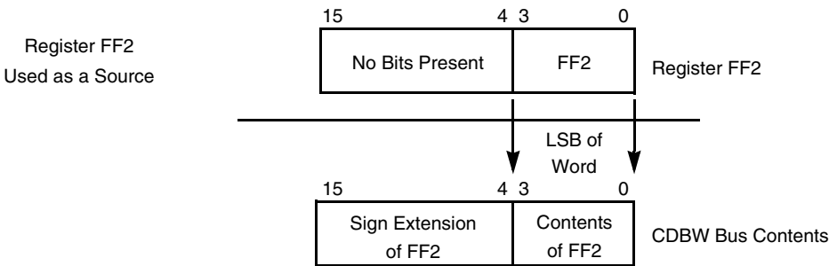
Figure 5-8. Reading the Accumulator Extension Registers (FF2)
