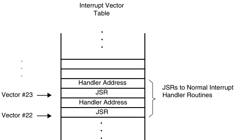
Figure 9-1. Interrupt Vector Table
