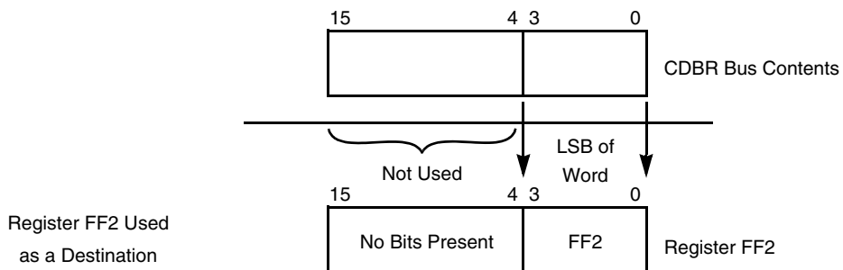
Figure 5-7. Writing the Accumulator Extension Registers (FF2)
