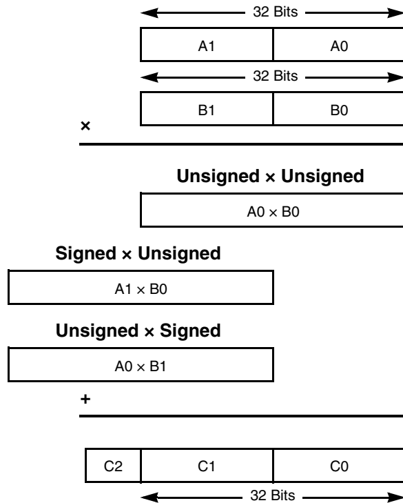
Figure 5-22. 32-Bit x 32-Bit → 32-Bit Signed Integer Multiplication
