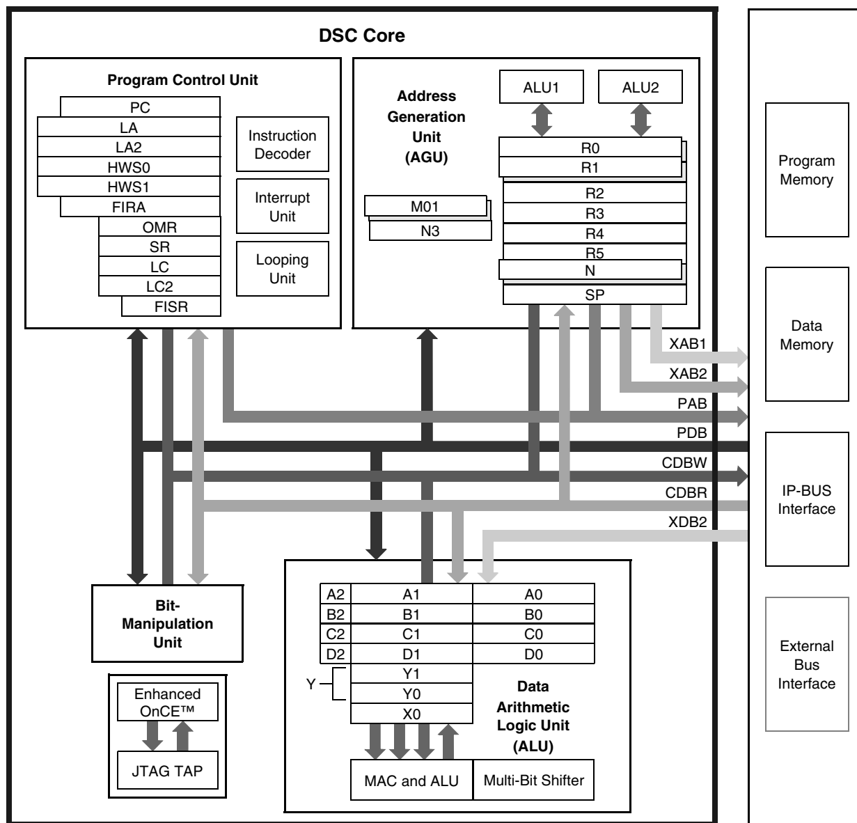
Figure 1-1. DSP56800EX/DSP56800E Core Block Diagram
