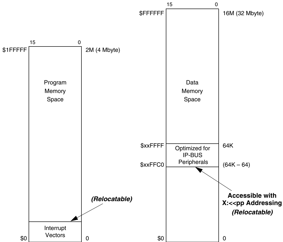
Figure 2-2. Dual Harvard Memory Architecture
