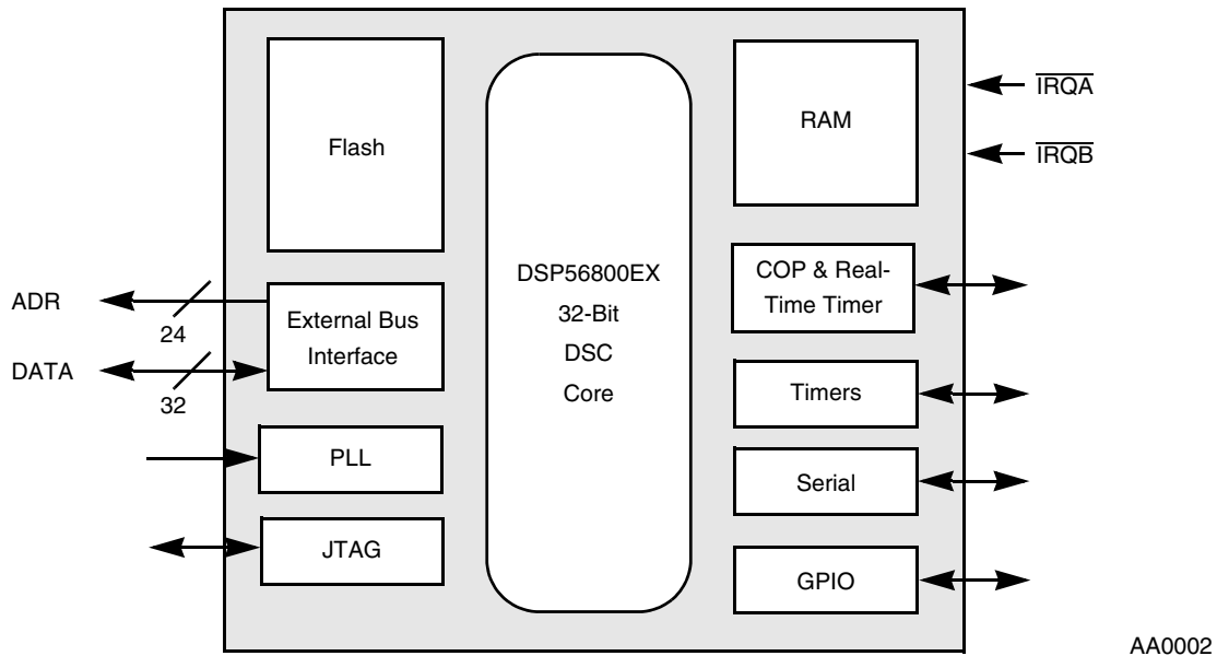
Figure 1-2. Example of Chip Based on DSP56800EX Core
