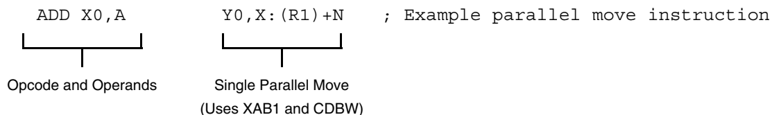
Figure 3-2. Single Parallel Move
