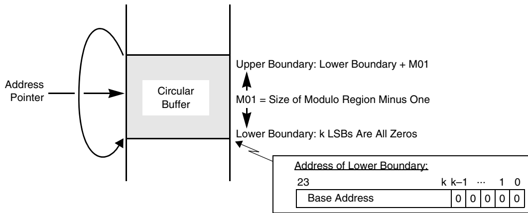
Figure 6-7. Circular Buffer
