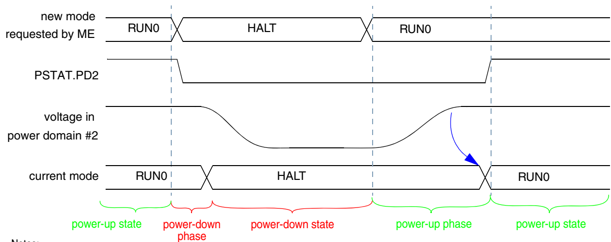
Figure 10-102. MC_PCU Events During Power Sequences (non-STANDBY mode)
