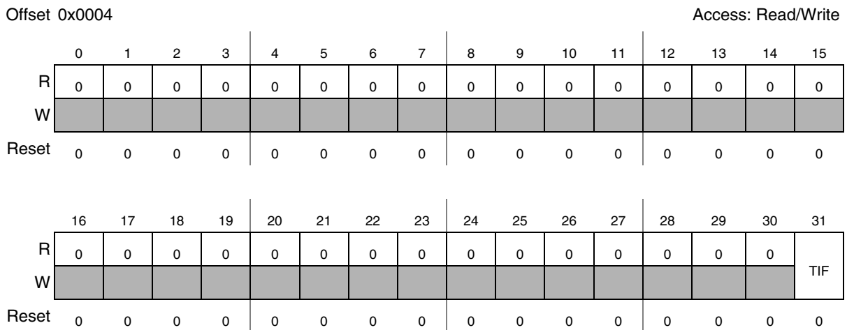
Figure 33-2. SWT Interrupt Register (SWT_IR)
