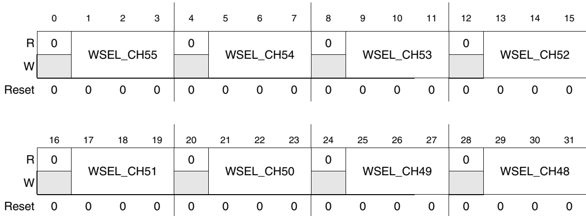
Figure 28-54. Channel Watchdog Select Register 6 (CWSELR6) – ADC_0
