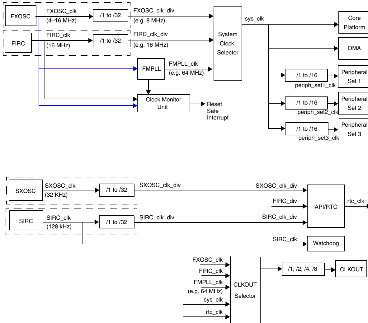
Figure 6-1. MPC5607B system clock generation
