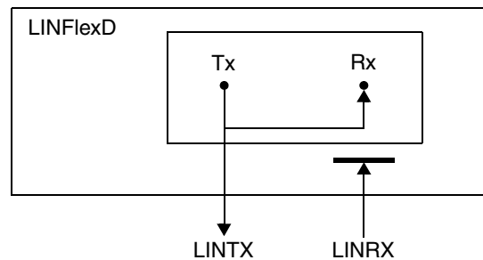
Figure 24-12. LINFlexD in Loop Back mode
