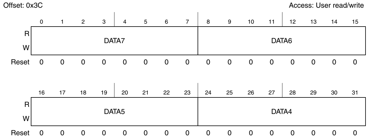
Figure 24-33. Buffer data register most significant (BDRM)
