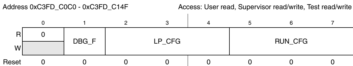
Figure 8-53. Peripheral Control Registers (ME_PCTL0...143)
