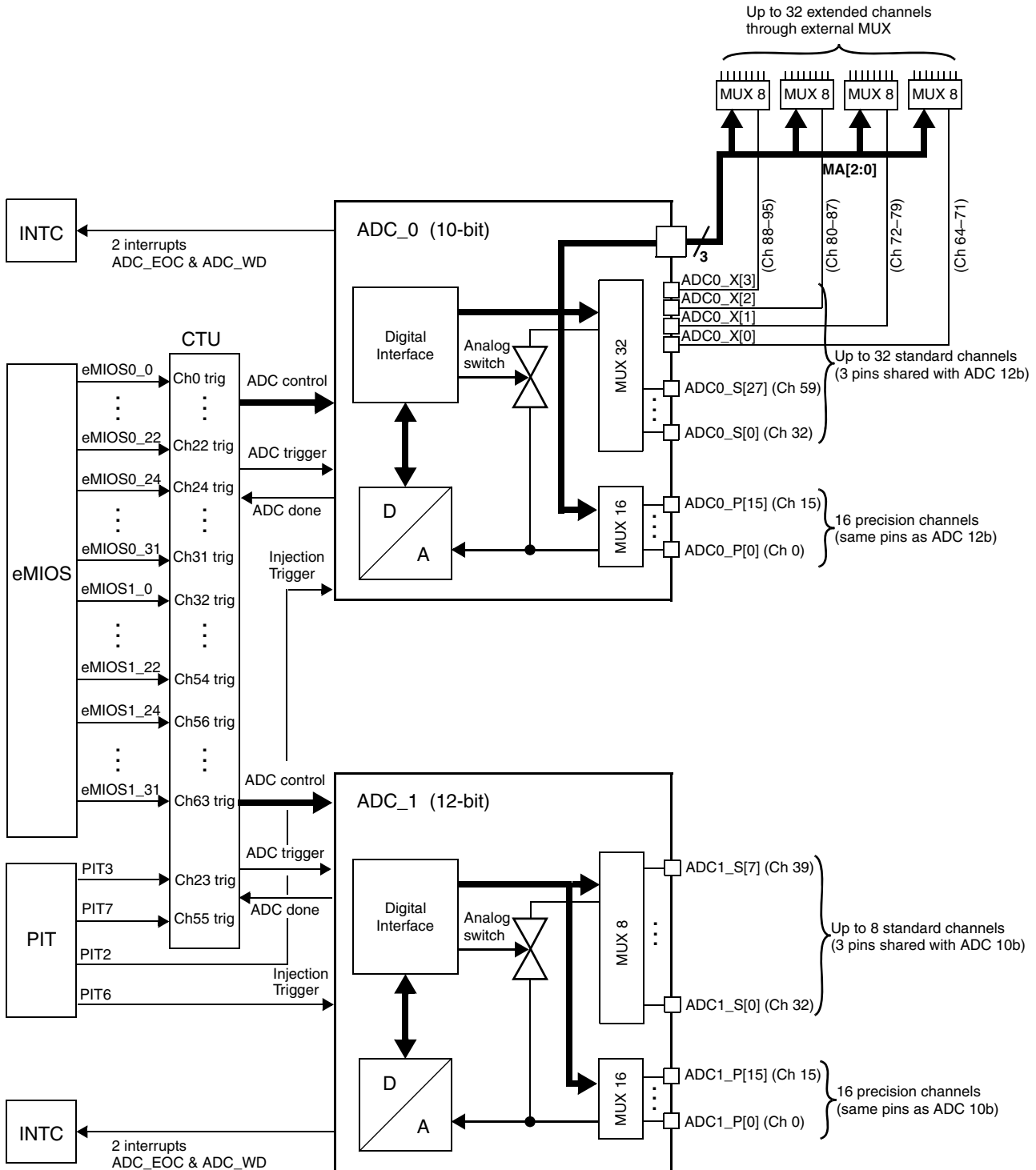
Figure 28-1. Implementation of ADC_0 and ADC_1
