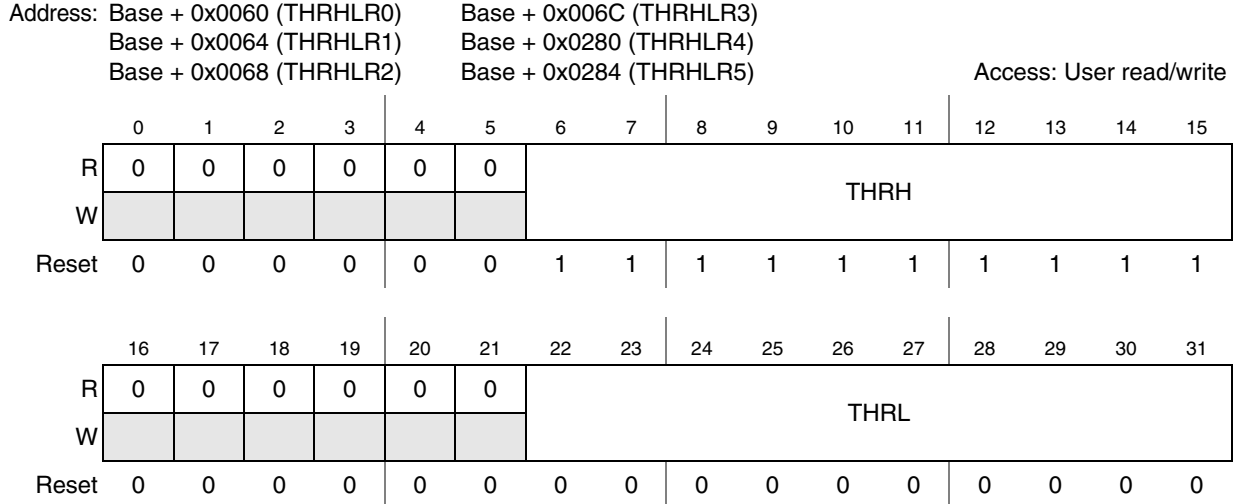
Figure 28-30. ADC_0 Threshold Register THRHLR[0..5]
