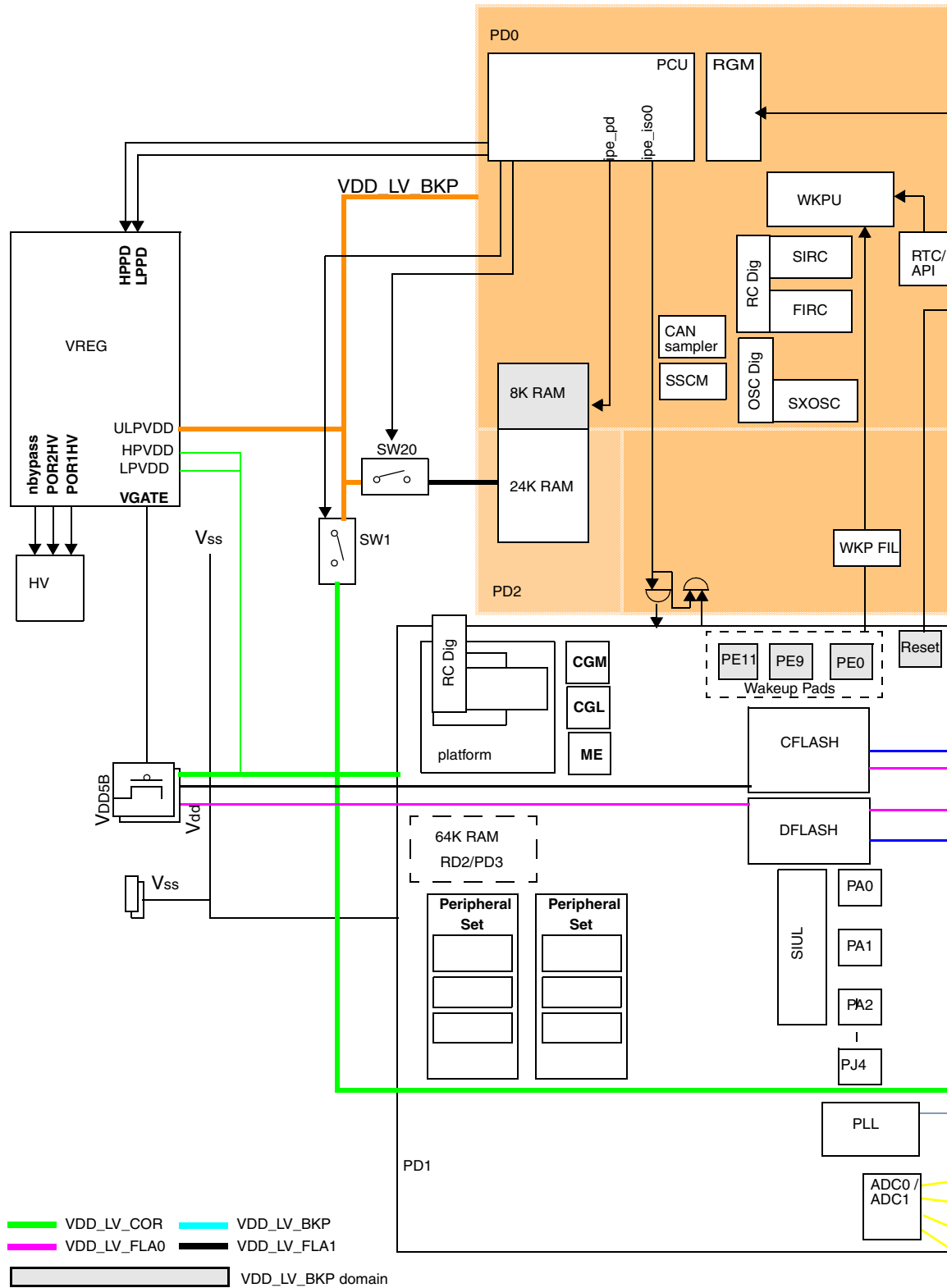
Figure 11-2. Power domain organization
