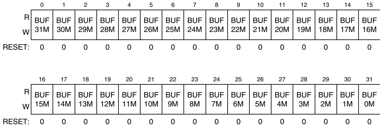
Figure 25-12. Interrupt Masks 1 Register (IMASK1)
