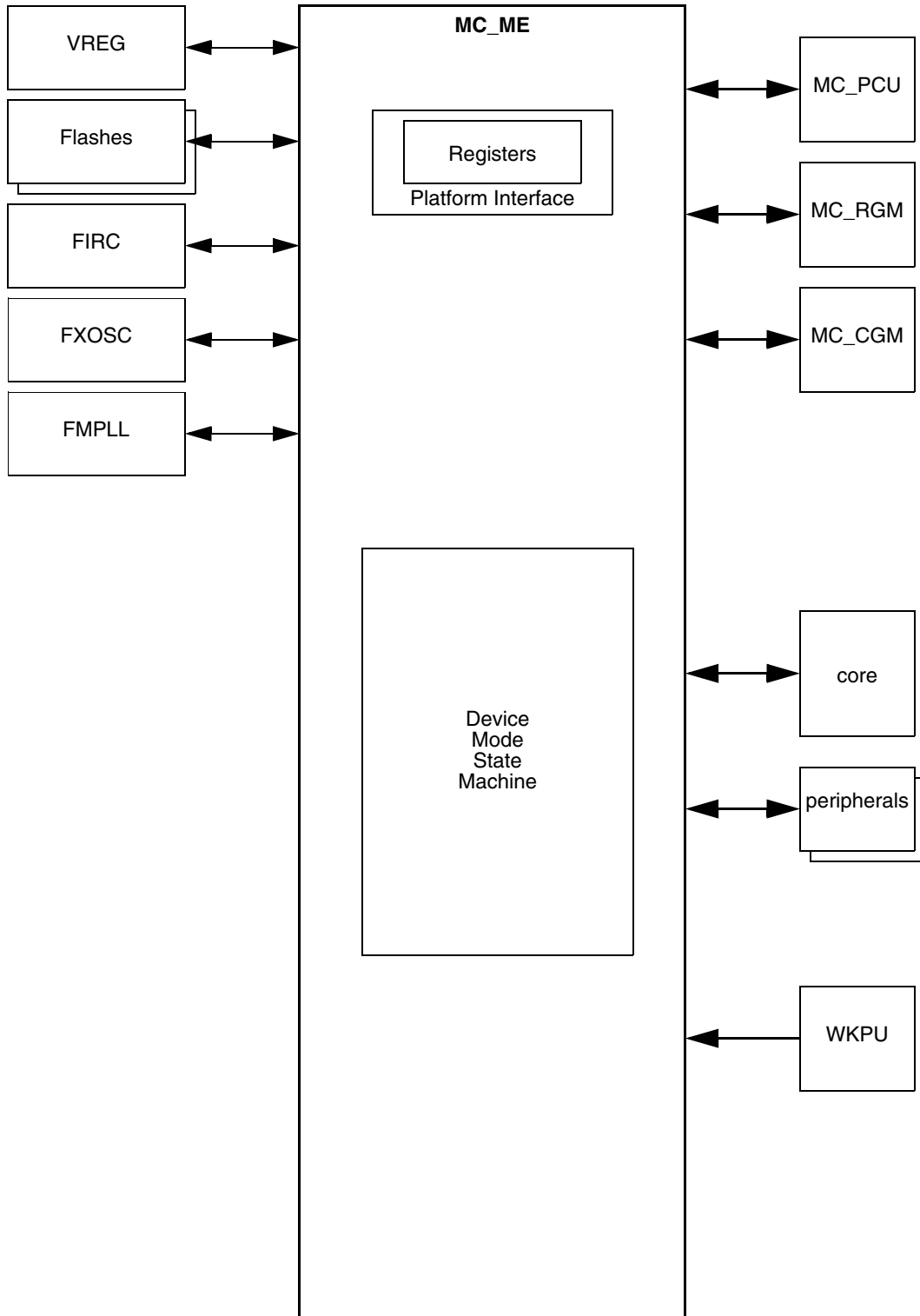
Figure 31. MC_ME block diagram
