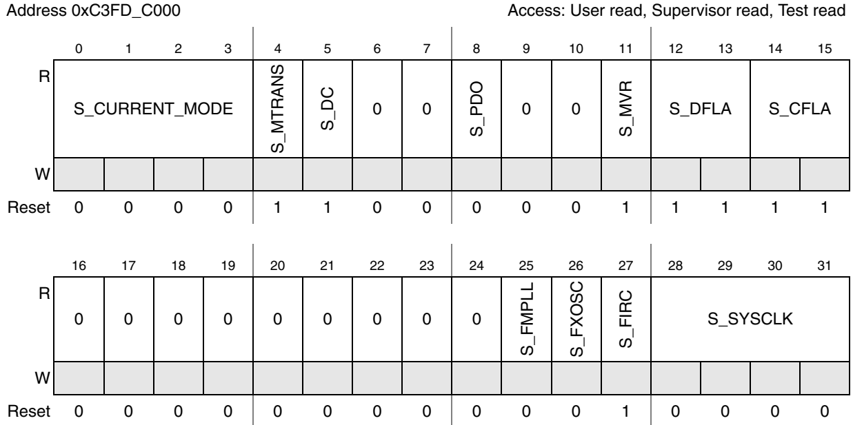
Figure 8-32. Global Status Register (ME_GS)
