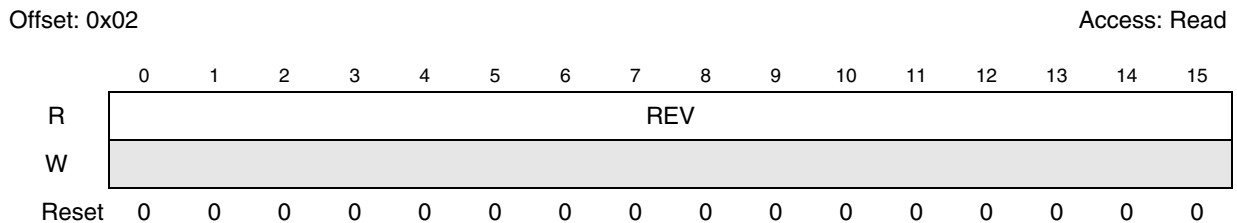
Figure 34-2. SoC-Defined Platform Revision Register (REV)
