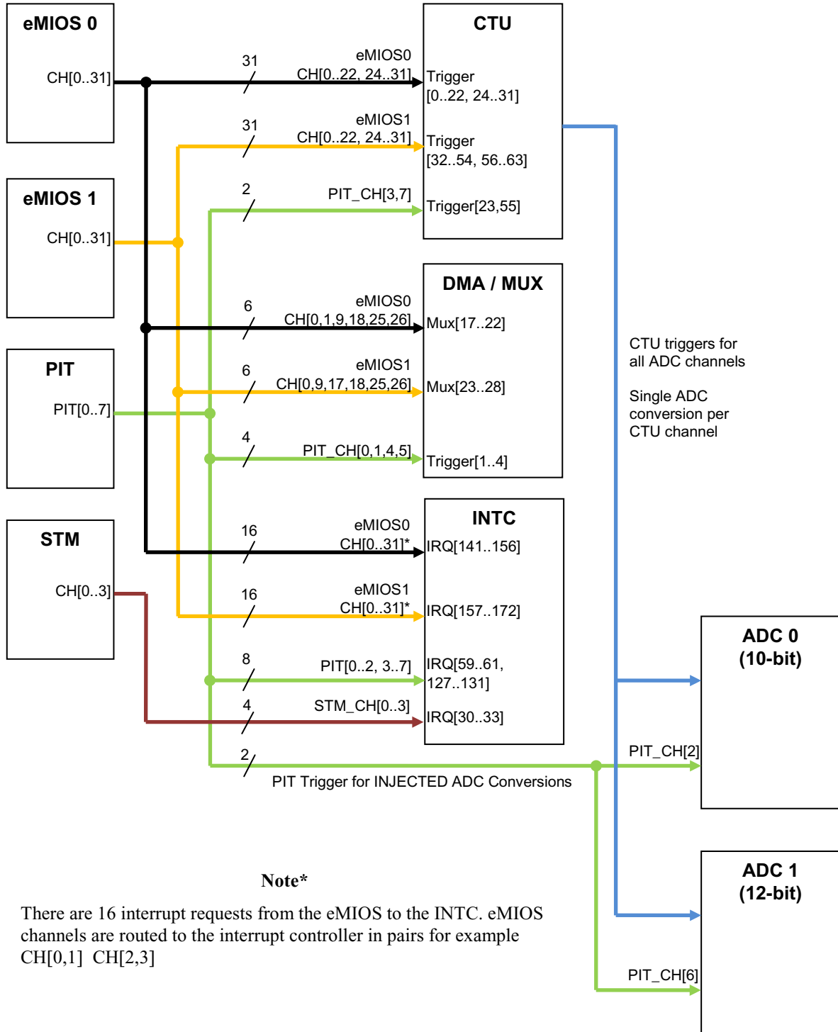
Figure 27-1. Interaction between timers and relevant peripherals
