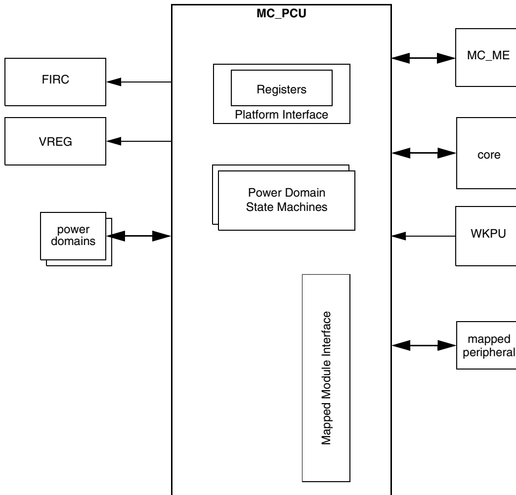
Figure 96. MC_PCU Block Diagram
