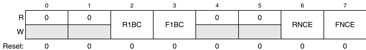
Figure 34-8. ECC Status Register (ESR)
