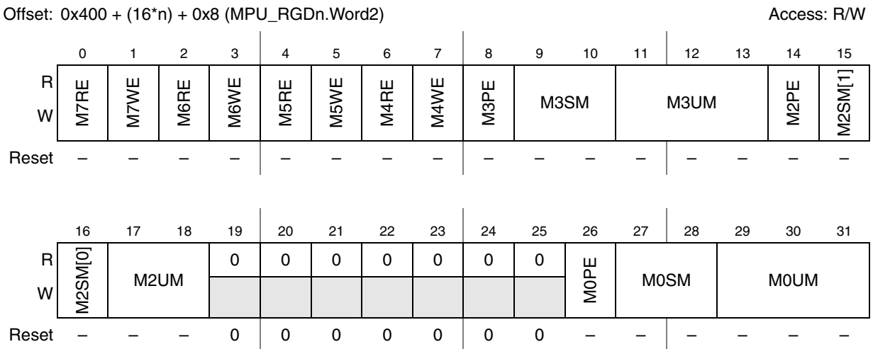
Figure 20-7. MPU Region Descriptor, Word 2 Register (MPU_RGDn.Word2)
