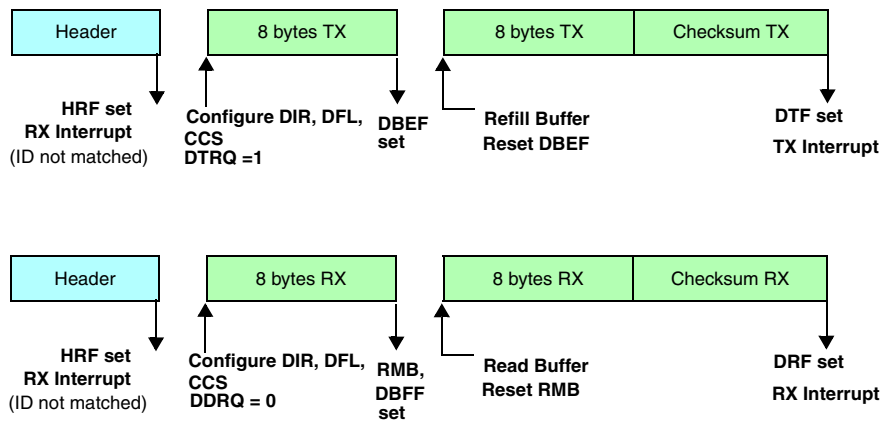
Figure 24-71. Programming consideration: extended frames
