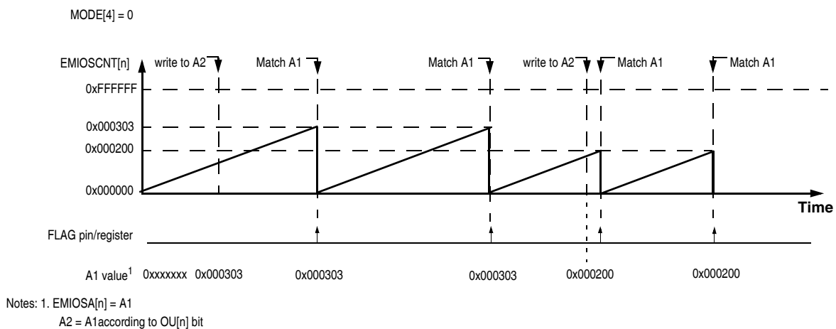
Figure 27-30. Modulus Counter Up mode example
