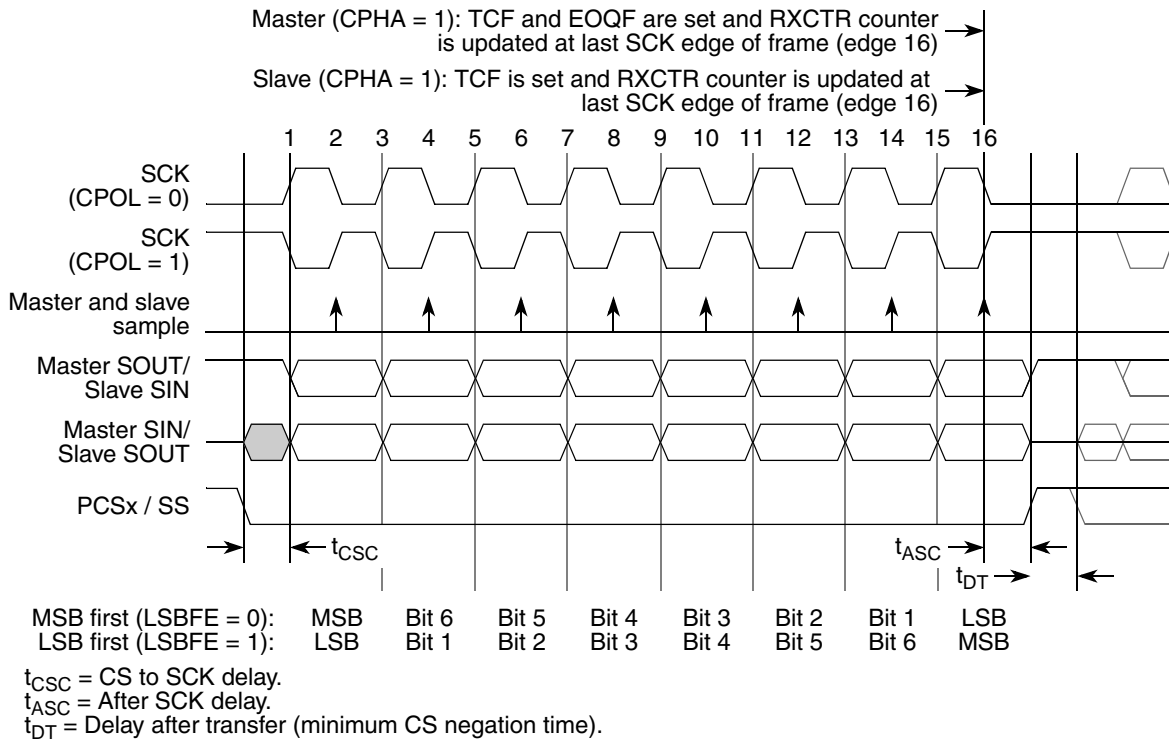
Figure 26-17. DSPI transfer timing diagram (MFE = 0, CPHA = 1, FMSZ = 8)
