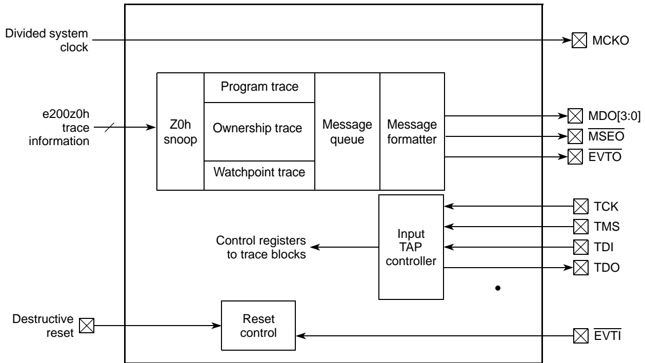
Figure 36-1. NDI functional block diagram
