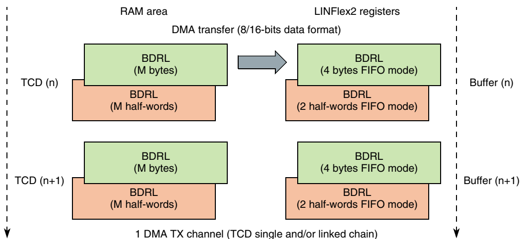
Figure 24-51. TCD chain memory map (UART node, TX mode)
