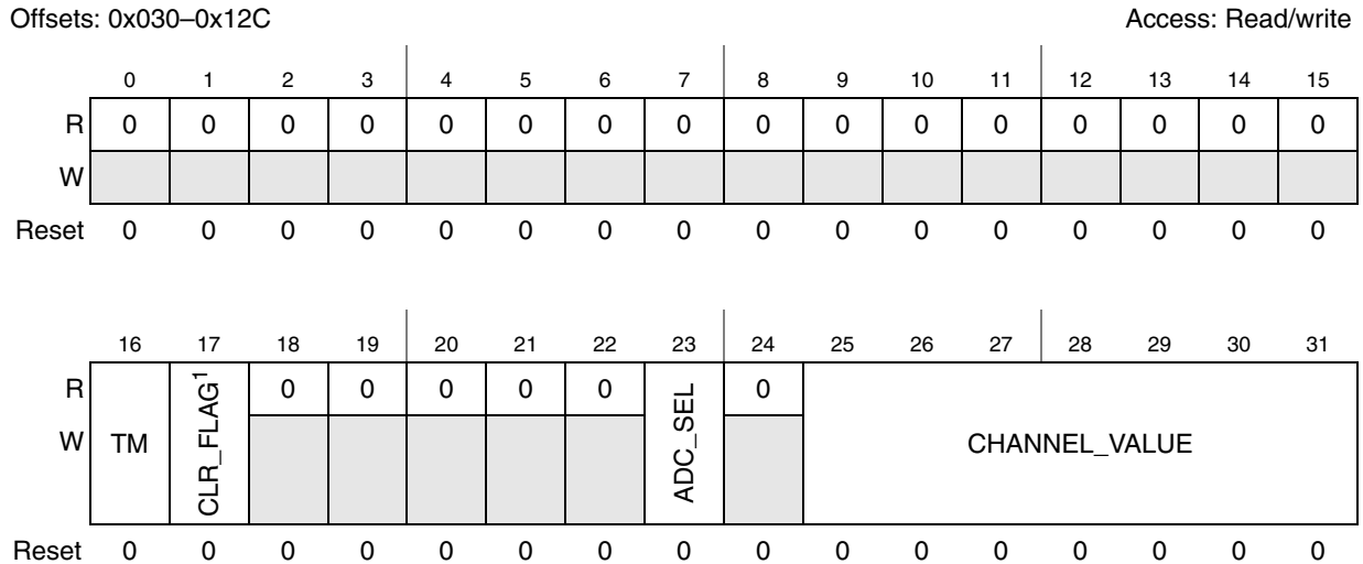
Figure 29-2. Event Configuration Registers (CTU_EVTCFGRx) (x = 0...63)
