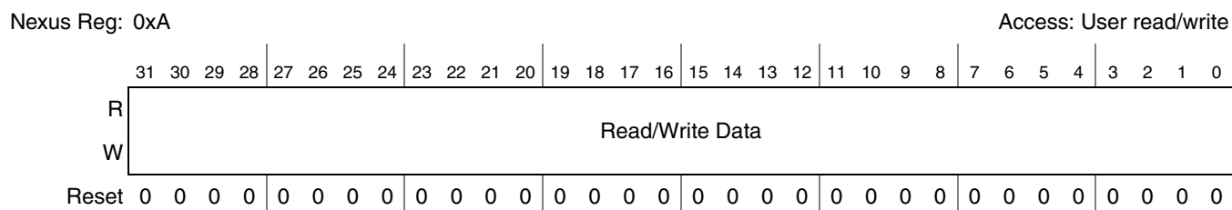
Figure 36-16. Read/Write Access Data Register (RWD)
