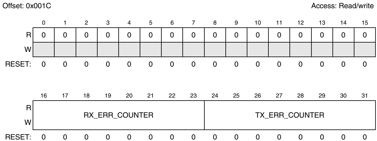
Figure 25-9. Error Counter Register (ECR)
