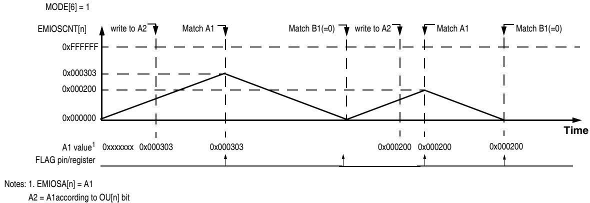
Figure 27-31. Modulus Counter Up/Down mode example
