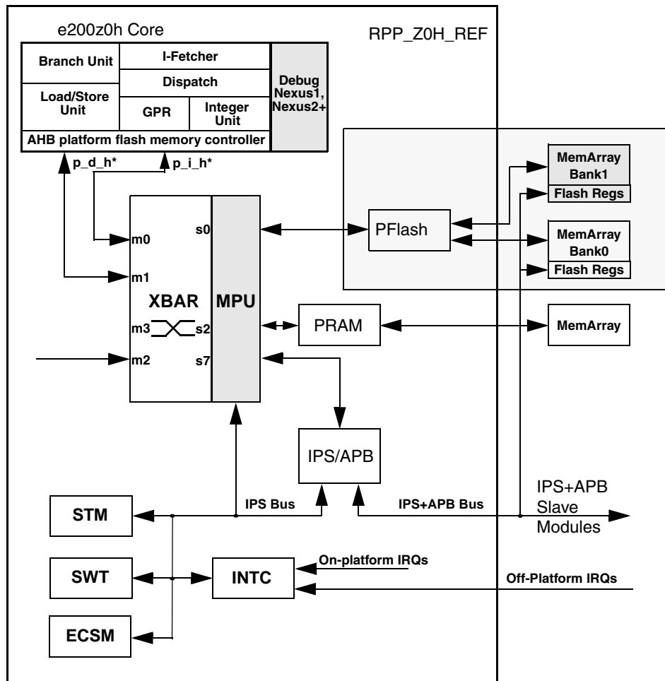
Figure 30-41. Power Architecture e200z0h RPP reference platform block diagram
