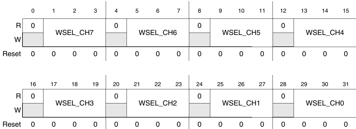
Figure 28-50. Channel Watchdog Select Register 0 (CWSELR0) – ADC_0
