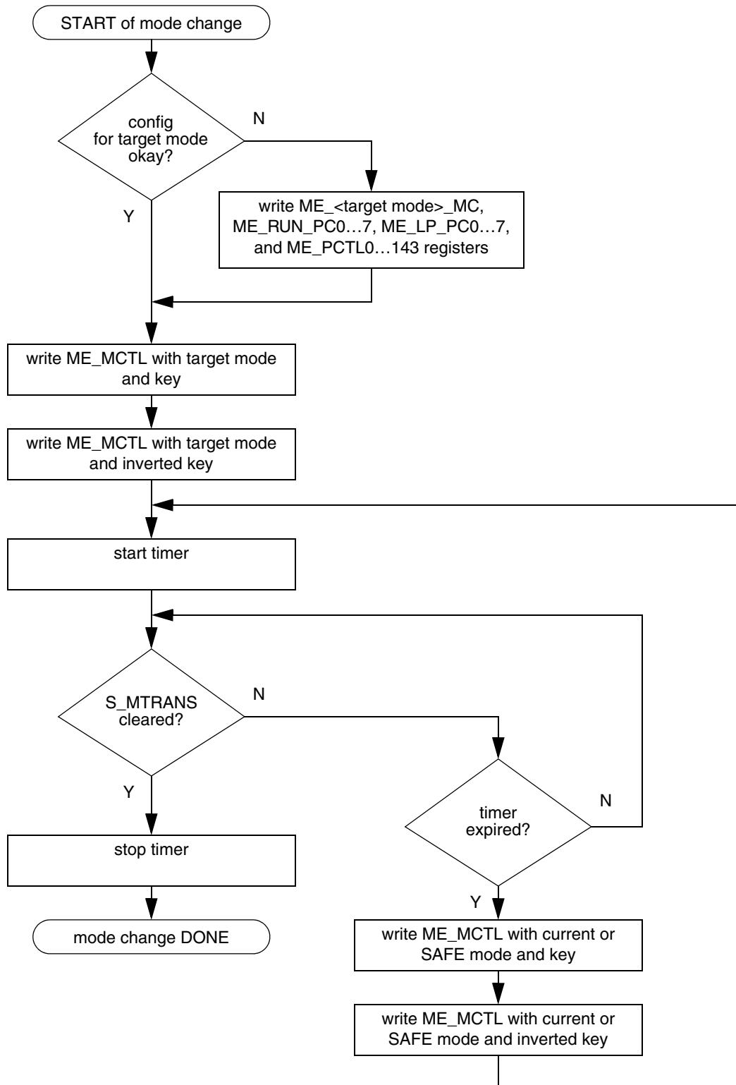
Figure 8-56. MC_ME Application Example Flow Diagram
