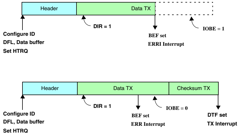
Figure 24-59. Programming consideration: master node, transmitter, bit error
