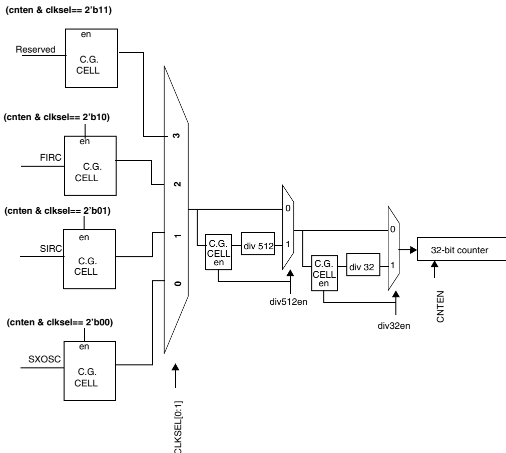
Figure 13-2. Clock gating for RTC clocks
