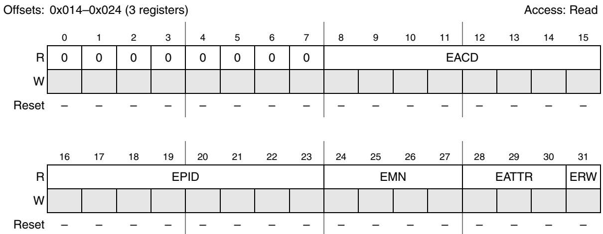
Figure 20-4. MPU Error Detail Register, Slave Port n (MPU_EDRn)
