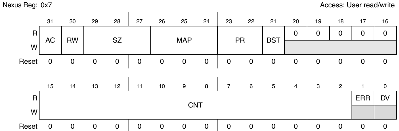
Figure 36-14. Read/Write Access Control/Status Register (RWCS)
