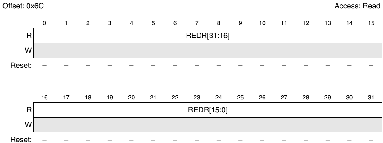
Figure 34-18. Platform RAM ECC Data Register (PREDR)
