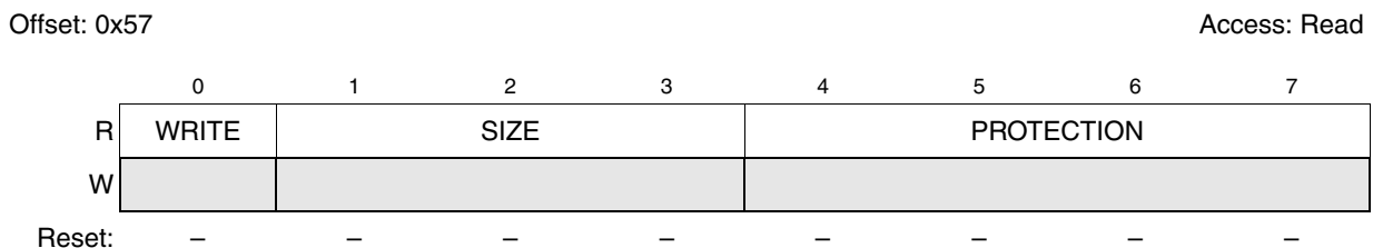
Figure 34-12. Platform Flash ECC Attributes Register (PFEAT)
