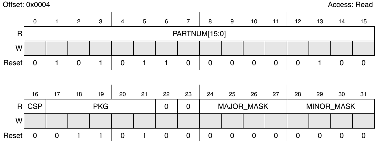
Figure 21-2. MCU ID Register #1 (MIDR1)
