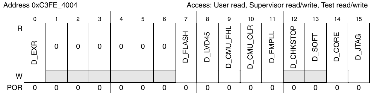
Figure 9-4. Functional Event Reset Disable Register (RGM_FERD)
