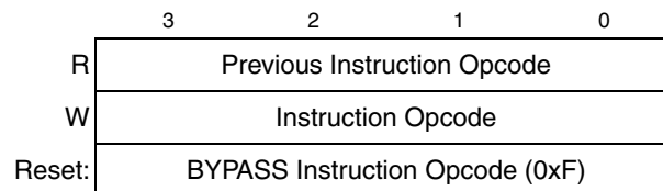
Figure 36-3. 4-Bit Instruction Register
