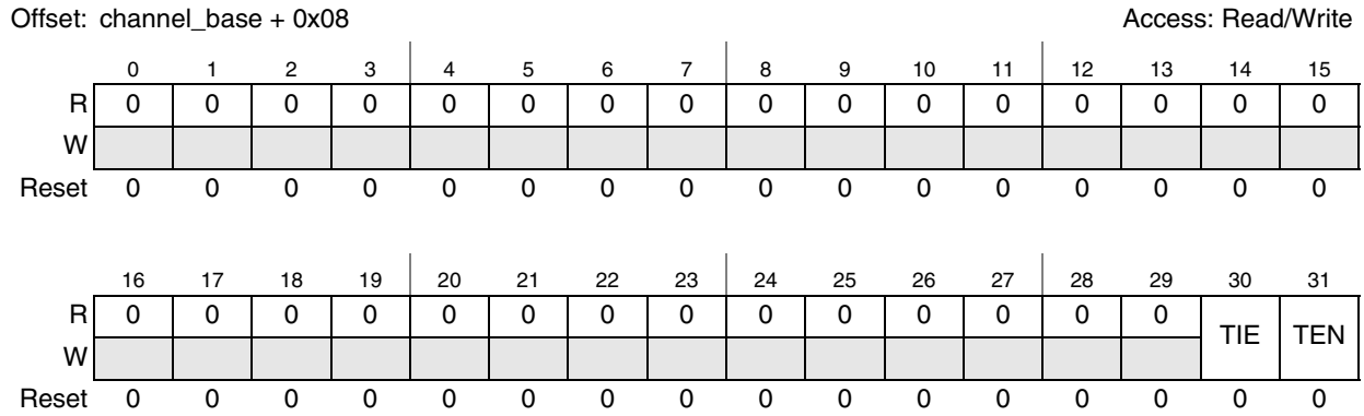
Figure 27-60. Timer Control Register (TCTRL)
