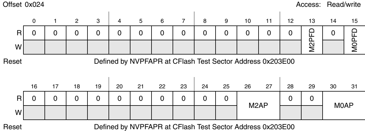
Figure 30-44. PFlash Access Protection Register (PFAPR)
