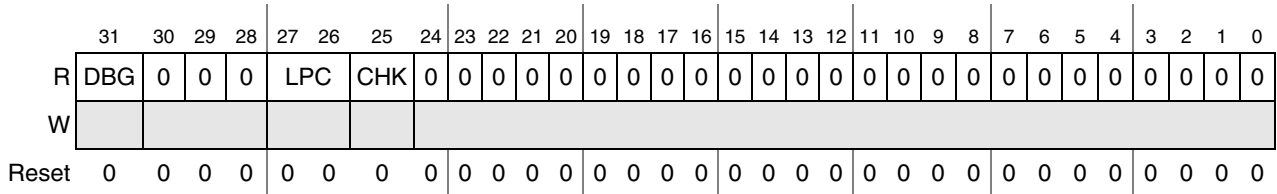
Figure 36-13. Development Status Register (DS)
