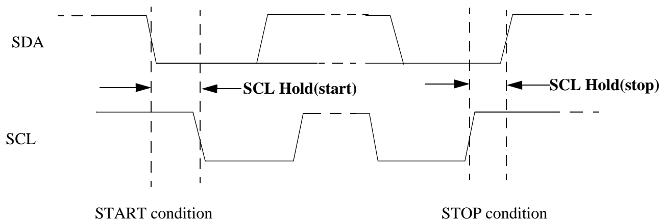
Figure 22-5. SCL divider and SDA hold
