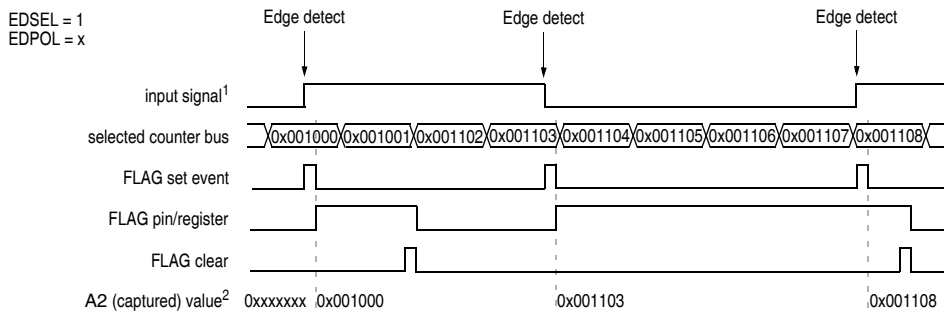
Figure 27-18. Single action input capture with rising edge triggering example
