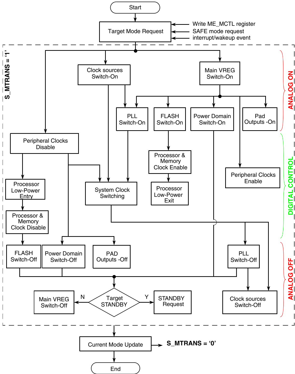
Figure 8-55. MC_ME Transition Diagram
