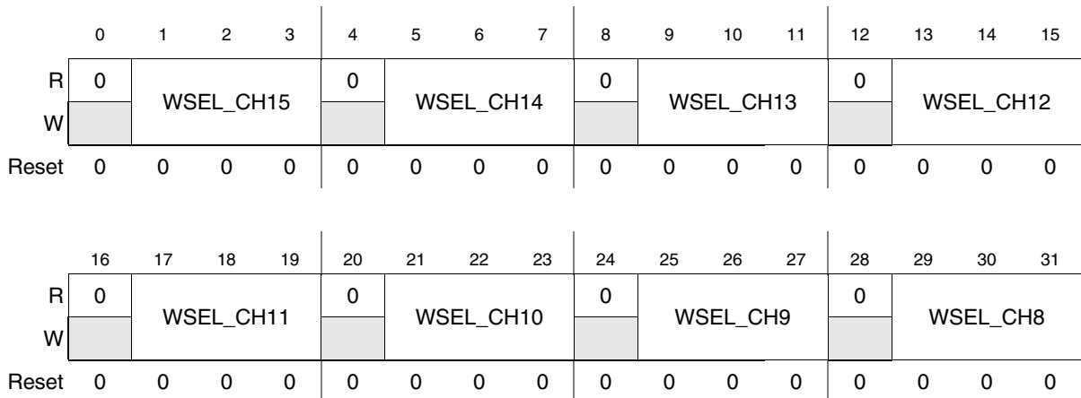
Figure 28-51. Channel Watchdog Select Register 1 (CWSELR1) – ADC_0
