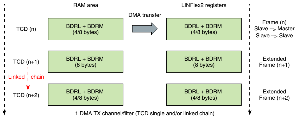
Figure 24-47. TCD chain memory map (slave node, TX mode)
