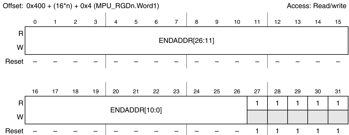
Figure 20-6. MPU Region Descriptor, Word 1 Register (MPU_RGDn.Word1)
