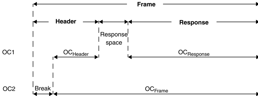
Figure 23-32. Header and response timeout
