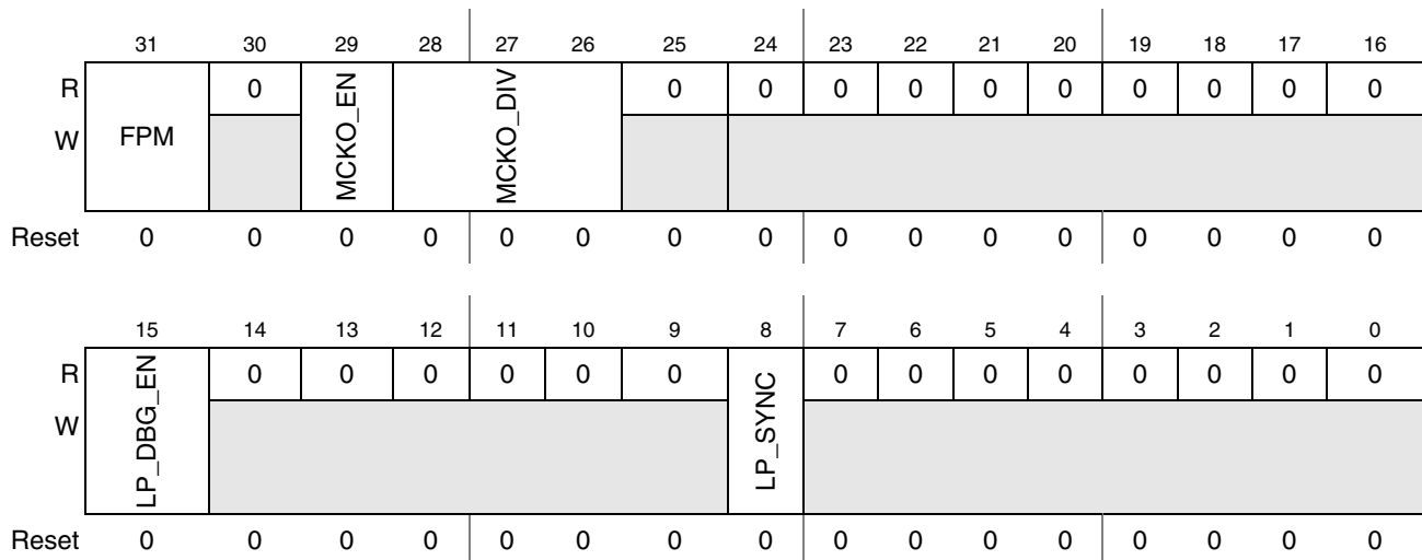
Figure 36-4. Port Configuration Register (PCR)
