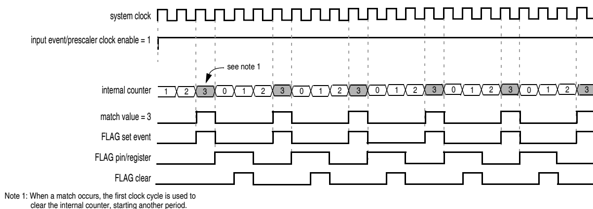
Figure 27-52. Time base period when running in the fastest prescaler ratio
