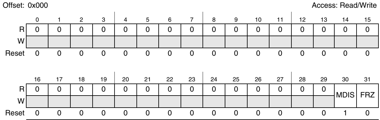
Figure 27-57. PIT Module Control Register (PITMCR)
