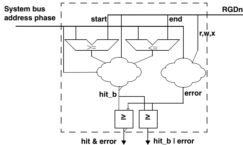
Figure 20-10. MPU access evaluation macro
