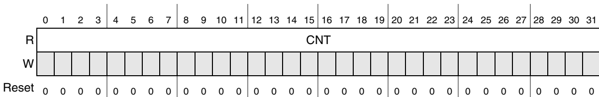
Figure 33-6. SWT Counter Output Register (SWT_CO)
