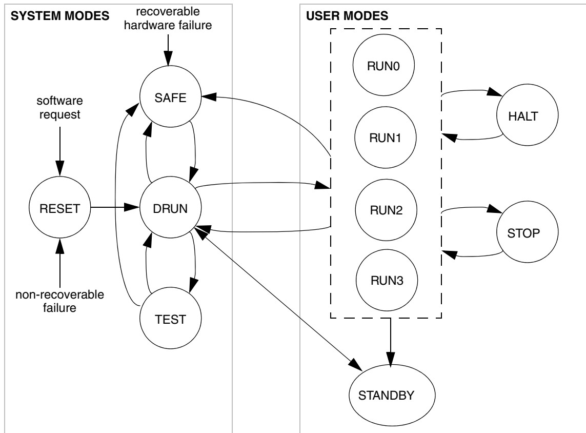
Figure 8-54. MC_ME Mode Diagram
