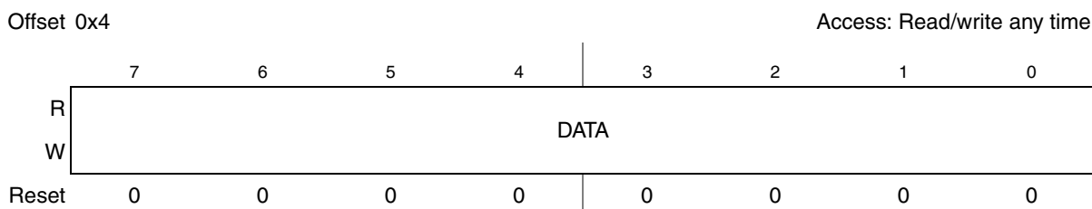
Figure 22-8. I 2 C Bus Data I/O Register (IBDR)
