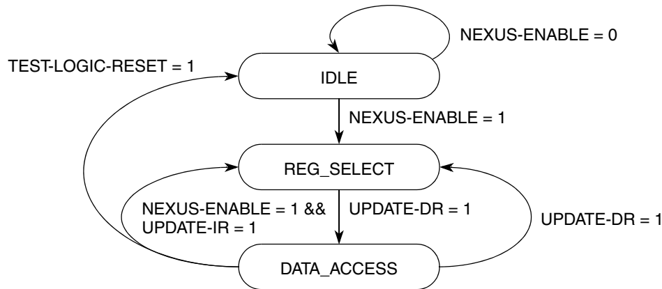
Figure 36-8. NEXUS Controller State Machine
