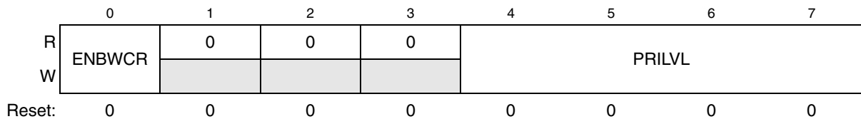
Figure 34-4. Miscellaneous Wakeup Control (MWCR) Register
