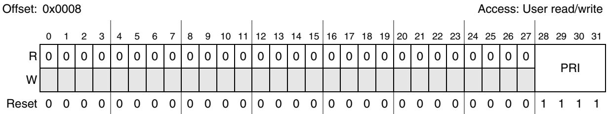
Figure 18-3. INTC Current Priority Register (INTC_CPR)
