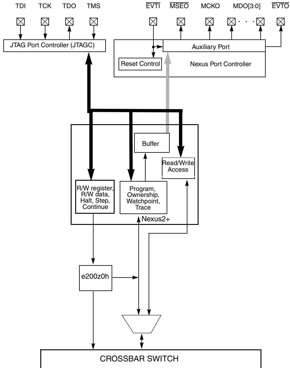
Figure 36-2. NDI implementation block diagram
