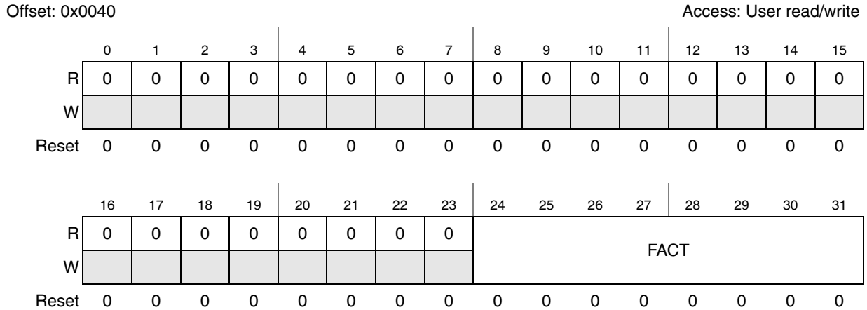
Figure 23-22. Identifier filter enable register (IFER)
