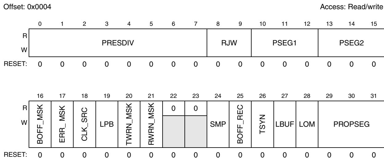
Figure 25-6. Control Register (CTRL)
