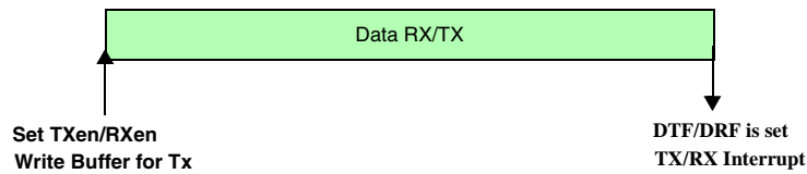
Figure 24-75. Programming consideration: UART mode
