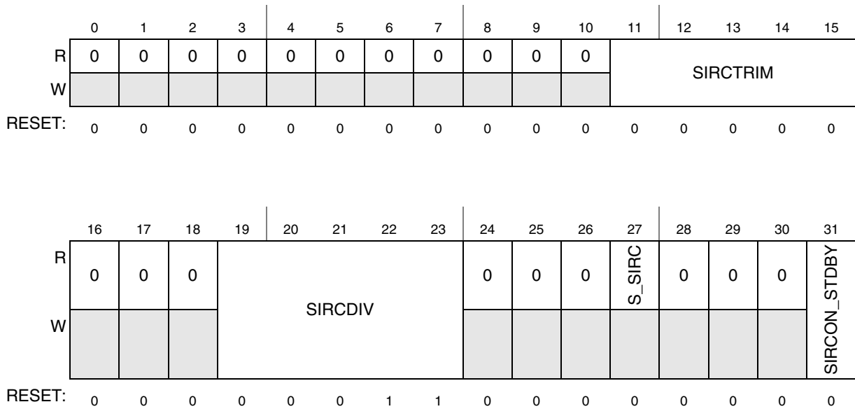
Figure 6-4. Low Power RC Control Register (SIRC_CTL)
