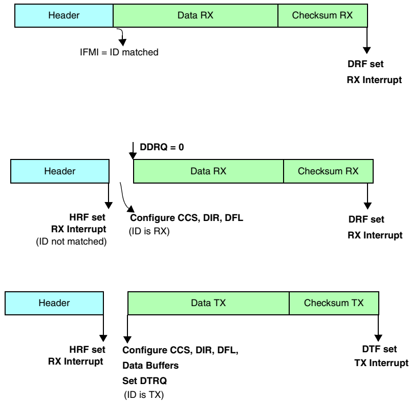
Figure 24-69. Programming consideration: slave node, RX filter, BF is set
