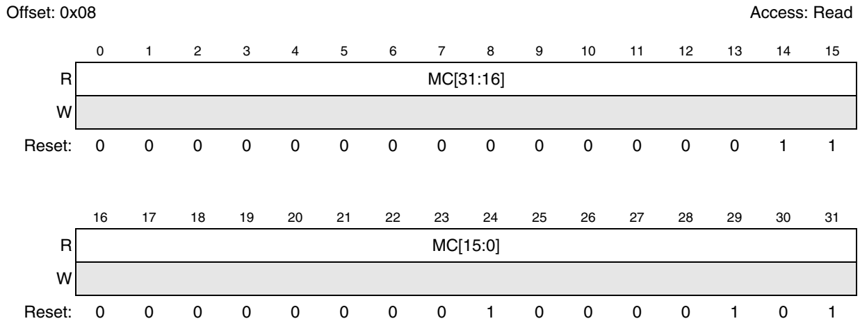
Figure 34-3. IPS On-Platform Module Configuration Register (IOPMC)
