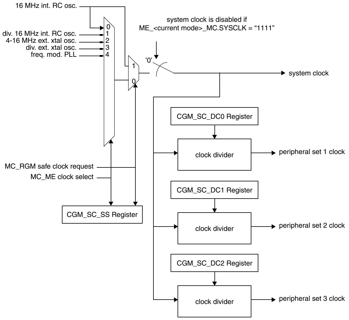
Figure 7-6. MC_CGM System Clock Generation Overview
