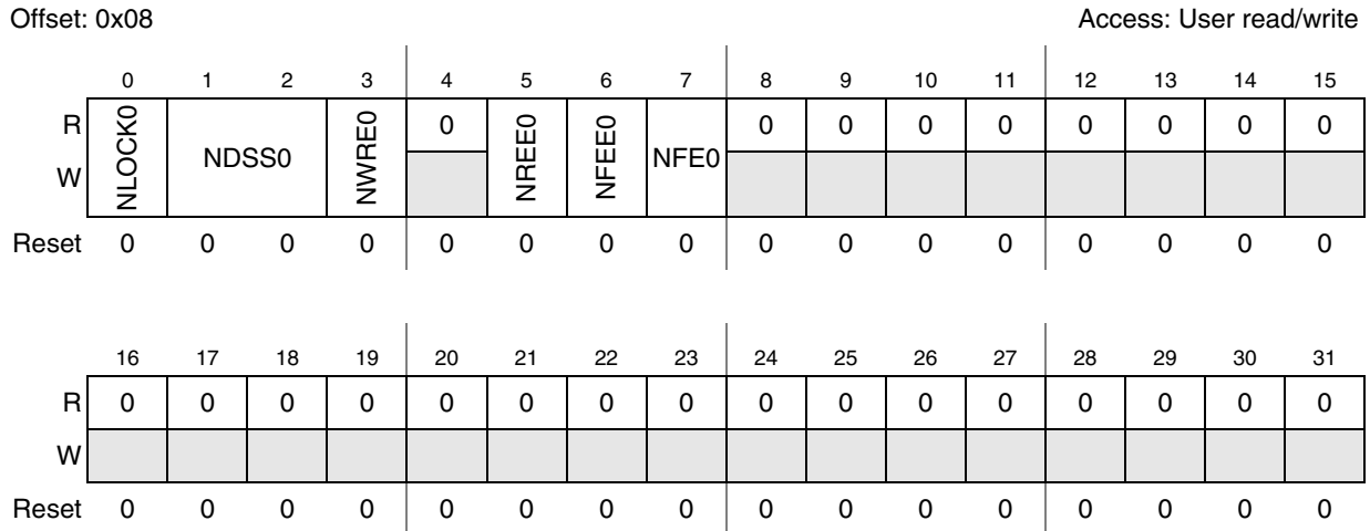
Figure 12-3. NMI Configuration Register (NCR)
