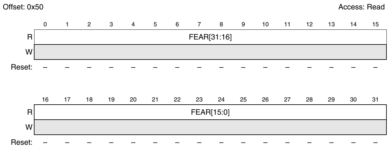
Figure 34-10. Platform Flash ECC Address Register (PFEAR)
