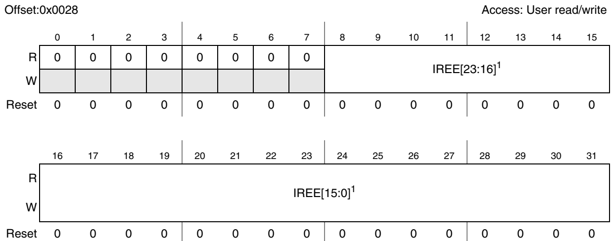
Figure 21-6. Interrupt Rising-Edge Event Enable Register (IREER)
