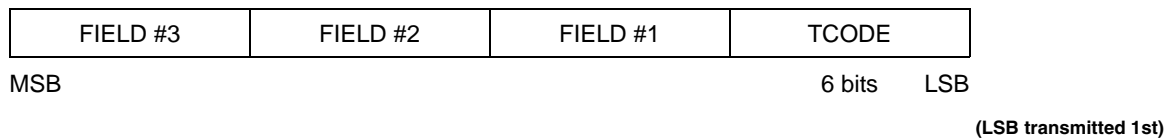
Figure 36-7. Transmission Sequence of Messages
