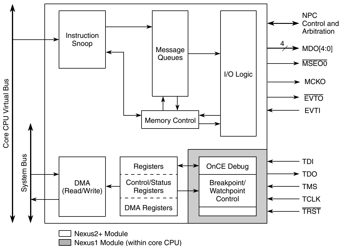
Figure 36-10. e200z0 Nexus2+ Functional Block Diagram
