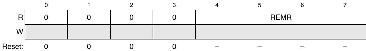
Figure 34-16. Platform RAM ECC Master Number Register (PREMR)
