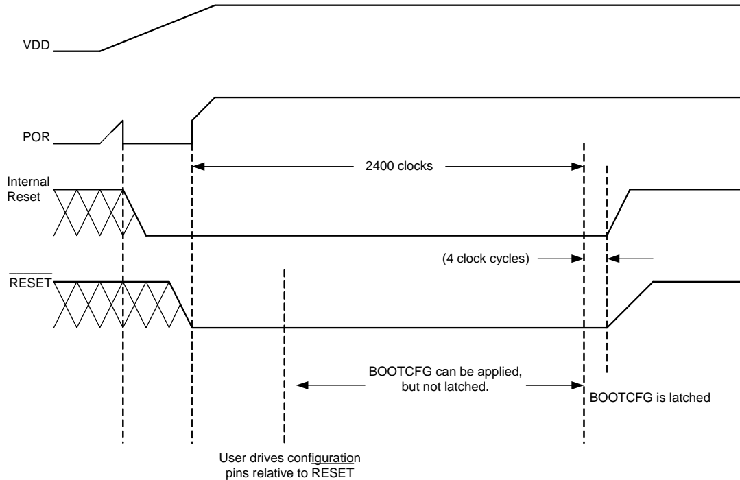
Figure 9-12. Reset configuration timing
