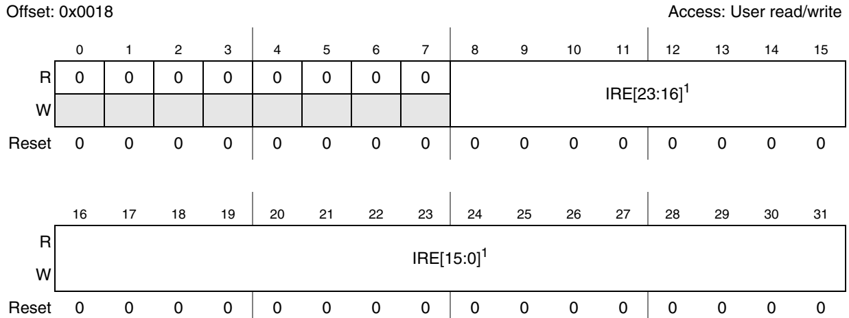
Figure 21-5. Interrupt Request Enable Register (IRER)
