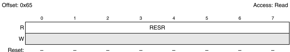
Figure 34-15. Platform RAM ECC Syndrome Register (PRESR)
