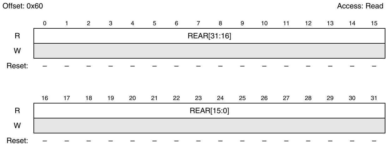
Figure 34-14. Platform RAM ECC Address Register (PREAR)
