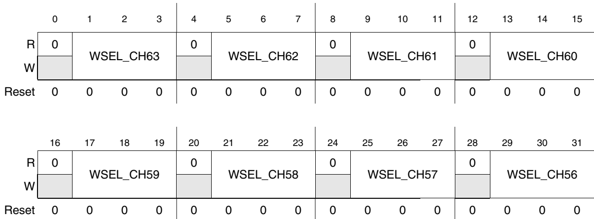
Figure 28-55. Channel Watchdog Select Register 7 (CWSELR7) – ADC_0
