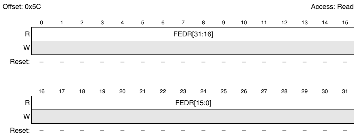
Figure 34-13. Platform Flash ECC Data Register (PFEDR)
