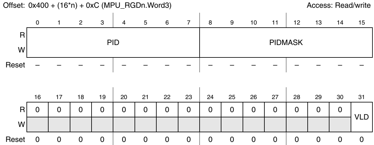
Figure 20-8. MPU Region Descriptor, Word 3 Register (MPU_RGDn.Word3)
