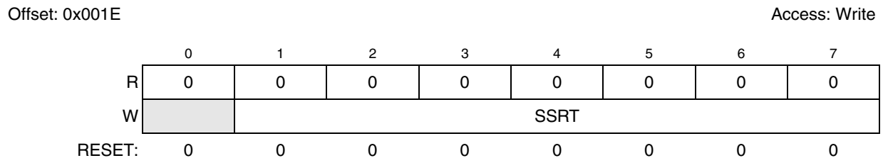
Figure 16-12. DMA Set START Bit (EDMA_SSBR) Register
