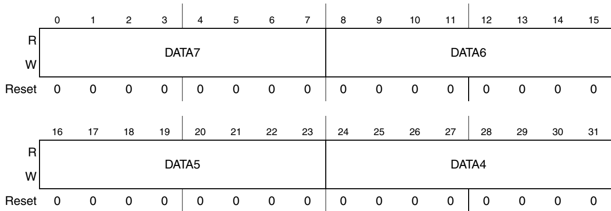
Figure 23-21. Buffer data register MSB (BDRM)
