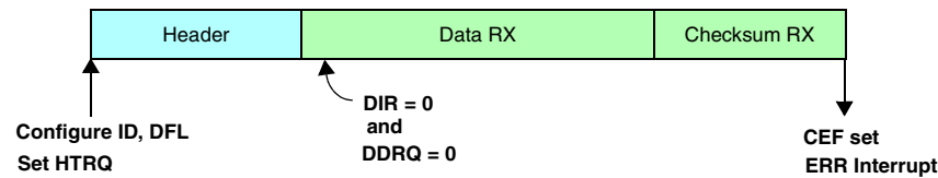
Figure 24-60. Programming consideration: master node, receiver, checksum error
