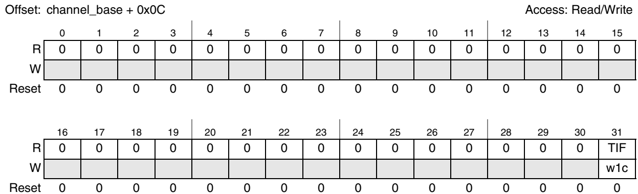
Figure 27-61. Timer Flag Register (TFLG)
