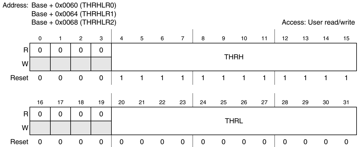
Figure 28-31. ADC_1 Threshold Register THRHLR[0..2]
