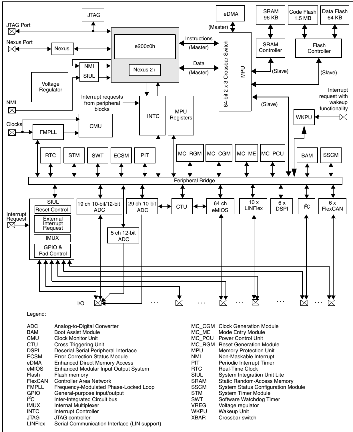
Figure 2. MPC5607B block diagram
