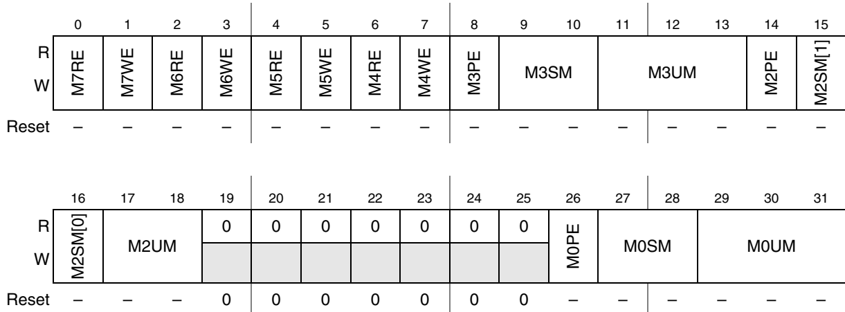
Figure 20-9. MPU RGD Alternate Access Control n (MPU_RGDAACn)
