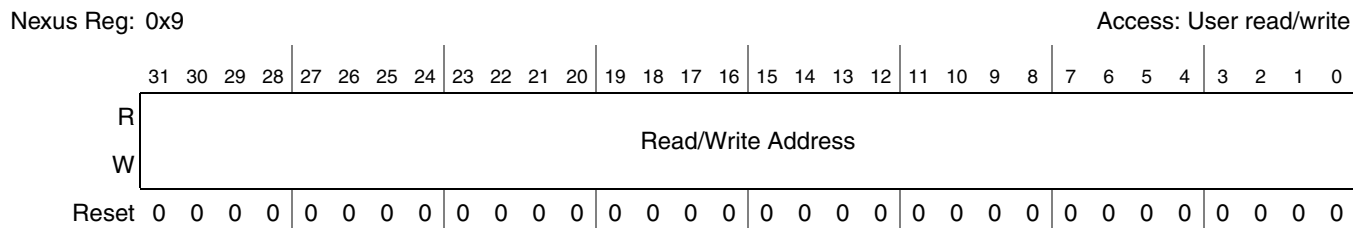
Figure 36-15. Read/Write Access Address Register (RWA)
