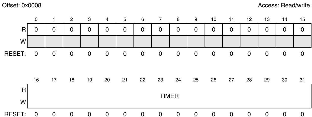
Figure 25-7. Free Running Timer (TIMER)
