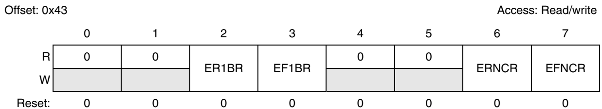
Figure 34-7. ECC Configuration (ECR) Register
