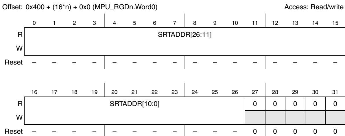
Figure 20-5. MPU Region Descriptor, Word 0 Register (MPU_RGDn.Word0)
