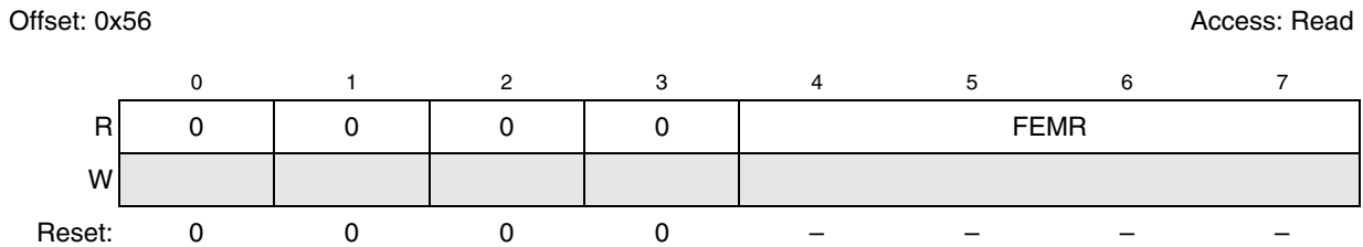
Figure 34-11. Platform Flash ECC Master Number Register (PFEMR)
