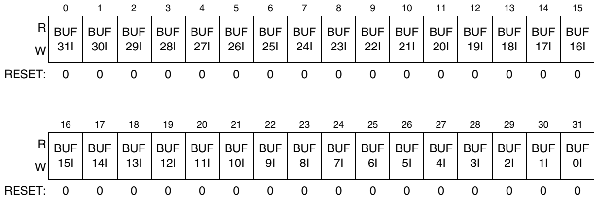
Figure 25-14. Interrupt Flags 1 Register (IFLAG1)
