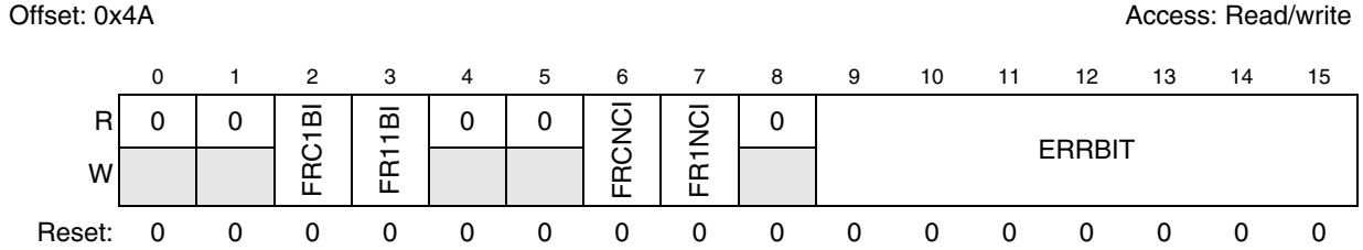
Figure 34-9. ECC Error Generation Register (EEGR)
