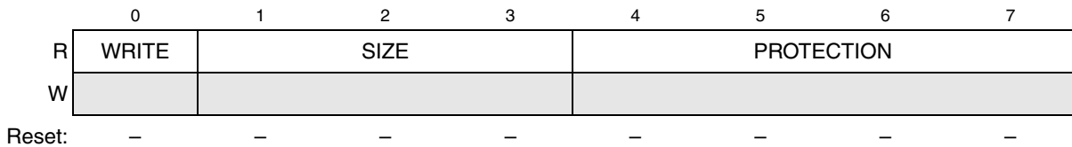
Figure 34-17. Platform RAM ECC Attributes Register (PREAT)
