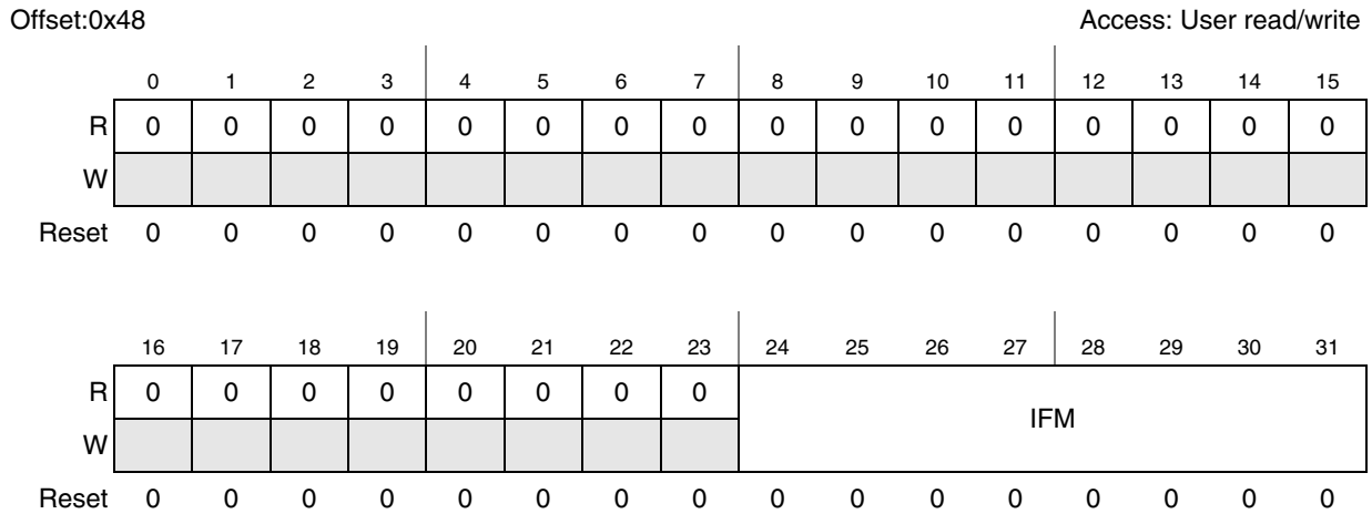
Figure 24-36. Identifier filter mode register (IFMR)
