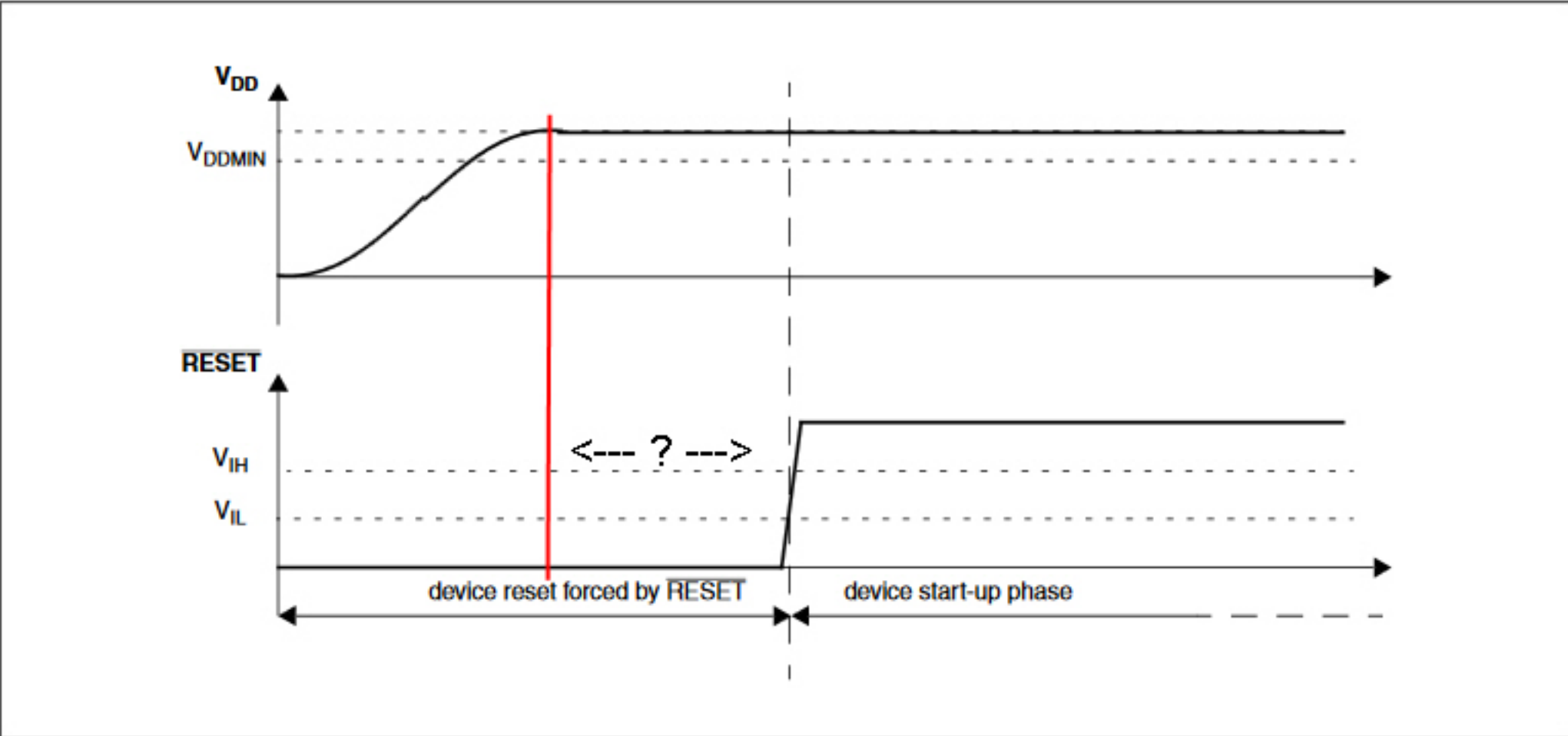
Figure 8. Start-up reset requirements
