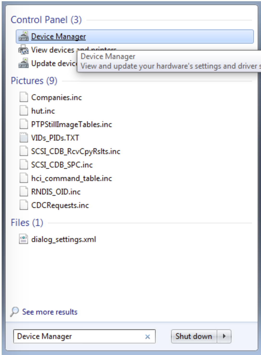
Figure 41. Device Manager
