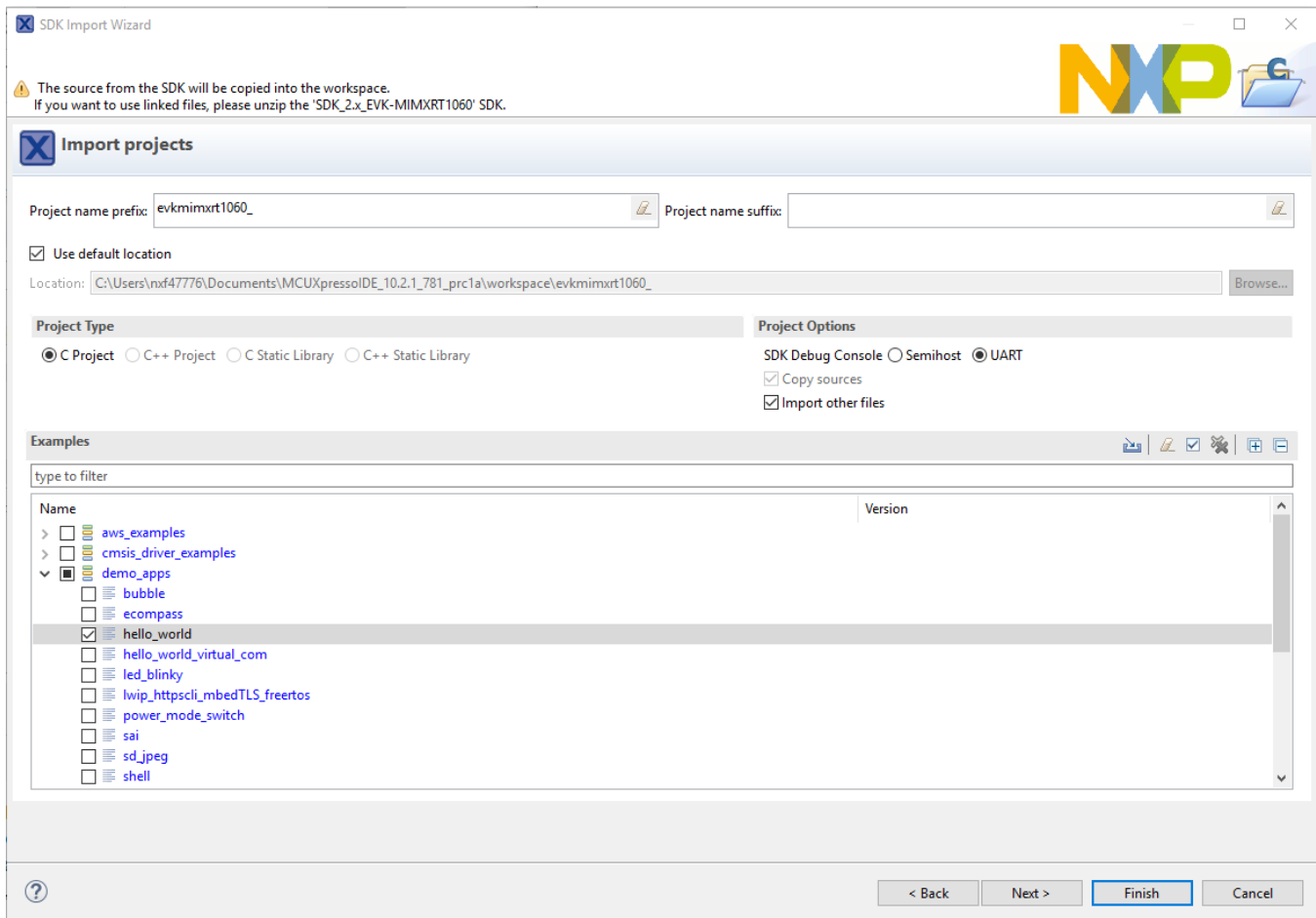
Figure 30. Select "hello_world"
