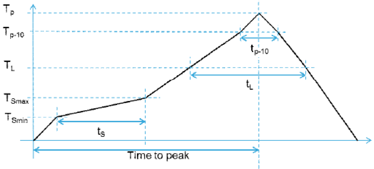
Figure 34. Solder profile
