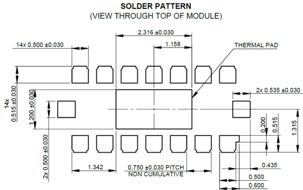
Figure 35. Recommended solder pattern
