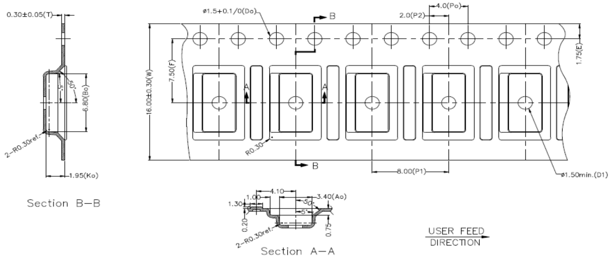
Figure 33. VL53L8CX tape and reel packaging drawing
