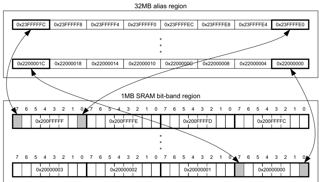
Figure 2-1 Bit-band mapping
