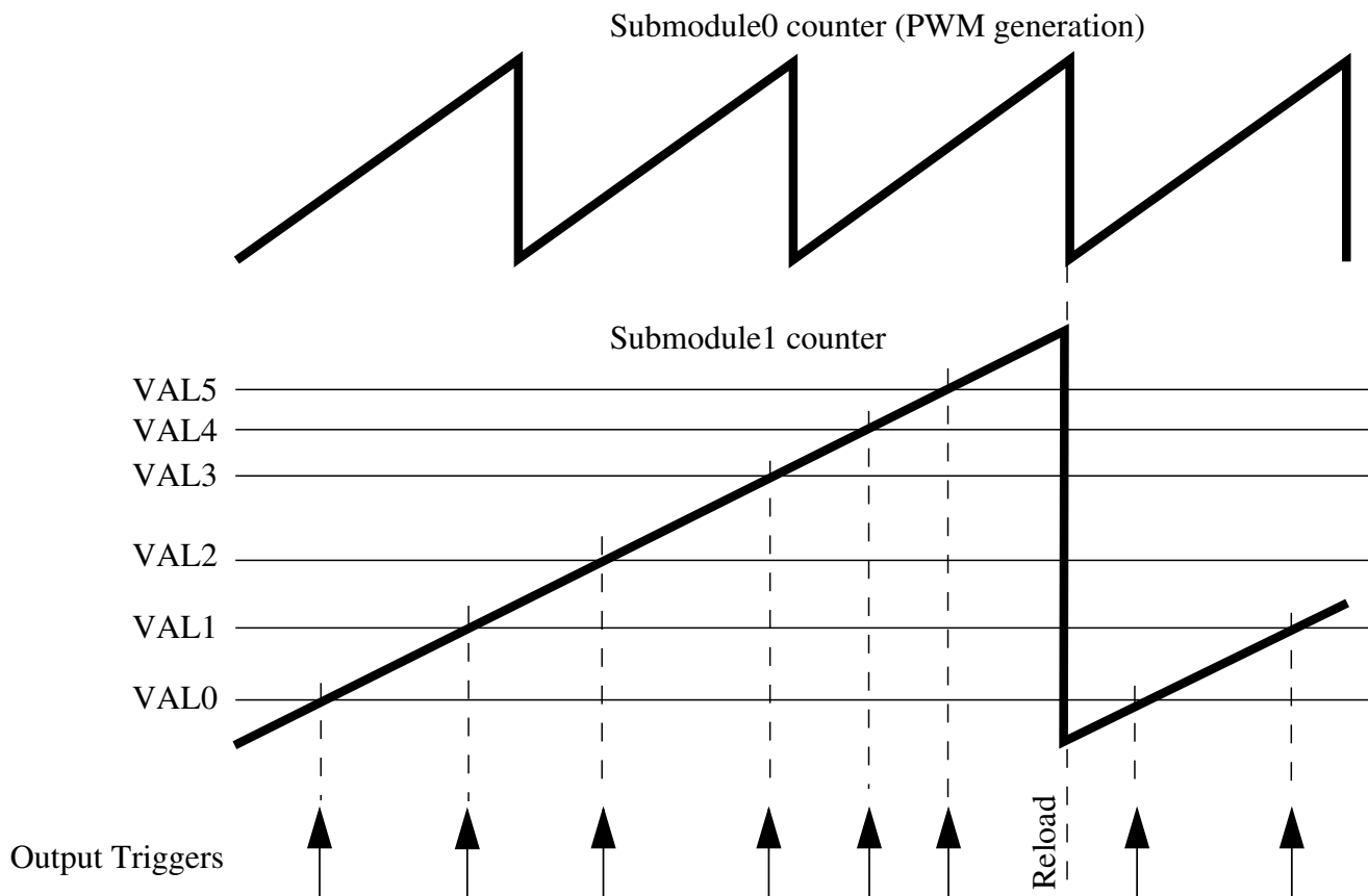
Figure 28-211. Multiple Output Triggers Over Several PWM Cycles
