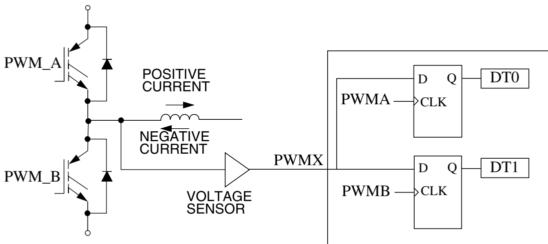
Figure 28-226. Current-status Sense Scheme for Deadtime Correction
