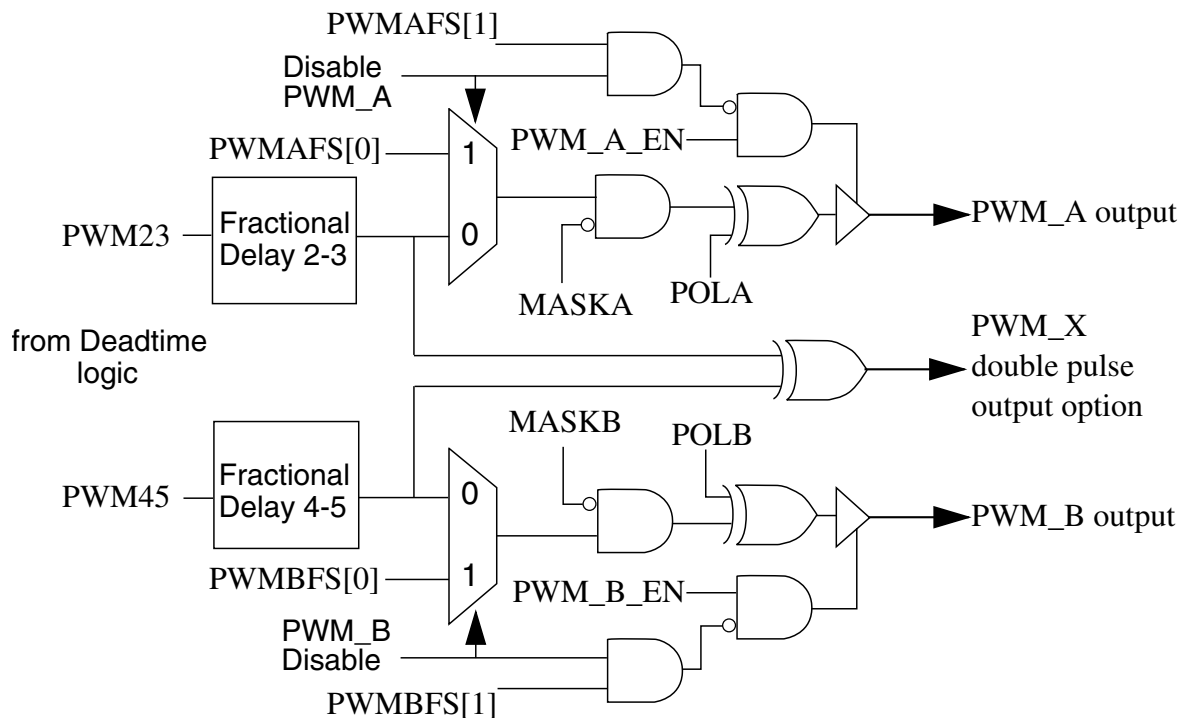
Figure 28-228. Fractional Delay and Output Logic Section
