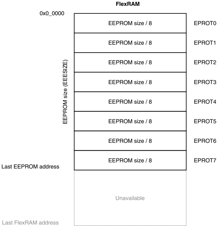
Figure 20-28. EEPROM protection
