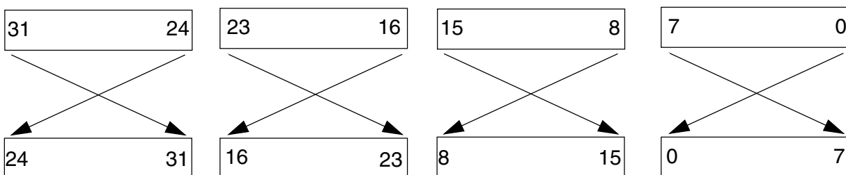
Figure 23-5. Transpose type 01
