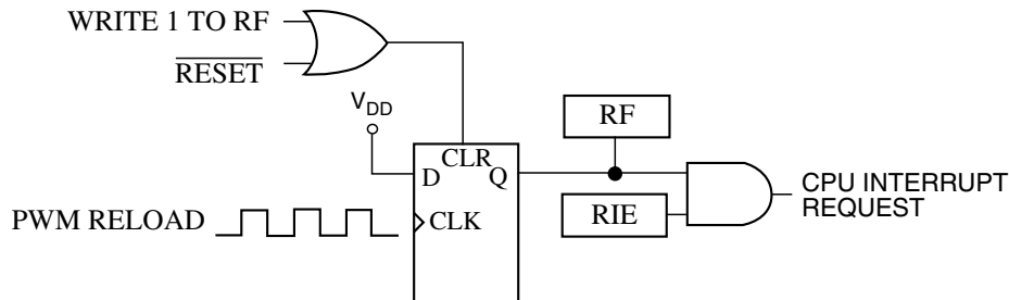
Figure 28-237. PWMF Reload Interrupt Request
