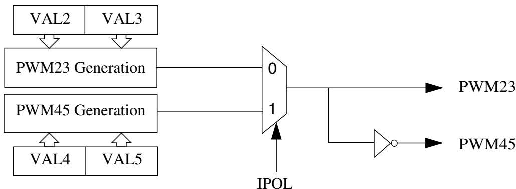
Figure 28-221. Complementary Channel Pair
