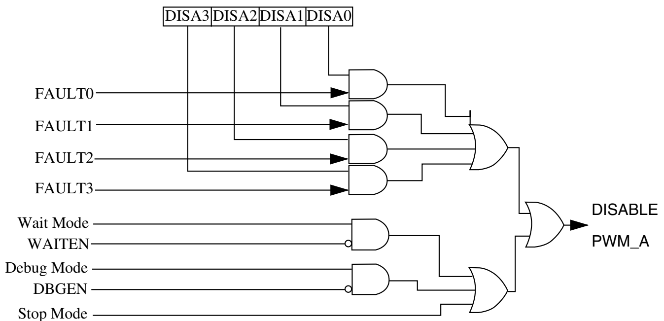
Figure 28-230. Fault Decoder for PWM_A
