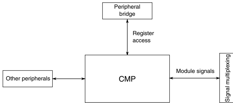
Figure 3-16. CMP Configuration
