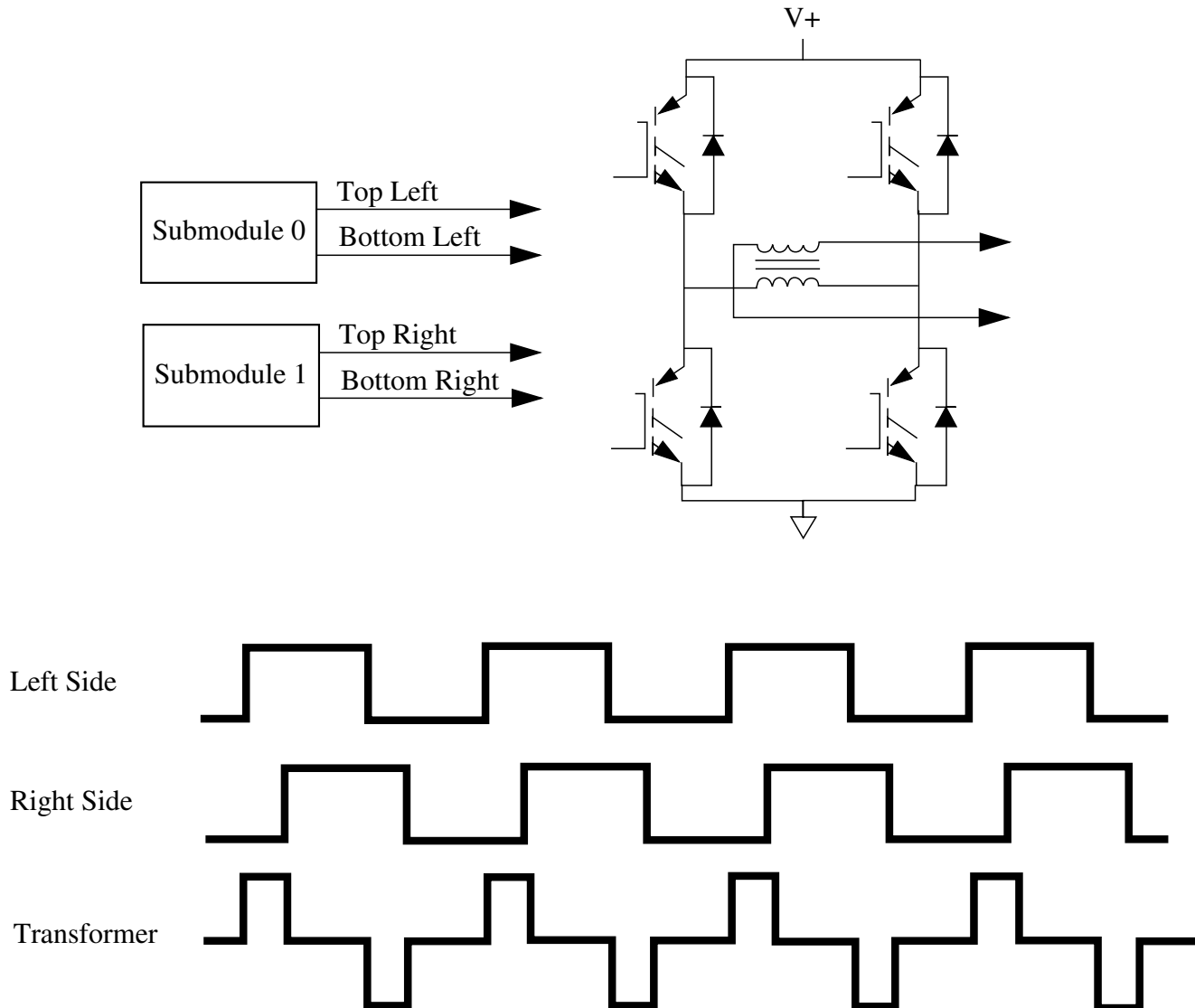
Figure 28-208. Phase Shifted PWMs Applied to a Transformer Primary
