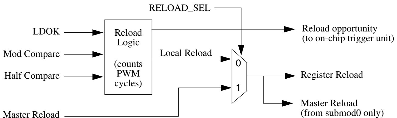
Figure 28-217. Register Reload Logic
