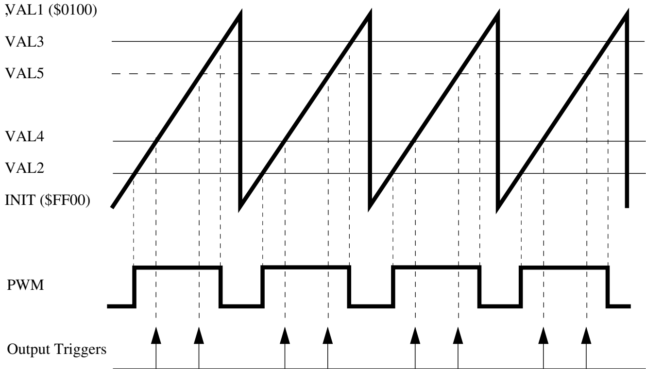
Figure 28-210. Multiple Output Trigger Generation in Hardware
