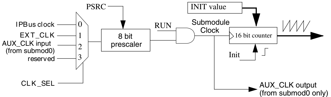
Figure 28-216. Clocking Block Diagram for Each PWM Submodule
