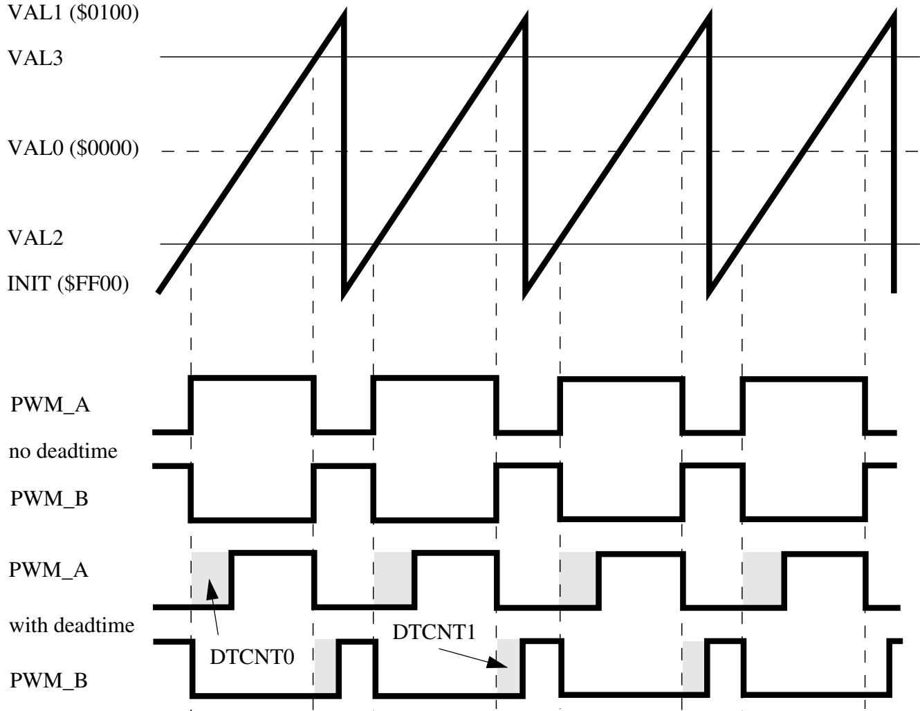
Figure 28-224. Deadtime Insertion
