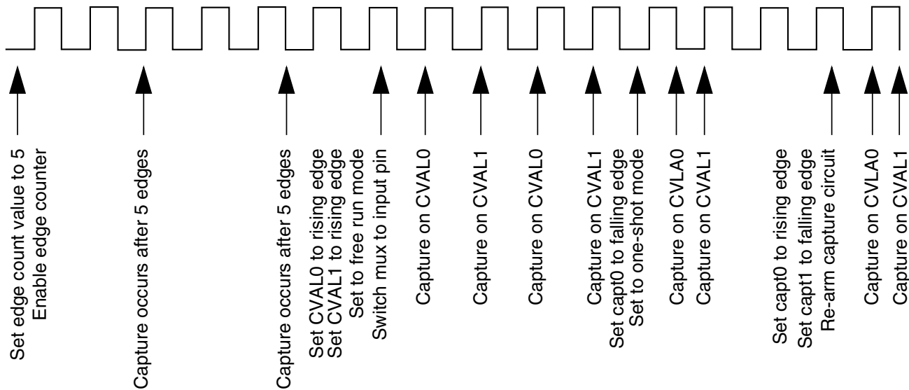
Figure 28-212. Capture Capabilities of the E-Capture Circuit
