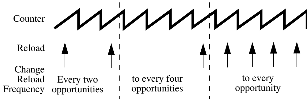
Figure 28-235. Half Cycle Reload Frequency Change
