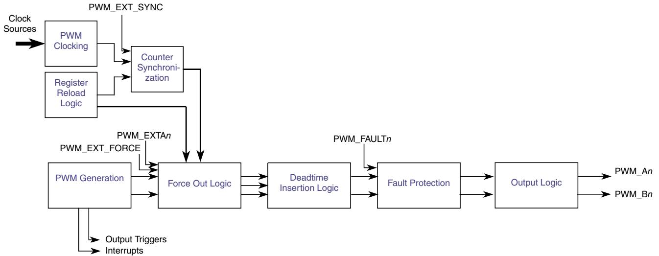
Figure 28-215. High-Level Output PWM Generation Block Diagram
