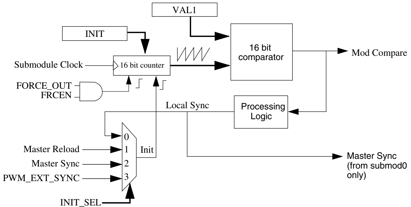
Figure 28-218. Submodule Timer Synchronization
