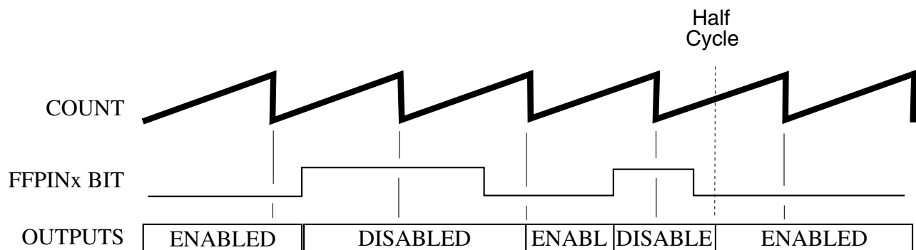
Figure 28-231. Automatic Fault Clearing
