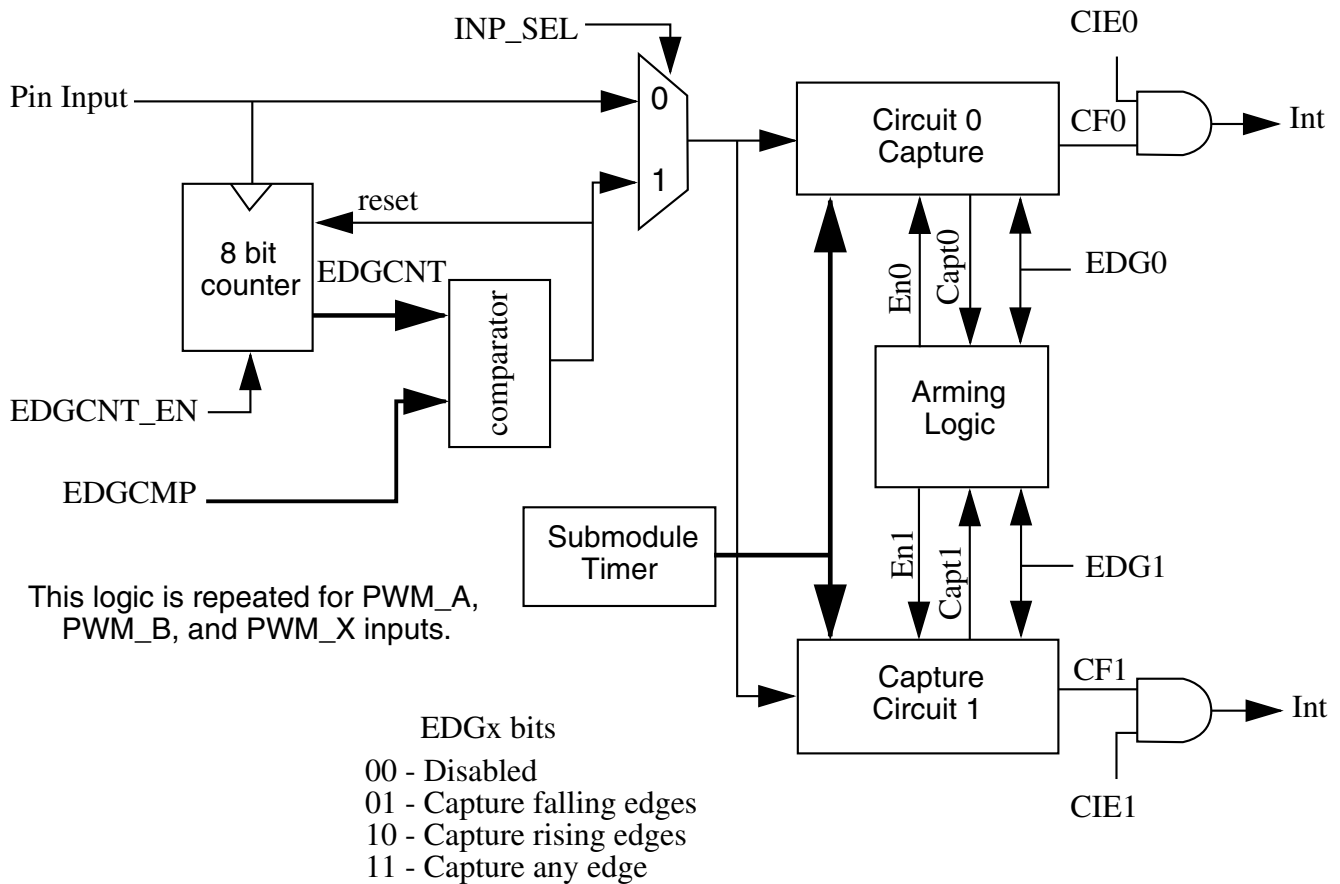
Figure 28-229. Enhanced Capture (E-Capture) Logic
