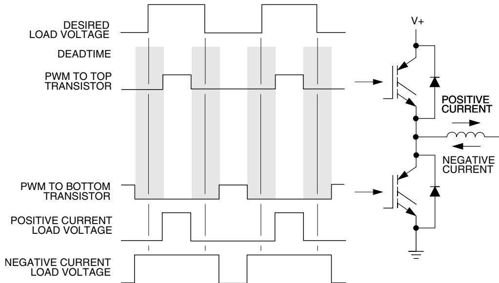
Figure 28-225. Deadtime Distortion
