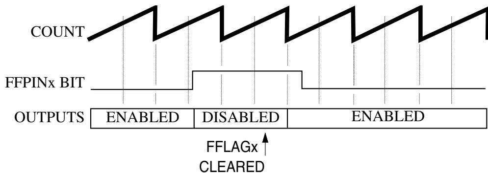
Figure 28-233. Manual Fault Clearing (FCTRL[FSAFE]=1)
