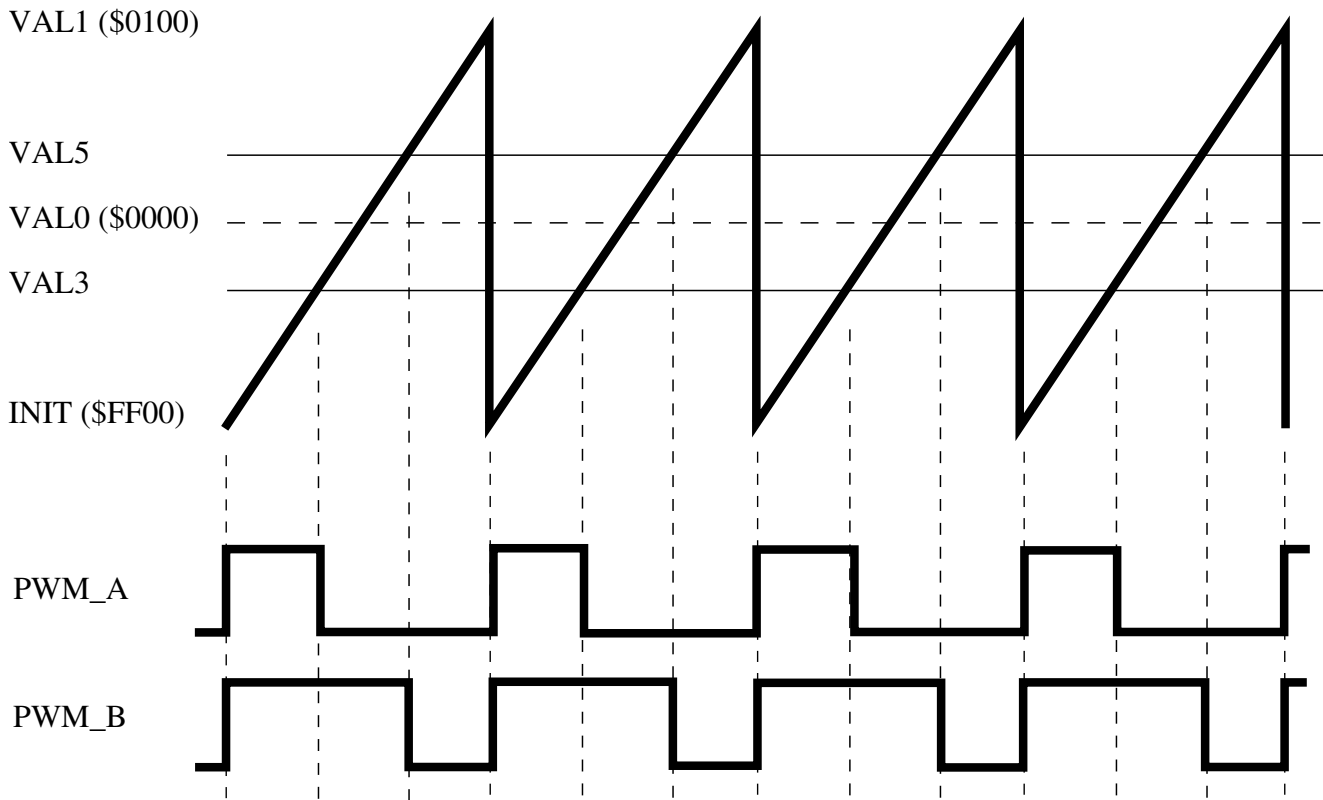
Figure 28-206. Edge Aligned Example (INIT=VAL2=VAL4)
