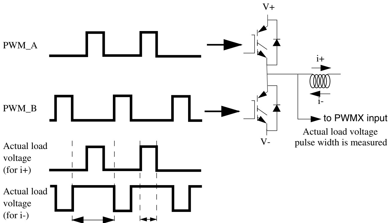
Figure 28-213. Output Pulse Width Measurement Possible with the E-Capture Circuit
