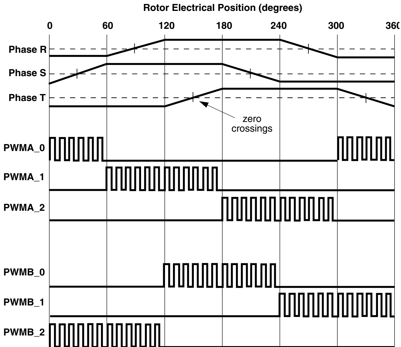
Figure 28-214. Sensorless BLDC Commutation Using the Force Out Function
