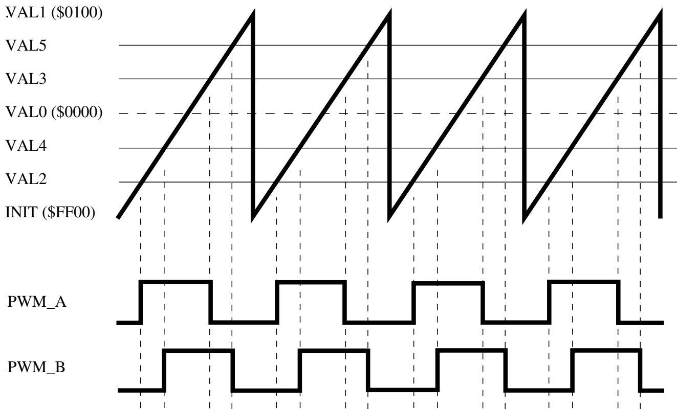
Figure 28-207. Phase Shifted Outputs Example
