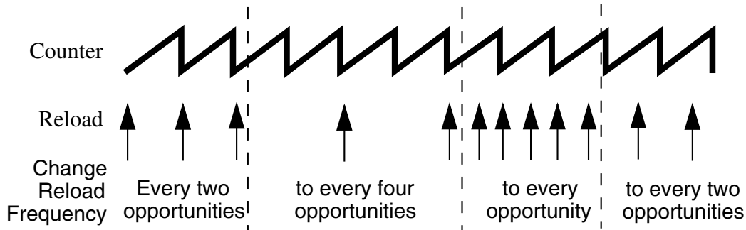
Figure 28-236. Full and Half Cycle Reload Frequency Change
