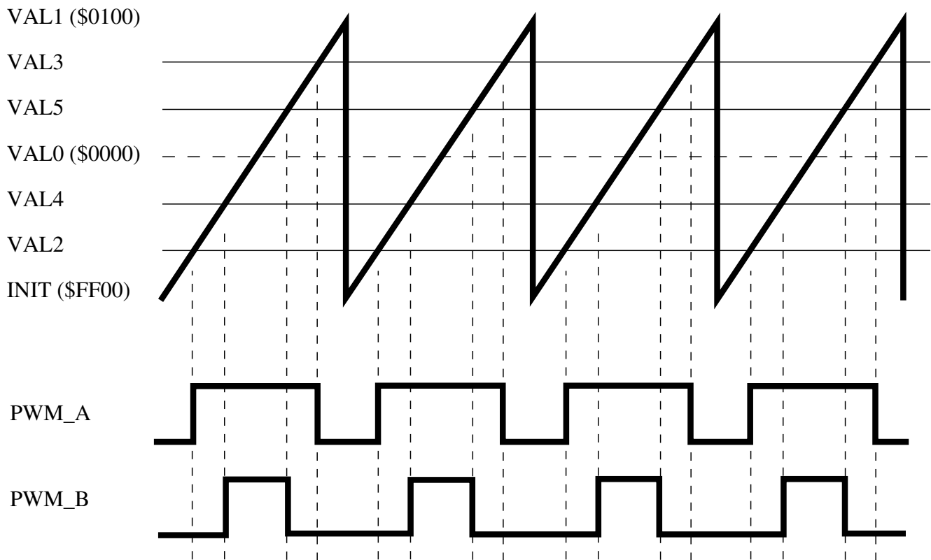
Figure 28-205. Center Aligned Example
