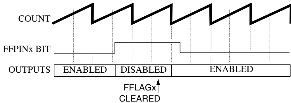
Figure 28-232. Manual Fault Clearing (FCTRL[FSAFE]=0)
