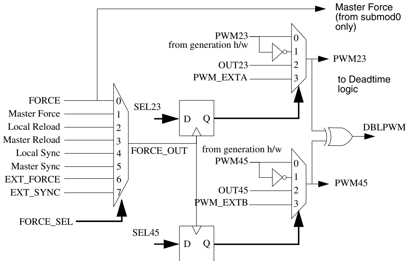
Figure 28-220. Force Out Logic
