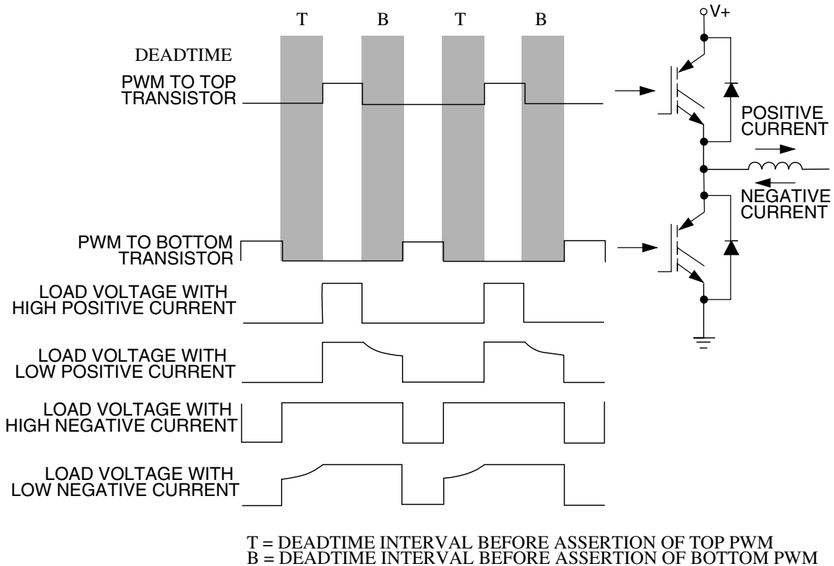
Figure 28-227. Output Voltage Waveforms
