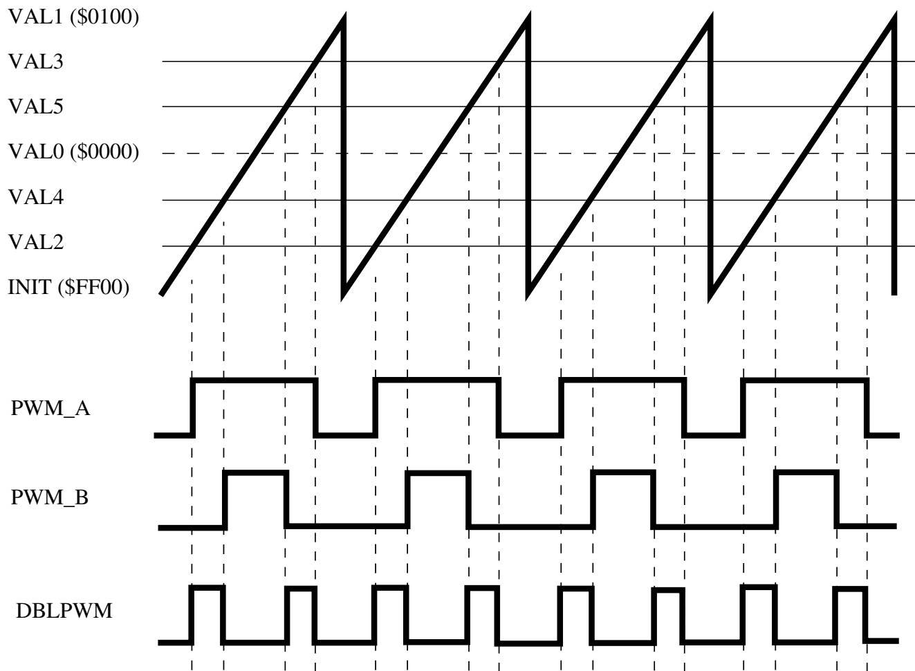
Figure 28-209. Double Switching Output Example
