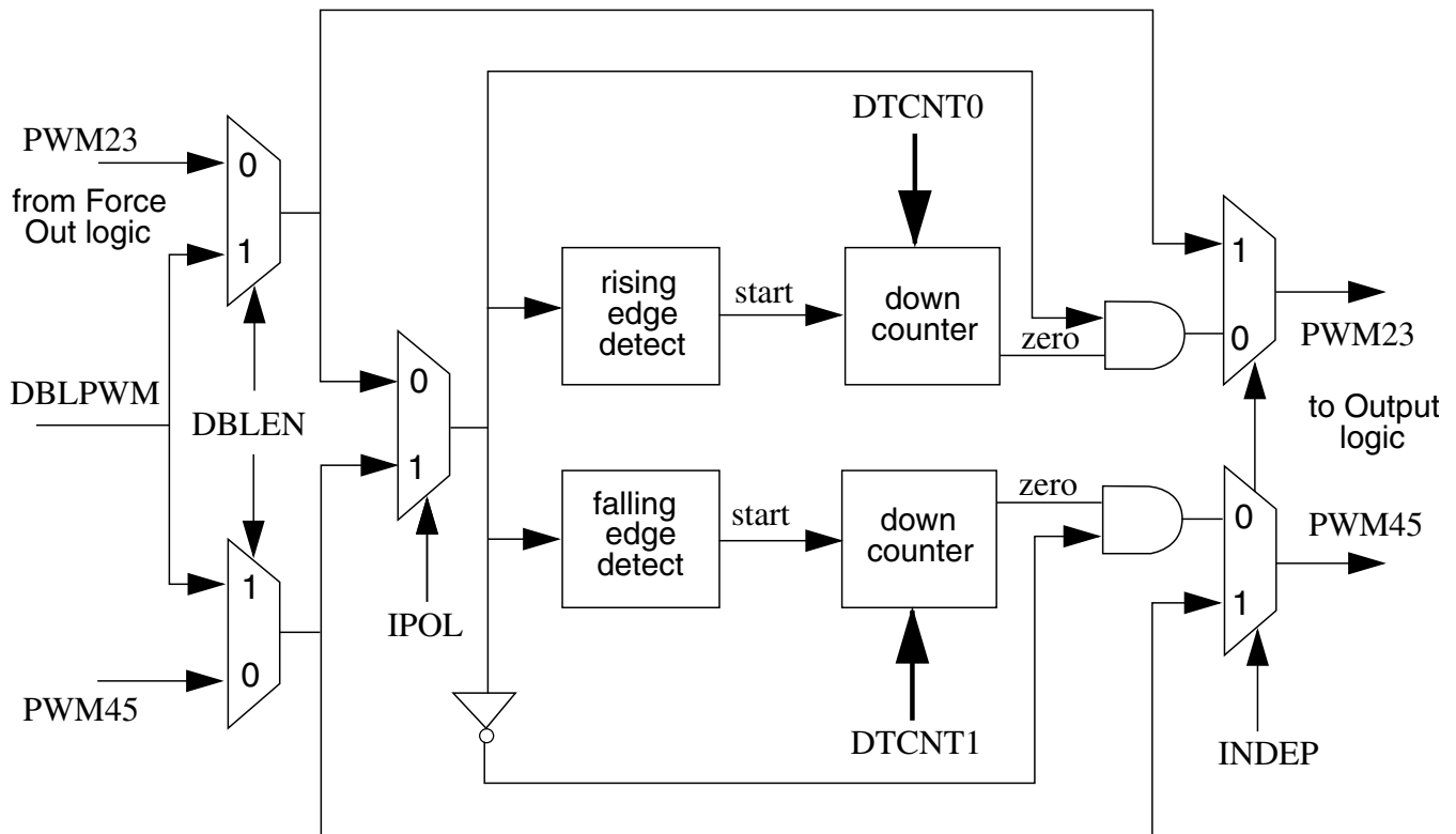
Figure 28-223. Deadtime Insertion Logic
