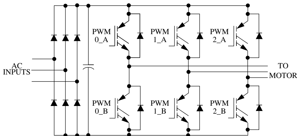
Figure 28-222. Typical 3 Phase AC Motor Drive
