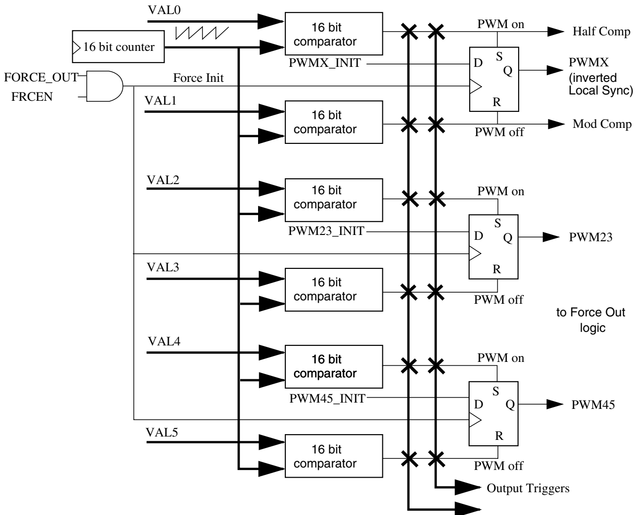
Figure 28-219. PWM Generation Hardware
