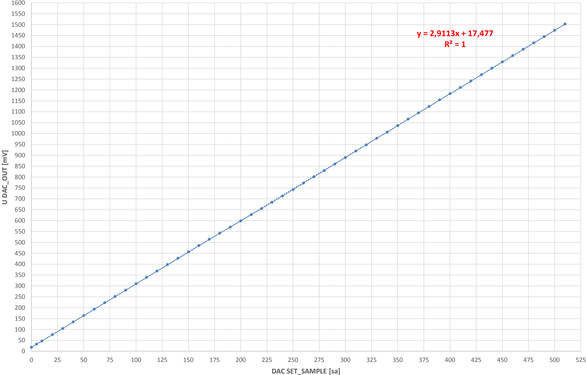
DAC SET_SAMPLE [sa] vs. U DAC_OUT [mV]
