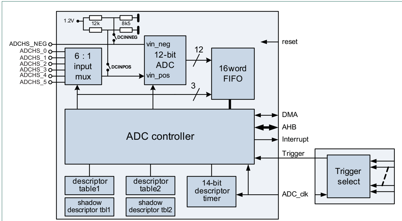
Fig 182. ADCHS block diagram
