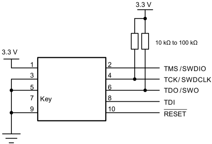
Fig 180. Cortex Debug Connector
