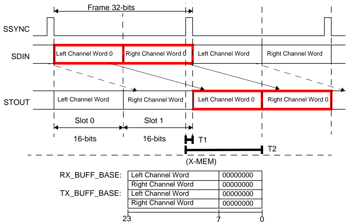
Figure 7. Codec Data Format and Layout in Memory
