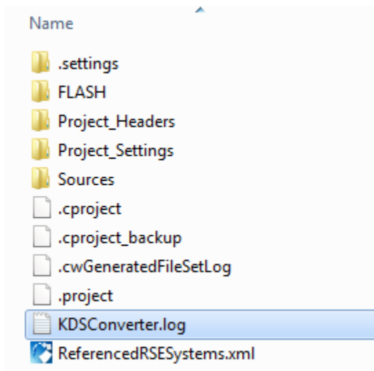
Figure 9. Conversion log
