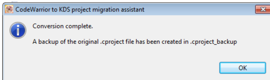
Figure 8. Conversion completed
