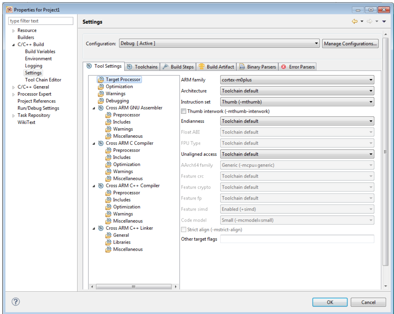
Figure 14. Build settings
