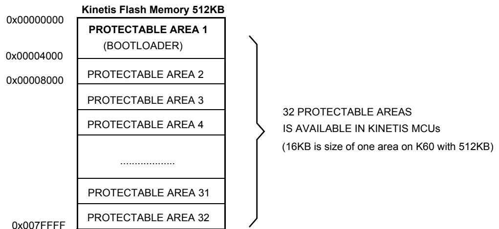
Figure 24. System of flash memory protection in Kinetis MCUs
