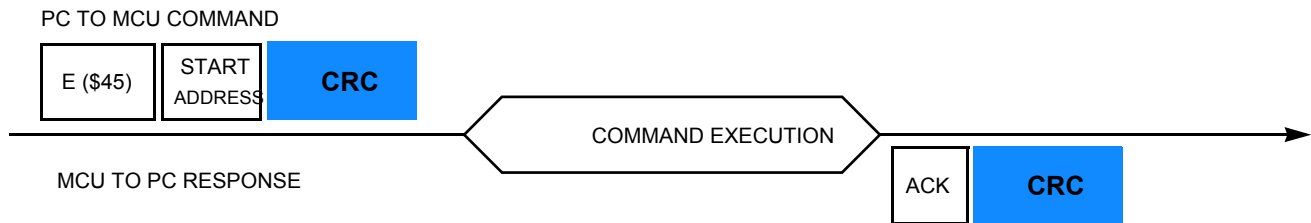
Figure 10. Erase command
