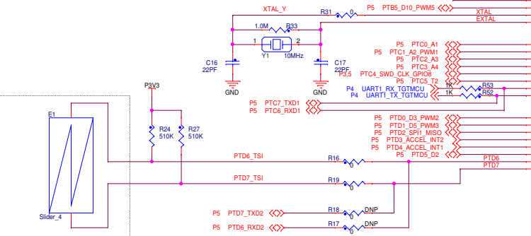
TSI CAPACITIVE/TOUCH INTERFACE
