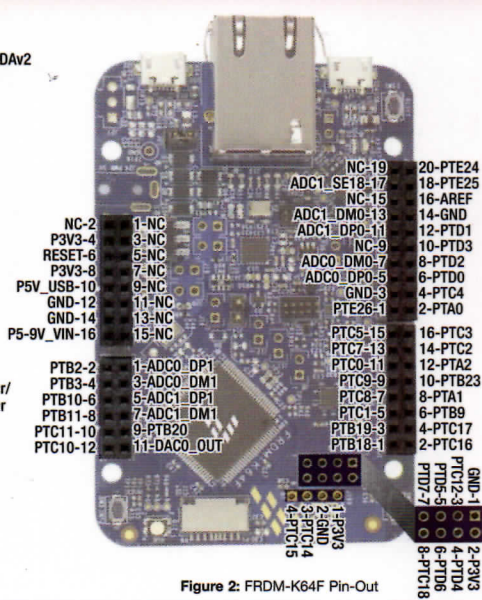
Figure 2: FRDM-K64F Pin-Out
