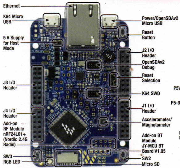
Figure 1: FRDM-K64F Callouts
