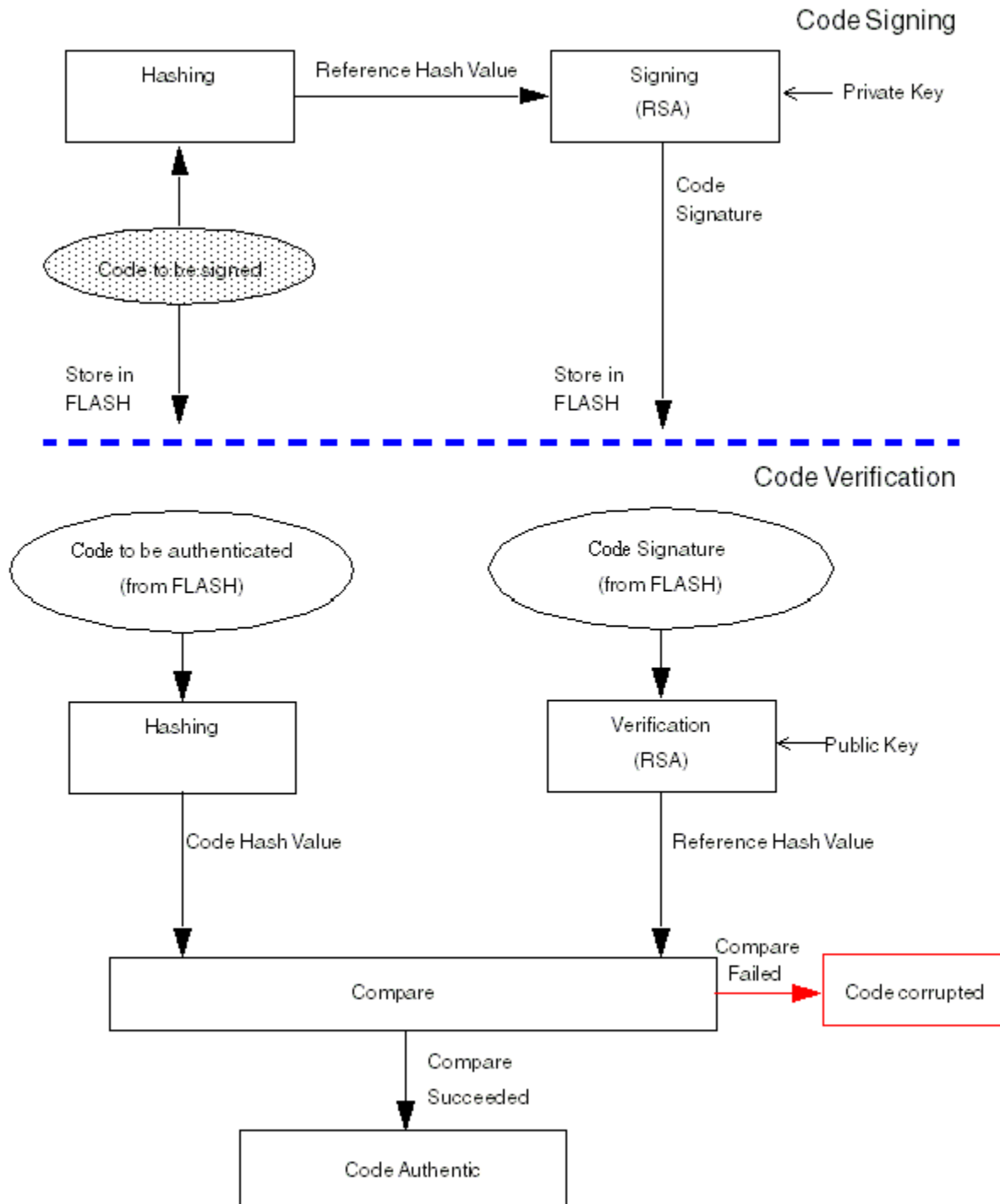
Figure 11-2. Code signing and authentication processes
