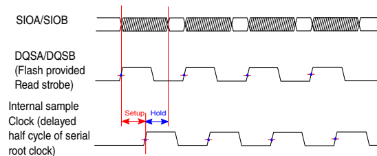
Figure 30-33. Input Timing 2 for Flash provided read strobe in SDR mode
