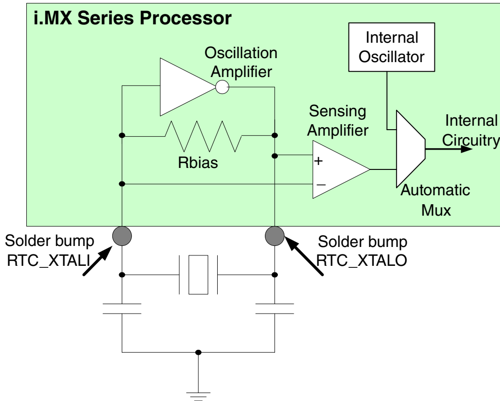
Figure 62-2. Oscillator Configuration (32 kHz)
