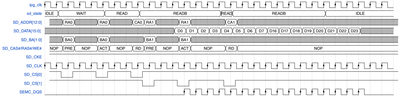
Figure 49-13. AXI command - Pipelined SDRAM Read
