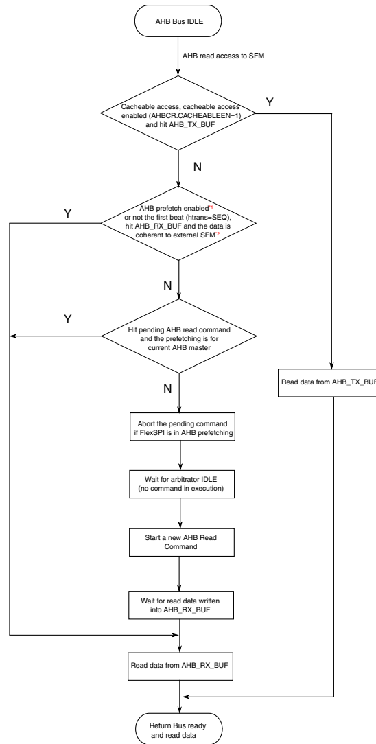
Figure 30-21. Hardware operation in response to AHB read access to Flash
