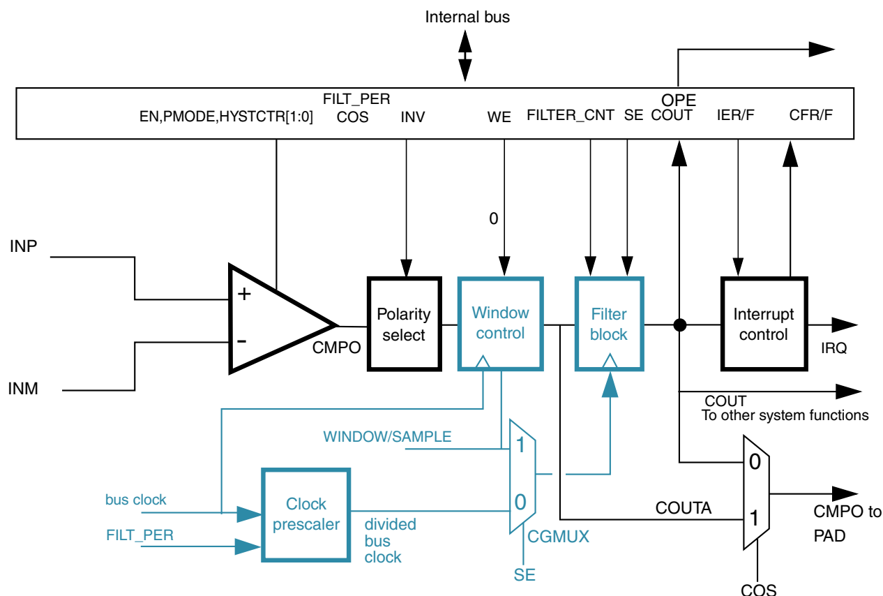
Figure 13-3. Comparator operation in Continuous mode
