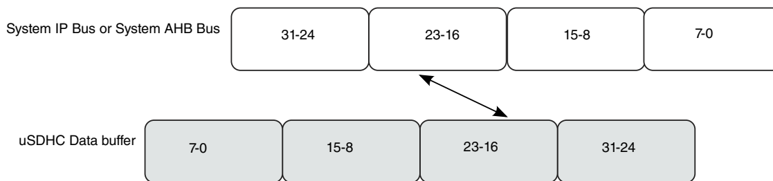
Figure 57-4. Data Swap between System Bus and uSDHC Data Buffer in Byte Little Endian Mode
