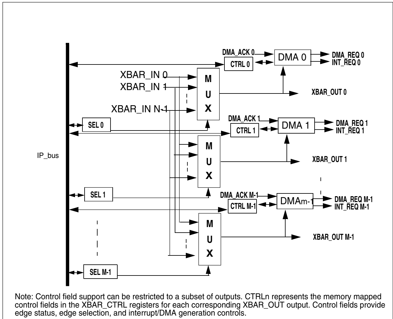
Figure 60-2. XBAR Block Diagram
