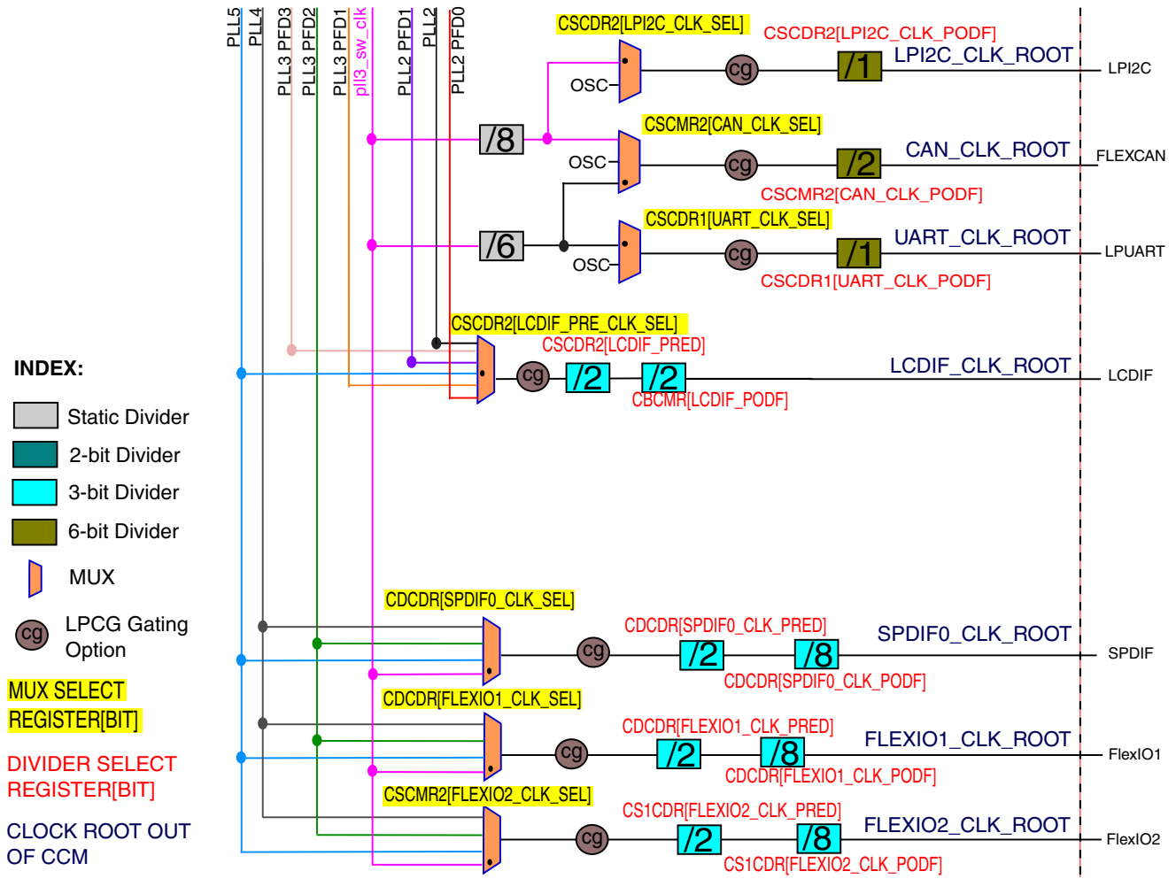
Figure 18-3. Clock Tree - Part 2
