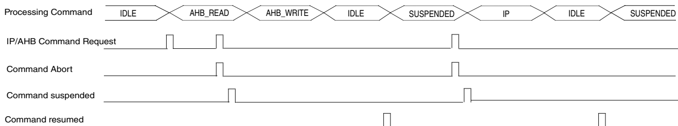
Figure 30-22. Command Instructions Execution on FlexSPI interface
