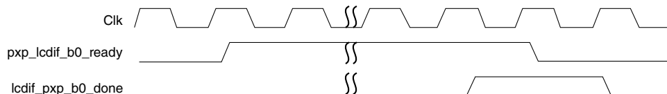
Figure 46-16. Buffer Sharing Protocol
