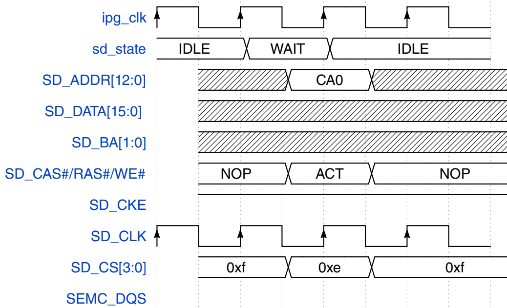
Figure 49-8. IP command - SDRAM PRECHARGE ALL
