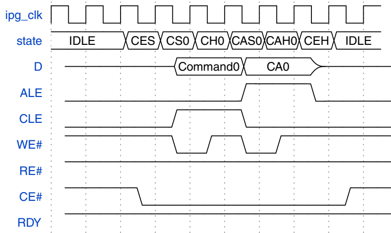
Figure 49-36. NAND Flash access command type - Command + Address Phase
