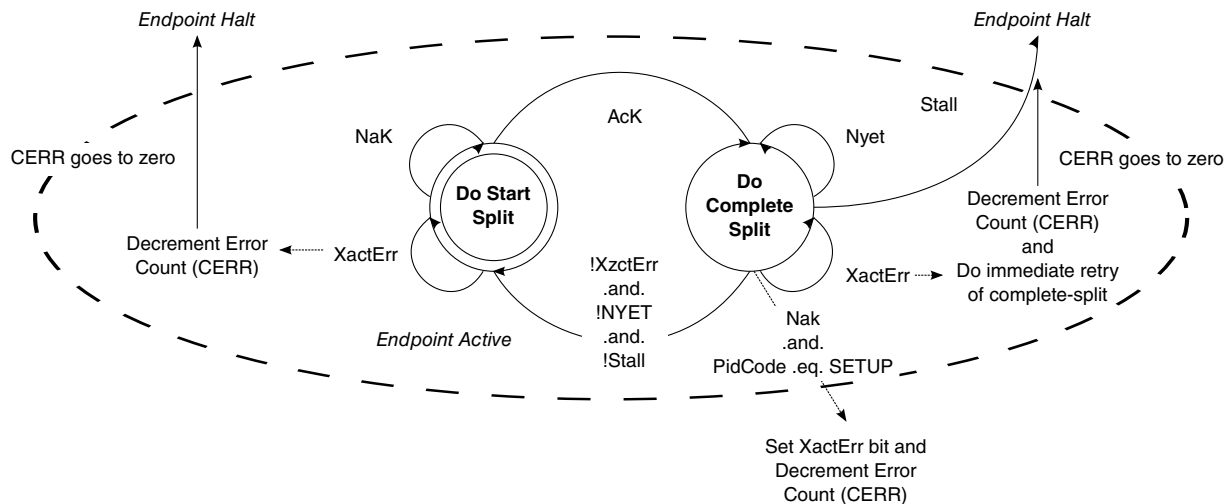
Figure 55-19. Host Controller Asynchronous Schedule Split-Transaction State Machine
