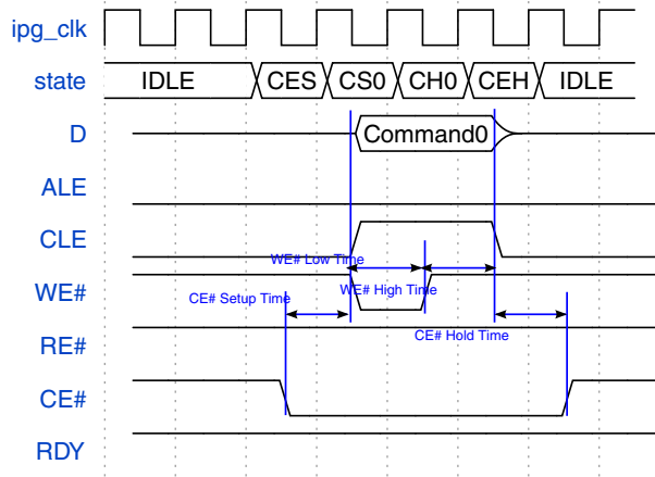
Figure 49-34. NAND Flash access command type - Command Phase Only
