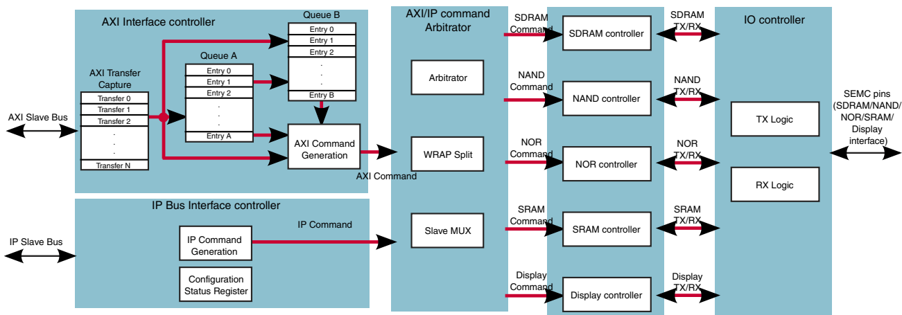
Figure 49-1. SEMC block diagram
