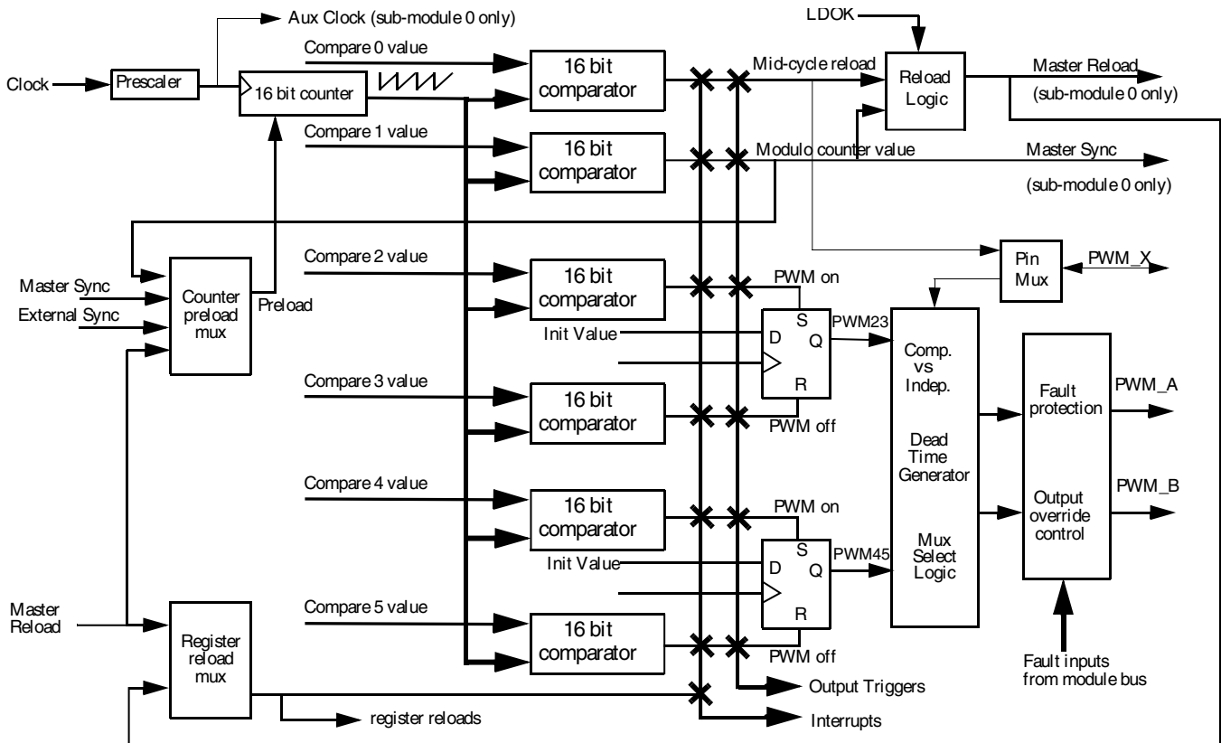
Figure 28-1. PWM Submodule Block Diagram
