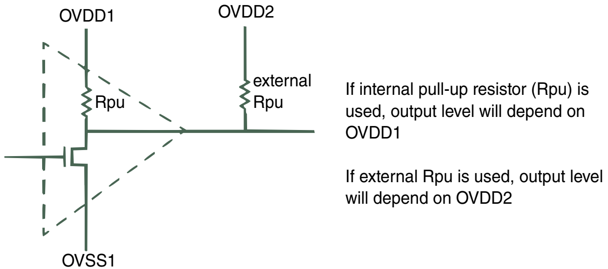
Figure 32-8. Output buffer in open drain mode
