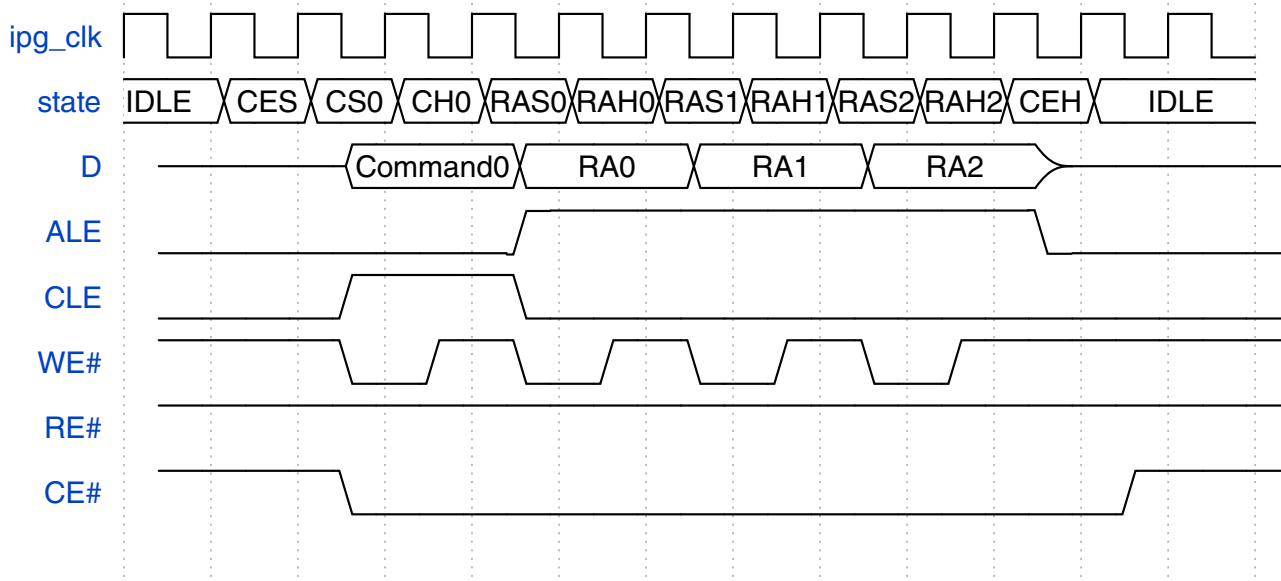
Figure 49-32. NAND Flash access Address type - Three Byte Row Address
