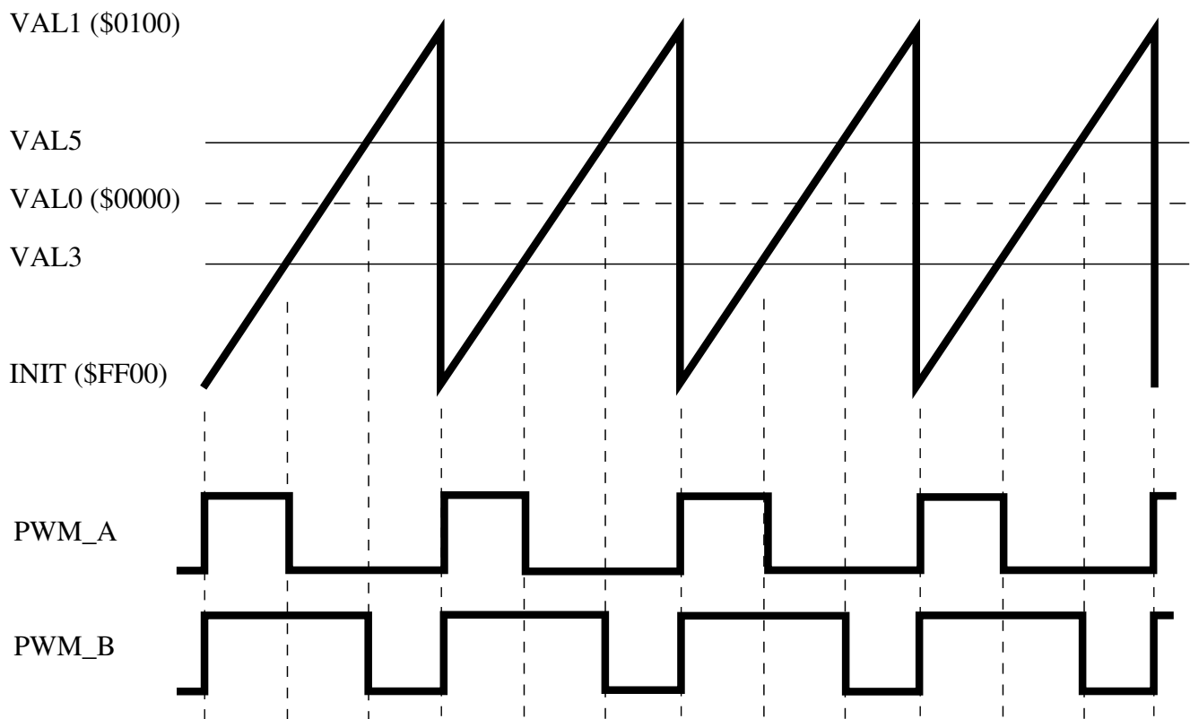
Figure 28-3. Edge Aligned Example (INIT=VAL2=VAL4)
