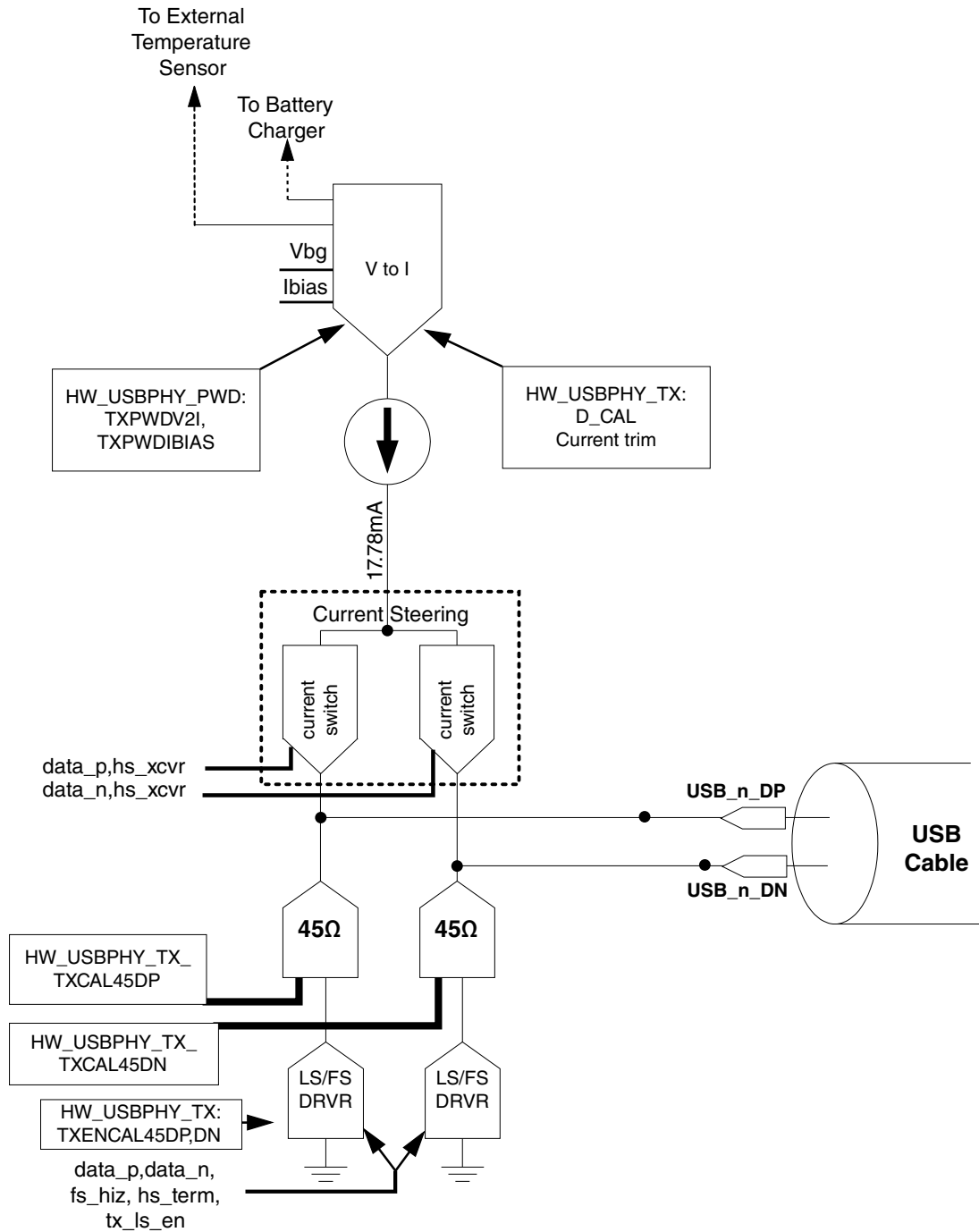
Figure 56-2. USB 2.0 PHY Transmitter Block Diagram
