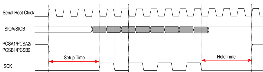
Figure 30-27. Chip selection output timing for DDR sequence
