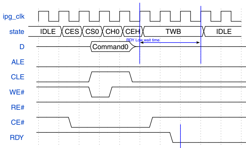
Figure 49-35. NAND Flash access command type - Command + Wait Phase
