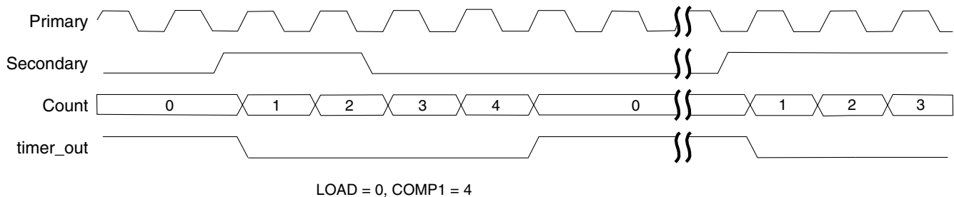
Figure 47-6. One-Shot Mode (CTRL[LENGTH]=1)
