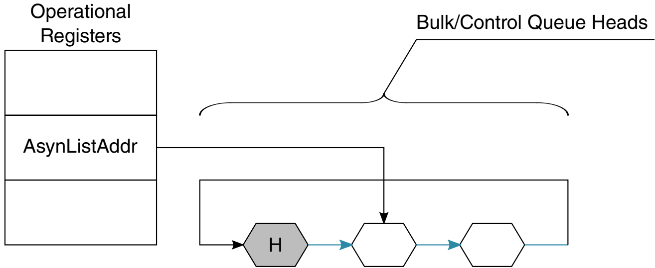
Figure 55-3. Asynchronous Schedule Organization
