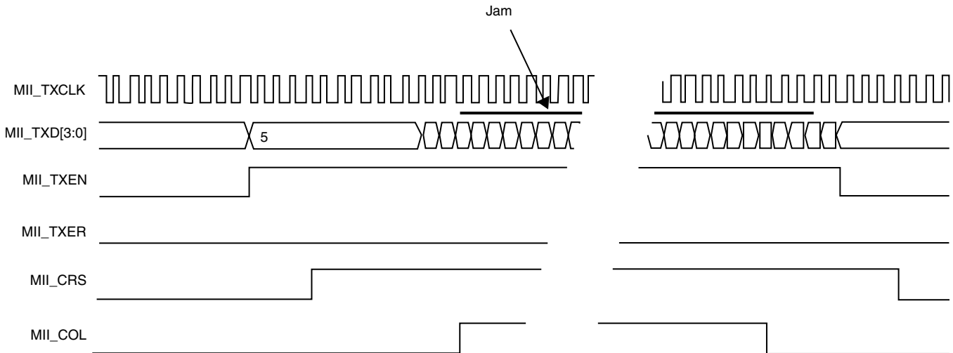
Figure 24-24. MII transmit operation — transmission with collision
