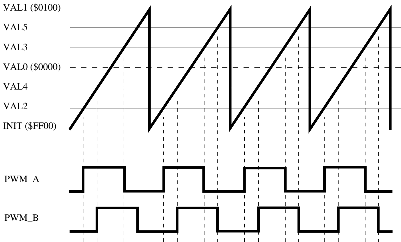
Figure 28-4. Phase Shifted Outputs Example
