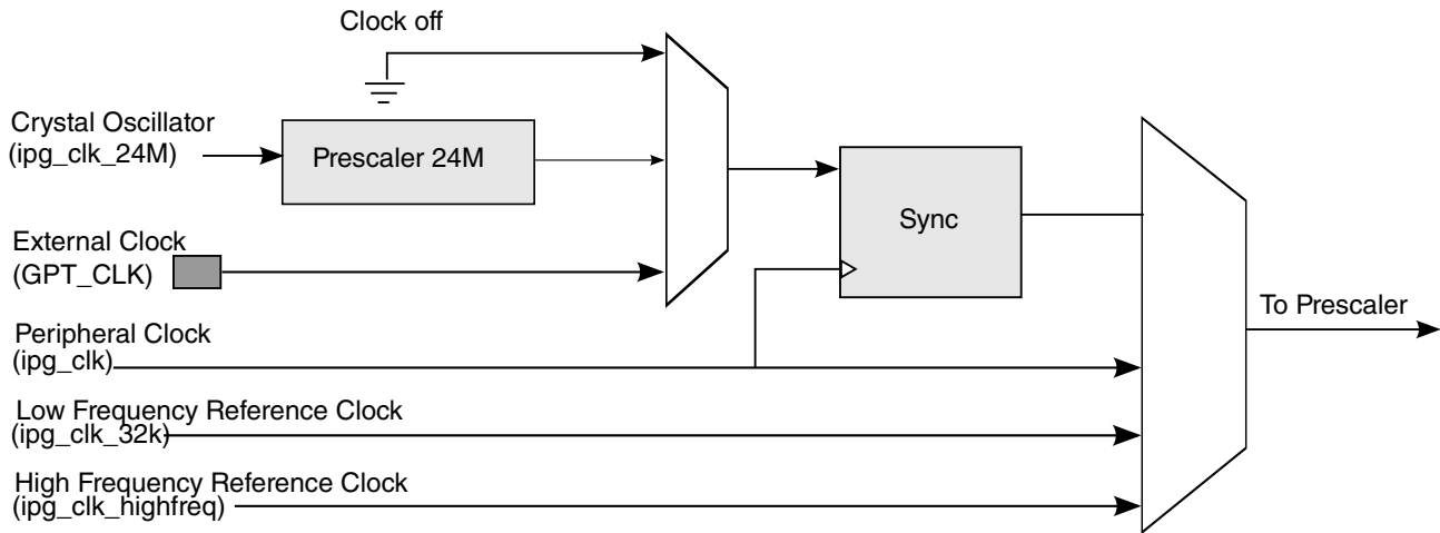
Figure 33-2. GPT Counter Clocks Diagram
