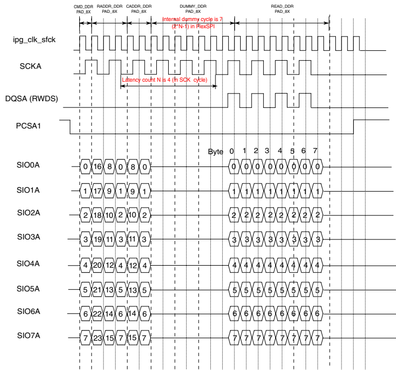
Figure 30-9. HyperBus device read transaction with single latency count
