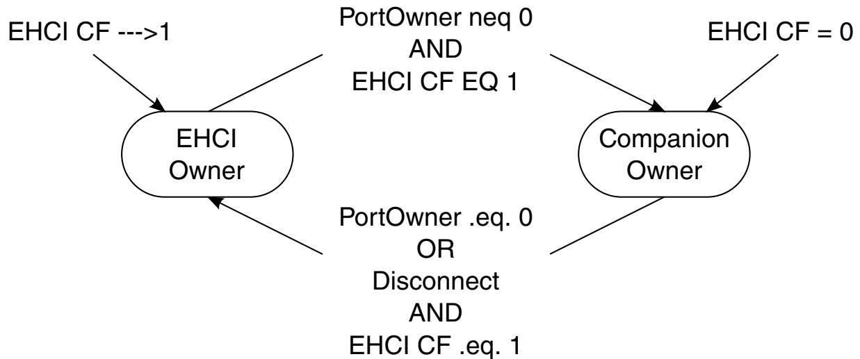
Figure 55-5. Port Owner Handoff State Machine
