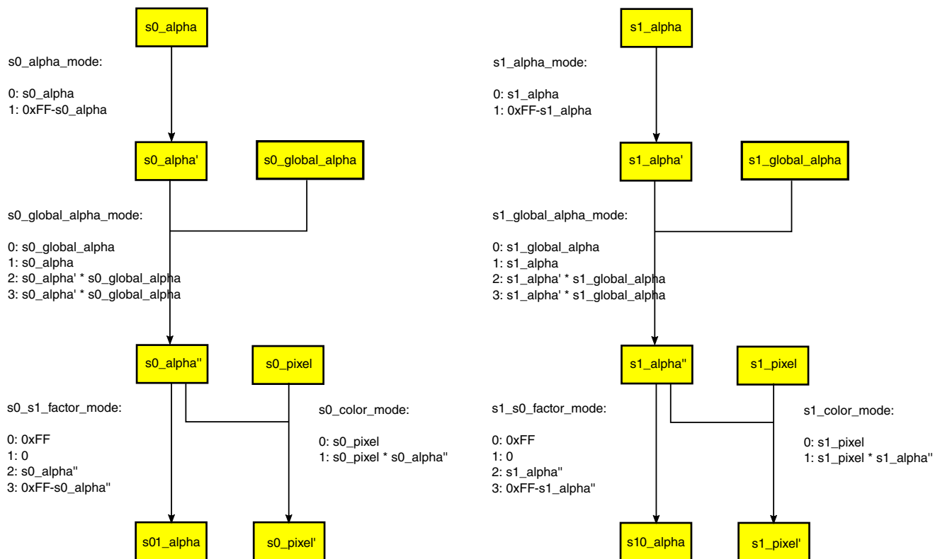
Figure 46-9. Porter-Duff Alpha Blend
