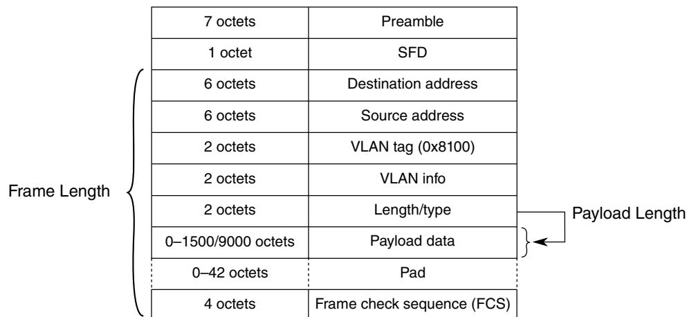
Figure 24-3. VLAN-tagged MAC frame format overview
