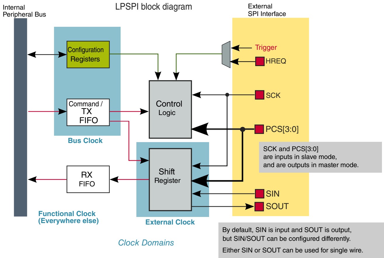
Figure 38-1. Block Diagram
