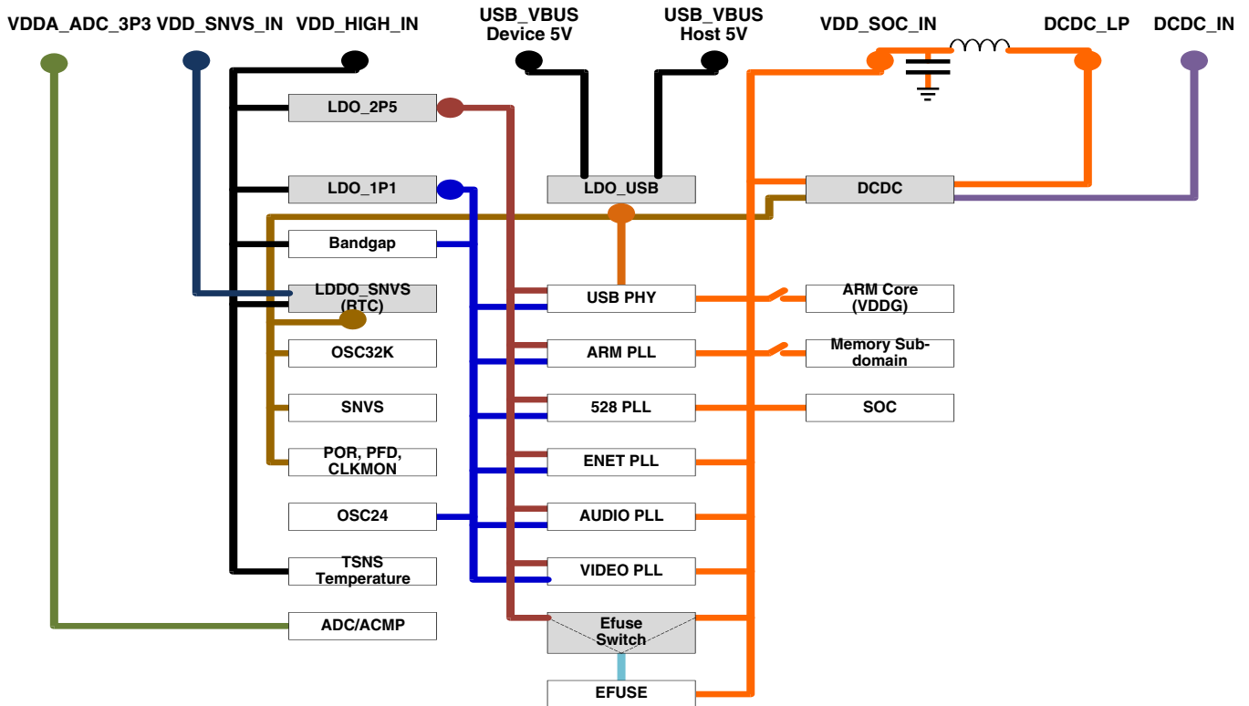
Figure 10-5. SOC Power Tree
