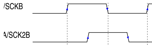
Figure 30-32. Input Timing 1 for Flash provided read strobe in DDR mode
