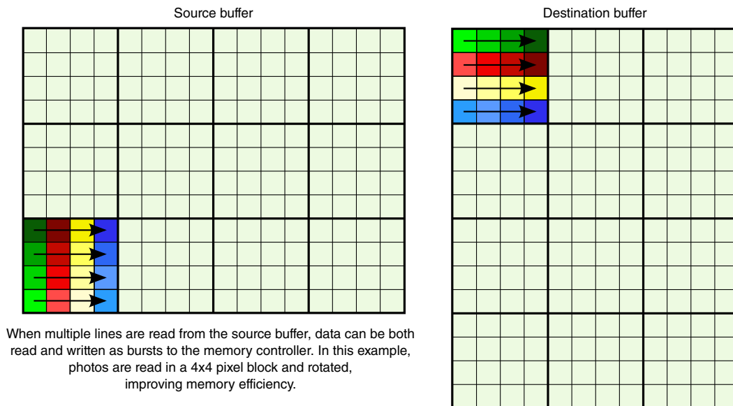
Figure 46-11. Rotated Sub-blocks
