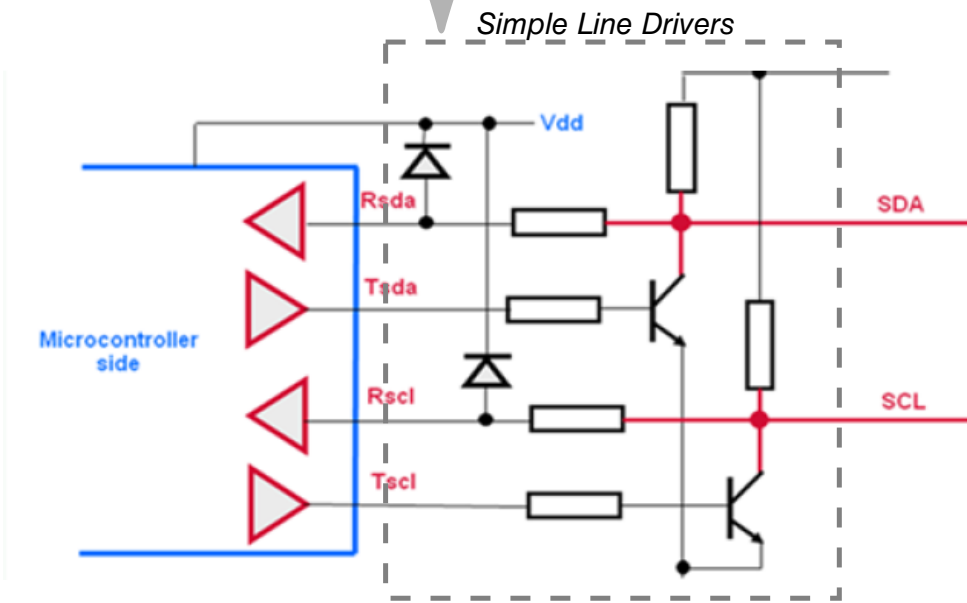
Figure 37-6. 4-Wire scheme
