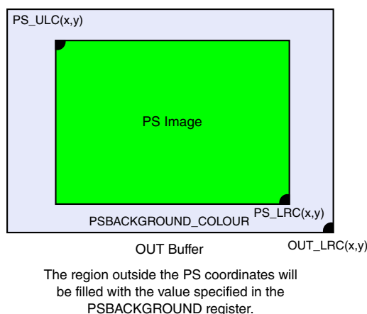
Figure 46-19. OUT Buffer
