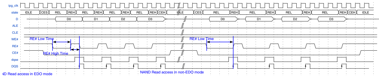
Figure 49-46. NAND Flash Read Access in EDO or non-EDO mode
