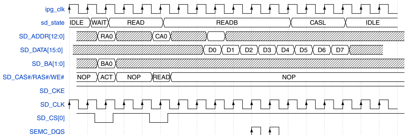
Figure 49-9. IP command - SDRAM READ
