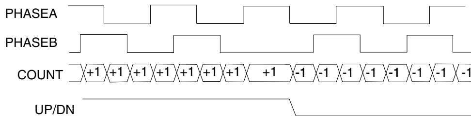
Figure 47-3. Quadrature Incremental Position Encoder
