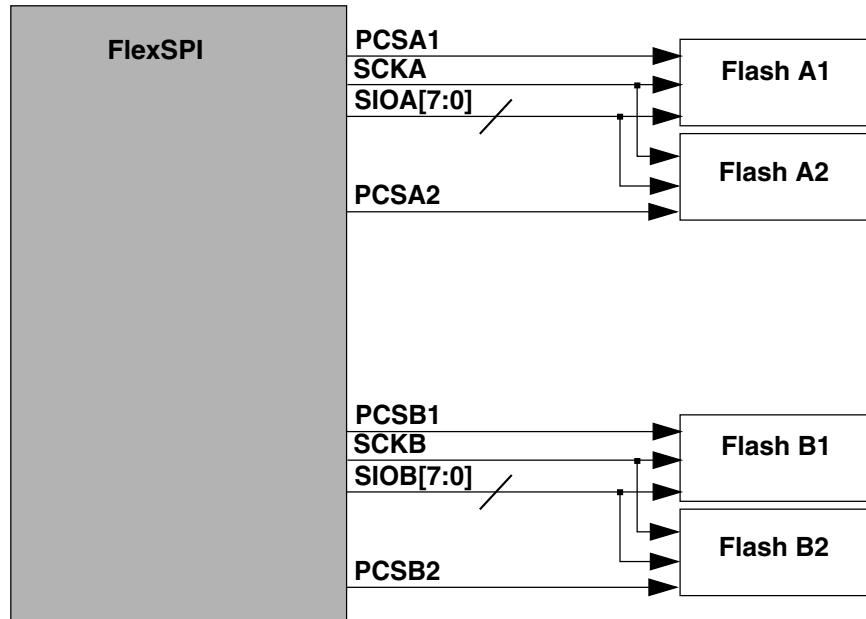
Figure 30-2. Flash connection diagram with four devices
