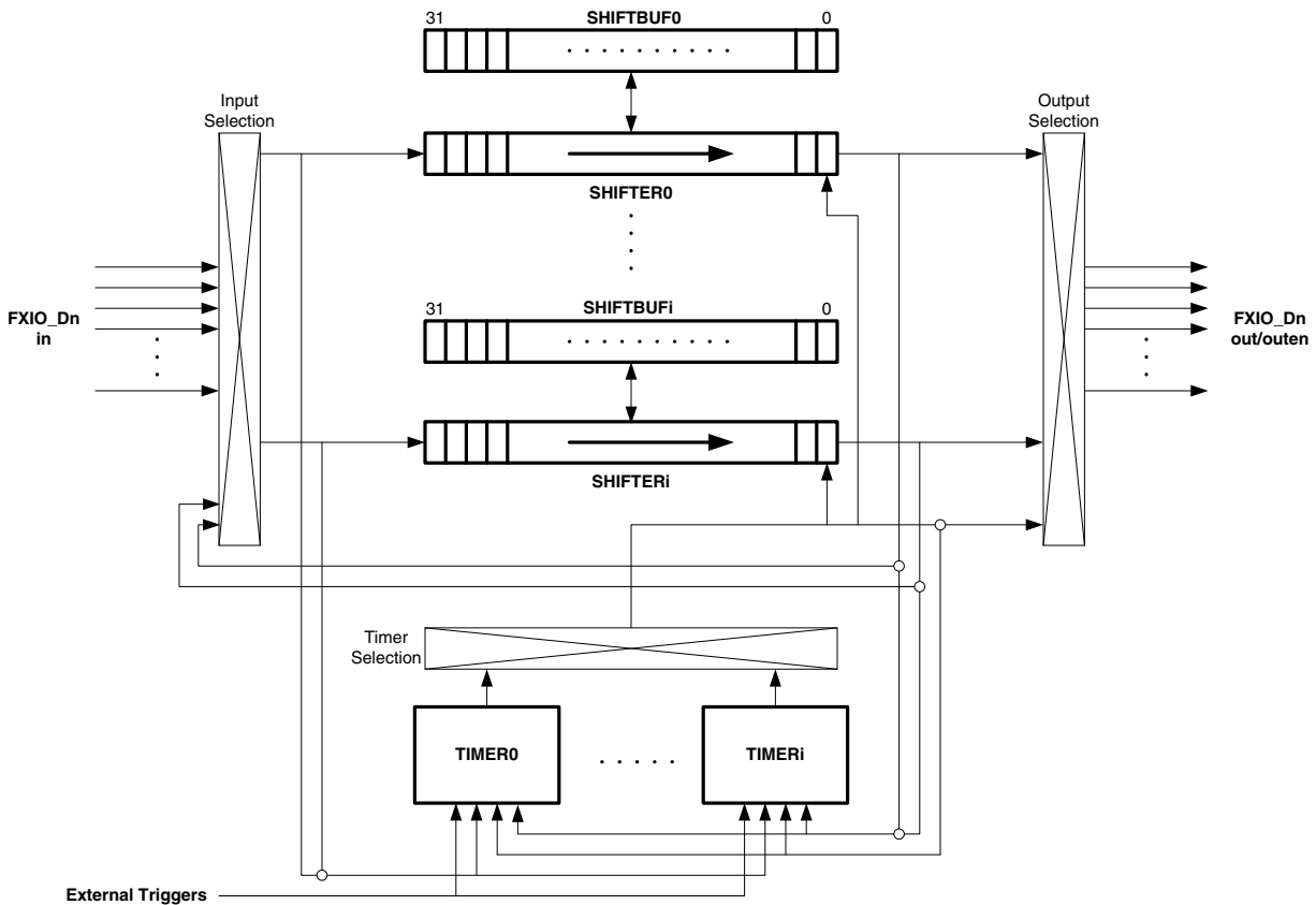
Figure 27-1. FlexIO block diagram
