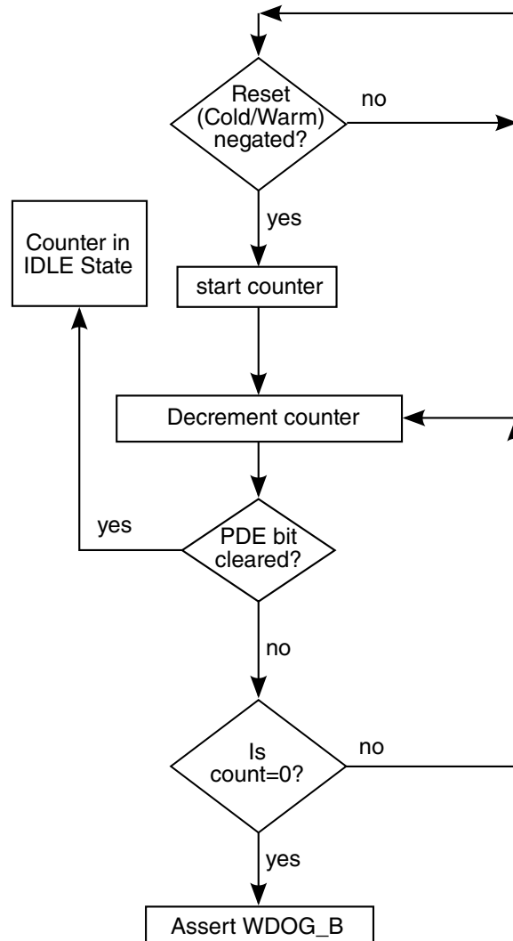
Figure 58-5. Power-Down Counter Flow Diagram
