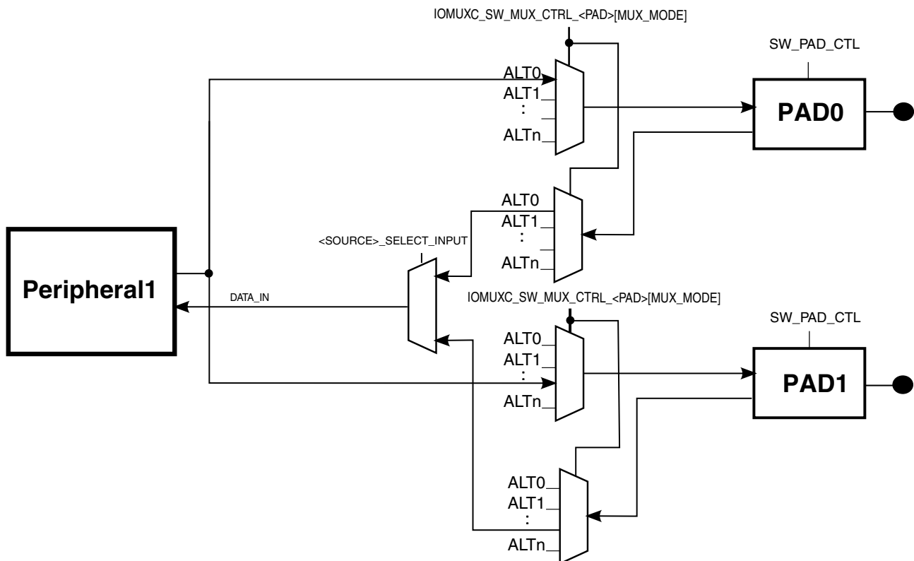
Figure 34-2. IOMUX Cell Block Diagram
