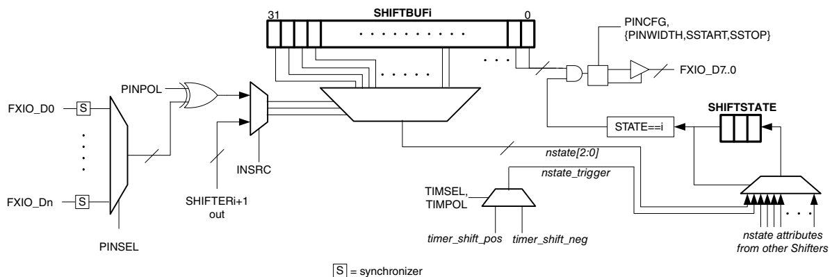
Figure 27-3. State Microarchitecture
