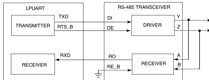
Figure 39-4. Transceiver driver enable using RTS_B
