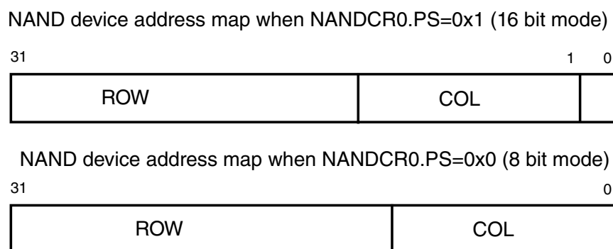
Figure 49-27. NAND Flash Address Map
