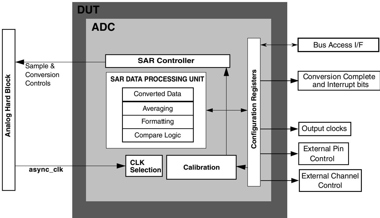
Figure 14-1. ADC I/F block diagram
