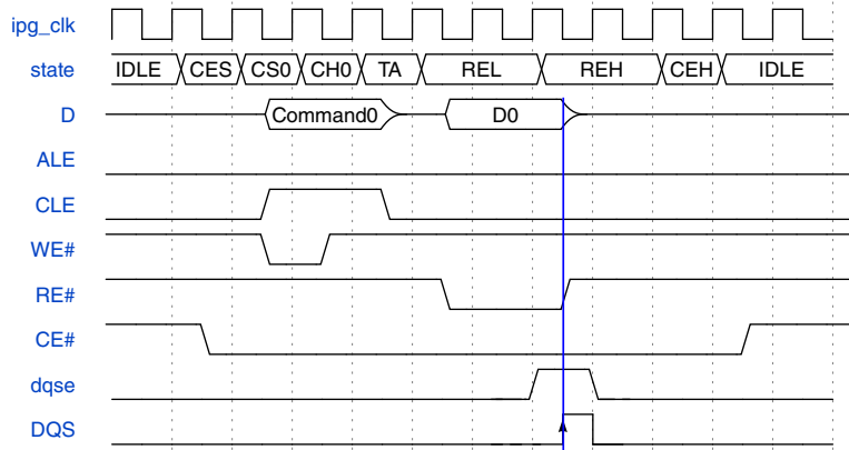
Figure 49-40. NAND Flash access command type - Command + Read Phase
