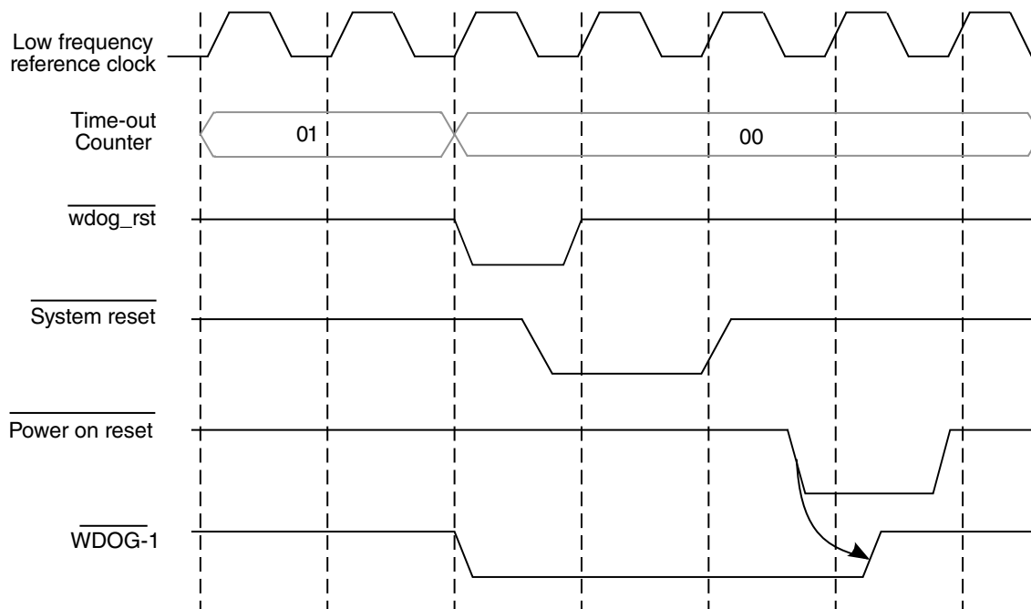
Figure 58-4. WDOG timeout condition/WDT bit is set
