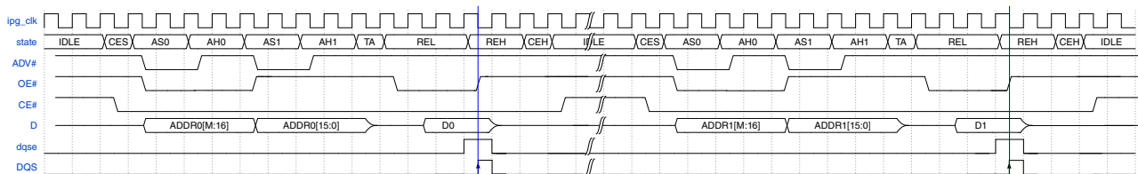
Figure 49-49. Flash Read in ASYNC mode (AADM)
