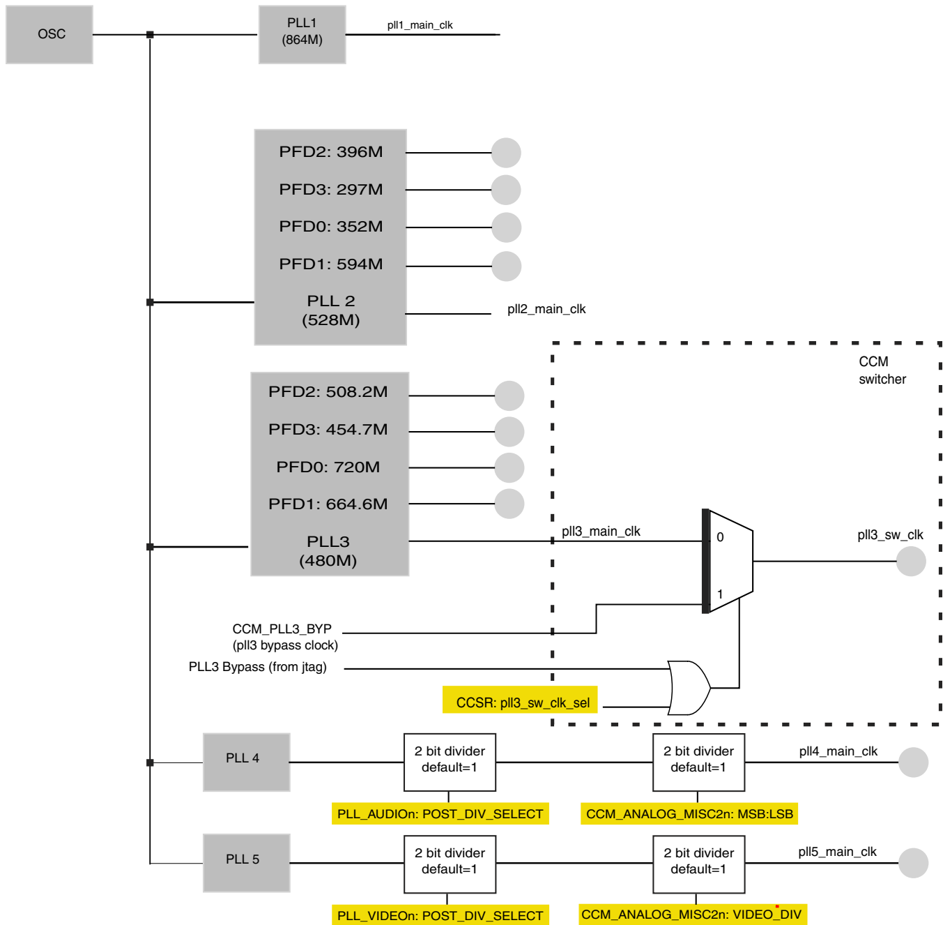
Figure 18-4. Switcher clock generation
