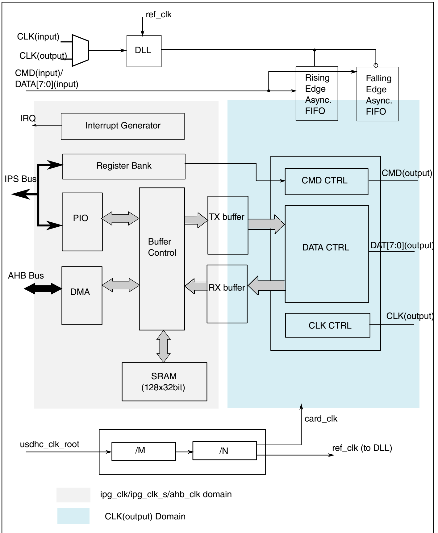
Figure 57-2. ultra Secure Digital Host Controller Block Diagram
