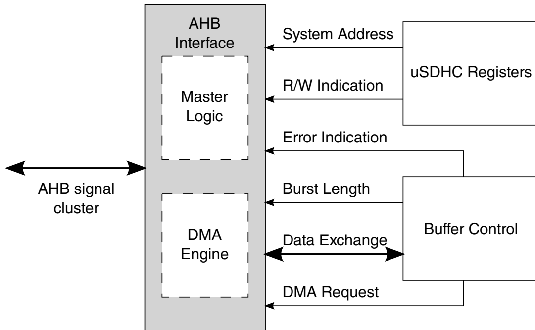
Figure 57-7. DMA AHB Interface Block
