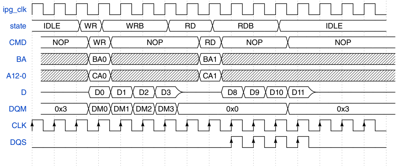
Figure 49-22. SDRAM Write-to-Read access (CL=1)
