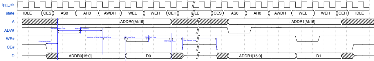
Figure 49-51. Flash Write in ASYNC mode (ADMUX)
