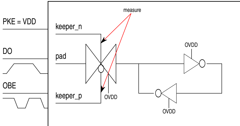
Figure 32-7. Keeper functional diagram
