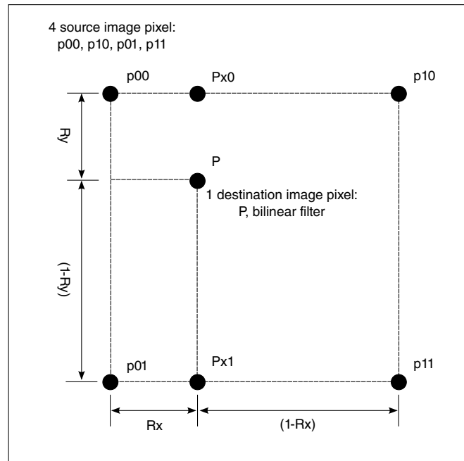
Figure 46-5. Output Pixel Value
