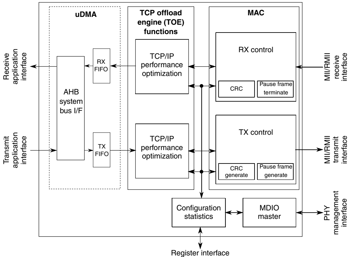
Figure 24-1. Ethernet MAC-NET core block diagram
