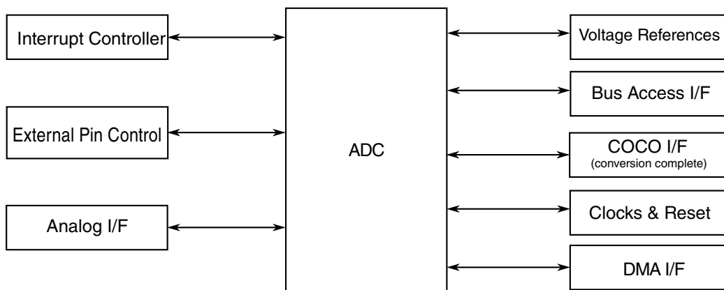
Figure 14-3. ADC module interface
