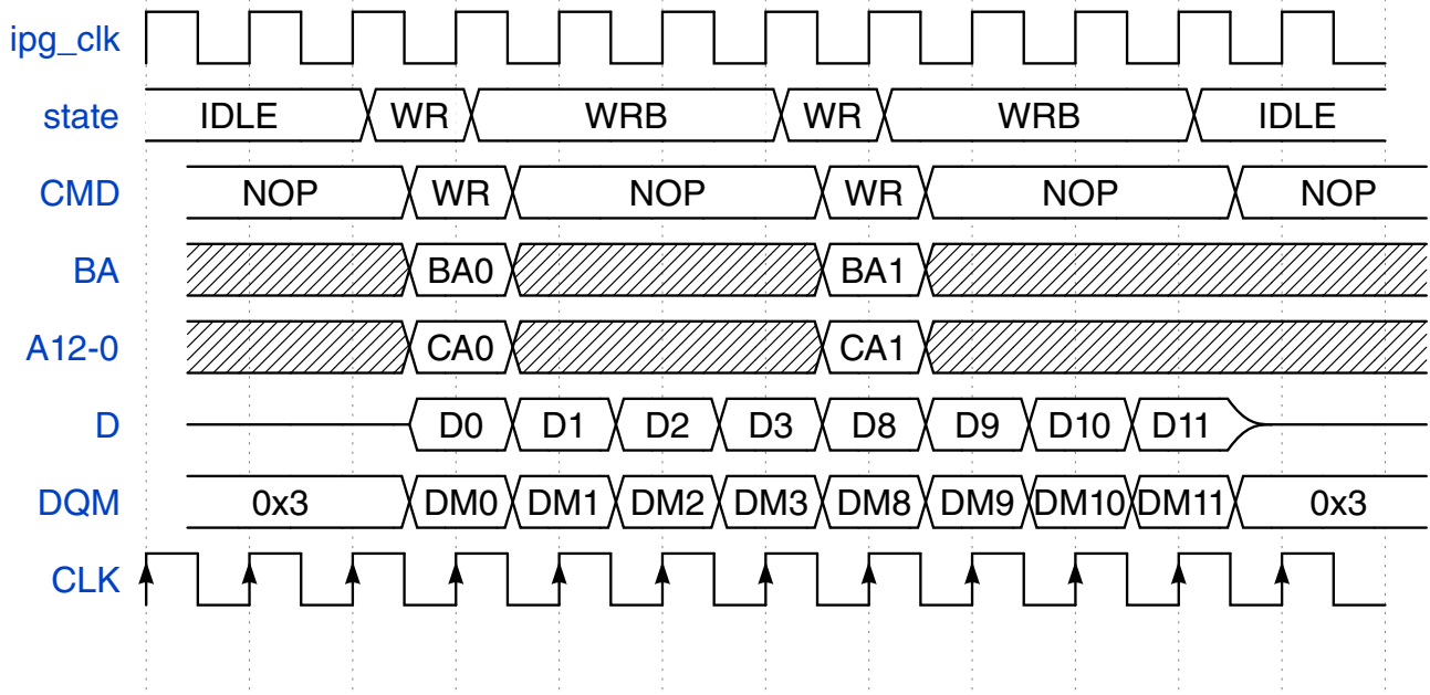
Figure 49-21. SDRAM Write-to-Write access
