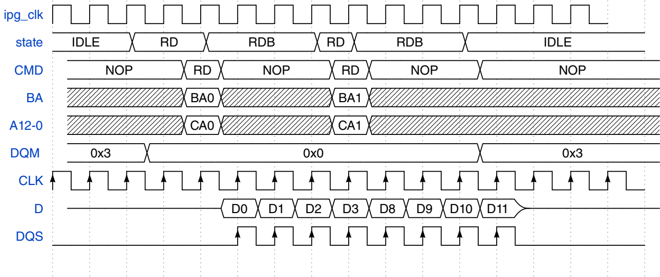
Figure 49-15. SDRAM Read-to-Read access (CL=1)
