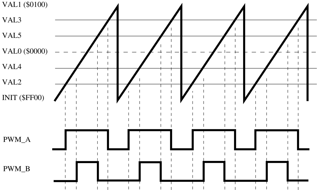
Figure 28-2. Center Aligned Example
