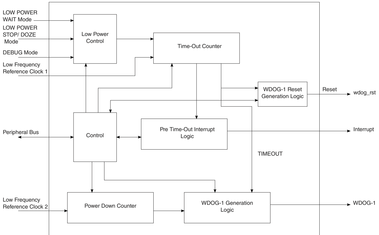
Figure 58-1. WDOG Diagram
