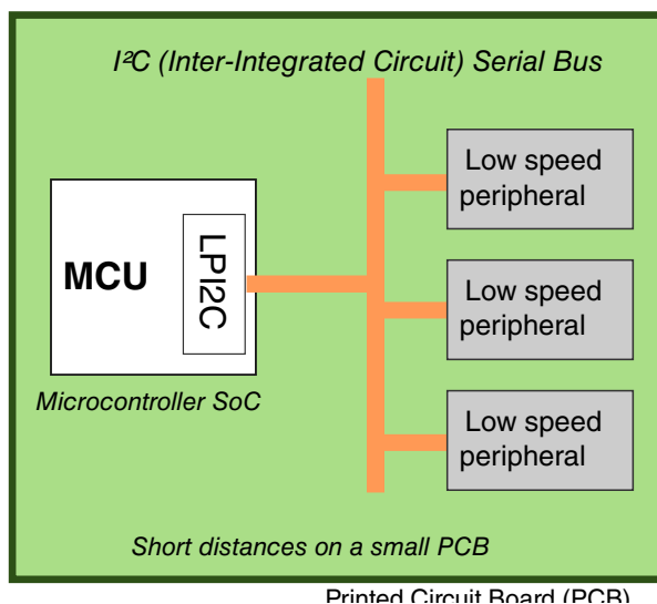
Figure 37-1. I 2 C bus connects MCU to low speed peripherals on PCB
