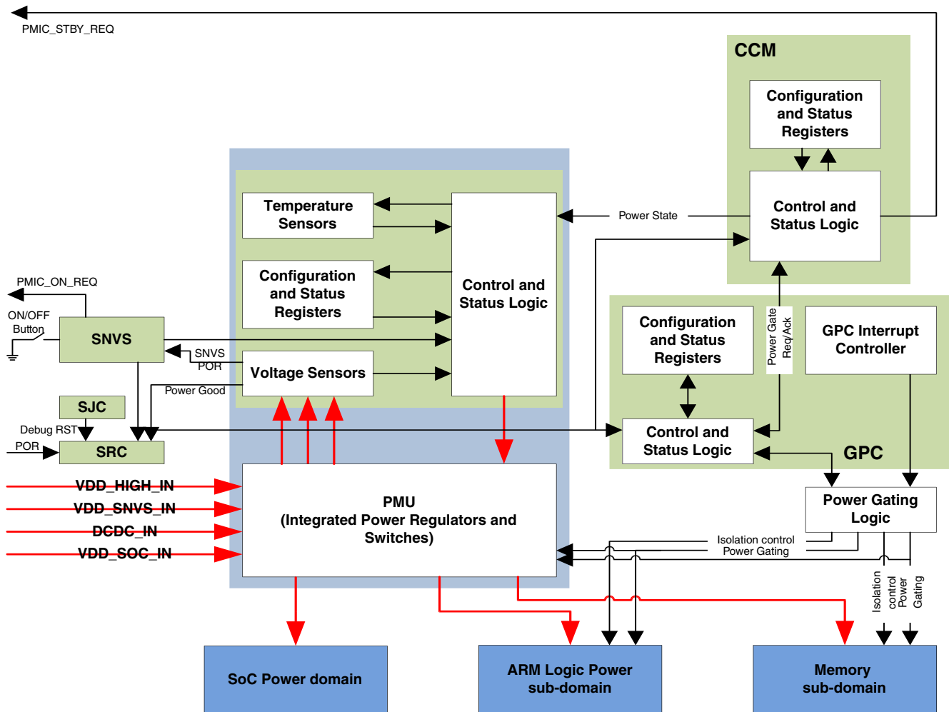
Figure 10-4. Power Management System
