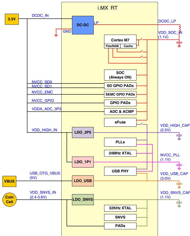
Figure 45-1. Power system overview
