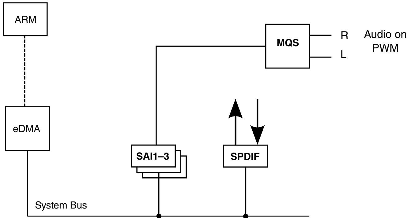
Figure 9-2. Audio subsystem block diagram
