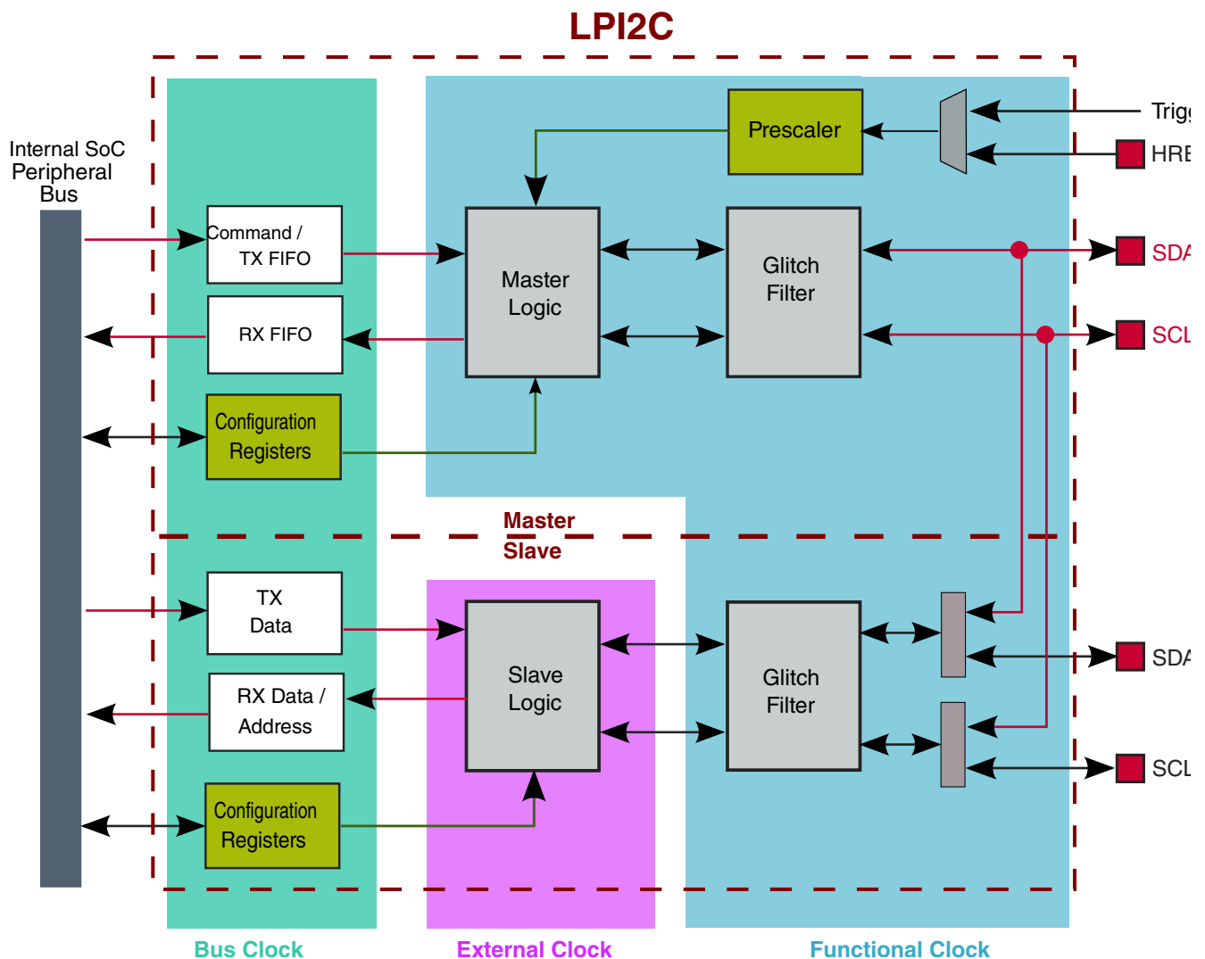
Figure 37-4. LPI2C block diagram
