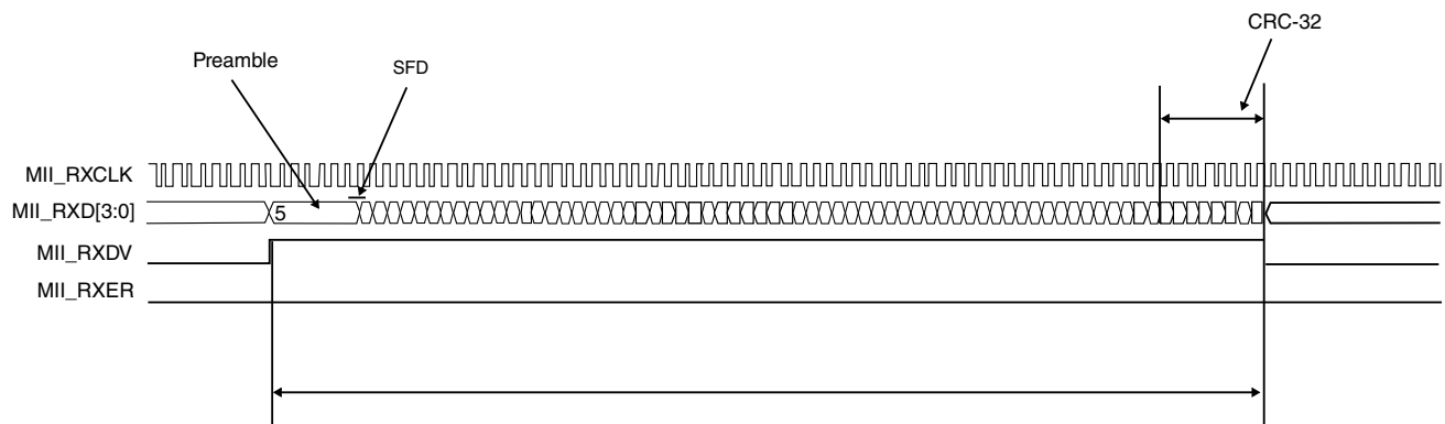
Figure 24-25. MII receive operation
