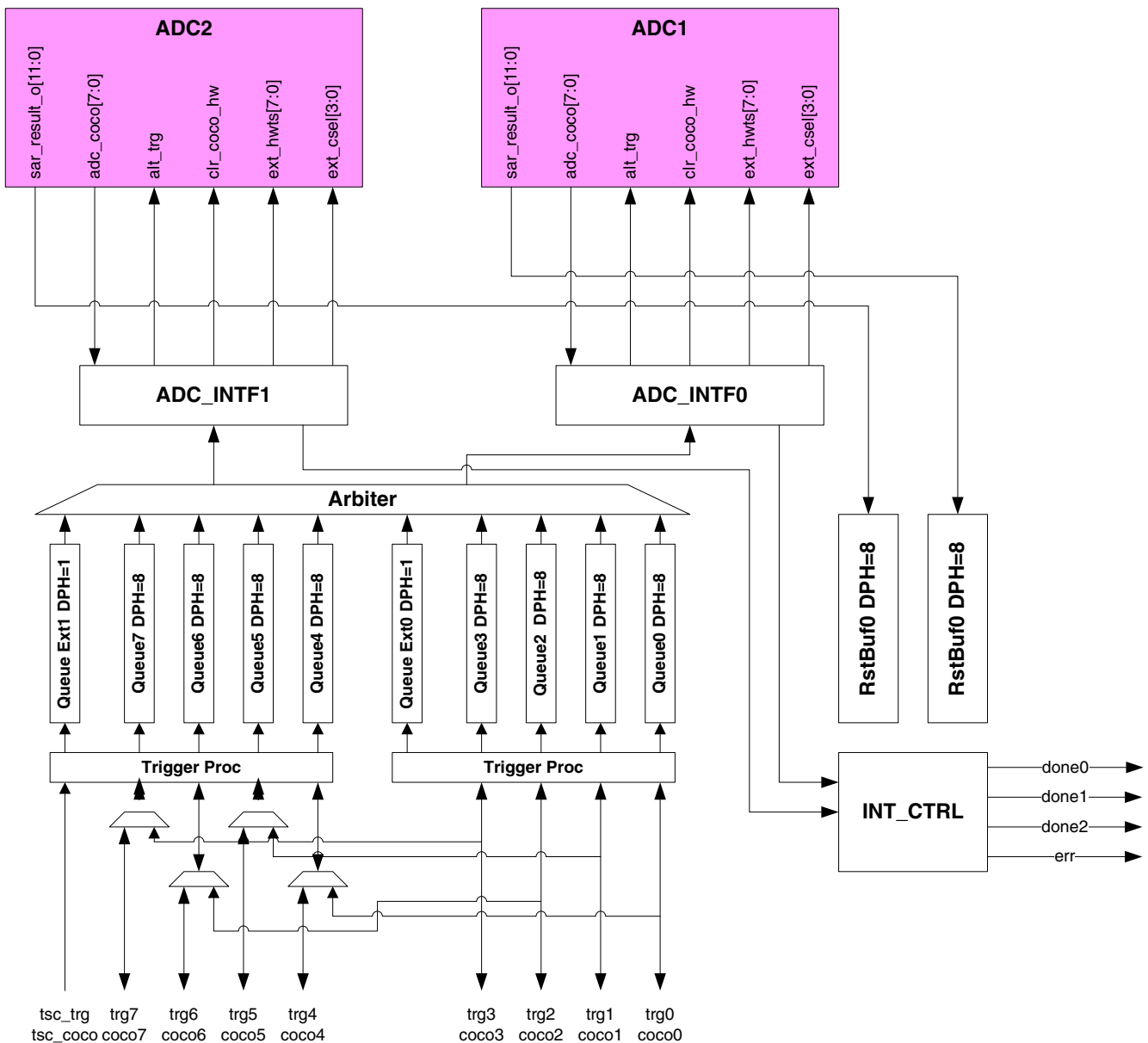
Figure 15-1. ADC_ETC block diagram
