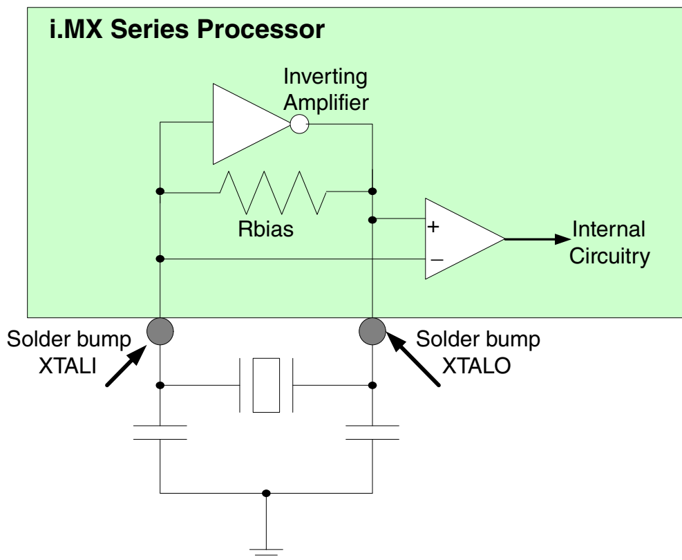
Figure 62-1. Oscillator Configuration (24 MHz)
