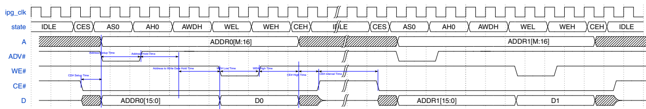
Figure 49-57. SRAM Write in ASYNC mode (ADMUX)
