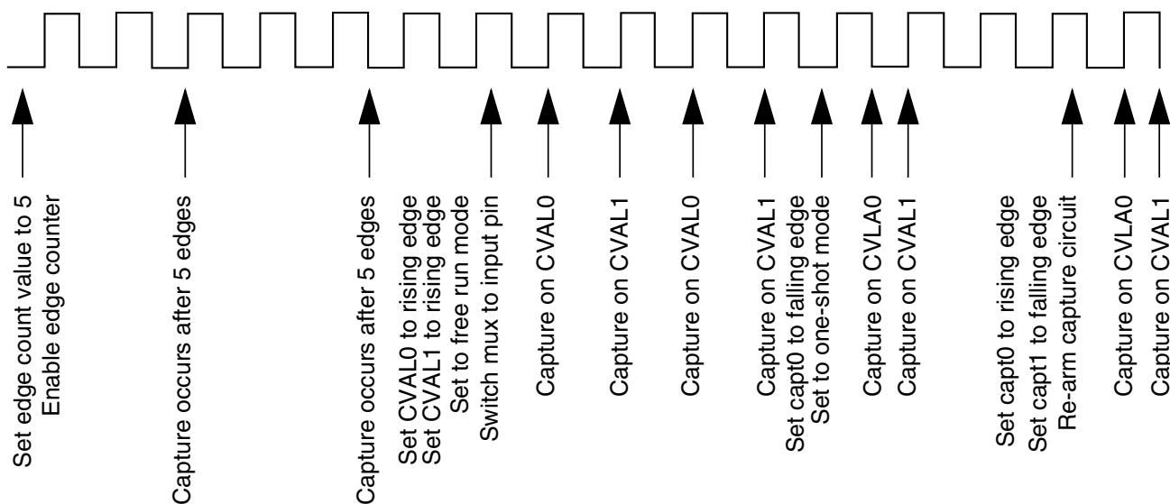
Figure 28-9. Capture Capabilities of the E-Capture Circuit
