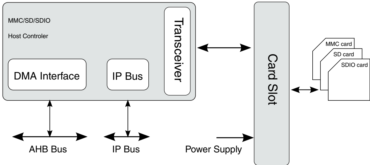
Figure 57-1. System Connection of the uSDHC
