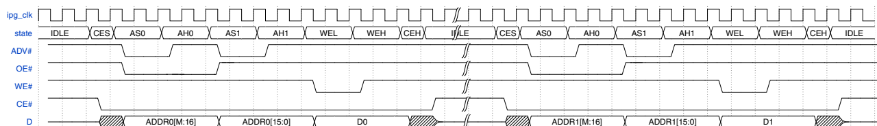
Figure 49-58. SRAM Write in ASYNC mode (AADM)
