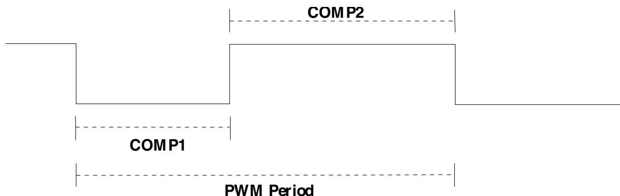
Figure 47-2. Variable PWM Waveform
