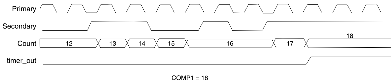
Figure 47-4. Triggered Count Mode 1 (CTRL[LENGTH]=0)
