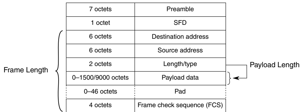
Figure 24-2. MAC frame format overview
