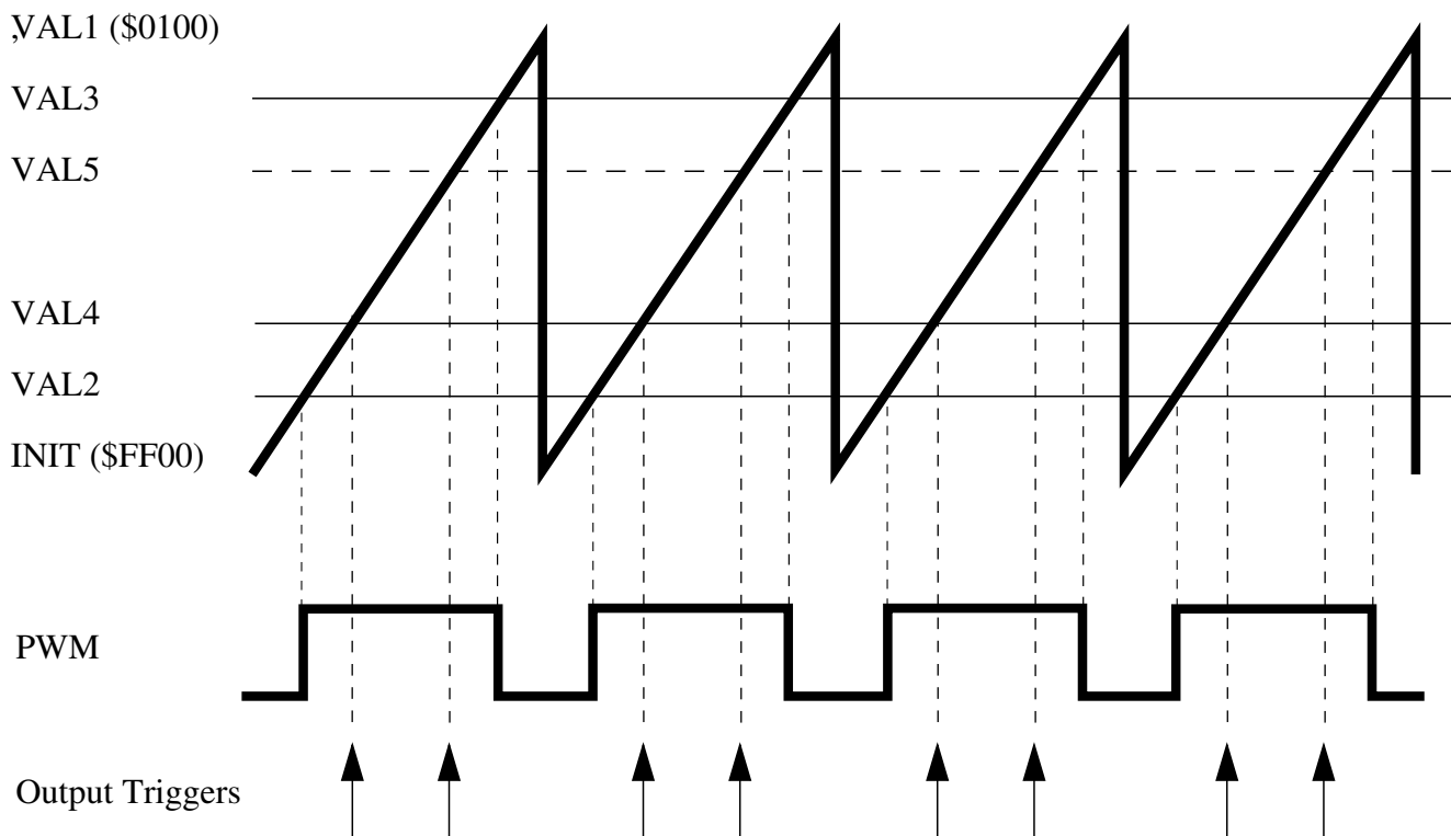
Figure 28-7. Multiple Output Trigger Generation in Hardware
