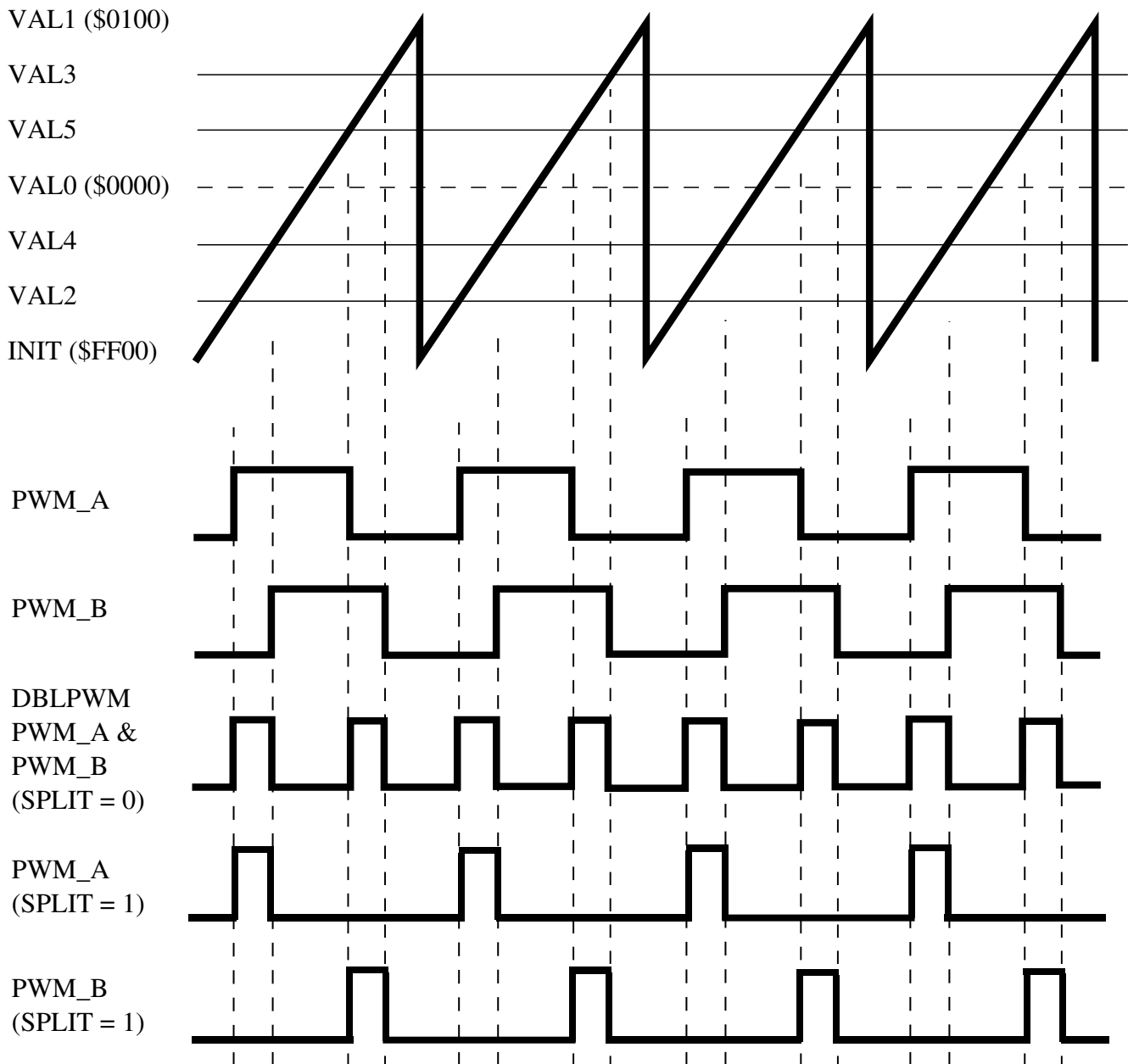
Figure 28-6. Double Switching Output Example
