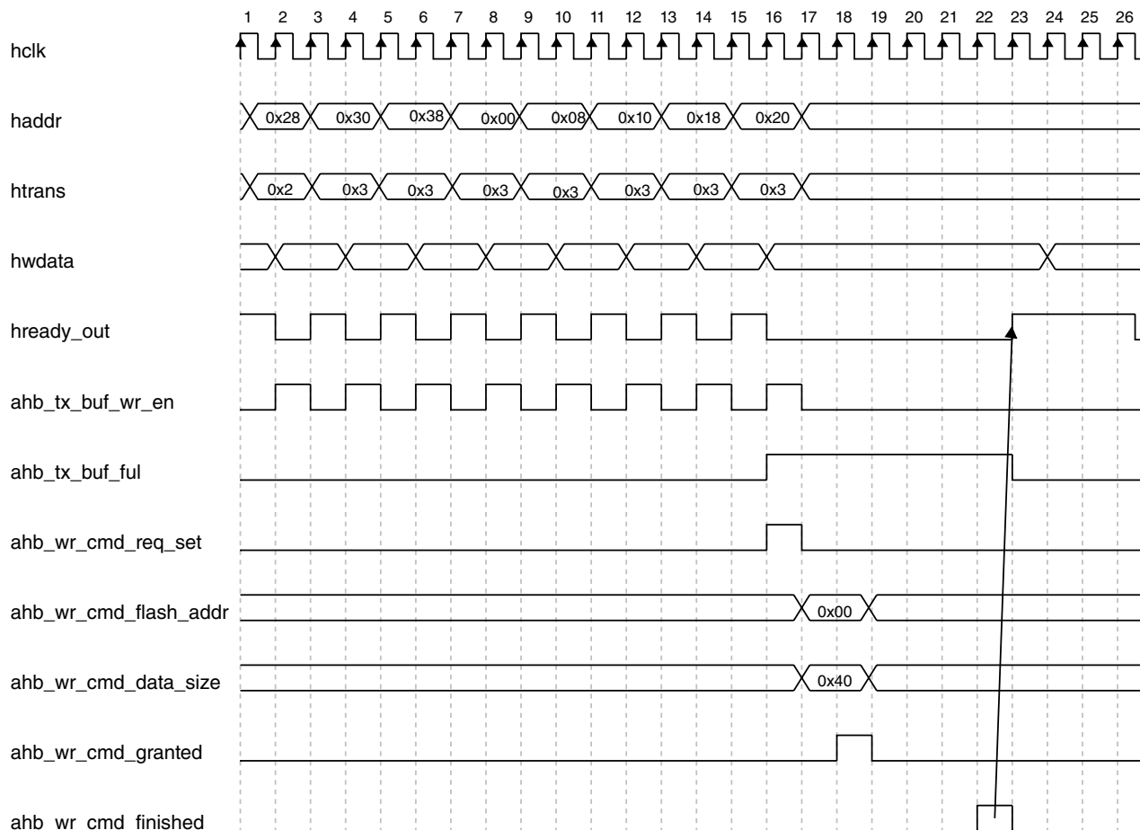
Figure 30-20. AHB write access (WRAP8/64bit/Non-Bufferable)
