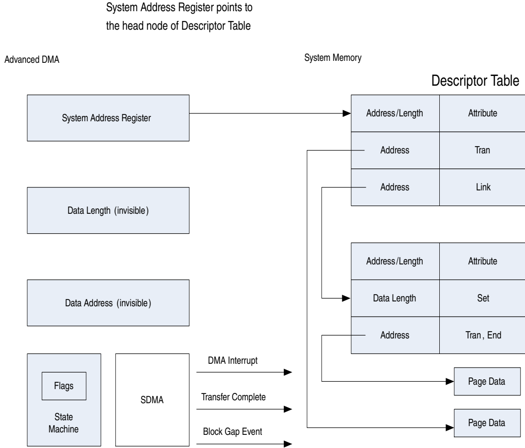
Figure 57-9. Concept and Access Method of ADMA1 Descriptor Table
