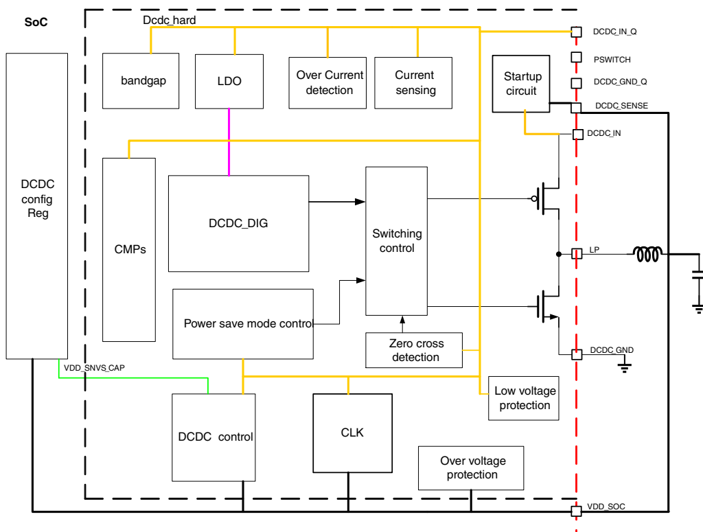
Figure 20-1. DCDC block diagram
