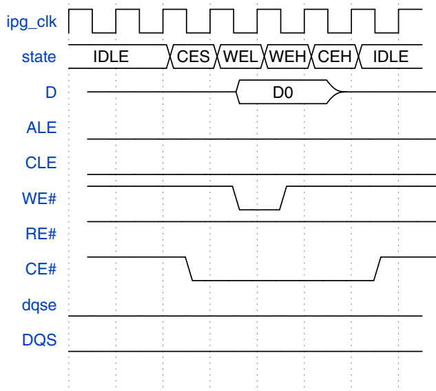
Figure 49-43. NAND Flash access command type - Write Phase Only
