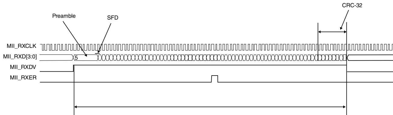
Figure 24-26. MII receive operation — errored frame
