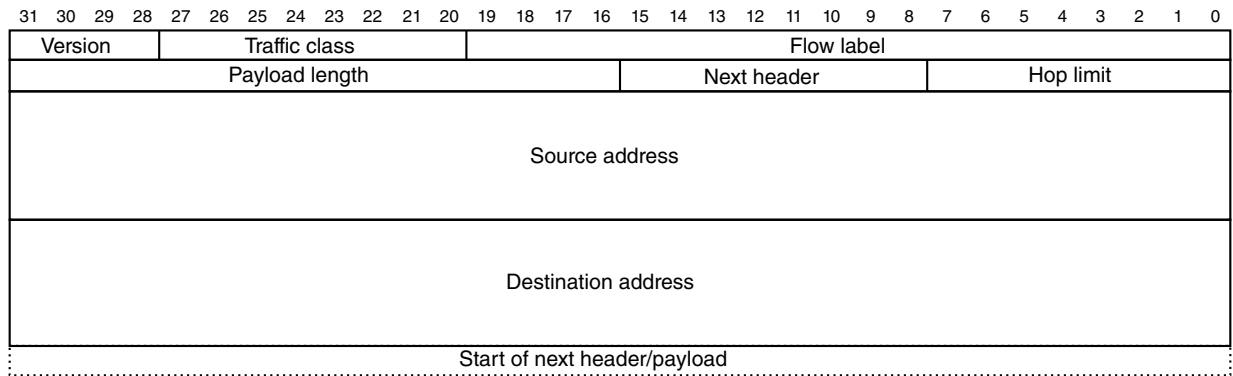
Figure 24-4. IPv6 header format
