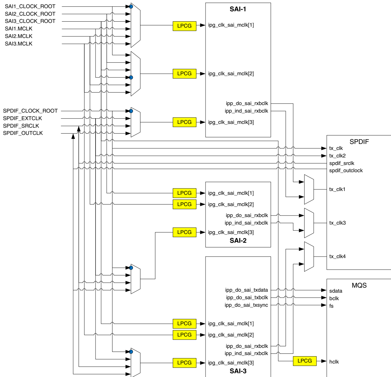
Figure 9-3. Audio subsystem clocking diagram
