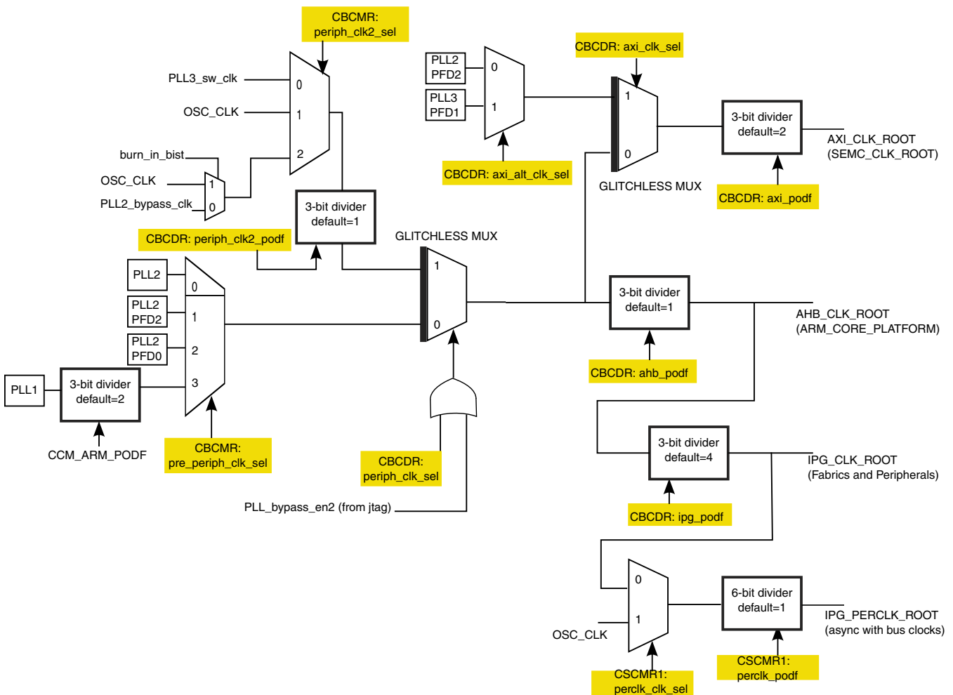
Figure 18-5. BUS clock generation
