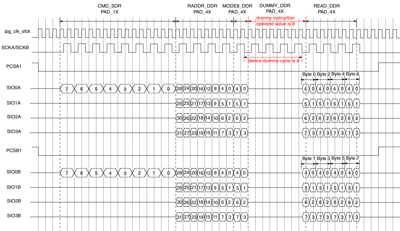
Figure 30-8. Flash access sequence example (DDR Quad I/O Read sequence)
