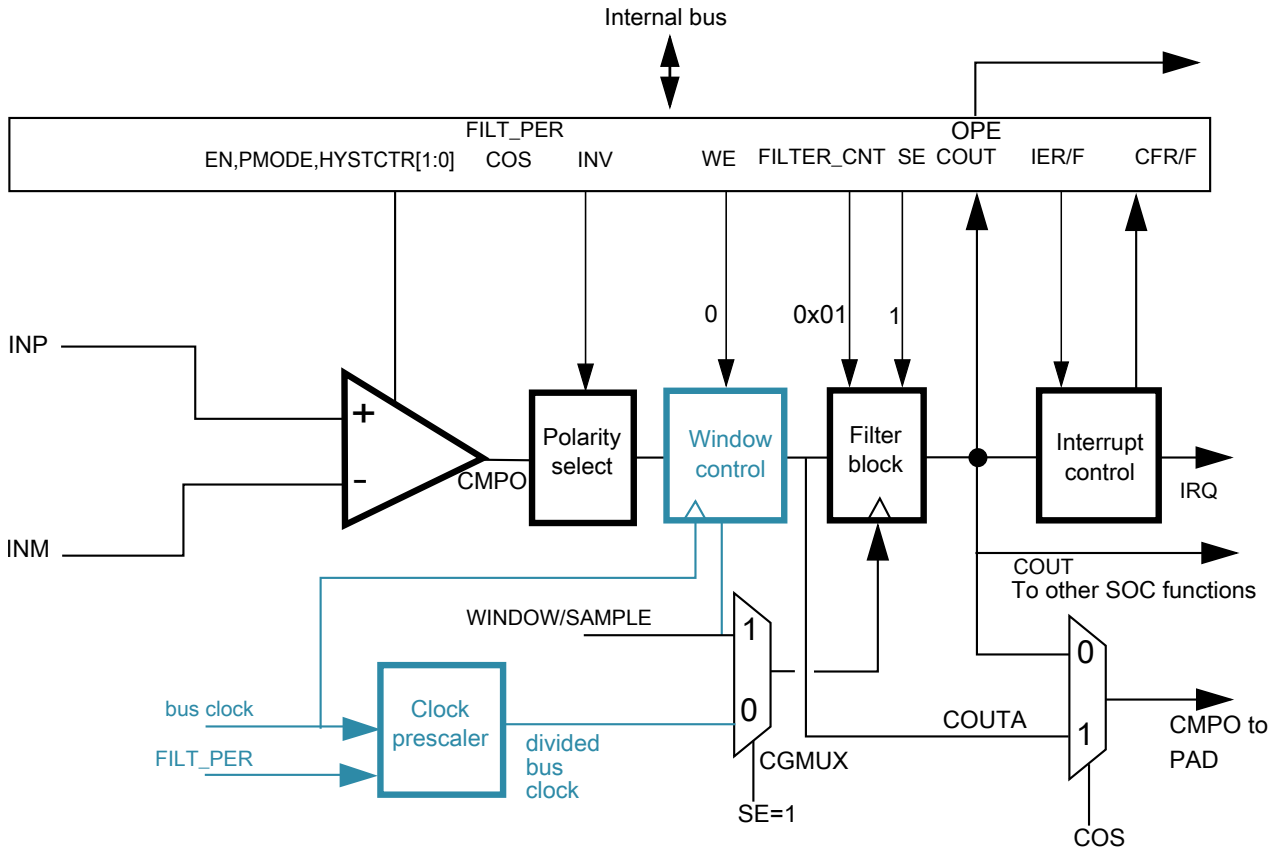
Figure 13-4. Sampled, Non-Filtered (# 3A): sampling point externally driven
