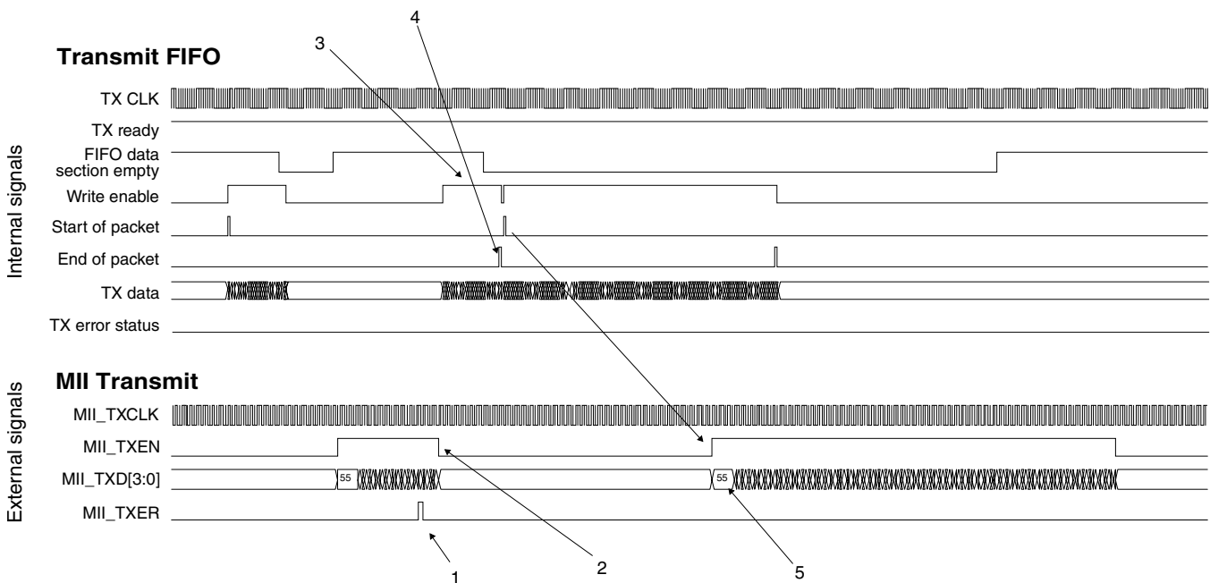
Figure 24-16. Transmit FIFO underflow protection
