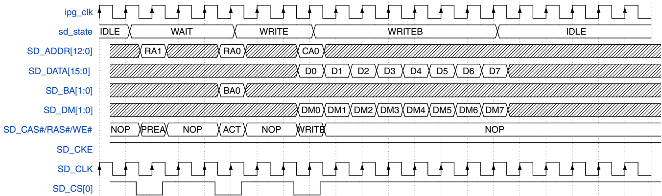
Figure 49-12. AXI command - SDRAM Write
