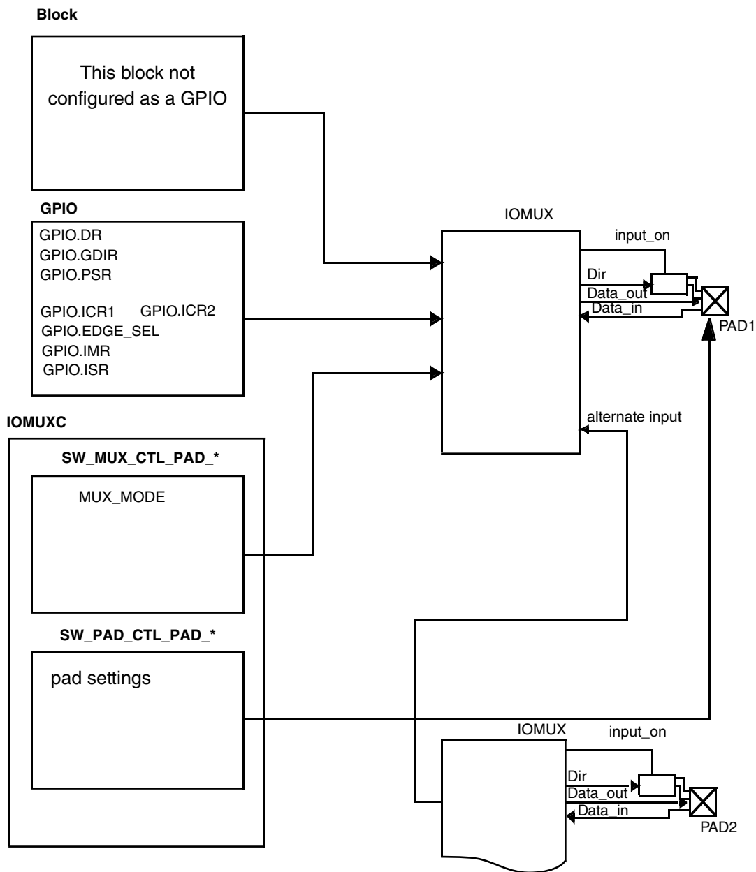
Figure 32-1. Chip IOMUX Scheme
