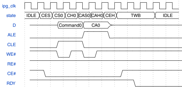
Figure 49-37. NAND Flash access command type - Command + Address + Wait Phase
