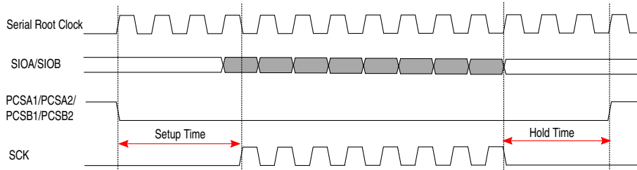
Figure 30-26. Chip selection output timing for SDR sequence
