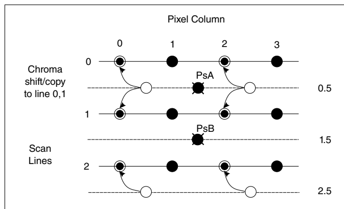
Figure 46-8. Scaled Chroma Computation Examples
