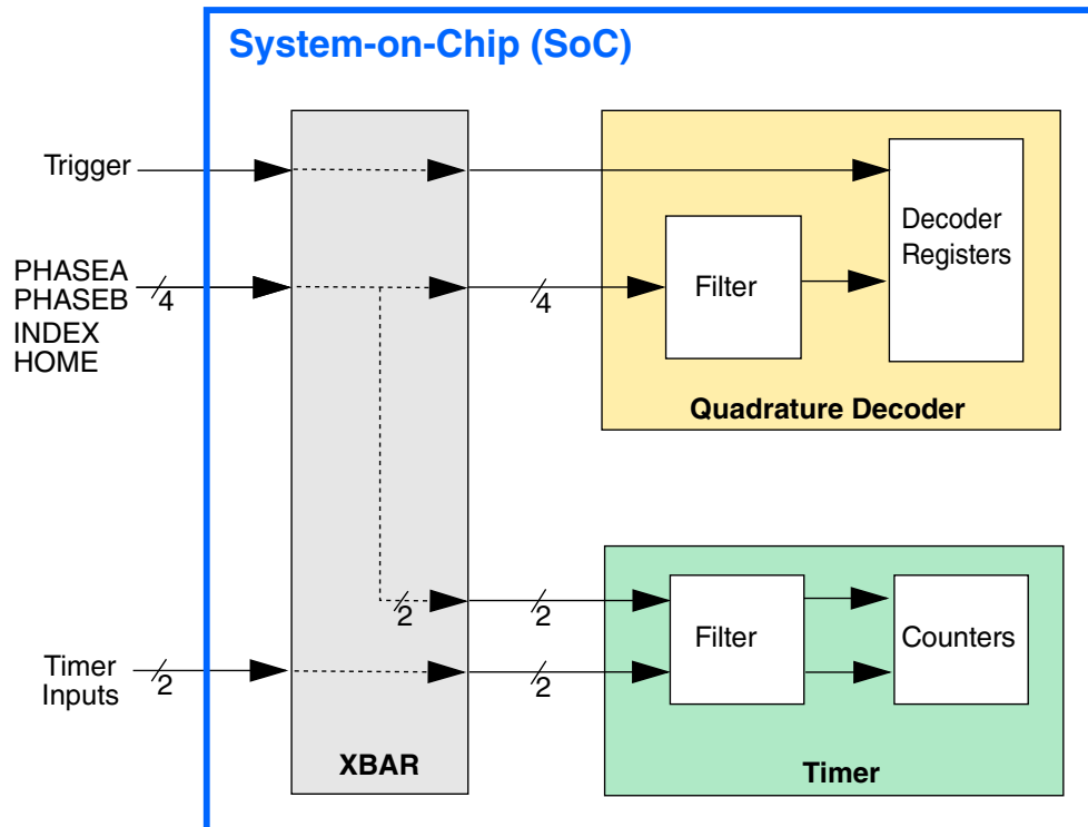
Figure 23-1. System Block Diagram
