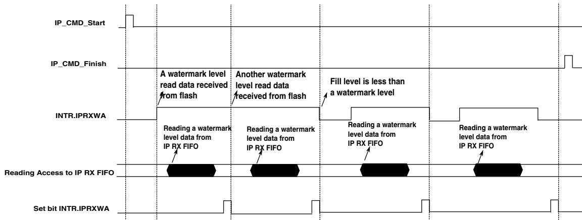
Figure 30-13. Reading IP RX FIFO by processor
