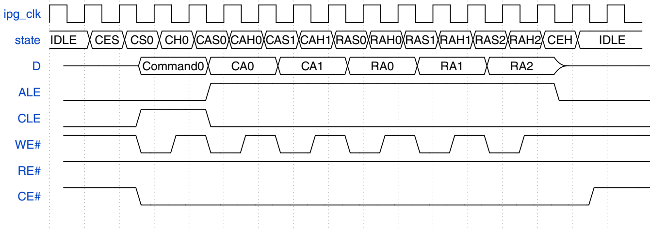
Figure 49-33. NAND Flash access Address type - Five Byte Row/Column Address
