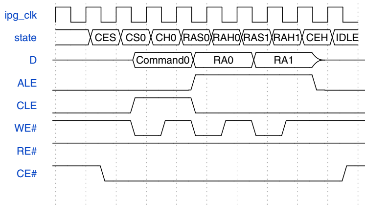
Figure 49-31. NAND Flash access Address type - Two Byte Row Address
