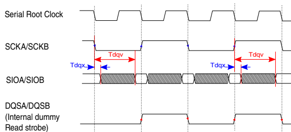
Figure 30-30. Input Timing for sampling with dummy read strobe in DDR mode
