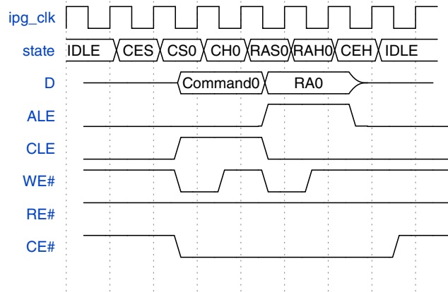
Figure 49-30. NAND Flash access Address type - One Byte Row Address
