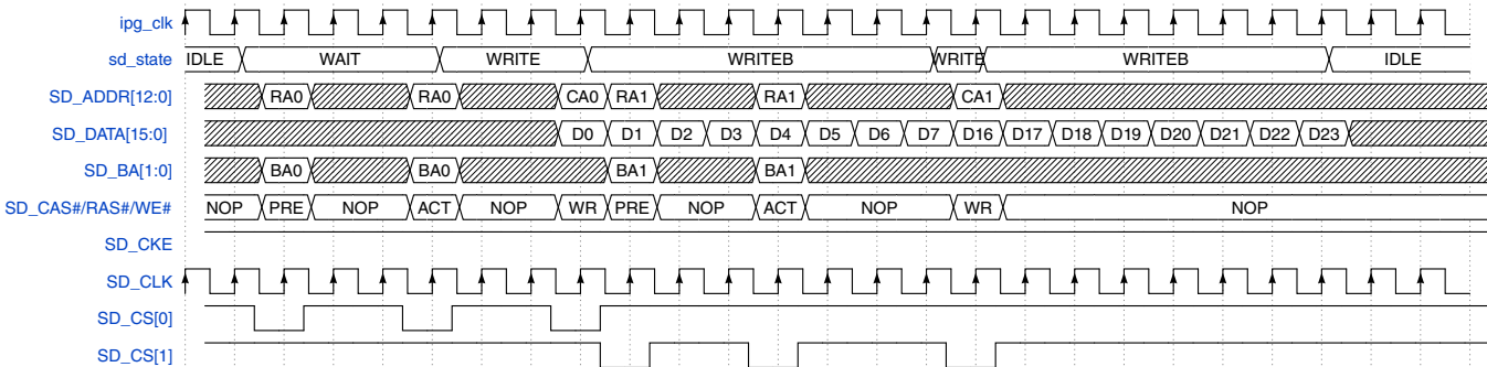
Figure 49-14. AXI command - Pipelined SDRAM Write
