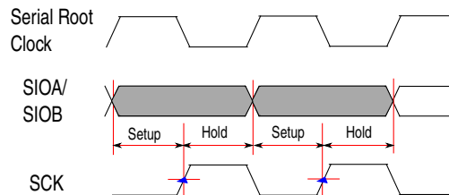
Figure 30-23. SDR instruction in SDR sequence
