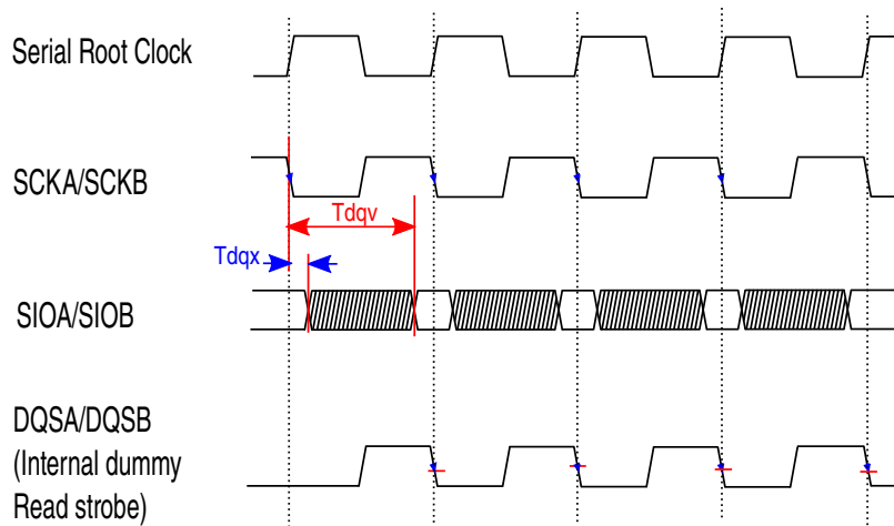
Figure 30-29. Input Timing for sampling with dummy read strobe in SDR mode
