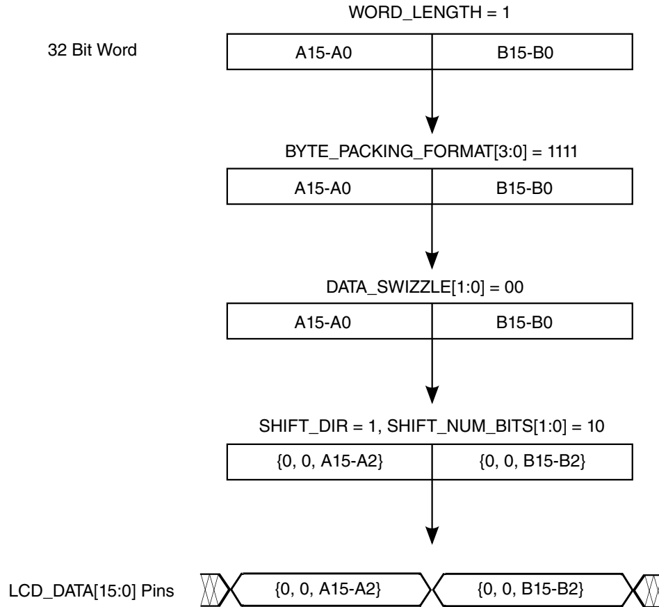
Figure 36-5. Register programming for write mode
