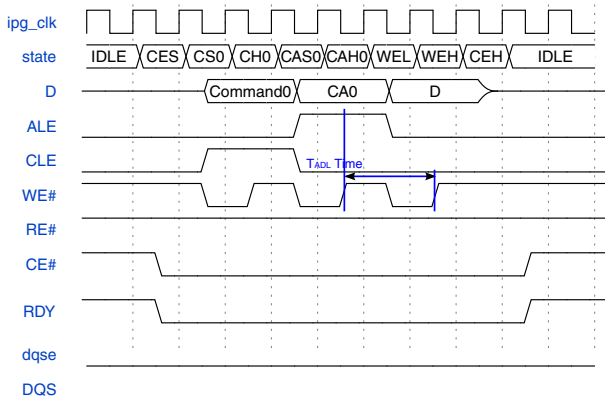
Figure 49-39. NAND Flash access command type - Command + Address + Write Phase
