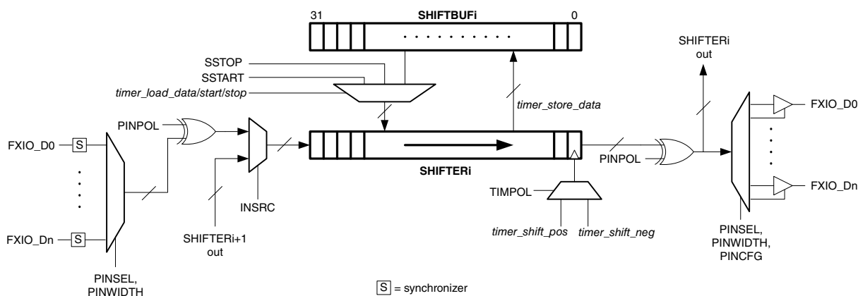
Figure 27-2. Shifter Microarchitecture
