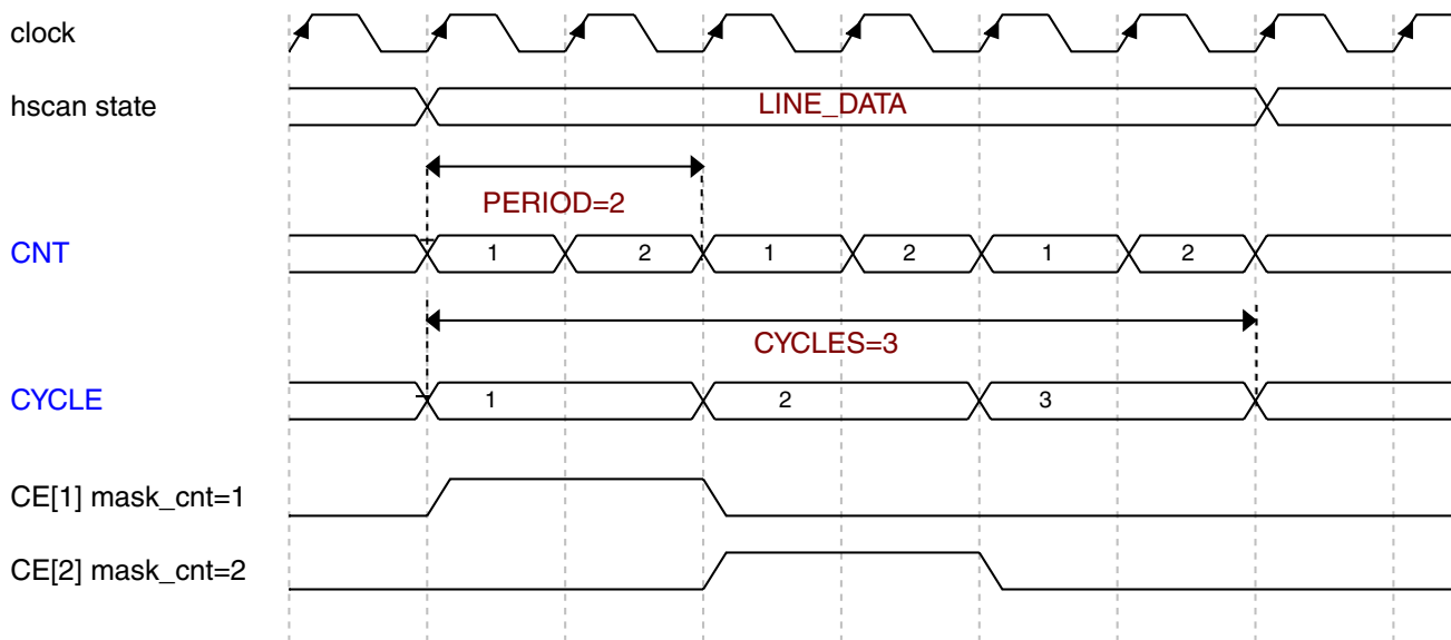
Figure 36-8. Definition of CNT, CYCLE, PERIOD
