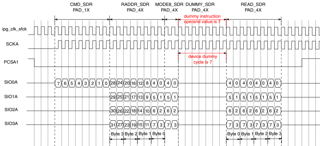
Figure 30-7. Flash access sequence example (SDR Quad I/O Read sequence)
