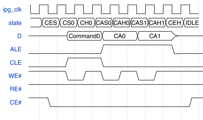
Figure 49-29. NAND Flash access Address type - Two Byte Column Address
