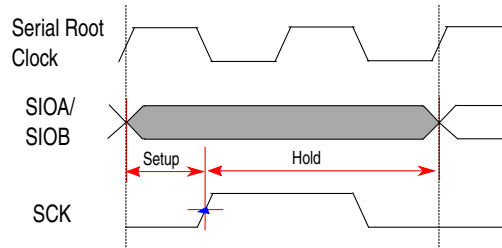
Figure 30-24. SDR instruction in DDR sequence
