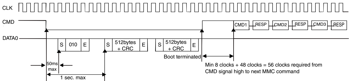
Figure 57-16. MultiMediaCard state diagram (normal boot mode)
