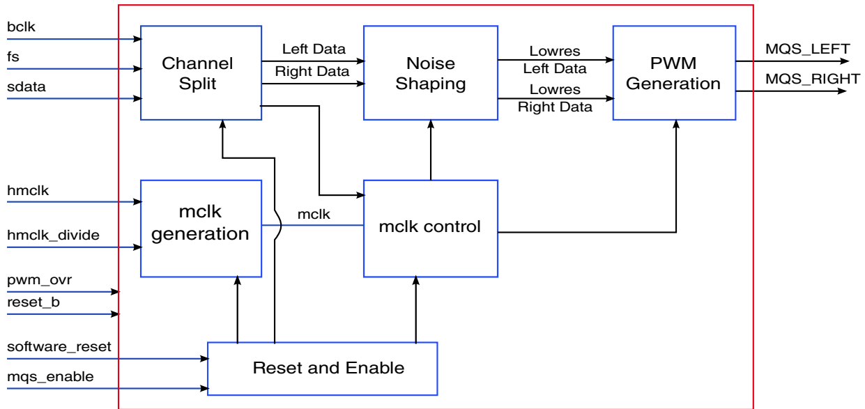
Figure 40-1. Block Diagram
