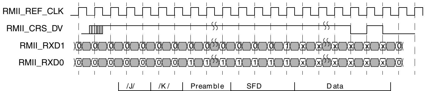
Figure 24-19. RMII receive operation
