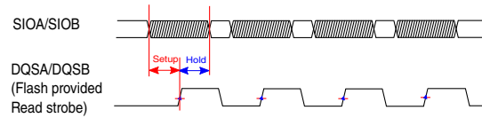
Figure 30-31. Input Timing 1 for Flash provided read strobe in SDR mode
