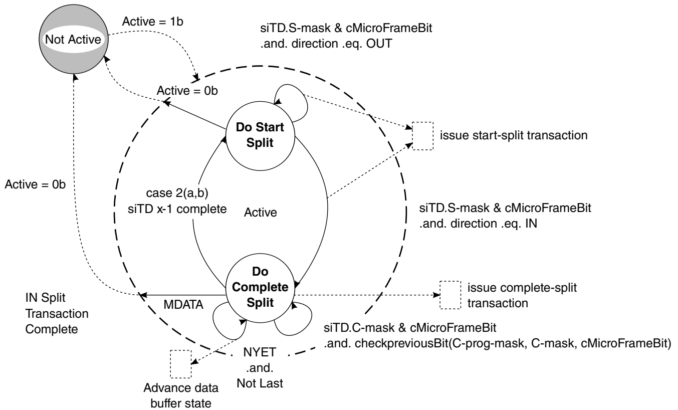
Figure 55-26. Split Transaction State Machine for Isochronous
