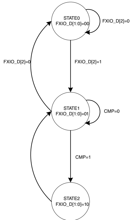
Figure 27-5. State Diagram
