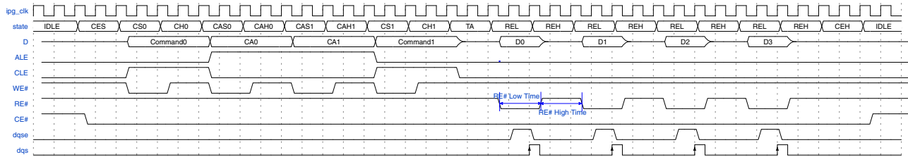
Figure 49-44. NAND Flash access command type - Command + Address + Command + Read Phase
