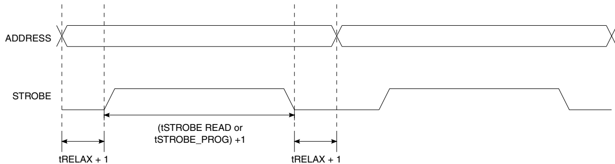
Figure 42-3. STROBE Signal Creation and Timing
