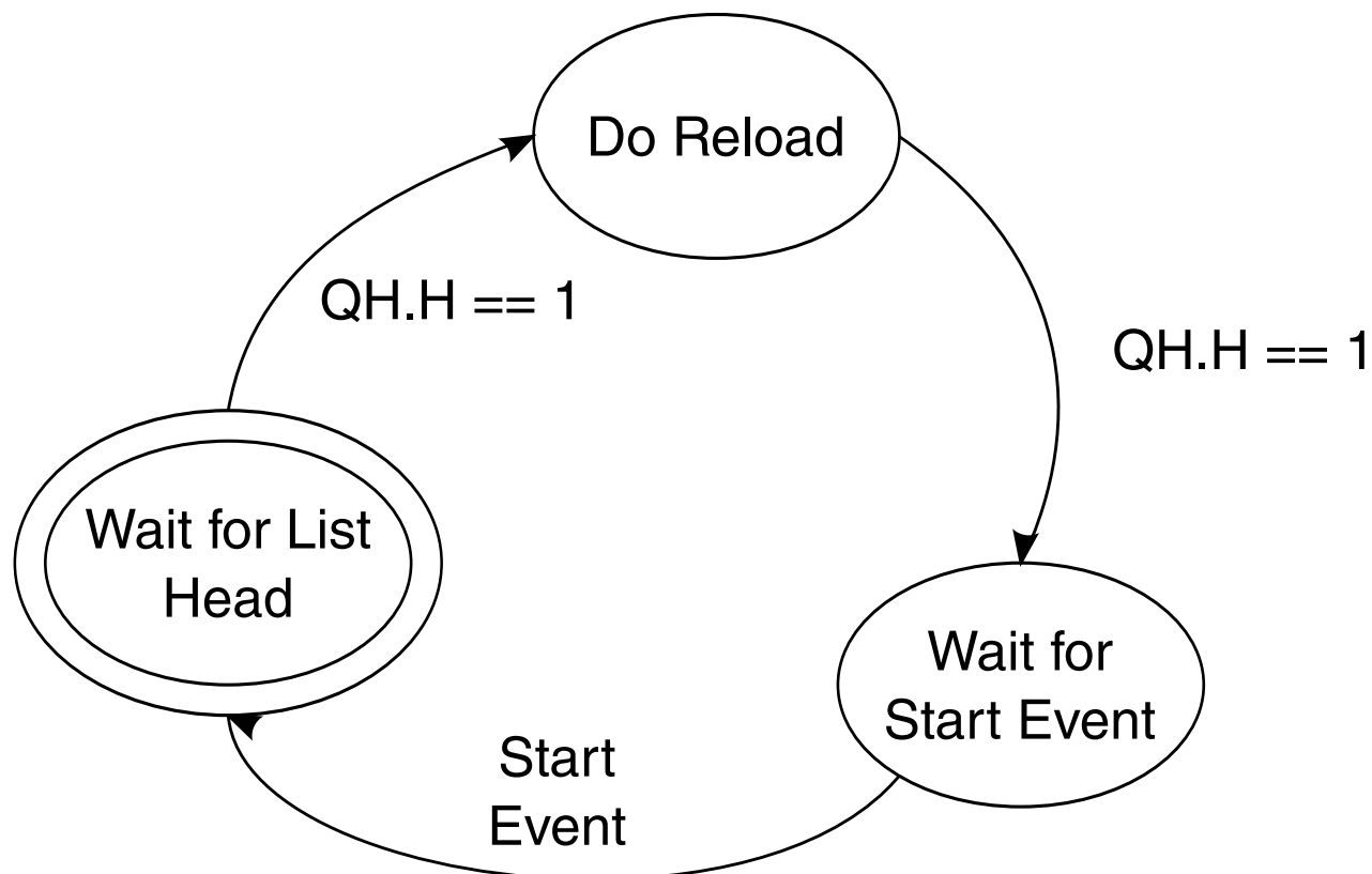
Figure 55-16. Example HC State Machine for Controlling Nak Counter Reloads
