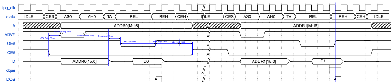
Figure 49-48. Flash Read in ASYNC mode (ADMUX)
