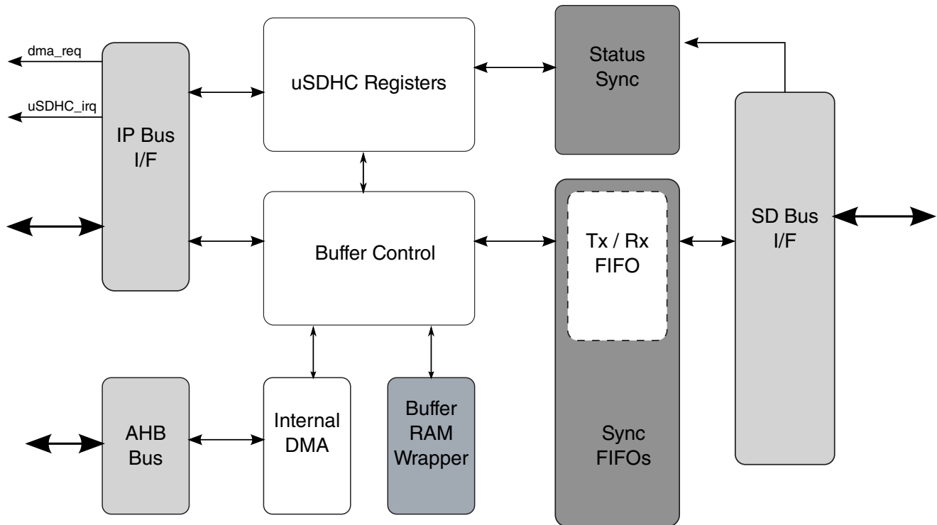
Figure 57-3. uSDHC Buffer Scheme
