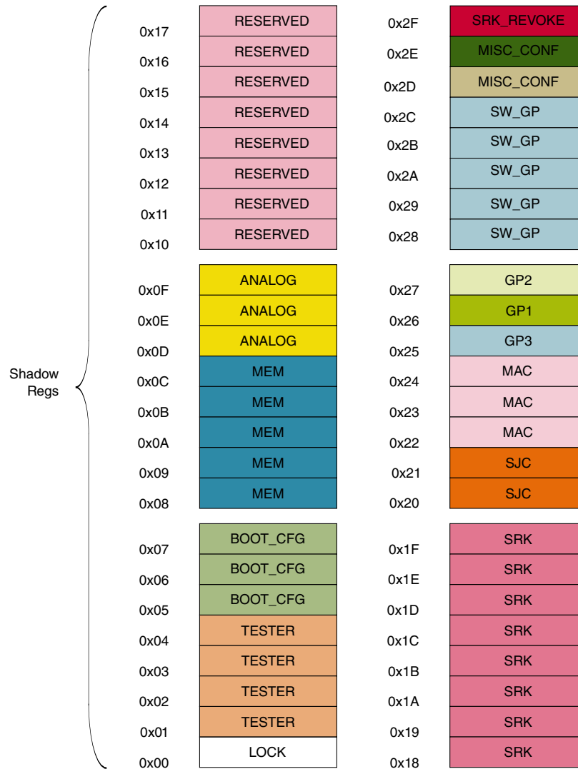
Figure 42-2. OTP Memory Footprint
