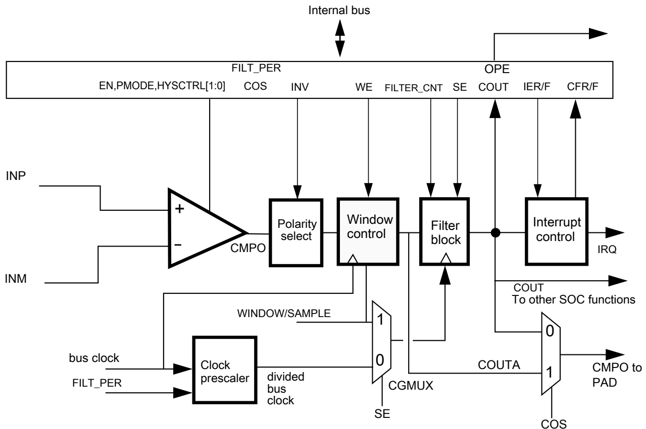
Figure 13-2. Comparator module block diagram
