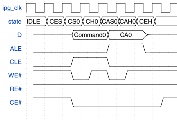
Figure 49-28. NAND Flash access Address type - One Byte Column Address
