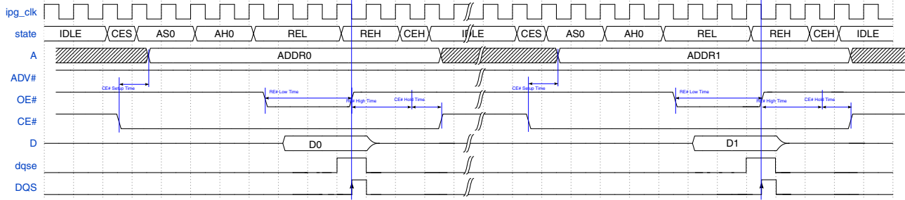
Figure 49-53. SRAM Read in ASYNC mode (Non-ADMUX)
