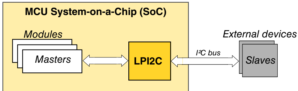
Figure 37-2. LPI2C connects masters in MCU to external slaves on PCB
