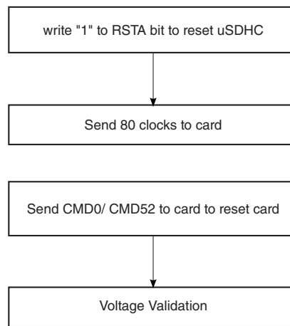
Figure 57-19. Flow Chart for Reset of the uSDHC and SD I/O Card
