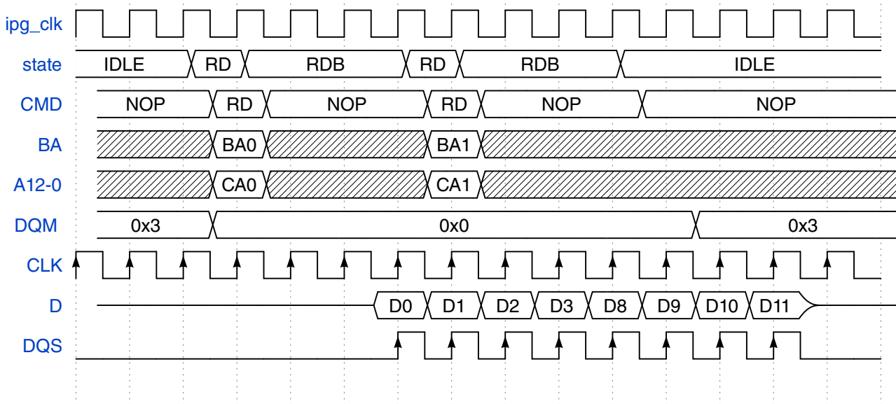
Figure 49-17. SDRAM Read-to-Read access (CL=3)
