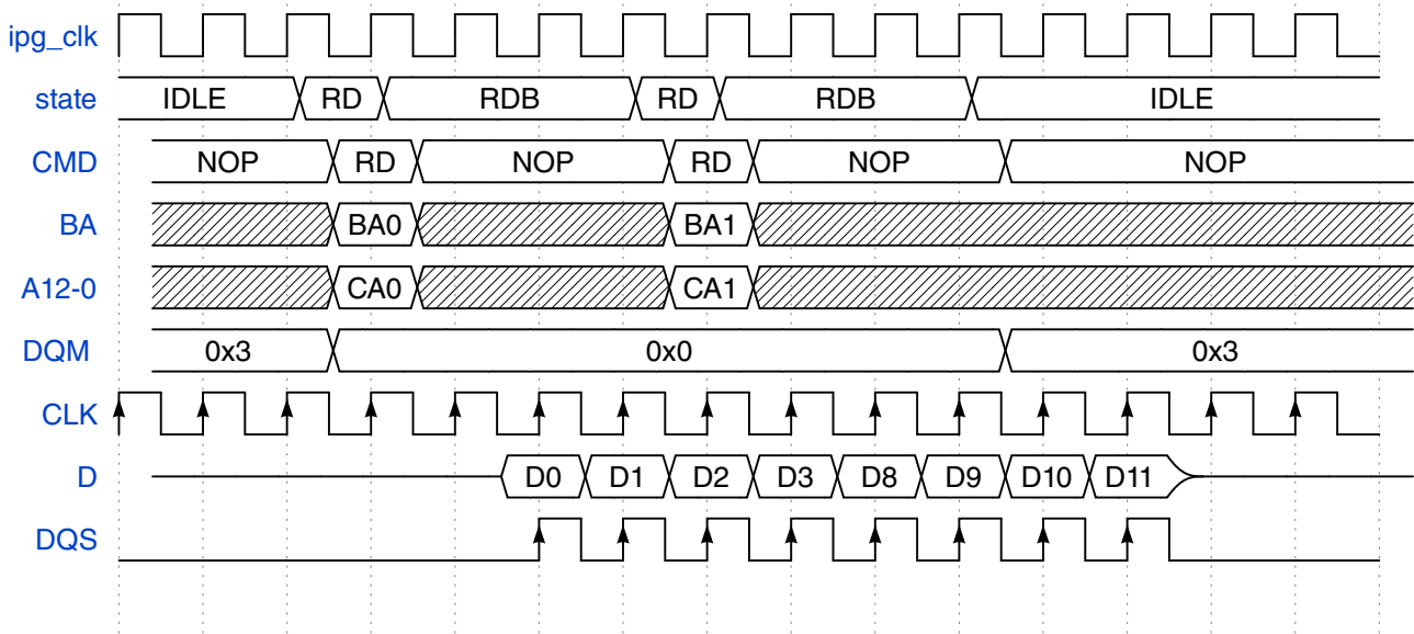
Figure 49-16. SDRAM Read-to-Read access (CL=2)
