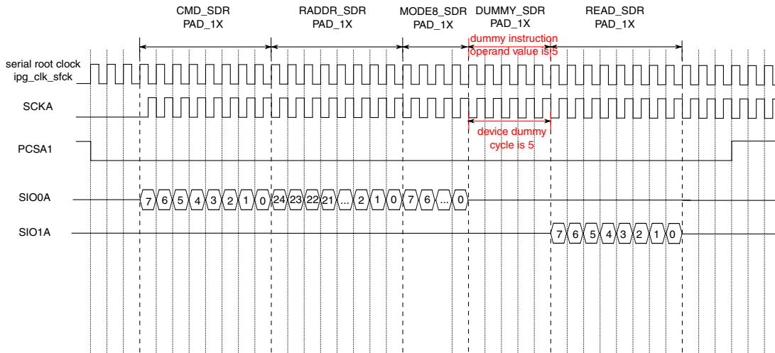
Figure 30-6. Flash access sequence example (SDR Single I/O Read sequence)
