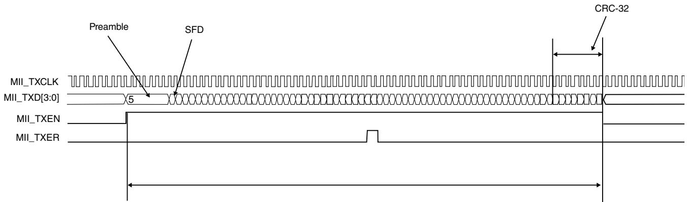
Figure 24-23. MII transmit operation — errored frame
