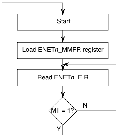
Figure 24-18. MDIO access overview
