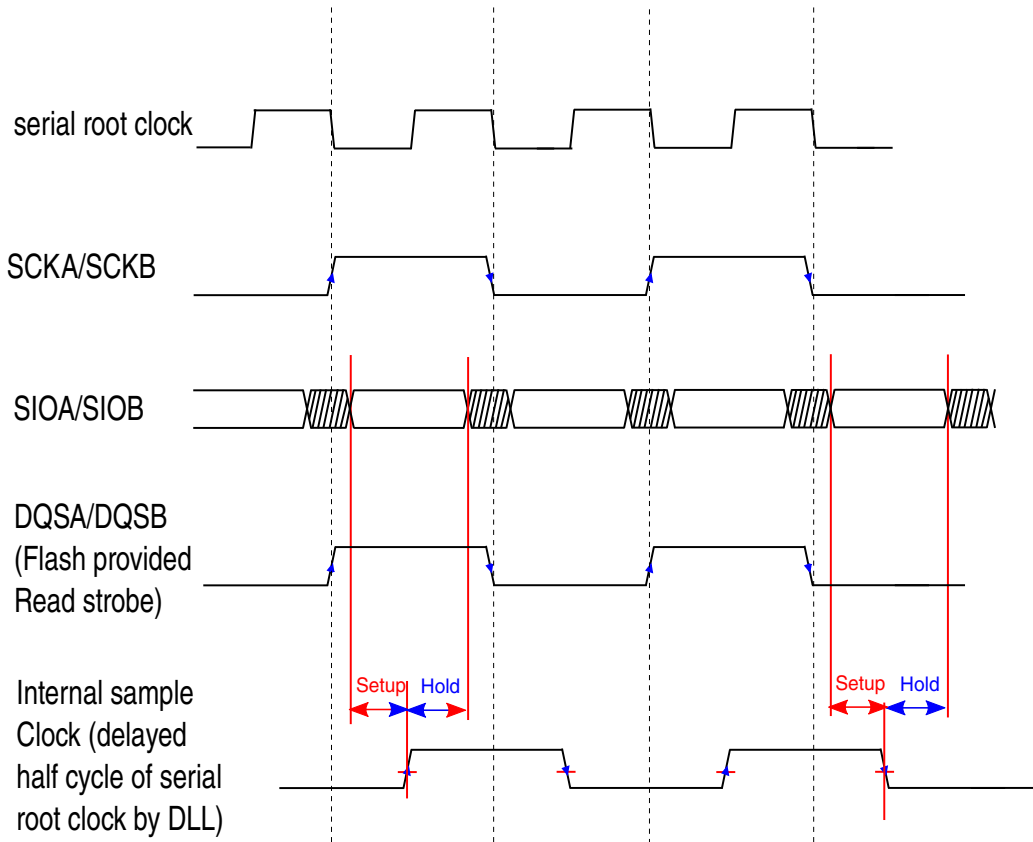
Figure 30-34. Input Timing 2 for Flash provided read strobe in DDR mode
