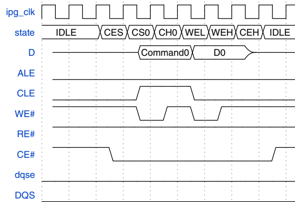
Figure 49-41. NAND Flash access command type - Command + Write Phase
