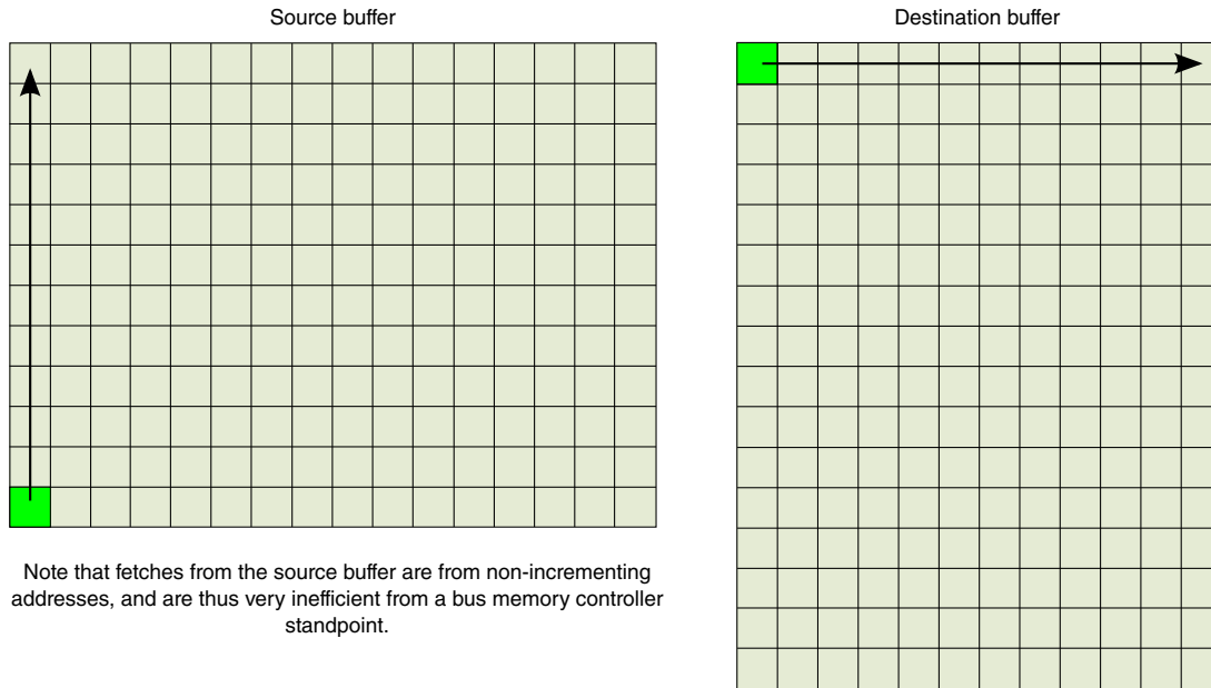
Figure 46-10. Rotation Read and Write
