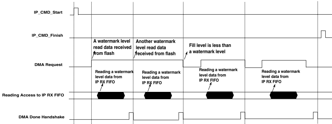
Figure 30-14. Reading from IP RX FIFO by DMA
