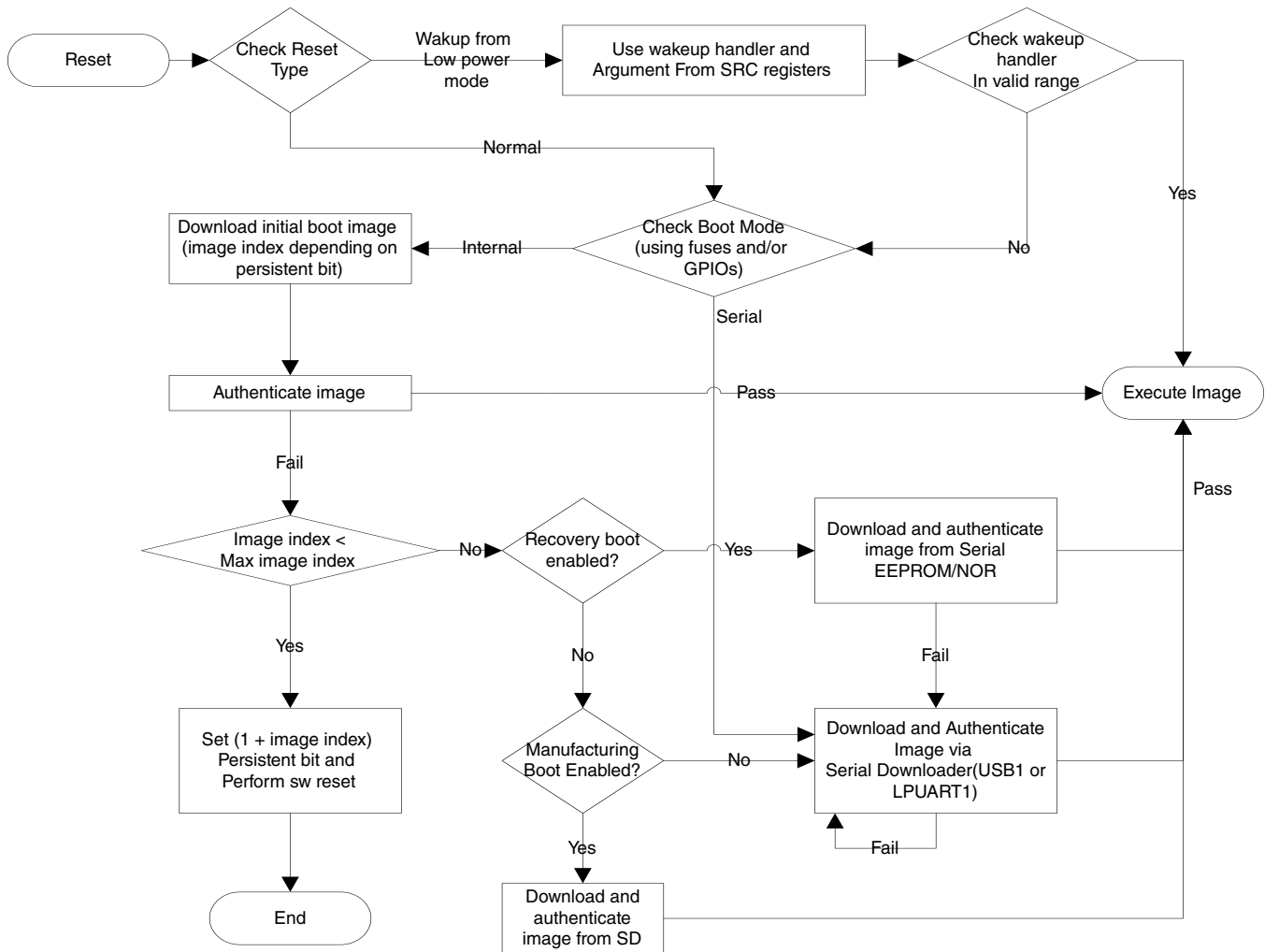
Figure 8-1. Boot flow
