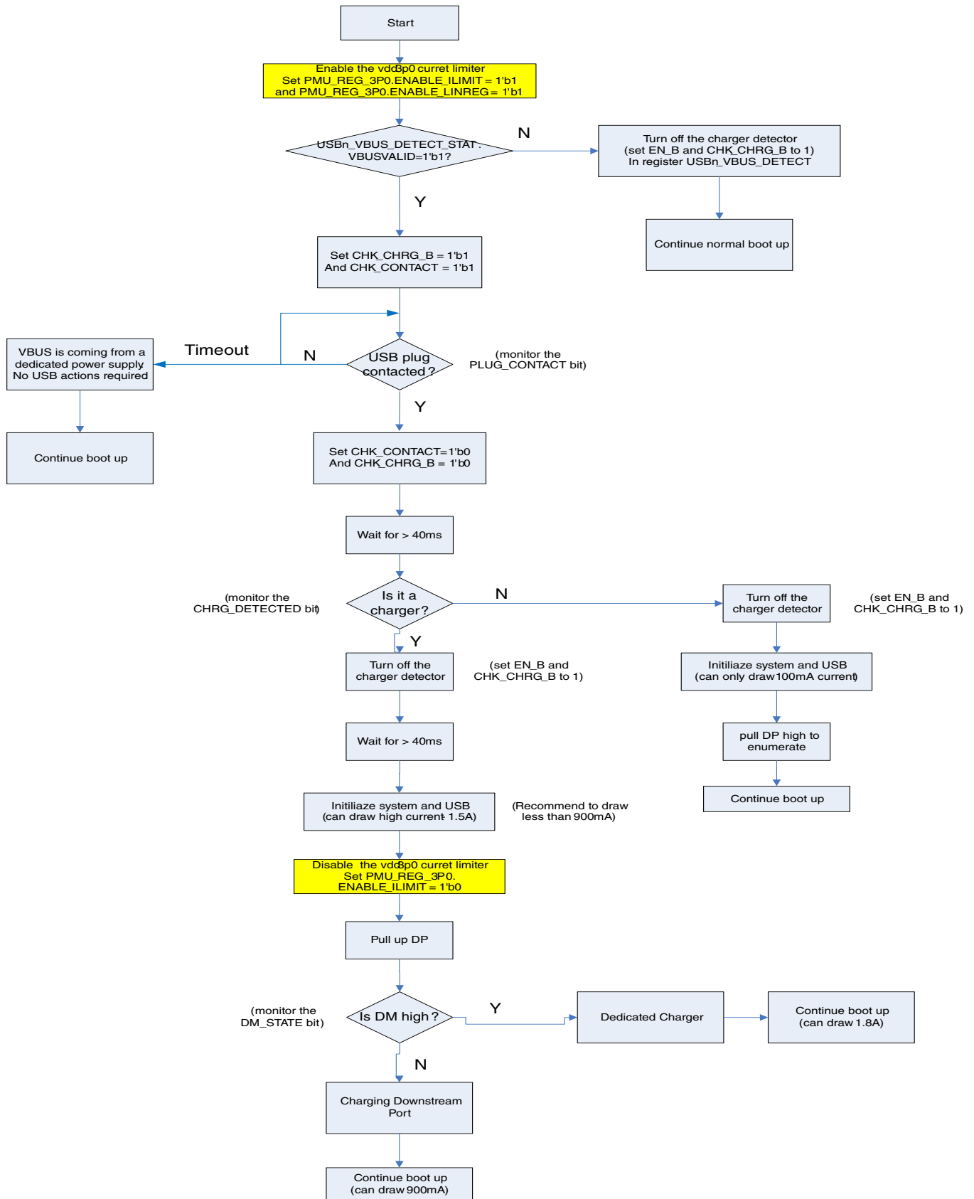
Figure 56-3. USBPHY Charger Detection Software Flow
