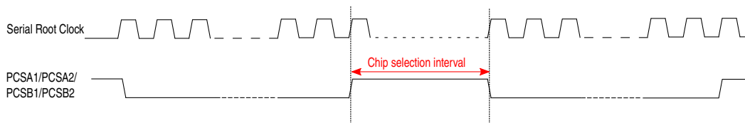
Figure 30-28. Chip Selection Valid interval
