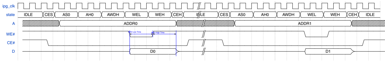
Figure 49-56. SRAM Write in ASYNC mode (Non-ADMUX)
