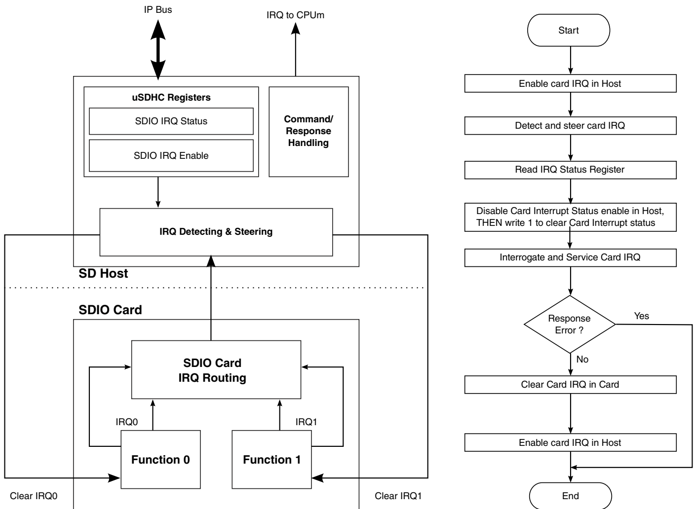
Figure 57-15. Card Interrupt Scheme and Card Interrupt Detection and Handling Procedure
