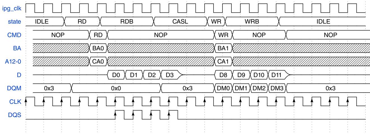
Figure 49-18. SDRAM Read-to-Write access (CL=1)
