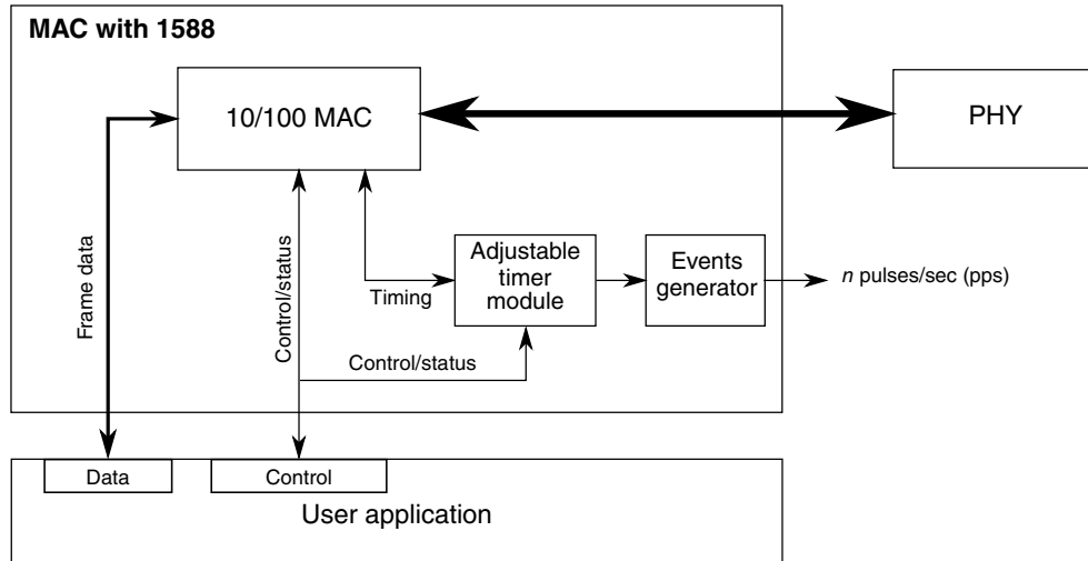
Figure 24-9. IEEE 1588 functions overview
