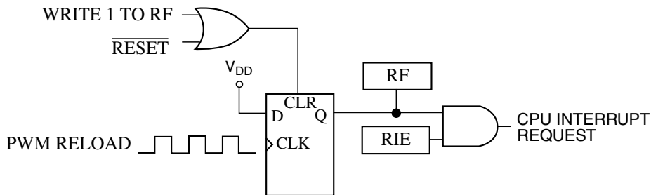
Figure 28-34. PWMF Reload Interrupt Request
