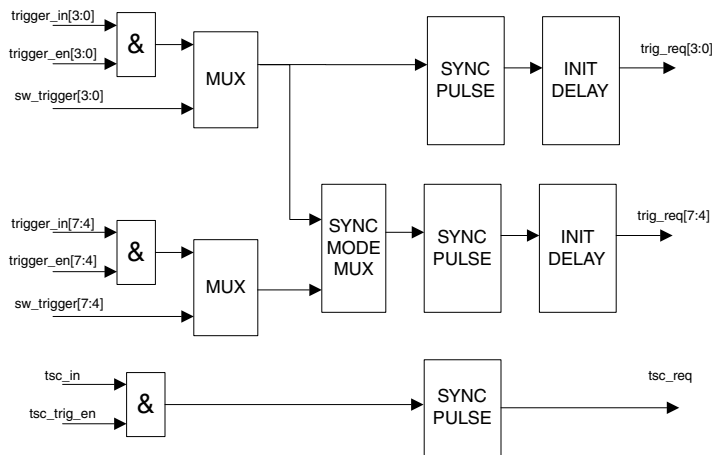
Figure 15-2. Trigger process diagram
