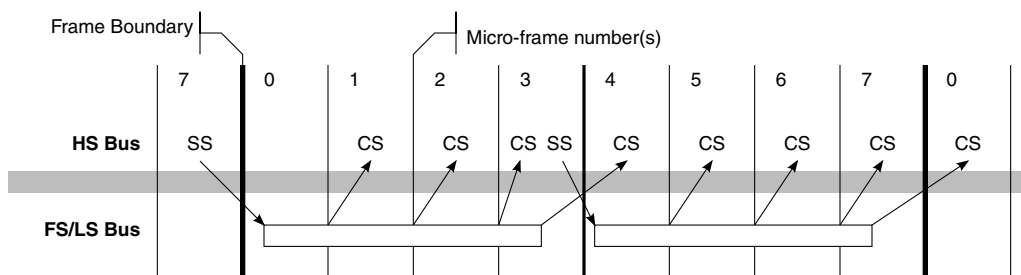
Figure 55-9. Frame Boundary Relationship between HS bus and FS/LS Bus
