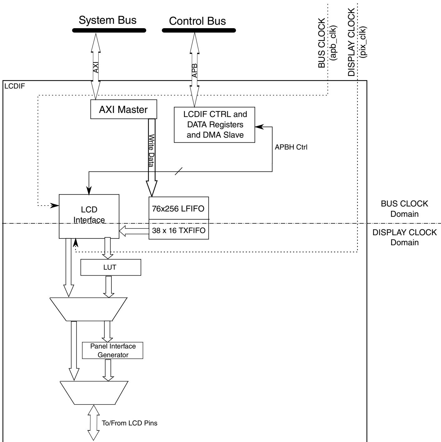
Figure 36-1. Top-Level Block Diagram of LCDIF subsystem
