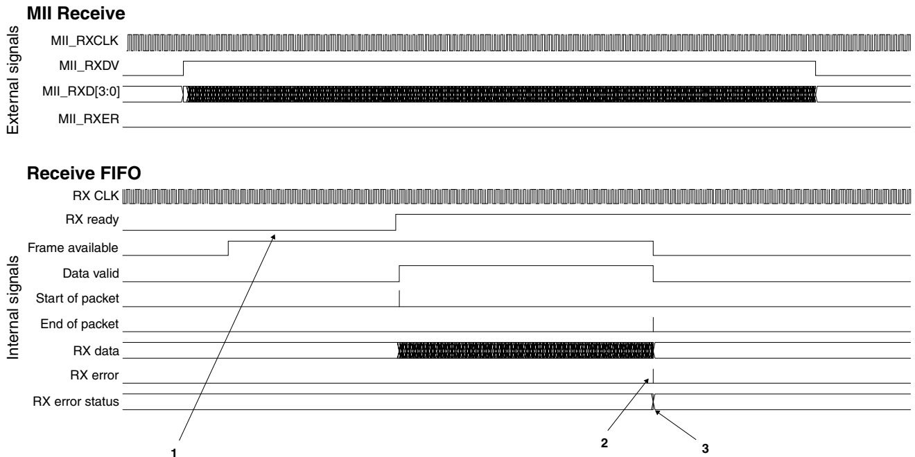
Figure 24-17. Receive FIFO overflow protection
