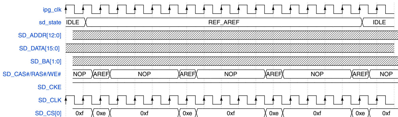
Figure 49-25. Refresh command - SDRAM Auto Refresh
