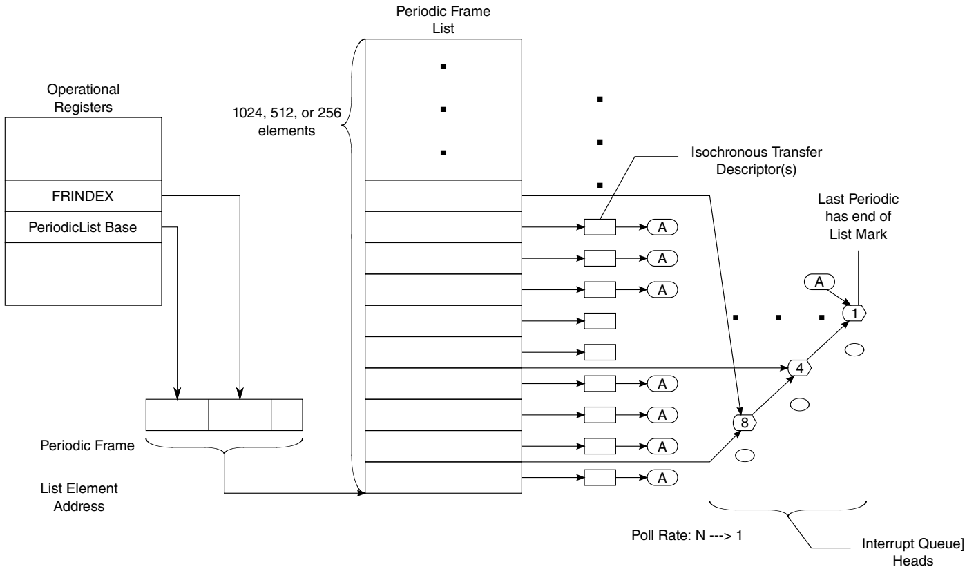
Figure 55-2. Periodic Schedule Organization
