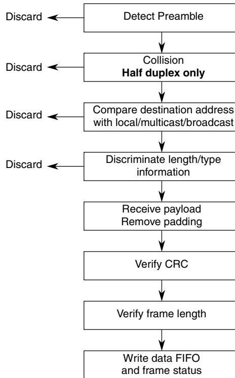
Figure 24-5. MAC receive flow
