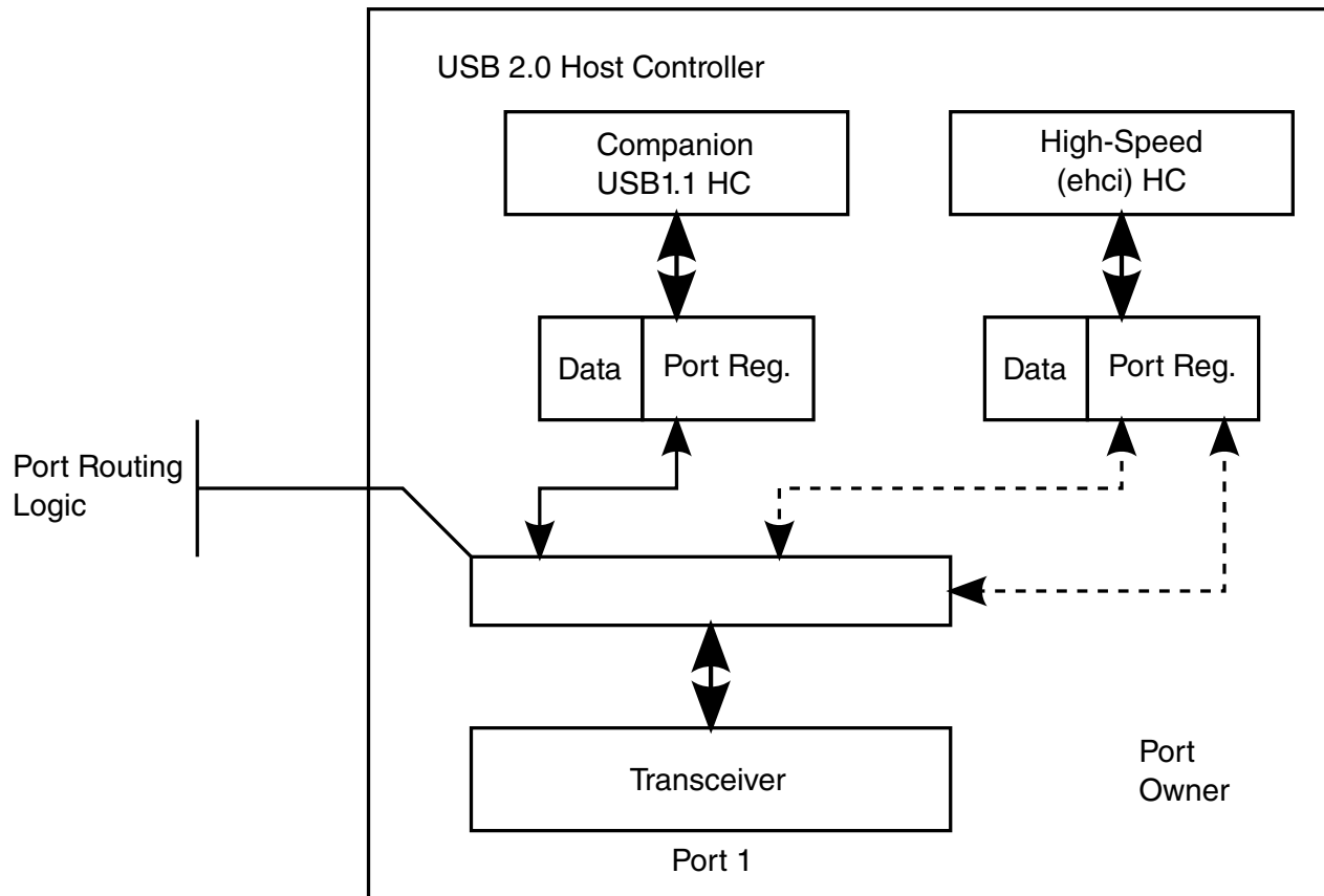
Figure 55-4. Example USB 2.0 Host Controller Port Routing Block Diagram
