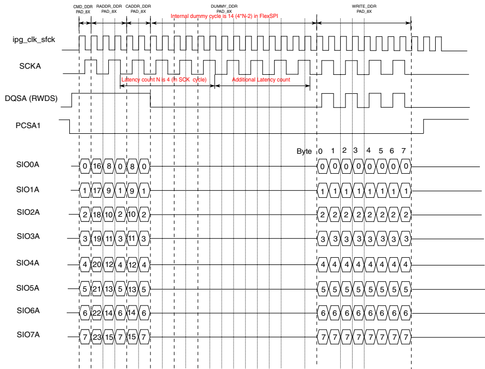
Figure 30-12. HyperBus device write transaction with additional latency count
