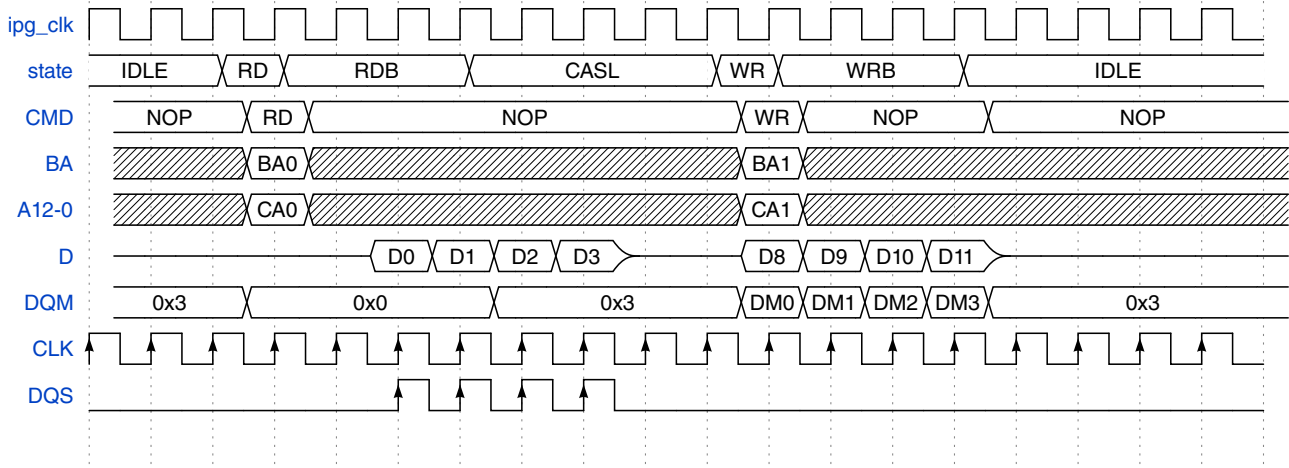
Figure 49-19. SDRAM Read-to-Write access (CL=2)
