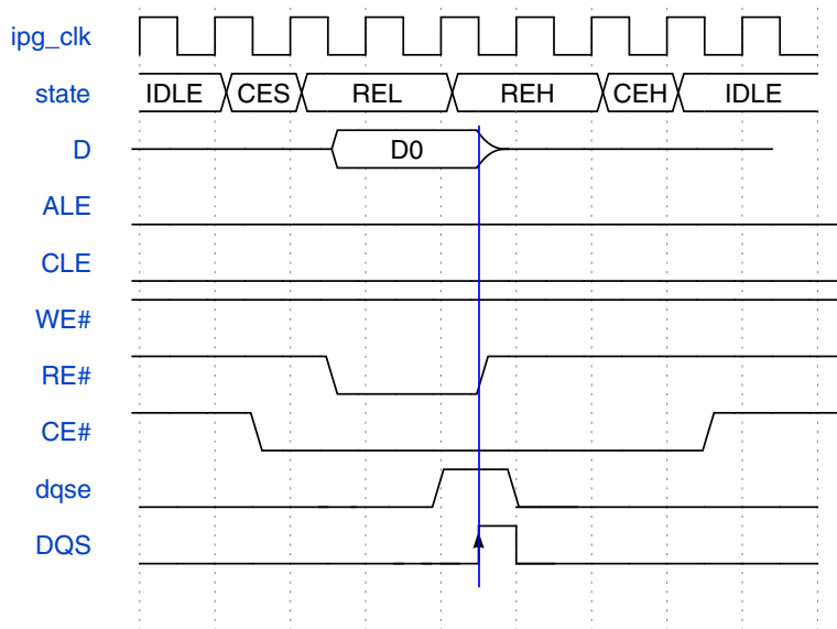
Figure 49-42. NAND Flash access command type - Read Phase Only
