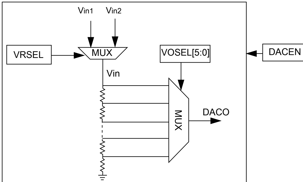
Figure 13-12. 6-bit DAC block diagram
