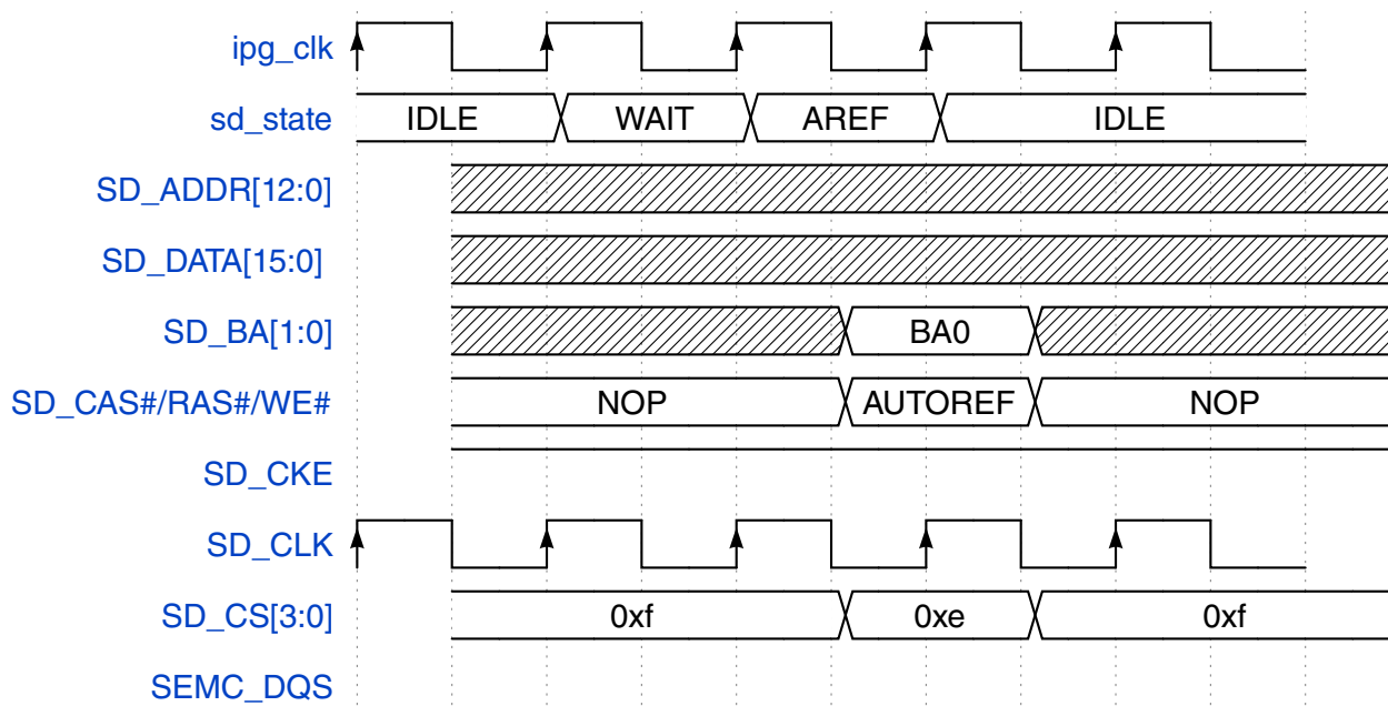
Figure 49-4. IP command - SDRAM Auto Refresh
