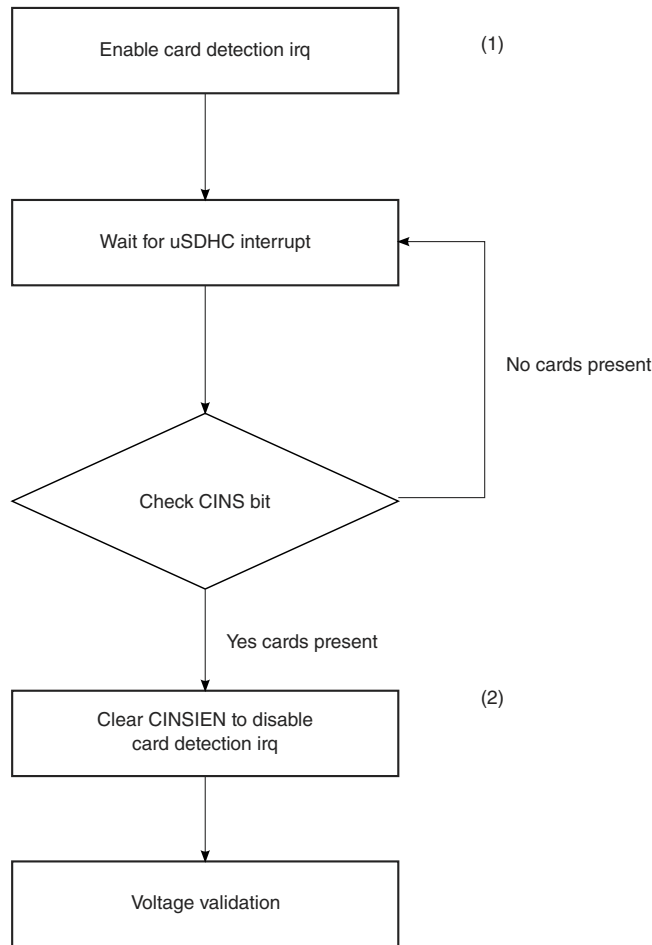
Figure 57-18. Flow Diagram for Card Detection
