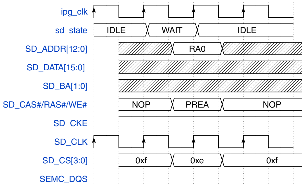
Figure 49-7. IP command - SDRAM PRECHARGE ALL
