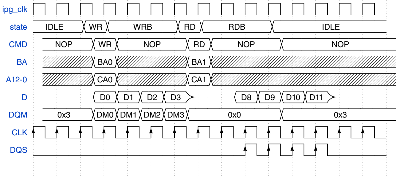
Figure 49-23. SDRAM Write-to-Read access (CL=2)
