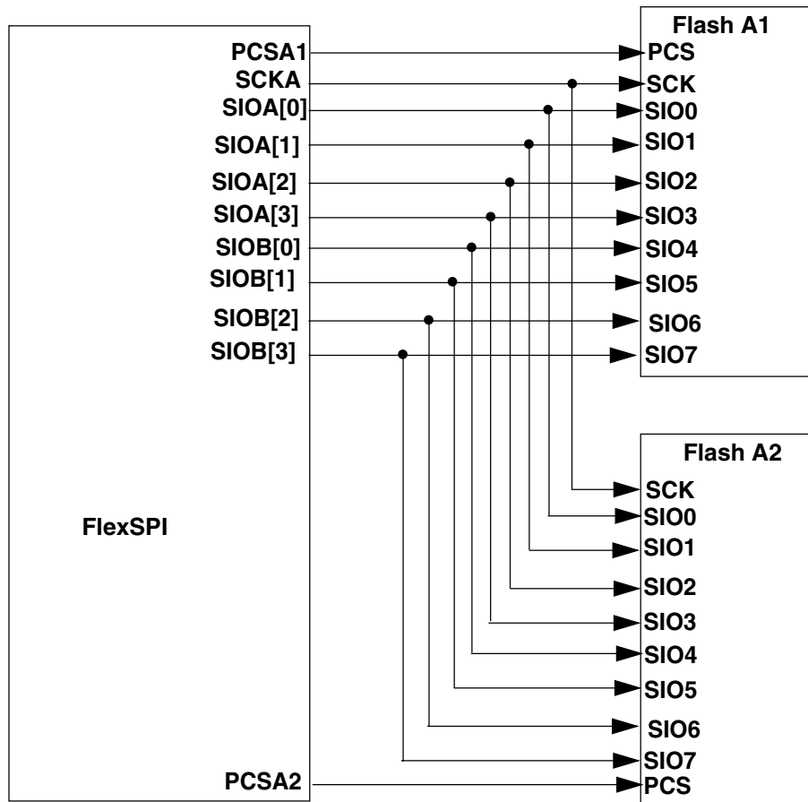
Figure 30-3. Flash connection diagram with combination mode
