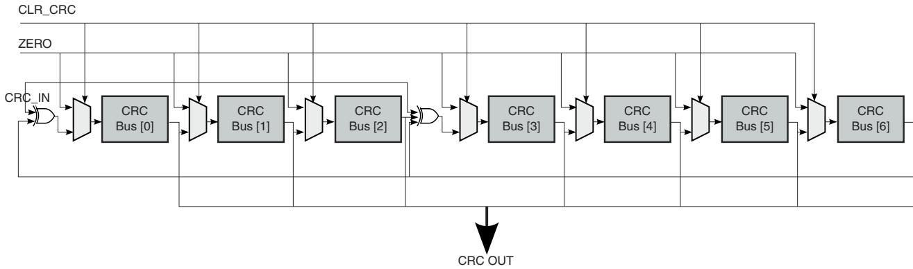
Figure 57-13. Command CRC Shift Register
