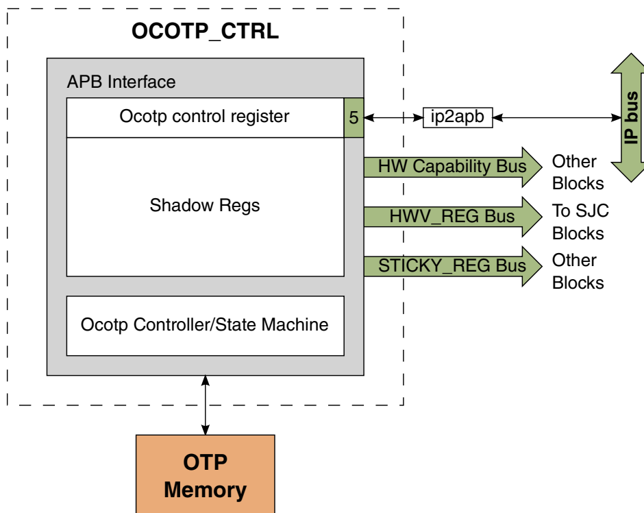
Figure 42-1. OCOTP System Level Diagram
