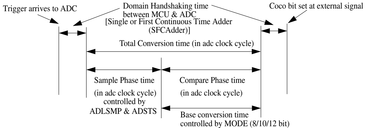
Figure 14-4. ADC conversion time details
