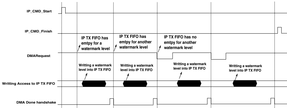
Figure 30-16. Filling from IP TX FIFO by DMA
