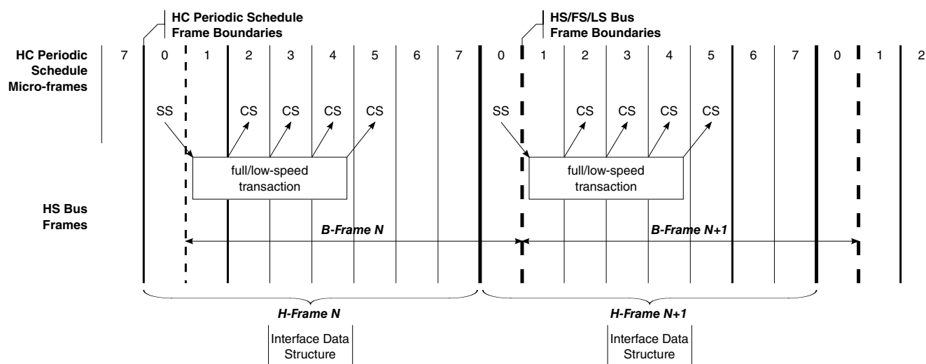
Figure 55-10. Relationship of Periodic Schedule Frame Boundaries to Bus Frame Boundaries
