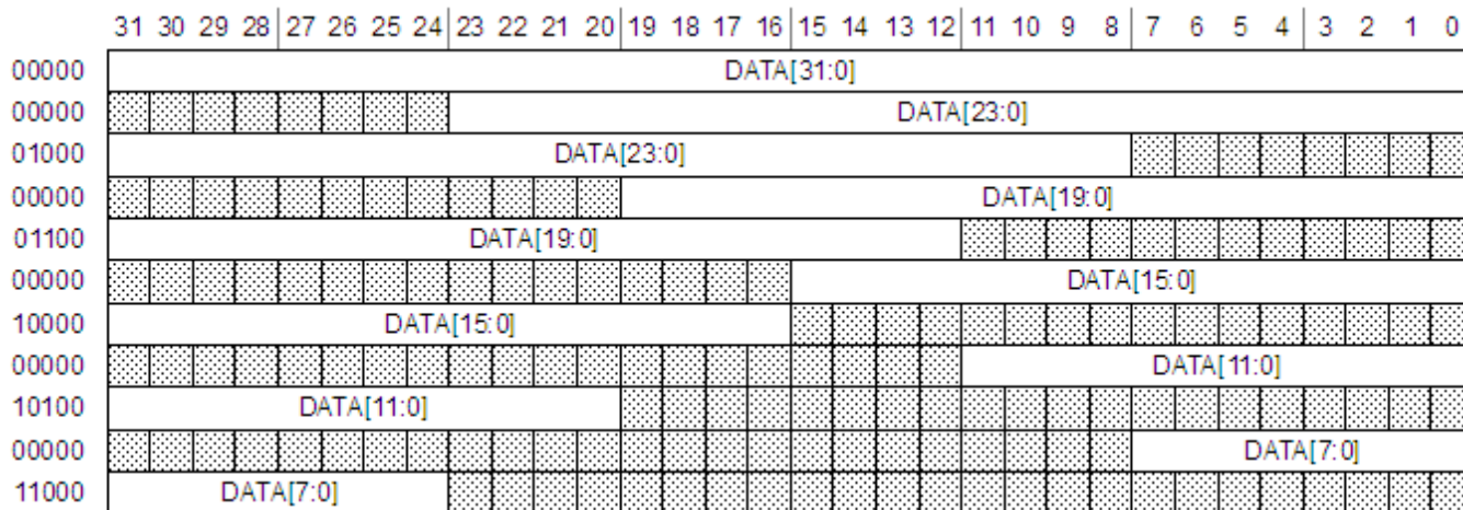
Figure 48-2. SAI first bit shifted, LSB first
