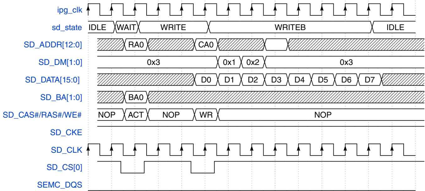
Figure 49-10. IP command - SDRAM WRITE
