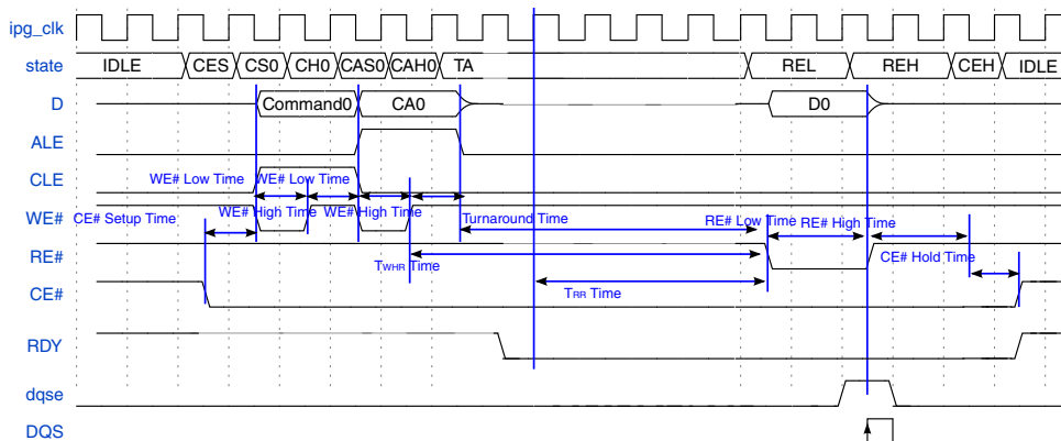
Figure 49-38. NAND Flash access command type - Command + Address + Read Phase
