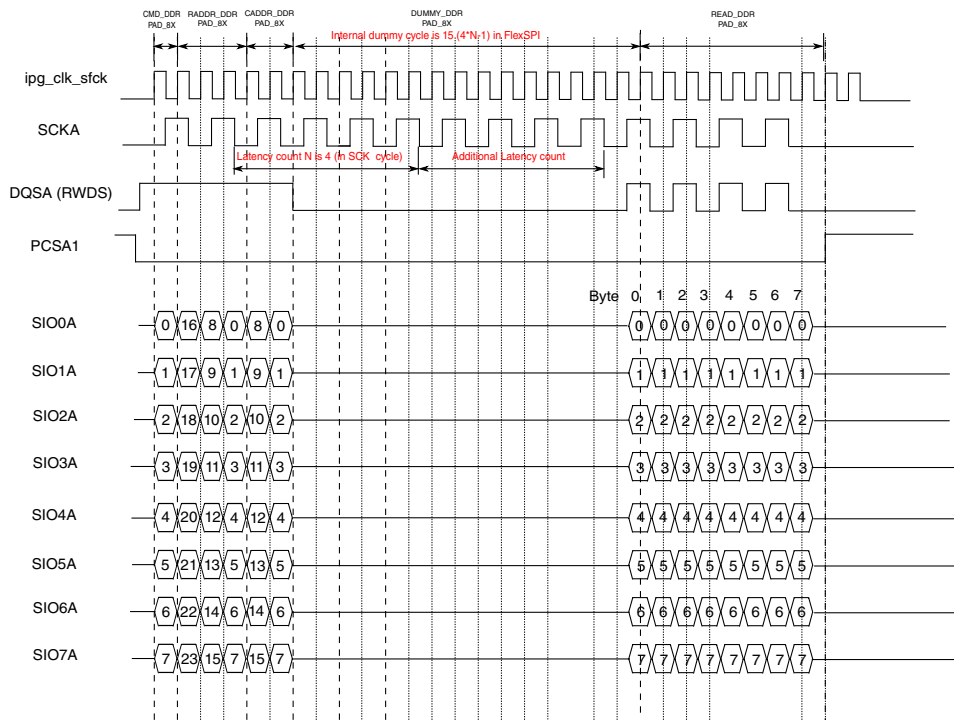
Figure 30-10. HyperBus device read transaction with additional latency count
