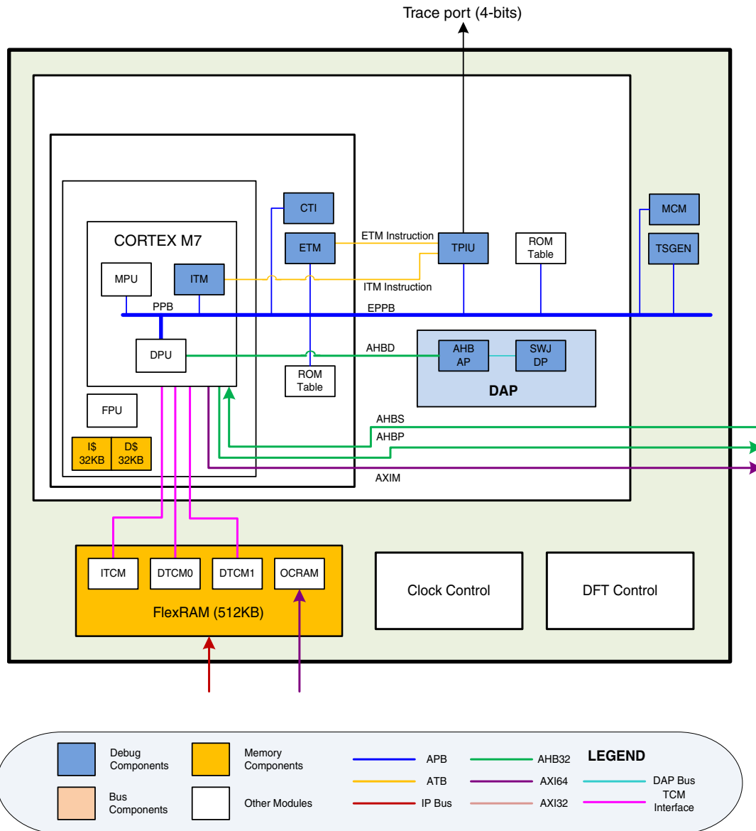
Figure 12-1. Cortex-M7 Platform Block Diagram
