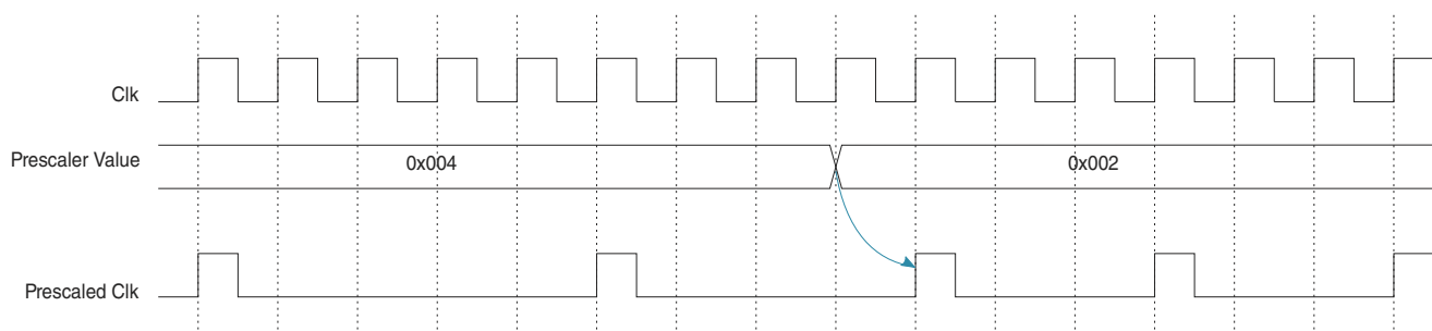
Figure 33-3. Prescaler Value Change Timing Diagram
