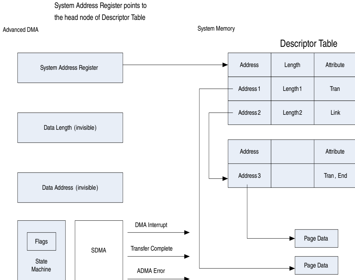
Figure 57-11. Concept and Access Method of ADMA2 Descriptor Table
