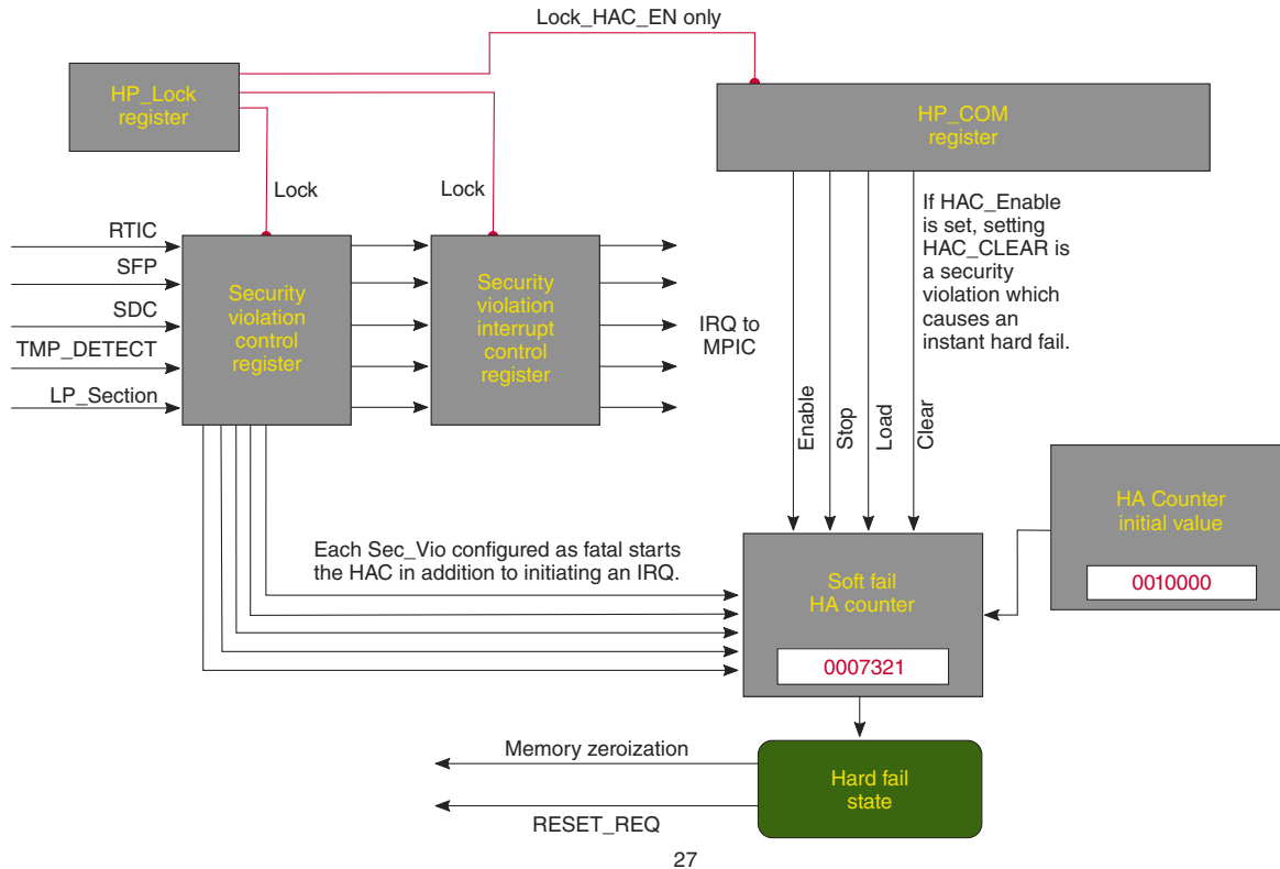
Figure 50-1. Relationship Between the Registers
