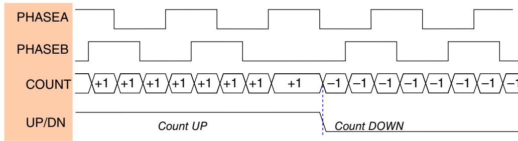
Figure 23-3. Quadrature Decoder Signals
