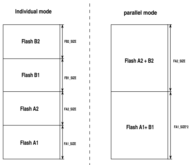
Figure 30-4. Flash memory map in individual and parallel mode
