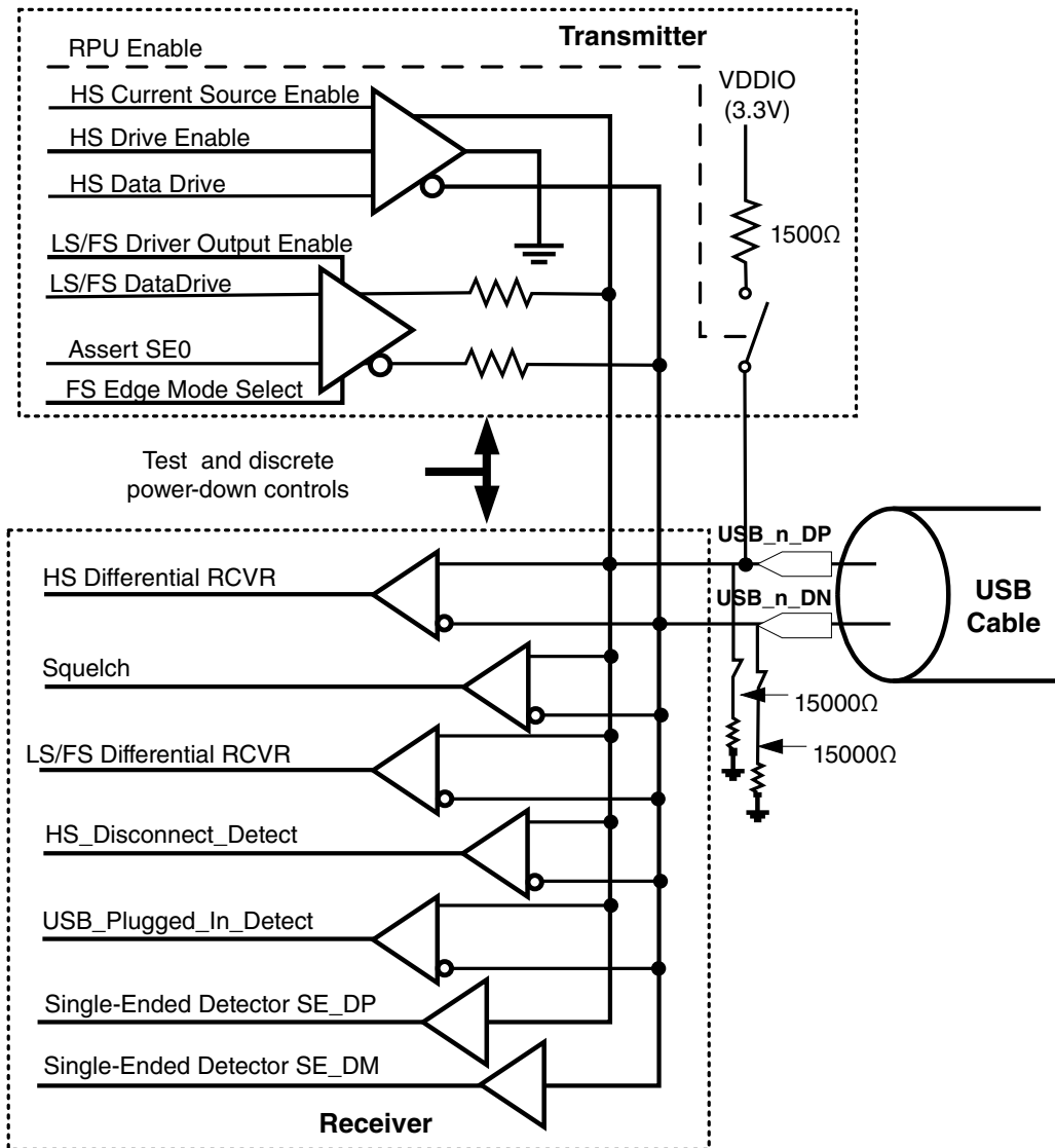
Figure 56-1. USB 2.0 PHY Analog Transceiver Block Diagram
