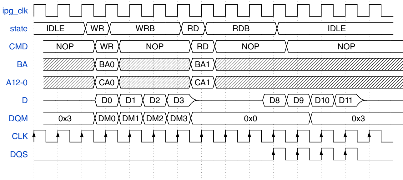
Figure 49-24. SDRAM Write-to-Read access (CL=3)
