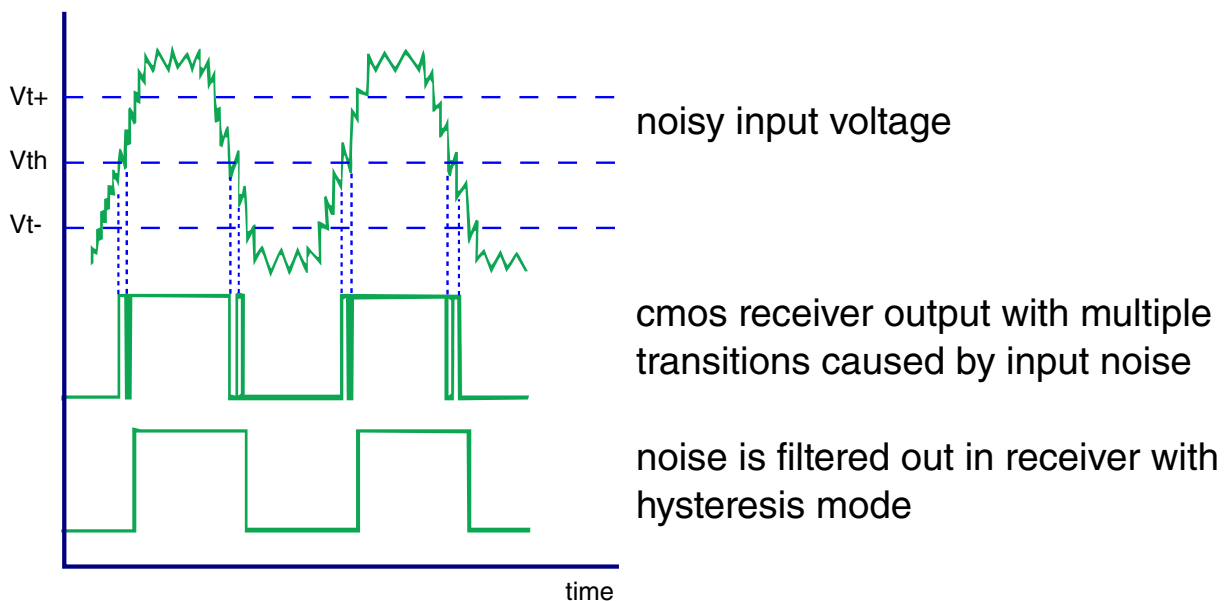
Figure 32-5. Receiver output in CMOS and hysteresis
