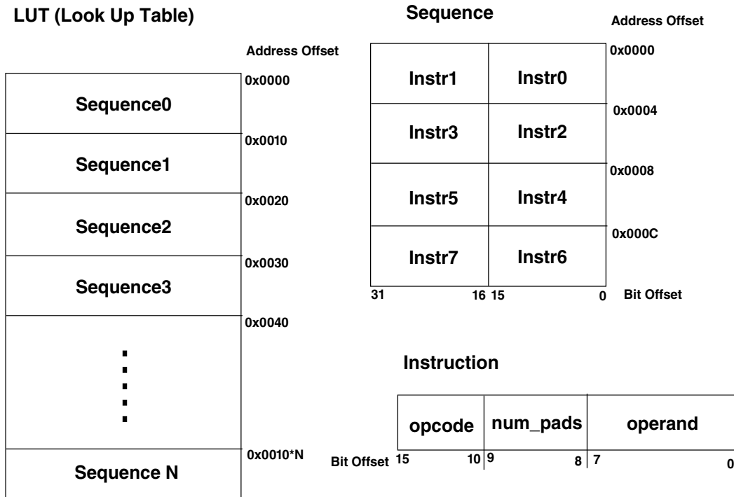
Figure 30-5. LUT and sequence structure
