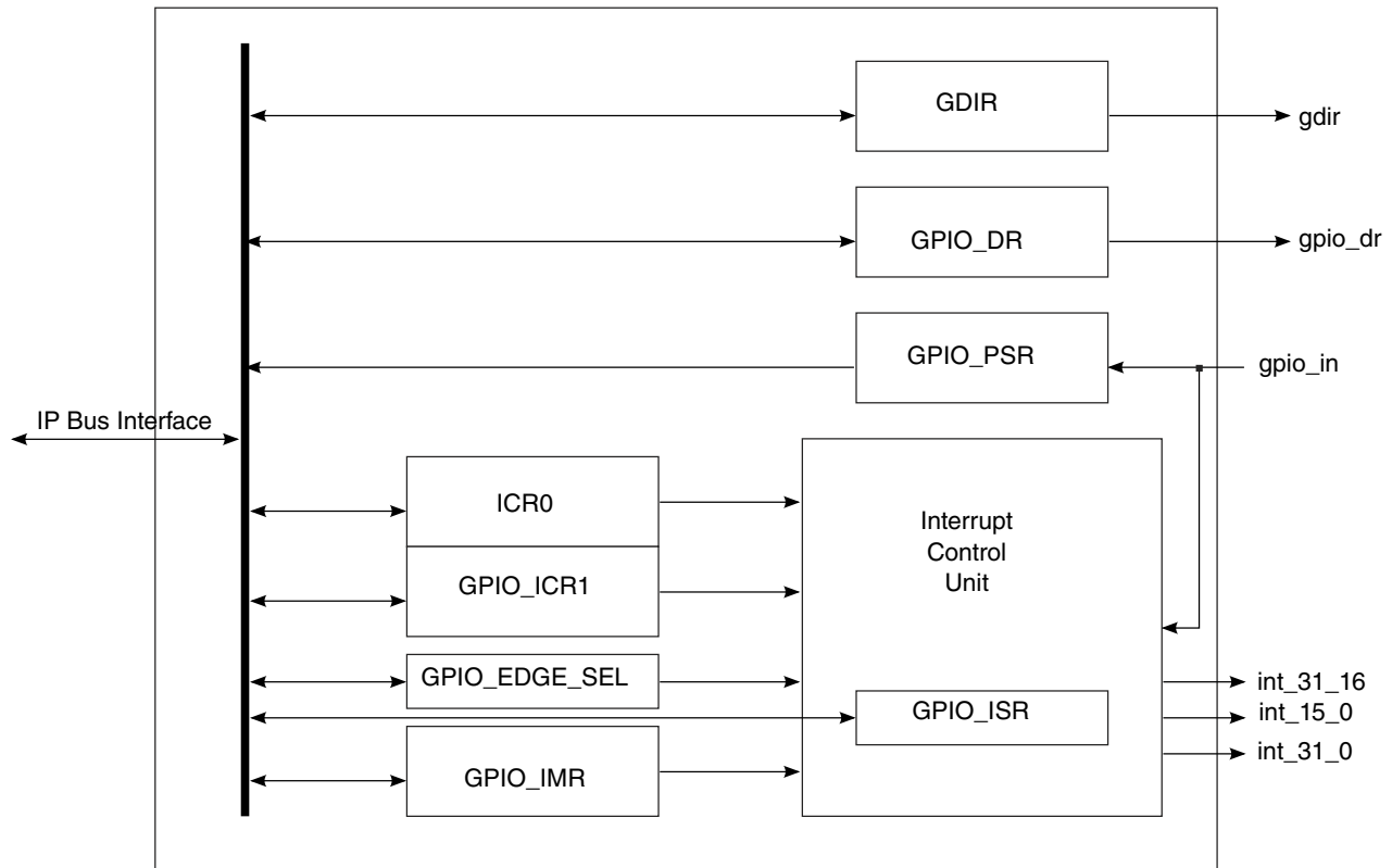
Figure 32-2. GPIO Block Diagram
