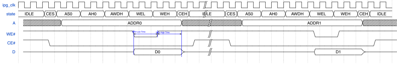
Figure 49-50. Flash Write in ASYNC mode (Non-ADMUX)
