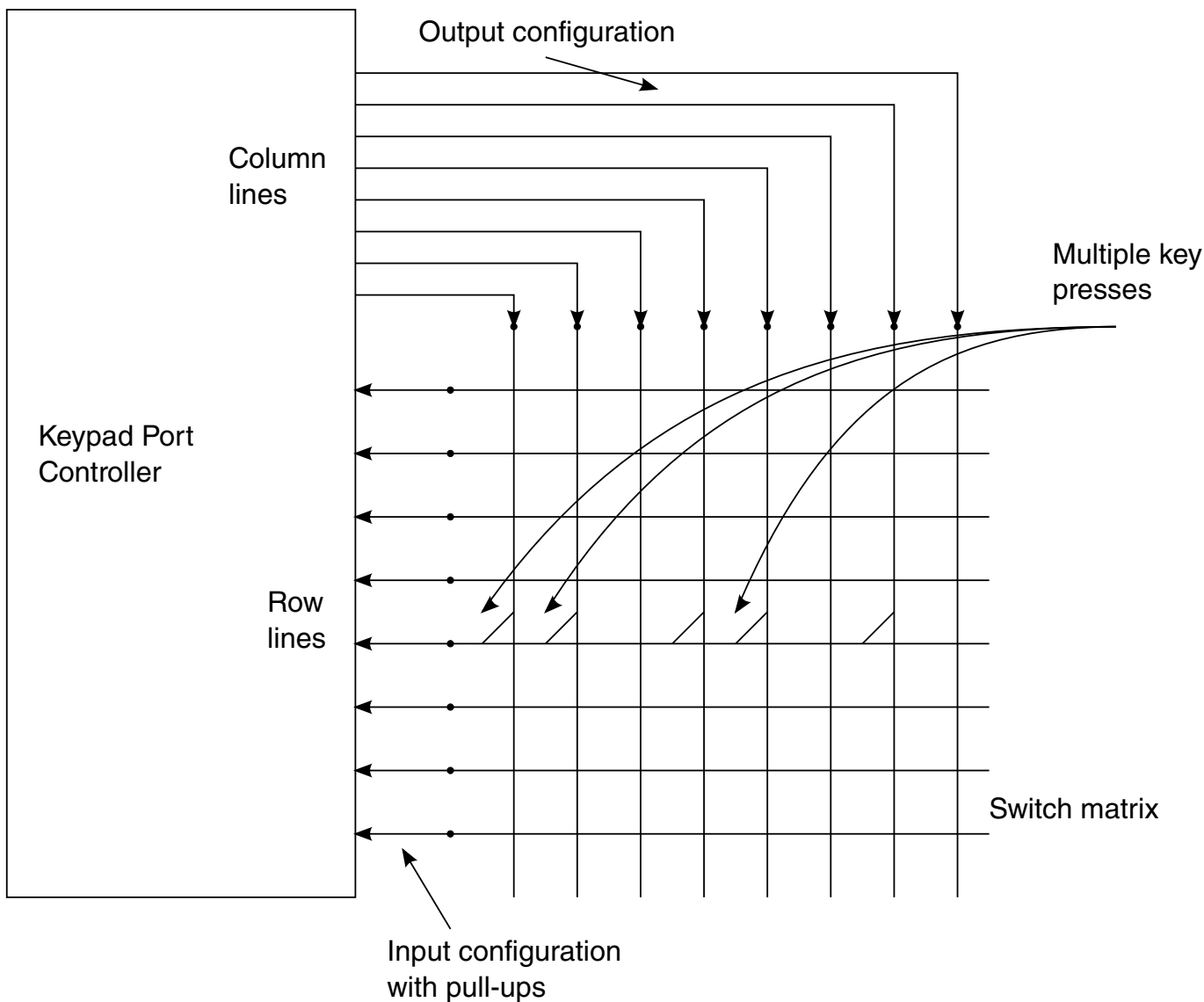
Figure 35-4. Multiple Key Presses on Same Row Line (Simplified View)
