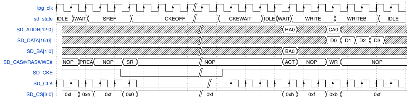
Figure 49-3. IP command - SDRAM Self Refresh
