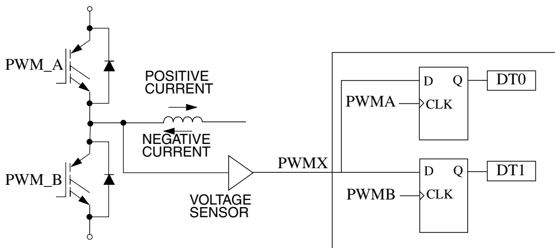
Figure 28-23. Current-status Sense Scheme for Deadtime Correction
