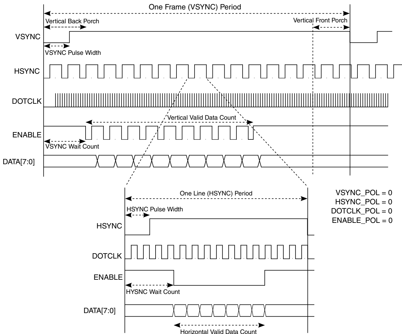
Figure 36-7. DOTCLK protocol with programmable parameters
