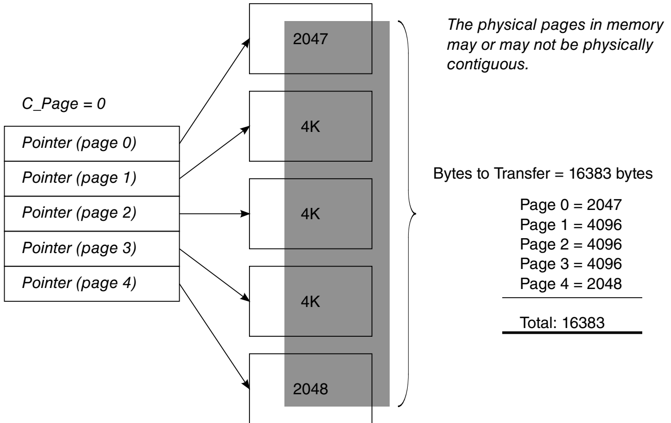
Figure 55-18. Example Mapping of qTD Buffer Pointers to Buffer Pages
