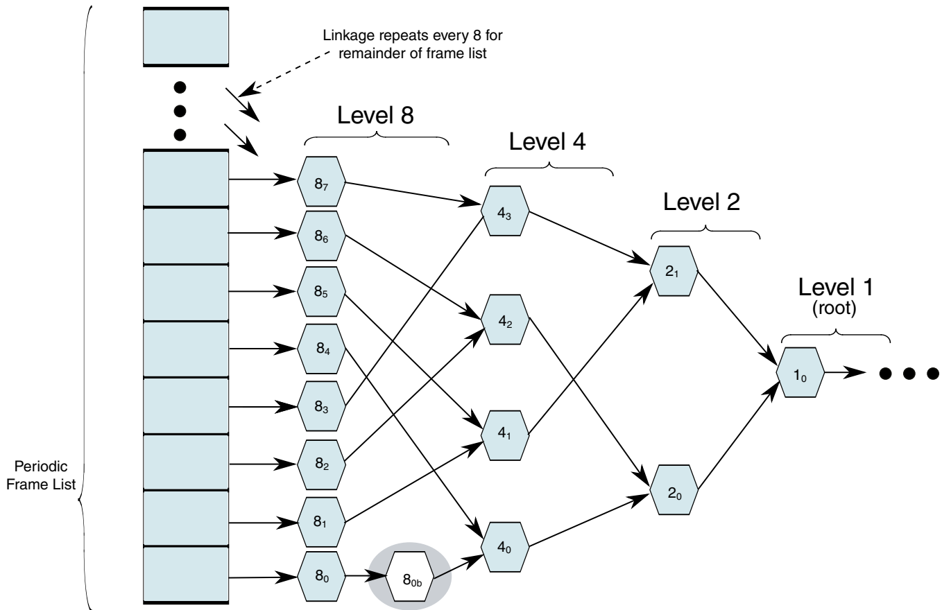
Figure 55-21. General Structure of EHCI Periodic Schedule Utilizing Interrupt Spreading
