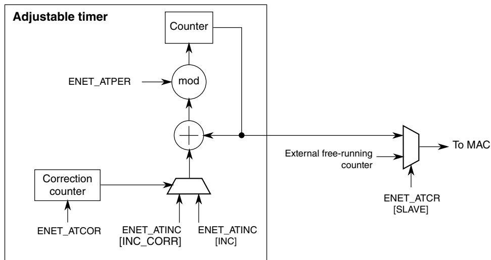
Figure 24-10. Adjustable timer implementation detail
