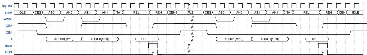
Figure 49-55. SRAM Read in ASYNC mode (AADM)
