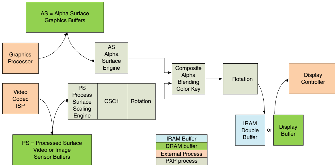
Figure 46-1. PXP Architecture
