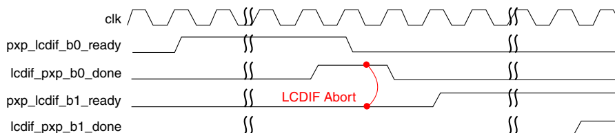
Figure 46-17. LCDIF Abort
