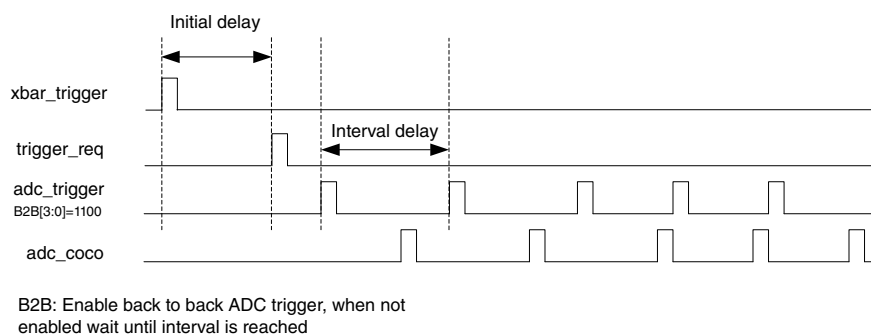
Figure 15-3. ETC ADC interface timing
