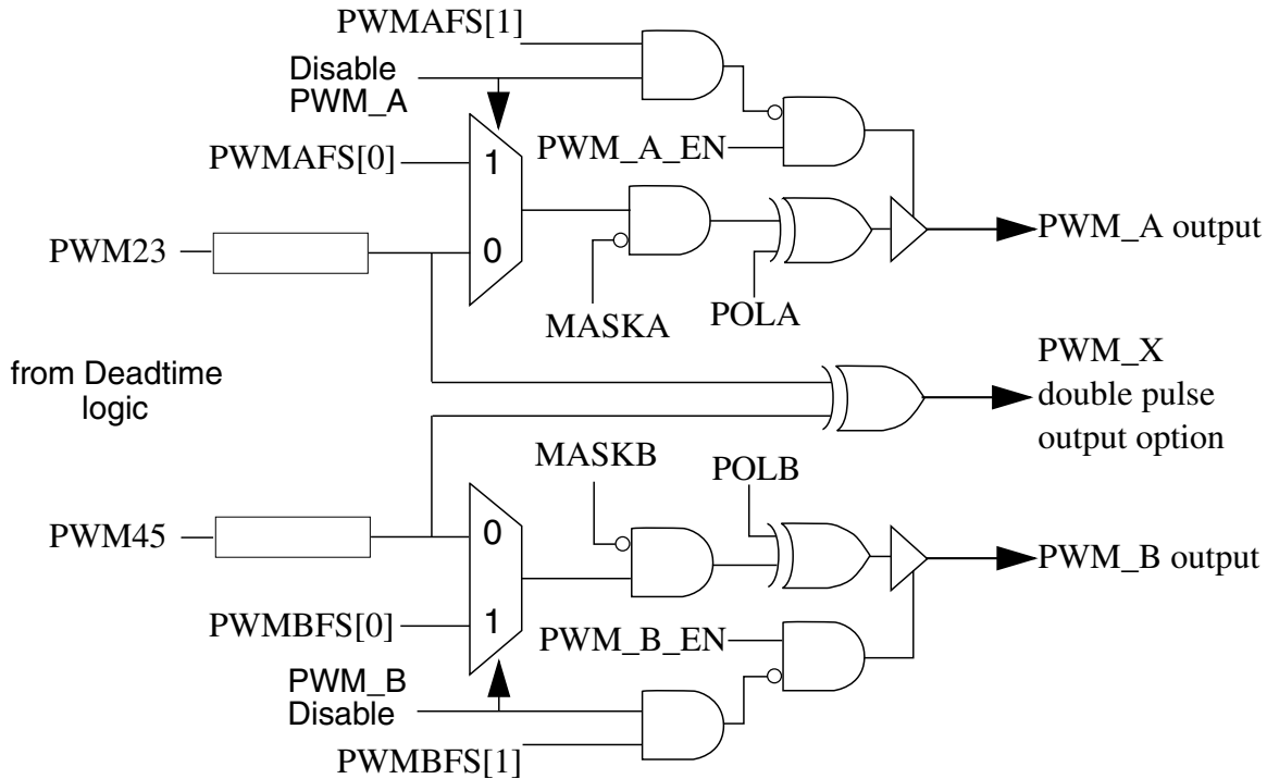
Figure 28-25. Output Logic
