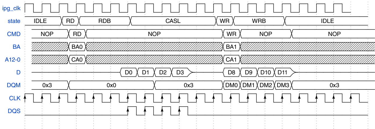
Figure 49-20. SDRAM Read-to-Write access (CL=3)
