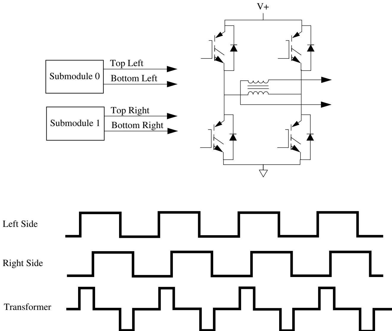
Figure 28-5. Phase Shifted PWMs Applied to a Transformer Primary
