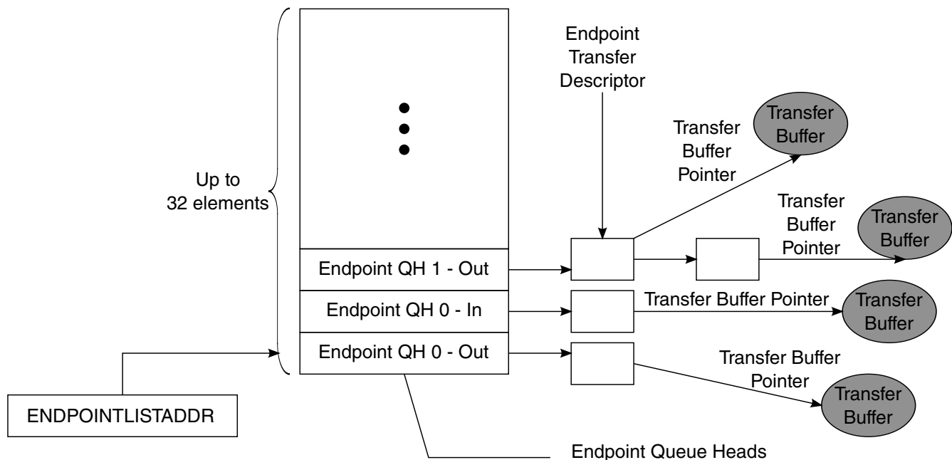
Figure 55-27. EndPoint Queue Head Organization
