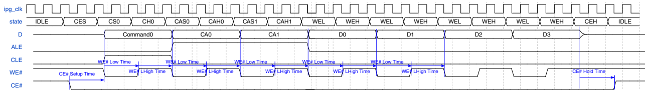
Figure 49-45. NAND Flash access command type - Command + Address + Write Phase
