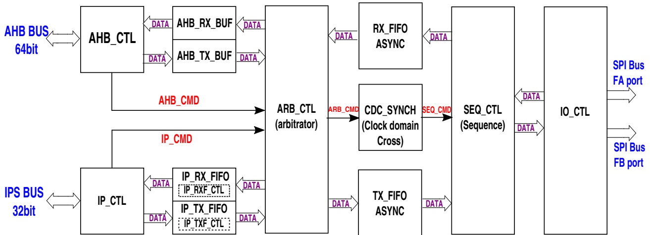
Figure 30-1. FlexSPI block diagram
