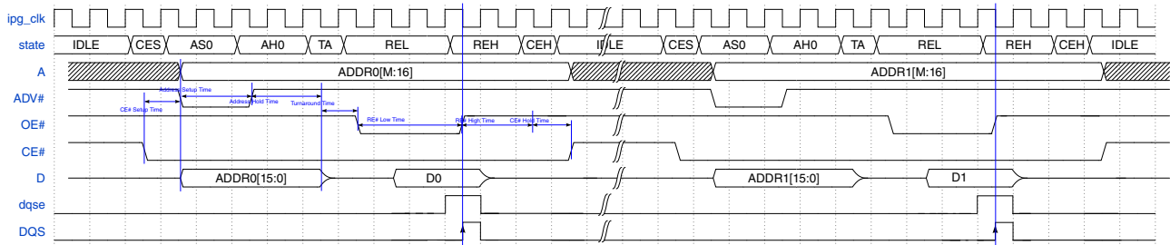
Figure 49-54. SRAM Read in ASYNC mode (ADMUX)
