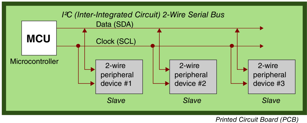
Figure 37-5. 2-Wire scheme
