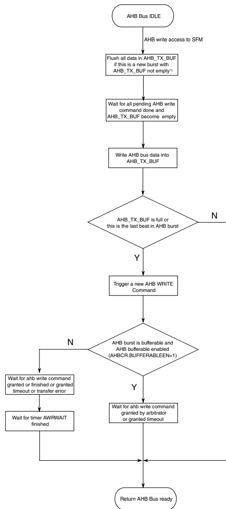
Figure 30-17. Hardware operation in response to AHB write access to Flash
