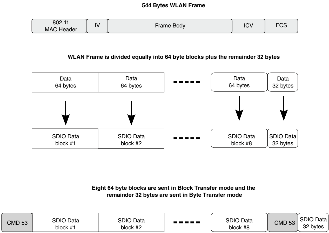
Figure 57-6. Example for Dividing Large Data Transfers
