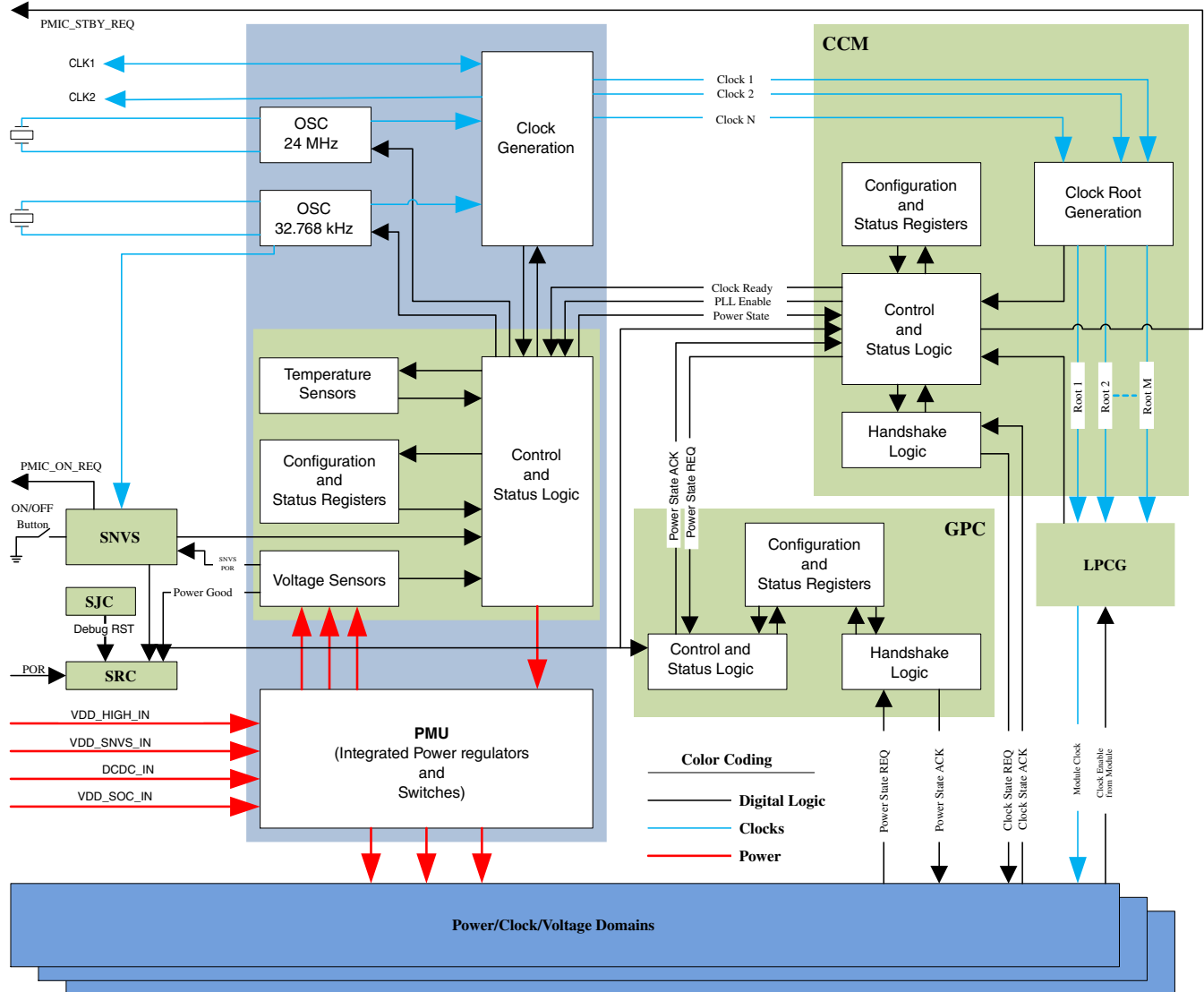
Figure 10-1. Power and clock management framework
