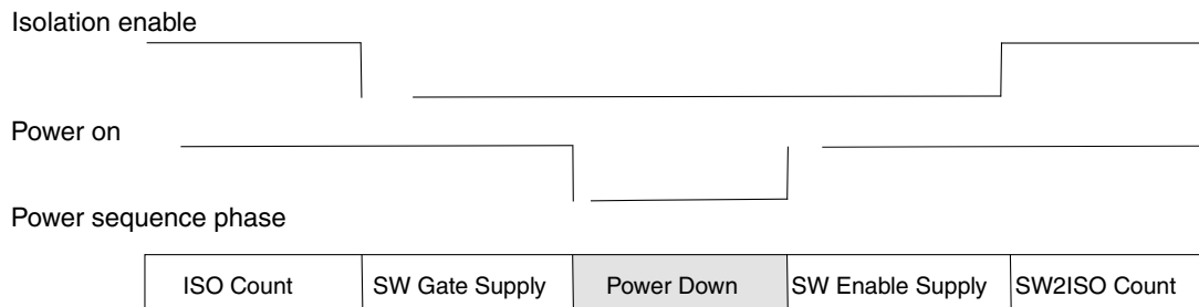
Figure 10-8. PDRAMx isolation and power on switch flow
