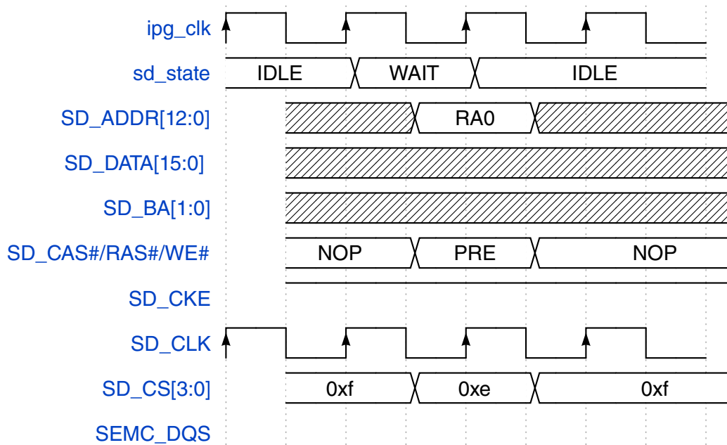
Figure 49-6. IP command - SDRAM PRECHARGE
