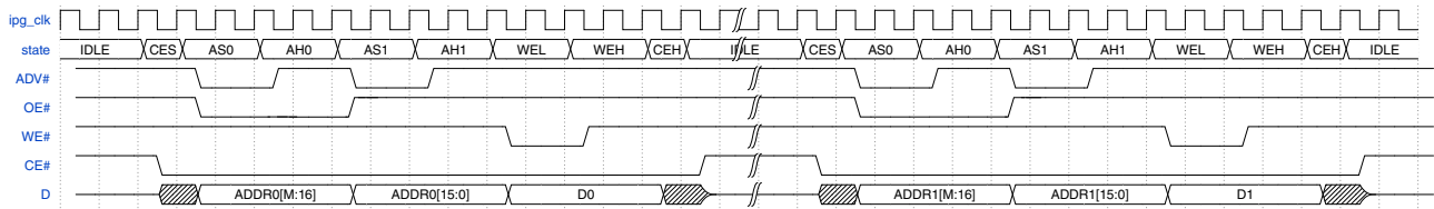
Figure 49-52. Flash Write in ASYNC mode (AADM)
