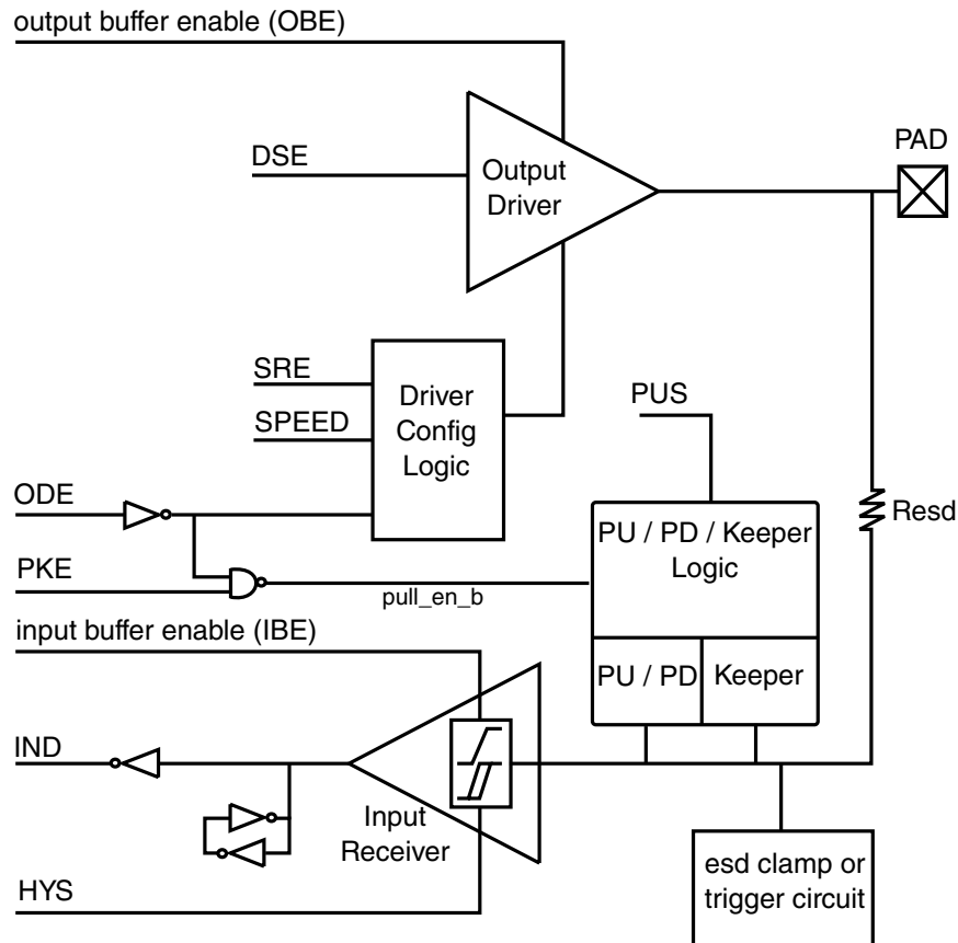
Figure 32-3. GPIO pad functional diagram
