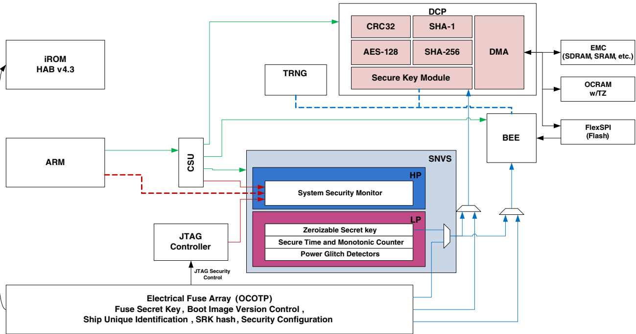
Figure 11-1. Security subsystem (simplified)
