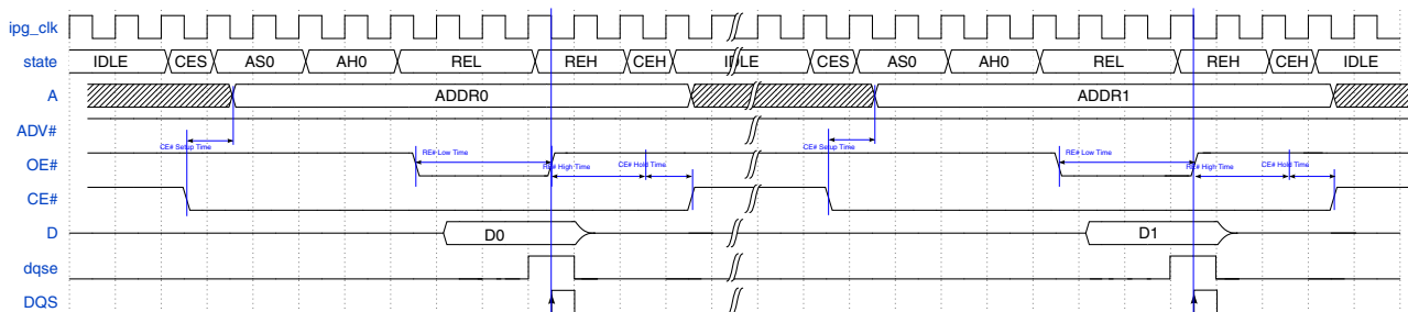
Figure 49-47. Flash Read in ASYNC mode (Non-ADMUX)
