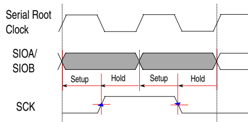
Figure 30-25. DDR instruction in DDR sequence
