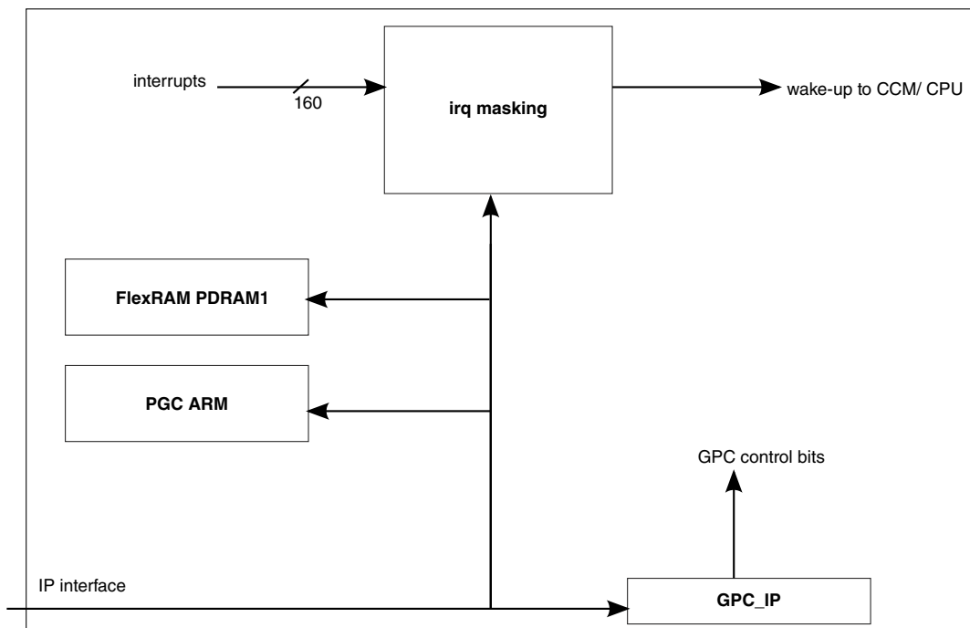
Figure 31-1. GPC Block Diagram
