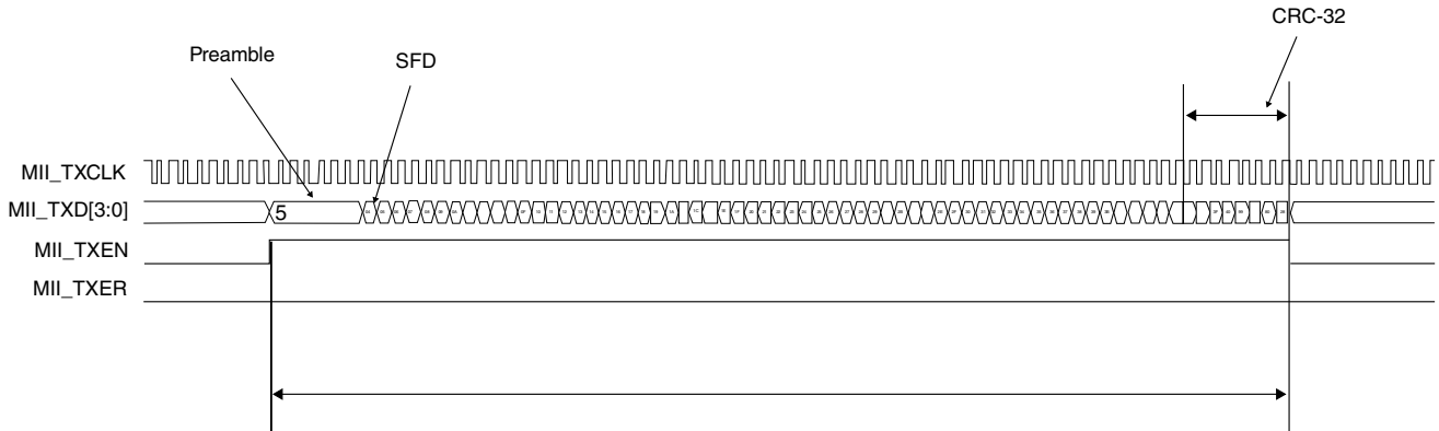
Figure 24-22. MII transmit operation
