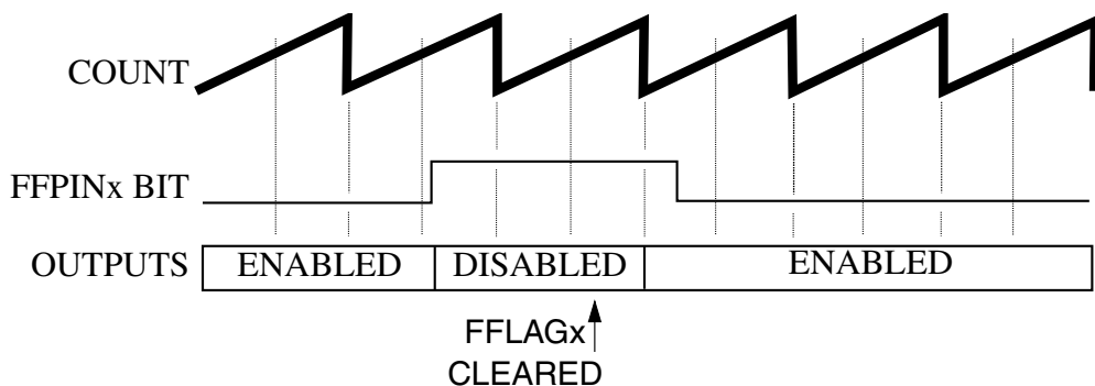
Figure 28-29. Manual Fault Clearing (FCTRL[FSAFE]=0)
