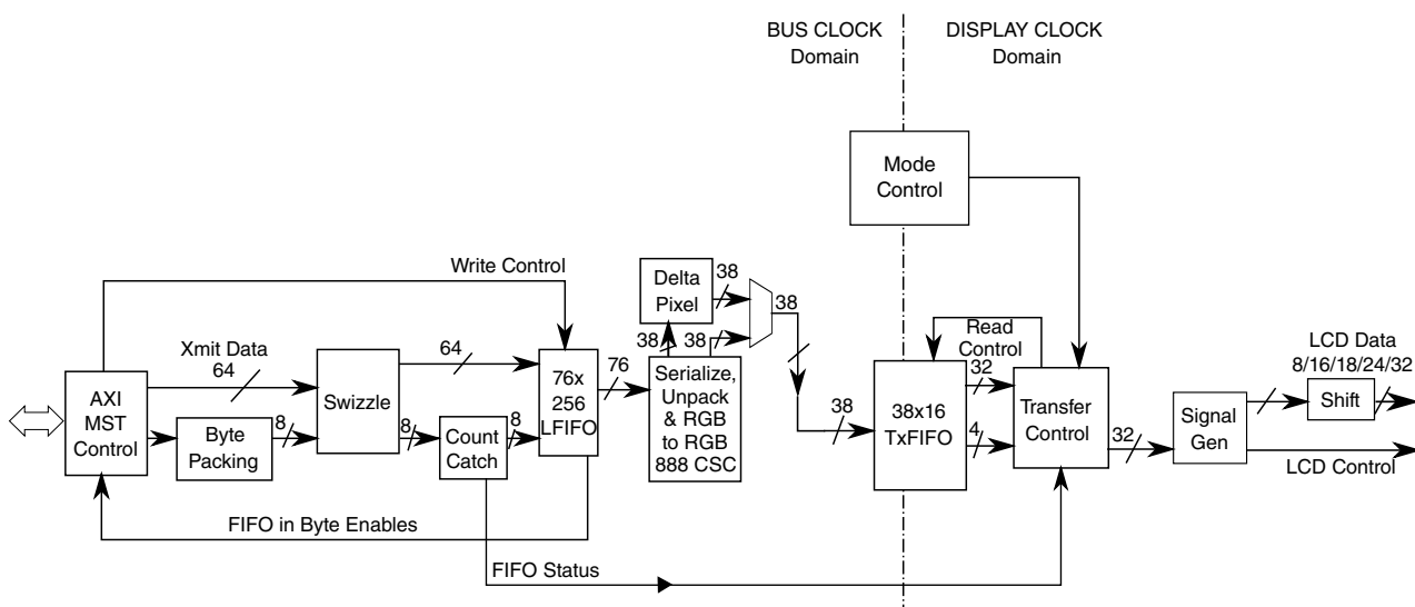
Figure 36-2. General Operations in Write Data Path
