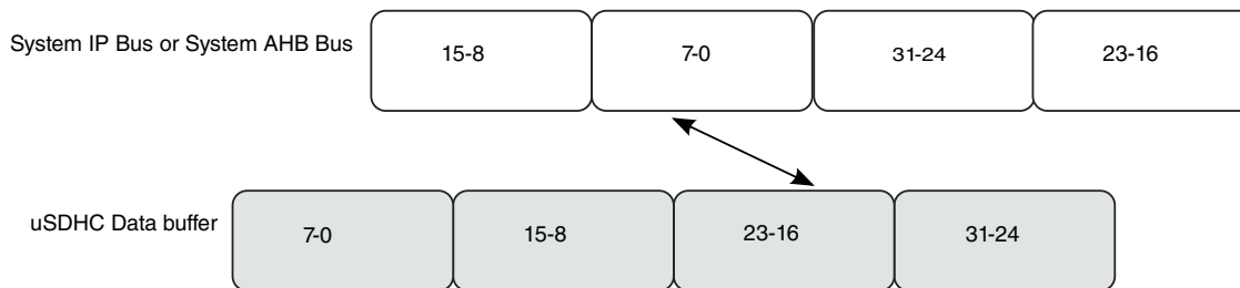
Figure 57-5. Data Swap between System Bus and uSDHC Data Buffer in Half Word Big Endian Mode
