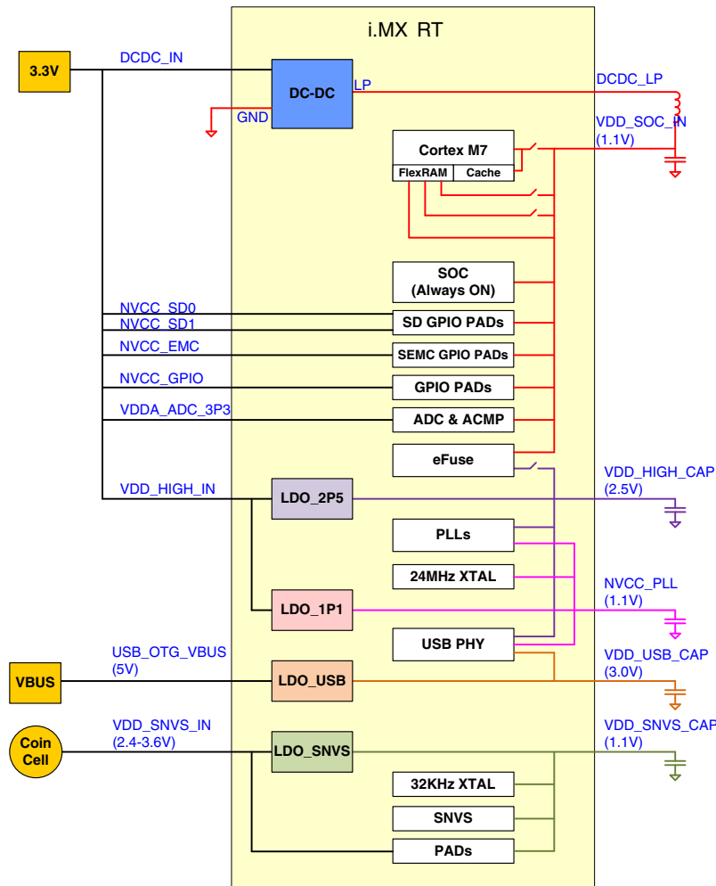
Figure 10-10. SOC Power Architecture
