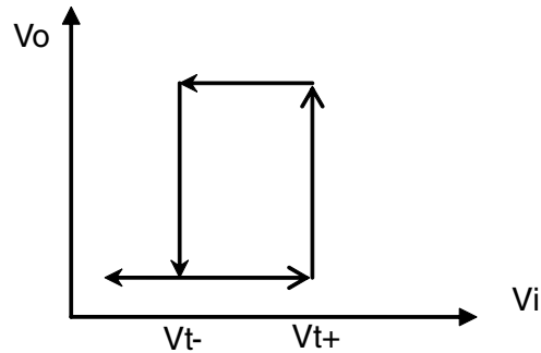
Figure 32-4. Schmitt trigger transfer characteristic
