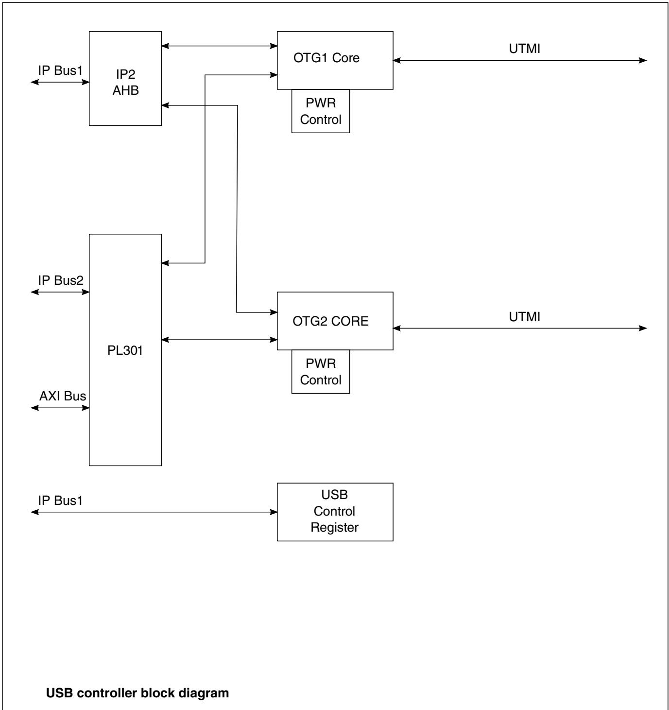
Figure 55-1. USB block diagram
