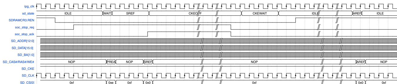
Figure 49-26. Stop mode Enter and Exit- SDRAM
