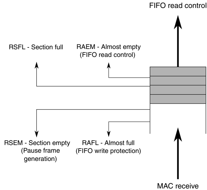
Figure 24-11. Receive FIFO overview
