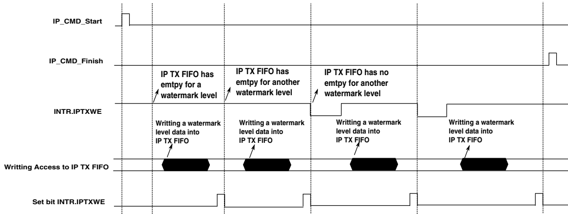
Figure 30-15. Filling IP TX FIFO by processor
