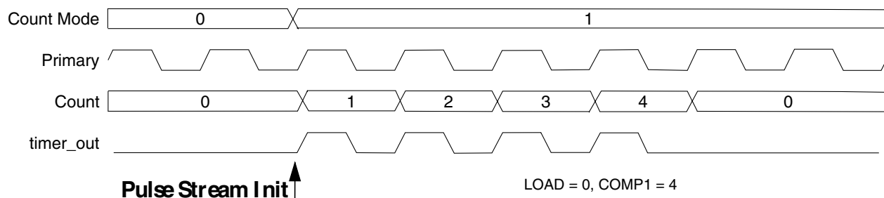
Figure 47-7. Pulse Output Mode
