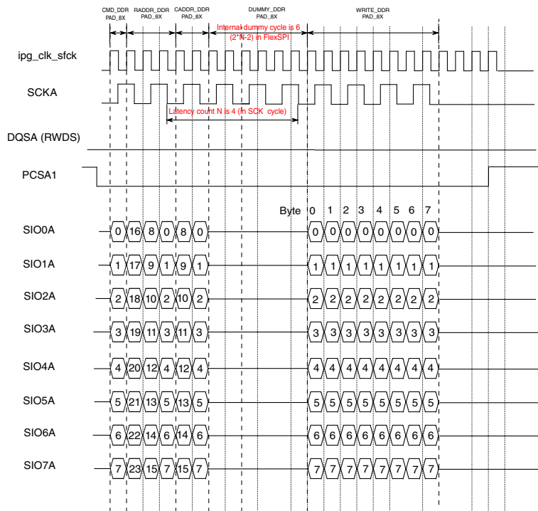
Figure 30-11. HyperBus device write transaction with single latency count
