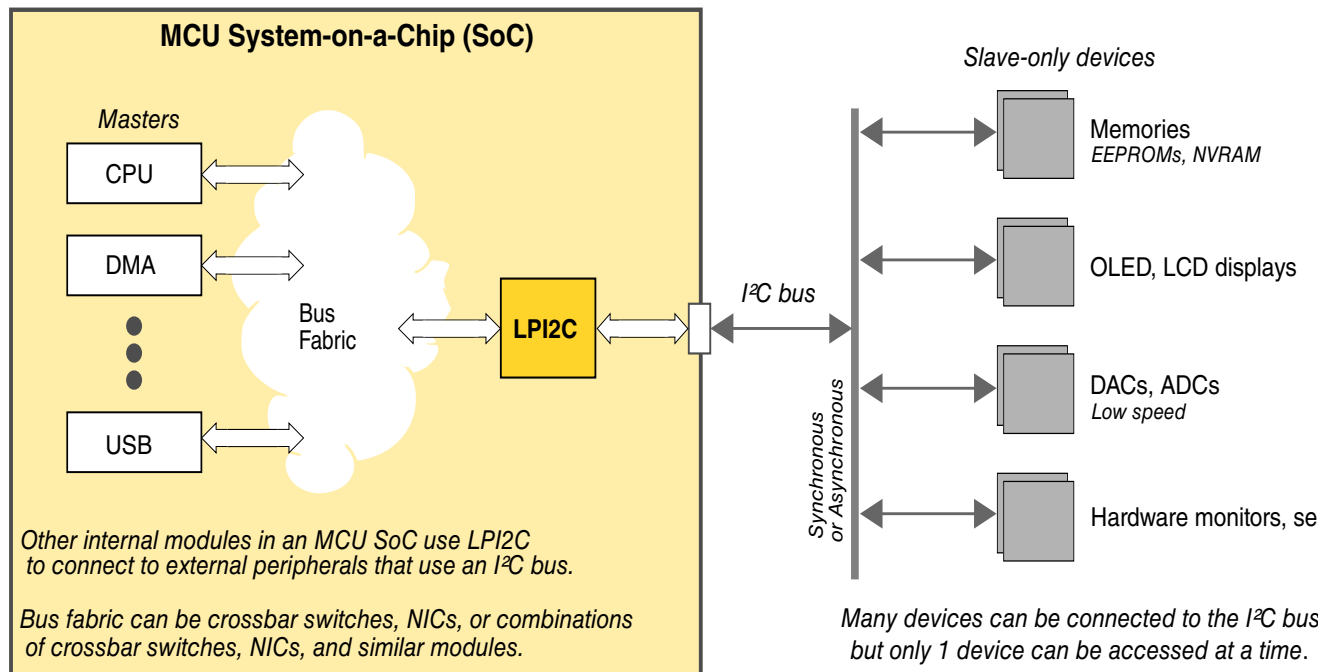
Figure 37-3. Typical LPI2C connection scheme
