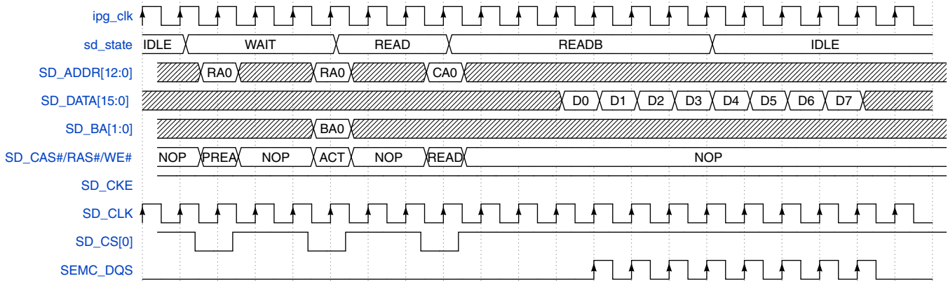
Figure 49-11. AXI command - SDRAM Read
