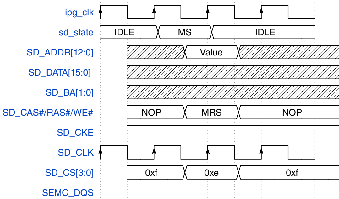
Figure 49-5. IP command - SDRAM MODE REGISTER SET
