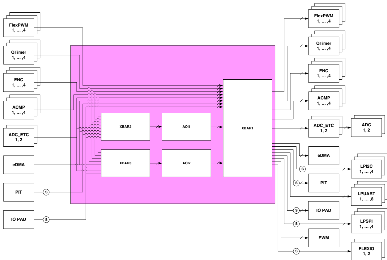
Figure 61-1. On-Chip Cross Trigger Network
