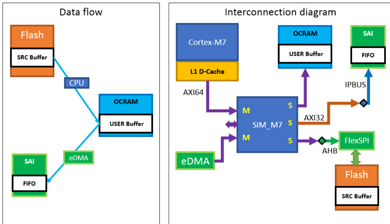
Figure 2. Data flow & Subsystem diagram
