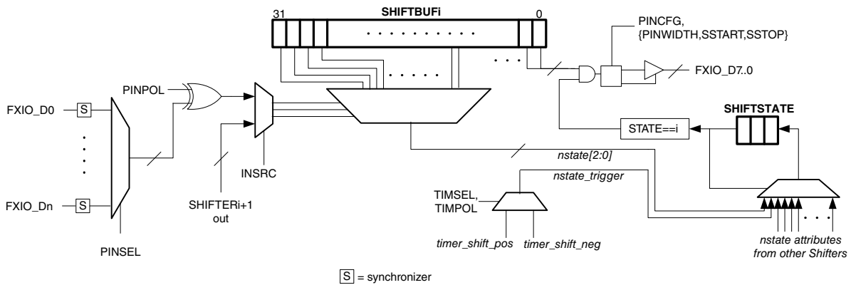
Figure 44-3. State Microarchitecture
