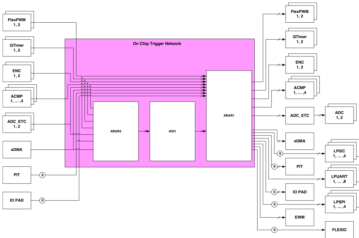
Figure 54-1. On-Chip Cross Trigger Network
