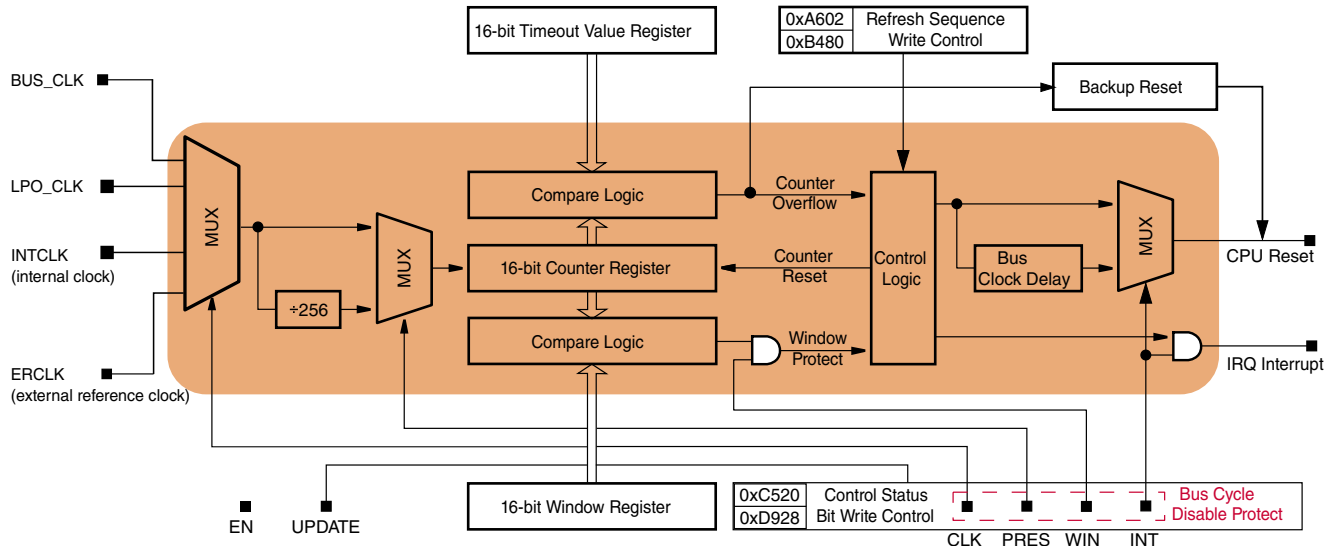
Figure 52-1. WDOG block diagram
