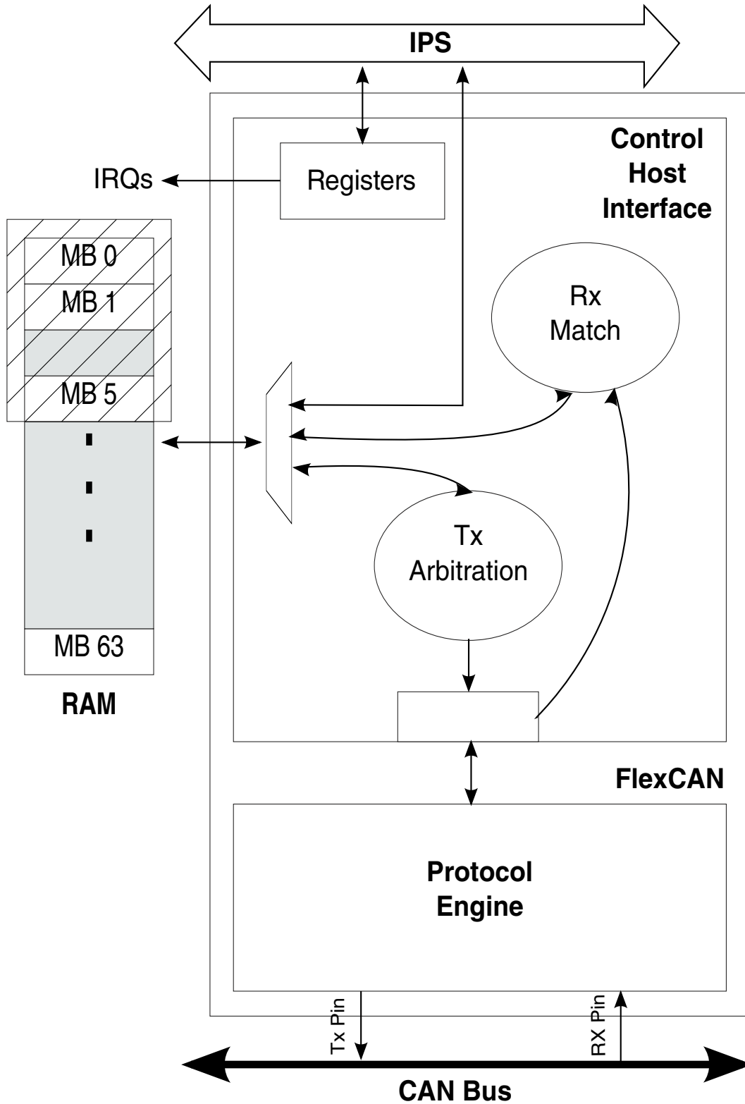
Figure 39-1. FLEXCAN Block Diagram
