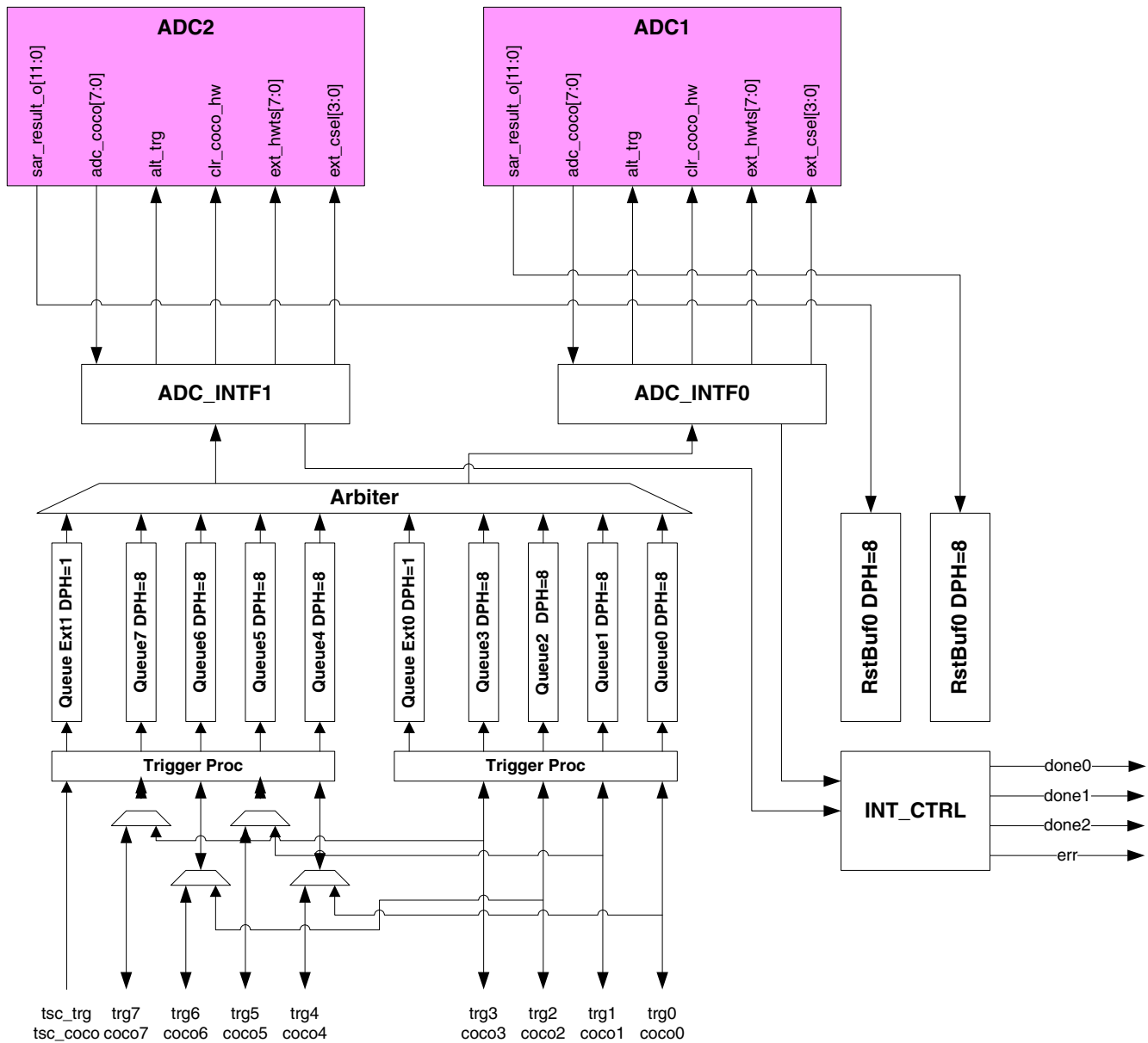
Figure 61-1. ADC_ETC block diagram
