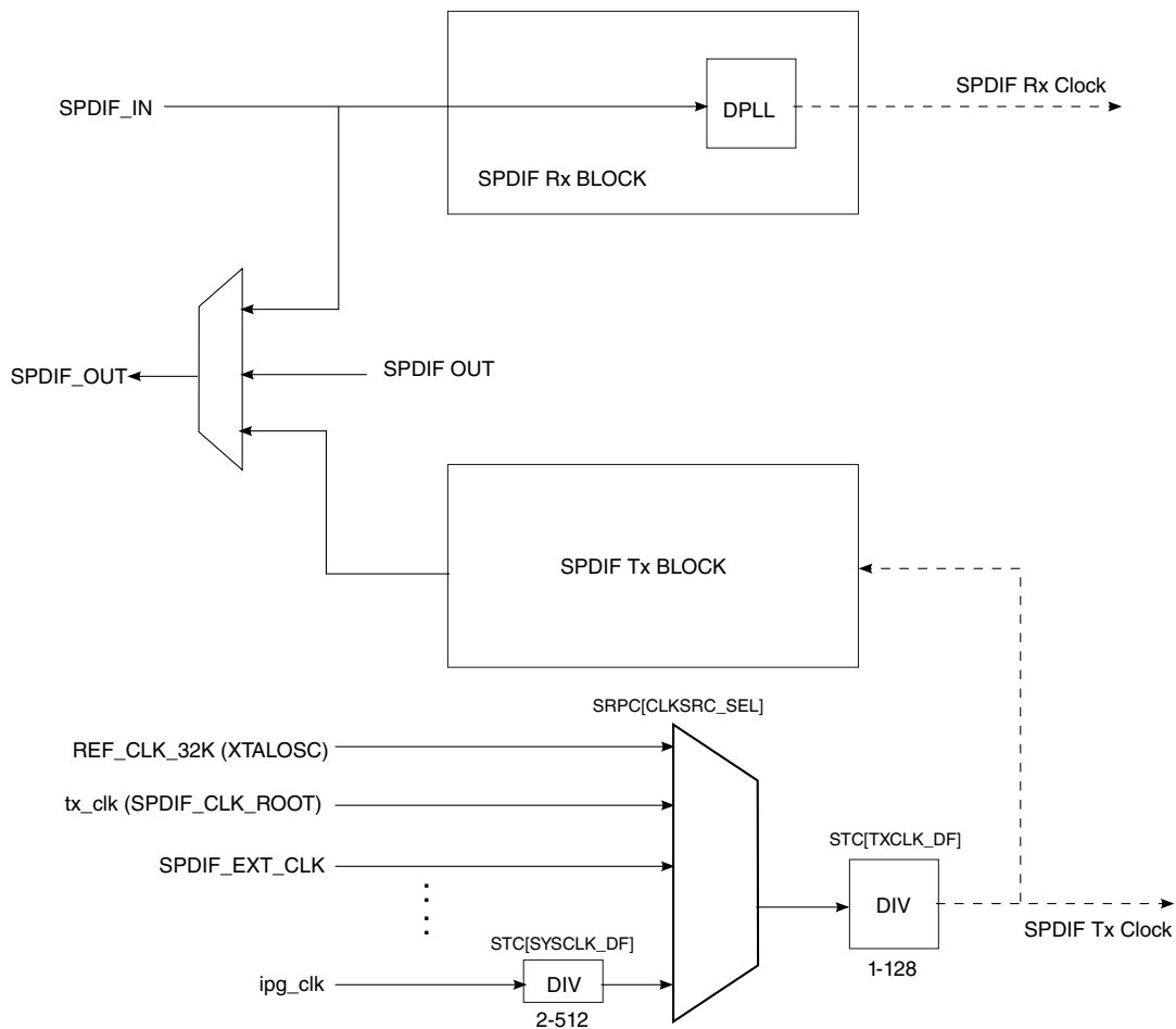
Figure 35-2. SPDIF Transceiver Clock Diagram
