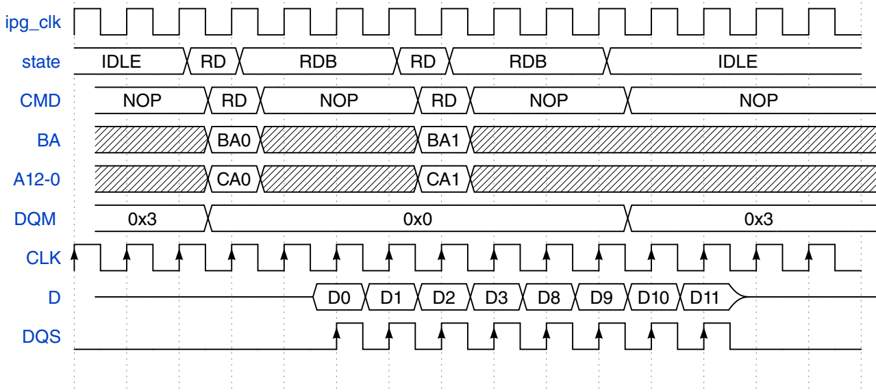
Figure 24-16. SDRAM Read-to-Read access (CL=2)
