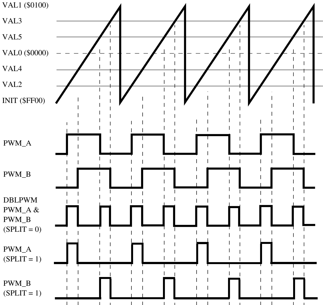
Figure 49-6. Double Switching Output Example
