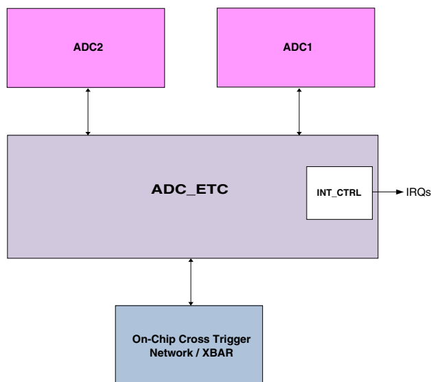
Figure 58-1. Block Diagram (Simplified)
