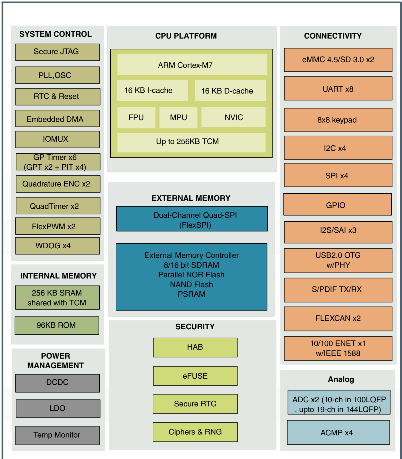
Figure 1-2. Simplified Block Diagram
