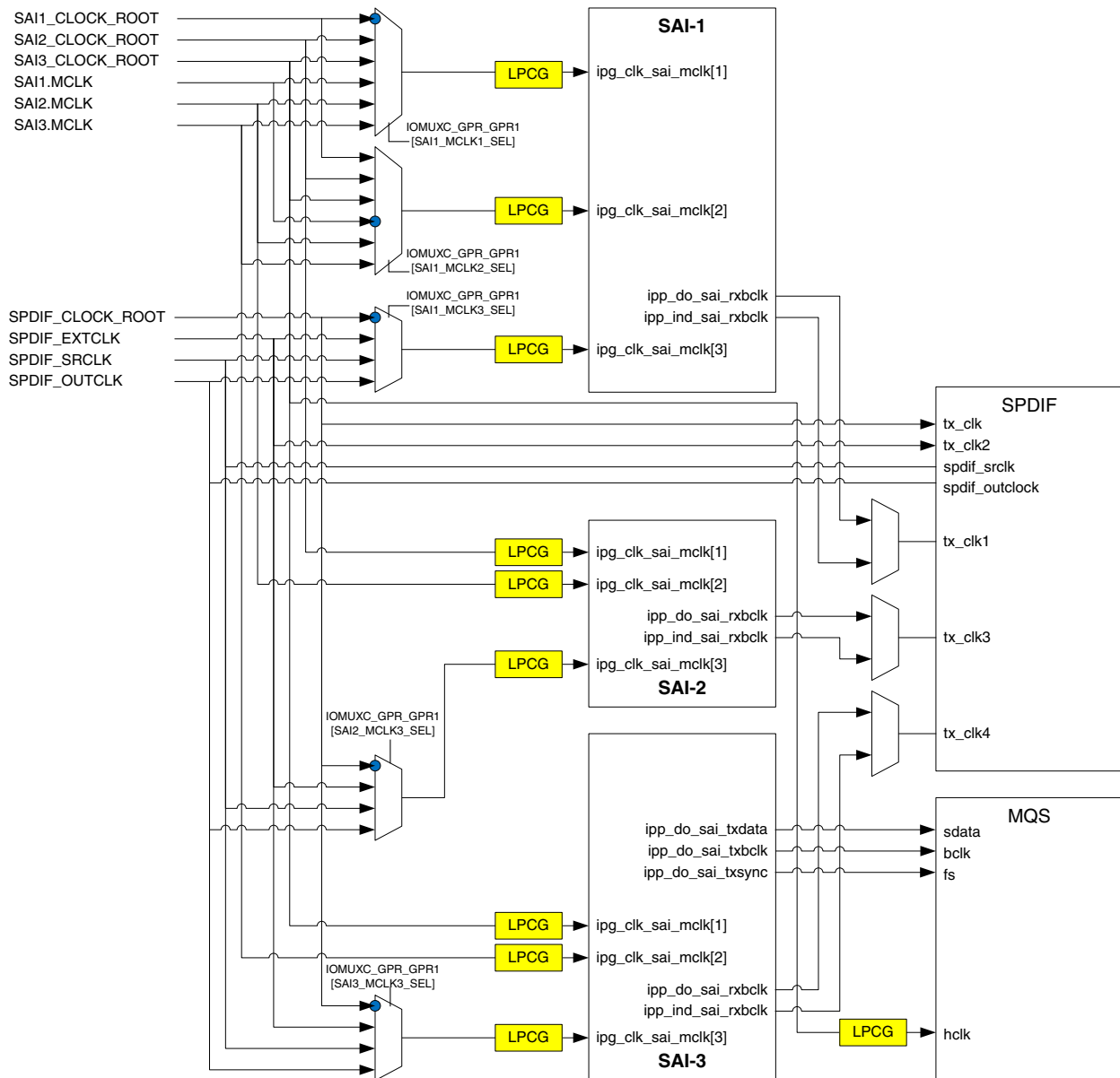
Figure 32-3. Audio subsystem clocking diagram
