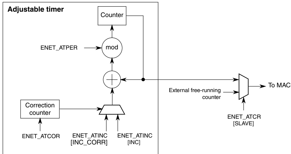
Figure 36-10. Adjustable timer implementation detail
