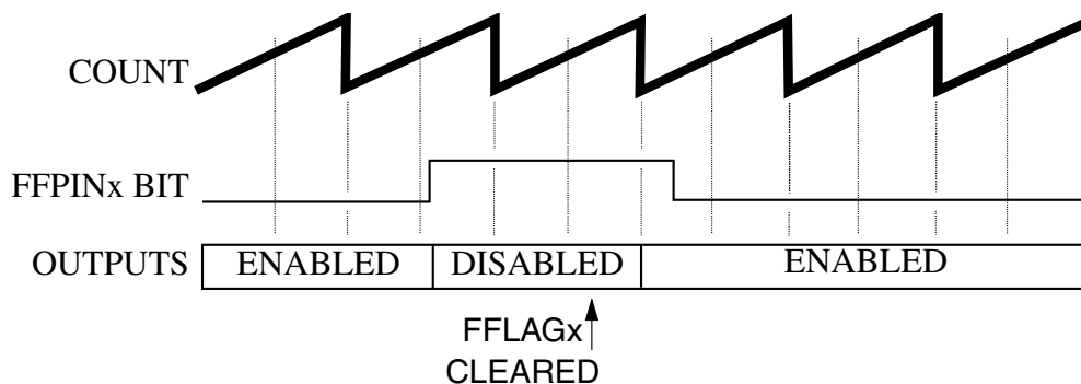
Figure 49-29. Manual Fault Clearing (FCTRL[FSAFE]=0)
