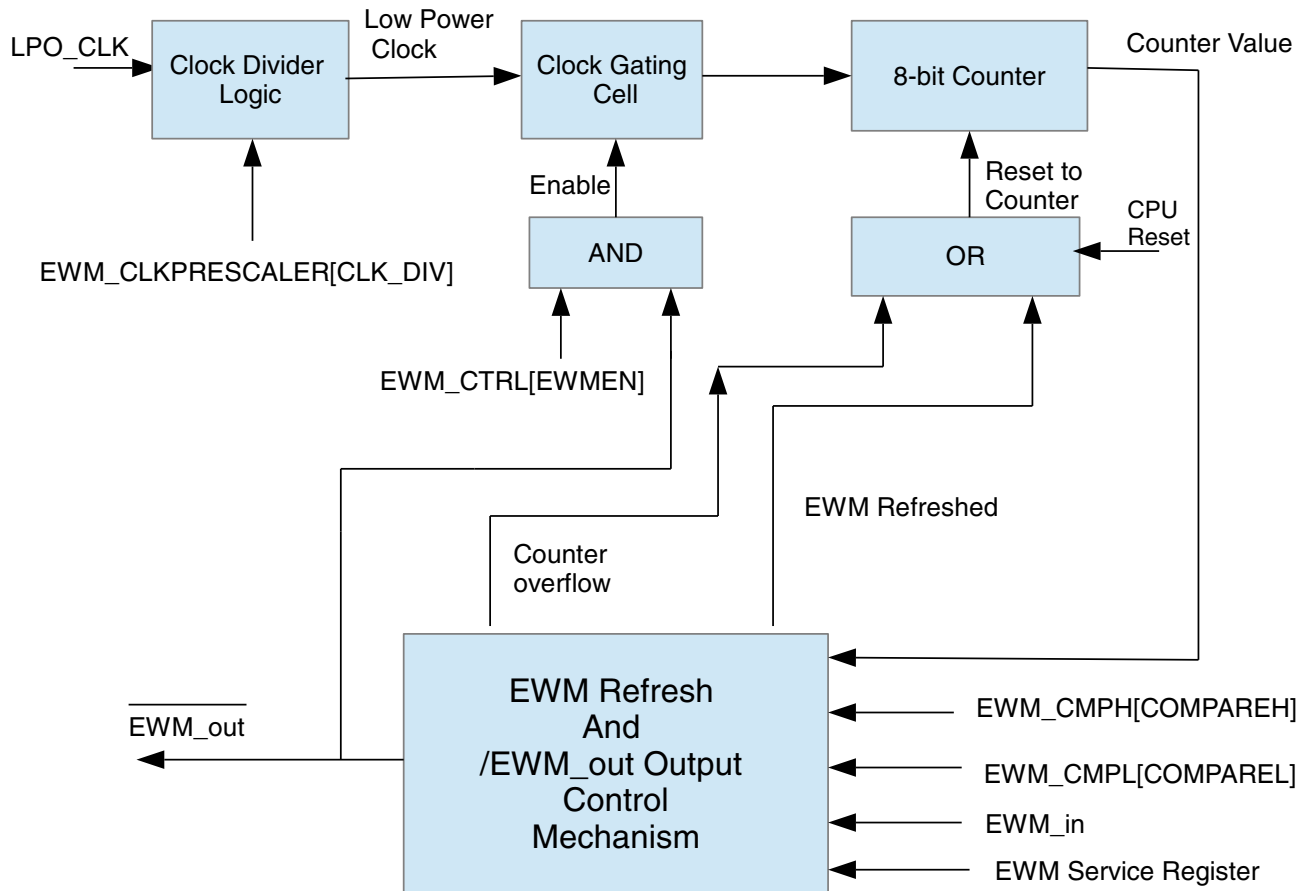
Figure 53-1. EWM Block Diagram
