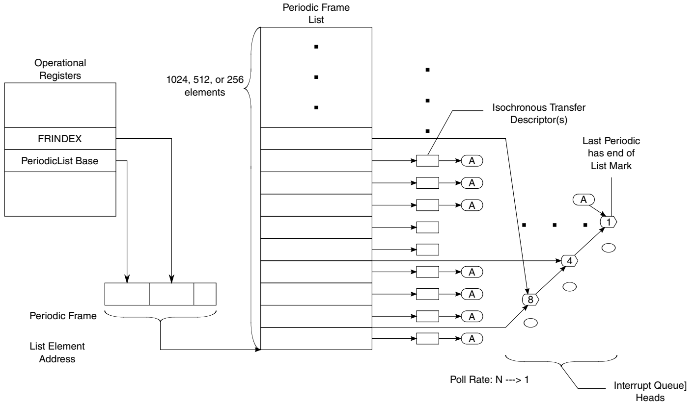
Figure 37-2. Periodic Schedule Organization
