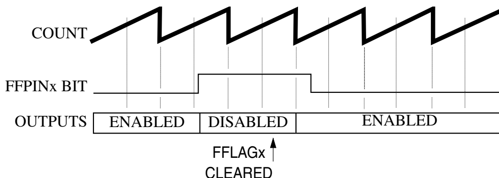
Figure 49-30. Manual Fault Clearing (FCTRL[FSAFE]=1)
