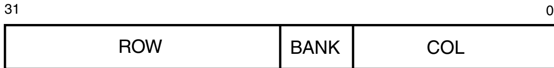
Figure 24-2. SDRAM device address map
