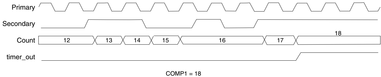
Figure 48-4. Triggered Count Mode 1 (CTRL[LENGTH]=0)
