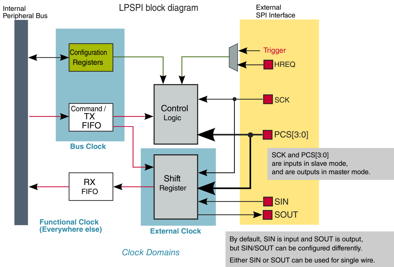
Figure 42-1. Block Diagram
