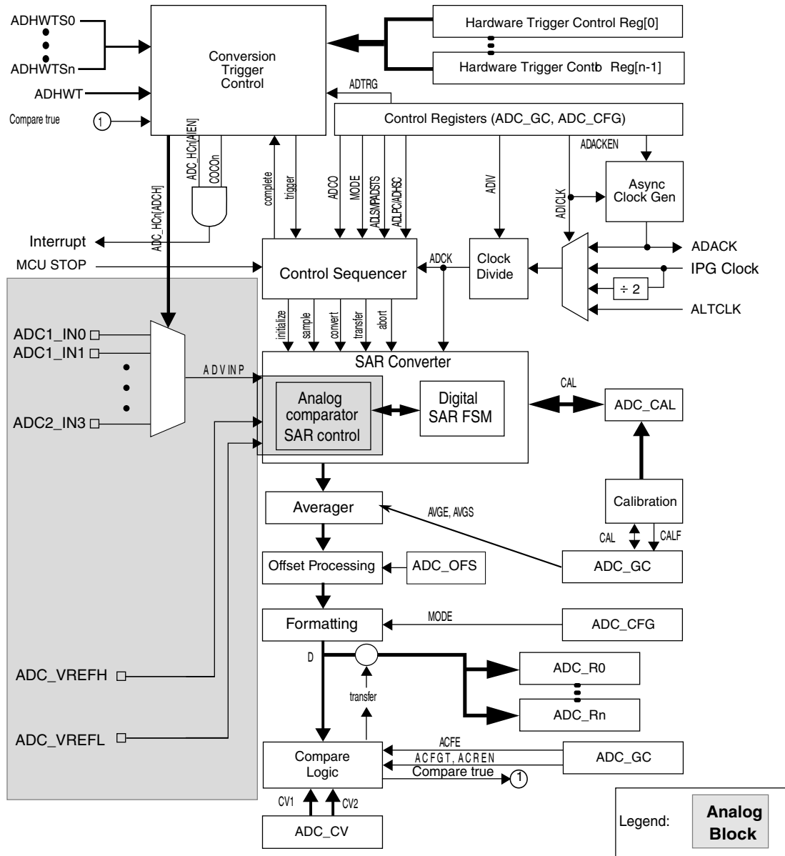
Figure 60-2. ADC block diagram
