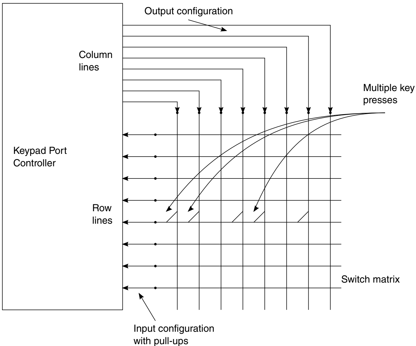
Figure 40-4. Multiple Key Presses on Same Row Line (Simplified View)
