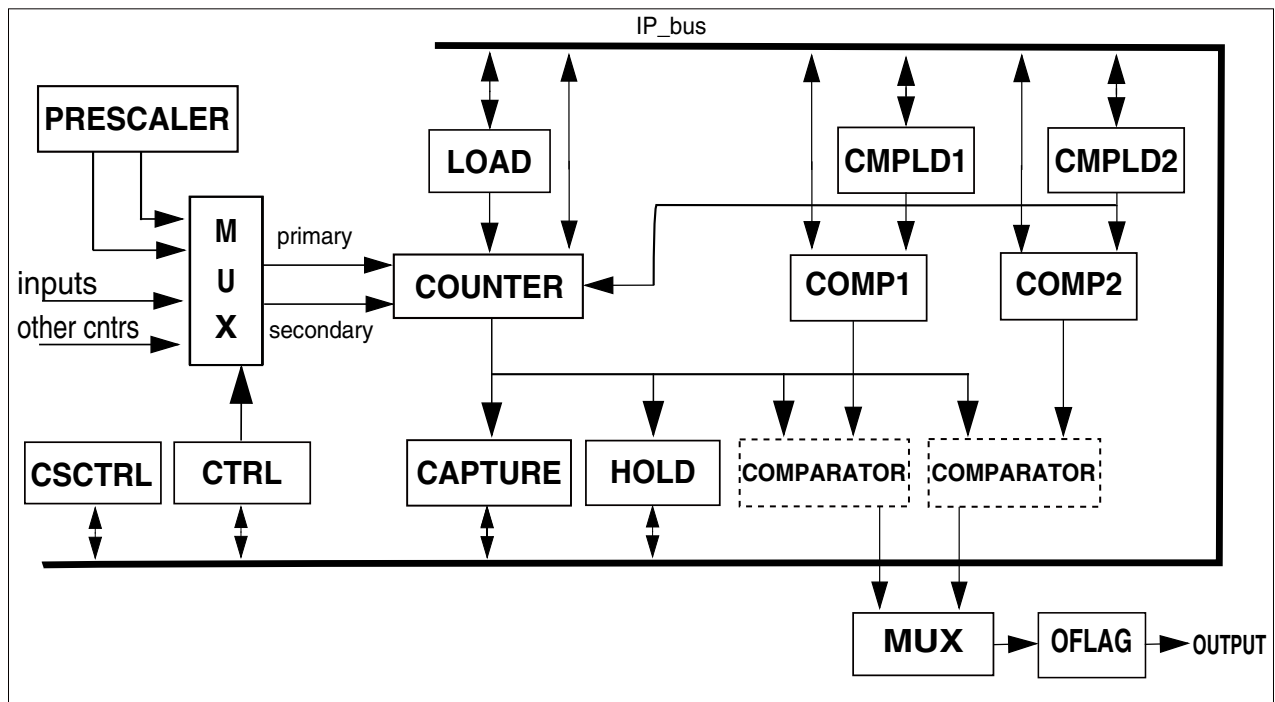
Figure 48-1. Quad Timer Block Diagram
