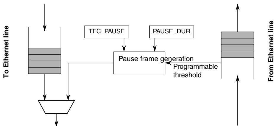
Figure 36-8. Pause frame generation overview
