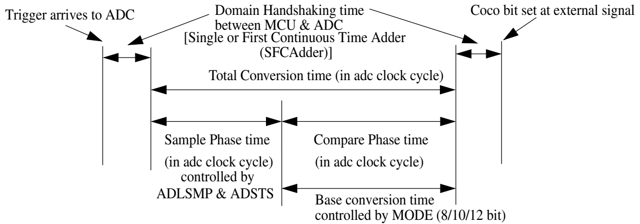
Figure 60-4. ADC conversion time details
