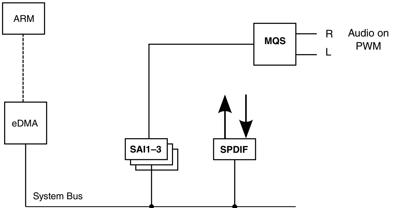
Figure 32-1. Audio subsystem block diagram
