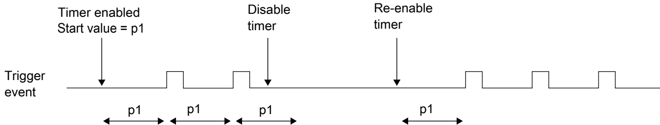
Figure 47-2. Stopping and starting a timer
