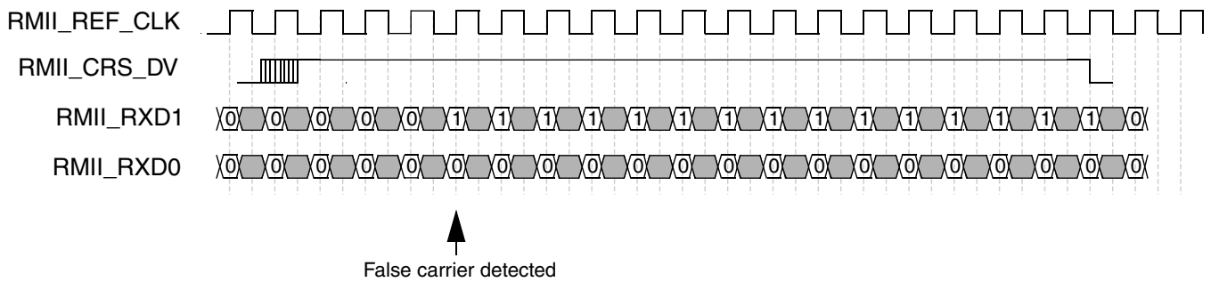
Figure 36-20. RMIi receive operation with false carrier
