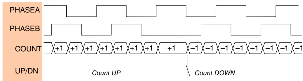
Figure 50-3. Quadrature Decoder Signals
