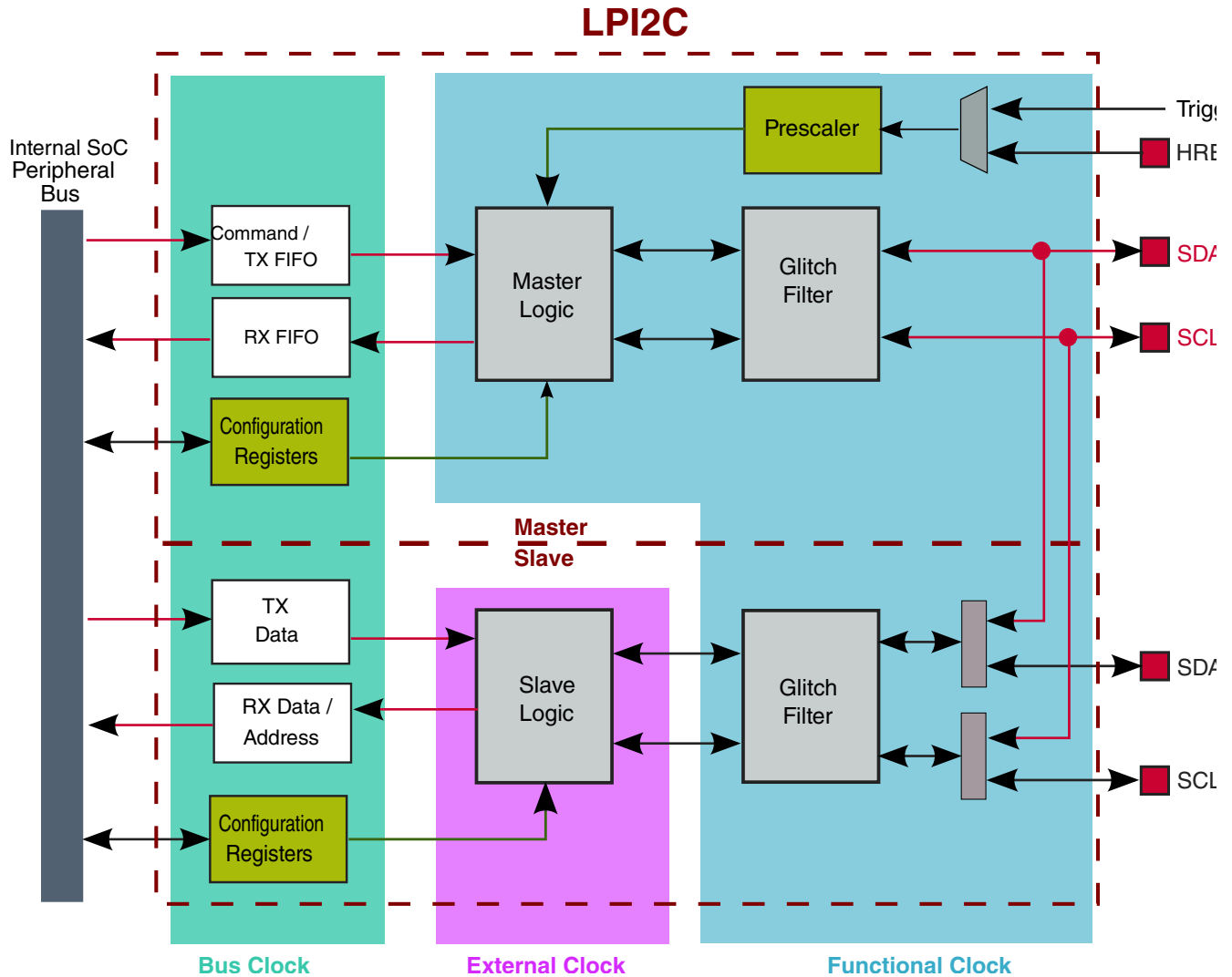
Figure 41-4. LPI2C block diagram
