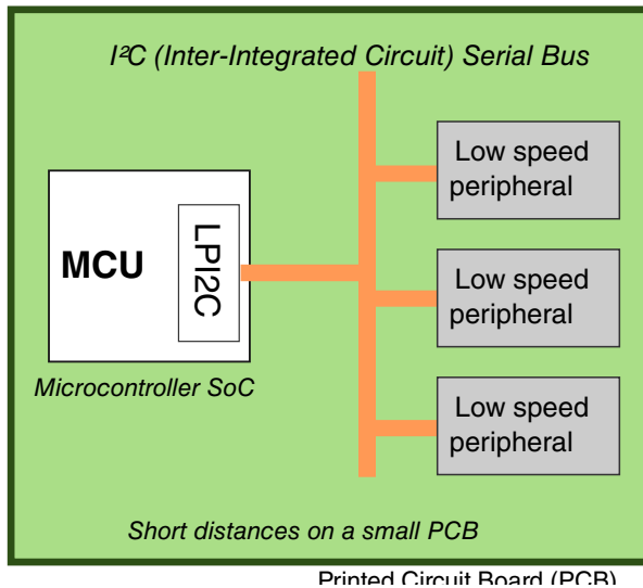
Figure 41-1. I 2 C bus connects MCU to low speed peripherals on PCB
