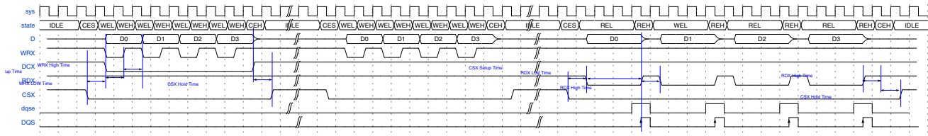
Figure 24-53. DBI Read/Write operation
