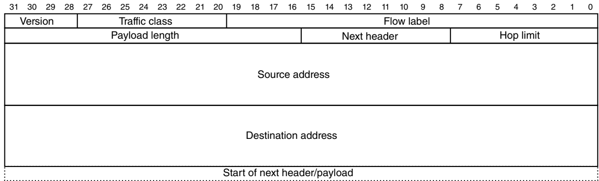
Figure 36-4. IPv6 header format
