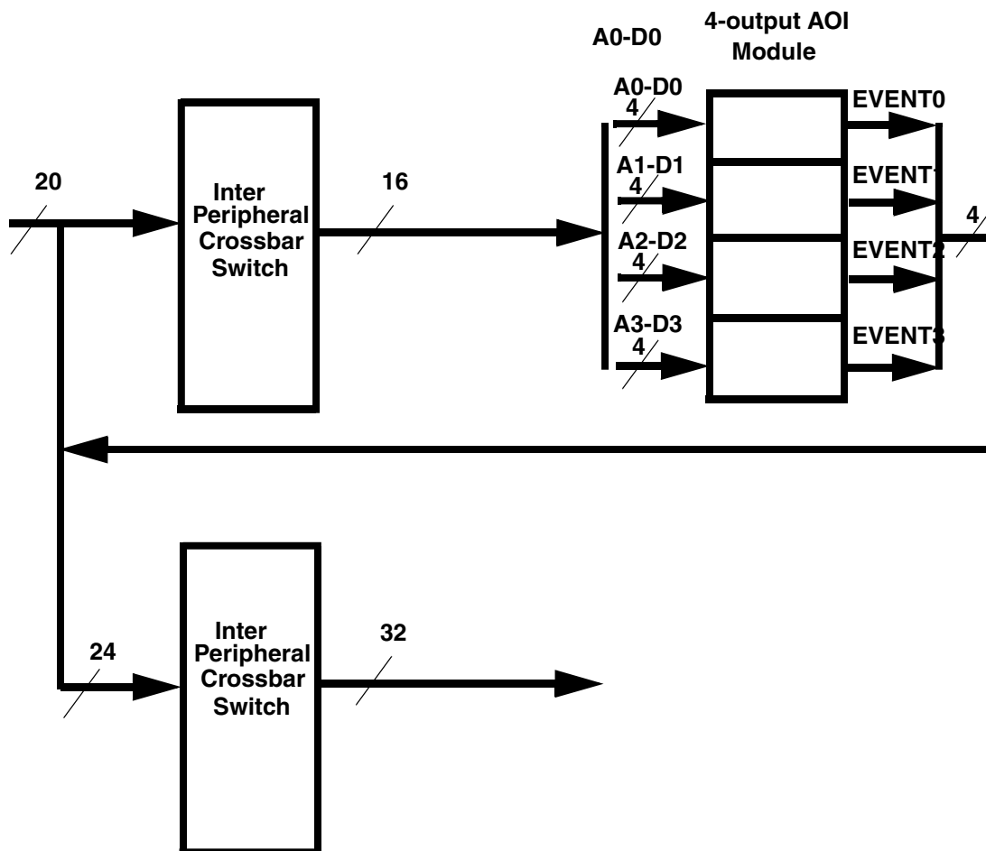
Figure 57-2. Integration Example of AOI with two Inter-Peripheral Crossbar Switches
