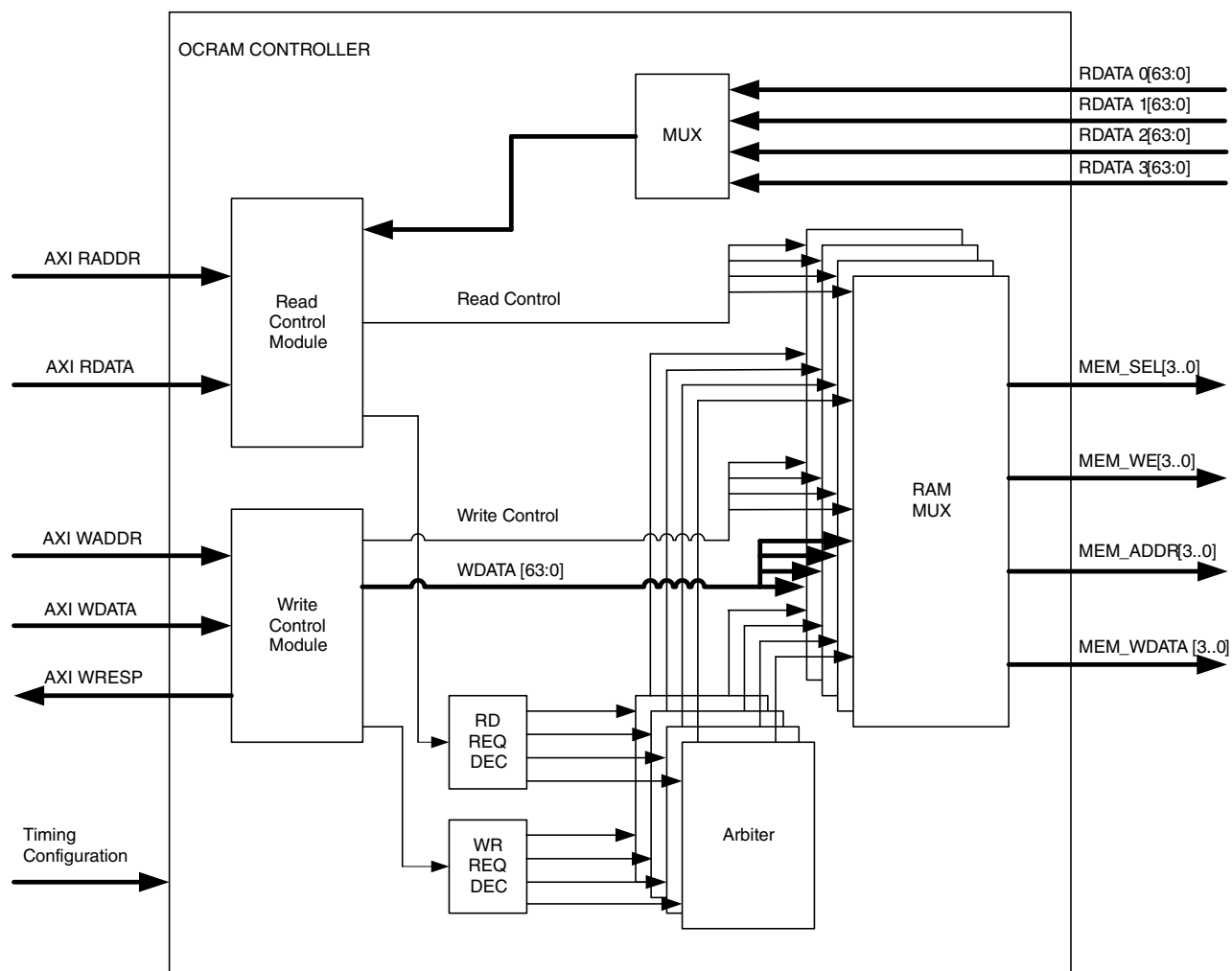
Figure 29-1. On-chip RAM Block Diagram
