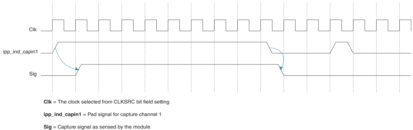
Figure 46-4. Input Capture Event Timing
