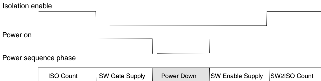
Figure 12-7. PDRAMx isolation and power on switch flow
