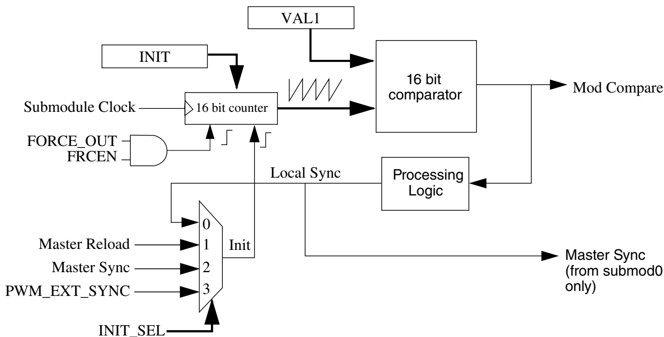
Figure 49-15. Submodule Timer Synchronization
