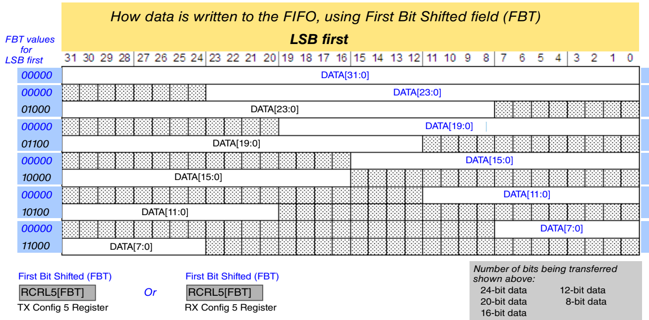
Figure 33-2. SAI first bit shifted, LSB first
