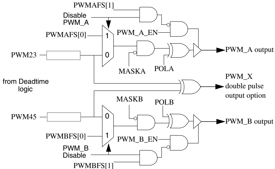
Figure 49-25. Output Logic
