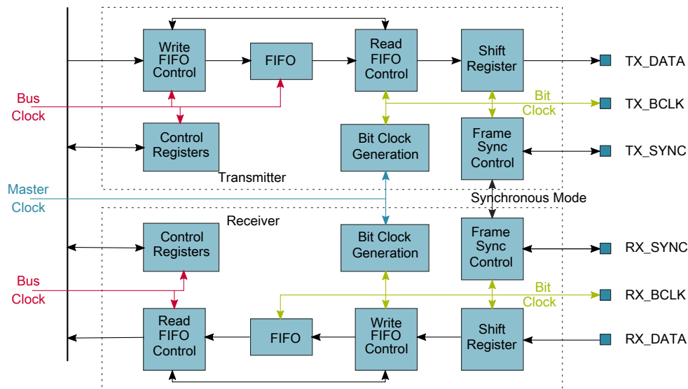
Figure 33-1. I 2 S/SAI block diagram
