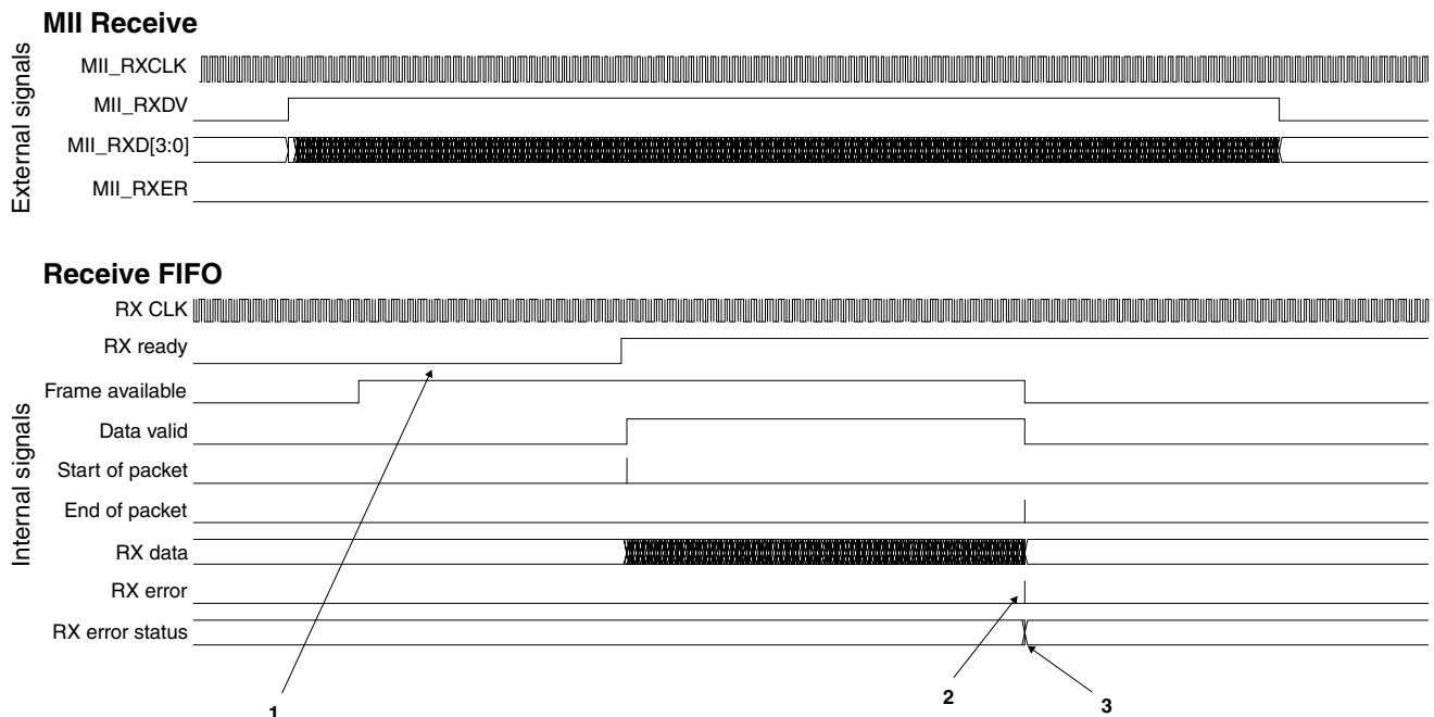
Figure 36-17. Receive FIFO overflow protection
