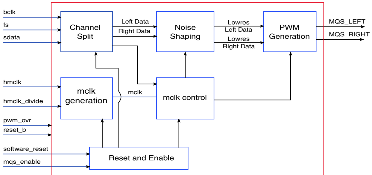
Figure 34-1. Block Diagram
