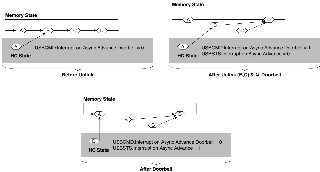
Figure 37-13. Generic Queue Head Unlink Scenario
