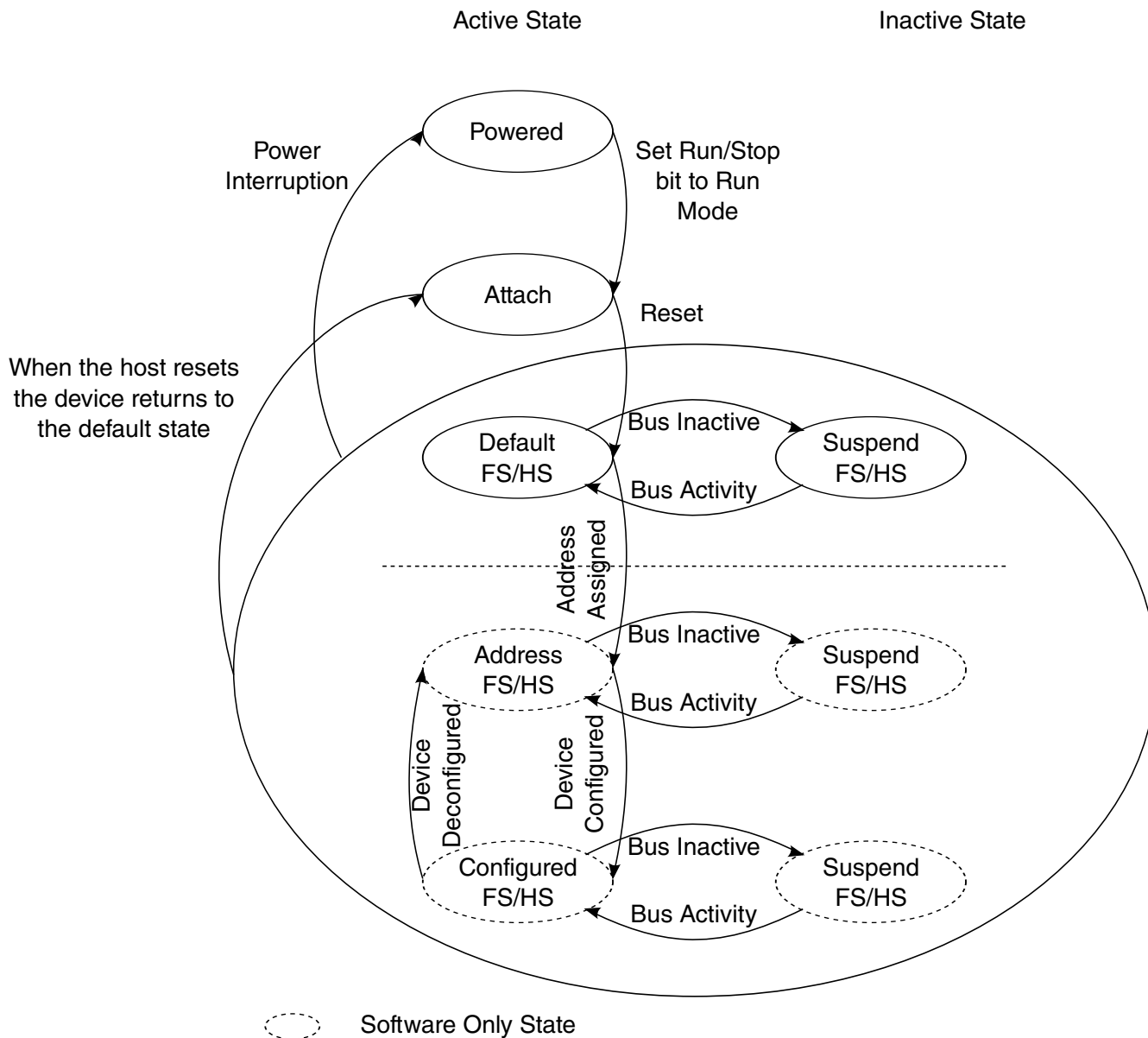
Figure 37-28. Device State Diagram
