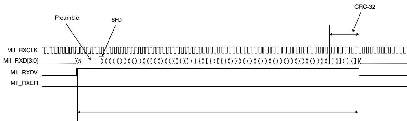
Figure 36-25. MII receive operation
