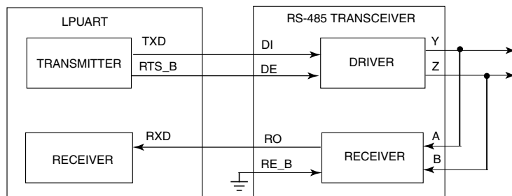
Figure 43-4. Transceiver driver enable using RTS_B
