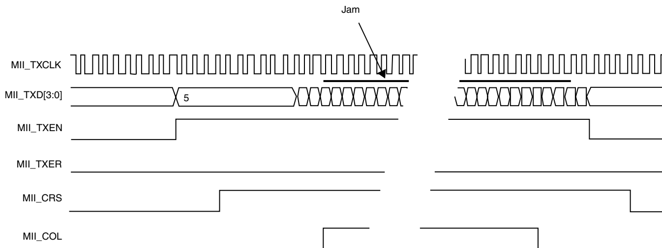
Figure 36-24. MII transmit operation — transmission with collision
