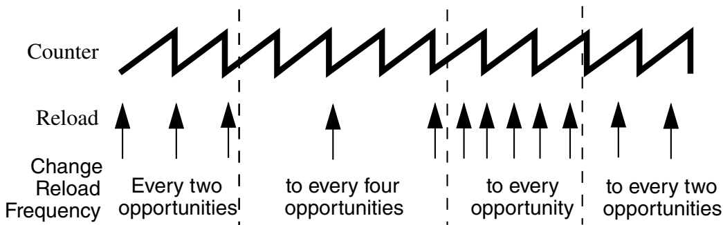
Figure 49-33. Full and Half Cycle Reload Frequency Change
