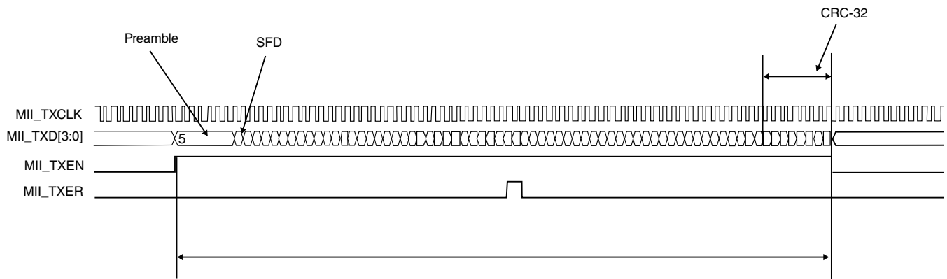
Figure 36-23. MII transmit operation — errored frame
