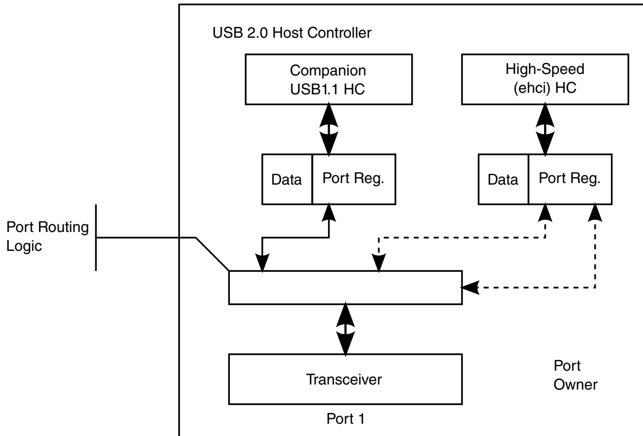
Figure 37-4. Example USB 2.0 Host Controller Port Routing Block Diagram
