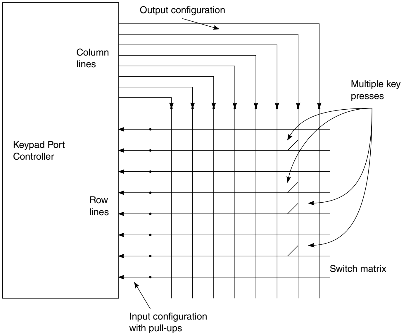
Figure 40-3. Multiple Key Presses on Same Column Line (Simplified View)
