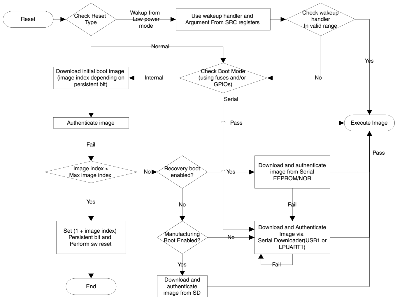
Figure 8-1. Boot flow
