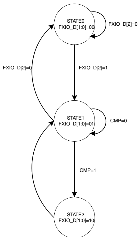
Figure 44-5. State Diagram
