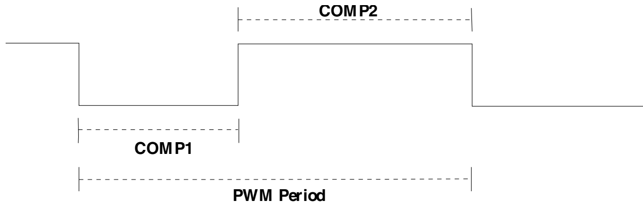
Figure 48-2. Variable PWM Waveform
