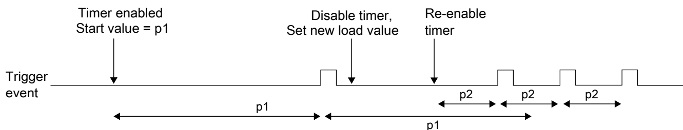
Figure 47-3. Modifying running timer period
