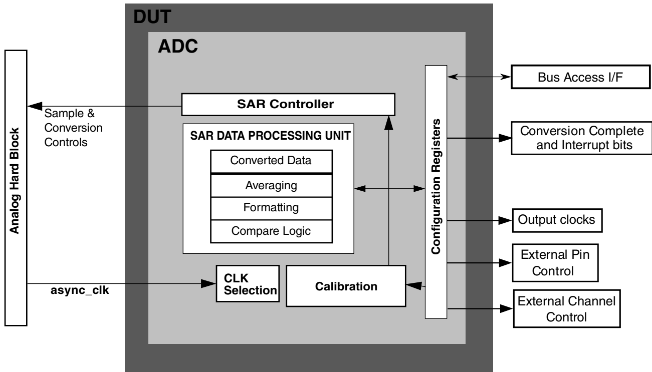
Figure 60-1. ADC I/F block diagram
