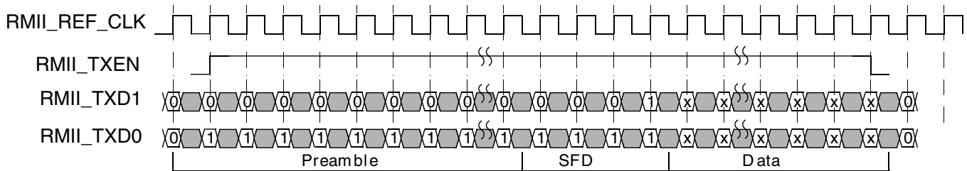
Figure 36-21. RMIi transmit operation
