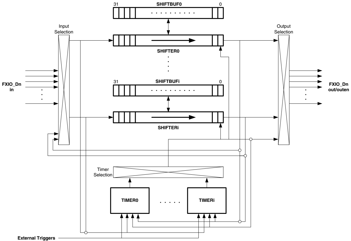
Figure 44-1. FlexIO block diagram
