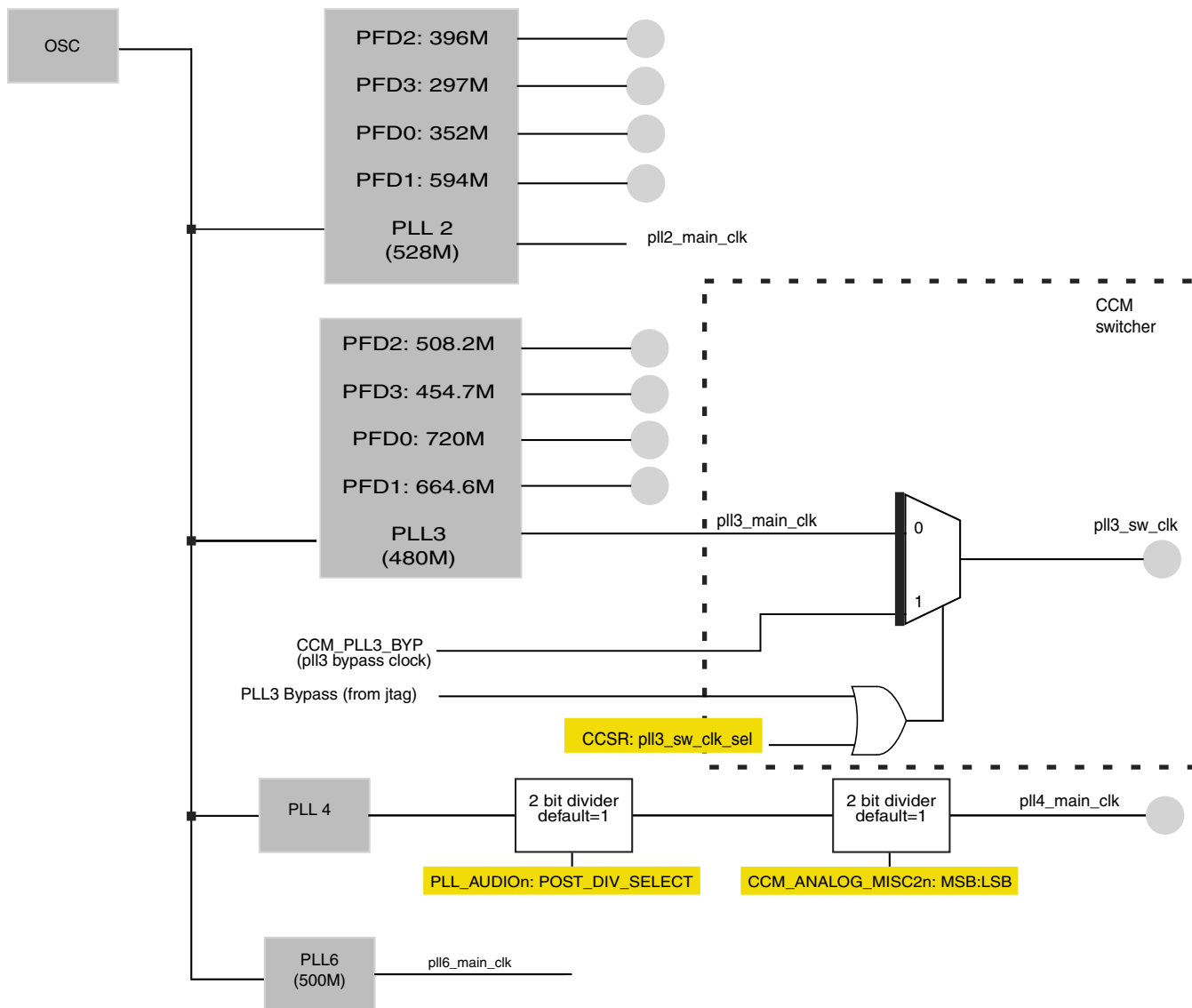
Figure 13-4. Switcher clock generation
