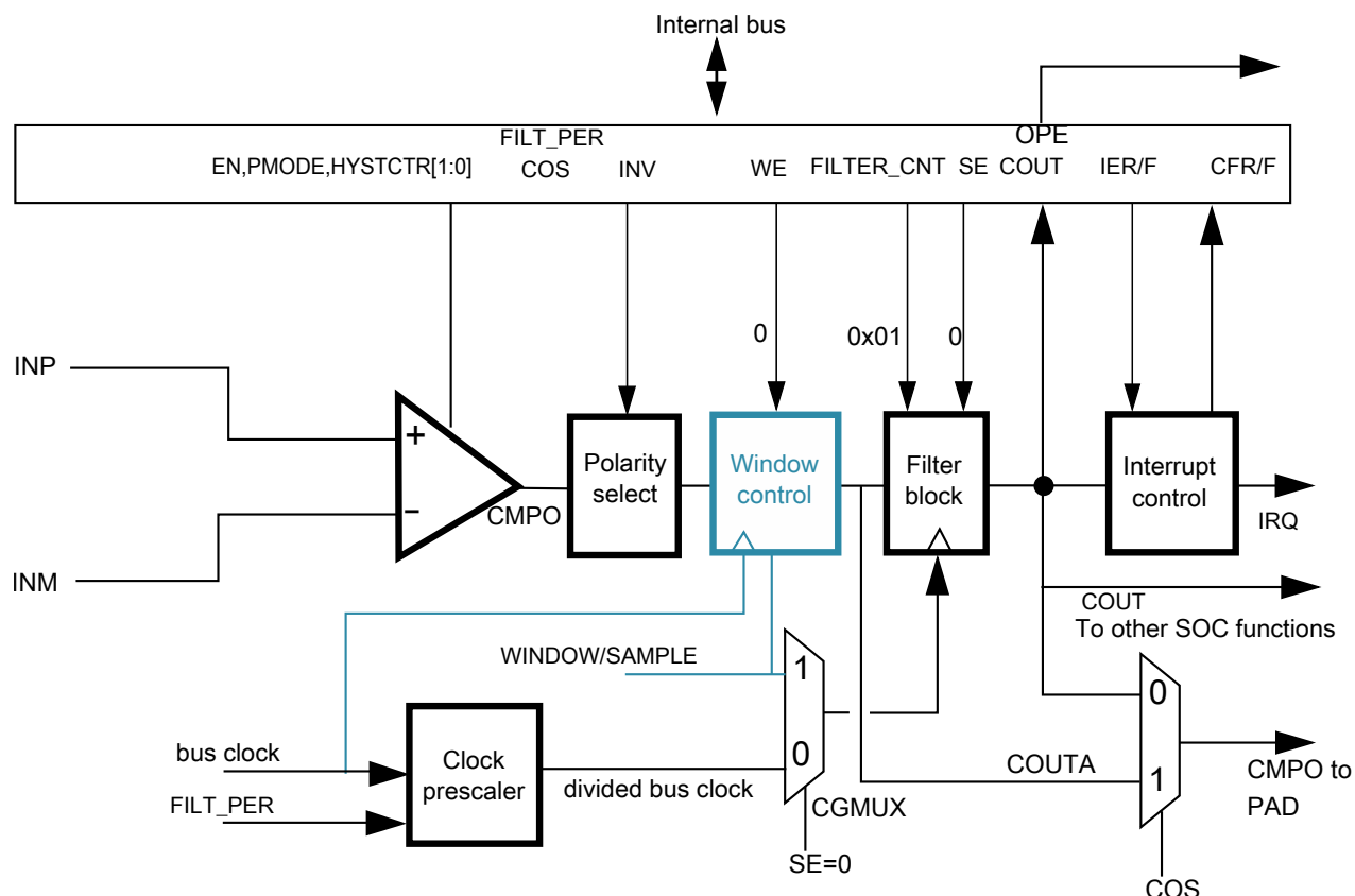
Figure 59-5. Sampled, Non-Filtered (# 3B): sampling interval internally derived
