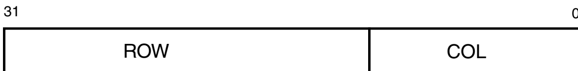
Figure 24-27. NAND Flash Address Map
