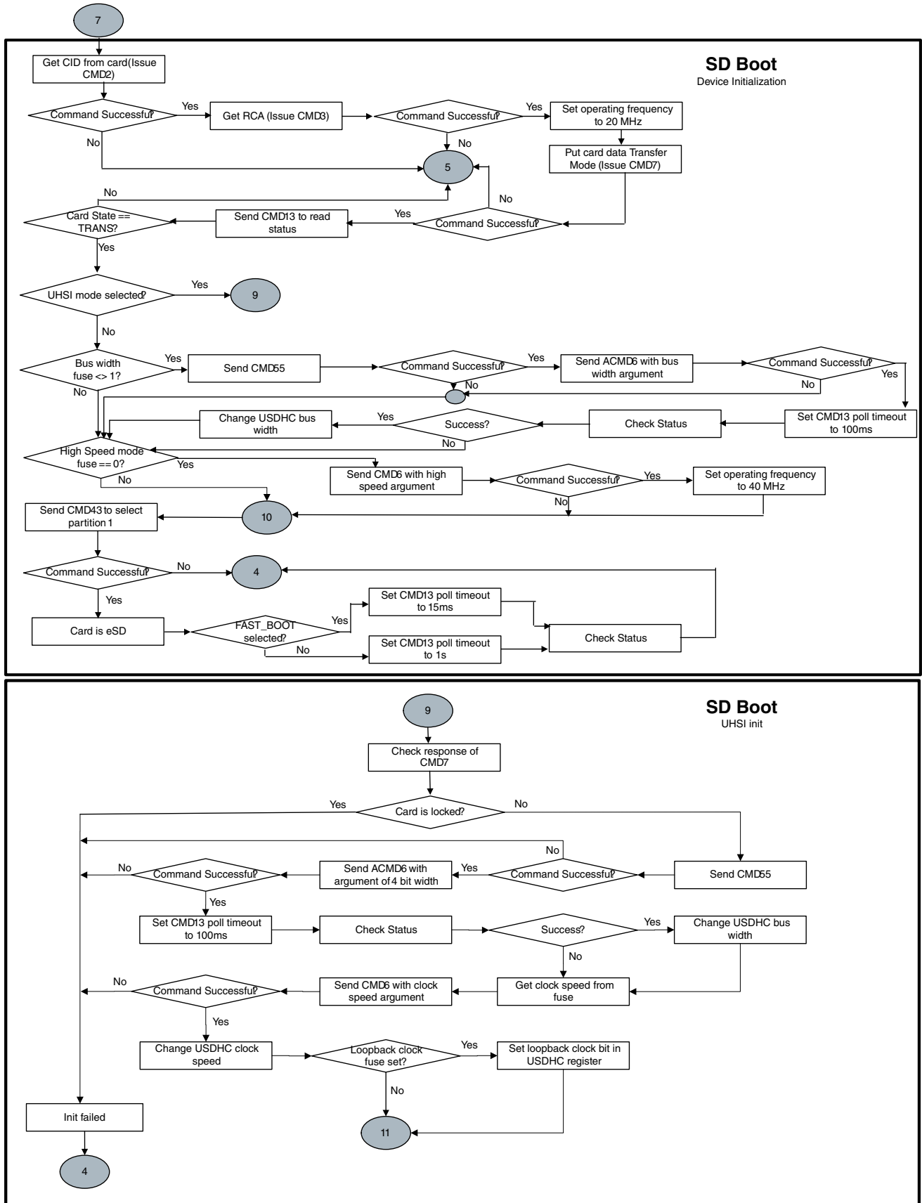
Figure 8-10. Expansion device (MMCSD/eSD/SDXC) boot flow (4 of 6) i.MX RT1020 Processor Reference Manual, Rev. 1, 12/2018
