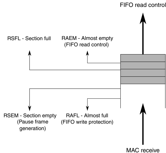
Figure 36-11. Receive FIFO overview
