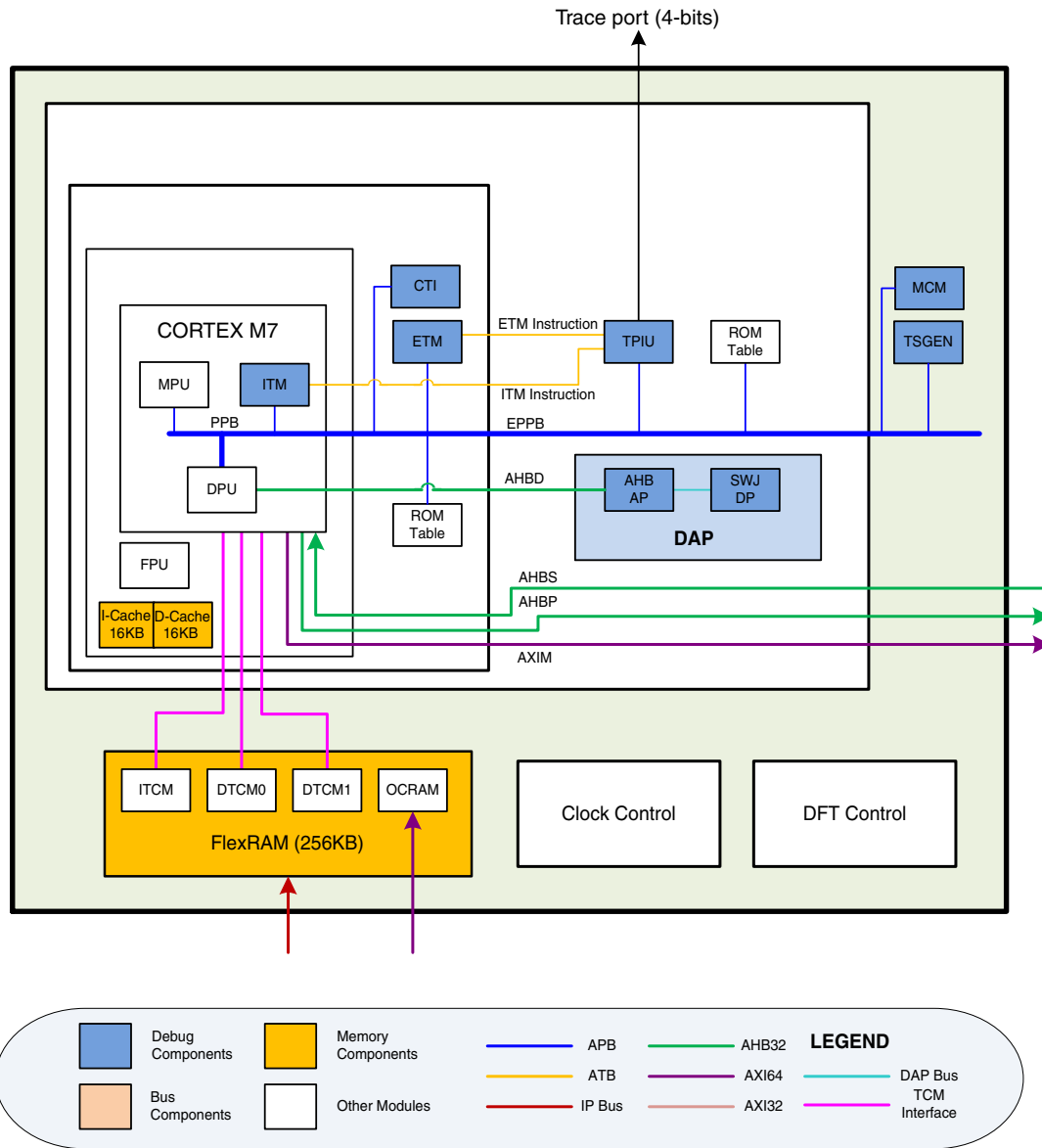
Figure 27-1. Cortex-M7 Platform Block Diagram
