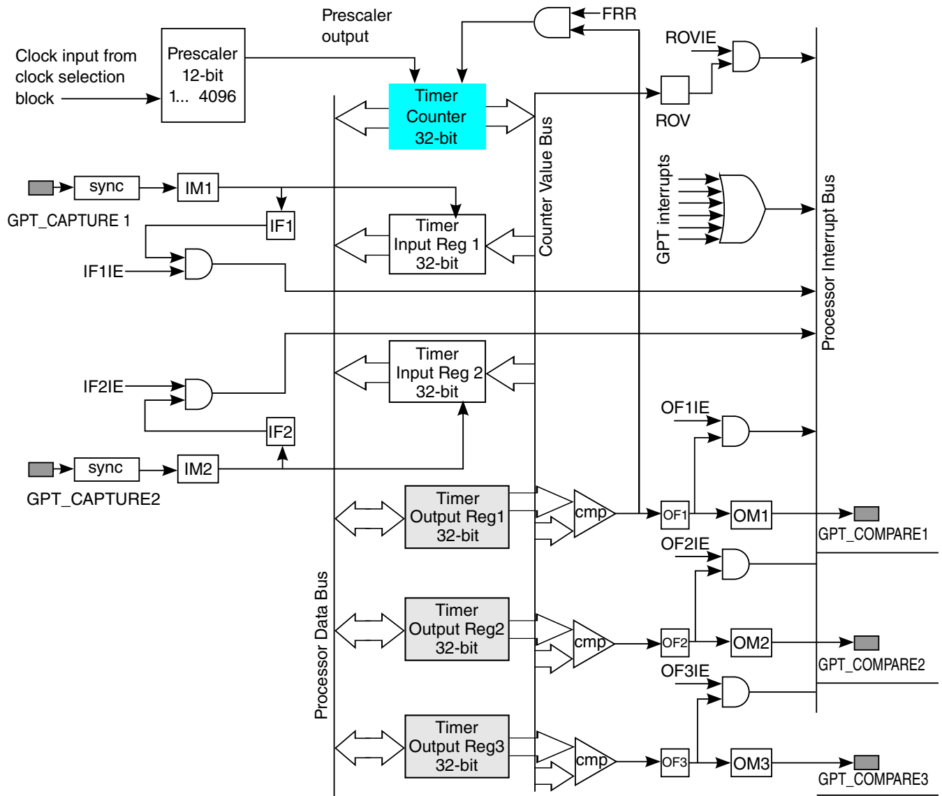
Figure 46-1. GPT Block Diagram
