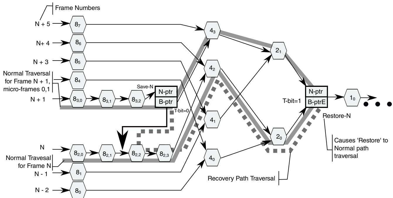
Figure 37-22. Example Host Controller Traversal of Recovery Path via FSTNs
