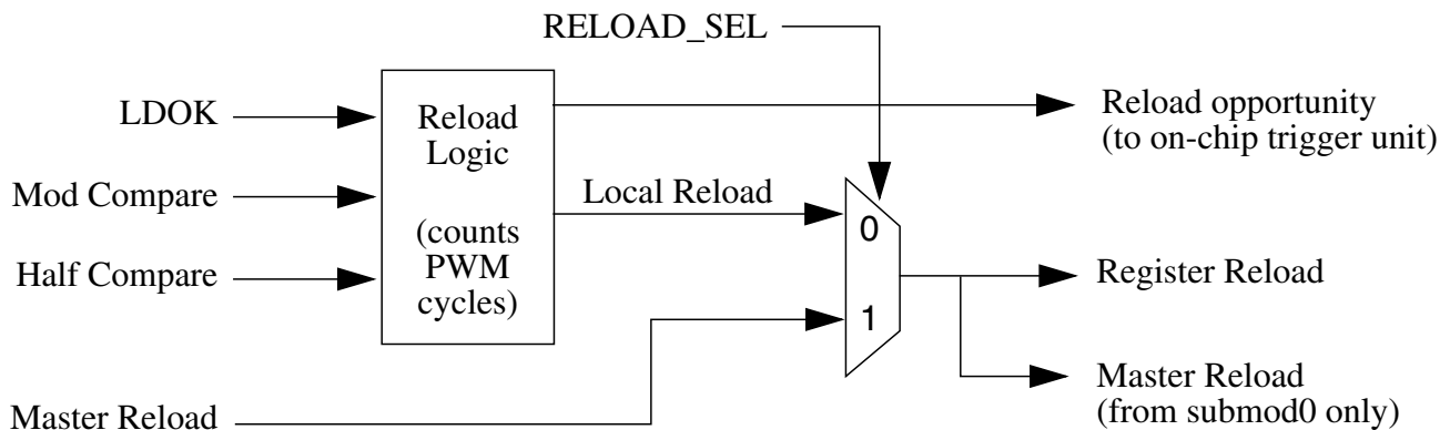
Figure 49-14. Register Reload Logic
