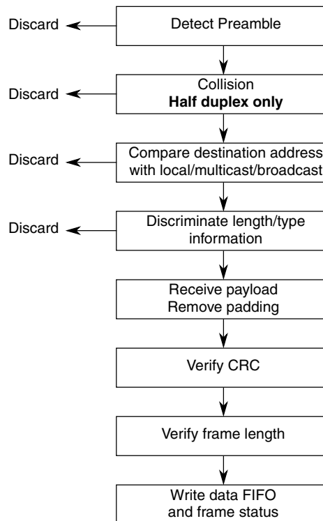
Figure 36-5. MAC receive flow
