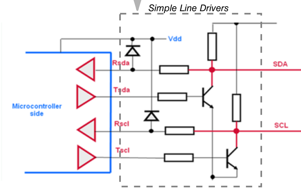
Figure 41-6. 4-Wire scheme
