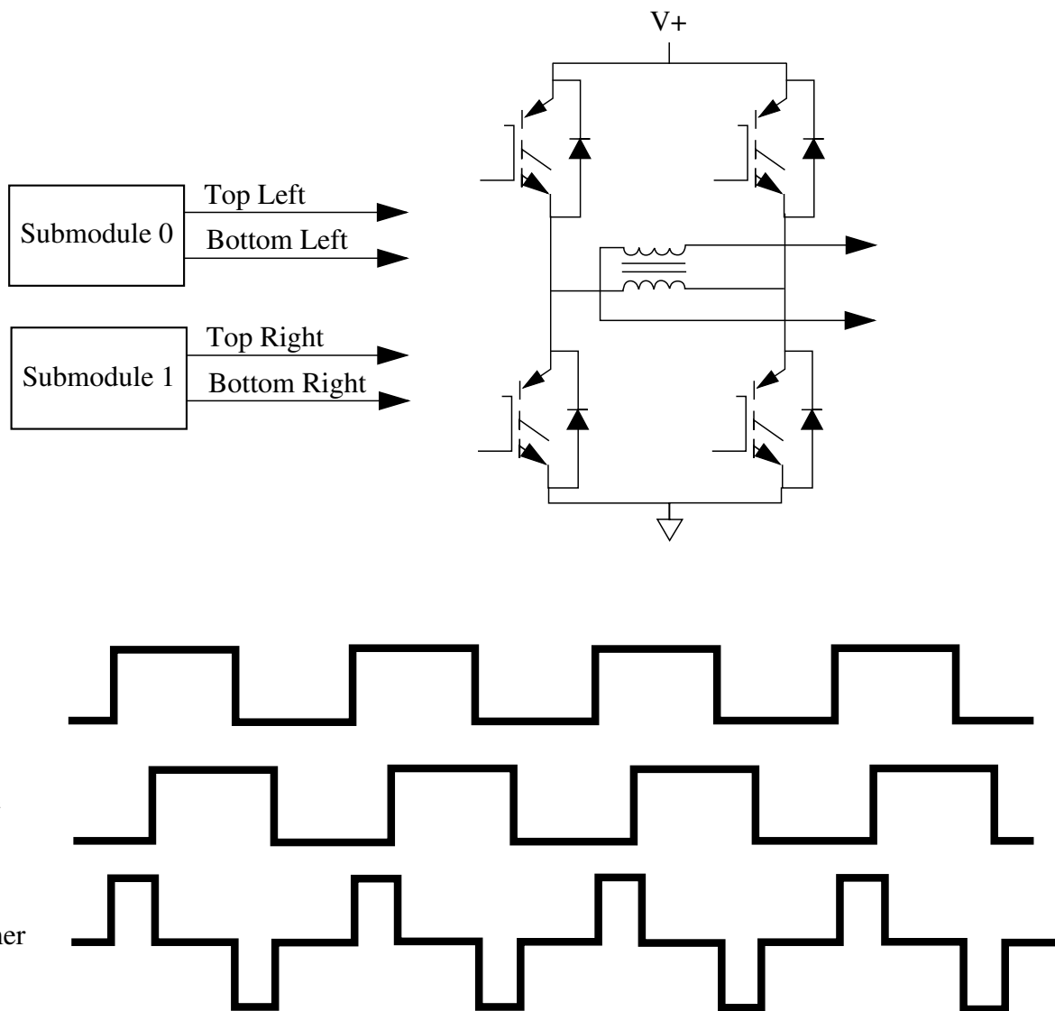
Figure 49-5. Phase Shifted PWMs Applied to a Transformer Primary
