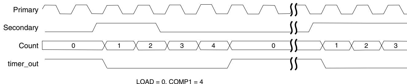
Figure 48-6. One-Shot Mode (CTRL[LENGTH]=1)
