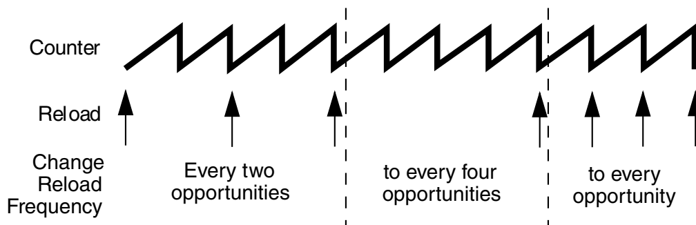
Figure 49-31. Full Cycle Reload Frequency Change
