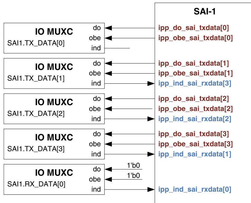
Figure 32-2. SAI-1 TX/RX Data Multiplexing
