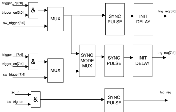
Figure 61-2. Trigger process diagram
