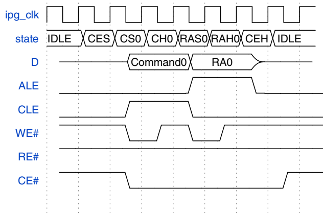
Figure 24-30. NAND Flash access Address type - One Byte Row Address
