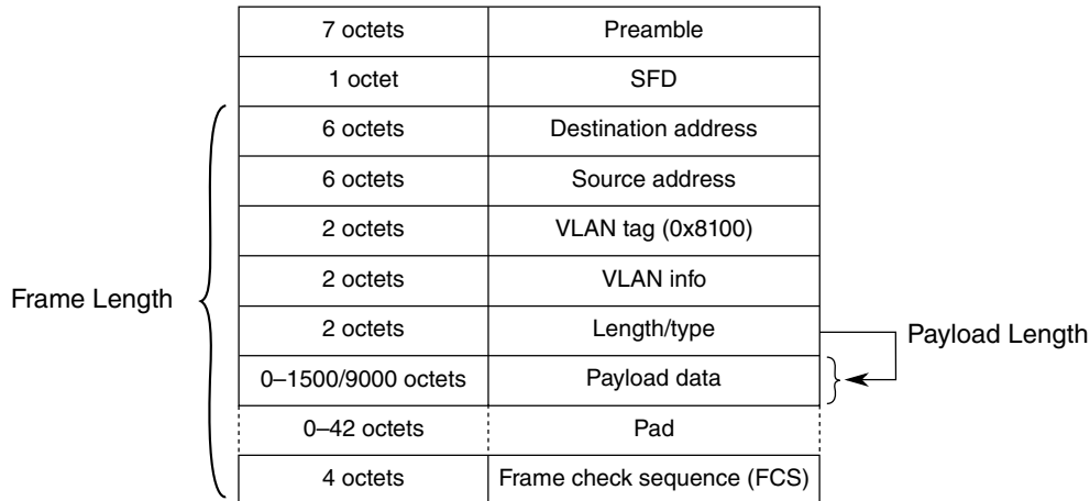
Figure 36-3. VLAN-tagged MAC frame format overview
