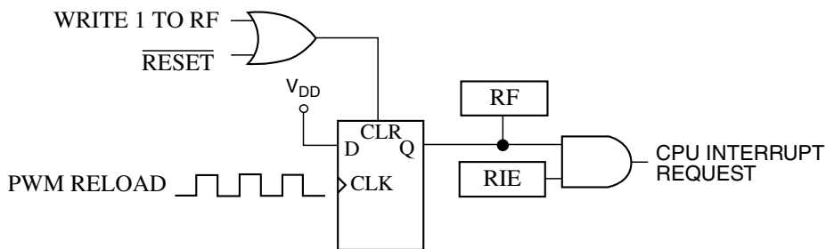
Figure 49-34. PWMF Reload Interrupt Request
