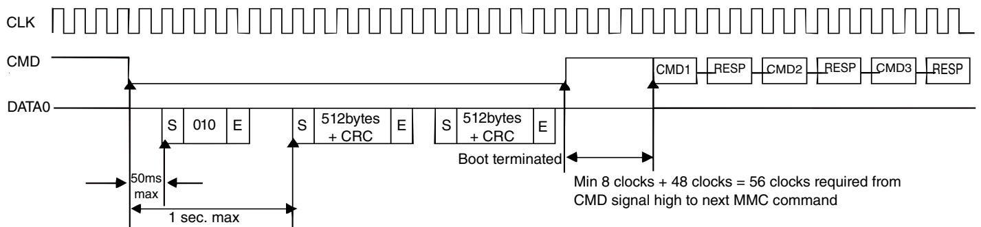
Figure 25-16. MultiMediaCard state diagram (normal boot mode)
