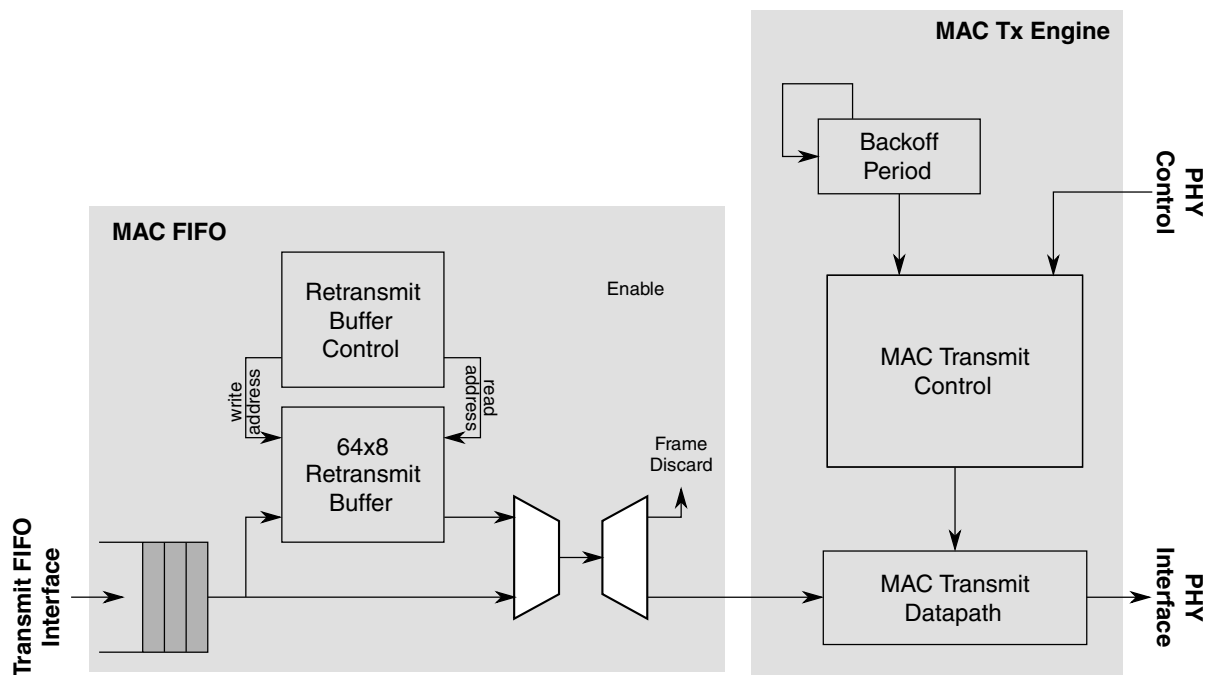
Figure 36-7. Packet re-transmit overview
