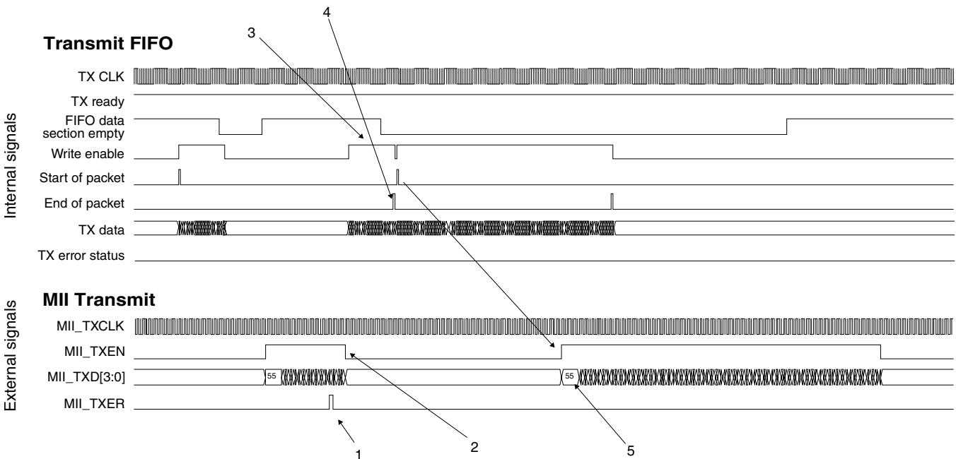
Figure 36-16. Transmit FIFO underflow protection
