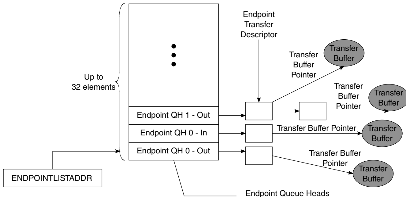
Figure 37-27. EndPoint Queue Head Organization
