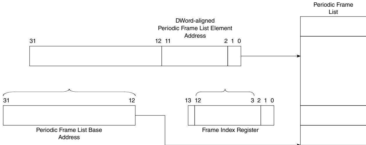
Figure 37-6. Derivation of Pointer into Frame List Array
