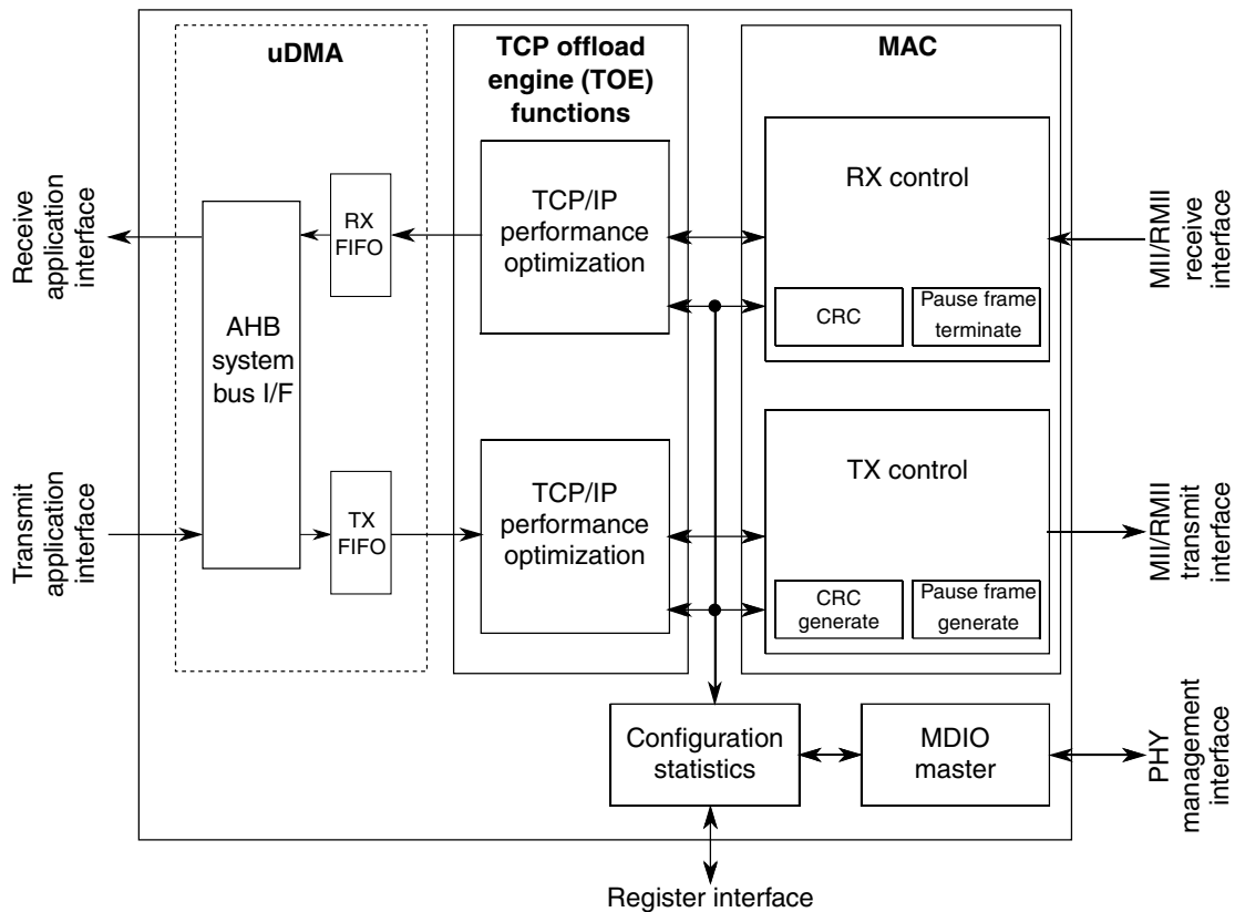
Figure 36-1. Ethernet MAC-NET core block diagram
