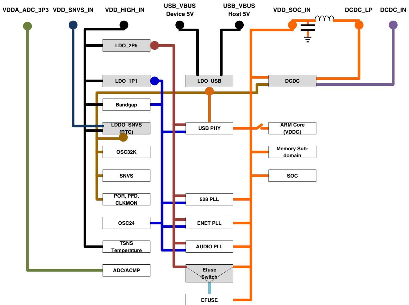
Figure 12-4. SOC Power Tree
