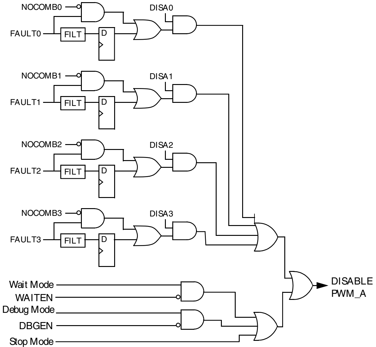
Figure 49-27. Fault Decoder for PWM_A
