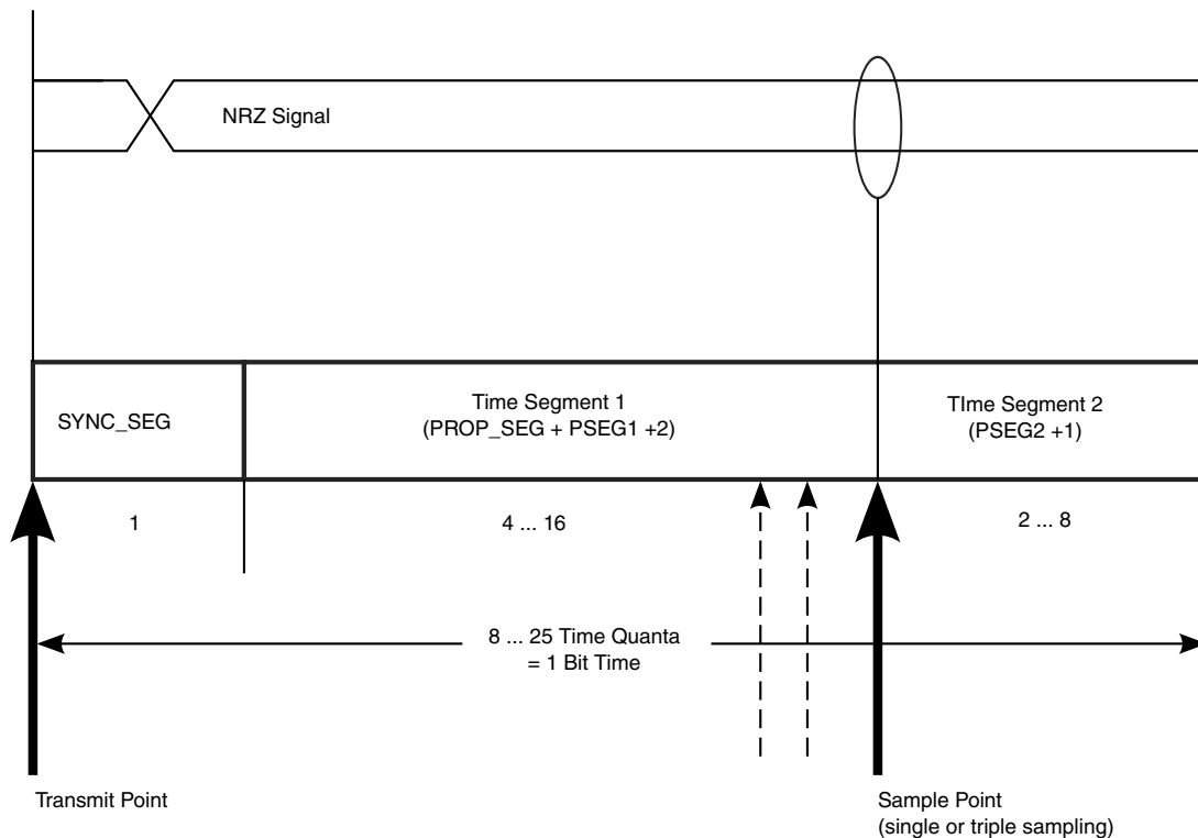
Figure 39-2. Segments within the Bit Time
