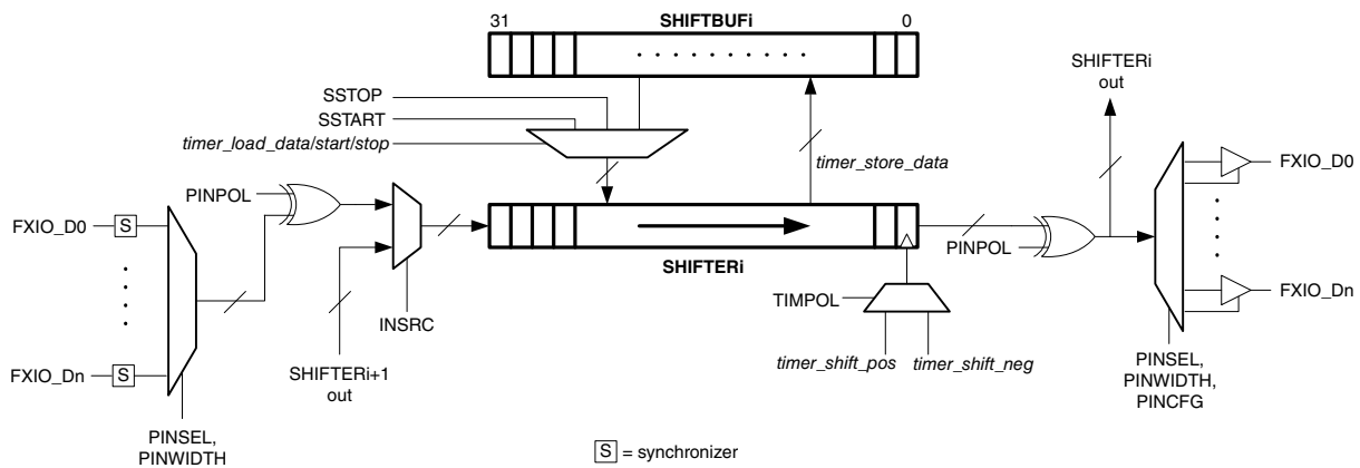
Figure 44-2. Shifter Microarchitecture
