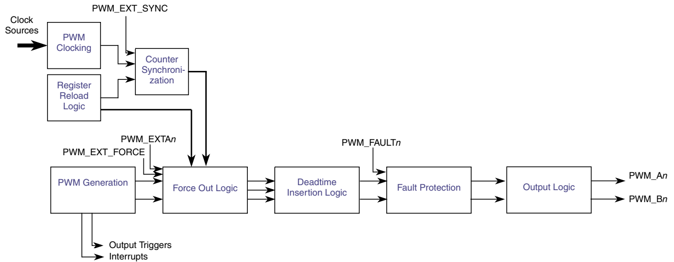
Figure 49-12. High-Level Output PWM Generation Block Diagram
