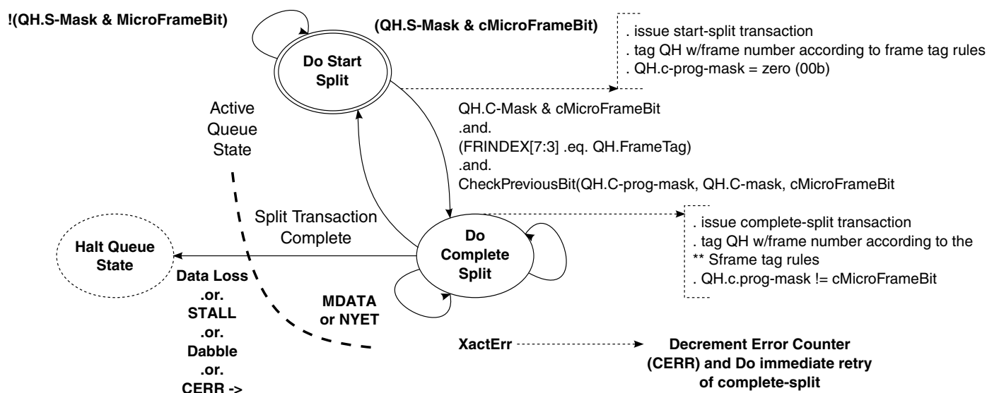
Figure 37-23. Split Transaction State Machine for Interrupt
