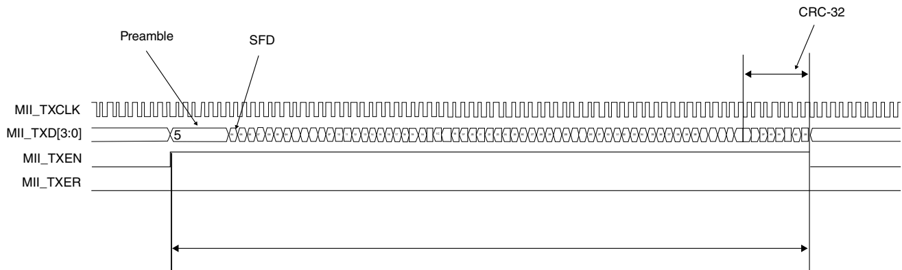
Figure 36-22. MII transmit operation
