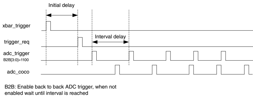
Figure 61-3. ETC ADC interface timing
