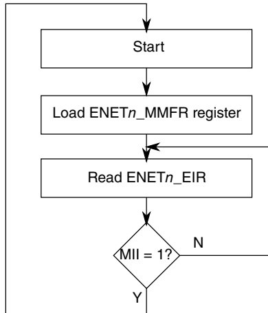
Figure 36-18. MDIO access overview
