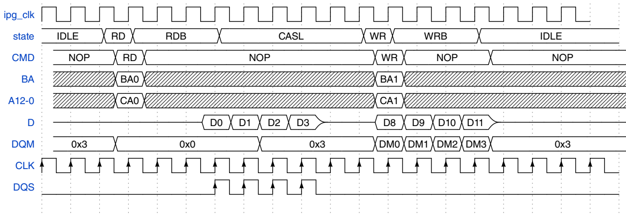
Figure 24-20. SDRAM Read-to-Write access (CL=3)
