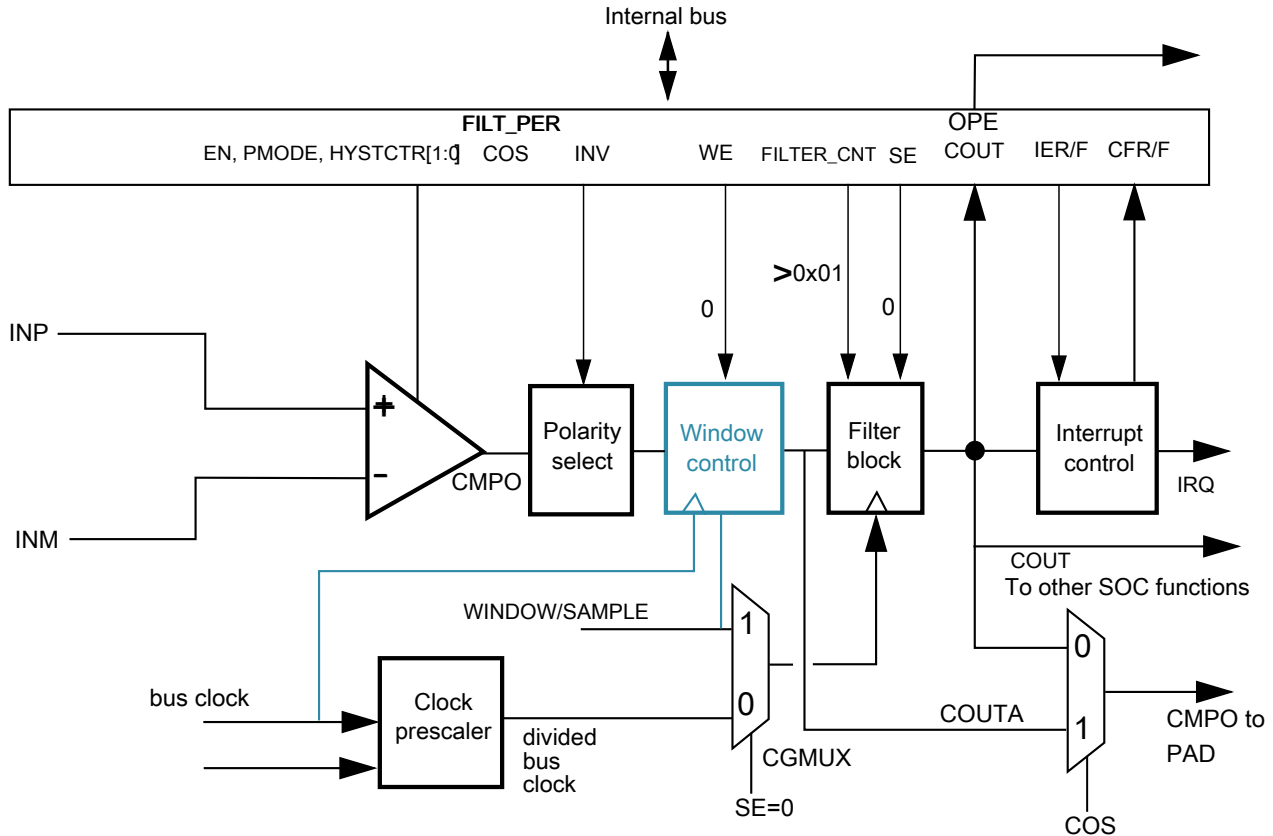
Figure 59-7. Sampled, Filtered (# 4B): sampling point internally derived
