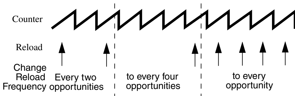
Figure 49-32. Half Cycle Reload Frequency Change
