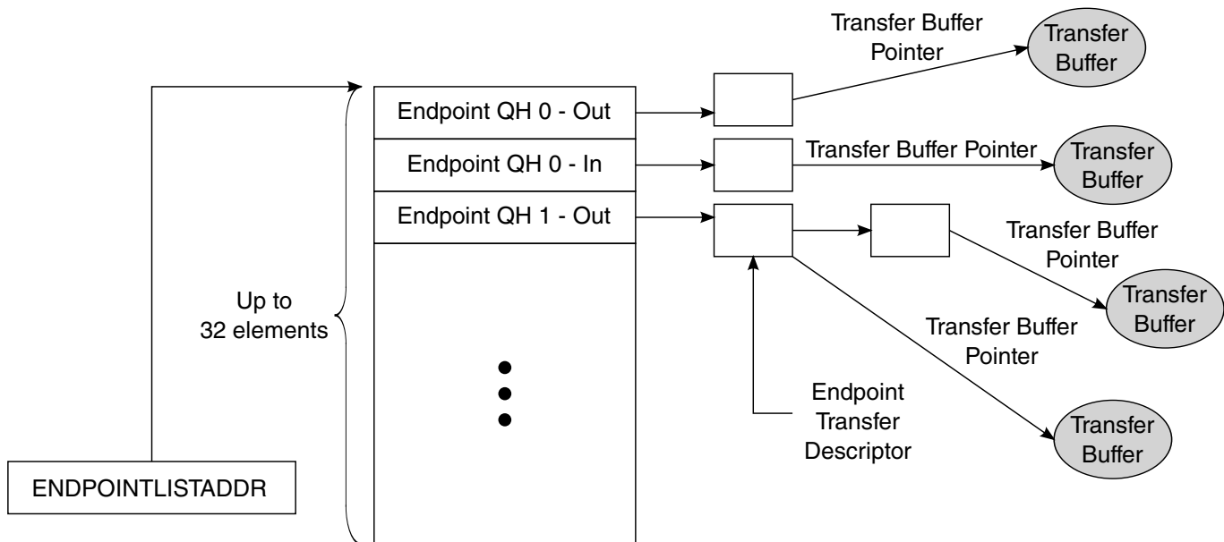
Figure 37-29. End Point Queue Head Diagram
