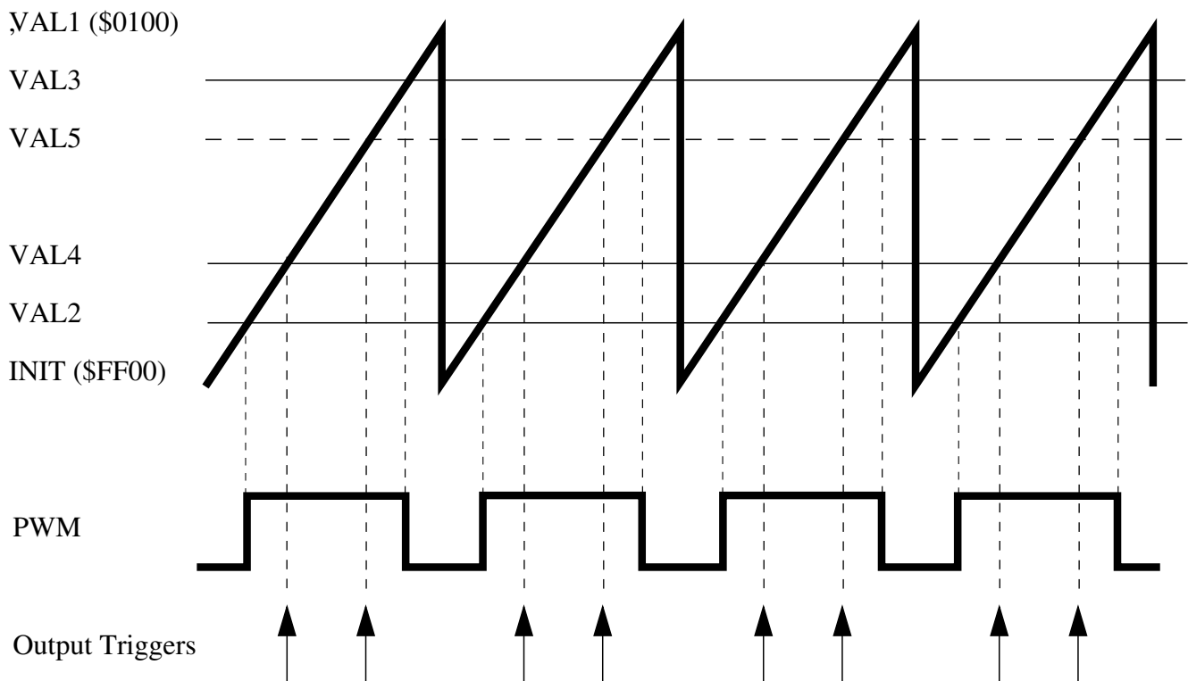
Figure 49-7. Multiple Output Trigger Generation in Hardware
