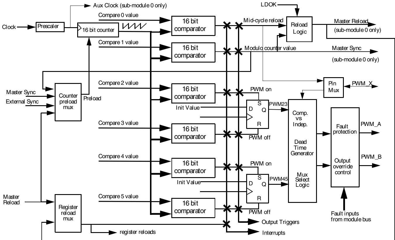
Figure 49-1. PWM Submodule Block Diagram
