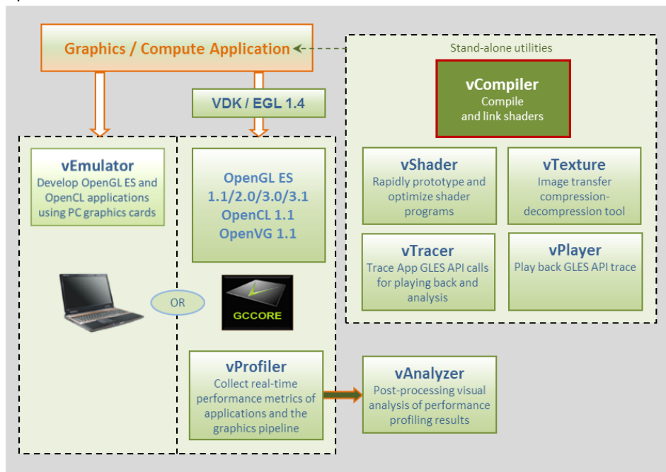
Figure 38 vCompiler compiler/linker
