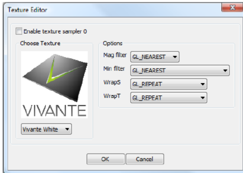
Figure 37 Textures
