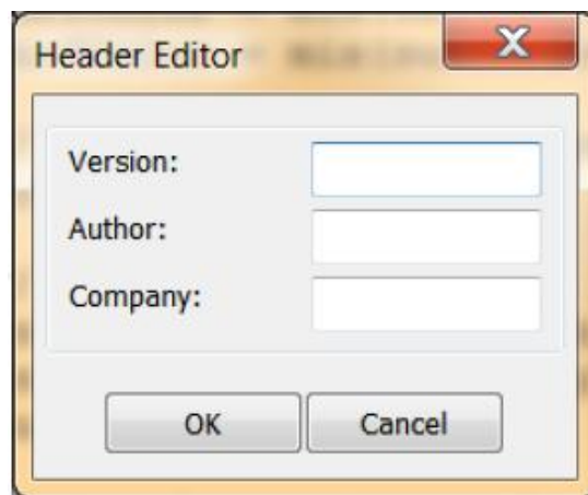
Figure 33 Header editor
