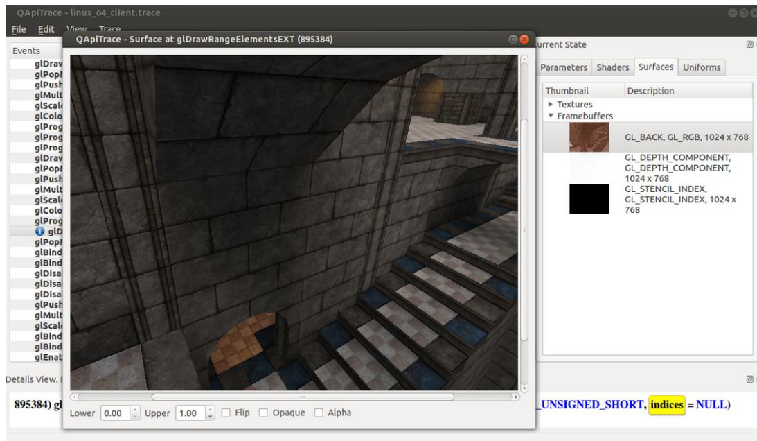
Figure 58 Checking Framebuffer
