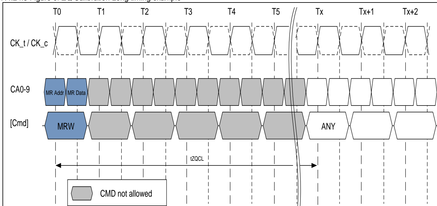
7.4.24.3 Figure of ZQ Calibration Long timing example
