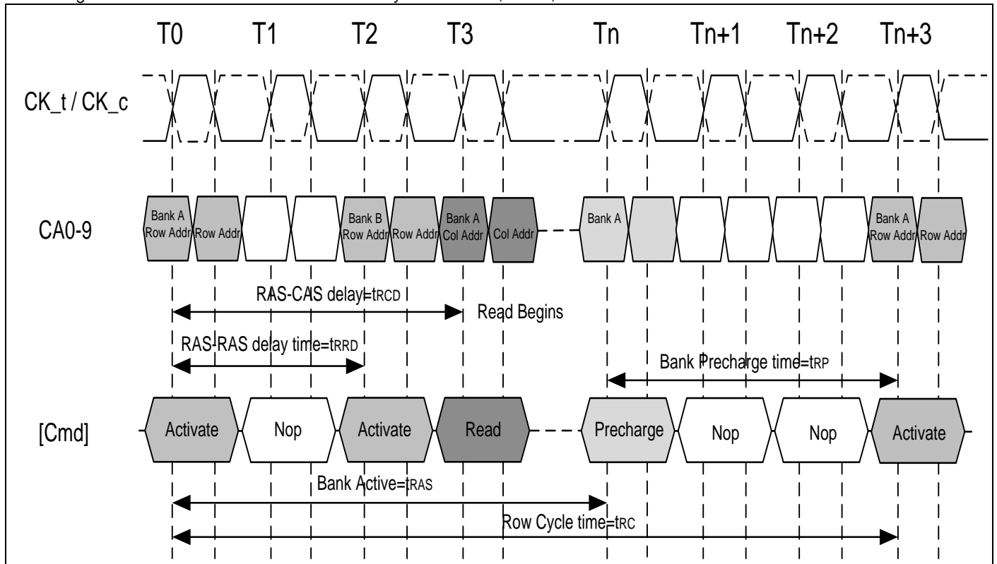
7.4.1.1 Figure of LPDDR2-S4 : Activate command cycle : t RCD =3,t RP =3,t RRD =2
