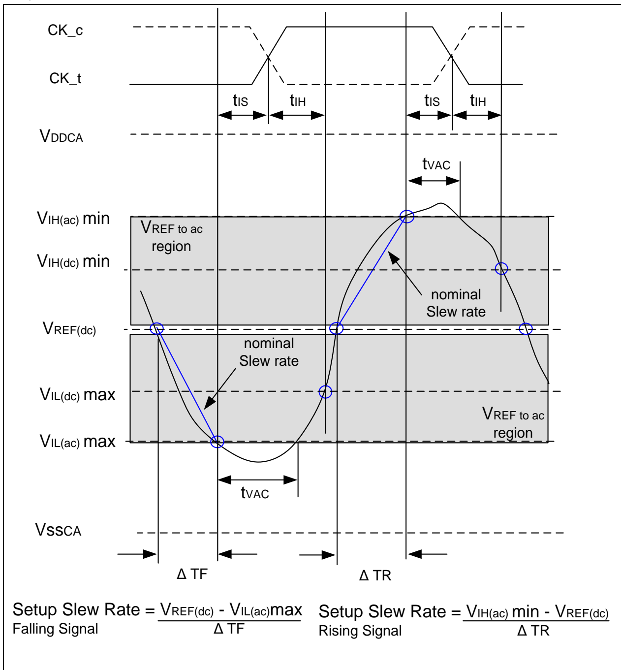
8.6.2.5 Figure of nominal slew rate and tVAC for tIS for CA and CS_n with respect to clock.
