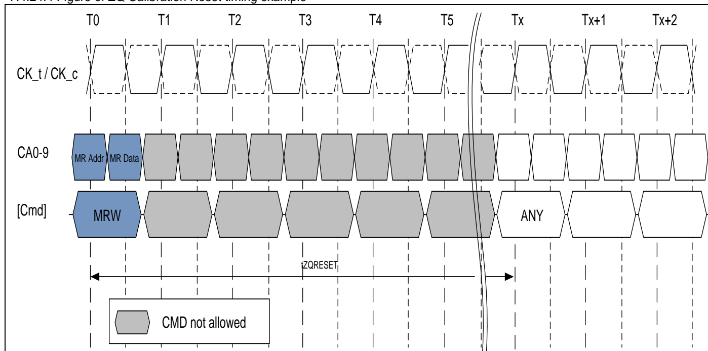
7.4.24.4 Figure of ZQ Calibration Reset timing example
