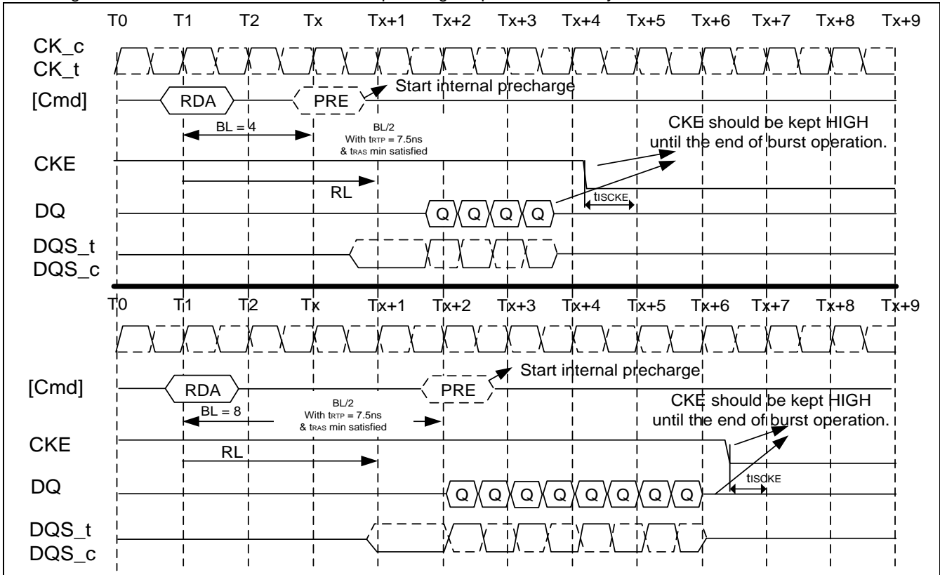
7.4.26.5 Figure of LPDDR2 SDRAM Read with auto precharge to power-down entry
