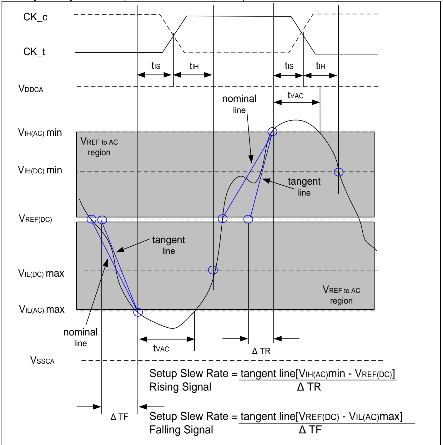
8.6.2.7 Figure of tangent line for setup time tIS for CA and CS_n with respect to clock
