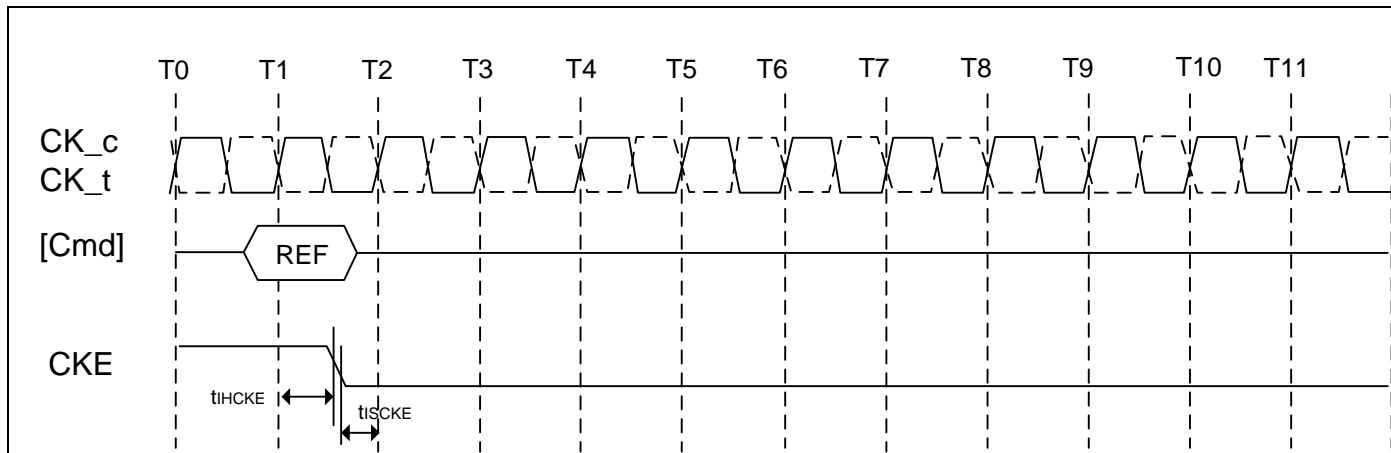
7.4.26.8 Figure of LPDDR2-S4 Refresh command to power-down entry
