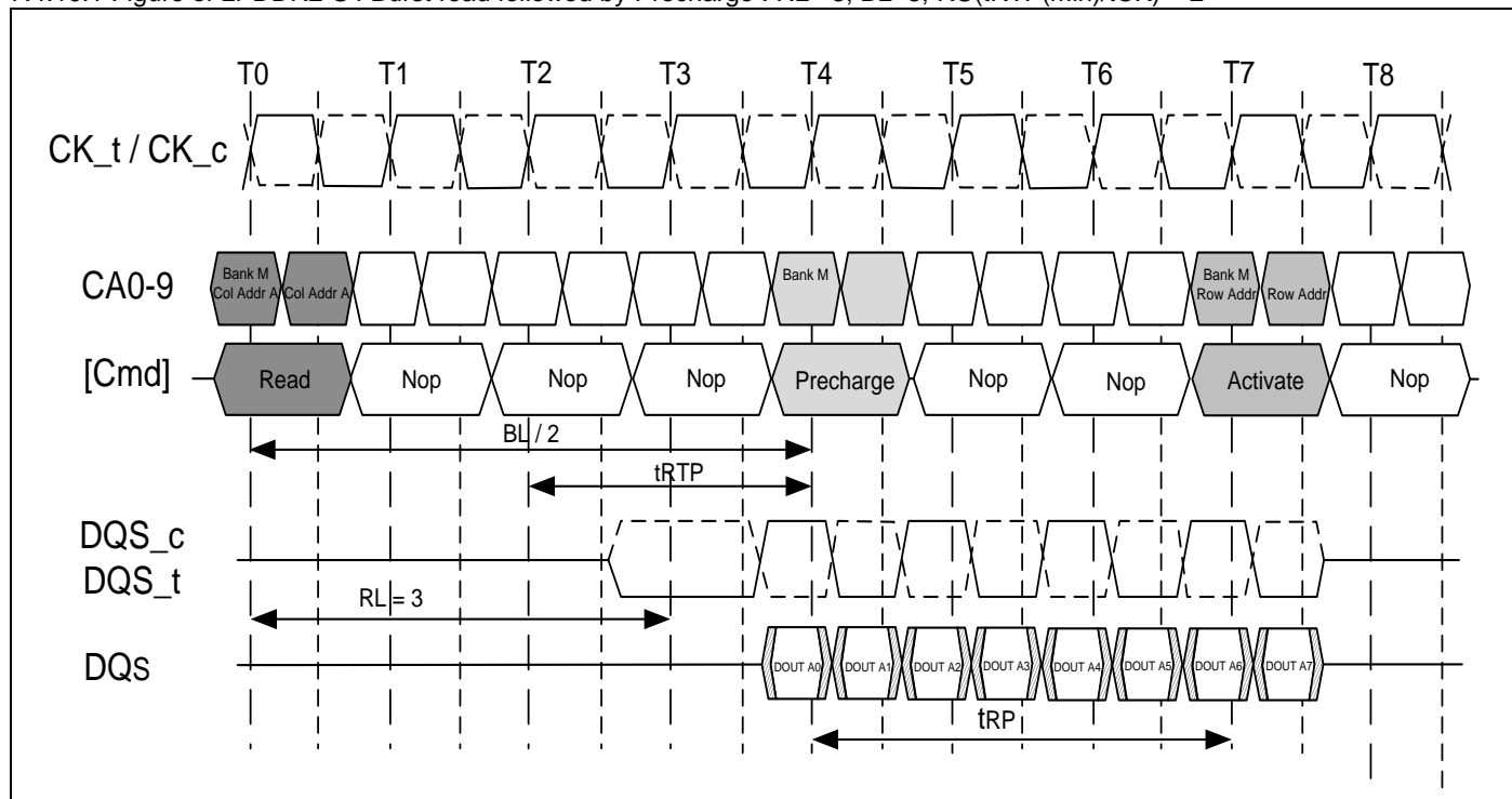
7.4.10.1 Figure of LPDDR2-S4 Burst read followed by Precharge : RL= 3, BL=8, RU(tRTP(min))/tCK) = 2
