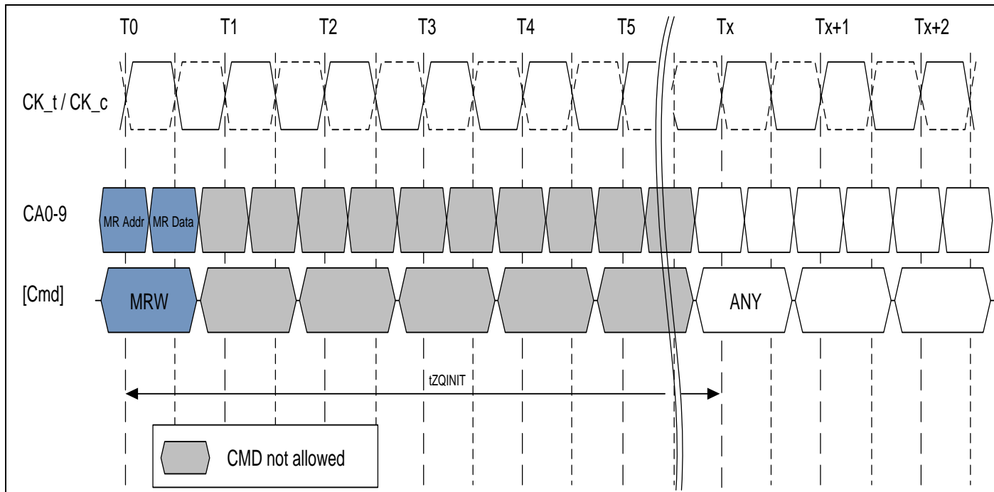
7.4.24.1 Figure of ZQ Calibration Initialization timing example
