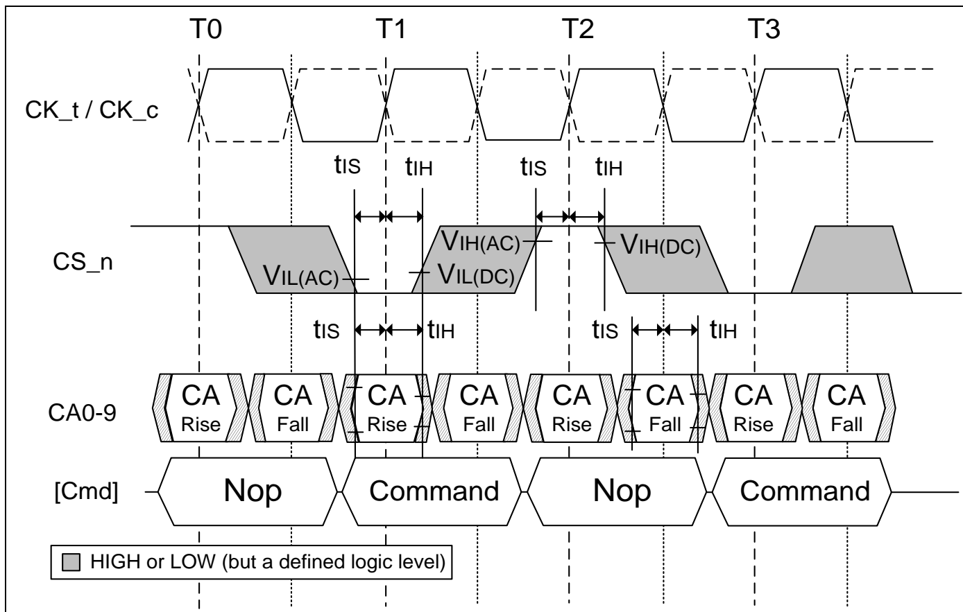
7.4.1.3 Figure of LPDDR2 Command Input Setup and Hold Timing
