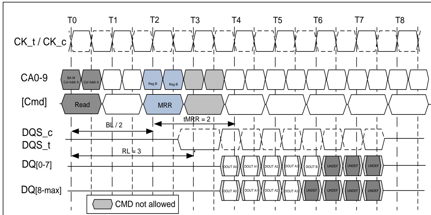
7.4.20.2 Figure of LPDDR2 Read to MRR timing example : RL = 3, tMRR = 2
