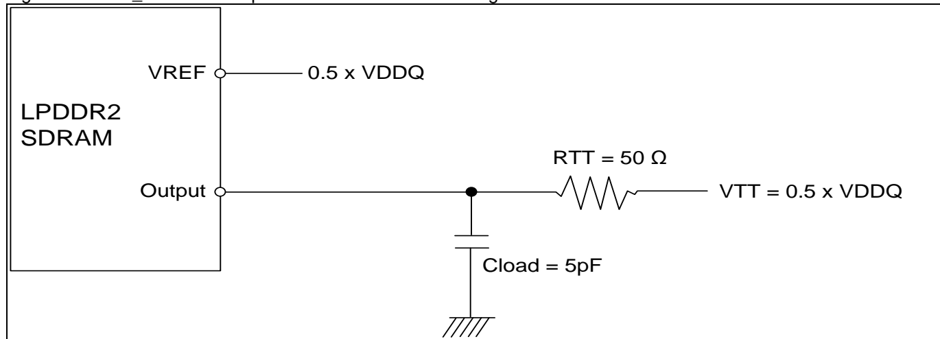
Figure of HSUL_12 Driver Output Reference Load for Timing and Slew Rate
