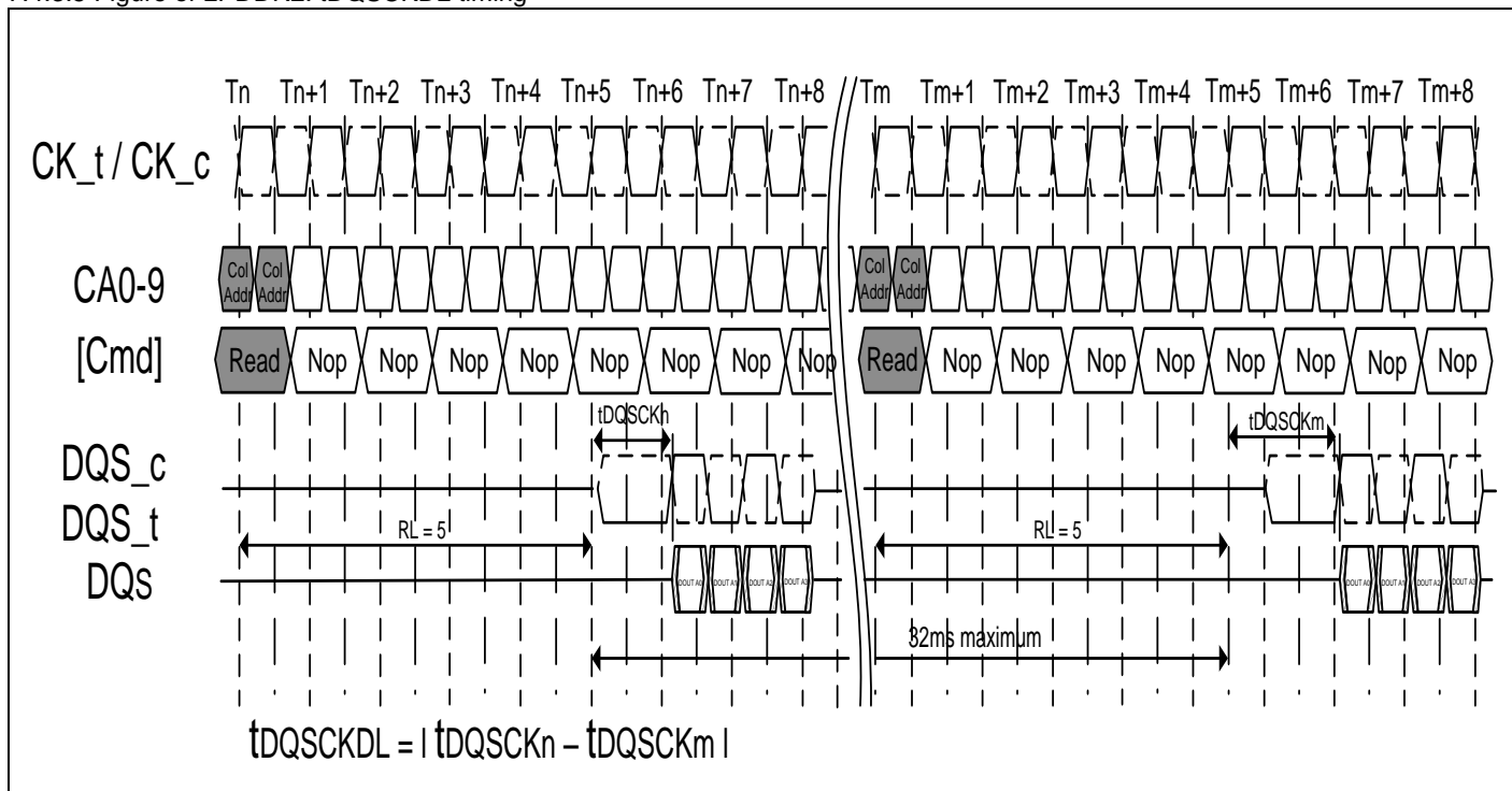
7.4.3.5 Figure of LPDDR2: tDQSCKDL timing
