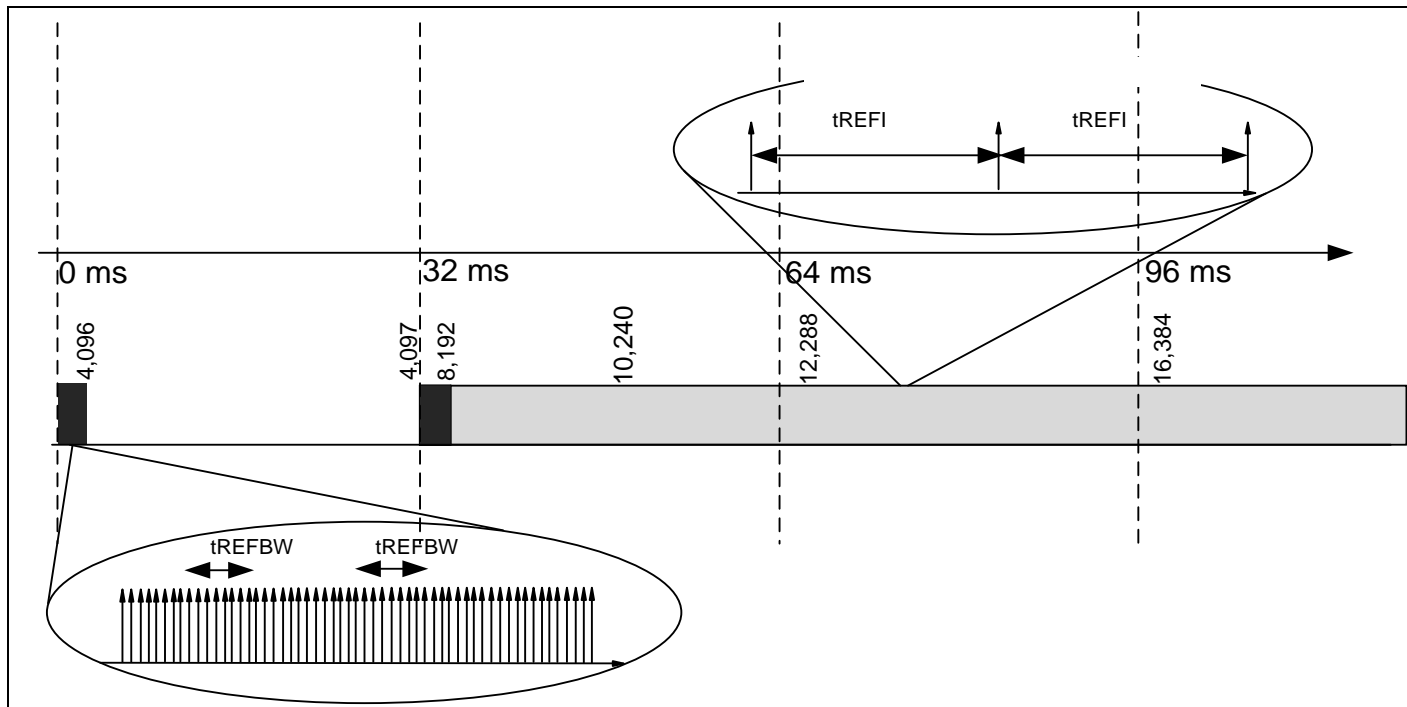
7.4.16.3 Figure of LPDDR2-S4: Allowable Transition from Repetitive Burst Refresh with Subsequent Refresh Pause to Regular, Distributed Refresh Pattern
