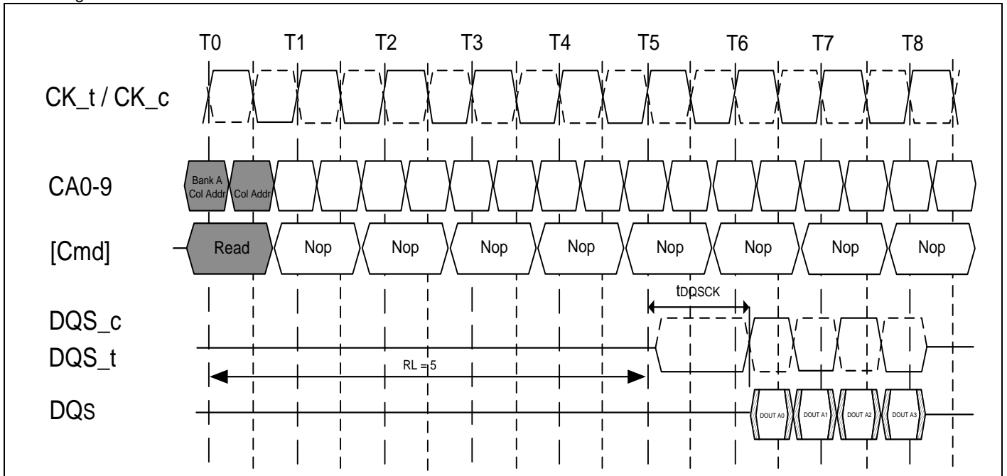
7.4.3.3 Figure of LPDDR2-S4 : Burst read : RL = 5. BL = 4. tDQSK > tCK
