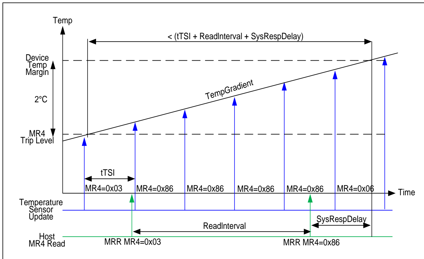
7.4.21.1 Figure of Temp Sensor Timing
