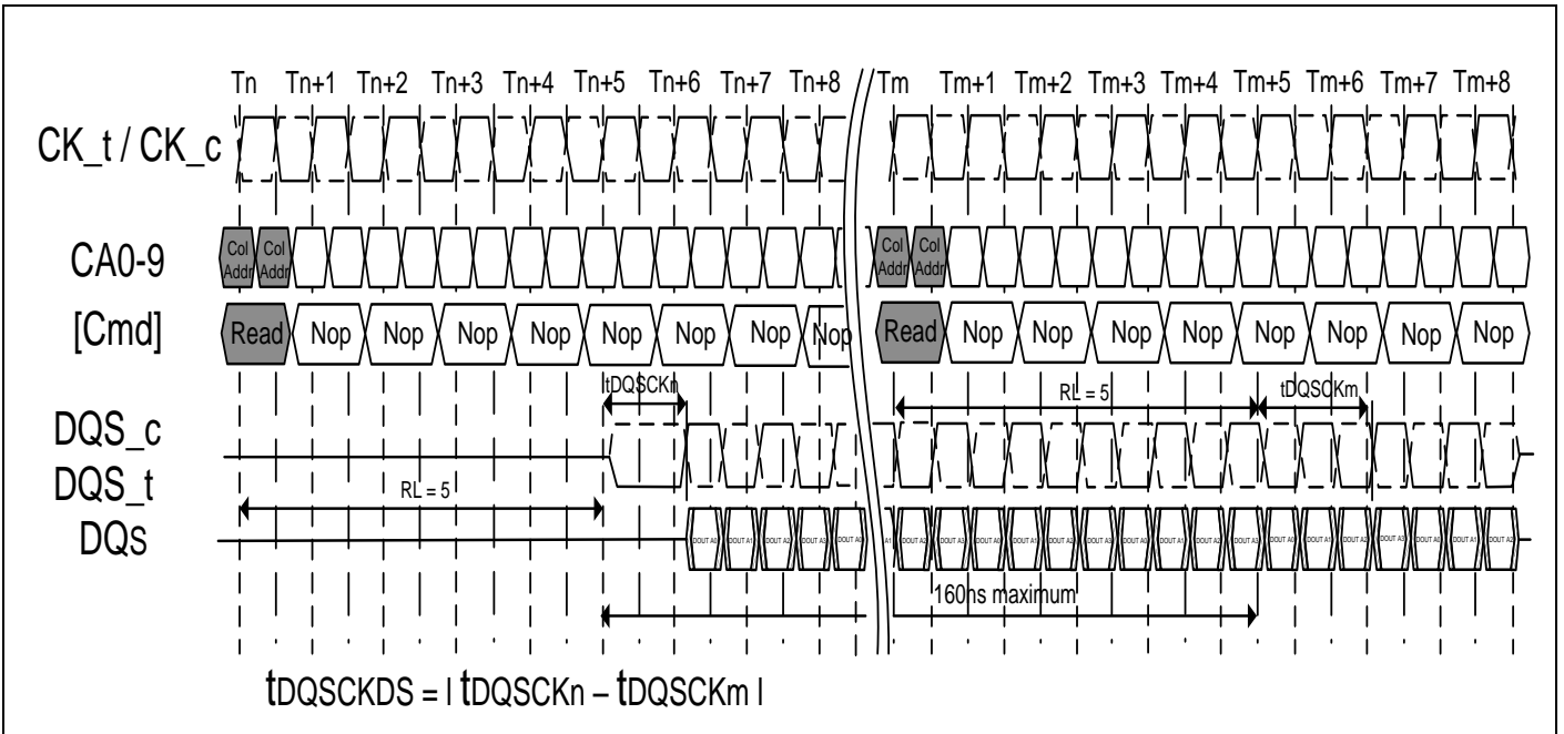
7.4.3.7 Figure of LPDDR2: tDQSKDS timing
