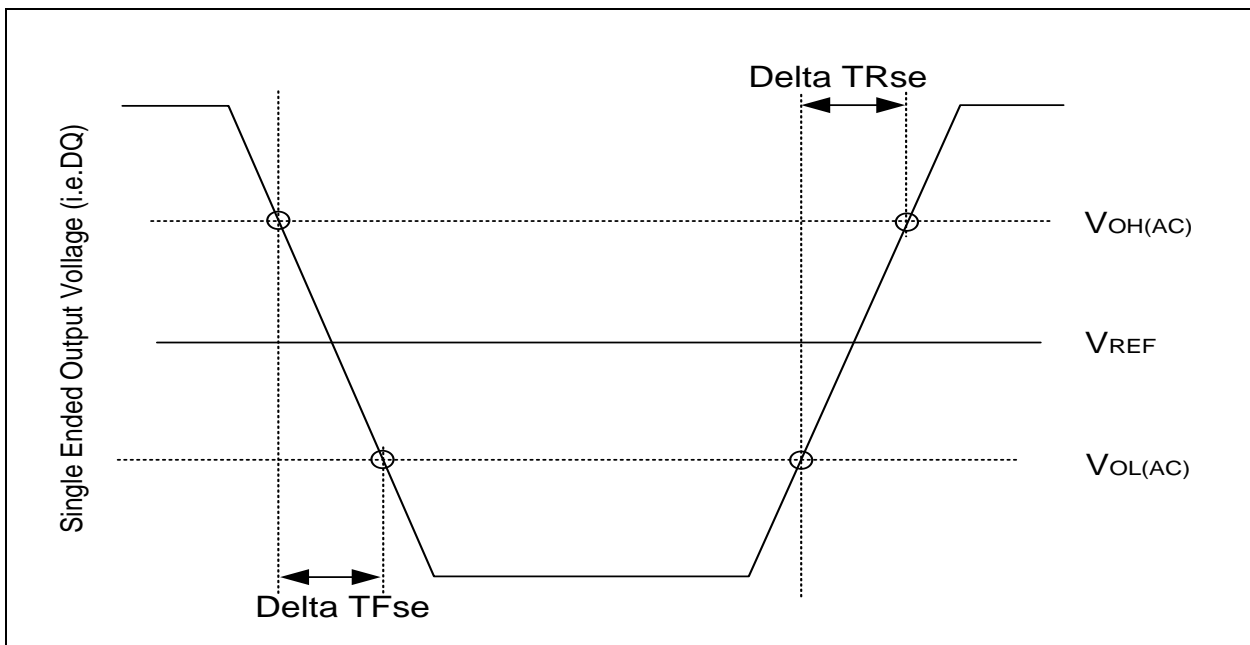
Figure of Single Ended Output Slew Rate Definiton
