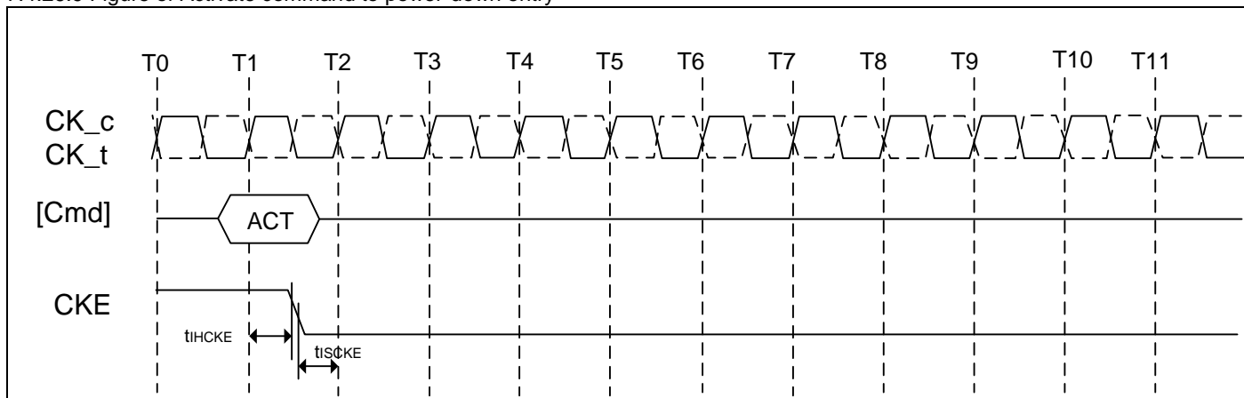
7.4.26.9 Figure of Activate command to power-down entry
