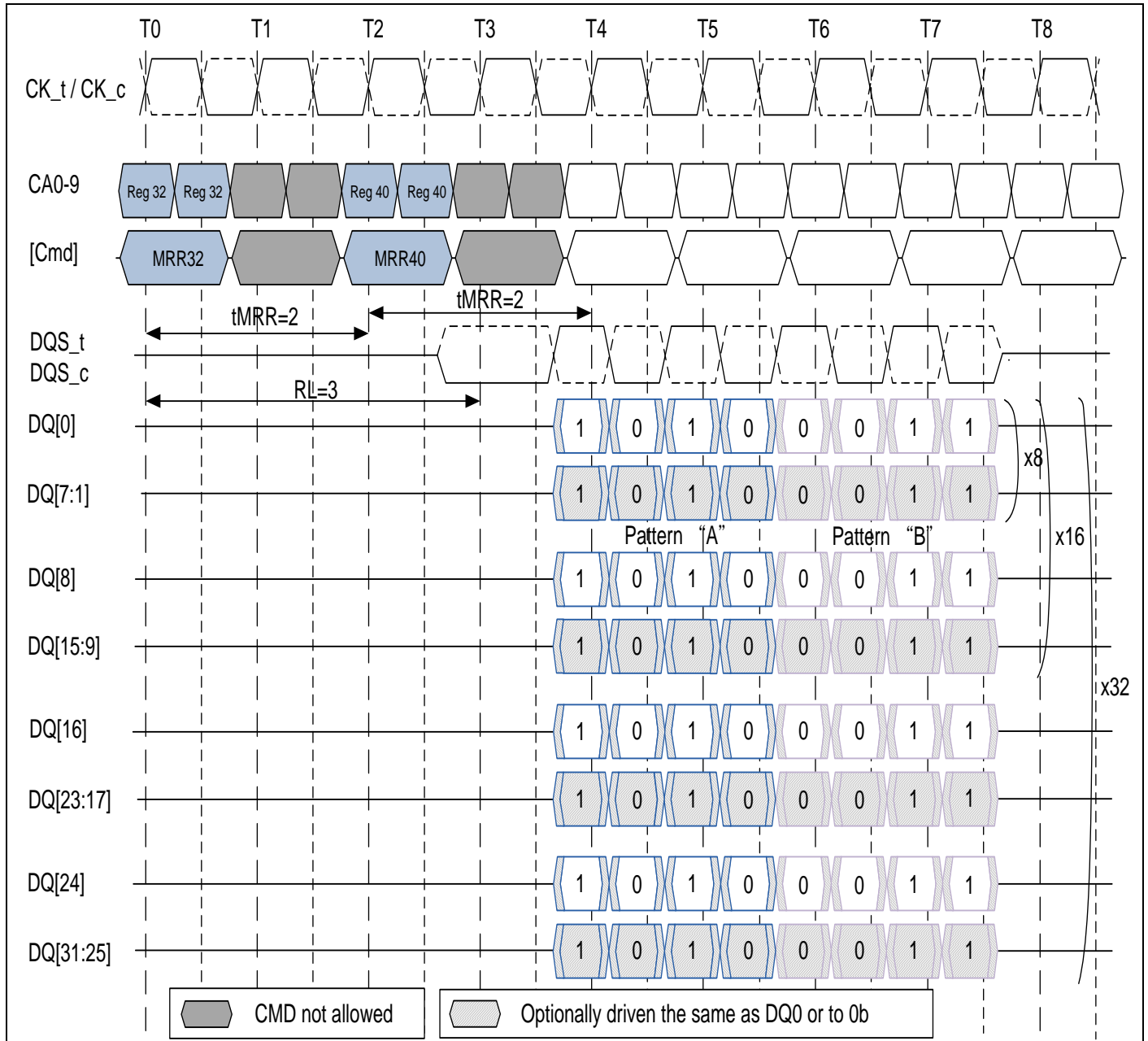
7.4.21.3 Figure of MR32 and MR40 DQ Calibration timing example: RL = 3, tMRR = 2
