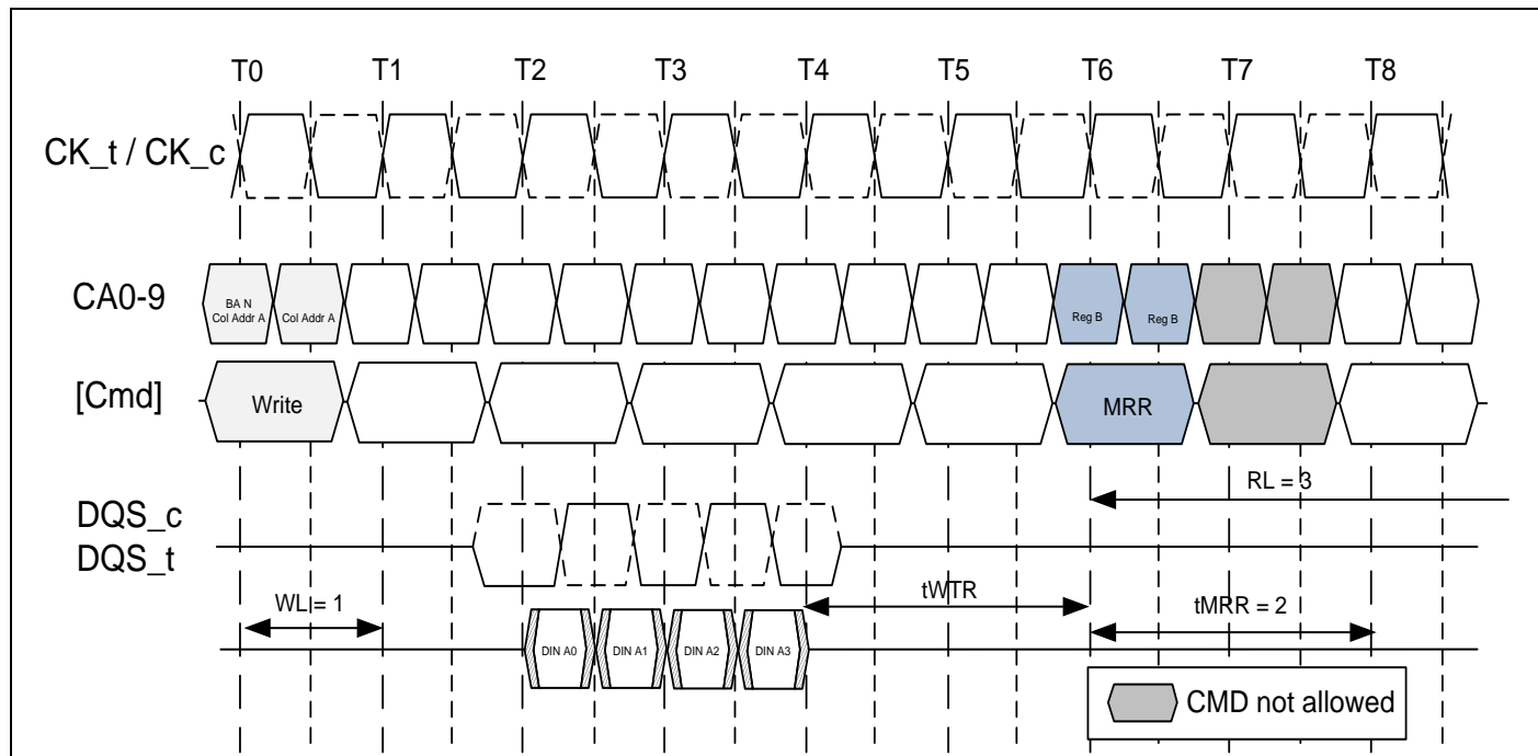
7.4.20.3 Figure of LPDDR2 : Burst Write Followed by MRR : RL = 3, WL = 1, BL = 4
