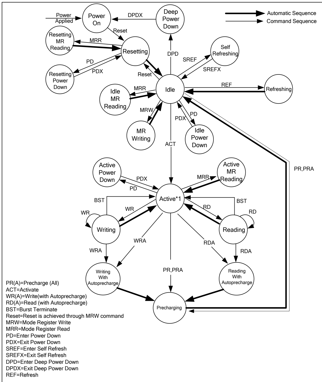
7.1.1 Figure of Simplified LPDDR2 Bus Interface State Diagram
