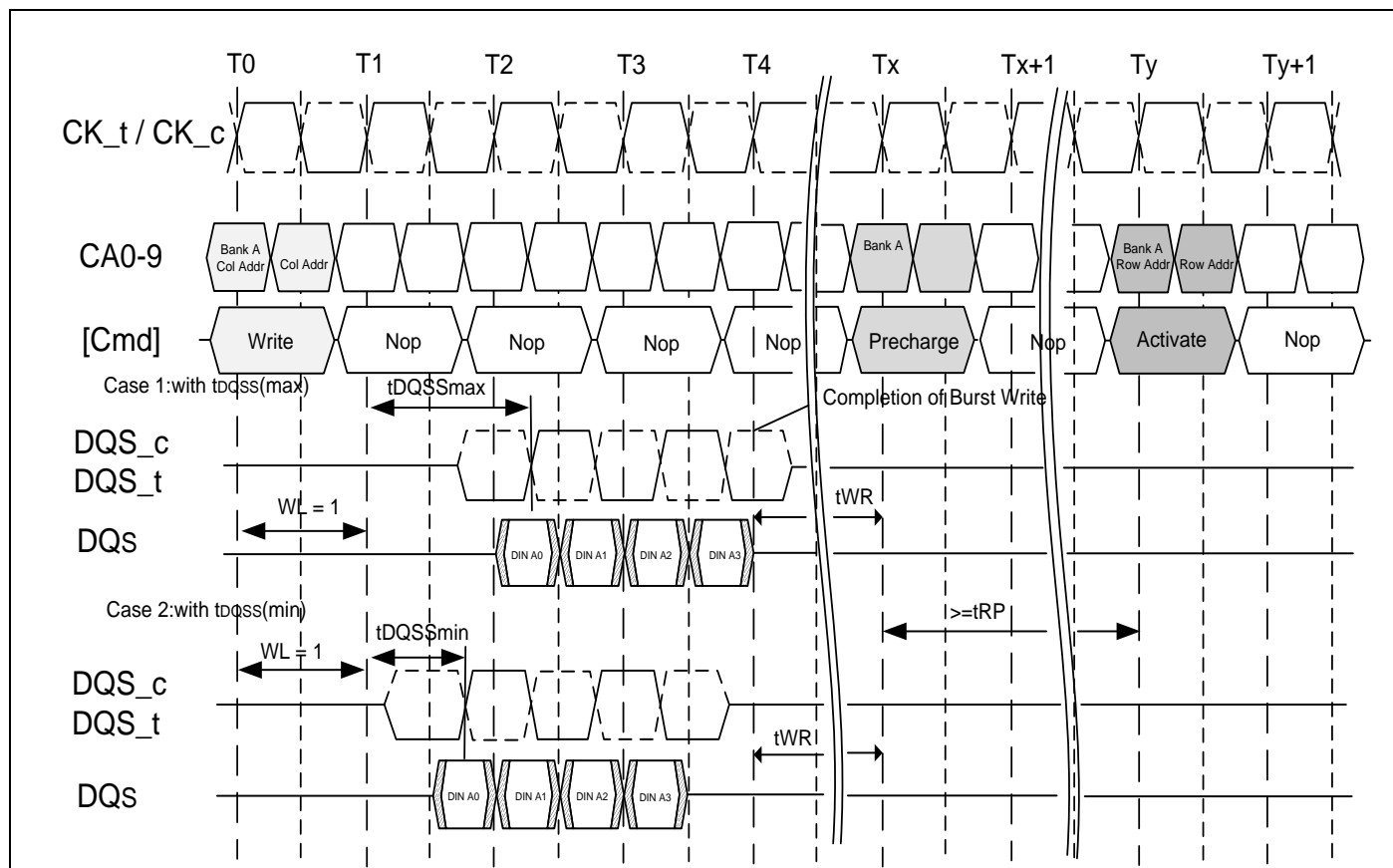
7.4.11.1 Figure of LPDDR2-S4 : Burst write follwed by precharge : WL = 1, BL = 4
