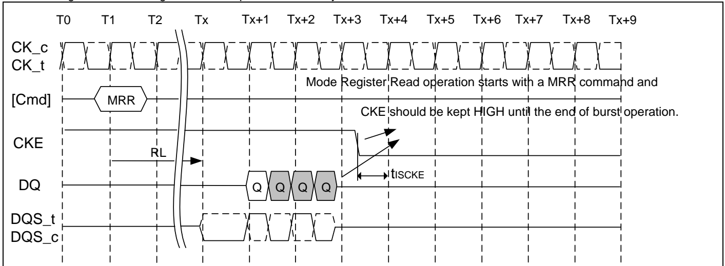
7.4.26.11 Figure of Mode Register Read to power-down entry
