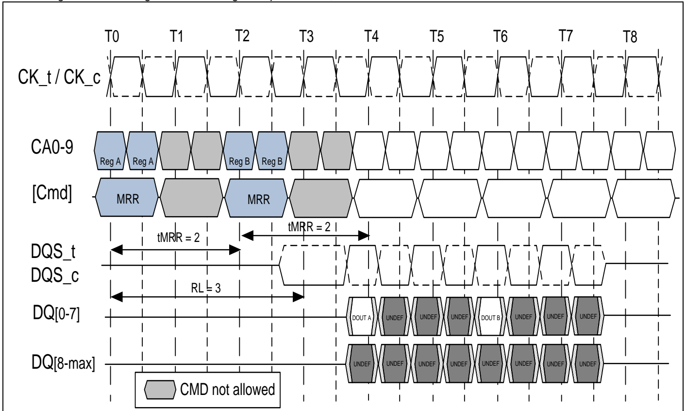
7.4.20.1 Figure of Mode Register Read timing example : RL = 3, tMRR = 2
