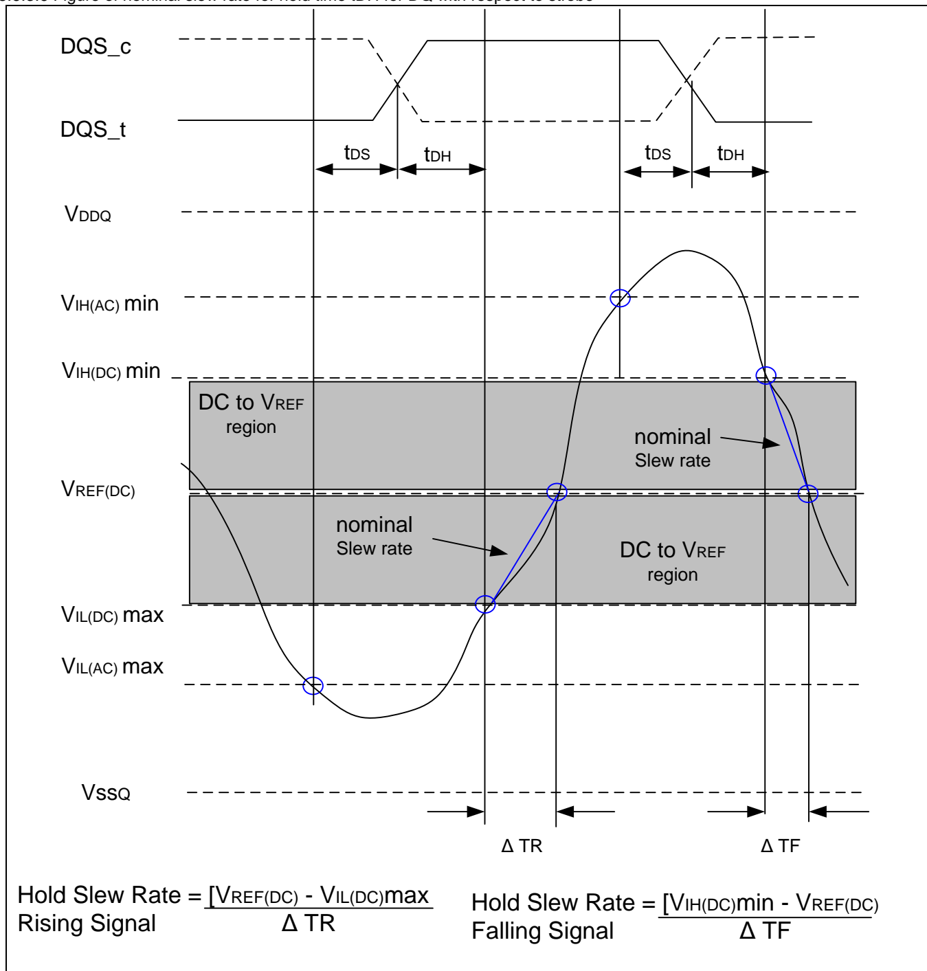
8.6.3.6 Figure of nominal slew rate for hold time t DH for DQ with respect to strobe
