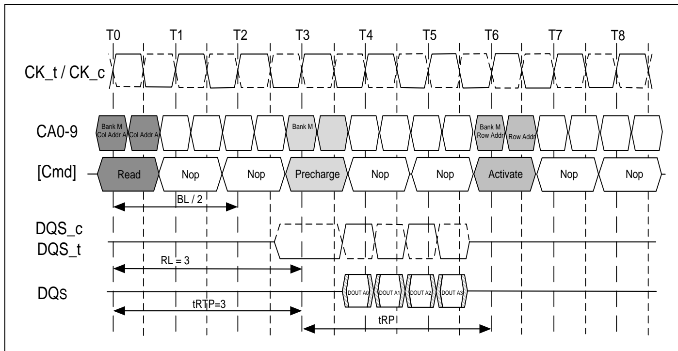
7.4.10.2 Figure of LPDDR2-S4 : Burst read followed by Precharge : RL= 3, BL=4, RU(tRTP(min))/tCK)=3
