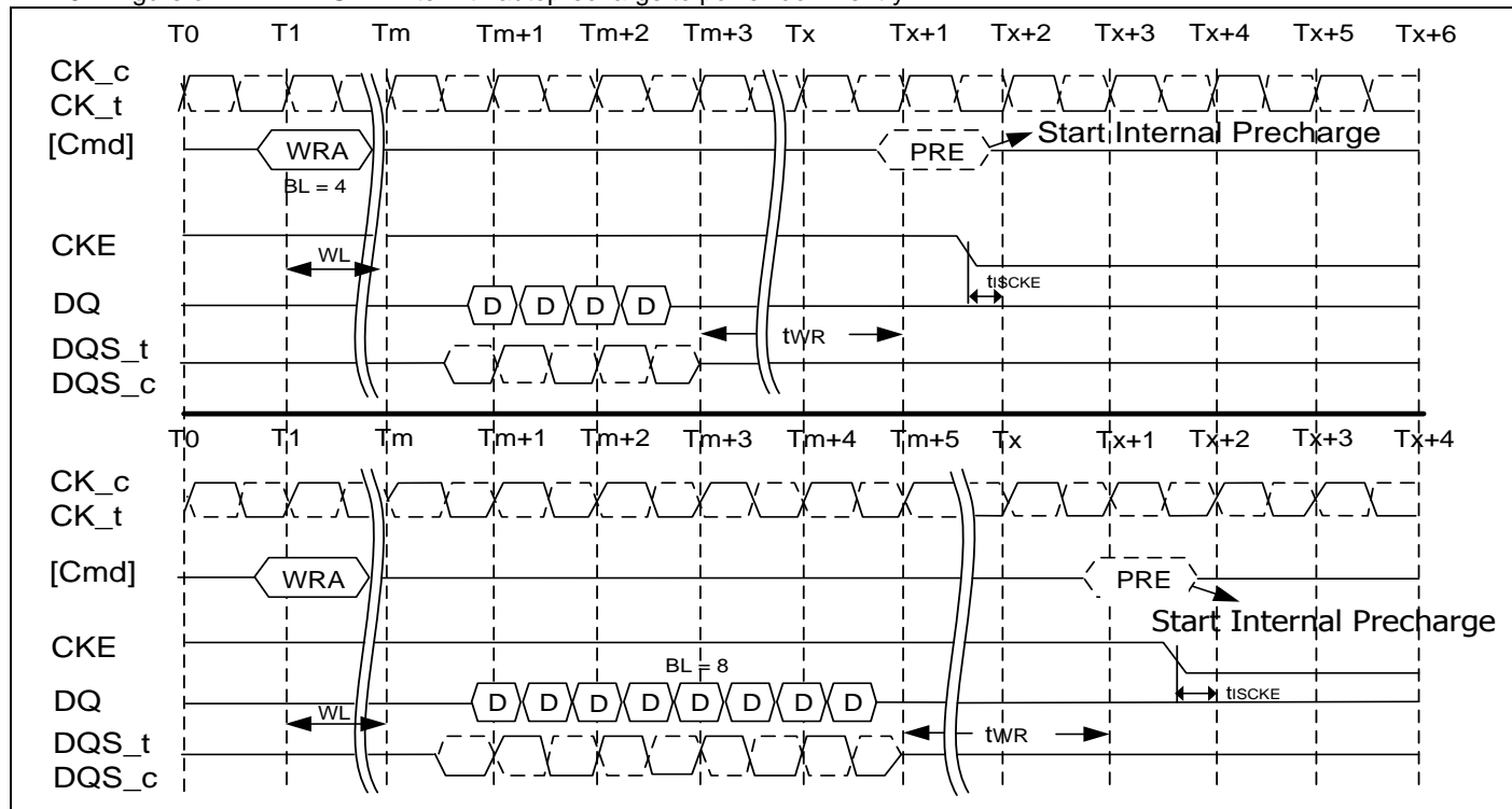
7.4.26.7 Figure of LPDDR2-S4: Write with autoprecharge to power-down entry
