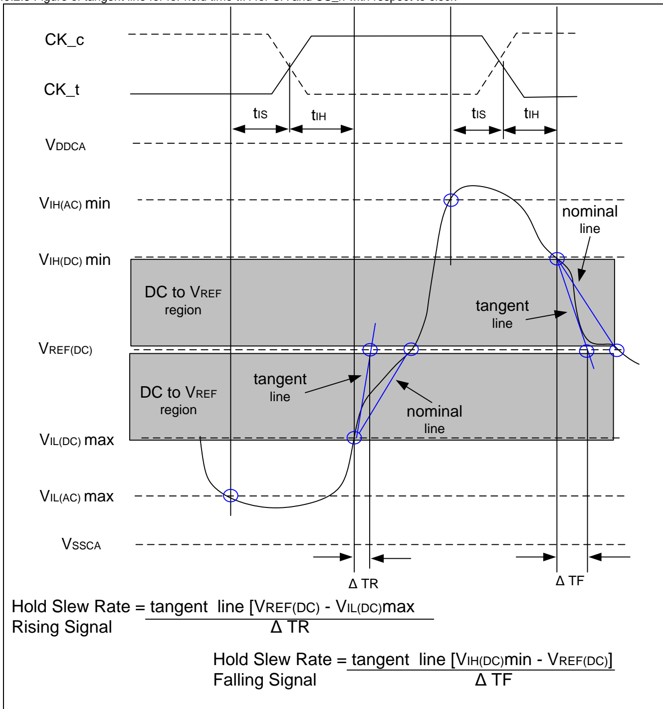
8.6.2.8 Figure of tangent line for for hold time tIH for CA and CS_n with respect to clock
