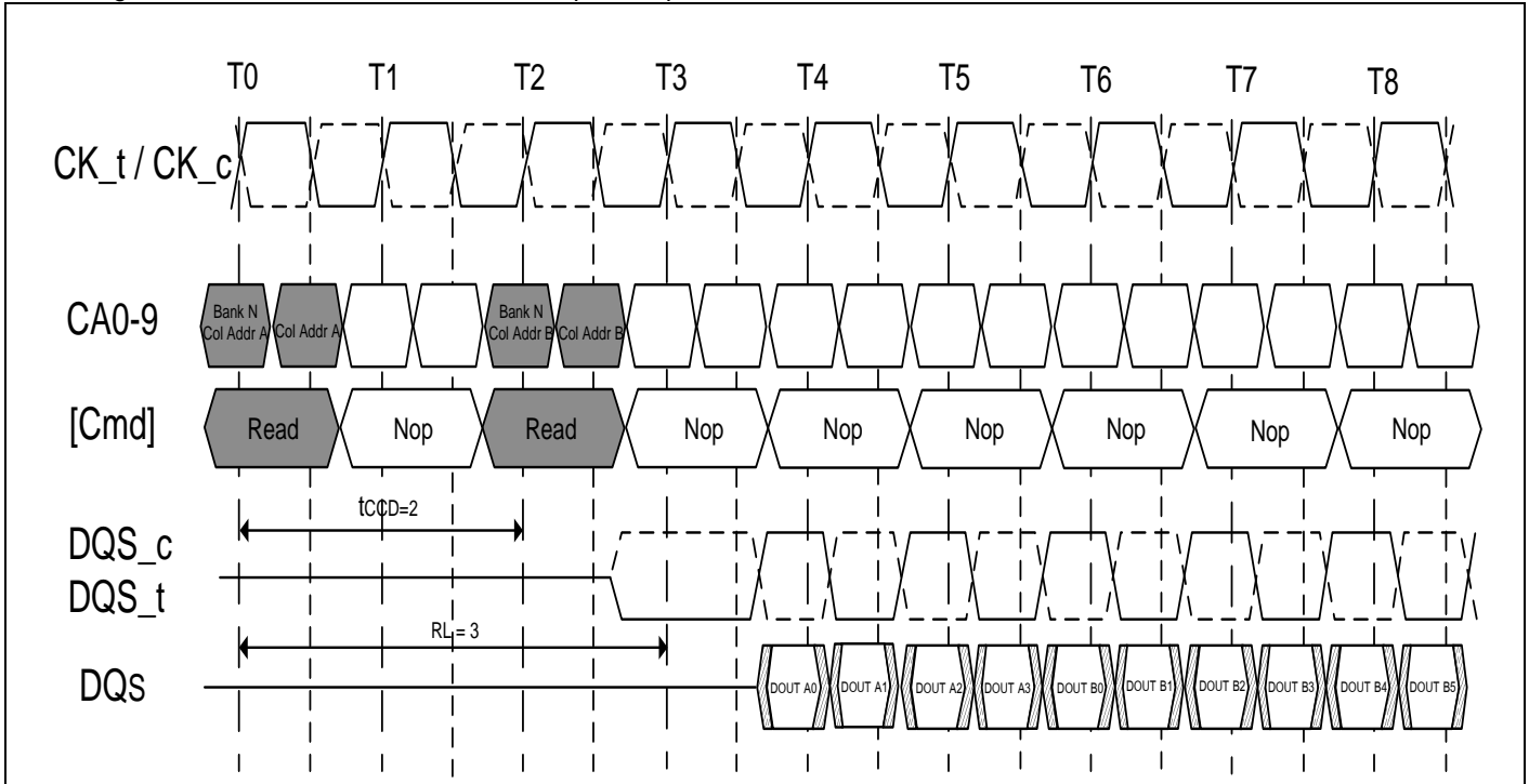
7.4.4.1 Figure of LPDDR2-S4 : Read burst interrupt example : RL = 3, BL= 8, tCCD=2
