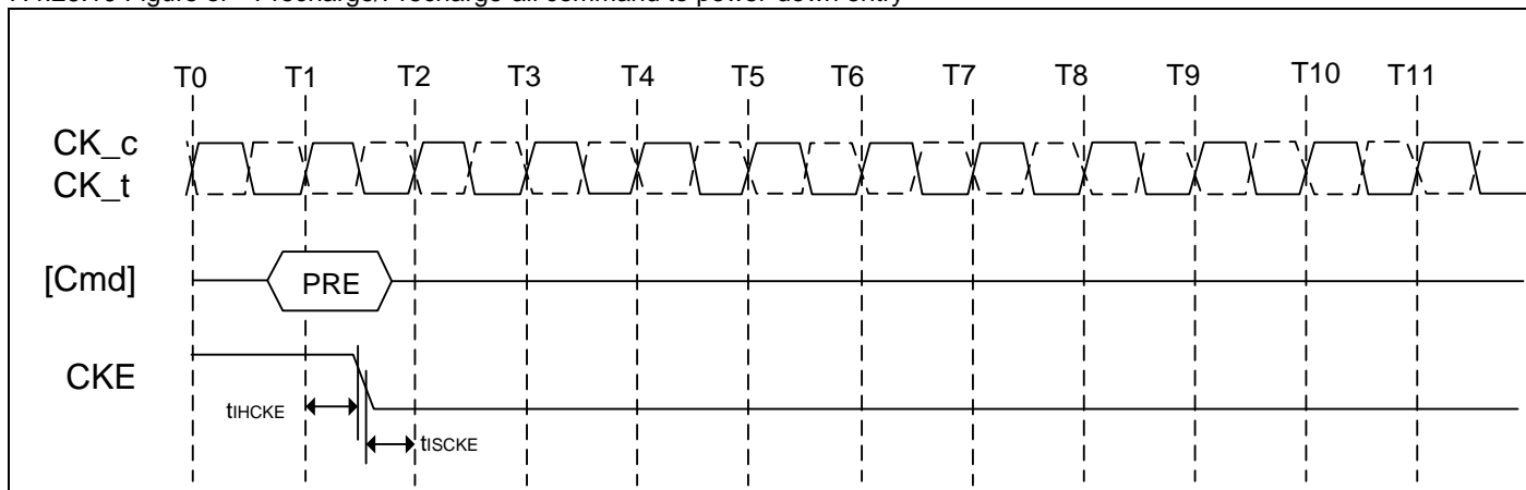
7.4.26.10 Figure of Precharge/Precharge-all command to power-down entry
