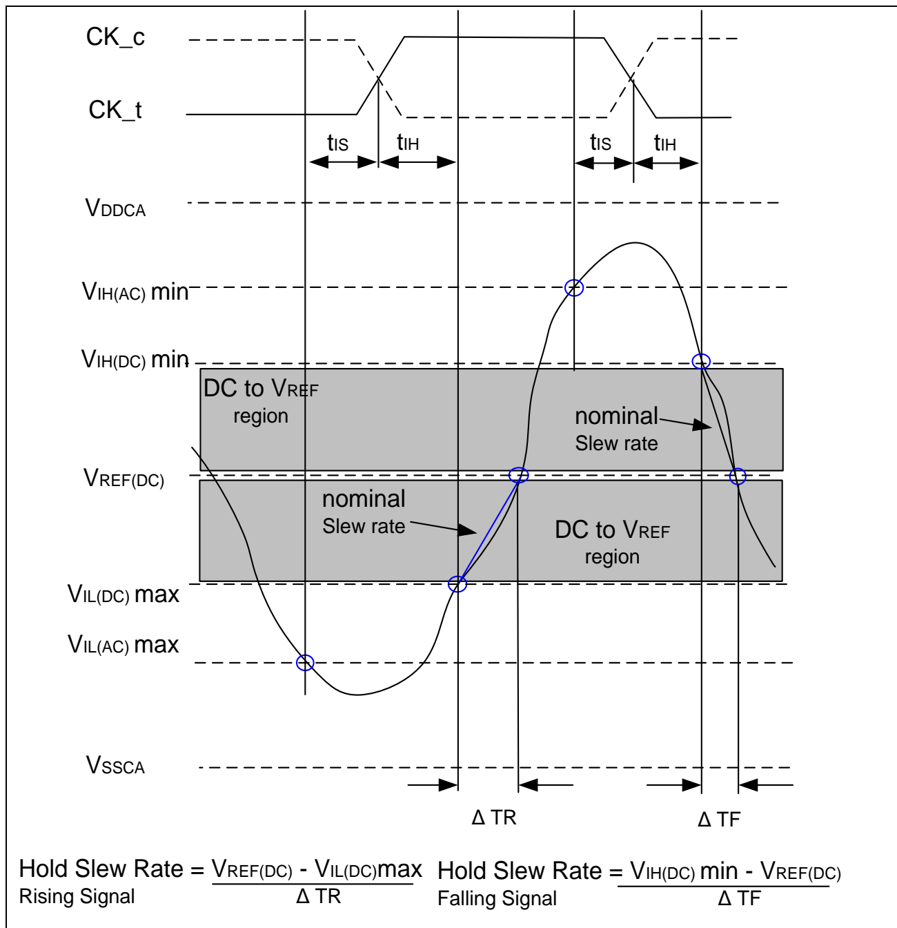
8.6.2.6 Figure of nominal slew rate for hold time tIH for CA and CS_n with respect to clock
