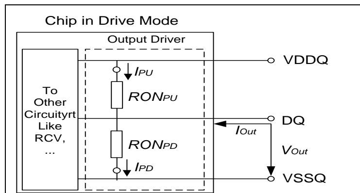
Figure of Output Driver Definition of Voltages and Currents
