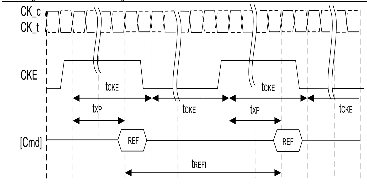
7.4.26.3 Figure of Refresh to Refresh timing with CKE intensive environment for LPDDR2 SDRAM
