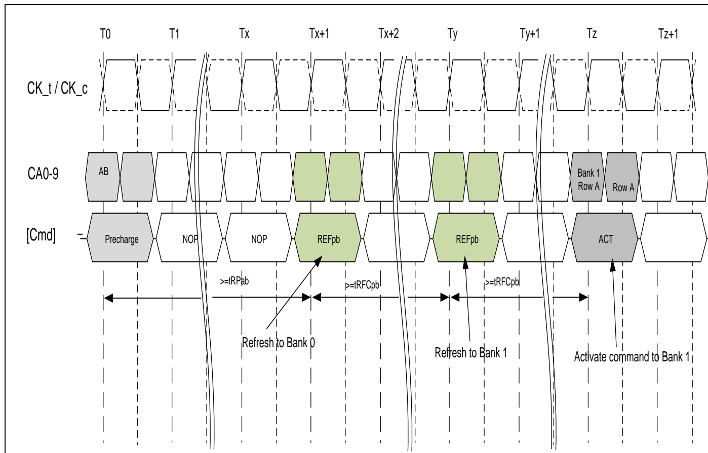
7.4.16.7 Figure of LPDDR2-S4 Per Bank Refresh Operation
