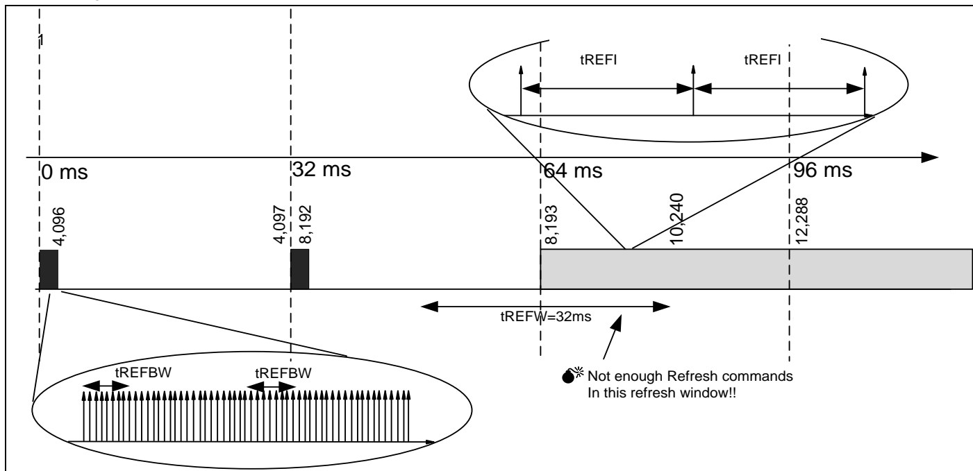
7.4.16.4 Figure of LPDDR2-S4: NOT-Allowable Transition from Repetitive Burst Refresh with Subsequent Refresh Pause to Regular, Distributed Refresh Pattern
