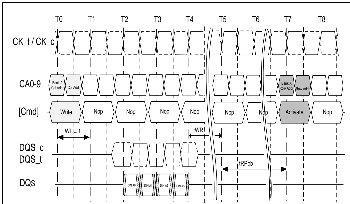
7.4.14.1 Figure of LPDDR2-S4 : Burst write w/Auto precharge : WL = 1, BL= 4
