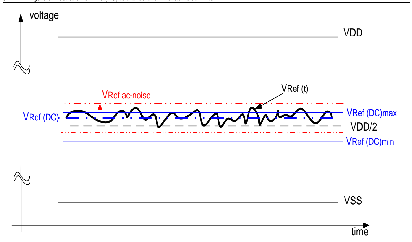
8.2.4.2.1 Figure of Illustration of VRef(DC) tolerance and VRef ac-noise limits
