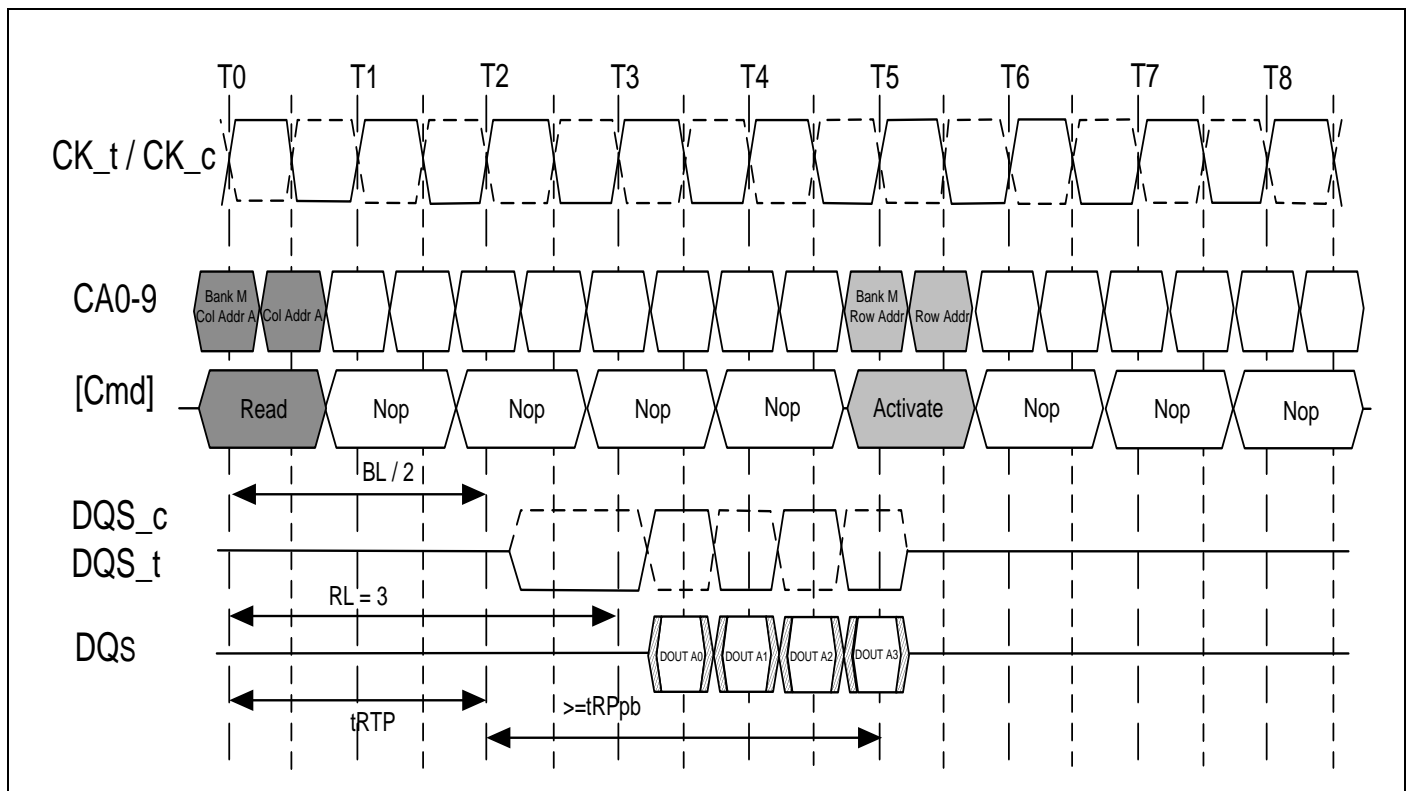
7.4.13.1 Figure of LPDDR2-S4 : Burst read with Auto-Precharge : RL= 3, BL=4, RU(tRTP(min)/tCK)=2
