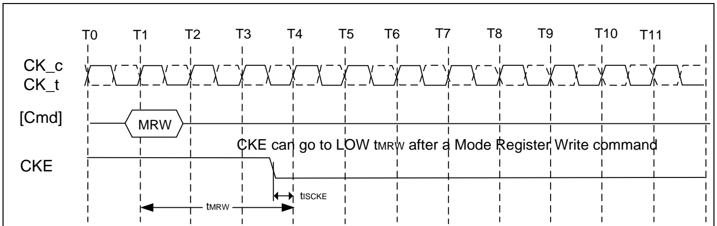
7.4.26.12 Figure of MRW command to power-down entry
