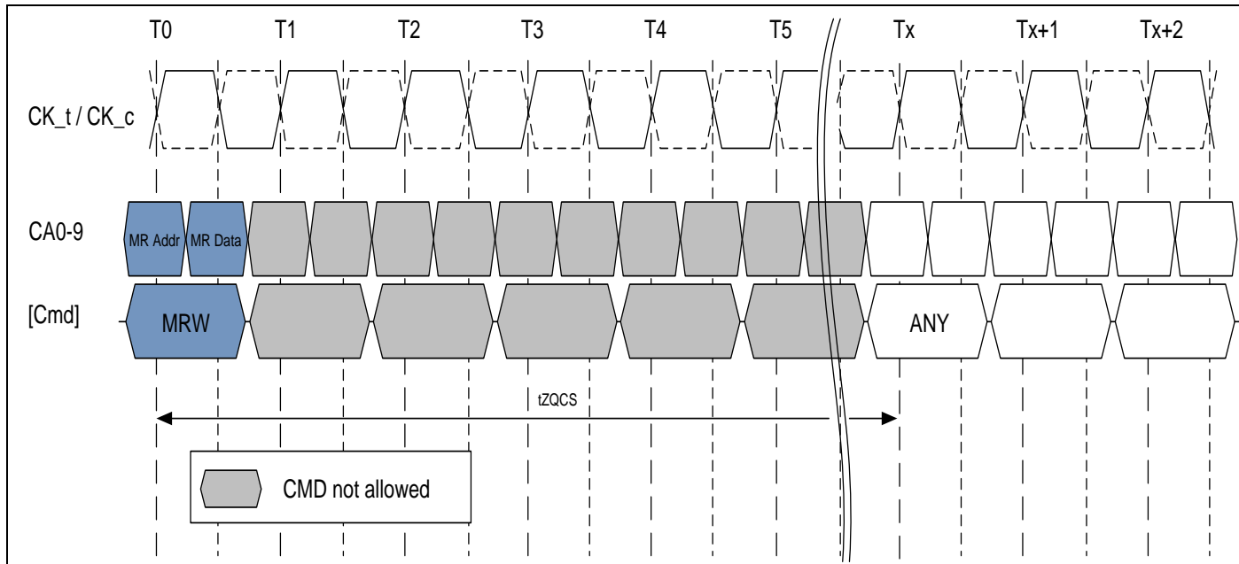
7.4.24.2 Figure of ZQ Calibration Short timing example
