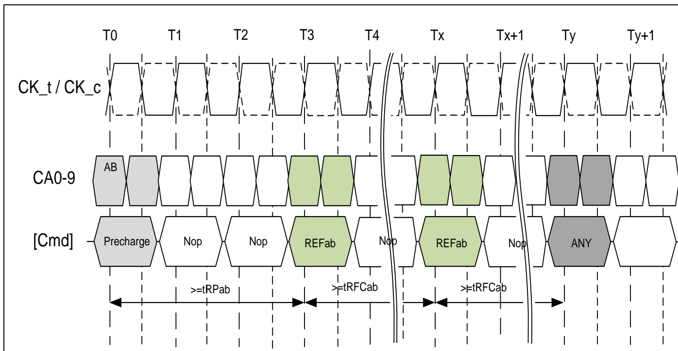
7.4.16.6 Figure of LPDDR2-S4 All Bank Refresh Operation
