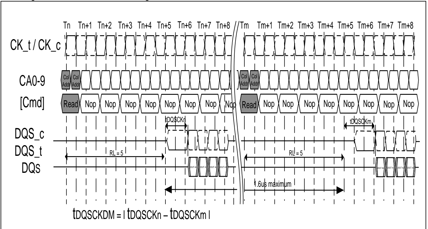
7.4.3.6 Figure of LPDDR2: tDQSKDM timing
