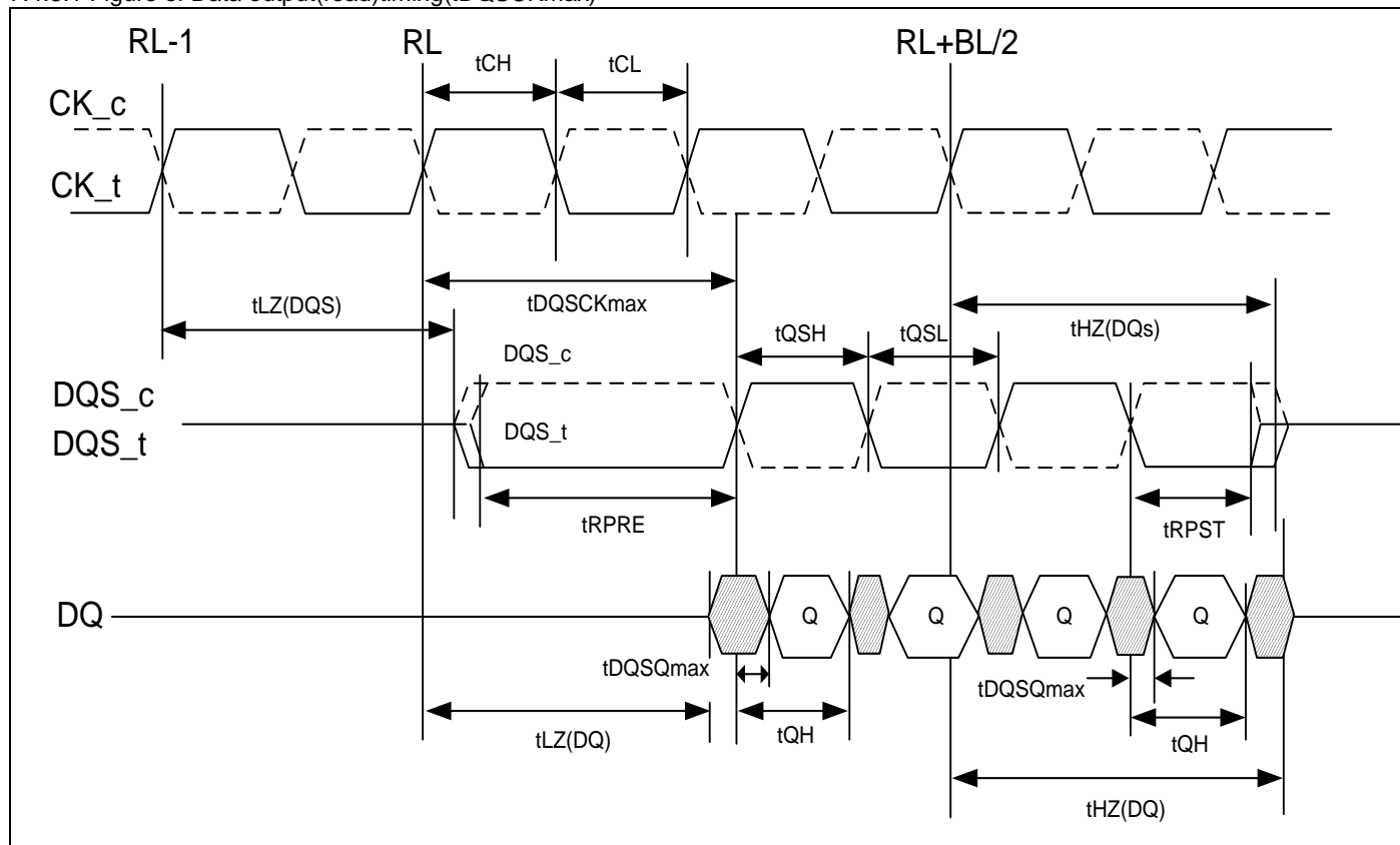
7.4.3.1 Figure of Data output(read)timing(tDQCKmax)
