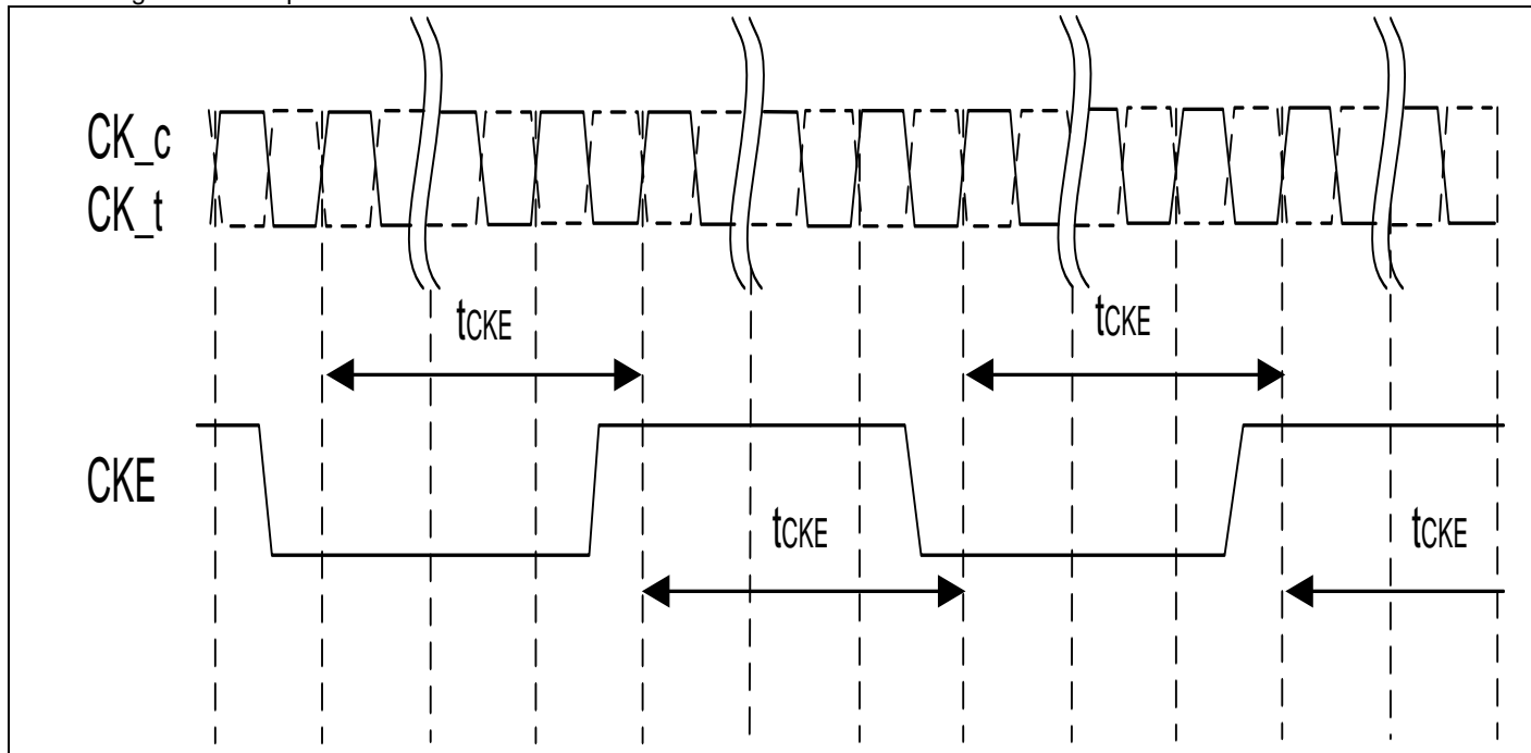
7.4.26.2 Figure of Example of CKE intensive environment
