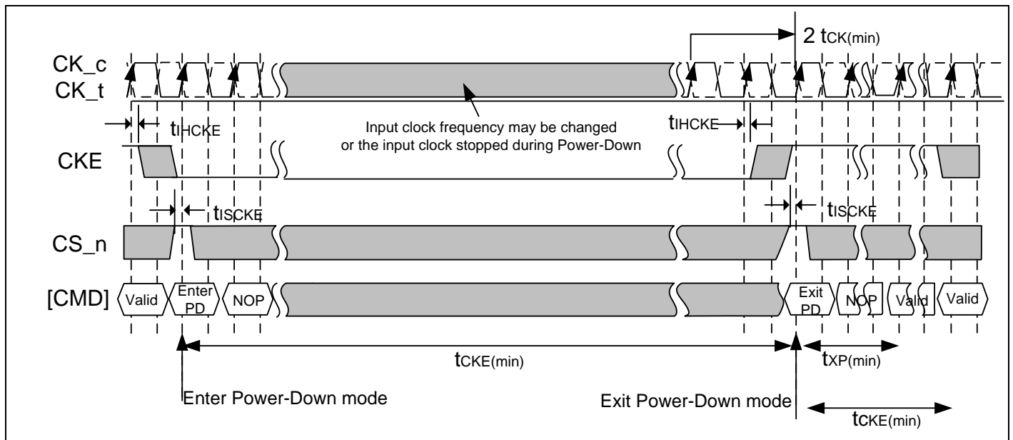
7.4.26.1 Figure of LPDDR2-S4 : Basic power down entry and exit timing diagram
