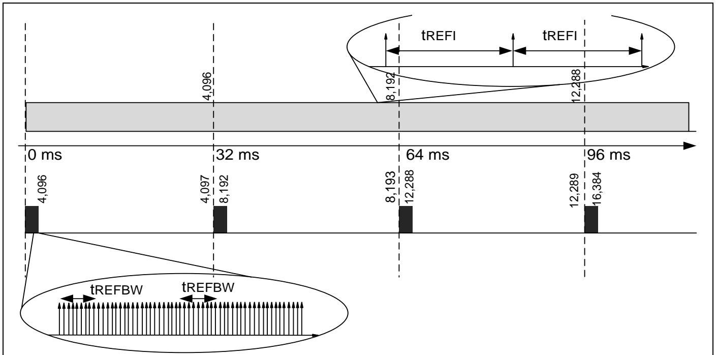
7.4.16.2 Figure of LPDDR2-S4 Regular, Distributed Refresh Pattern vs. Repetitive Burst Refresh with Subsequent Refresh Pause
