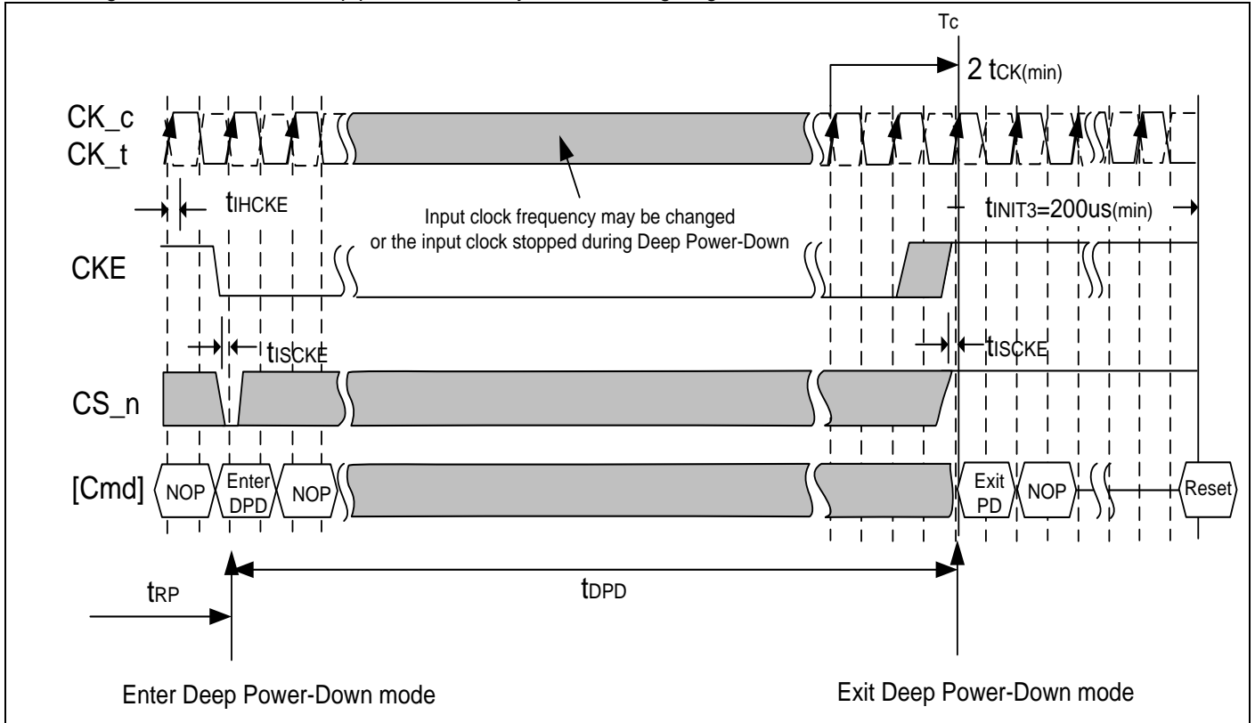
7.4.27.1 Figure of LPDDR2-S4 Deep power down entry and exit timing diagram
