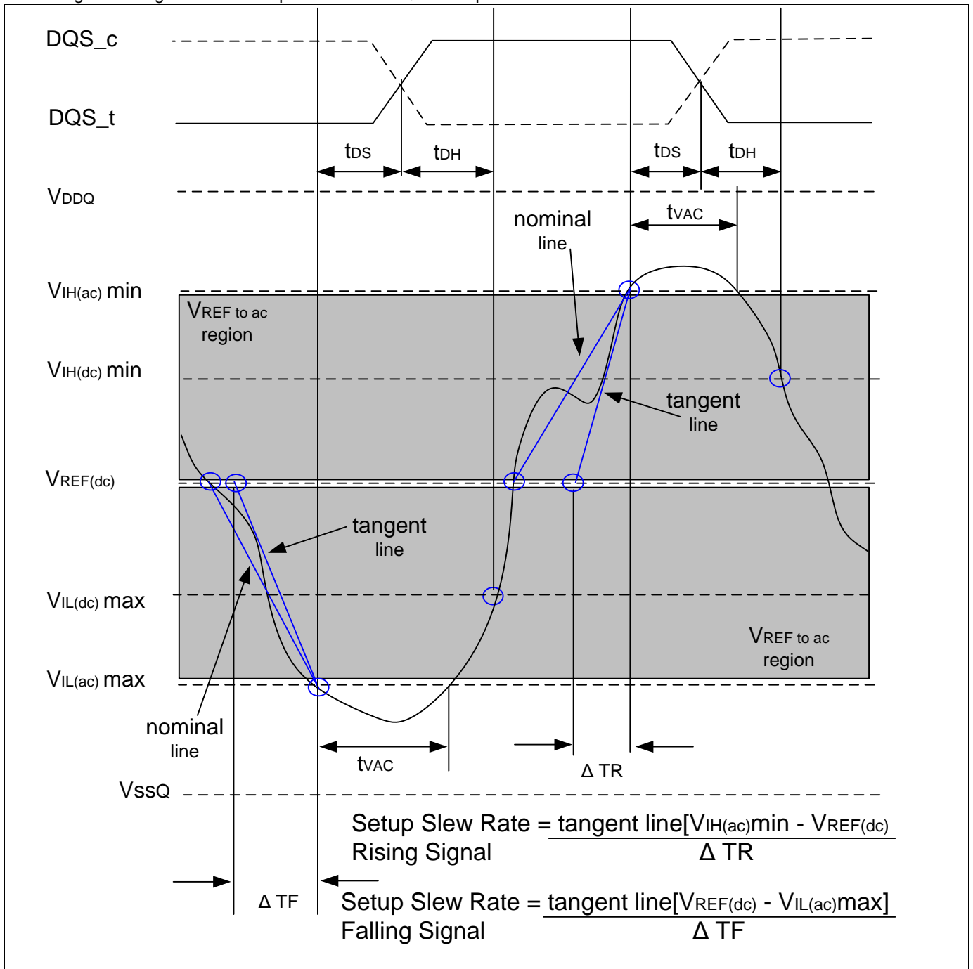
8.6.3.7 Figure of tangent line for setup time tDS for DQ with respect to strobe
