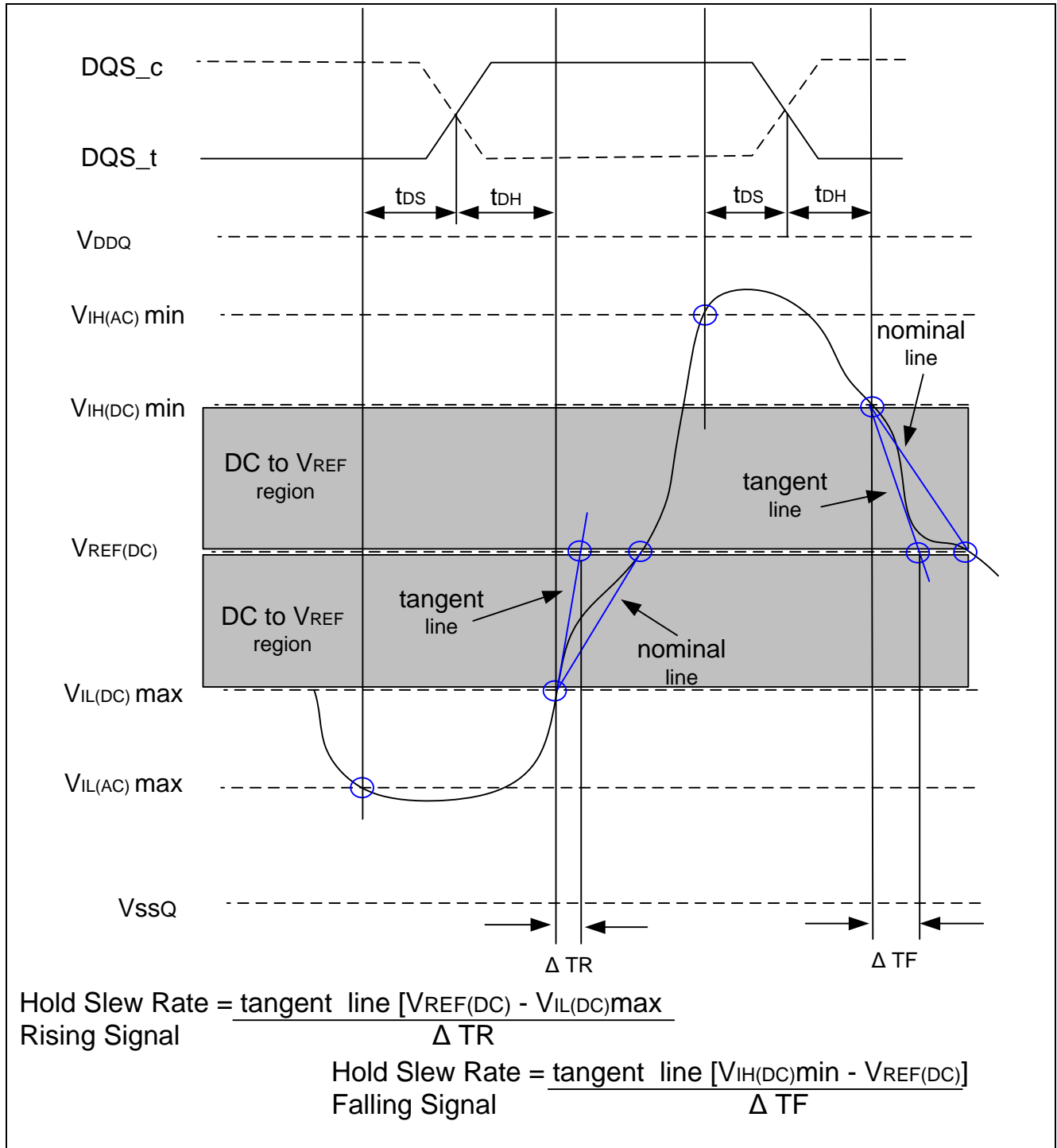
8.6.3.8 Figure of tangent line for for hold time t DH for DQ with respect to strobe
