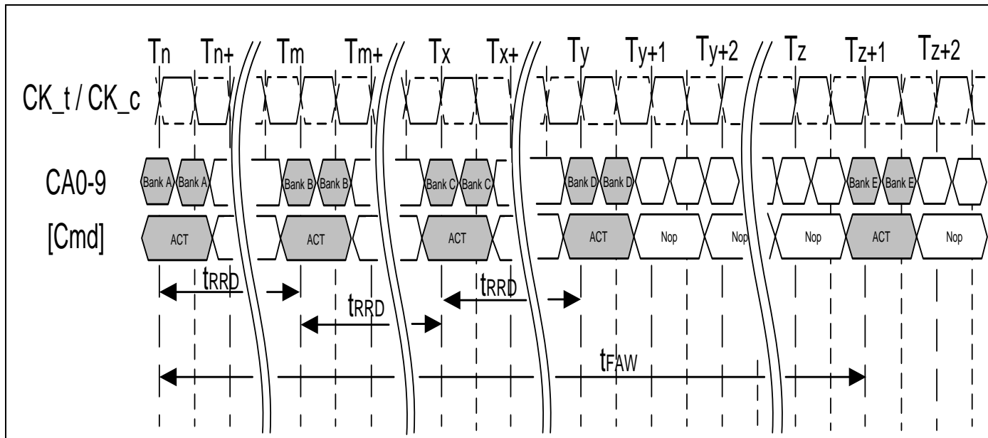
7.4.1.2 Figure of LPDDR2-S4: tFAW timing
