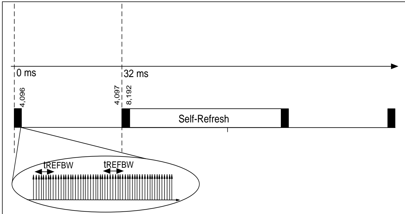
7.4.16.5 Figure of LPDDR2-S4: Recommended Self-refresh entry and exit in conjunction with a Burst/Pause Refresh patterns.
