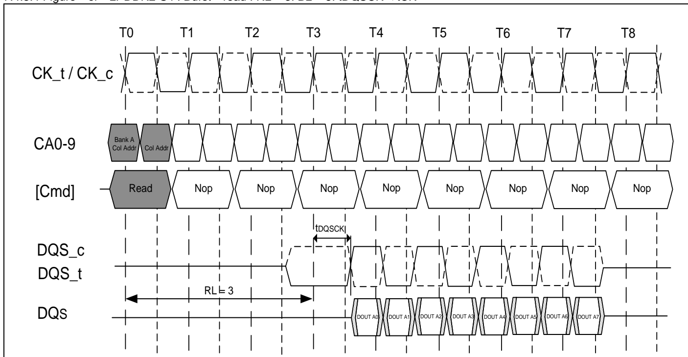
7.4.3.4 Figure of LPDDR2-S4 : Burst read : RL = 3. BL = 8. tDQSCK < tCK
