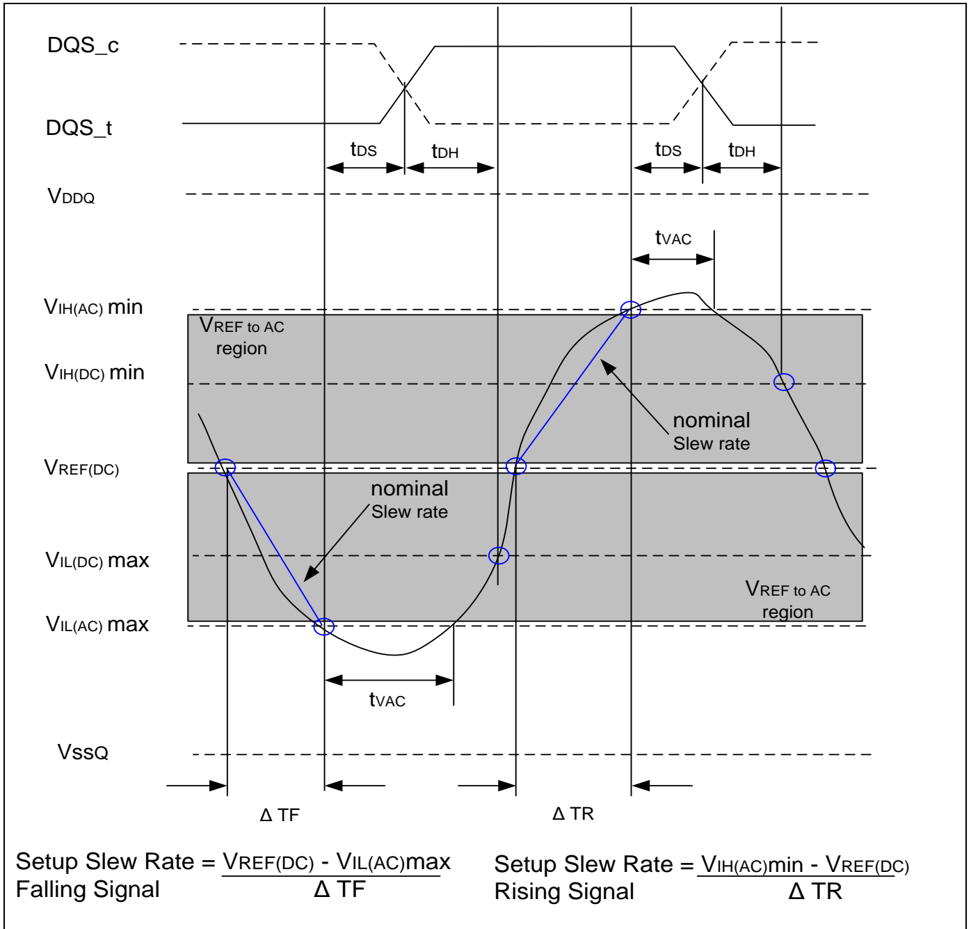
8.6.3.5 Figure of nominal slew rate and tVAC for setup time tDS for DQ with respect to strobe
