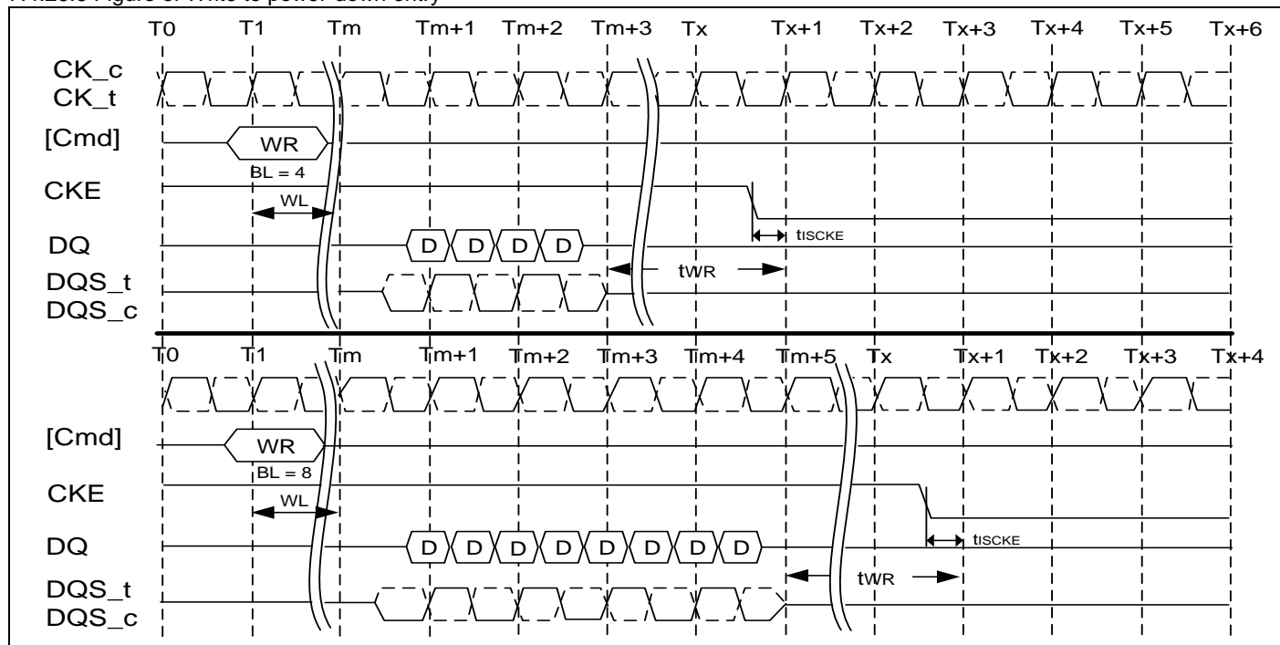
7.4.26.6 Figure of Write to power-down entry
