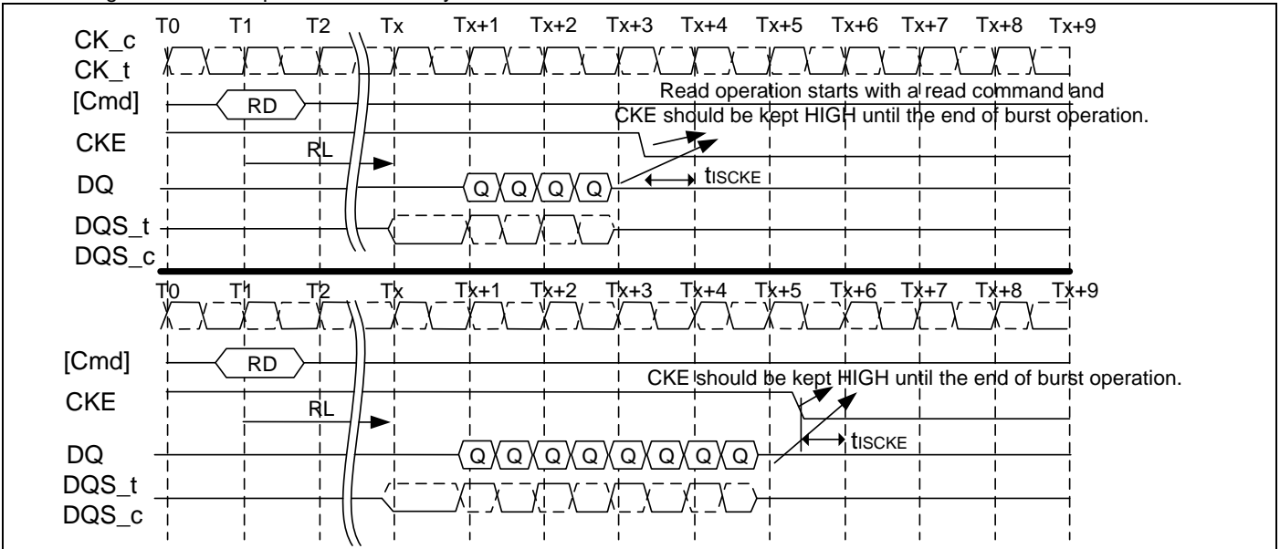
7.4.26.4 Figure of Read to power – down entry
