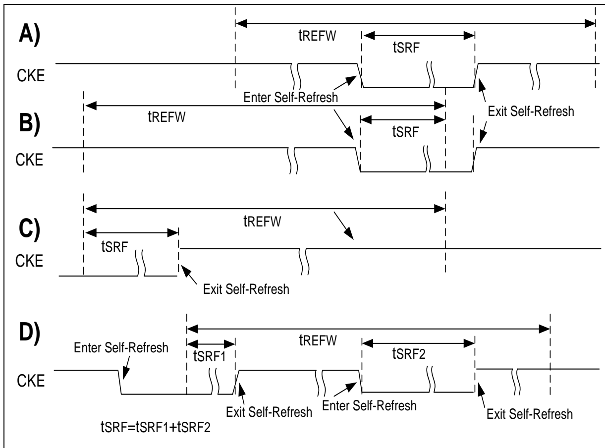
7.4.16.1 Figure of LPDDR2-S4 : Definition of tSRF
