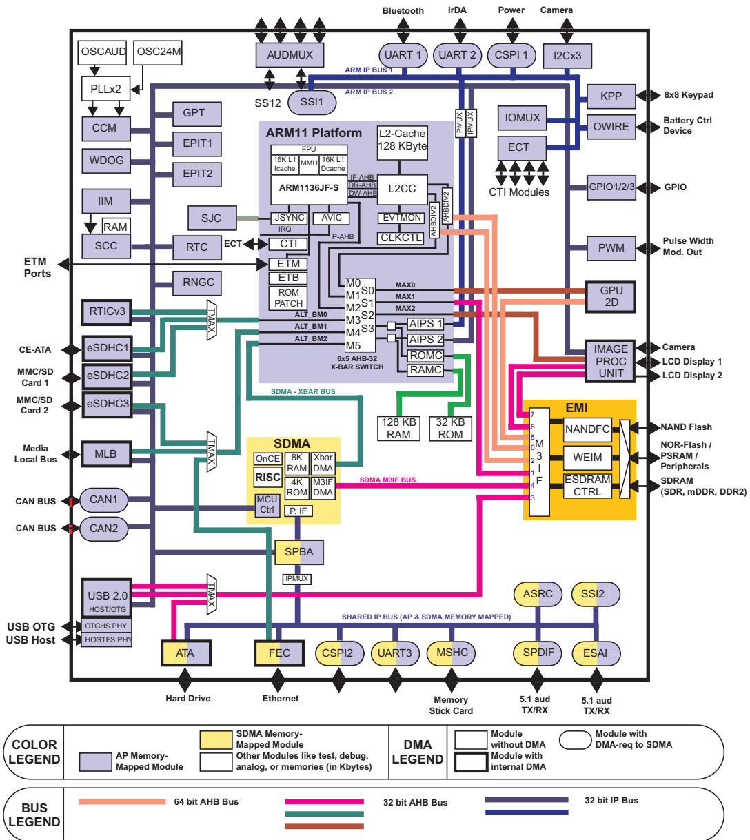
Figure 1-3. Ringo Detailed Block Diagram
