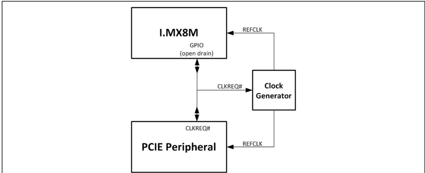
Figure 26. Connection diagram
