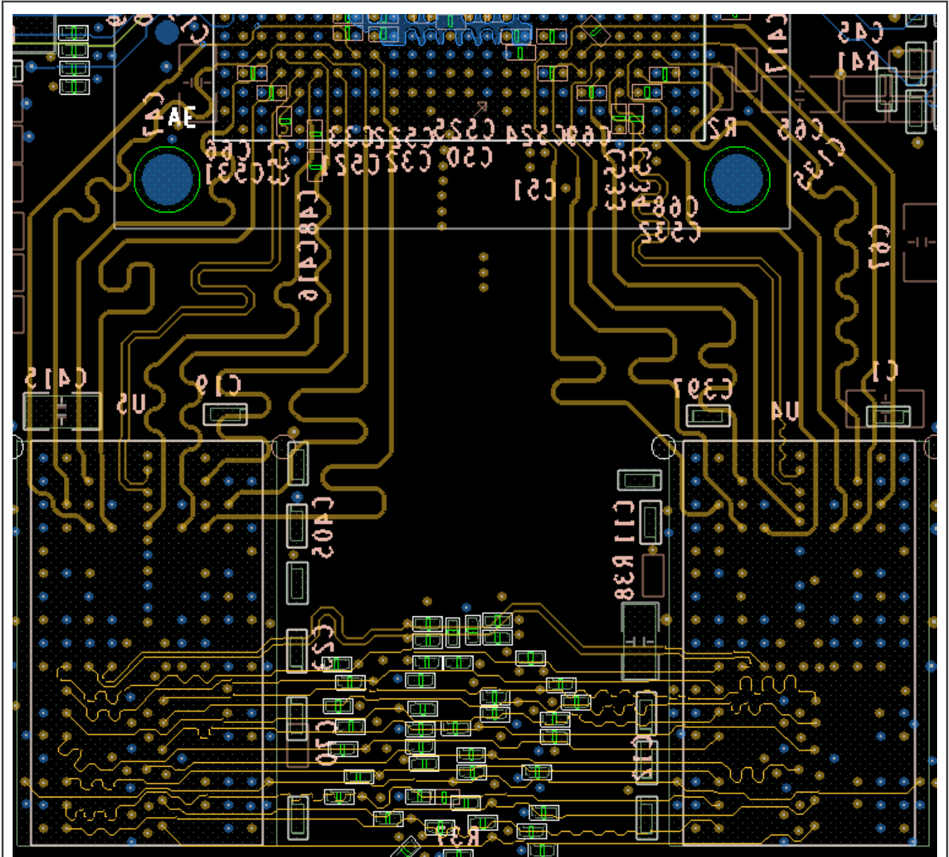
Figure 10. i.MX 8MDQLQ validation board DDR4 routing (Layer 3)
