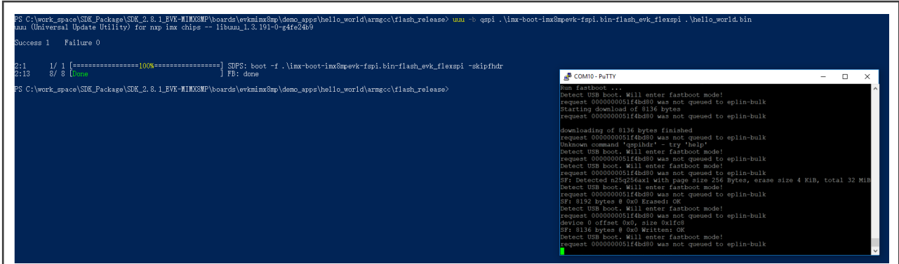
Figure 30. Command line and fast boot console output when executing UUU
