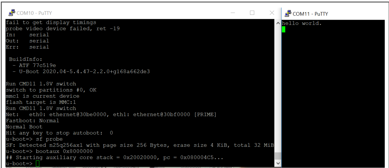
Figure 32. Console output from QSPI Boot
