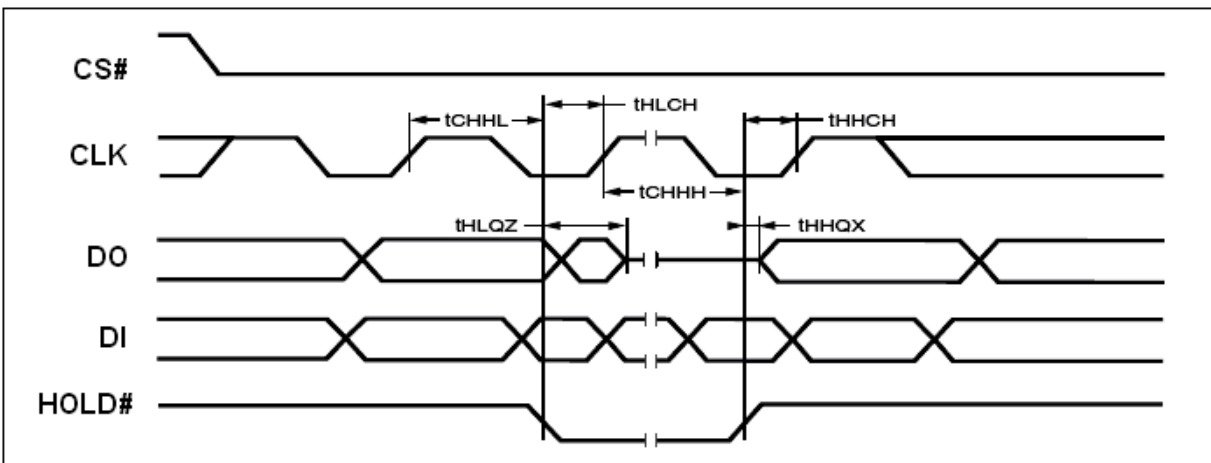
Figure 45. Hold Timing
