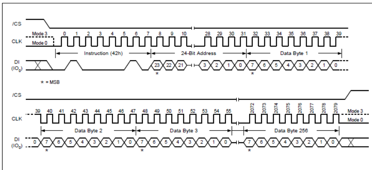
Figure 37. Program OTP array
