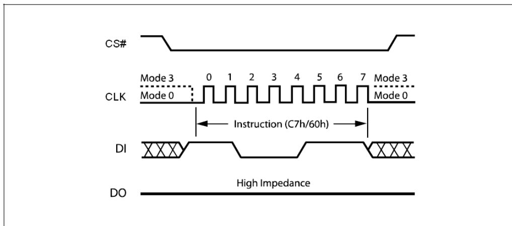
Figure 31. Chip Erase Instruction Sequence Diagram
