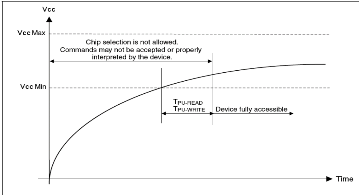
Figure 41. Power-up Timing
