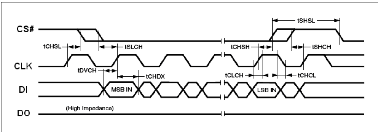
Figure 44. Input Timing
