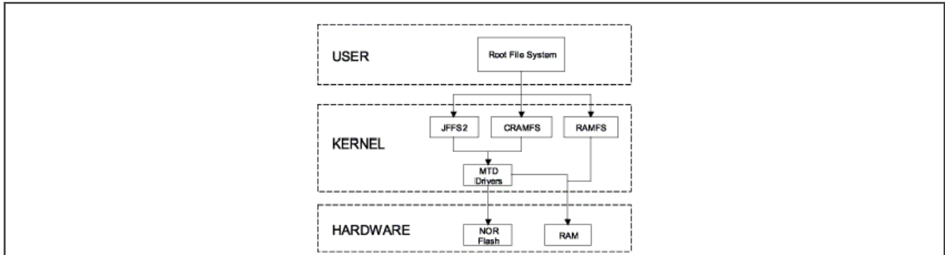
Figure 5. Components of a Flash-Based File System
