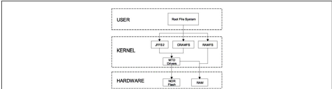
Figure 6. Components of a Flash-Based File System
