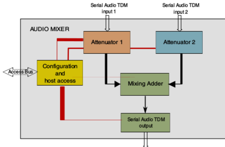
Figure 31. Audio Mixer block diagram
