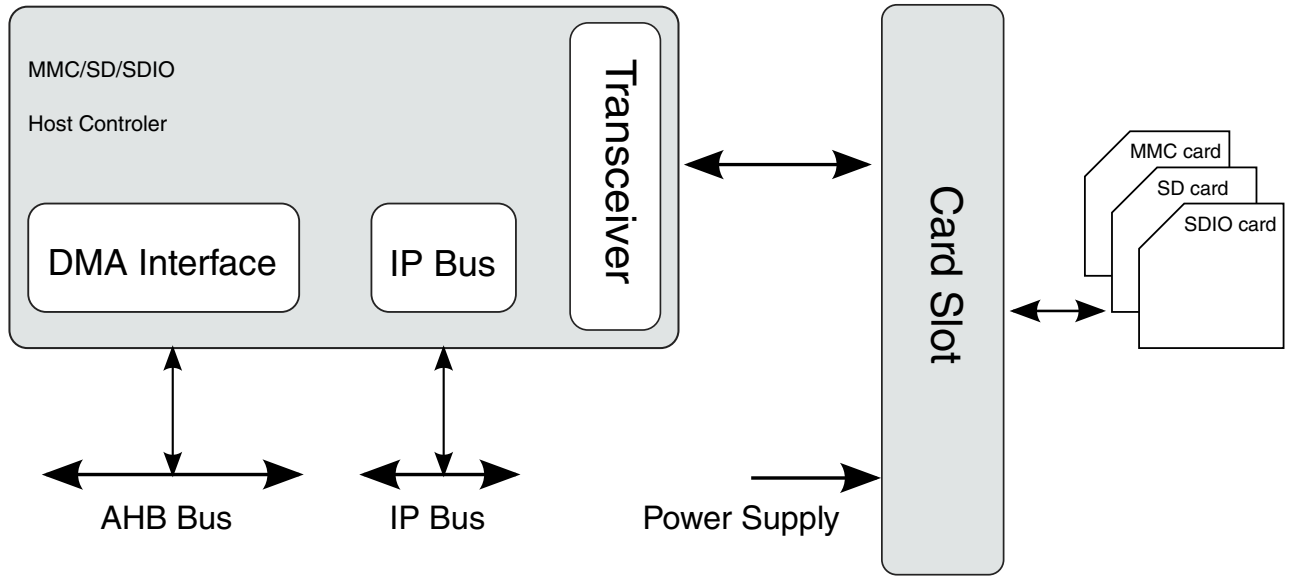
Figure 58-1. System Connection of the uSDHC
