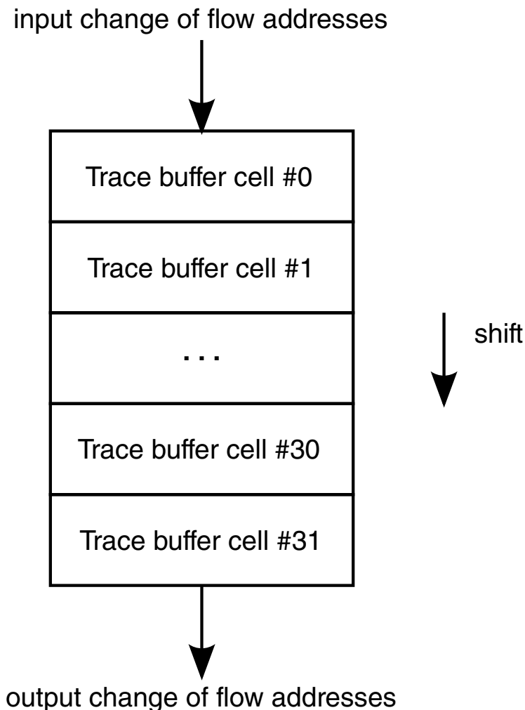
Figure 46-15. Trace Buffer
