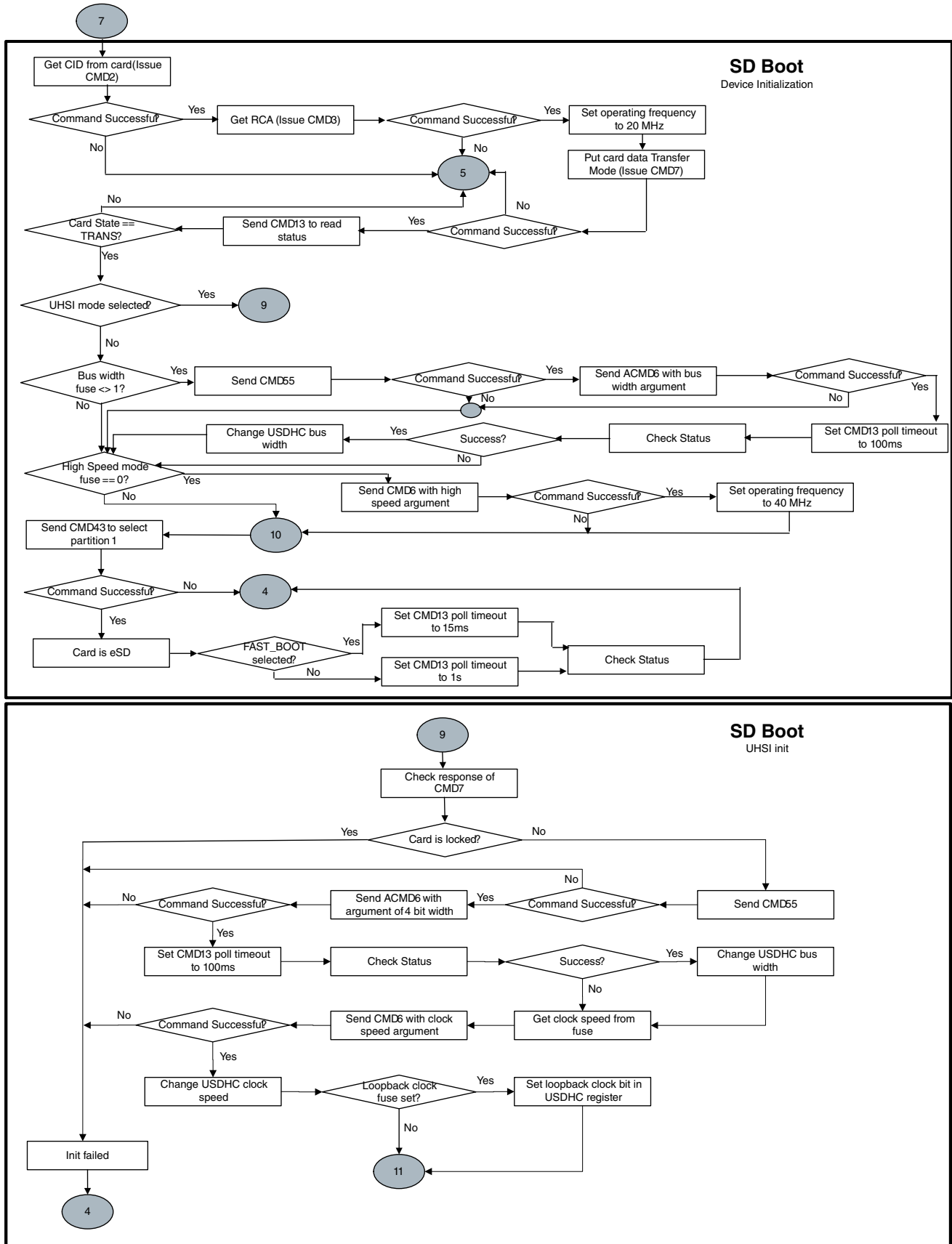
Figure 8-15. Expansion device (MMCSD/eSD/SDXC) boot flow (4 of 6) i.MX 6ULL Applications Processor Reference Manual, Rev. 1, 11/2017
