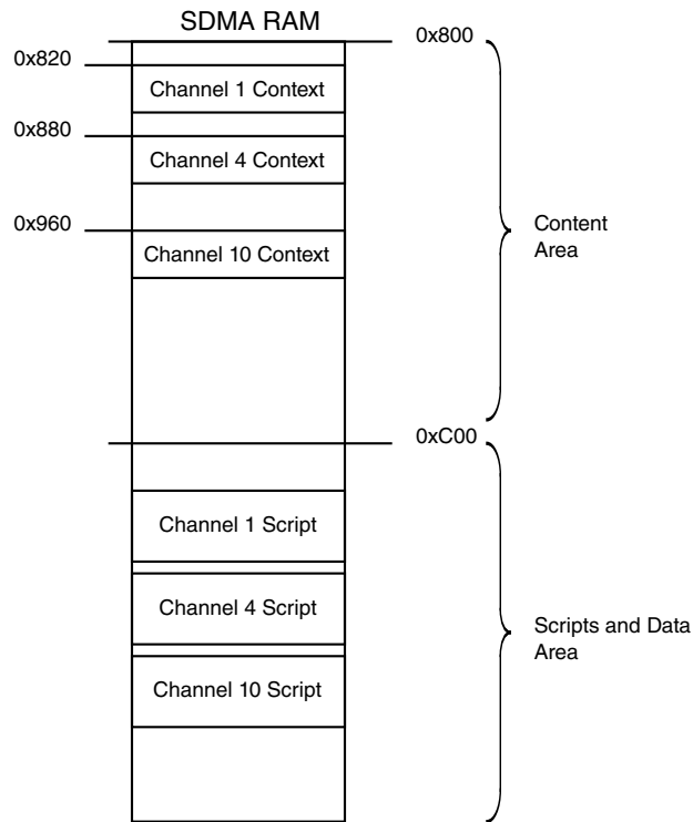
Figure 46-18. Example of SDMA RAM After Boot Session
