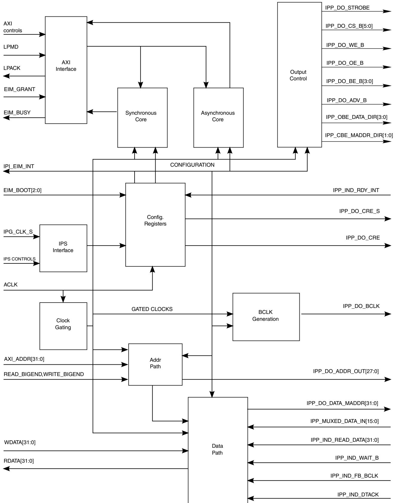
Figure 21-1. EIM Diagram
