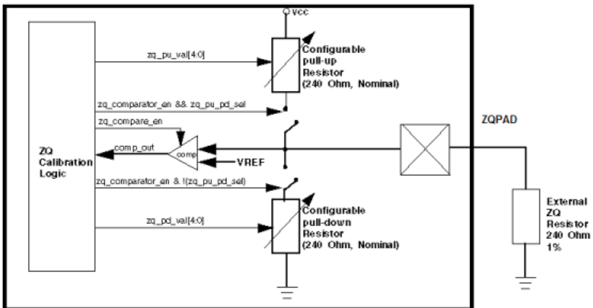
Figure 35-8. MMDC ZQ IF with PAD
