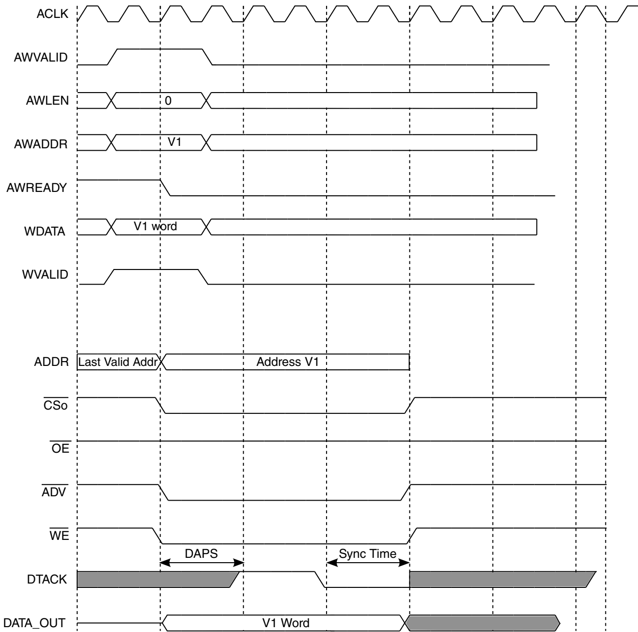
Figure 21-18. DAPS = 2
