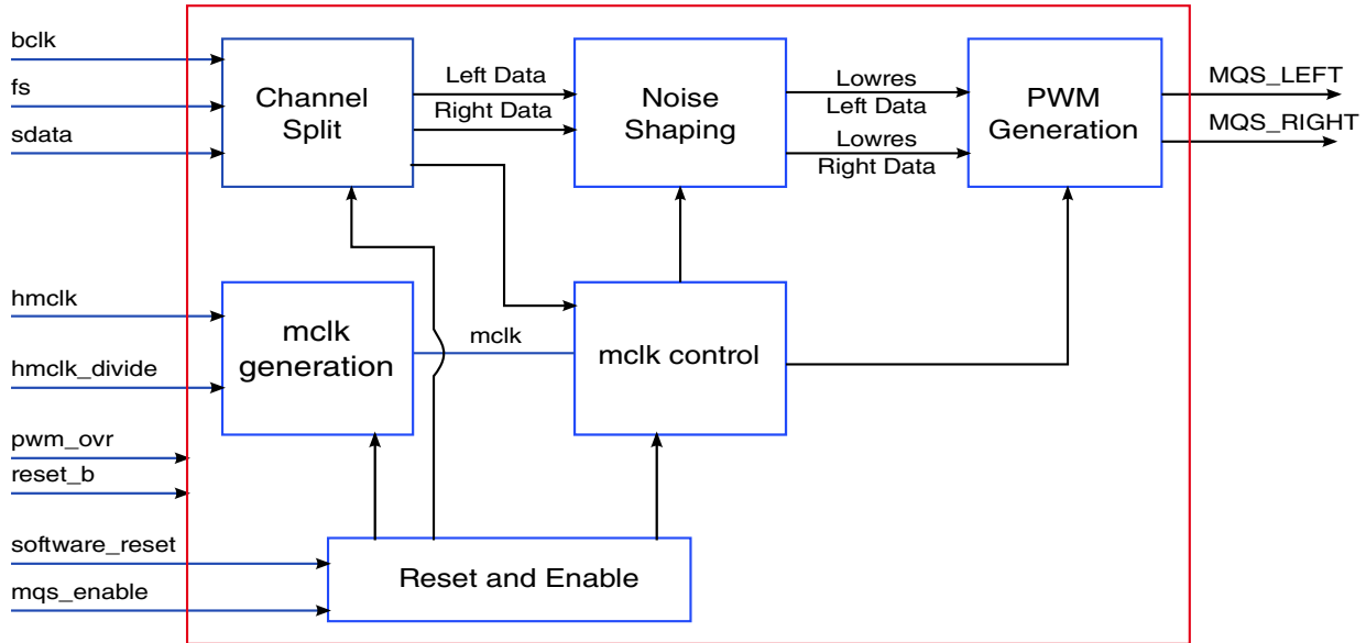
Figure 36-1. Block Diagram
