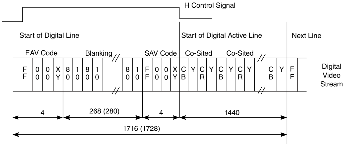
Figure 34-15. Digital Video Interface
