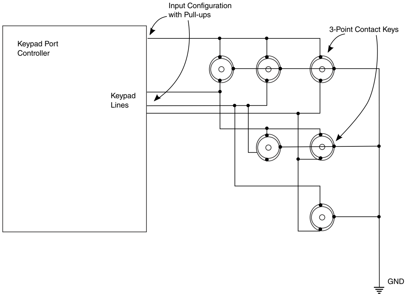
Figure 33-7. KPP Interface with 3-point Contact Key Matrix (Simplified View)
