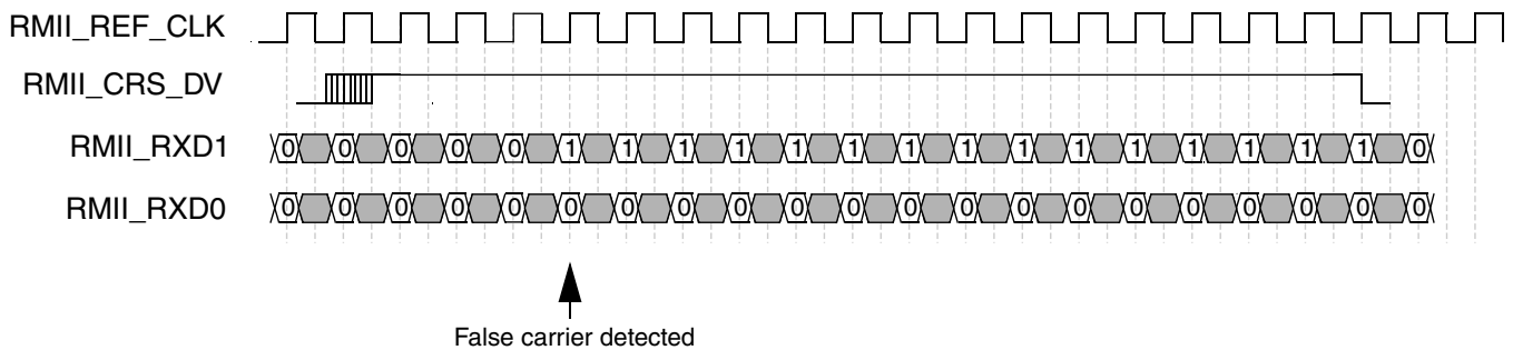
Figure 22-20. RMII receive operation with false carrier
