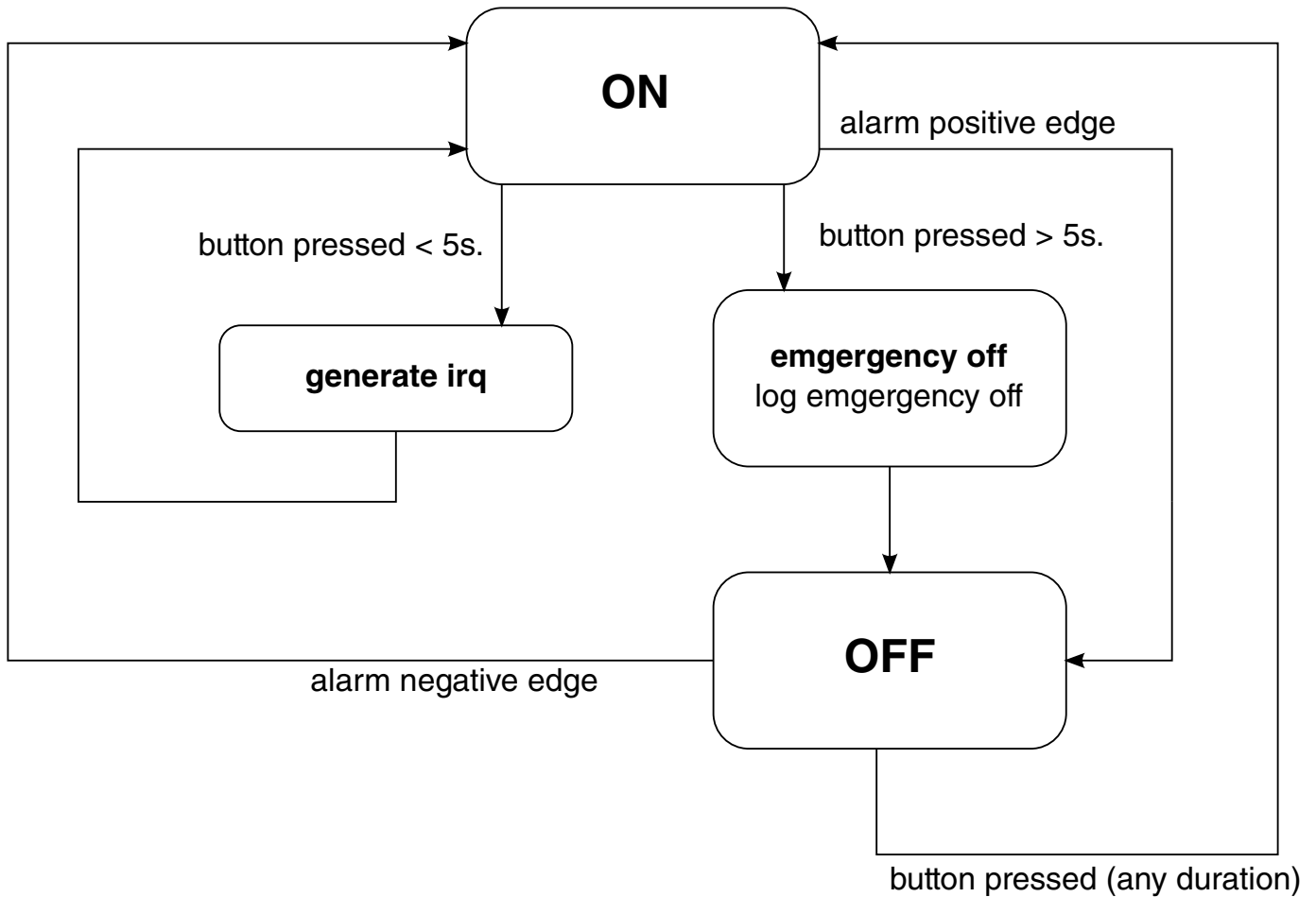
Figure 51-4. FSM
