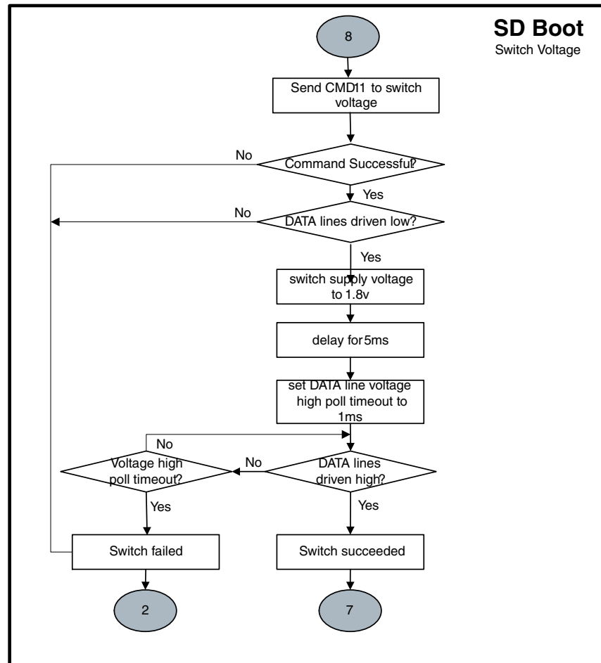
Figure 8-14. Expansion device (SD/eSD/SDXC) boot flow (3 of 6) part 2
