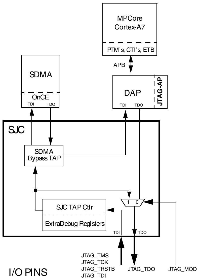
Figure 47-1. System JTAG Controller (SJC) Block Diagram
