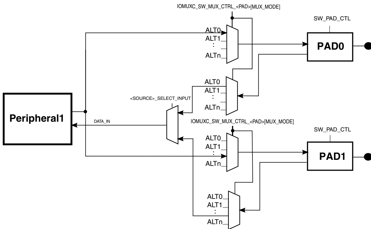
Figure 32-2. IOMUX Cell Block Diagram
