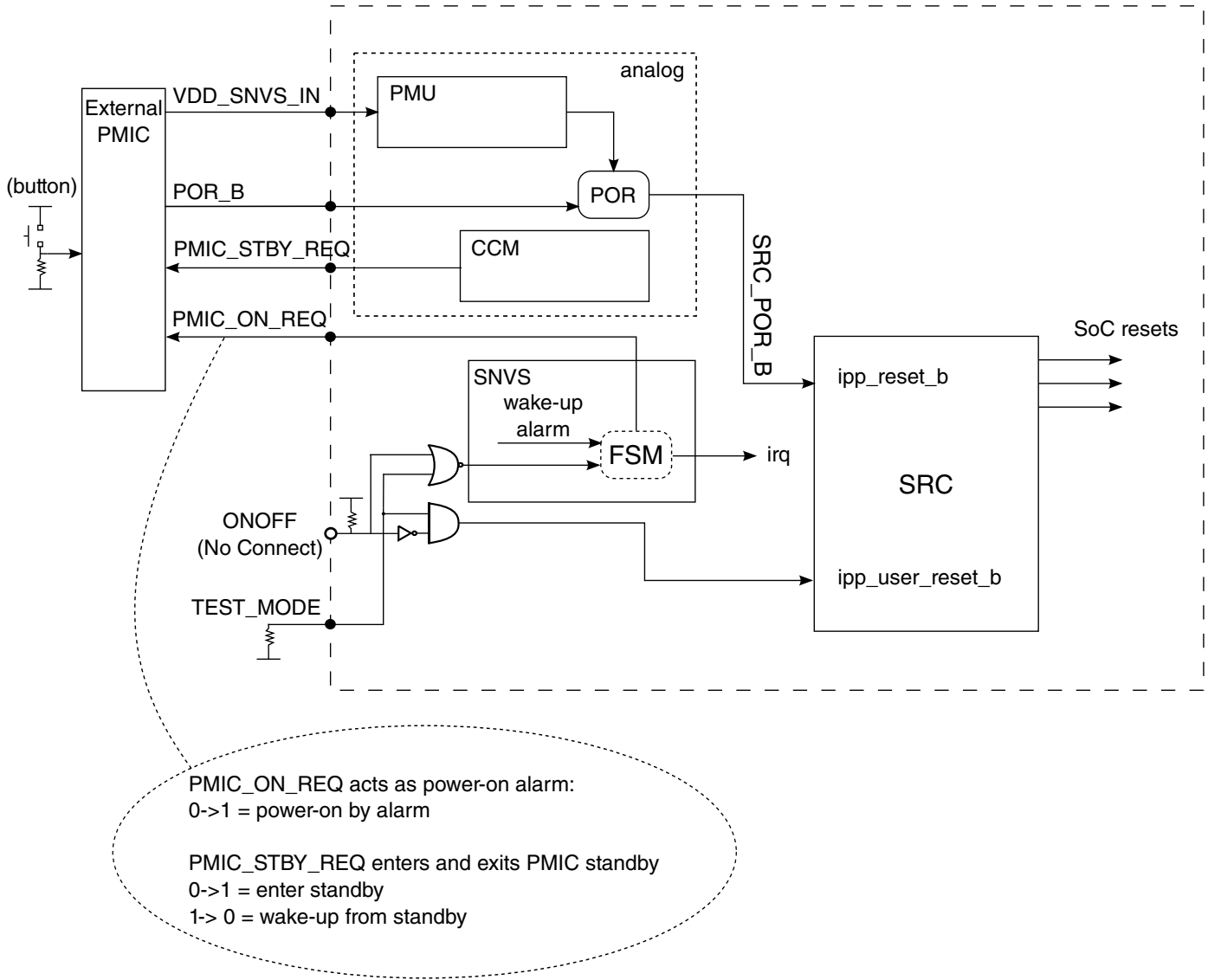
Figure 51-2. Chip reset scheme under external PMIC control
