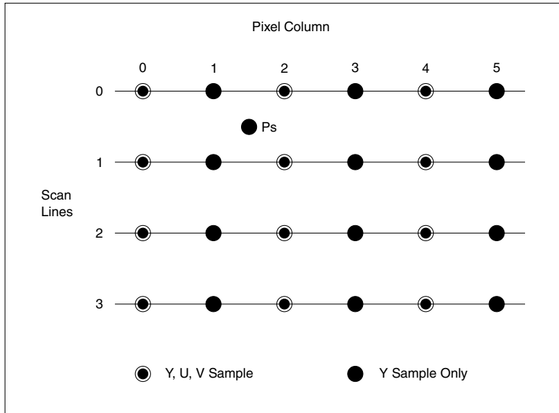
Figure 41-6. YUV Sample Positioning, 4:2:2
