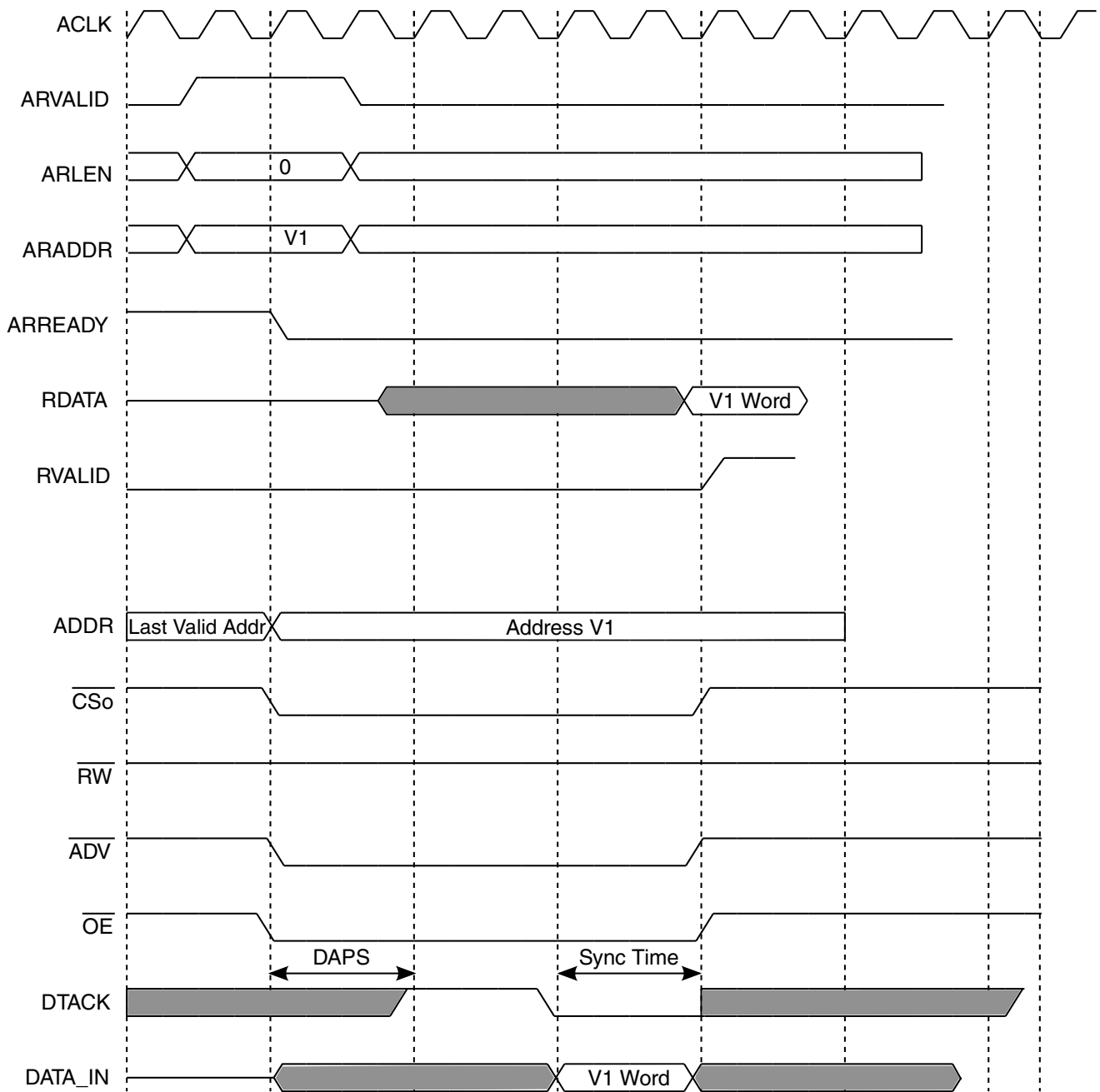
Figure 21-15. DAPS = 2
