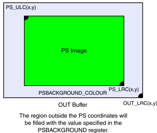
Figure 41-21. OUT Buffer
