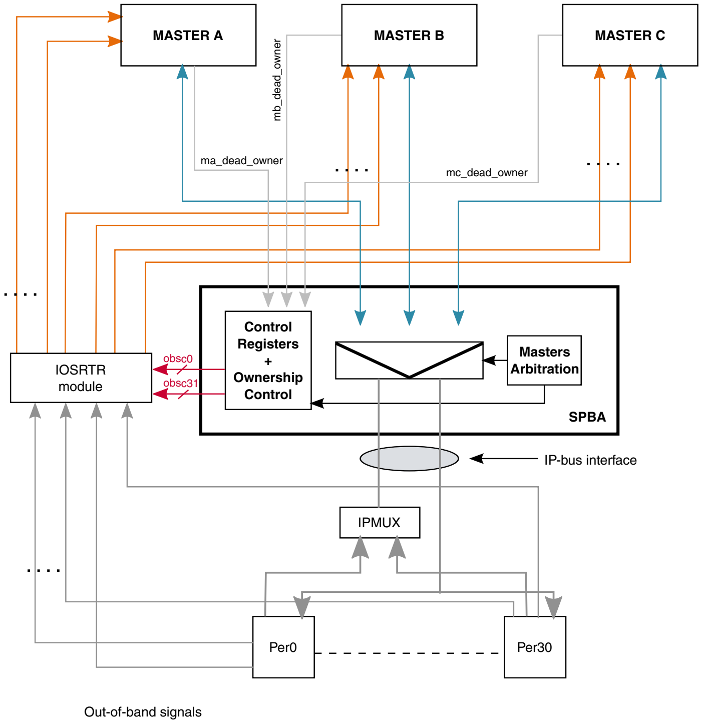
Figure 49-1. SPBA Block Diagram
