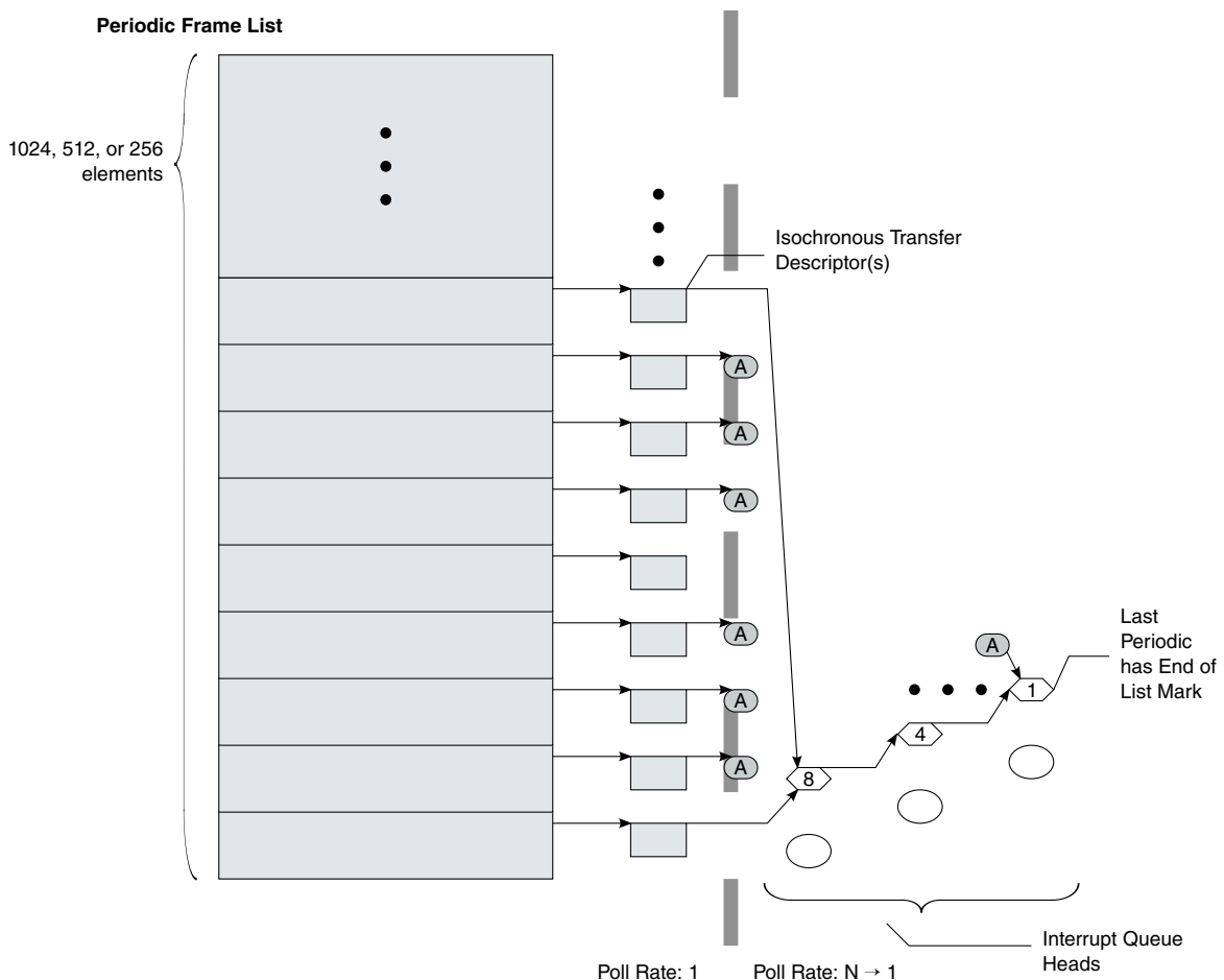
Figure 56-11. Example Periodic Schedule
