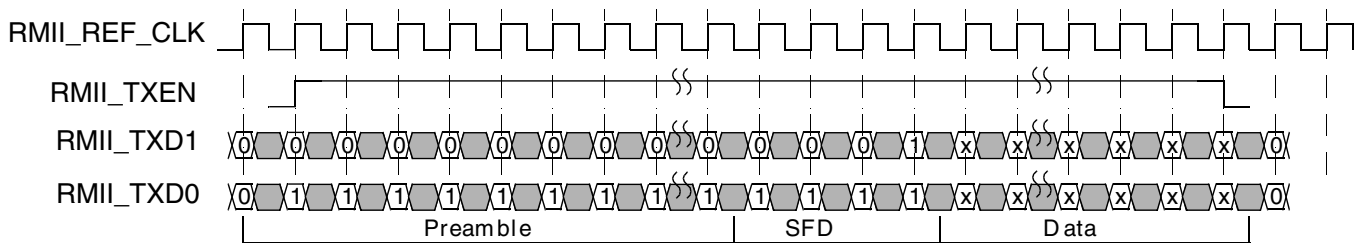
Figure 22-21. RMII transmit operation
