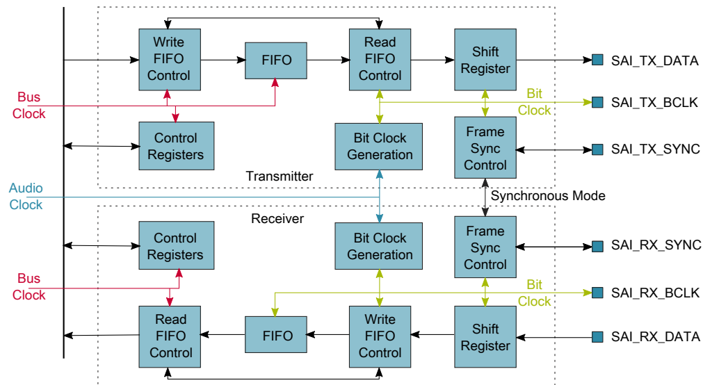
Figure 45-1. I 2 S/SAI block diagram
