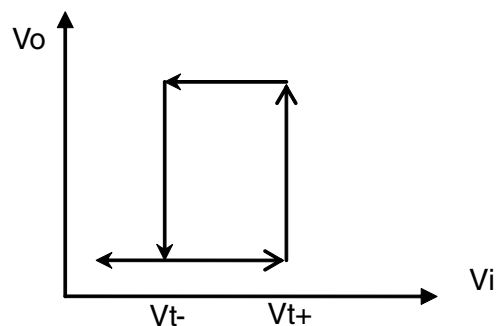
Figure 28-4. Schmitt trigger transfer characteristic
