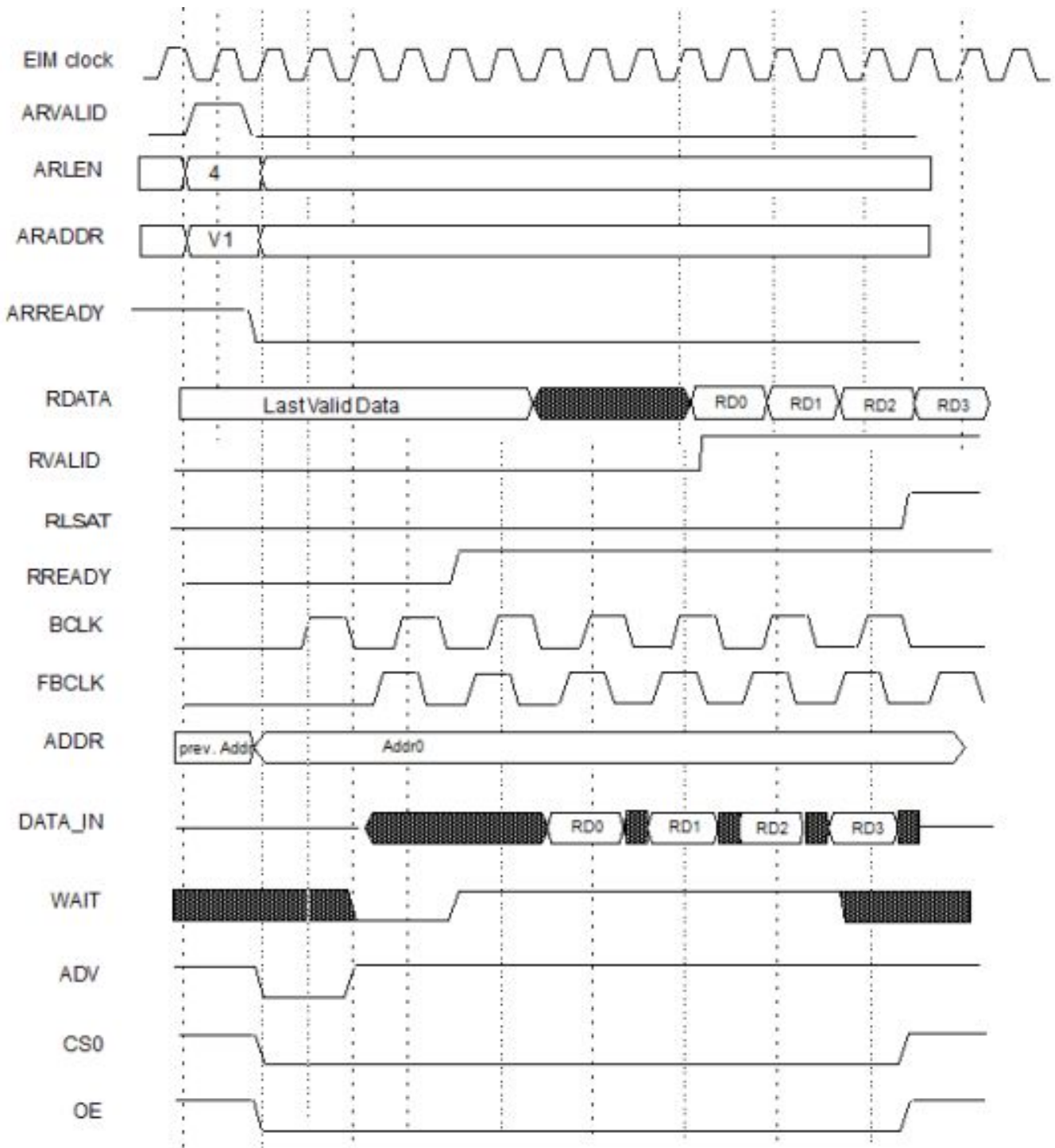
Figure 21-13. BCD=1, RL = 3
