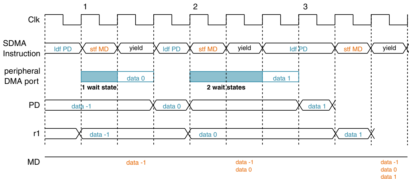
Figure 46-21. Peripheral to External Memory Example (1)
