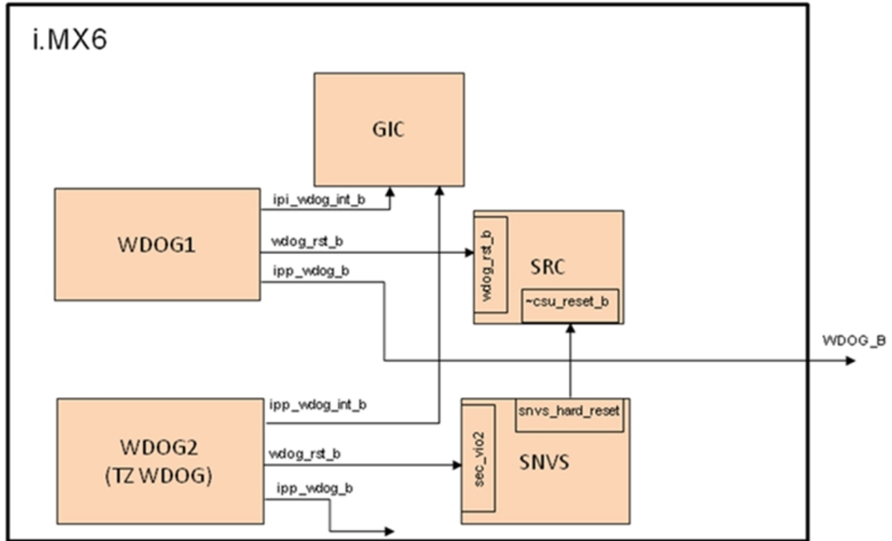
Figure 59-2. System integration
