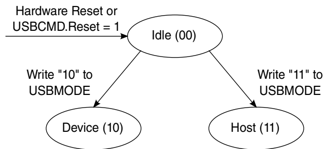
Figure 56-1. Controller Mode
