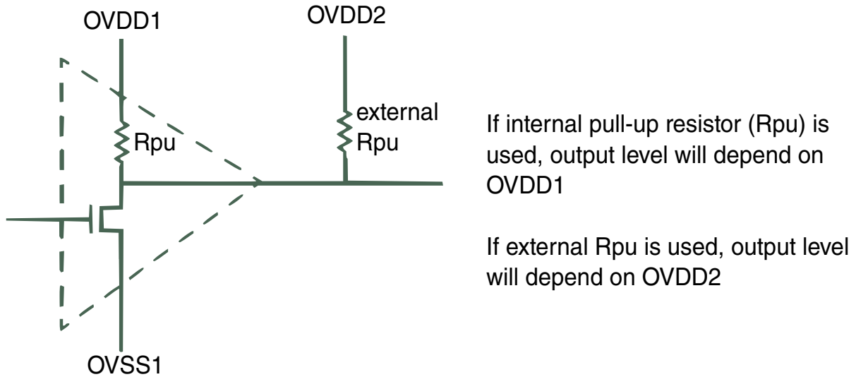
Figure 28-8. Output buffer in open drain mode
