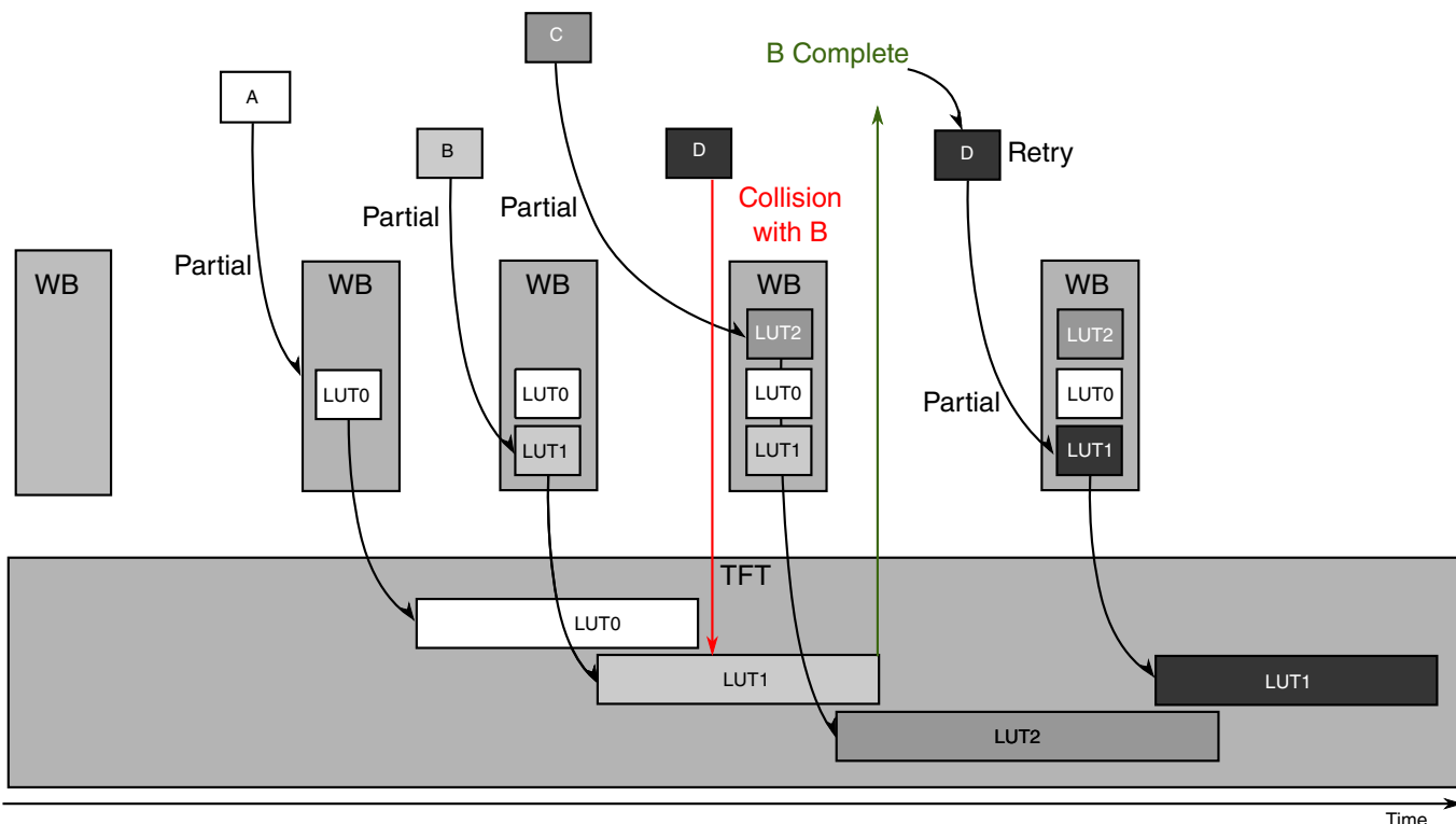
Figure 23-9. Collision Sequence
