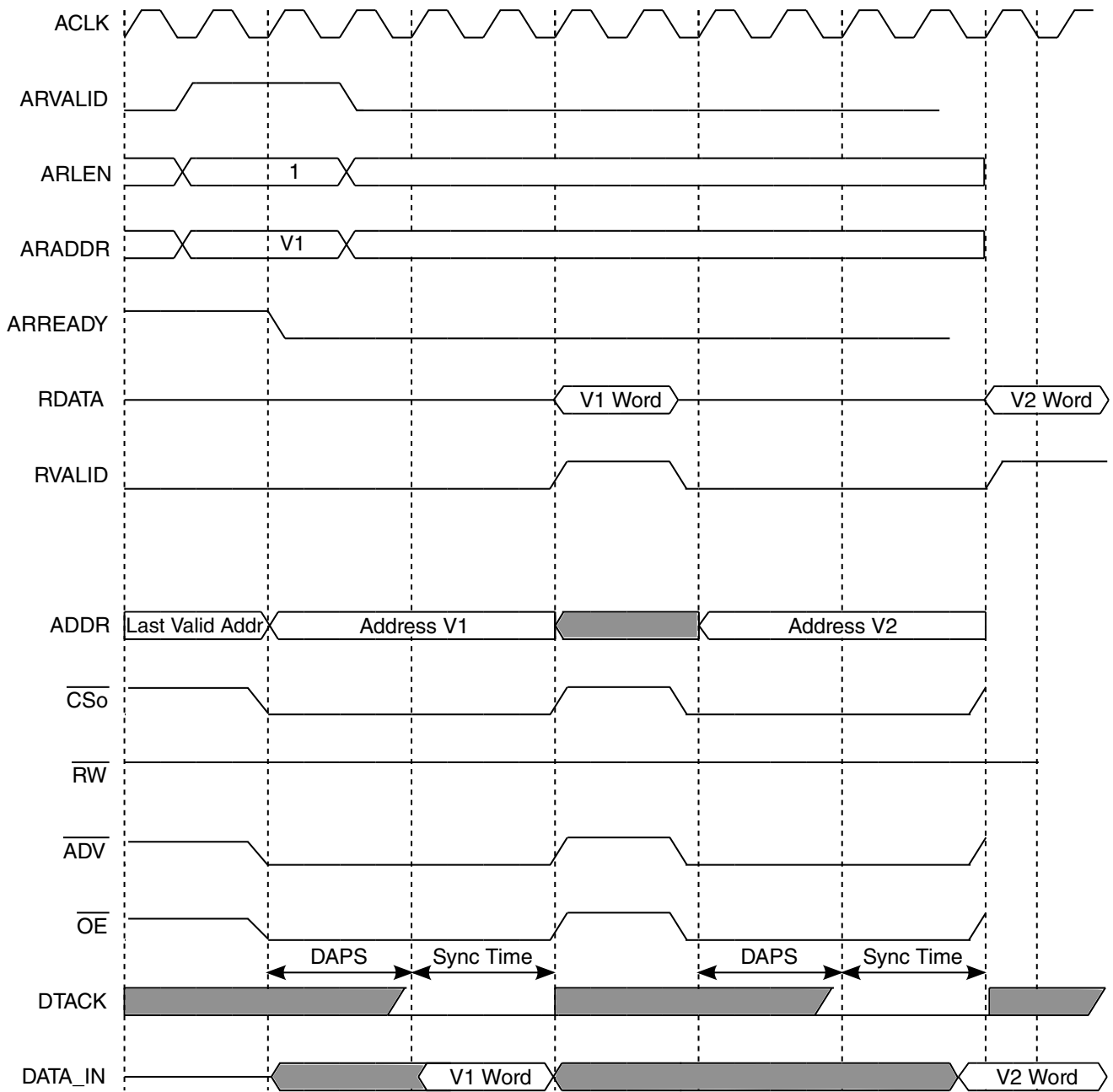
Figure 21-19. DAPS = 2 CSREC = 2
