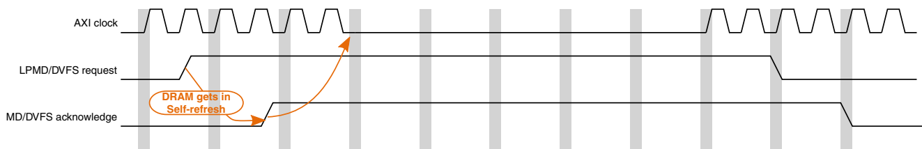
Figure 35-4. LPMD/DVFS Hardware/Software Handshaking
