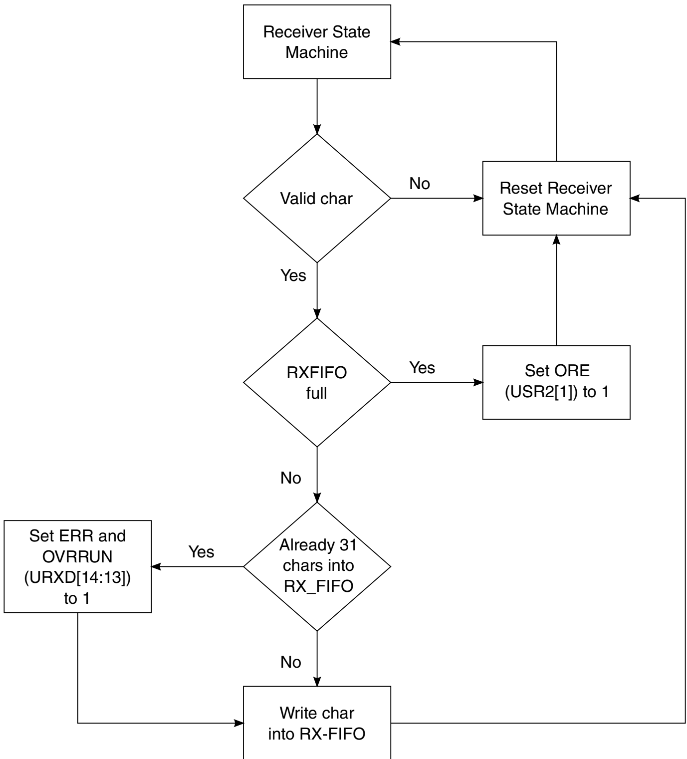
Figure 55-5. Receiver Flow Chart
