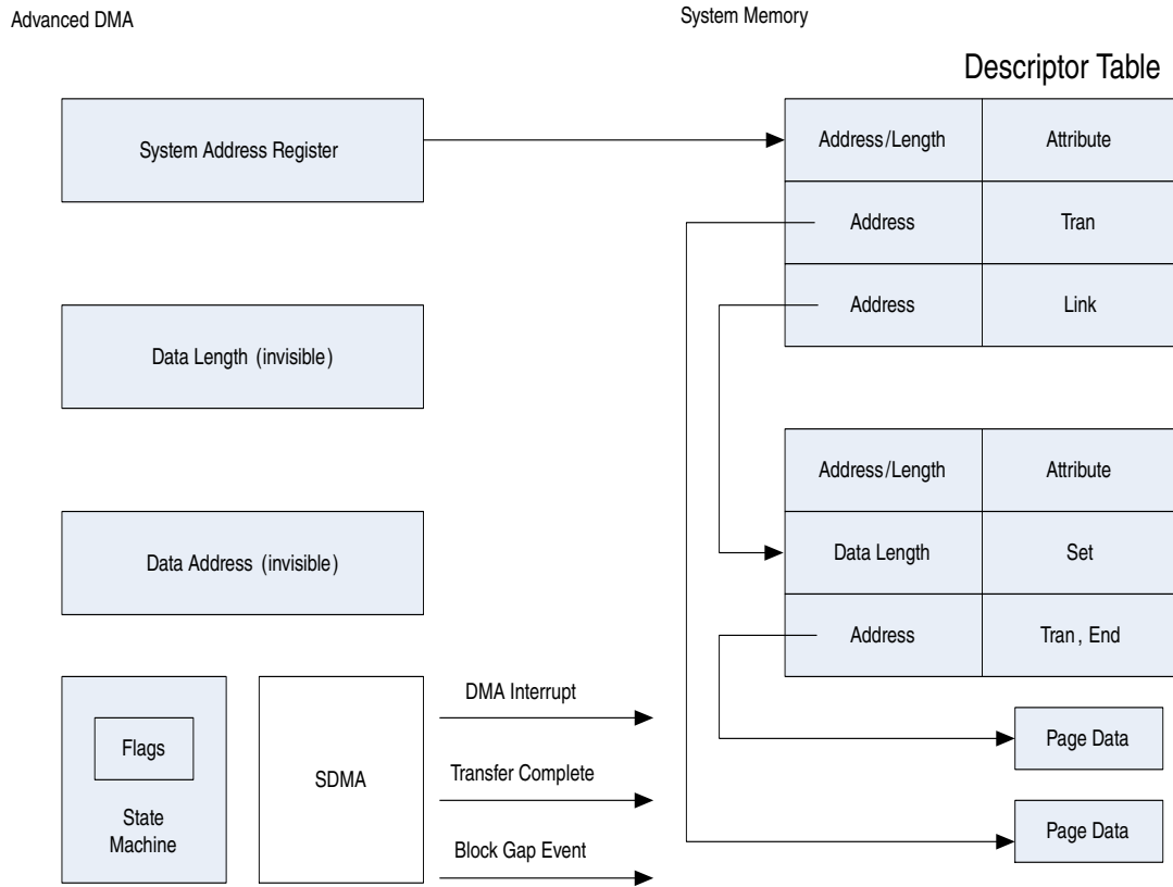
Figure 58-9. Concept and Access Method of ADMA1 Descriptor Table
