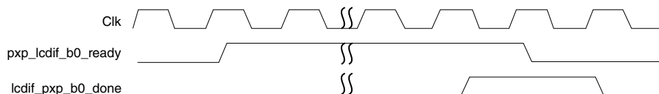
Figure 41-18. Buffer Sharing Protocol
