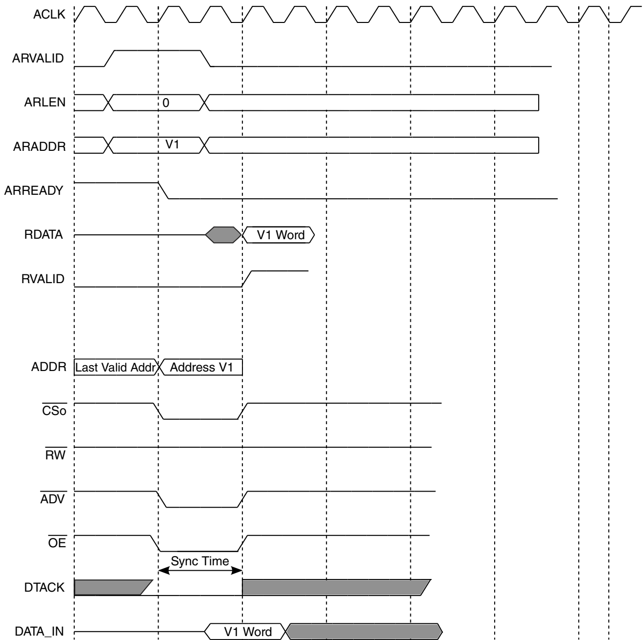
Figure 21-17. DAPS = 0
