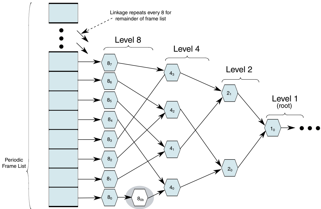
Figure 56-21. General Structure of EHCI Periodic Schedule Utilizing Interrupt Spreading
