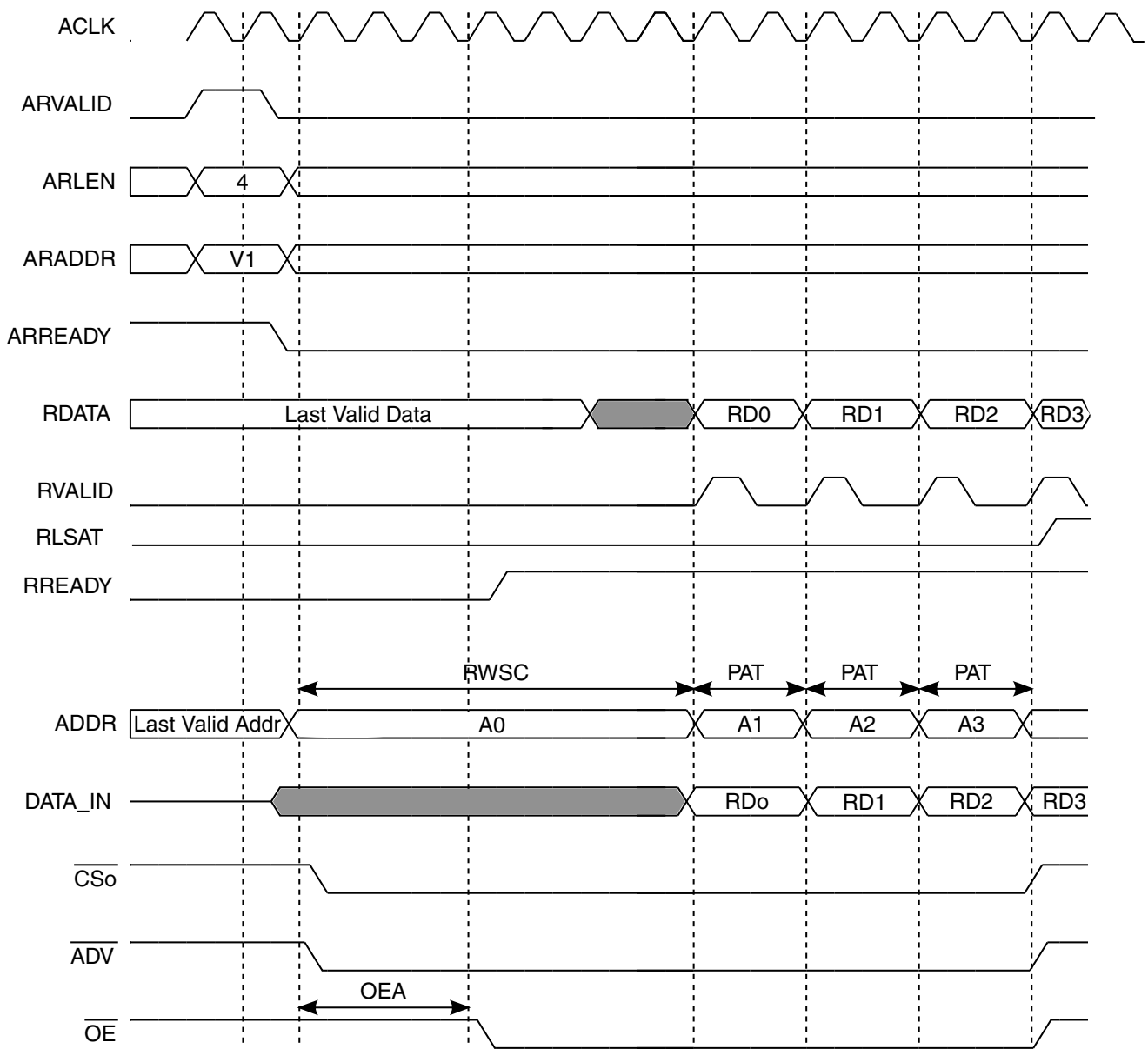
Figure 21-14. PAT = 2
