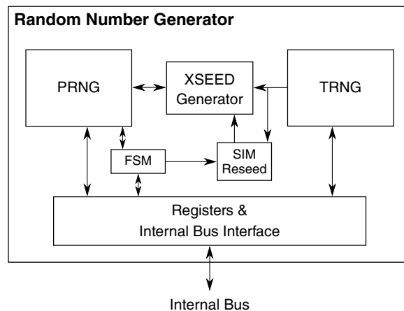
Figure 44-1. RNG block diagram
