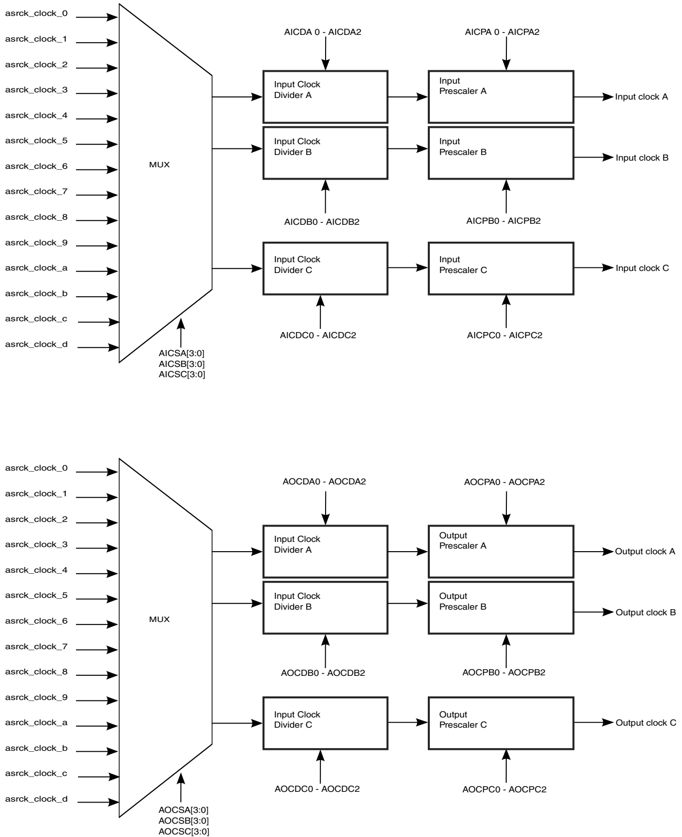
Figure 16-4. Clock Source Selector and Divider
