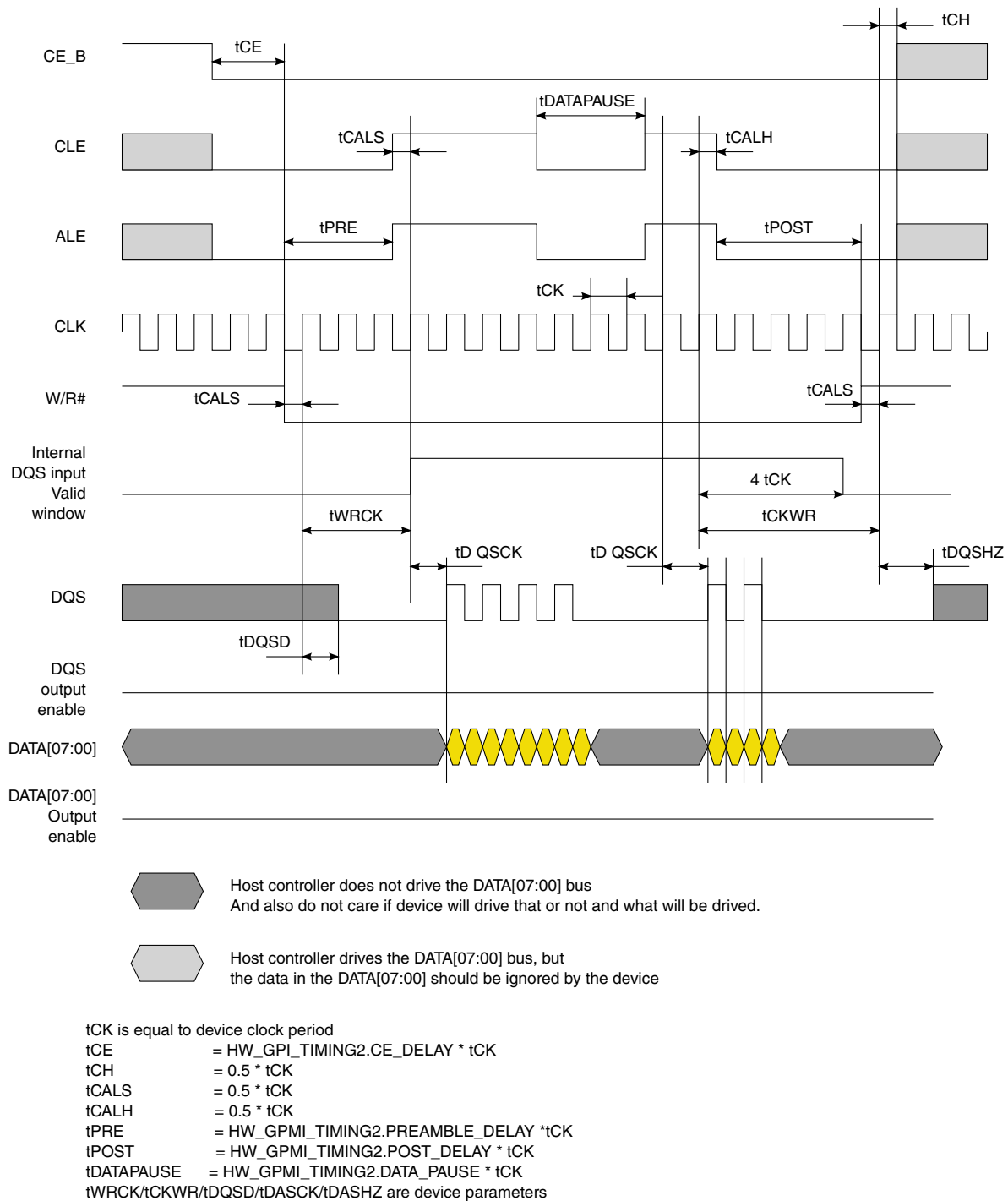
Figure 29-9. ONFI Source Synchronous Mode Data Read Timing Diagram
