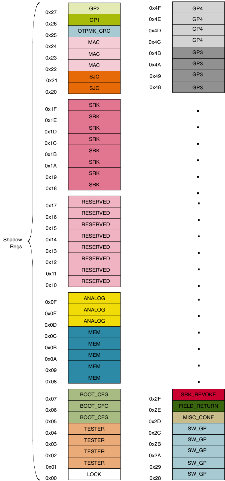
Figure 37-2. OTP Memory Footprint
