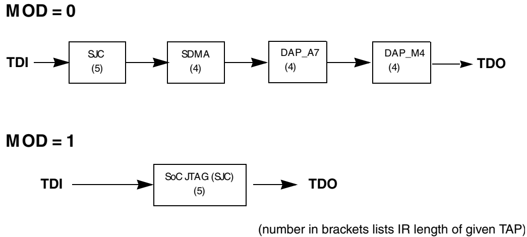
Figure 47-2. SJC Mode Selection Using MOD Pin Sampling
