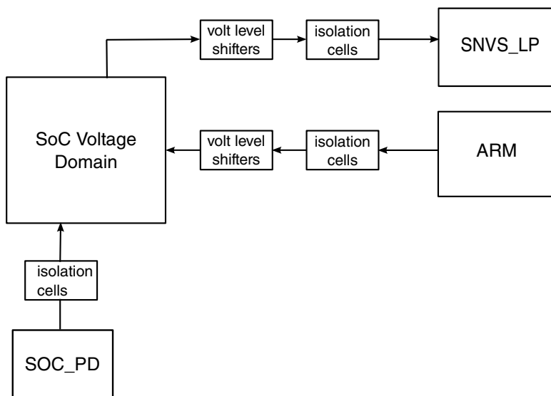
Note: The arrows refer to the signal directions for the voltage level shifters and isolation cells
