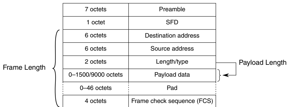
Figure 22-2. MAC frame format overview
