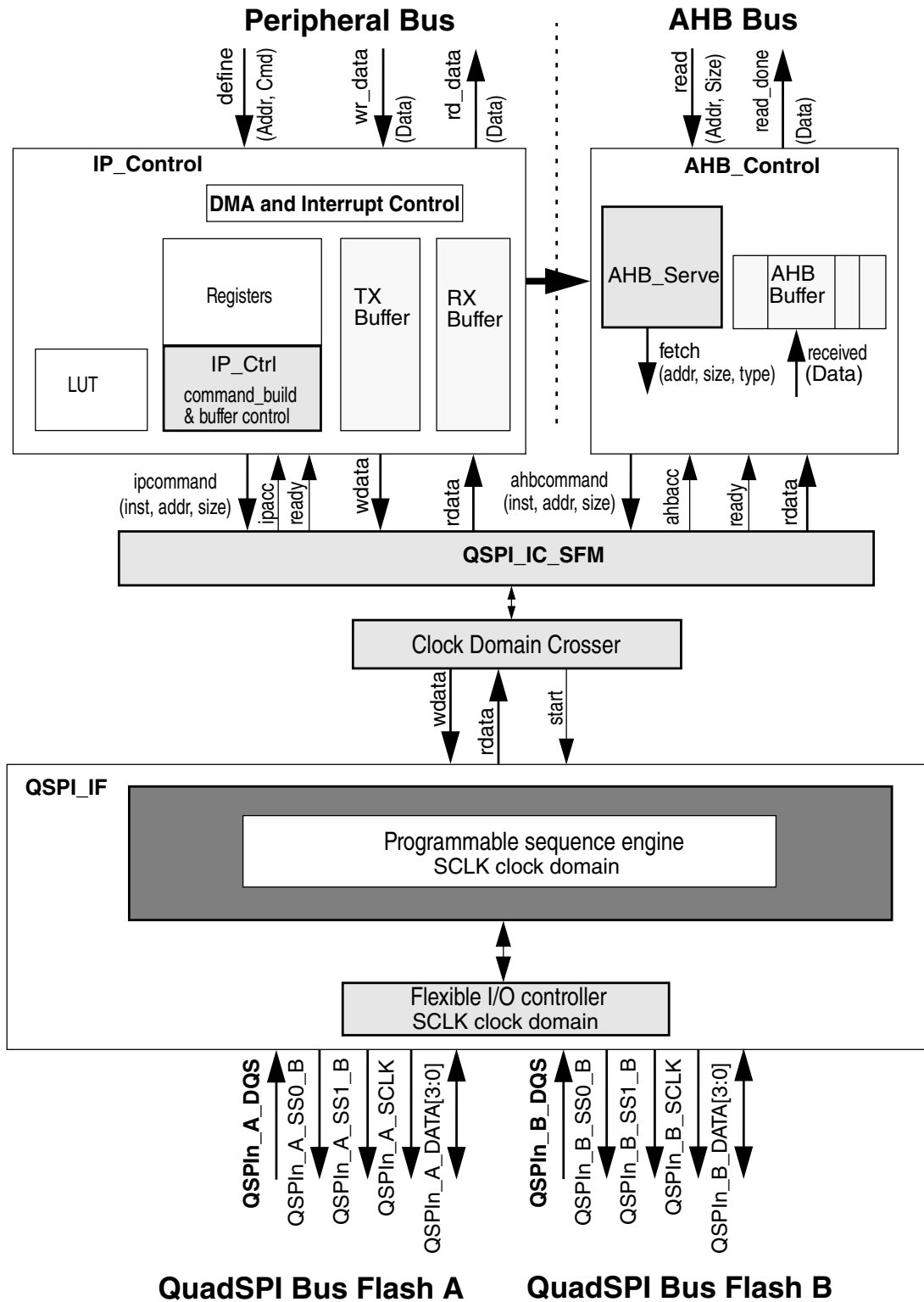
Figure 42-1. QuadSPI Block Diagram
