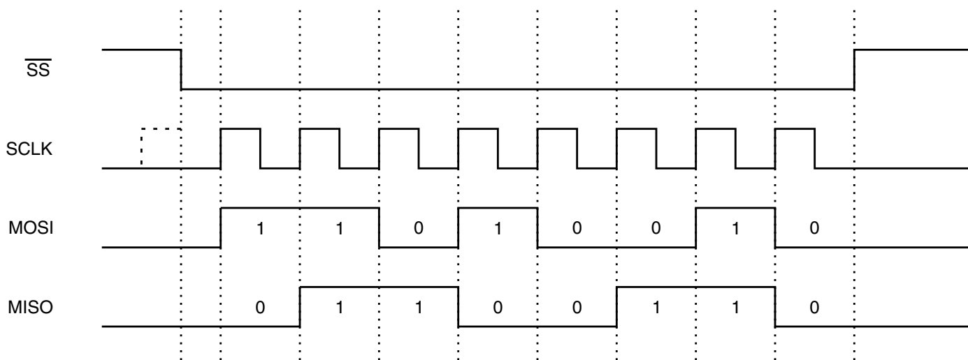
Figure 20-4. Typical SPI Burst (8-bit Transfer)
