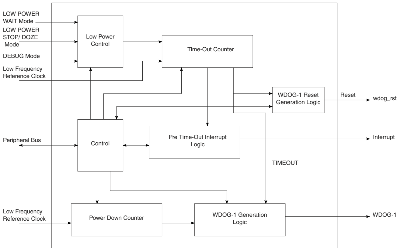
Figure 59-1. WDOG Diagram
