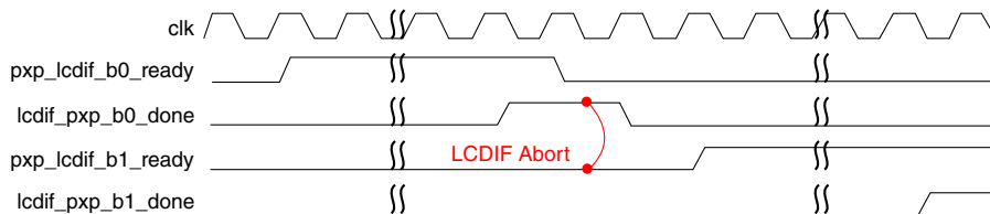
Figure 41-19. LCDIF Abort
