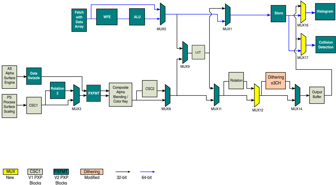
Figure 41-1. PXP Architecture
