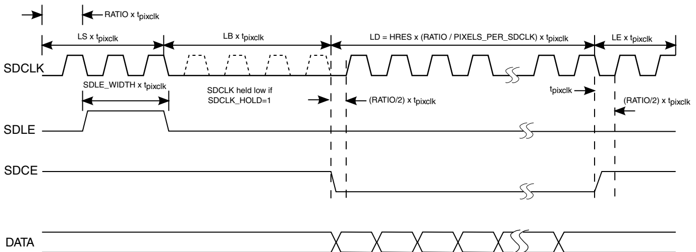
Figure 23-3. Line Timing ( DDR\_MODE = 0 )
