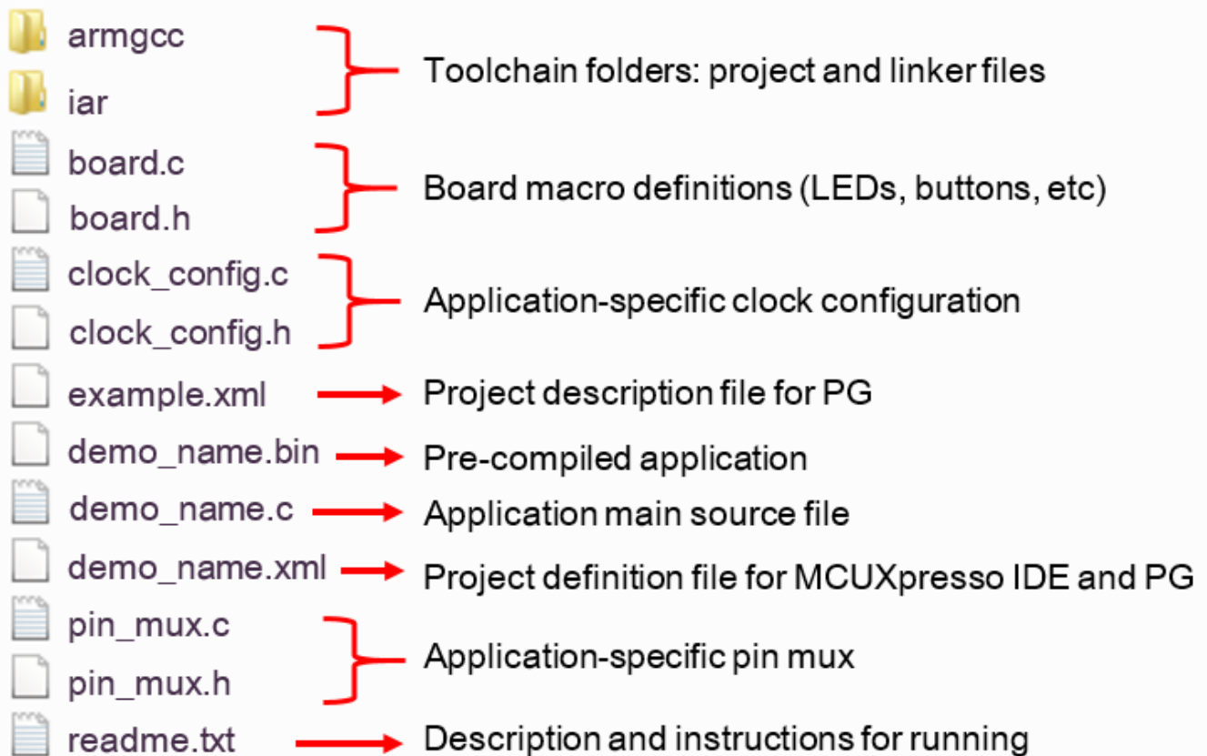
Figure 2. Application folder structure
