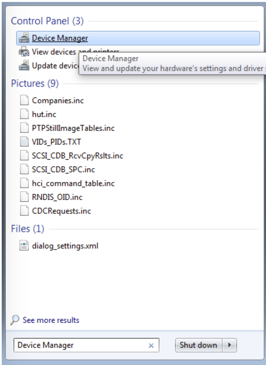
Figure 30. Device manager
