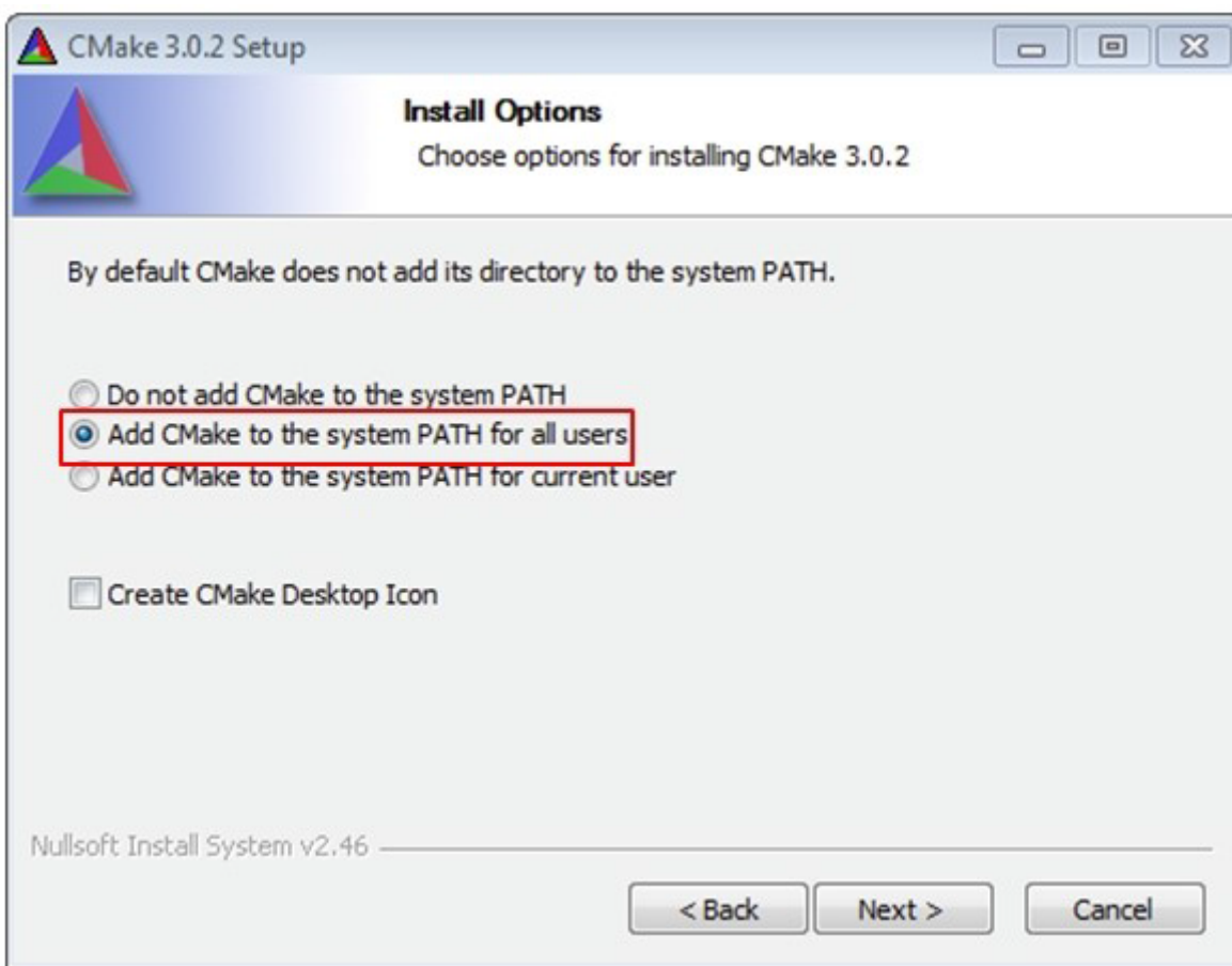
Figure 34. Install Cmake
