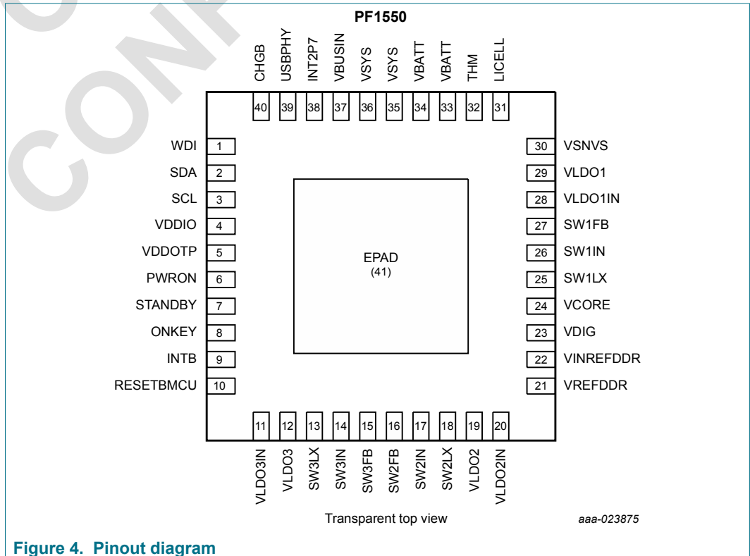
Figure 4. Pinout diagram
