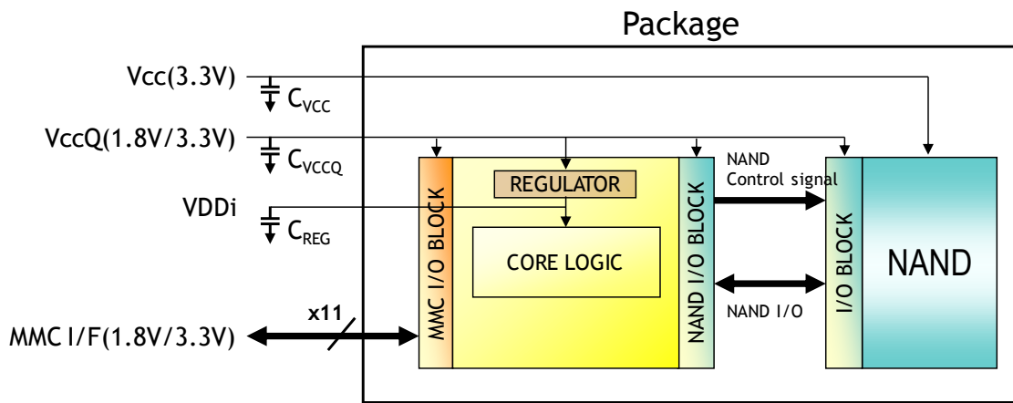
Figure 1 THGBMFG6C1LBAIL Block Diagram
