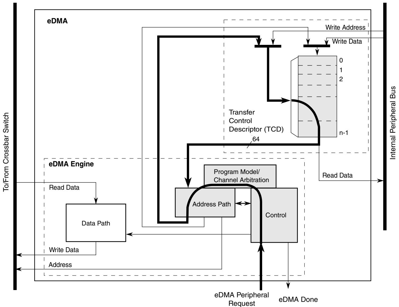
Figure 18-2. eDMA operation, part 1
