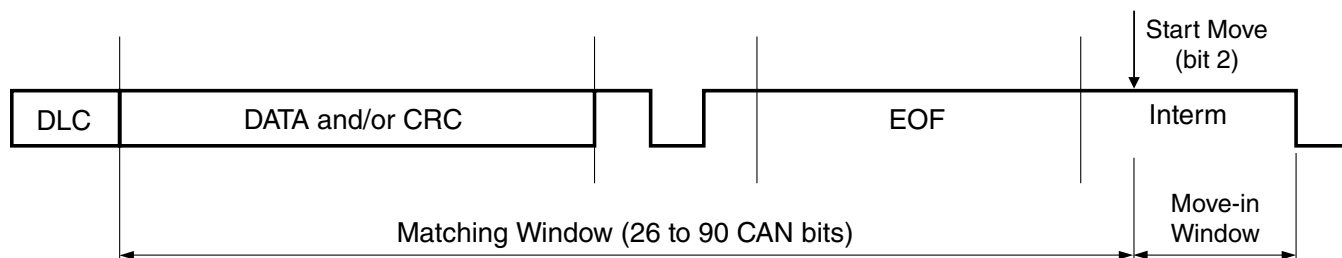
Figure 55-9. Matching and move-in time windows
