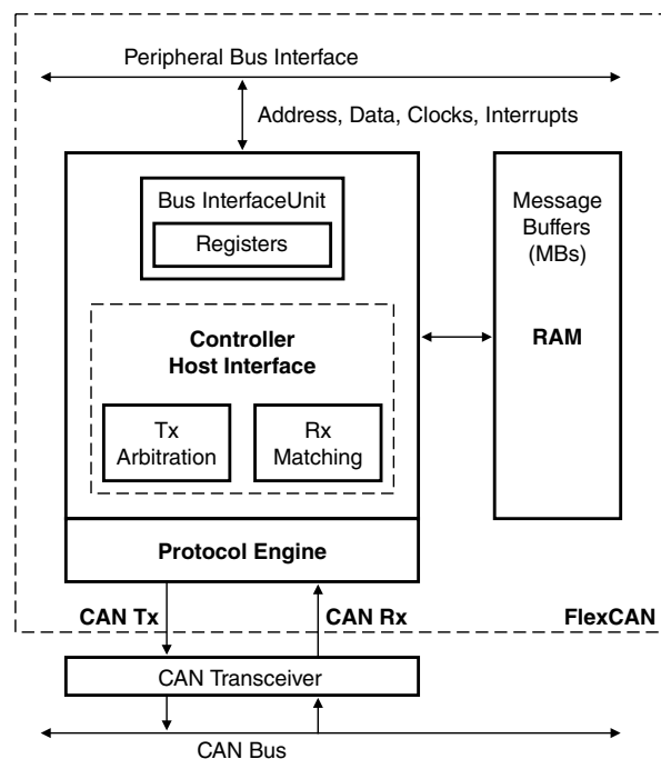
Figure 55-1. FlexCAN block diagram
