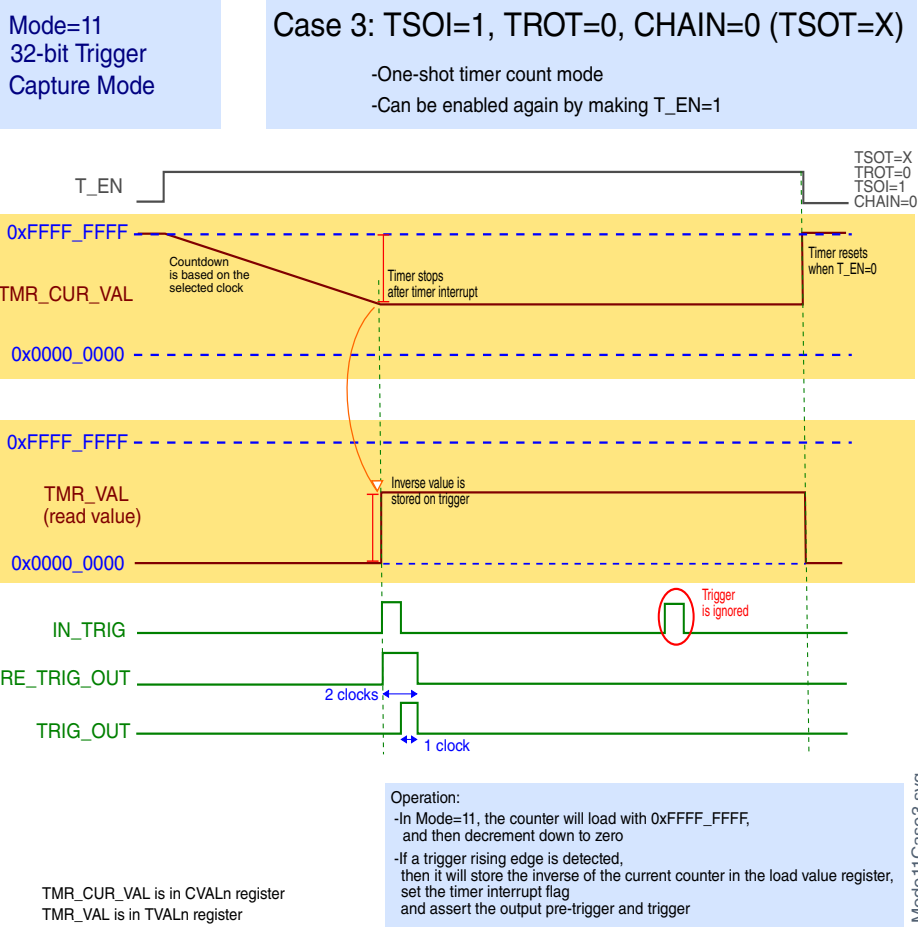
Figure 48-18. Case 3: TSOT = X, TROT = 0, TSOI = 1, CHAIN = 0
