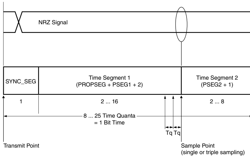
Figure 55-7. Segments within the bit time (example using CTRL1 bit timing variables for Classical CAN format)
