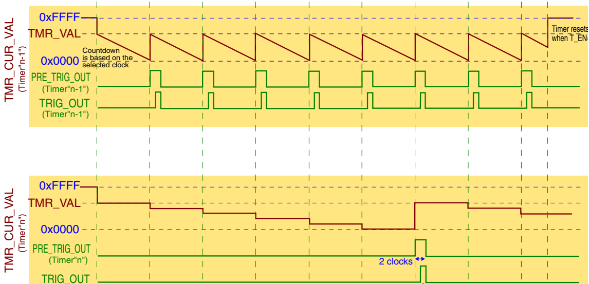
Figure 48-19. Chaining Effects
