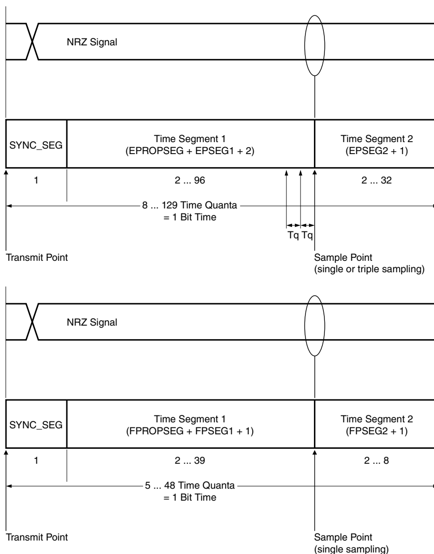
Figure 55-8. Segments within the bit time (example using CBT and FDCBT bit timing variables for CAN FD format)
