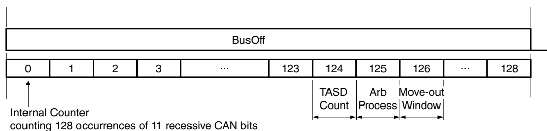
Figure 55-11. Arbitration at the end of bus off and move-out time windows
