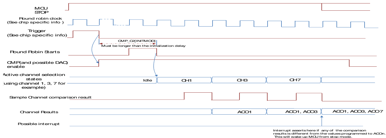
Figure 45-16. Trigger mode
