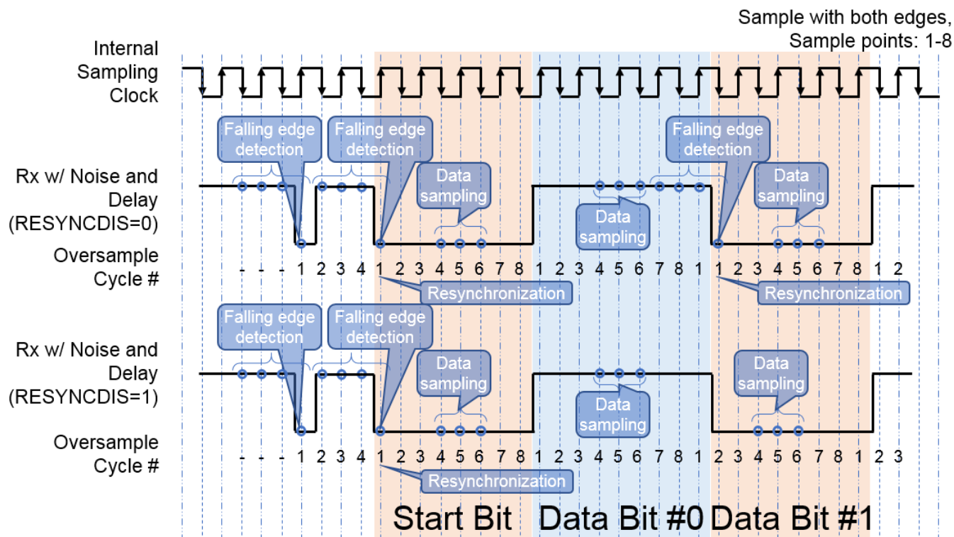
Figure 53-5. LPUART resynchronization
