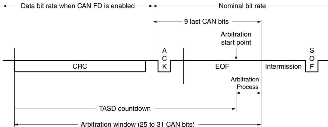
Figure 55-12. Optimal Tx Arbitration start point
