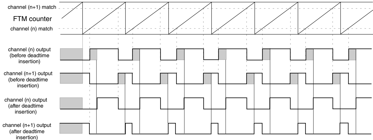
Figure 47-75. Deadtime insertion with ELSB:ELSA = 1:0, POL(n) = 0, and POL(n+1) = 0
