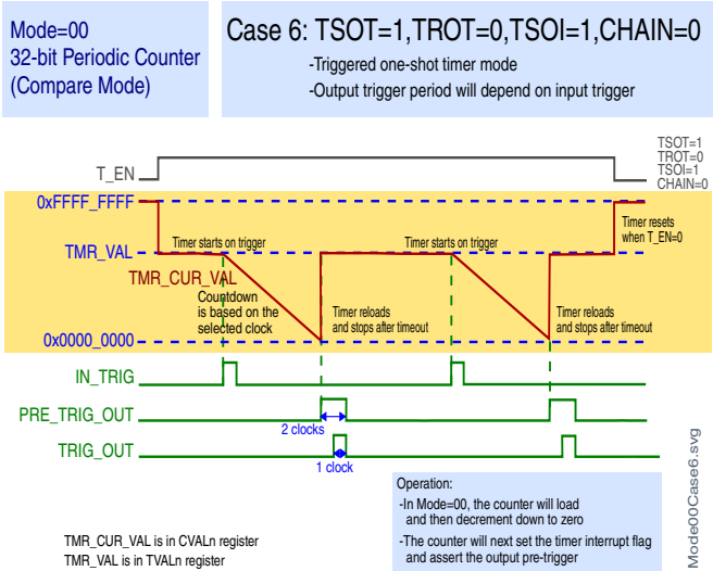
Figure 48-10. Case 6: TSOT = 1, TROT = 0, TSOI = 1, CHAIN = 0
