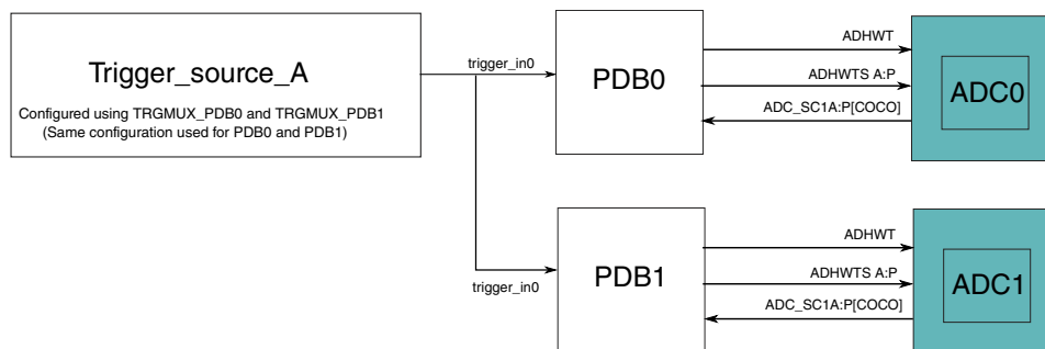
Figure 43-4. ADC triggering with same source
