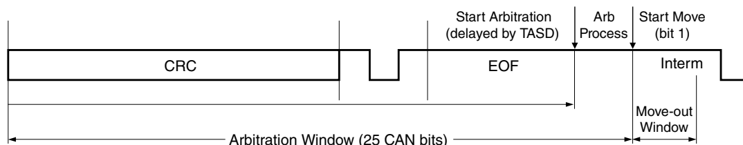
Figure 55-10. Arbitration and move-out time windows
