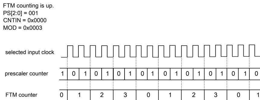
Figure 47-7. Example of the prescaler counter
