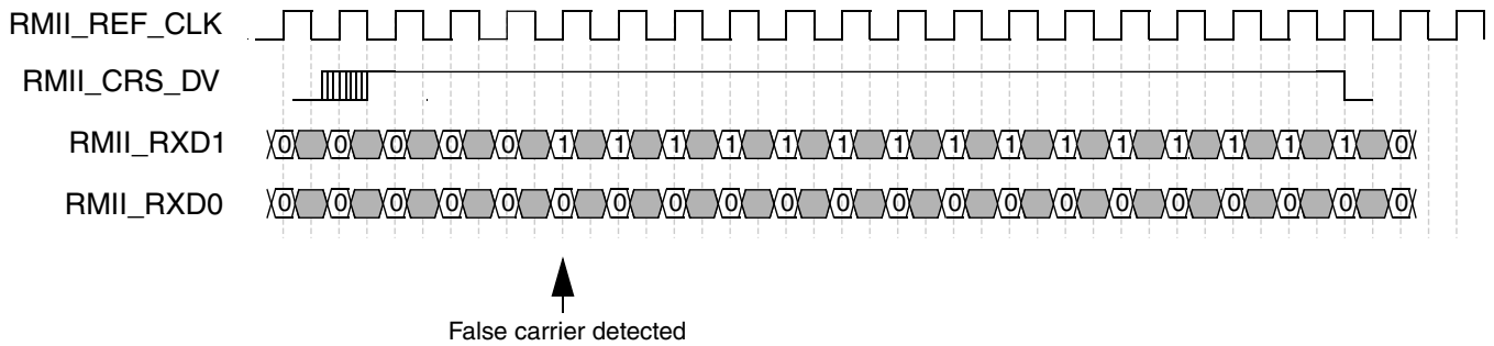
Figure 57-20. RMIi receive operation with false carrier
