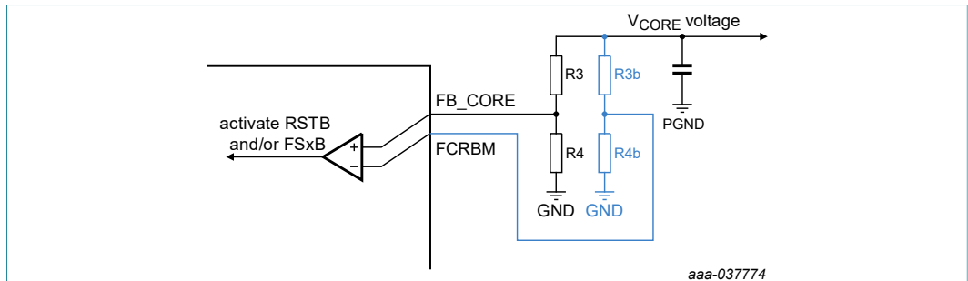
Figure 45. Feedback core resistor bridge monitoring (FCRBM)
