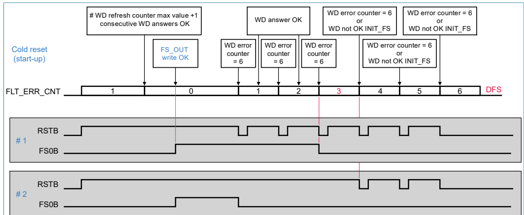
Figure 25. Example of RSTB and FS0B behavior when FLT_ERR_CNT ≥ intermediate value
