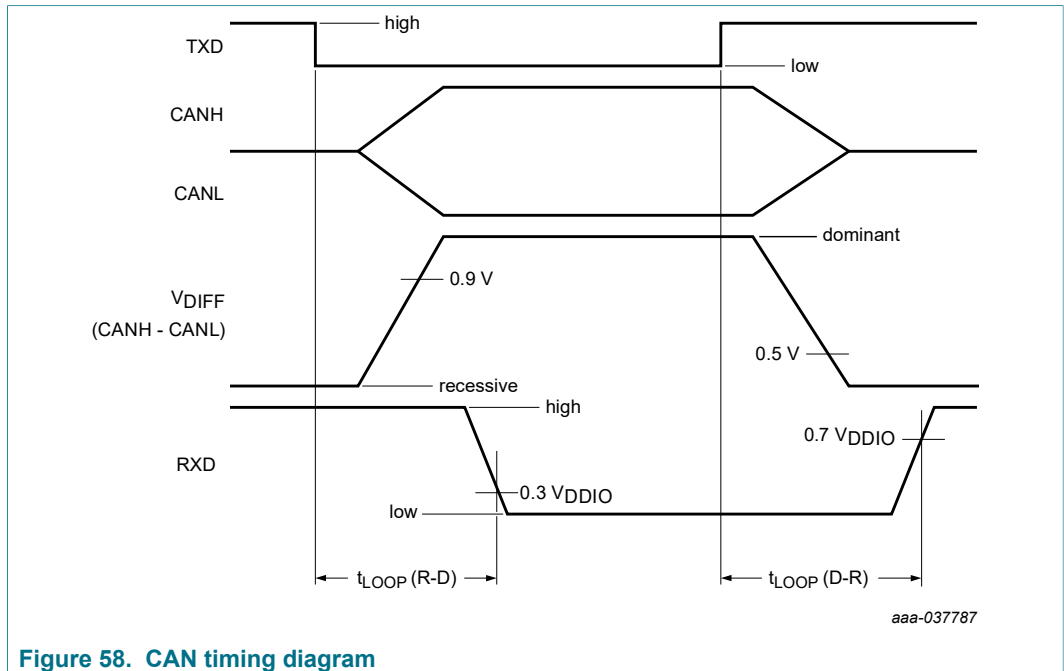
Figure 58. CAN timing diagram
