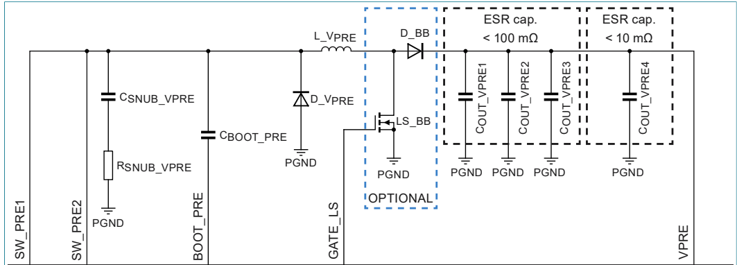
Figure 34. Pre-regulator: buck boost configuration
