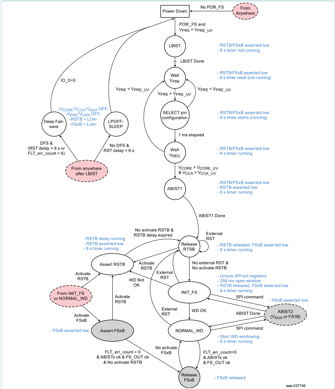
Figure 17. Detailed fail-safe state diagram
