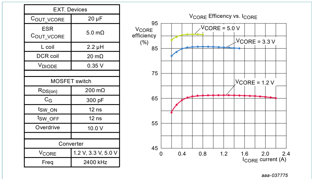
Figure 46. V CORE efficiency
