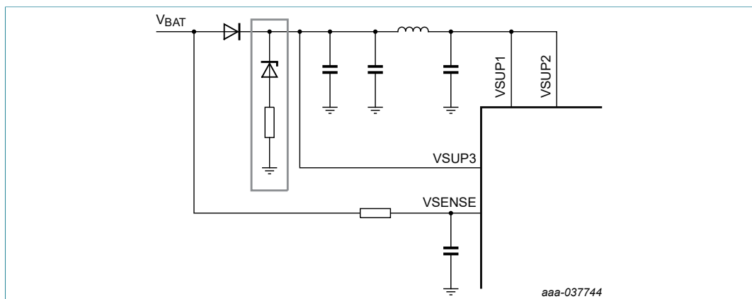
Figure 15. Components involved under ISO pulse in LPOFF
