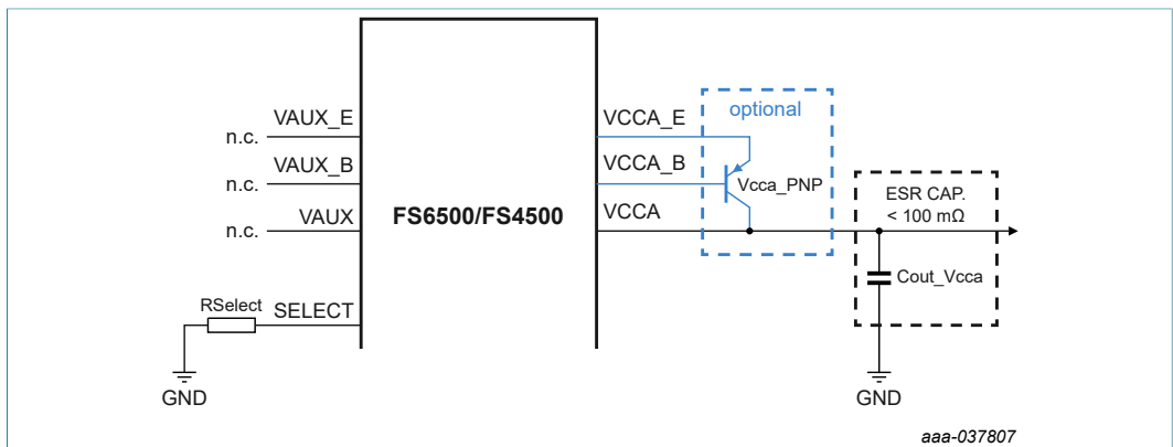
Figure 78. V_{CCA} connection, V_{AUX} not used, deep fail-safe enabled
