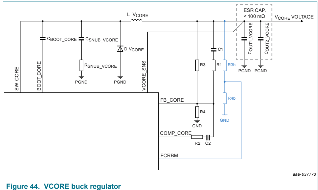
Figure 44. VCORE buck regulator
