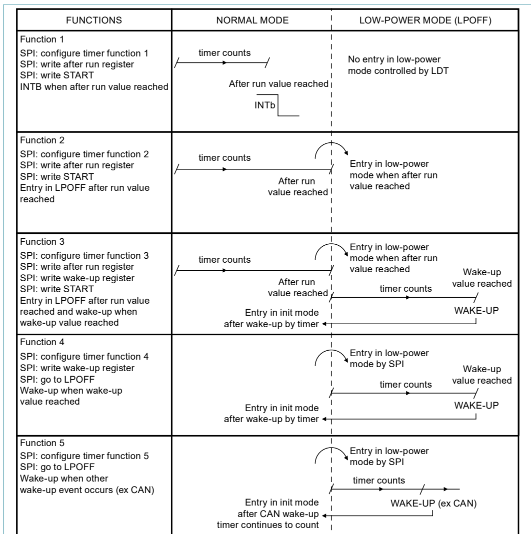
Figure 55. Long duration timer functions
