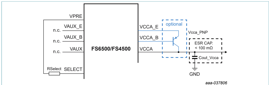
Figure 77. V_{CCA} connection, V_{AUX} not used, deep fail-safe disabled
