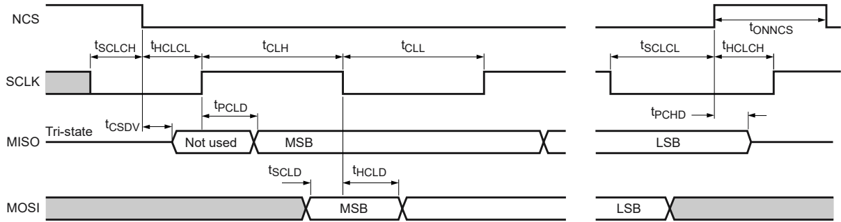
Figure 9. SPI timing diagram
