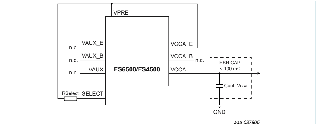
Figure 76. V_{AUX} not used, V_{CCA} configuration up to 100 mA, deep fail-safe disabled
