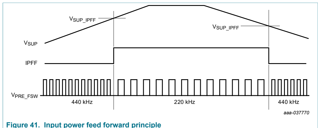
Figure 41. Input power feed forward principle
