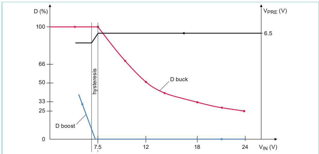
Figure 35. Transition between buck and boost
