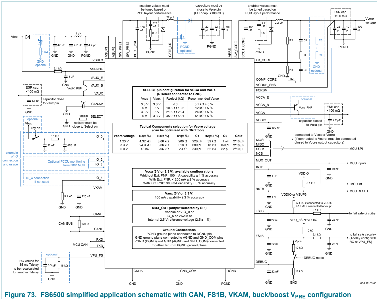
Figure 73. FS6500 simplified application schematic with CAN, FS1B, VKAM, buck/boost VPRE configuration
