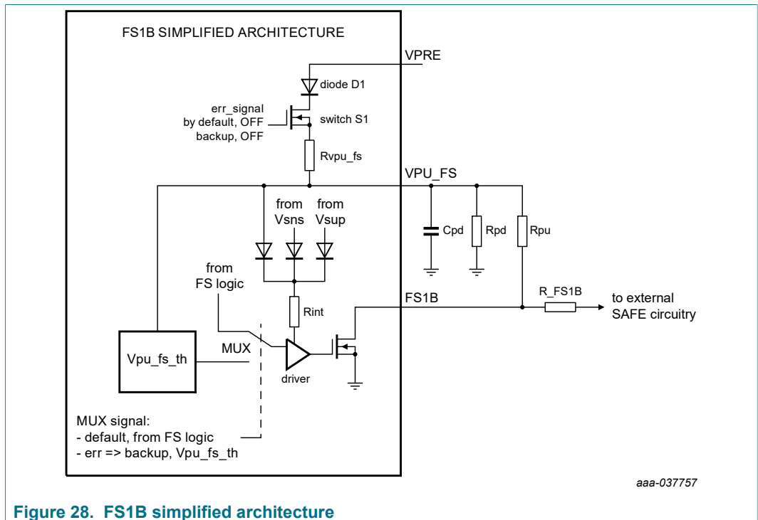
Figure 28. FS1B simplified architecture
