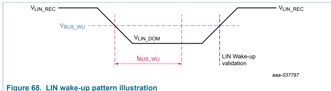
Figure 68. LIN wake-up pattern illustration
