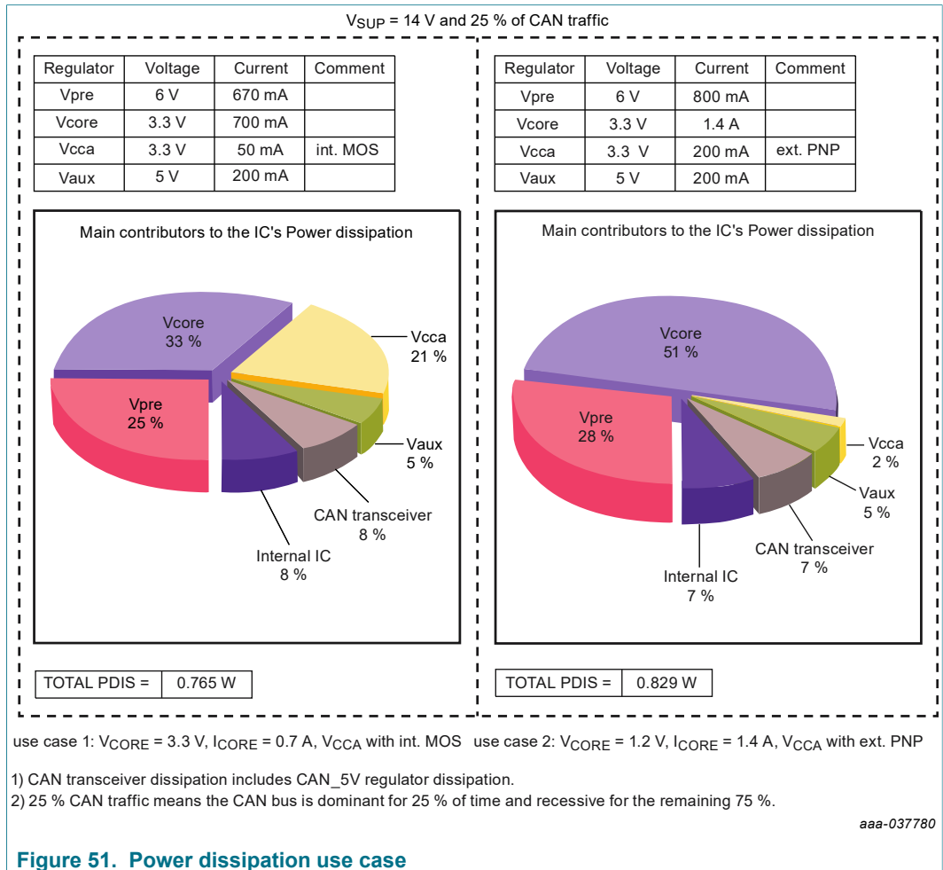
Figure 51. Power dissipation use case
