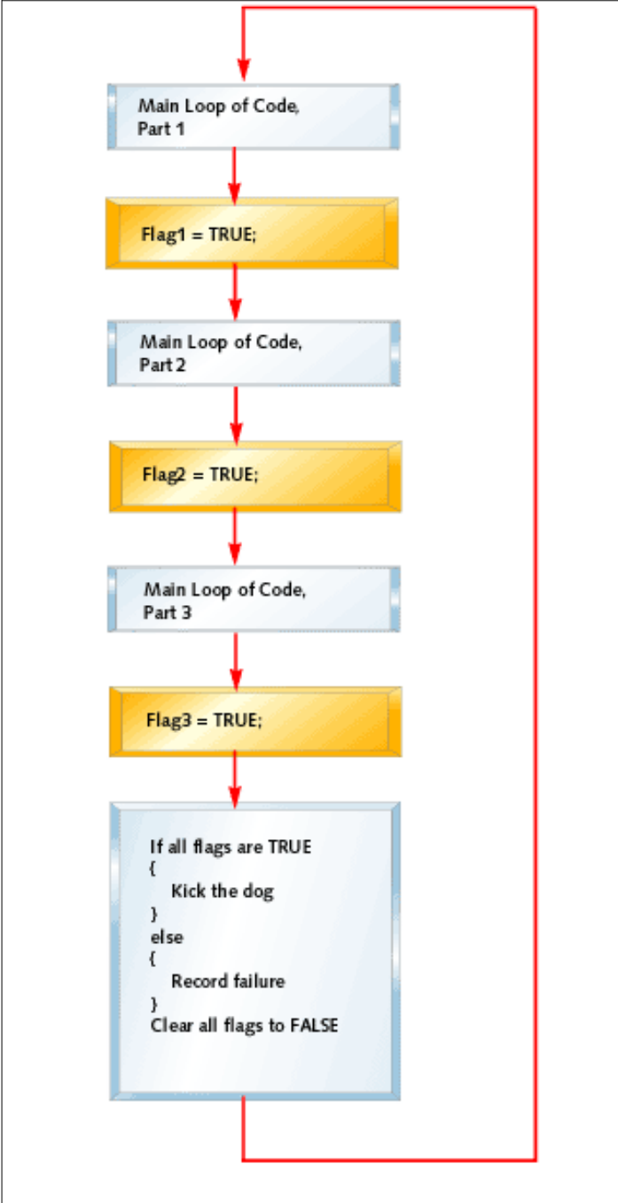
Figure 2: Use three flags to check that certain points within the main loop have been visited
