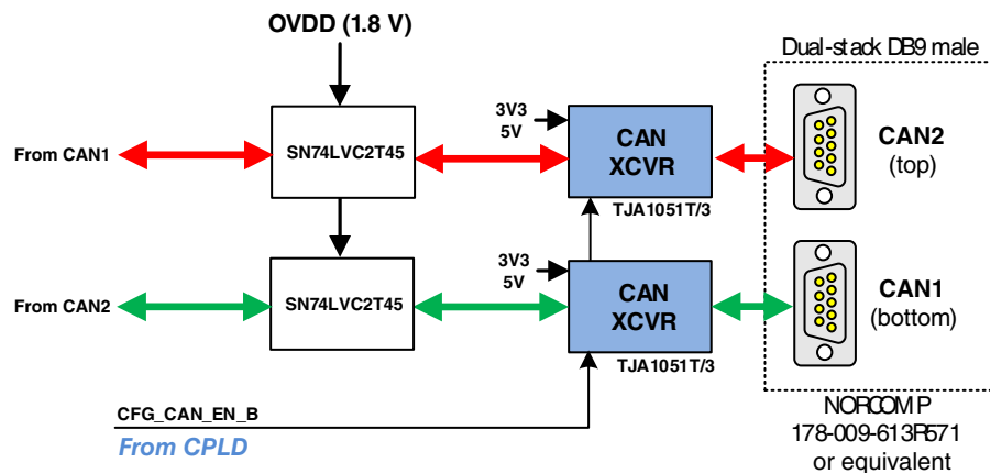
Figure 2-22. CAN architecture
