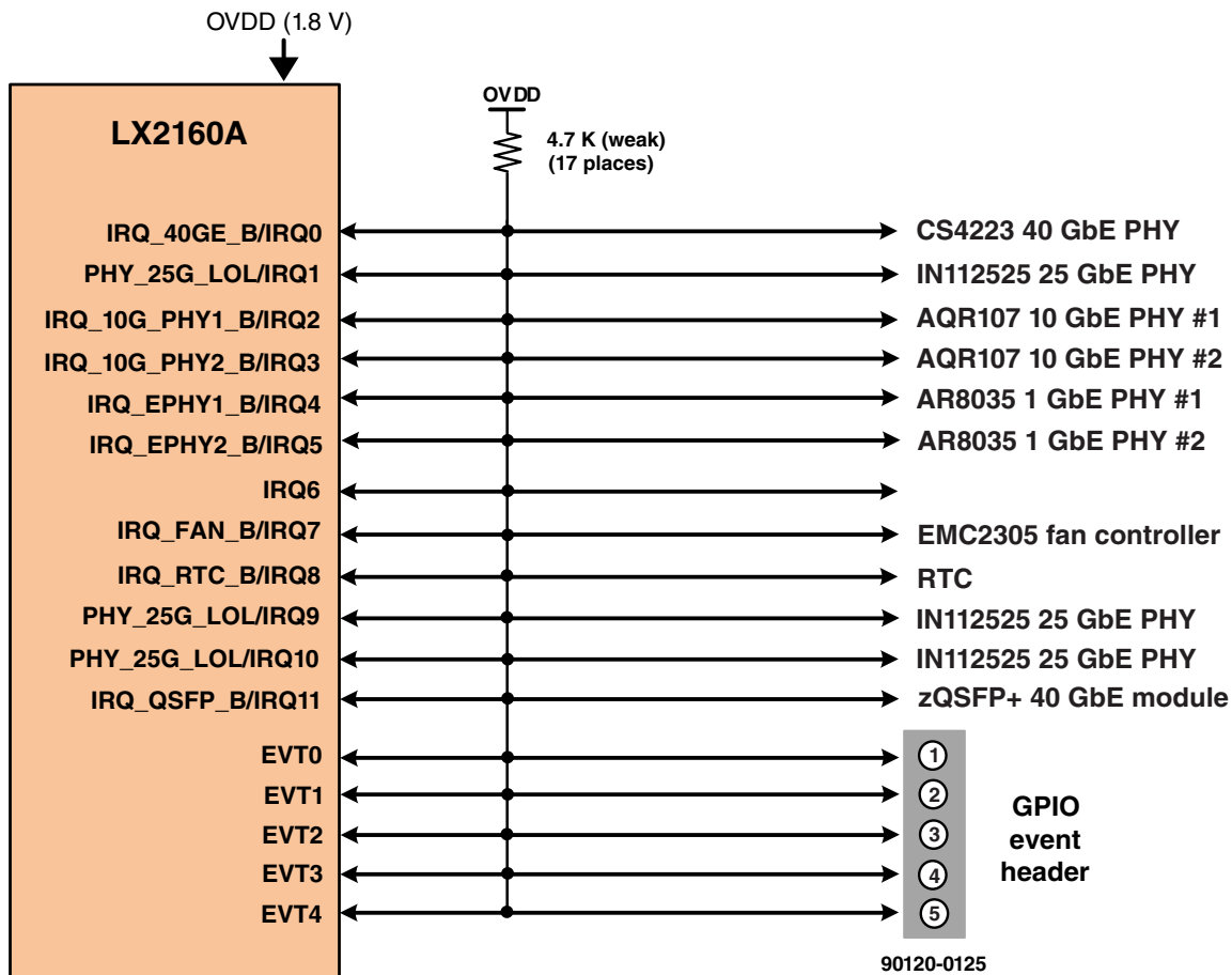
Figure 2-25. GPIO interface
