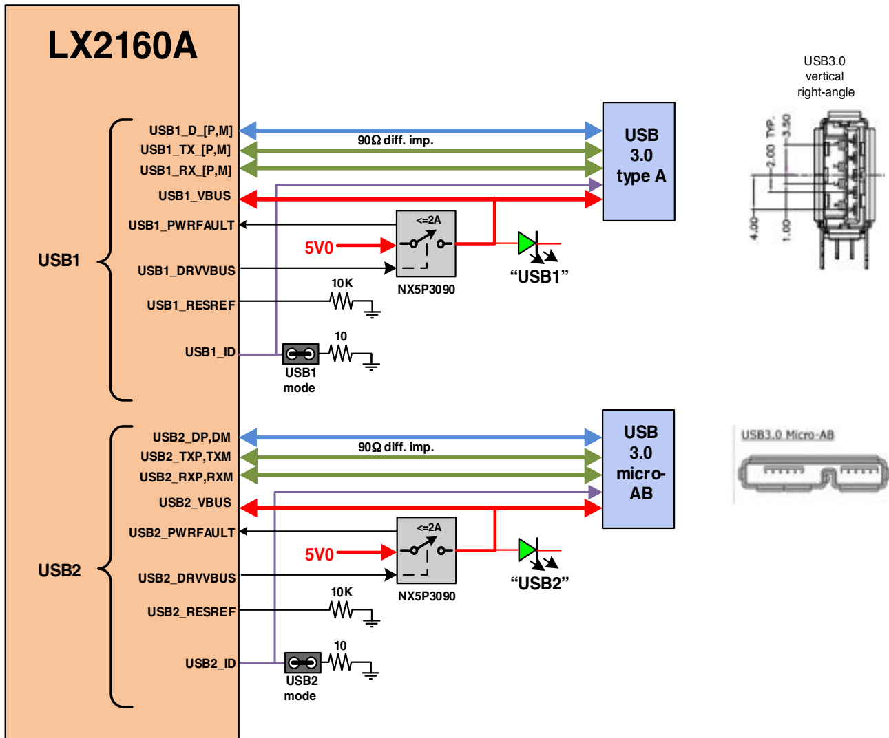
Figure 2-17. USB architecture
