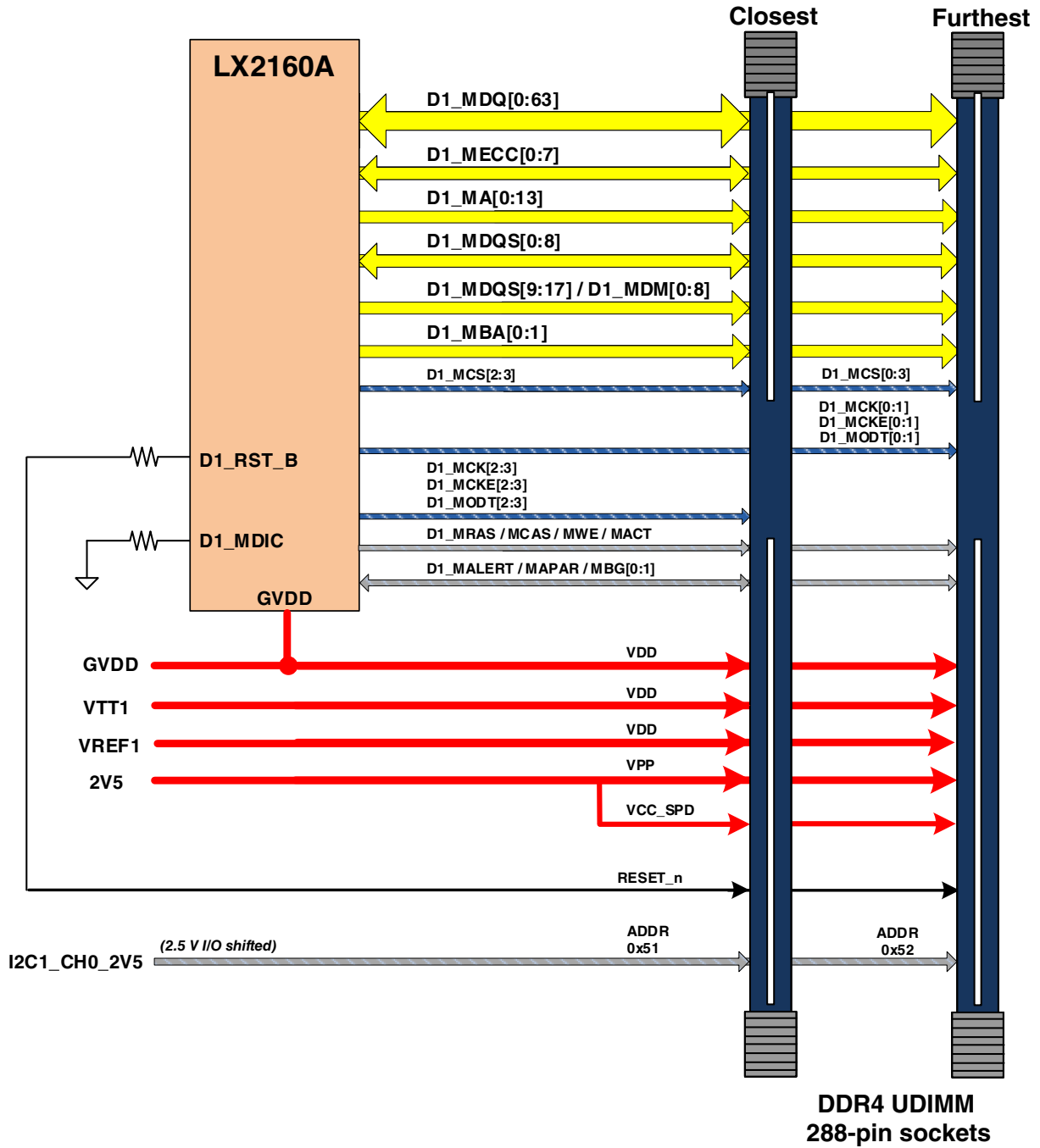
Figure 2-7. DDR#1 memory port architecture
