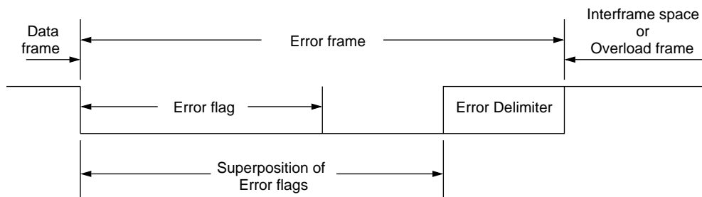
Figure 10-8 Error frame
