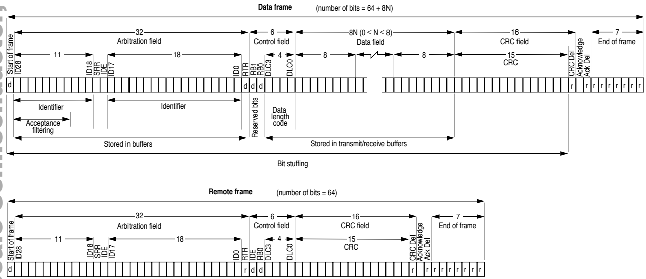
Figure 10-13 CAN frame format - Extended Format
