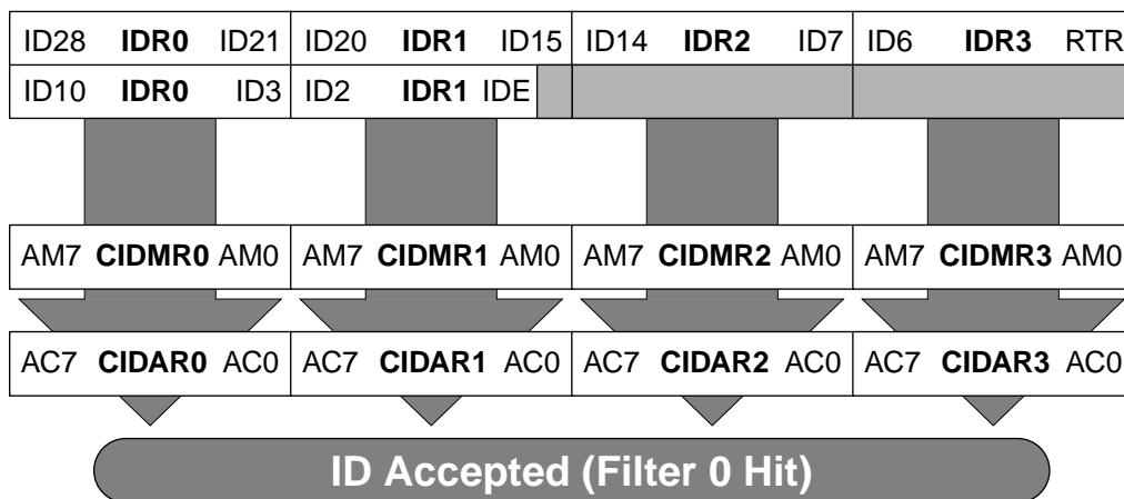
Figure C-3 Single 32 bit Maskable Identifier Acceptance Filter
