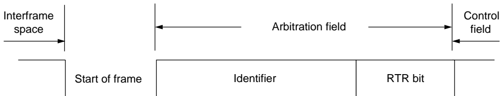
Figure 3-2 Arbitration field
