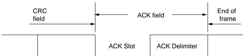
Figure 3-5 ACK field
