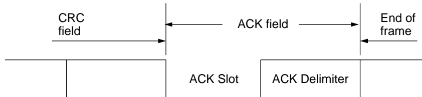
Figure 10-6 ACK field
