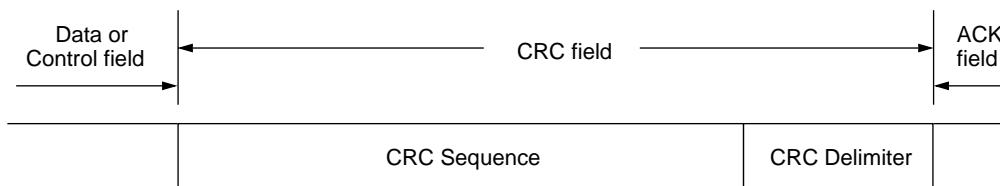
Figure 10-5 CRC field
