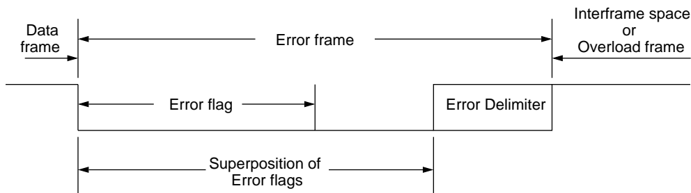
Figure 3-7 Error frame
