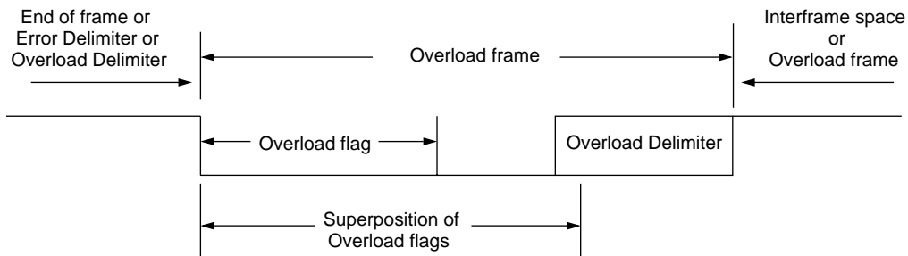
Figure 10-9 Overload frame
